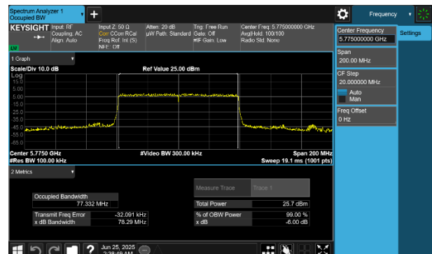
Plot 7-57 6dB BW & 99% OBW Antenna WF7 (80MHz BW 802.11be(RU) RU996 Index67 - Ch.155)
