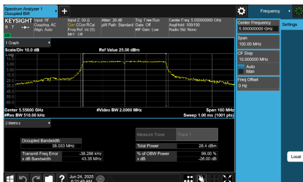
Plot 7-20 26dB BW & 99% OBW Antenna WF8 (40MHz BW 802.11be(RU) RU484 Index65 - Ch.110)
