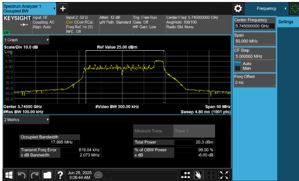
Plot 7-50 6dB BW & 99% OBW Antenna WF7 (20MHz BW 802.11be(RU) RU26 Index8 - Ch.149)
