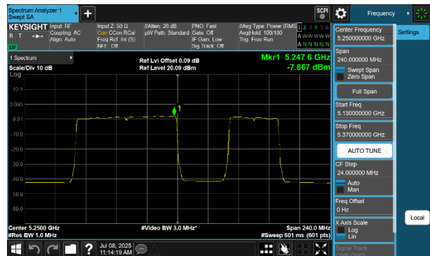
Plot 7-64 PSD Antenna WF5B (160MHz BW 802.11be(RU) RU996+484 Index94 - Ch.50)
