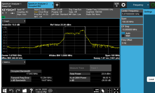
Plot 7-13 26dB BW & 99% OBW Antenna WF8 (40MHz BW 802.11be(RU) RU52 Index44 - Ch.134)
