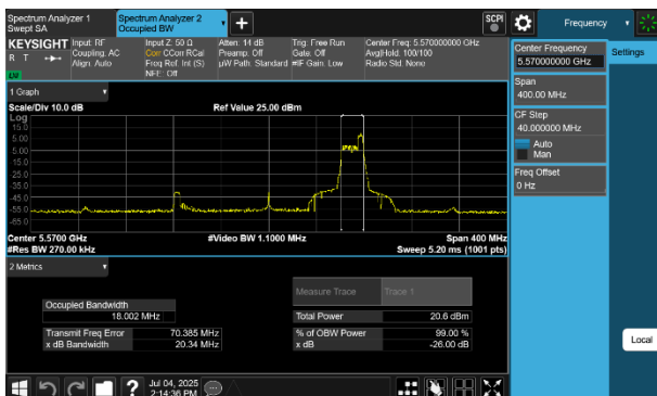
Plot 7-15 26dB BW & 99% OBW Antenna WF8 (160MHz BW 802.11be(RU) RU52 Index52 - Ch.114)
