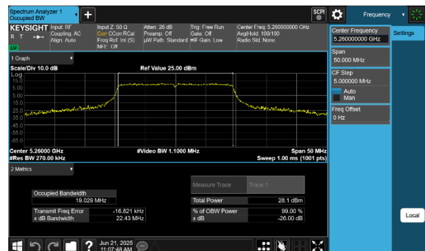
Plot 7-8 26dB BW & 99% OBW Antenna WF5B (20MHz BW 802.11be(RU) RU242 Index61 - Ch.52)
