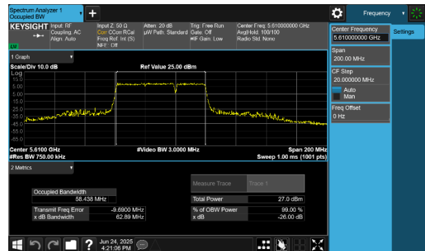
Plot 7-17 26dB BW & 99% OBW Antenna WF8 (80MHz BW 802.11be(RU) RU484+242 Index93 - Ch.122)
