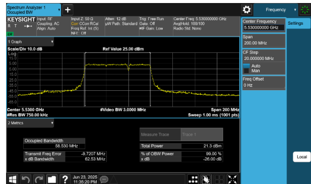
Plot 7-6 26dB BW & 99% OBW Antenna WF5B (80MHz BW 802.11be(RU) RU484+242 Index93 - Ch.106)
