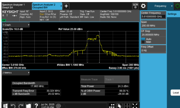
Plot 7-14 26dB BW & 99% OBW Antenna WF8 (80MHz BW 802.11be(RU) RU52 Index52 - Ch.122)
