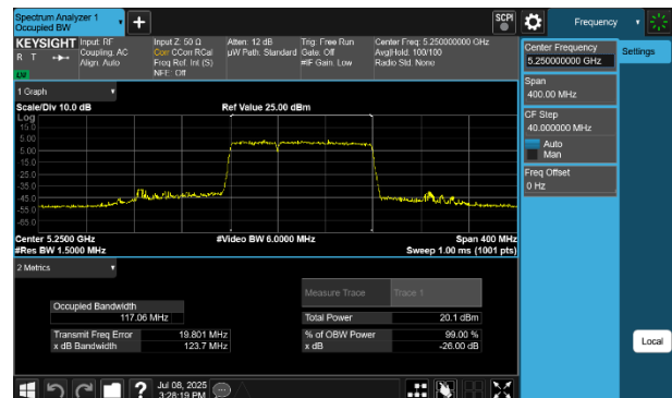
Plot 7-18 26dB BW & 99% OBW Antenna WF8 (160MHz BW 802.11be(RU) RU996+484 Index94 - Ch.50)
