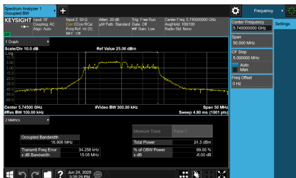
Plot 7-45 6dB BW & 99% OBW Antenna WF8 (20MHz BW 802.11be(RU) RU52+26 Index71 - Ch.149)
