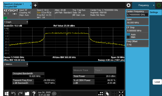
Plot 7-47 6dB BW & 99% OBW Antenna WF8 (20MHz BW 802.11be(RU) RU242 Index61 - Ch.149)
