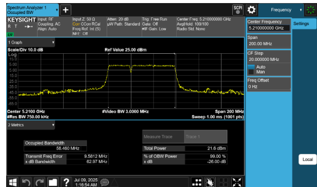
Plot 7-28 26dB BW & 99% OBW Antenna WF7 (80MHz BW 802.11be(RU) RU484+242 Index90 - Ch.42)
