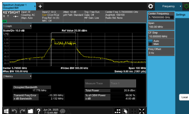
Plot 7-43 6dB BW & 99% OBW Antenna WF5B (40MHz BW 802.11be(RU) RU26 Index0 - Ch.159)
