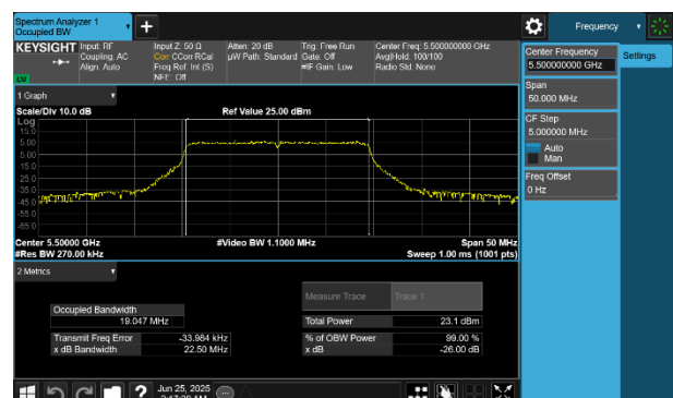
Plot 7-30 26dB BW & 99% OBW Antenna WF7 (20MHz BW 802.11be(RU) RU242 Index61 - Ch.100)
