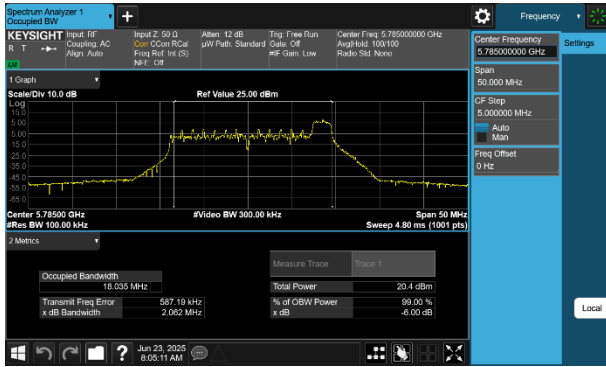
Plot 7-34 6dB BW & 99% OBW Antenna WF5B (20MHz BW 802.11be(RU) RU26 Index8 - Ch.157)
