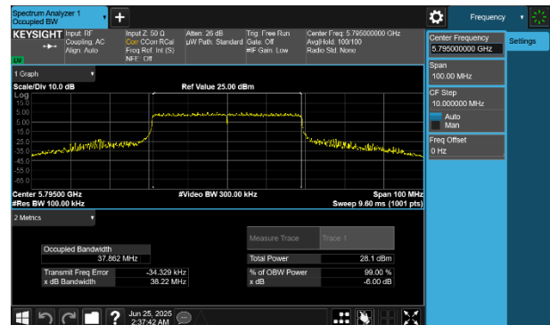
Plot 7-56 6dB BW & 99% OBW Antenna WF7 (40MHz BW 802.11be(RU) RU484 Index65 - Ch.159)
