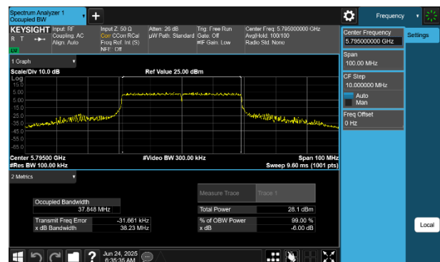
Plot 7-48 6dB BW & 99% OBW Antenna WF8 (40MHz BW 802.11be(RU) RU484 Index65 - Ch.159)
