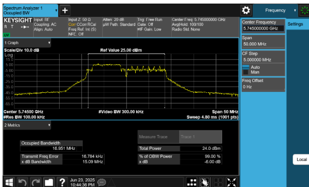
Plot 7-37 6dB BW & 99% OBW Antenna WF5B (20MHz BW 802.11be(RU) RU52+26 Index71 - Ch.149)
