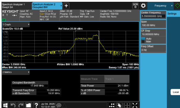
Plot 7-2 26dB BW & 99% OBW Antenna WF5B (40MHz BW 802.11be(RU) RU52 Index44 - Ch.110)
