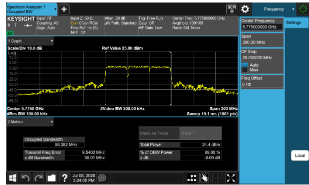
Plot 7-46 6dB BW & 99% OBW Antenna WF8 (80MHz BW 802.11be(RU) RU484+242 Index90 - Ch.155)
