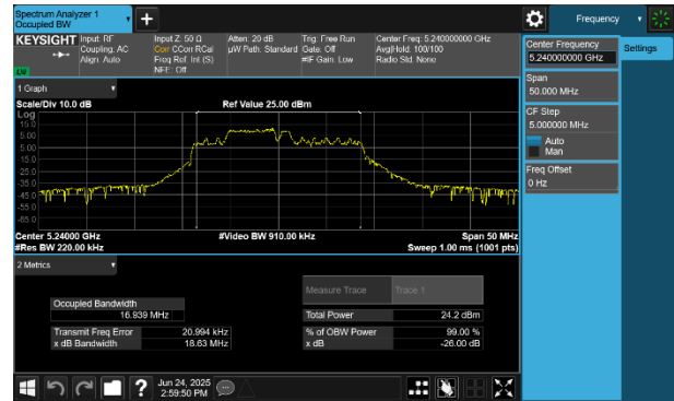
Plot 7-16 26dB BW & 99% OBW Antenna WF8 (20MHz BW 802.11be(RU) RU52+26 Index71 - Ch.48)
