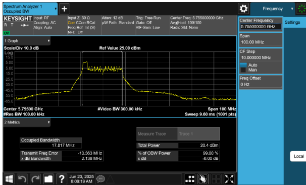
Plot 7-35 6dB BW & 99% OBW Antenna WF5B (40MHz BW 802.11be(RU) RU26 Index0 - Ch.151)
