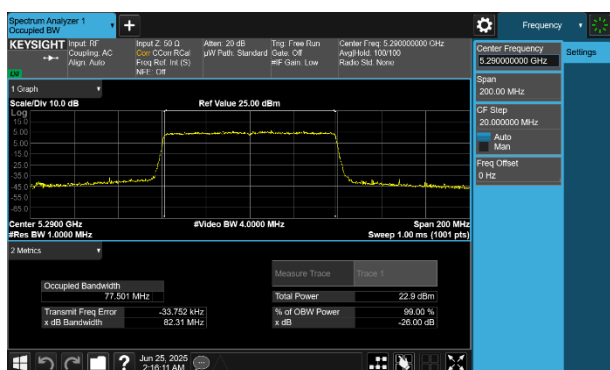
Plot 7-32 26dB BW & 99% OBW Antenna WF7 (80MHz BW 802.11be(RU) RU996 Index67 - Ch.58)
