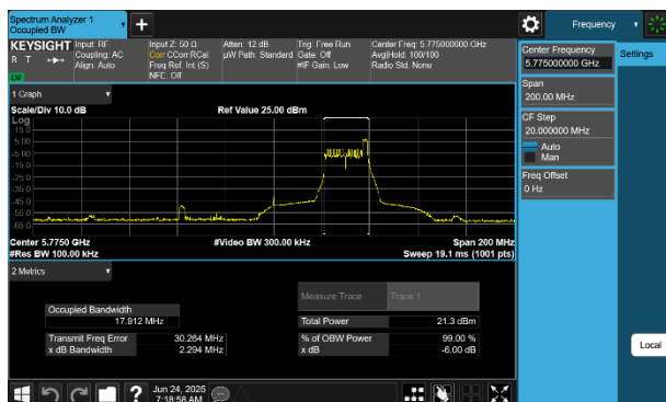
Plot 7-44 6dB BW & 99% OBW Antenna WF5B (80MHz BW 802.11be(RU) RU26 Index36 - Ch.155)
