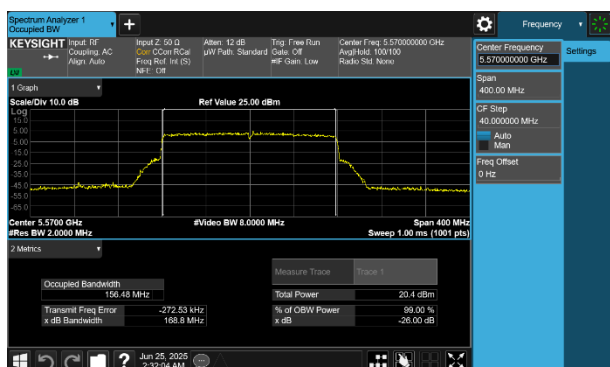
Plot 7-33 26dB BW & 99% OBW Antenna WF7 (160MHz BW 802.11be(RU) RU996X2 Index68 - Ch.114)
