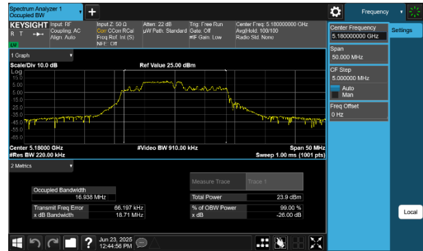
Plot 7-5 26dB BW & 99% OBW Antenna WF5B (20MHz BW 802.11be(RU) RU52+26 Index71 - Ch.36)
