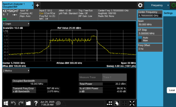
Plot 7-42 6dB BW & 99% OBW Antenna WF5B (20MHz BW 802.11be(RU) RU26 Index8 - Ch.157)
