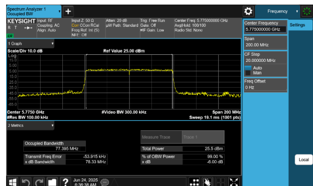
Plot 7-49 6dB BW & 99% OBW Antenna WF8 (80MHz BW 802.11be(RU) RU996 Index67 - Ch.155)
