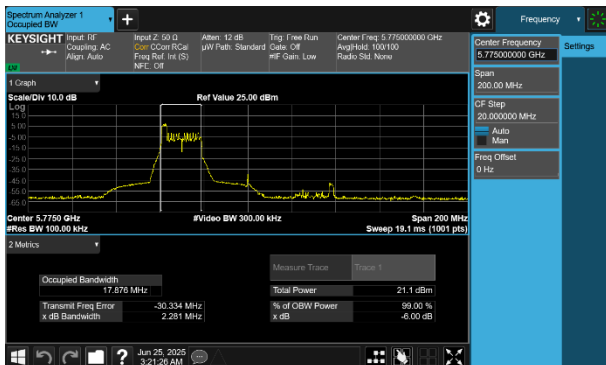
Plot 7-52 6dB BW & 99% OBW Antenna WF7 (80MHz BW 802.11be(RU) RU26 Index0 - Ch.155)
