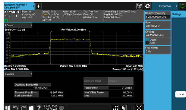
Plot 7-29 26dB BW & 99% OBW Antenna WF7 (160MHz BW 802.11be(RU) RU996+484 Index95 - Ch.50)
