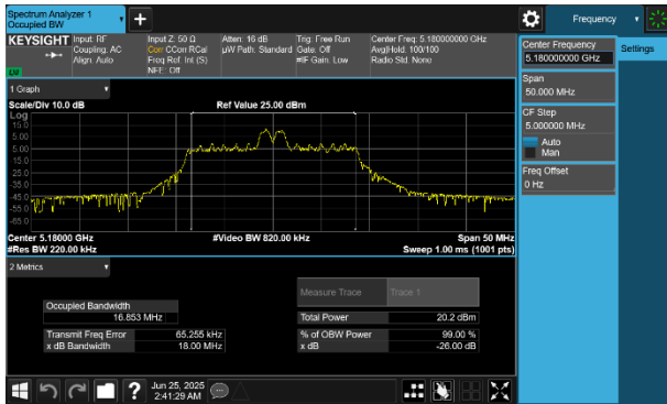
Plot 7-23 26dB BW & 99% OBW Antenna WF7 (20MHz BW 802.11be(RU) RU26 Index4 - Ch.36)
