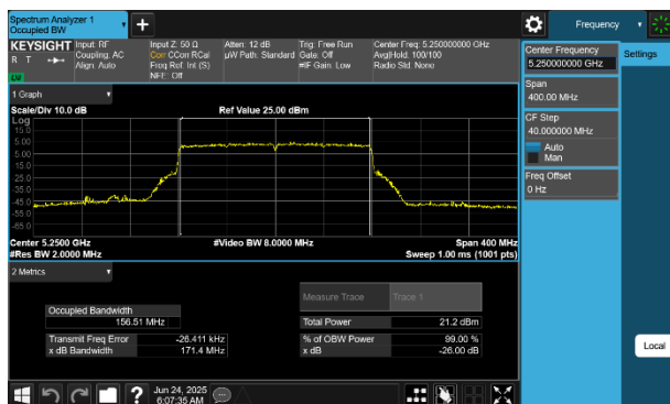
Plot 7-22 26dB BW & 99% OBW Antenna WF8 (160MHz BW 802.11be(RU) RU996X2 Index68 - Ch.50)
