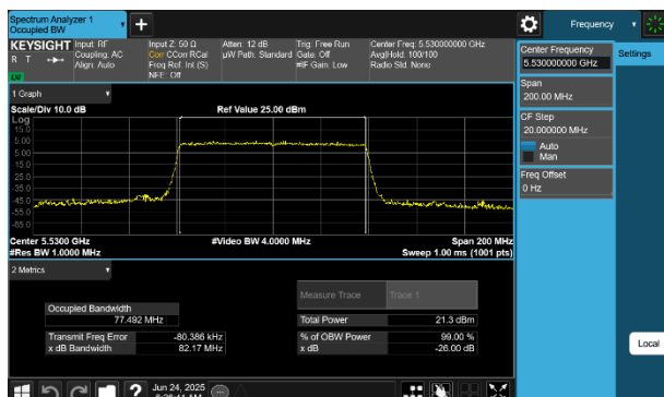
Plot 7-21 26dB BW & 99% OBW Antenna WF8 (80MHz BW 802.11be(RU) RU996 Index67 - Ch.106)
