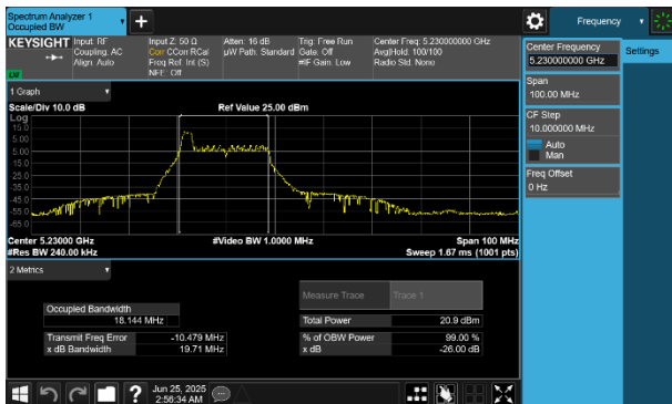
Plot 7-24 26dB BW & 99% OBW Antenna WF7 (40MHz BW 802.11be(RU) RU26 Index0 - Ch.46)
