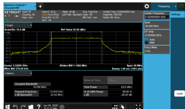
Plot 7-19 26dB BW & 99% OBW Antenna WF8 (20MHz BW 802.11be(RU) RU242 Index61 - Ch.64)
