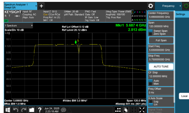
Plot 7-63 PSD Antenna WF5B (80MHz BW 802.11be(RU) RU484+242 Index93 - Ch.138)
