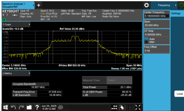
Plot 7-12 26dB BW & 99% OBW Antenna WF8 (20MHz BW 802.11be(RU) RU26 Index4 - Ch.36)
