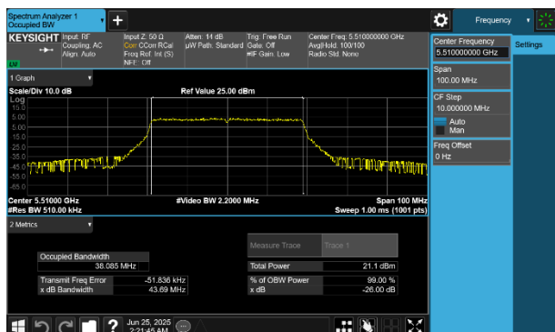
Plot 7-31 26dB BW & 99% OBW Antenna WF7 (40MHz BW 802.11be(RU) RU484 Index65 - Ch.102)
