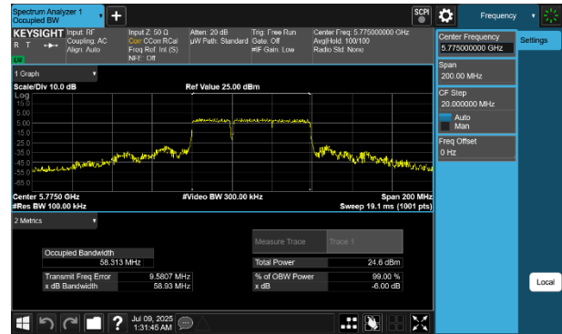
Plot 7-54 6dB BW & 99% OBW Antenna WF7 (80MHz BW 802.11be(RU) RU484+242 Index90 - Ch.155)
