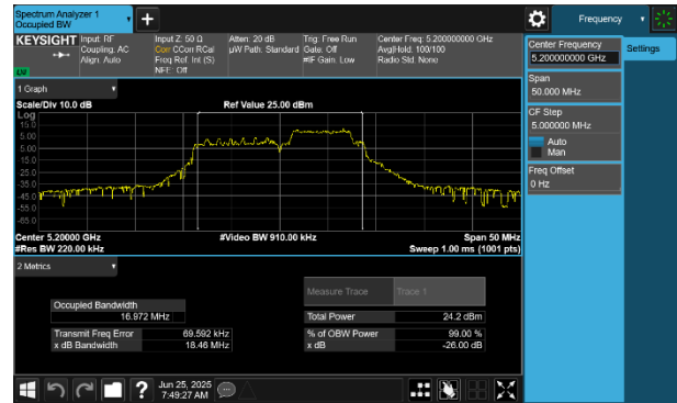
Plot 7-27 26dB BW & 99% OBW Antenna WF7 (20MHz BW 802.11be(RU) RU52+26 Index72 - Ch.40)
