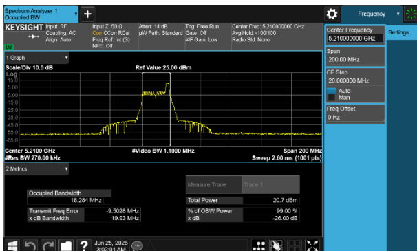
Plot 7-25 26dB BW & 99% OBW Antenna WF7 (80MHz BW 802.11be(RU) RU26 Index17 - Ch.42)
