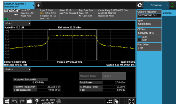
Plot 7-55 6dB BW & 99% OBW Antenna WF7 (20MHz BW 802.11be(RU) RU242 Index61 - Ch.165)
