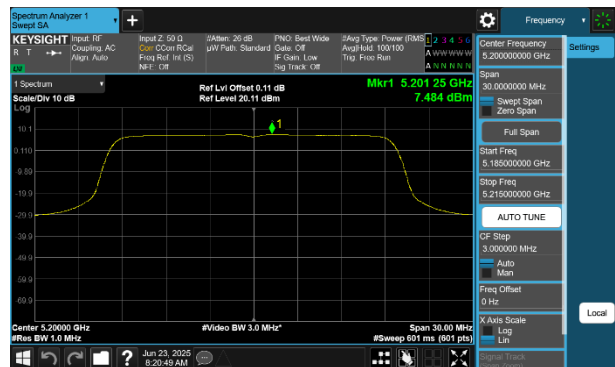
Plot 7-65 PSD Antenna WF5B (20MHz BW 802.11be(RU) RU242 Index61 - Ch.40)
