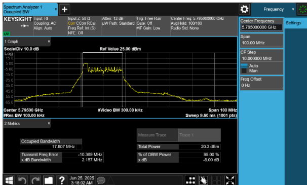
Plot 7-51 6dB BW & 99% OBW Antenna WF7 (40MHz BW 802.11be(RU) RU26 Index0 - Ch.159)
