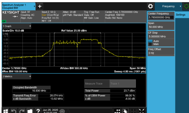
Plot 7-53 6dB BW & 99% OBW Antenna WF7 (20MHz BW 802.11be(RU) RU52+26 Index72 - Ch.157)
