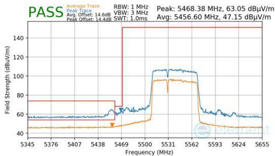
Plot 7-579. Antenna WF8 (Peak & Average, RU484+242, Index 90, Ch.106, MCS11)
