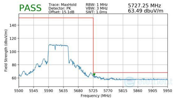
Plot 7-587. (FCC Only) Antenna WF8 (Peak, RU484+242, Index 90, Ch.122, MCS11)
