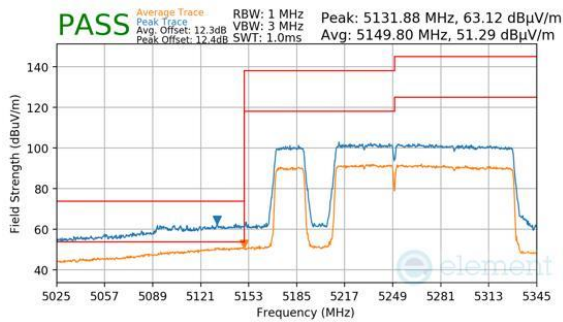
Plot 7-632. Antenna WF8 (Peak & Average, RU996+484+242, Index 97 (L), Ch.50, MCS11)
