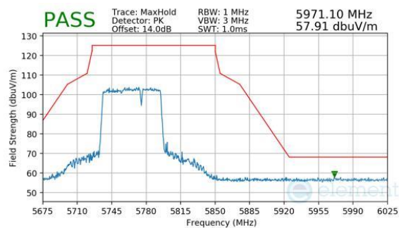
Plot 7-598. Antenna WF8 (Peak, RU484+242, Index 93, Ch.155, MCS11)
