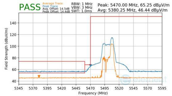
Plot 7-715. Antenna WF7 (Peak & Average, RU52, Index 40, Ch.102, MCS11)
