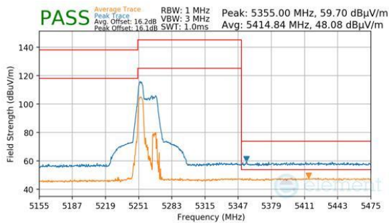
Plot 7-608. Antenna WF8 (Peak & Average, RU52, Index 37, Ch.50, MCS11)
