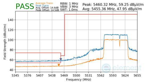
Plot 7-586. (FCC Only) Antenna WF8 (Peak & Average, RU484+242, Index 93, Ch.122, MCS11)
