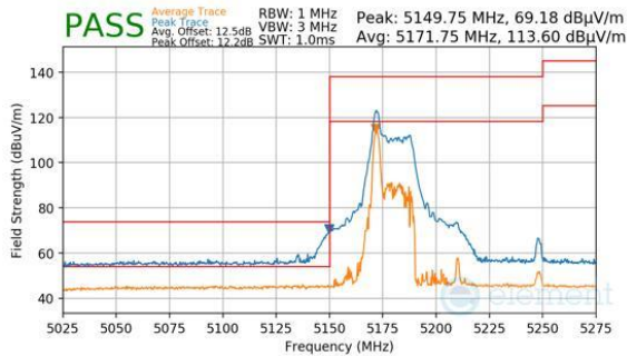
Plot 7-559. Antenna WF8 (Peak & Average, RU26, Index 0, Ch.42, MCS11)
