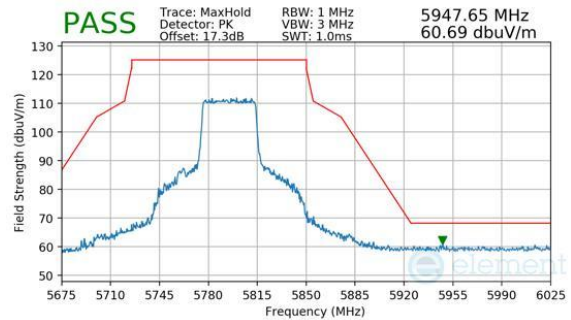
Plot 7-558. Antenna WF8 (Peak, RU484, Index 65, Ch.159, MCS11)
