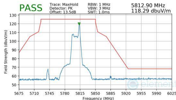
Plot 7-711. Antenna WF7 (Peak, RU26, Index 17, Ch.159, MCS11)
