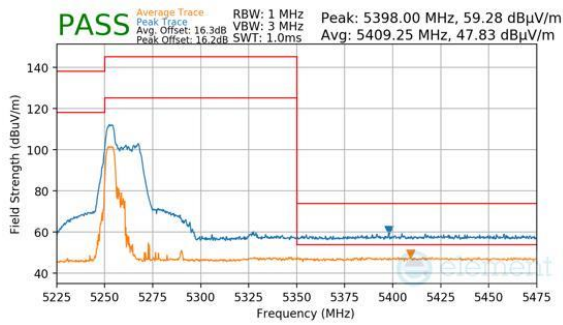
Plot 7-565. Antenna WF8 (Peak & Average, RU52, Index 37, Ch.58, MCS11)
