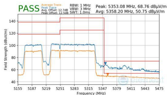
Plot 7-642. Antenna WF8 (Peak & Average, RU996+484+242, Index 98 (L), Ch.50, MCS11)
