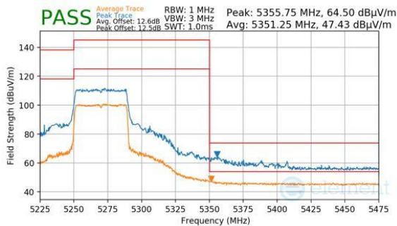
Plot 7-549. Antenna WF8 (Peak & Average, RU484, Index 65, Ch.54, MCS11)
