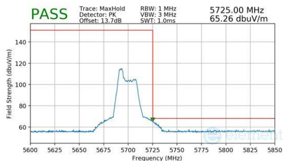
Plot 7-676. Antenna WF7 (Peak, RU52, Index 37, Ch.140, MCS11)
