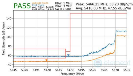
Plot 7-553. (FCC Only) Antenna WF8 (Peak & Average, RU484, Index 65, Ch.118, MCS11)
