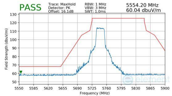
Plot 7-704. Antenna WF7 (Peak, RU242, Index 61, Ch.149, MCS11)
