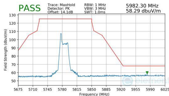
Plot 7-710. Antenna WF7 (Peak, RU26, Index 0, Ch.159, MCS11)
