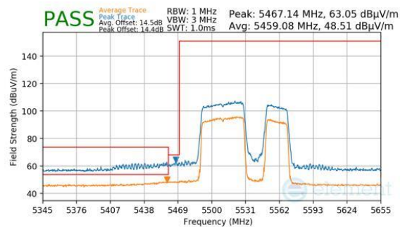
Plot 7-581. Antenna WF8 (Peak & Average, RU484+242, Index 92, Ch.106, MCS11)
