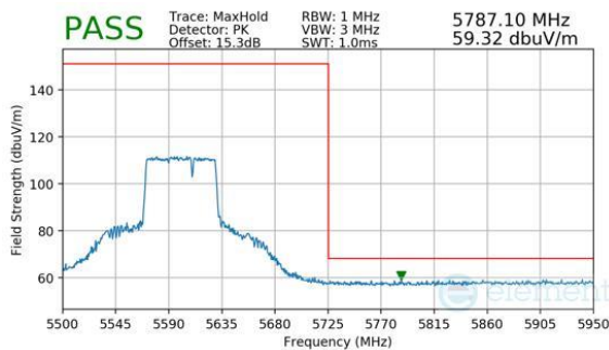
Plot 7-590. (FCC Only) Antenna WF8 (Peak, RU484+242, Index 93, Ch.122, MCS11)
