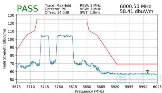
Plot 7-596. Antenna WF8 (Peak, RU484+242, Index 91, Ch.155, MCS11)
