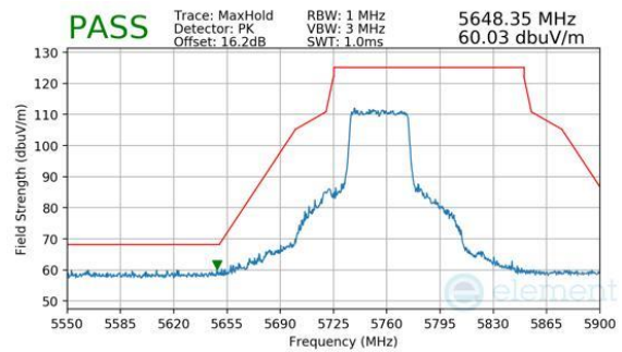
Plot 7-557. Antenna WF8 (Peak, RU484, Index 65, Ch.151, MCS11)
