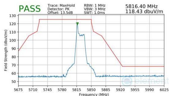
Plot 7-670. Antenna WF7 (Peak, RU26, Index 0, Ch.165, MCS11)
