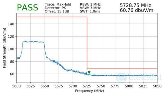
Plot 7-555. (FCC Only) Antenna WF8 (Peak, RU484, Index 65, Ch.126, MCS11)
