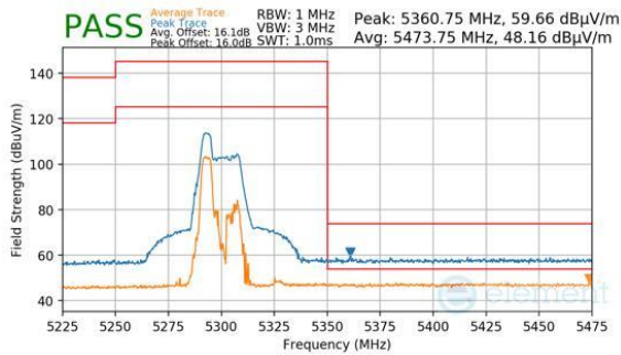
Plot 7-539. Antenna WF8 (Peak & Average, RU52, Index 37, Ch.62, MCS11)
