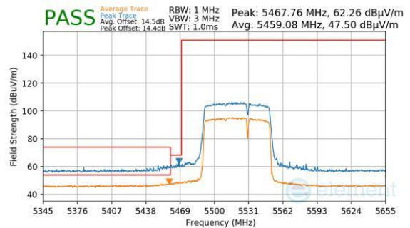
Plot 7-582. Antenna WF8 (Peak & Average, RU484+242, Index 93, Ch.106, MCS11)
