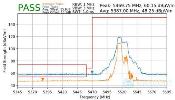
Plot 7-684. Antenna WF7 (Peak & Average, RU52+26, Index 70, Ch.104, MCS11)
