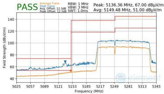
Plot 7-614. Antenna WF8 (Peak & Average, RU996+484, Index 94 (L), Ch.50, MCS11)
