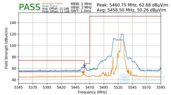
Plot 7-542. Antenna WF8 (Peak & Average, RU52, Index 44, Ch.102, MCS11)
