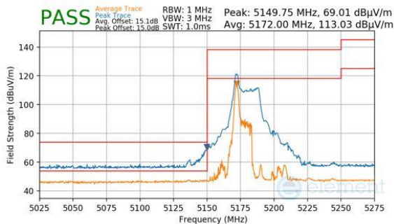
Plot 7-706. Antenna WF7 (Peak & Average, RU26, Index 0, Ch.38, MCS11)
