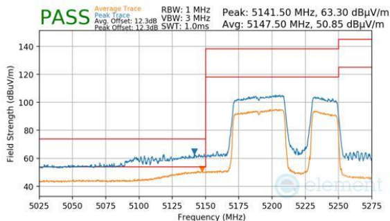
Plot 7-573. Antenna WF8 (Peak & Average, RU484+242, Index 92, Ch.42, MCS11)
