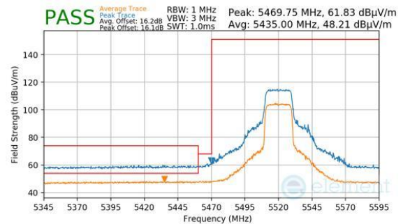
Plot 7-699. Antenna WF7 (Peak & Average, RU242, Index 61, Ch.104, MCS11)
