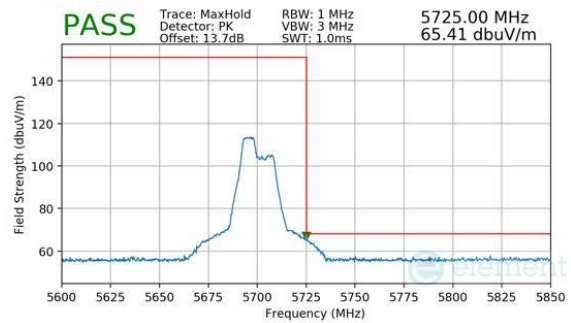
Plot 7-688. Antenna WF7 (Peak, RU52+26, Index 70, Ch.140, MCS11)
