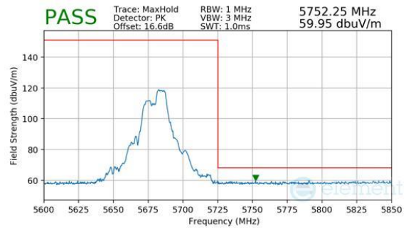
Plot 7-687. Antenna WF7 (Peak, RU52+26, Index 72, Ch.136, MCS11)
