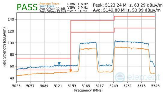
Plot 7-616. Antenna WF8 (Peak & Average, RU996+484, Index 95 (L), Ch.50, MCS11)
