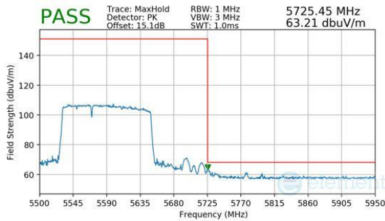
Plot 7-626. (FCC Only) Antenna WF8 (Peak, RU996+484, Index 94 (L), Ch.114, MCS11)
