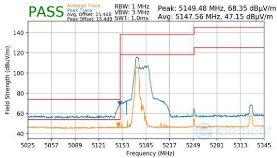
Plot 7-606. Antenna WF8 (Peak & Average, RU52, Index 37, Ch.50, MCS11)
