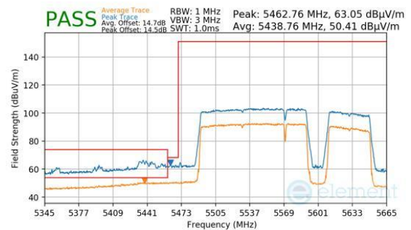
Plot 7-648. Antenna WF8 (Peak & Average, RU996+484+242, Index 97 (H), Ch.114, MCS11)
