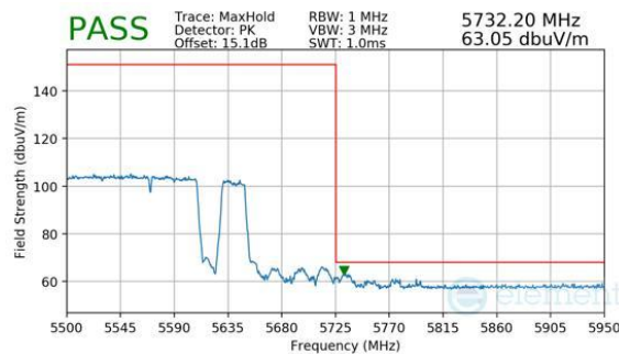
Plot 7-659. (FCC Only) Antenna WF8 (Peak, RU996+484+242, Index 98 (H), Ch.114, MCS11)
