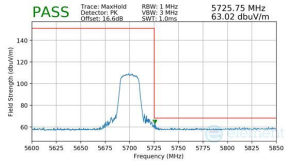
Plot 7-703. Antenna WF7 (Peak, RU242, Index 61, Ch.140, MCS11)
