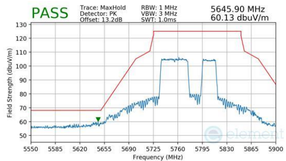
Plot 7-593. Antenna WF8 (Peak, RU484+242, Index 92, Ch.155, MCS11)
