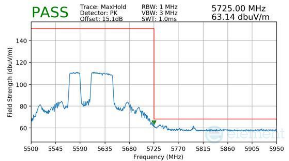
Plot 7-588. (FCC Only) Antenna WF8 (Peak, RU484+242, Index 91, Ch.122, MCS11)
