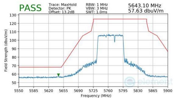
Plot 7-594. Antenna WF8 (Peak, RU484+242, Index 93, Ch.155, MCS11)
