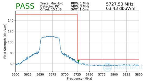
Plot 7-556. Antenna WF8 (Peak, RU484, Index 65, Ch.134, MCS11)
