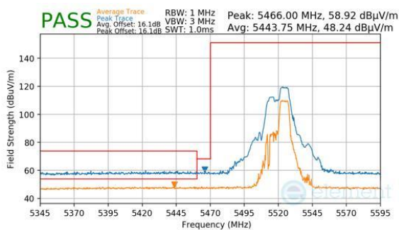
Plot 7-685. Antenna WF7 (Peak & Average, RU52+26, Index 72, Ch.104, MCS11)
