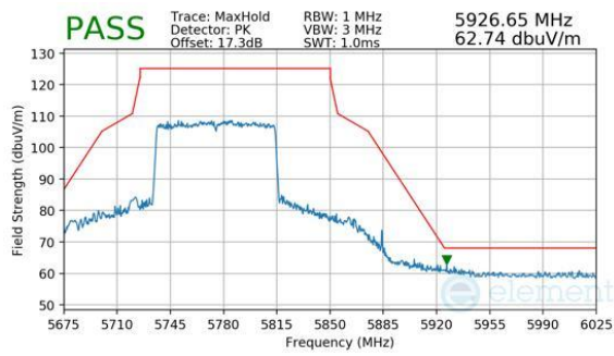
Plot 7-605. Antenna WF8 (Peak, RU996, Index 67, Ch.155, MCS11)
