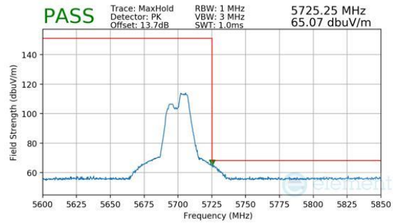
Plot 7-689. Antenna WF7 (Peak, RU52+26, Index 72, Ch.140, MCS11)
