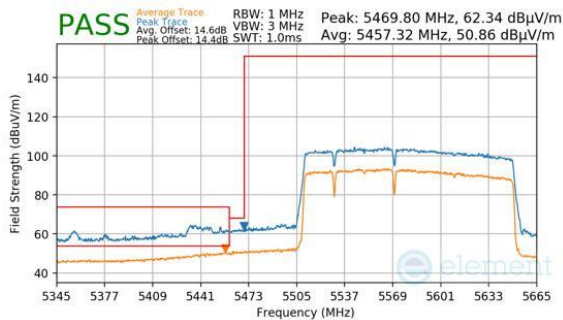
Plot 7-646. (FCC Only) Antenna WF8 (Peak & Average, RU996+484+242, Index 96 (L), Ch.114, MCS11)
