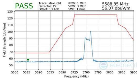
Plot 7-709. Antenna WF7 (Peak, RU26, Index 17, Ch.151, MCS11)
