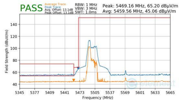
Plot 7-610. (FCC Only) Antenna WF8 (Peak & Average, RU52, Index 37, Ch.114, MCS11)
