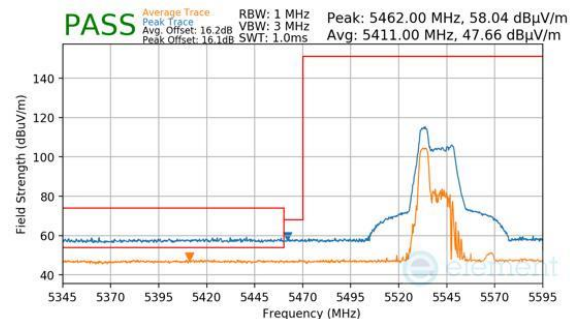
Plot 7-717. Antenna WF7 (Peak & Average, RU52, Index 37, Ch.110, MCS11)
