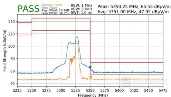
Plot 7-673. Antenna WF7 (Peak & Average, RU52, Index 40, Ch.64, MCS11)
