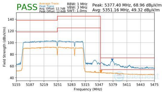
Plot 7-644. Antenna WF8 (Peak & Average, RU996+484+242, Index 99 (H), Ch.50, MCS11)
