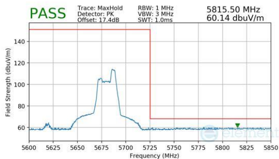
Plot 7-546. Antenna WF8 (Peak, RU52, Index 44, Ch.134, MCS11)
