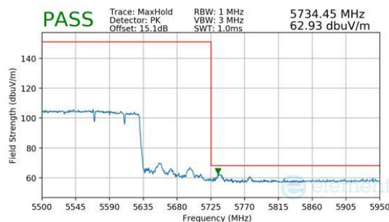
Plot 7-661. (FCC Only) Antenna WF8 (Peak, RU996+484+242, Index 99 (H), Ch.114, MCS11)
