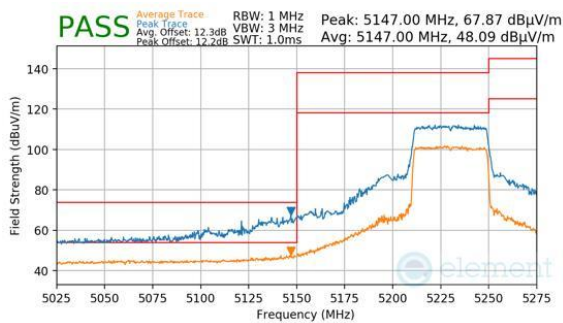
Plot 7-548. Antenna WF8 (Peak & Average, RU484, Index 65, Ch.46, MCS11)
