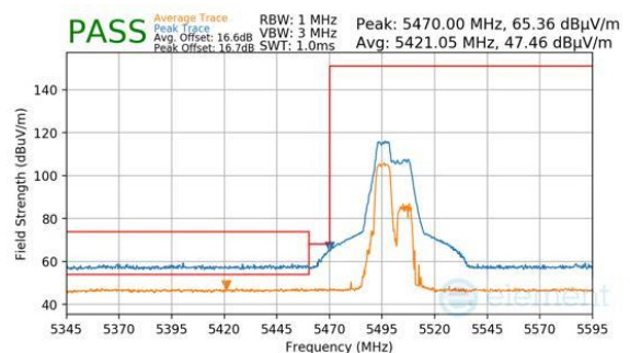
Plot 7-682. Antenna WF7 (Peak & Average, RU52+26, Index 70, Ch.100, MCS11)
