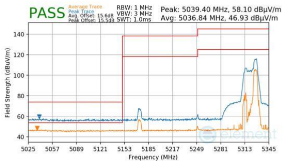
Plot 7-607. Antenna WF8 (Peak & Average, RU52, Index 52 (H), Ch.50, MCS11)
