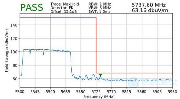
Plot 7-655. (FCC Only) Antenna WF8 (Peak, RU996+484+242, Index 96 (L), Ch.114, MCS11)
