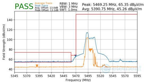
Plot 7-541. Antenna WF8 (Peak & Average, RU52, Index 37, Ch.102, MCS11)
