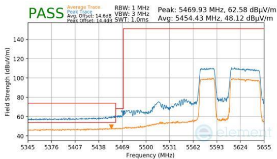
Plot 7-584. (FCC Only) Antenna WF8 (Peak & Average, RU484+242, Index 91, Ch.122, MCS11)
