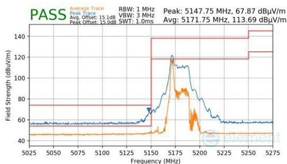
Plot 7-666. Antenna WF7 (Peak & Average, RU26, Index 0, Ch.36, MCS11)
