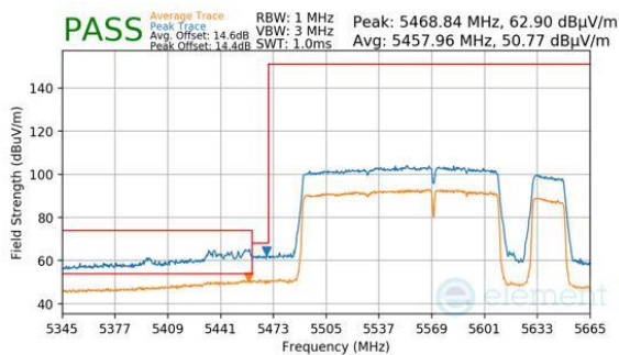
Plot 7-651. (FCC Only) Antenna WF8 (Peak & Average, RU996+484+242, Index 98 (H), Ch.114, MCS11)
