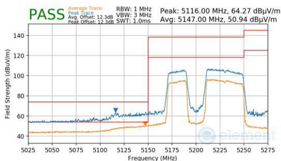
Plot 7-572. Antenna WF8 (Peak & Average, RU484+242, Index 91, Ch.42, MCS11)
