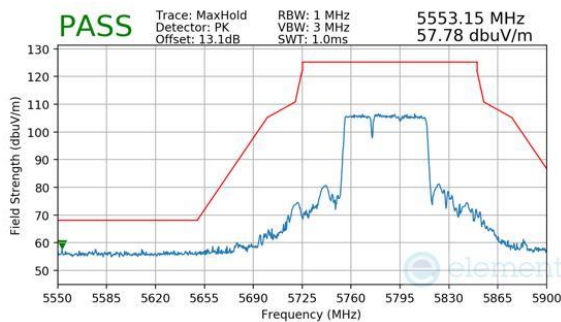
Plot 7-591. Antenna WF8 (Peak, RU484+242, Index 90, Ch.155, MCS11)
