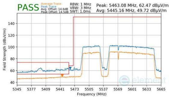
Plot 7-650. (FCC Only) Antenna WF8 (Peak & Average, RU996+484+242, Index 98 (L), Ch.114, MCS11)
