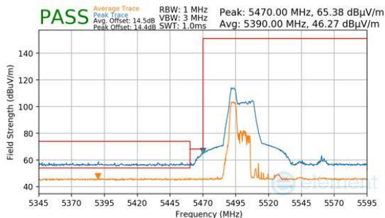
Plot 7-714. Antenna WF7 (Peak & Average, RU52, Index 37, Ch.102, MCS11)
