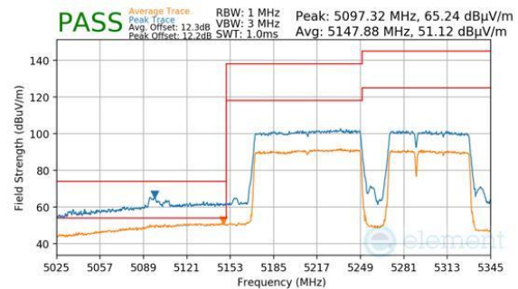
Plot 7-631. Antenna WF8 (Peak & Average, RU996+484+242, Index 96 (H), Ch.50, MCS11)
