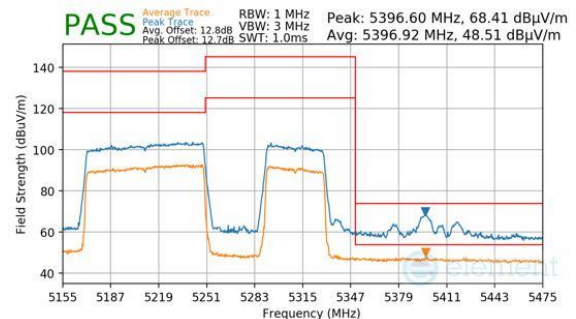
Plot 7-619. Antenna WF8 (Peak & Average, RU996+484, Index 94 (H), Ch.50, MCS11)
