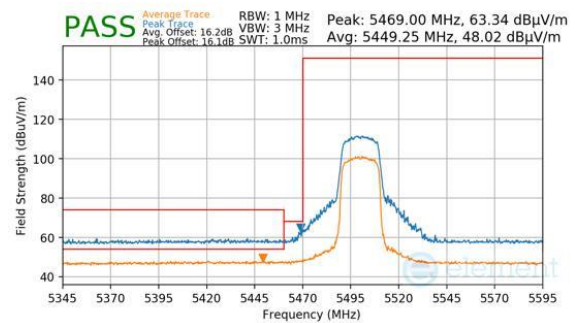
Plot 7-698. Antenna WF7 (Peak & Average, RU242, Index 61, Ch.100, MCS11)
