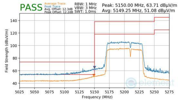
Plot 7-574. Antenna WF8 (Peak & Average, RU484+242, Index 93, Ch.42, MCS11)
