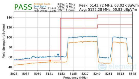
Plot 7-615. Antenna WF8 (Peak & Average, RU996+484, Index 94 (H), Ch.50, MCS11)
