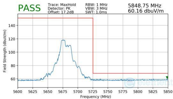
Plot 7-686. Antenna WF7 (Peak, RU52+26, Index 70, Ch.136, MCS11)
