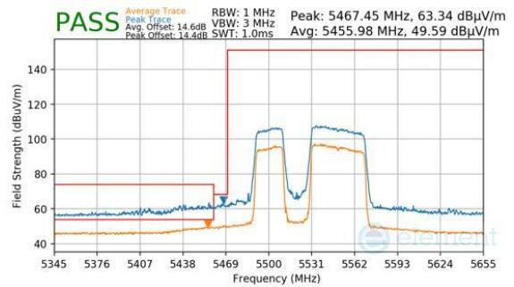
Plot 7-580. Antenna WF8 (Peak & Average, RU484+242, Index 91, Ch.106, MCS11)
