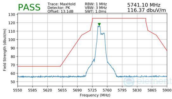
Plot 7-690. Antenna WF7 (Peak, RU52+26, Index 70, Ch.149, MCS11)
