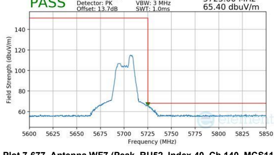
Plot 7-677. Antenna WF7 (Peak, RU52, Index 40, Ch.140, MCS11)
