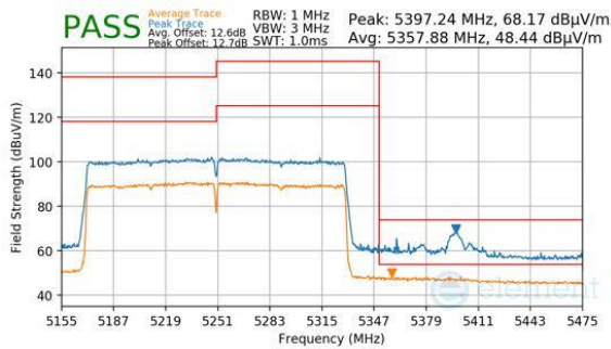
Plot 7-663. Antenna WF8 (Peak & Average, RU996X2, Index 68, Ch.50, MCS11)
