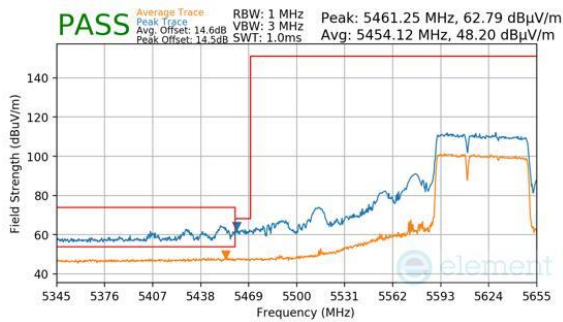
Plot 7-583. (FCC Only) Antenna WF8 (Peak & Average, RU484+242, Index 90, Ch.122, MCS11)
