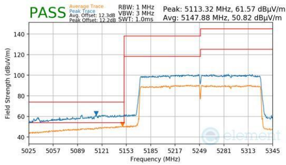
Plot 7-662. Antenna WF8 (Peak & Average, RU996X2, Index 68, Ch.50, MCS11)
