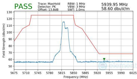
Plot 7-692. Antenna WF7 (Peak, RU52+26, Index 70, Ch.165, MCS11)
