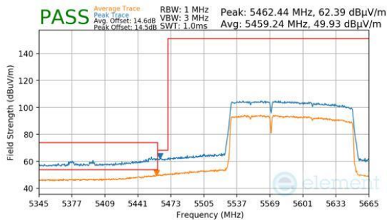
Plot 7-622. (FCC Only) Antenna WF8 (Peak & Average, RU996+484, Index 94 (L), Ch.114, MCS11)
