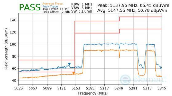
Plot 7-635. Antenna WF8 (Peak & Average, RU996+484+242, Index 98 (H), Ch.50, MCS11)
