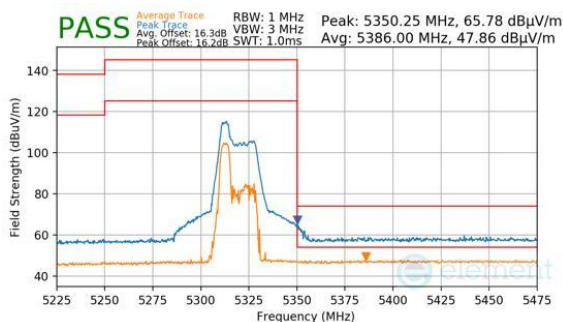
Plot 7-672. Antenna WF7 (Peak & Average, RU52, Index 37, Ch.64, MCS11)
