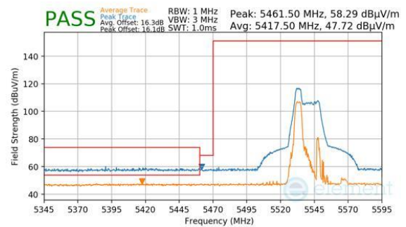
Plot 7-543. Antenna WF8 (Peak & Average, RU52, Index 37, Ch.110, MCS11)
