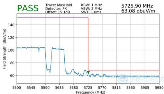
Plot 7-657. (FCC Only) Antenna WF8 (Peak, RU996+484+242, Index 97 (H), Ch.114, MCS11)
