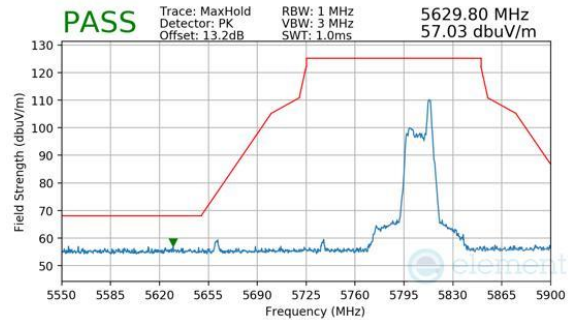
Plot 7-562. Antenna WF8 (Peak, RU26, Index 36, Ch.155, MCS11)
