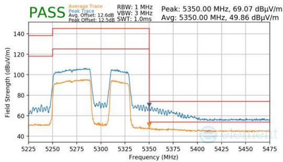
Plot 7-577. Antenna WF8 (Peak & Average, RU484+242, Index 92, Ch.58, MCS11)
