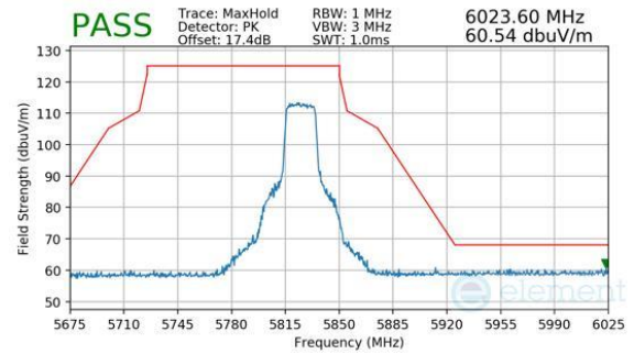
Plot 7-705. Antenna WF7 (Peak, RU242, Index 61, Ch.165, MCS11)
