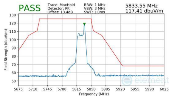
Plot 7-671. Antenna WF7 (Peak, RU26, Index 8, Ch.165, MCS11)
