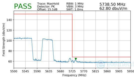
Plot 7-627. (FCC Only) Antenna WF8 (Peak, RU996+484, Index 94 (H), Ch.114, MCS11)
