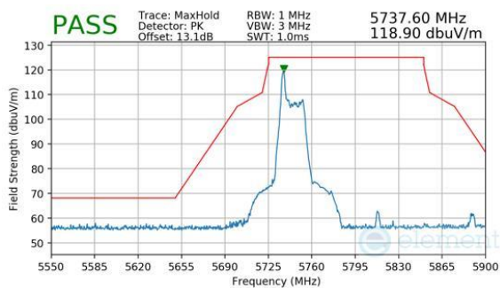
Plot 7-561. Antenna WF8 (Peak, RU26, Index 0, Ch.155, MCS11)
