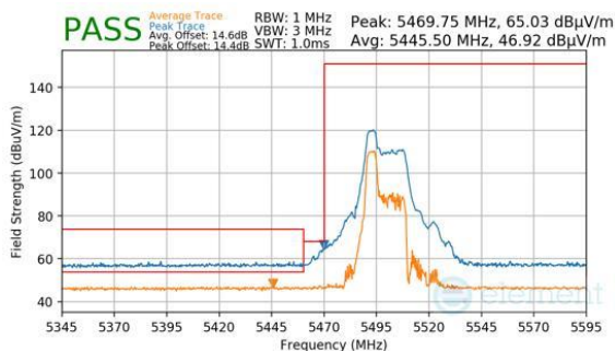
Plot 7-674. Antenna WF7 (Peak & Average, RU52, Index 37, Ch.100, MCS11)
