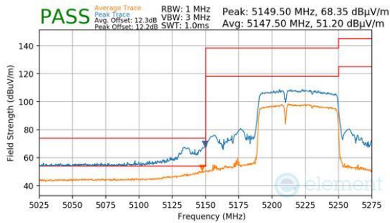
Plot 7-571. Antenna WF8 (Peak & Average, RU484+242, Index 90, Ch.42, MCS11)
