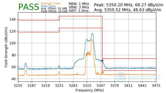
Plot 7-609. Antenna WF8 (Peak & Average, RU52, Index 52 (H), Ch.50, MCS11)
