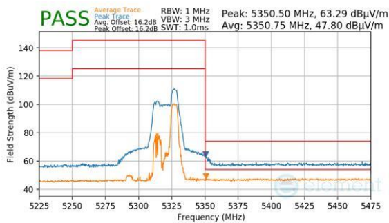
Plot 7-713. Antenna WF7 (Peak & Average, RU52, Index 44, Ch.62, MCS11)
