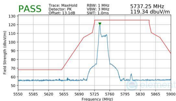
Plot 7-708. Antenna WF7 (Peak, RU26, Index 0, Ch.151, MCS11)
