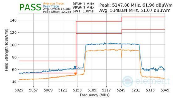
Plot 7-617. Antenna WF8 (Peak & Average, RU996+484, Index 95 (H), Ch.50, MCS11)
