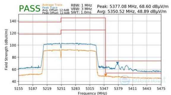
Plot 7-618. Antenna WF8 (Peak & Average, RU996+484, Index 94 (L), Ch.50, MCS11)
