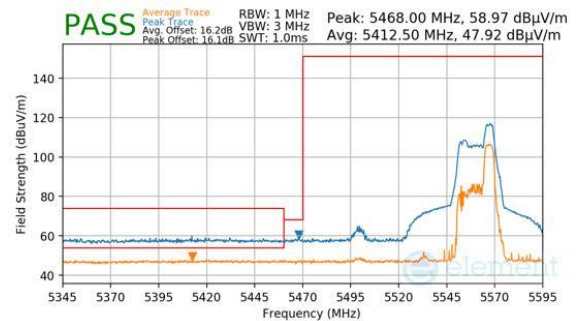
Plot 7-544. Antenna WF8 (Peak & Average, RU52, Index 44, Ch.110, MCS11)
