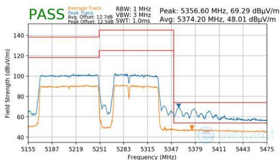
Plot 7-639. Antenna WF8 (Peak & Average, RU996+484+242, Index 96 (H), Ch.50, MCS11)
