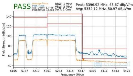
Plot 7-640. Antenna WF8 (Peak & Average, RU996+484+242, Index 97 (L), Ch.50, MCS11)
