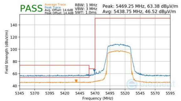
Plot 7-551. Antenna WF8 (Peak & Average, RU484, Index 65, Ch.102, MCS11)
