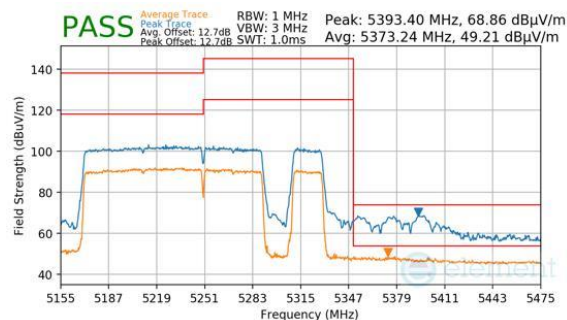
Plot 7-643. Antenna WF8 (Peak & Average, RU996+484+242, Index 98 (H), Ch.50, MCS11)
