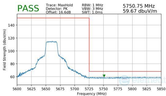
Plot 7-701. Antenna WF7 (Peak, RU242, Index 61, Ch.132, MCS11)
