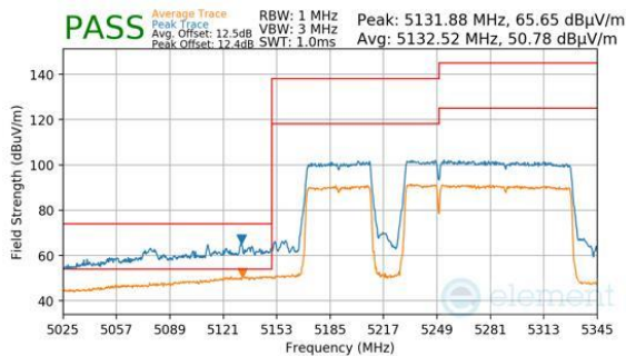
Plot 7-634. Antenna WF8 (Peak & Average, RU996+484+242, Index 98 (L), Ch.50, MCS11)
