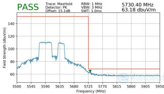
Plot 7-589. (FCC Only) Antenna WF8 (Peak, RU484+242, Index 92, Ch.122, MCS11)
