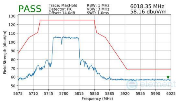
Plot 7-595. Antenna WF8 (Peak, RU484+242, Index 90, Ch.155, MCS11)
