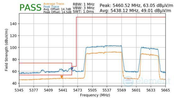
Plot 7-623. (FCC Only) Antenna WF8 (Peak & Average, RU996+484, Index 94 (H), Ch.114, MCS11)
