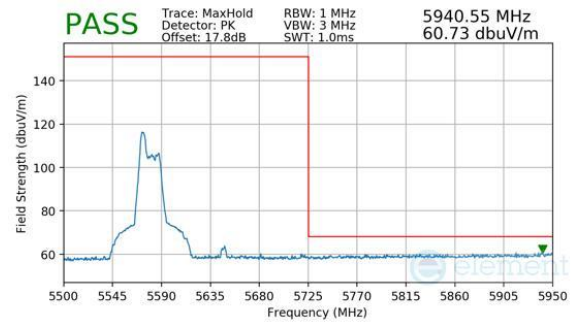
Plot 7-569. (FCC Only) Antenna WF8 (Peak, RU52, Index 37, Ch.122, MCS11)
