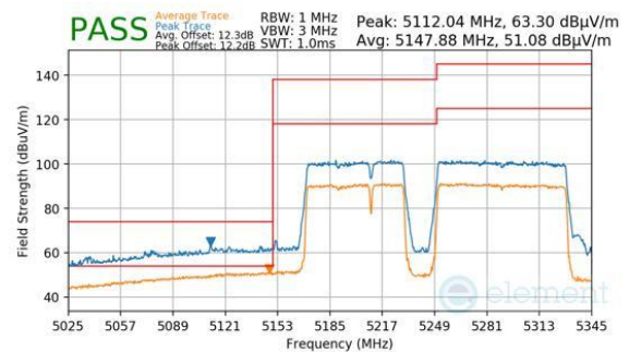
Plot 7-636. Antenna WF8 (Peak & Average, RU996+484+242, Index 99 (L), Ch.50, MCS11)
