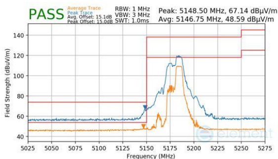
Plot 7-679. Antenna WF7 (Peak & Average, RU52+26, Index 72, Ch.36, MCS11)
