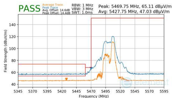
Plot 7-675. Antenna WF7 (Peak & Average, RU52, Index 40, Ch.100, MCS11)
