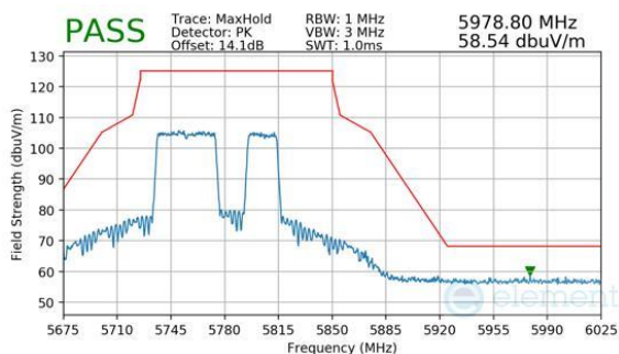
Plot 7-597. Antenna WF8 (Peak, RU484+242, Index 92, Ch.155, MCS11)
