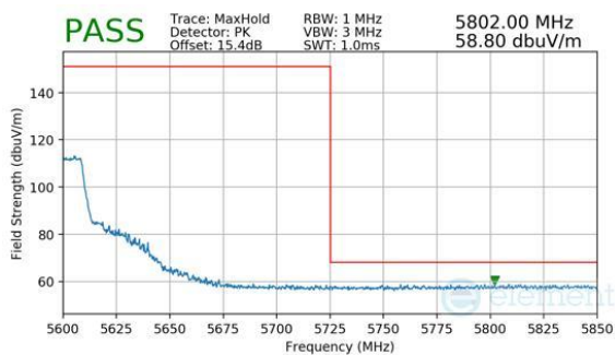
Plot 7-554. (FCC Only) Antenna WF8 (Peak, RU484, Index 65, Ch.118, MCS11)
