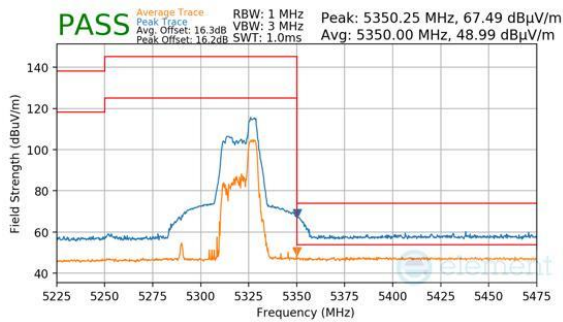
Plot 7-566. Antenna WF8 (Peak & Average, RU52, Index 52, Ch.58, MCS11)
