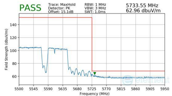
Plot 7-654. (FCC Only) Antenna WF8 (Peak, RU996+484+242, Index 96 (H), Ch.114, MCS11)
