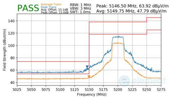
Plot 7-695. Antenna WF7 (Peak & Average, RU242, Index 61, Ch.40, MCS11)
