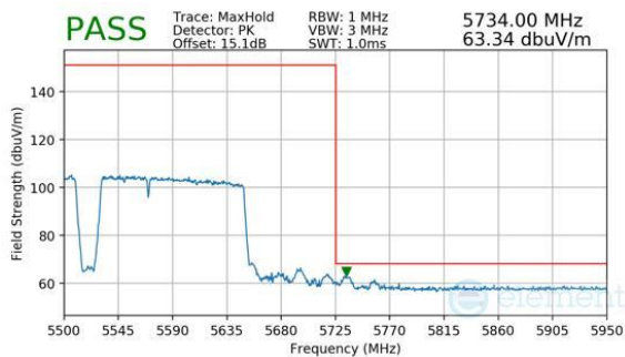
Plot 7-656. (FCC Only) Antenna WF8 (Peak, RU996+484+242, Index 97 (L), Ch.114, MCS11)
