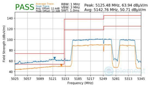
Plot 7-633. Antenna WF8 (Peak & Average, RU996+484+242, Index 97 (H), Ch.50, MCS11)
