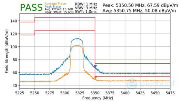
Plot 7-697. Antenna WF7 (Peak & Average, RU242, Index 61, Ch.64, MCS11)
