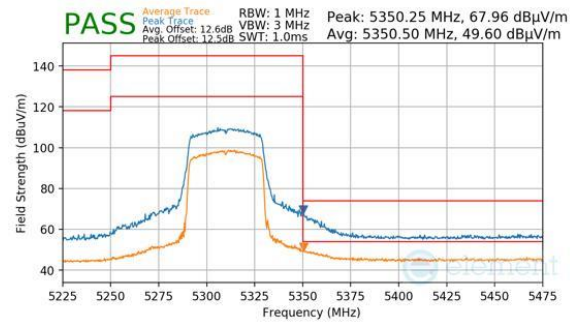
Plot 7-550. Antenna WF8 (Peak & Average, RU484, Index 65, Ch.62, MCS11)
