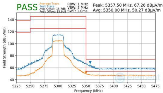
Plot 7-696. Antenna WF7 (Peak & Average, RU242, Index 61, Ch.60, MCS11)
