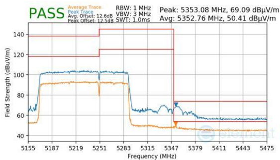
Plot 7-621. Antenna WF8 (Peak & Average, RU996+484, Index 95 (H), Ch.50, MCS11)
