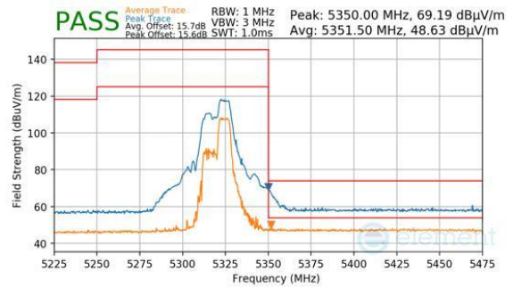
Plot 7-681. Antenna WF7 (Peak & Average, RU52+26, Index 72, Ch.64, MCS11)
