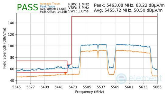
Plot 7-652. (FCC Only) Antenna WF8 (Peak & Average, RU996+484+242, Index 99 (L), Ch.114, MCS11)
