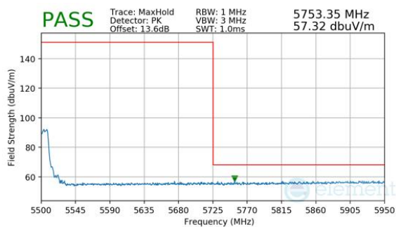
Plot 7-612. (FCC Only) Antenna WF8 (Peak, RU52, Index 37, Ch.114, MCS11)
