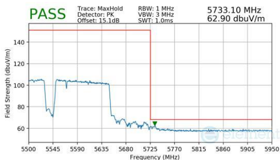
Plot 7-658. (FCC Only) Antenna WF8 (Peak, RU996+484+242, Index 98 (L), Ch.114, MCS11)
