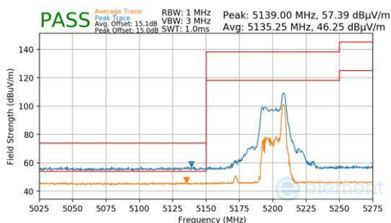
Plot 7-707. Antenna WF7 (Peak & Average, RU26, Index 17, Ch.38, MCS11)
