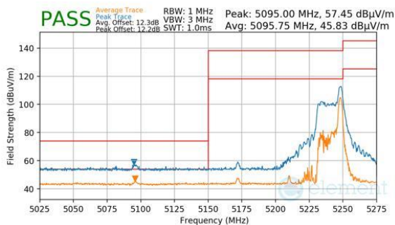
Plot 7-560. Antenna WF8 (Peak & Average, RU26, Index 36, Ch.42, MCS11)
