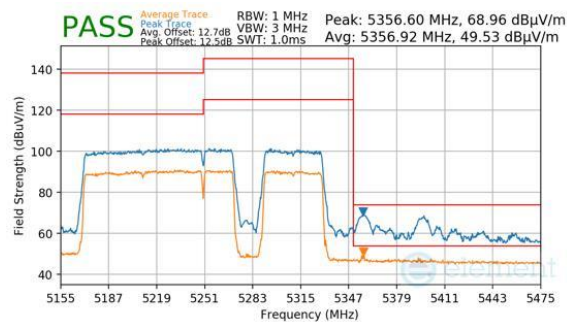
Plot 7-641. Antenna WF8 (Peak & Average, RU996+484+242, Index 97 (H), Ch.50, MCS11)
