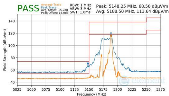
Plot 7-667. Antenna WF7 (Peak & Average, RU26, Index 8, Ch.36, MCS11)
