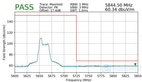
Plot 7-545. Antenna WF8 (Peak, RU52, Index 37, Ch.134, MCS11)
