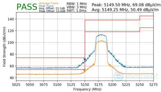
Plot 7-694. Antenna WF7 (Peak & Average, RU242, Index 61, Ch.36, MCS11)
