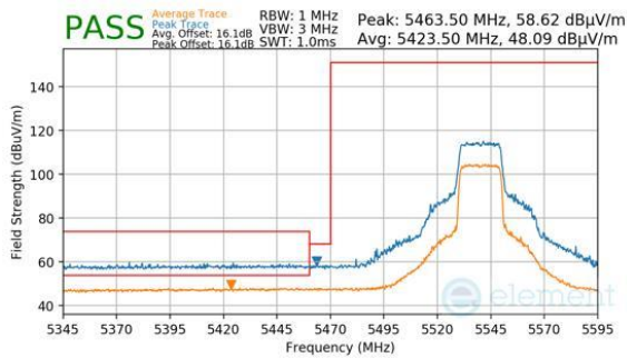
Plot 7-700. Antenna WF7 (Peak & Average, RU242, Index 61, Ch.108, MCS11)
