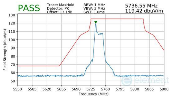
Plot 7-668. Antenna WF7 (Peak, RU26, Index 0, Ch.149, MCS11)
