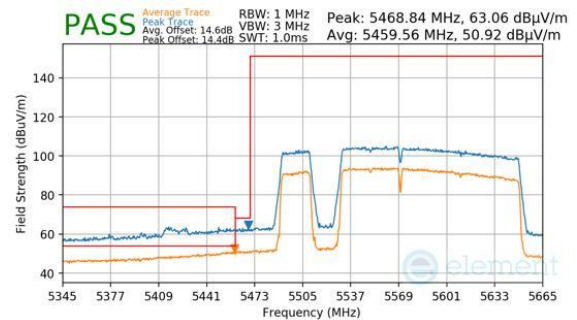
Plot 7-649. (FCC Only) Antenna WF8 (Peak & Average, RU996+484+242, Index 97 (L), Ch.114, MCS11)
