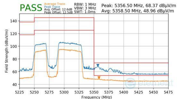
Plot 7-576. Antenna WF8 (Peak & Average, RU484+242, Index 91, Ch.58, MCS11)
