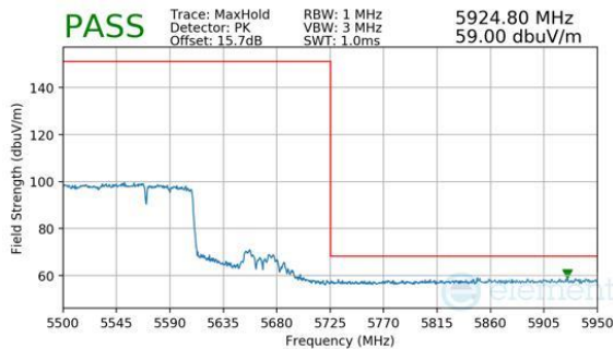
Plot 7-628. (FCC Only) Antenna WF8 (Peak, RU996+484, Index 95 (H), Ch.114, MCS11)
