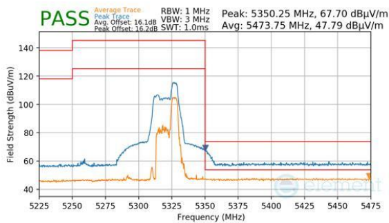
Plot 7-540. Antenna WF8 (Peak & Average, RU52, Index 44, Ch.62, MCS11)
