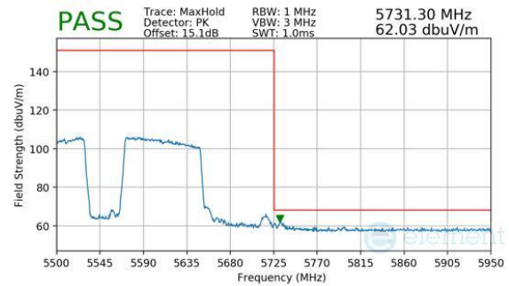
Plot 7-629. (FCC Only) Antenna WF8 (Peak, RU996+484, Index 95 (L), Ch.114, MCS11)
