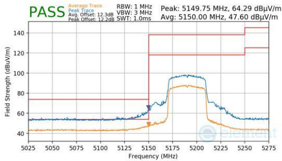
Plot 7-547. Antenna WF8 (Peak & Average, RU484, Index 65, Ch.38, MCS11)
