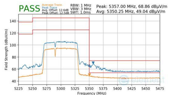
Plot 7-575. Antenna WF8 (Peak & Average, RU484+242, Index 90, Ch.58, MCS11)
