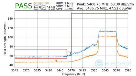
Plot 7-552. Antenna WF8 (Peak & Average, RU484, Index 65, Ch.110, MCS11)
