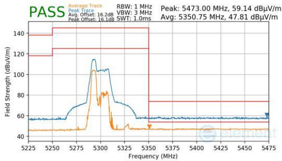
Plot 7-712. Antenna WF7 (Peak & Average, RU52, Index 37, Ch.62, MCS11)
