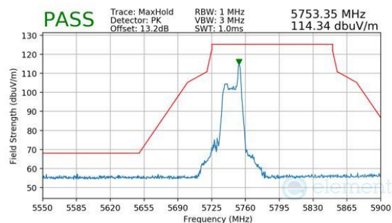
Plot 7-669. Antenna WF7 (Peak, RU26, Index 8, Ch.149, MCS11)
