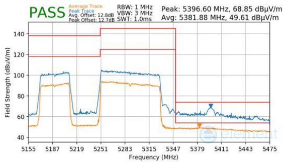
Plot 7-620. Antenna WF8 (Peak & Average, RU996+484, Index 95 (L), Ch.50, MCS11)
