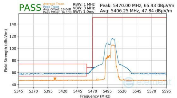
Plot 7-683. Antenna WF7 (Peak & Average, RU52+26, Index 72, Ch.100, MCS11)
