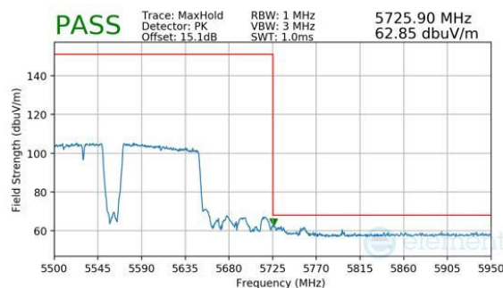
Plot 7-660. (FCC Only) Antenna WF8 (Peak, RU996+484+242, Index 99 (L), Ch.114, MCS11)
