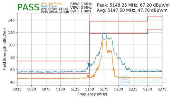
Plot 7-678. Antenna WF7 (Peak & Average, RU52+26, Index 70, Ch.36, MCS11)
