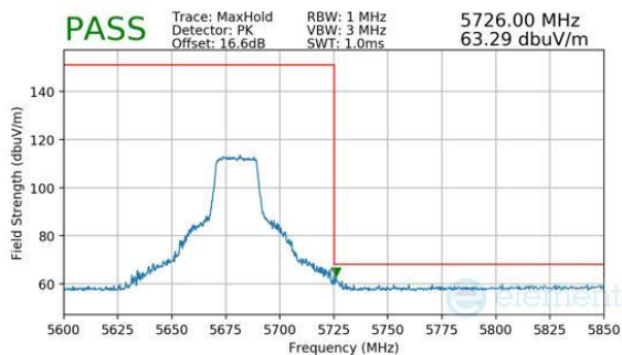
Plot 7-702. Antenna WF7 (Peak, RU242, Index 61, Ch.136, MCS11)
