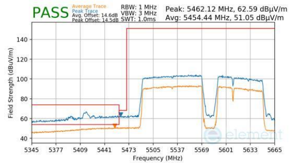
Plot 7-647. Antenna WF8 (Peak & Average, RU996+484+242, Index 96 (H), Ch.114, MCS11)
