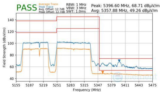
Plot 7-645. Antenna WF8 (Peak & Average, RU996+484+242, Index 99 (L), Ch.50, MCS11)
