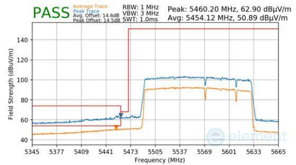
Plot 7-653. (FCC Only) Antenna WF8 (Peak & Average, RU996+484+242, Index 99 (H), Ch.114, MCS11)
