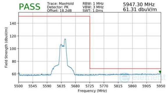
Plot 7-570. (FCC Only) Antenna WF8 (Peak, RU52, Index 52, Ch.122, MCS11)
