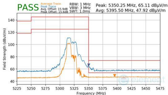
Plot 7-680. Antenna WF7 (Peak & Average, RU52+26, Index 70, Ch.64, MCS11)
