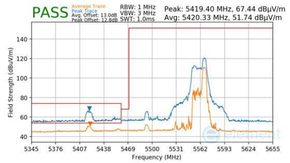
Plot 7-568. Antenna WF8 (Peak & Average, RU52, Index 52, Ch.106, MCS11)
