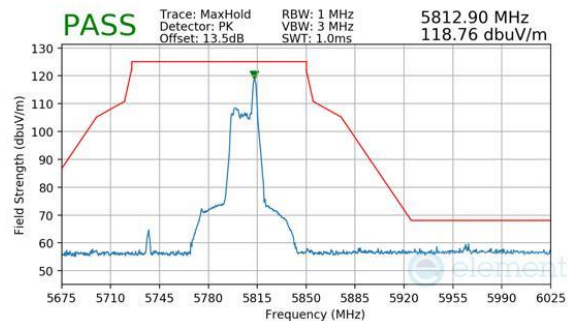
Plot 7-564. Antenna WF8 (Peak, RU26, Index 36, Ch.155, MCS11)
