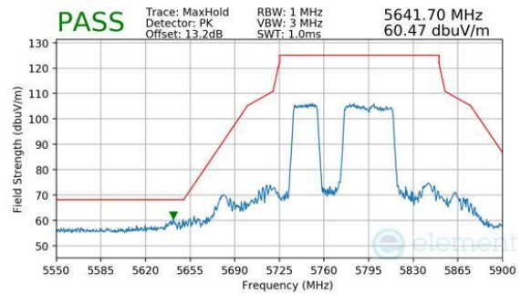
Plot 7-592. Antenna WF8 (Peak, RU484+242, Index 91, Ch.155, MCS11)
