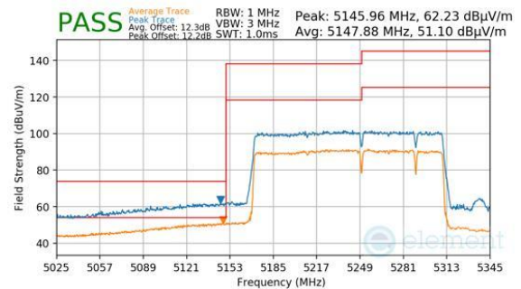
Plot 7-637. Antenna WF8 (Peak & Average, RU996+484+242, Index 99 (H), Ch.50, MCS11)
