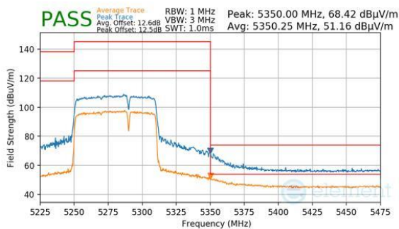
Plot 7-578. Antenna WF8 (Peak & Average, RU484+242, Index 93, Ch.58, MCS11)
