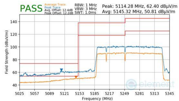
Plot 7-630. Antenna WF8 (Peak & Average, RU996+484+242, Index 96 (L), Ch.50, MCS11)
