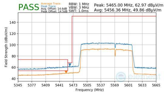
Plot 7-625. (FCC Only) Antenna WF8 (Peak & Average, RU996+484, Index 95 (H), Ch.114, MCS11)
