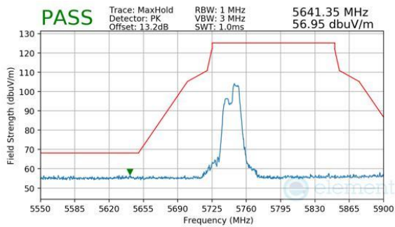
Plot 7-691. Antenna WF7 (Peak, RU52+26, Index 72, Ch.149, MCS11)
