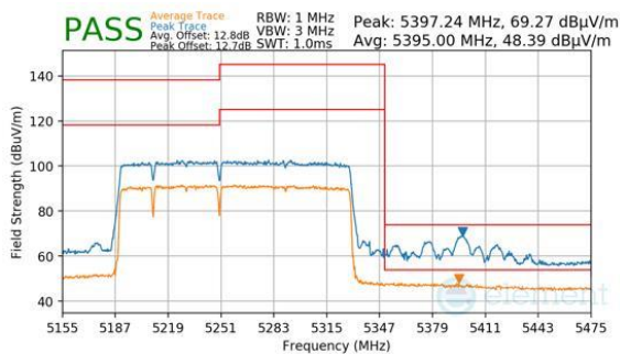
Plot 7-638. Antenna WF8 (Peak & Average, RU996+484+242, Index 96 (L), Ch.50, MCS11)
