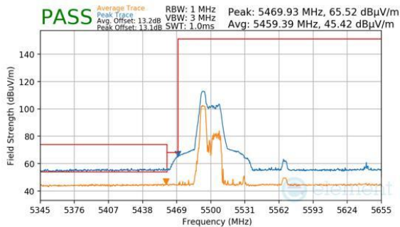
Plot 7-567. Antenna WF8 (Peak & Average, RU52, Index 37, Ch.106, MCS11)
