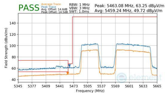
Plot 7-624. (FCC Only) Antenna WF8 (Peak & Average, RU996+484, Index 95 (L), Ch.114, MCS11)
