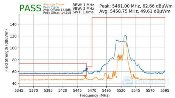
Plot 7-716. Antenna WF7 (Peak & Average, RU52, Index 44, Ch.102, MCS11)
