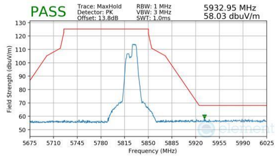
Plot 7-693. Antenna WF7 (Peak, RU52+26, Index 72, Ch.165, MCS11)
