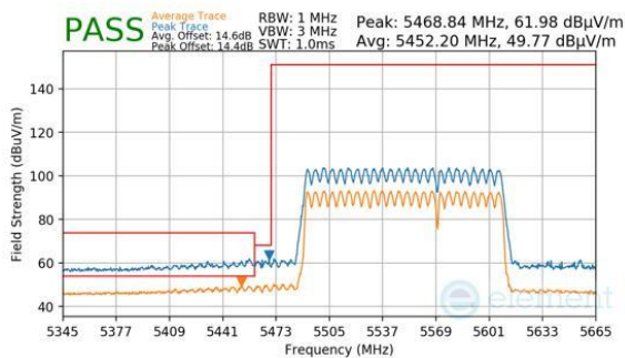
Plot 7-966. (FCC Only) CDD Primary (Peak & Average, RU996+484, Index 95 (H), Ch.114, MCS11)
