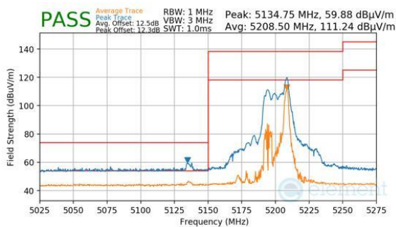
Plot 7-1043. CDD Diversity (Peak & Average, RU26, Index 17, Ch.38, MCS11)
