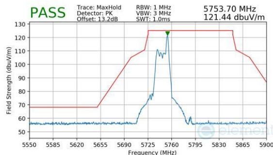
Plot 7-1006. CDD Diversity (Peak, RU26, Index 8, Ch.149, MCS11)
