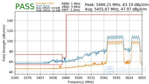
Plot 7-930. (FCC Only) CDD Primary (Peak & Average, RU484+242, Index 92, Ch.122, MCS11)
