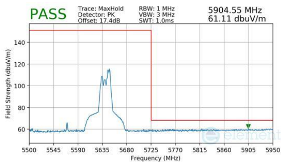
Plot 7-958. (FCC Only) CDD Primary (Peak, RU52, Index 52 (H), Ch.114, MCS11)
