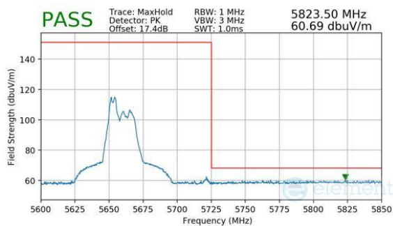
Plot 7-1054. CDD Diversity (Peak, RU52, Index 37, Ch.134, MCS11)
