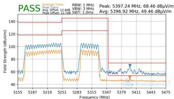
Plot 7-977. CDD Primary (Peak & Average, RU996+484+242, Index 94, Ch.50, MCS11)
