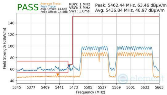
Plot 7-989. (FCC Only) CDD Primary (Peak & Average, RU996+484+242, Index 99 (L), Ch.114, MCS11)
