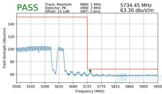
Plot 7-996. (FCC Only) CDD Primary (Peak, RU996+484+242, Index 98 (H), Ch.114, MCS11)
