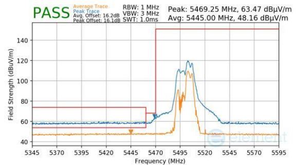
Plot 7-1020. CDD Diversity (Peak & Average, RU52+26, Index 72, Ch.100, MCS11)
