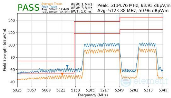
Plot 7-971. CDD Primary (Peak & Average, RU996+484+242, Index 94, Ch.50, MCS11)
