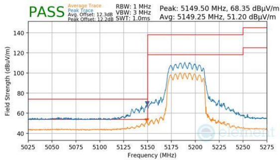
Plot 7-1056. CDD Diversity (Peak & Average, RU484, Index 65, Ch.38, MCS11)
