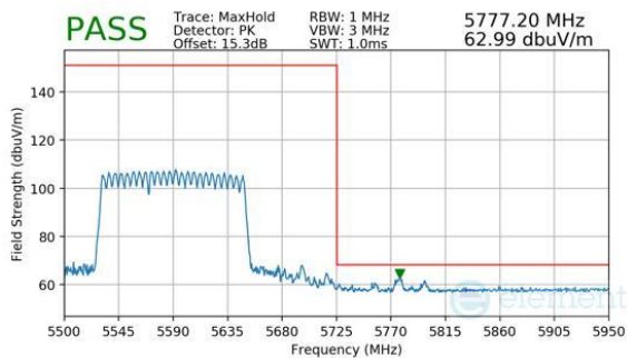
Plot 7-967. (FCC Only) CDD Primary (Peak, RU996+484, Index 94 (L), Ch.114, MCS11)
