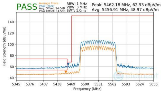
Plot 7-946. CDD Primary (Peak & Average, RU996, Index 67, Ch.106, MCS11)
