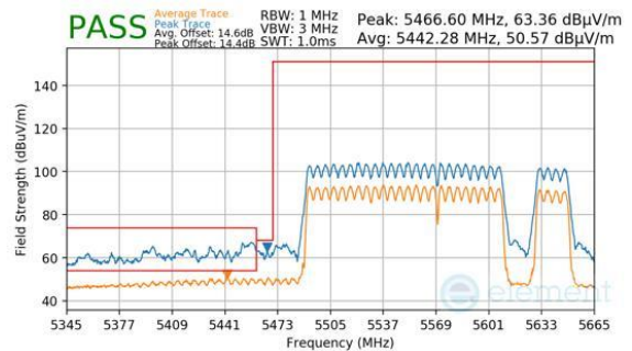
Plot 7-988. (FCC Only) CDD Primary (Peak & Average, RU996+484+242, Index 98 (H), Ch.114, MCS11)
