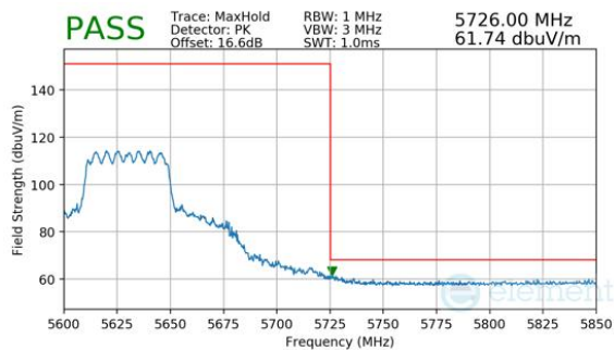
Plot 7-1062. (FCC Only) CDD Diversity (Peak, RU484, Index 65, Ch.126, MCS11)
