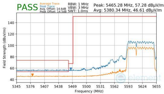
Plot 7-928. (FCC Only) CDD Primary (Peak & Average, RU484+242, Index 90, Ch.122, MCS11)
