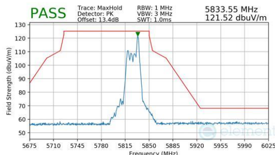
Plot 7-1008. CDD Diversity (Peak, RU26, Index 8, Ch.165, MCS11)
