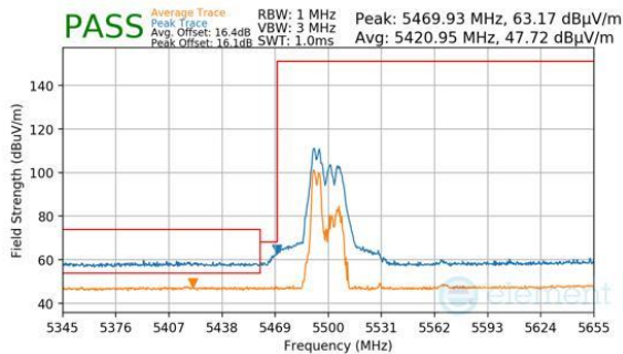
Plot 7-912. CDD Primary (Peak & Average, RU52, Index 37, Ch.106, MCS11)
