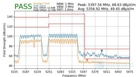
Plot 7-982. CDD Primary (Peak & Average, RU996+484+242, Index 99, Ch.50, MCS11)
