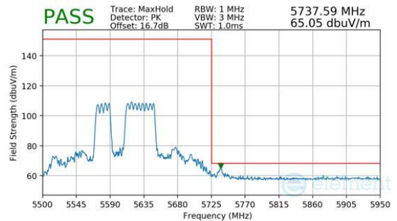
Plot 7-933. (FCC Only) CDD Primary (Peak, RU484+242, Index 91, Ch.122, MCS11)
