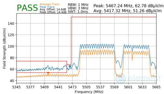
Plot 7-984. (FCC Only) CDD Primary (Peak & Average, RU996+484+242, Index 96 (H), Ch.114, MCS11)
