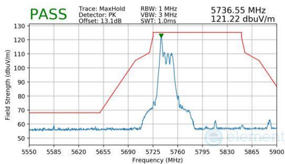
Plot 7-906. CDD Primary (Peak, RU26, Index 0, Ch.155, MCS11)
