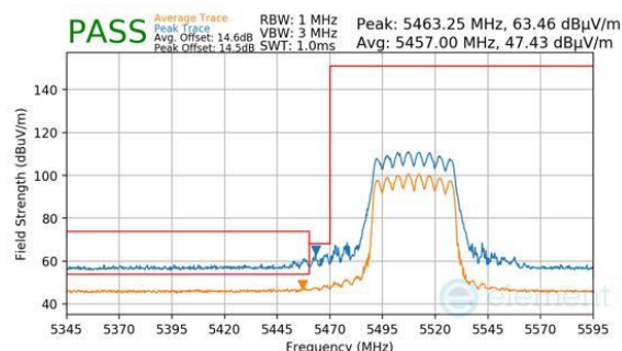
Plot 7-898. CDD Primary (Peak & Average, RU484, Index 65, Ch.102, MCS11)
