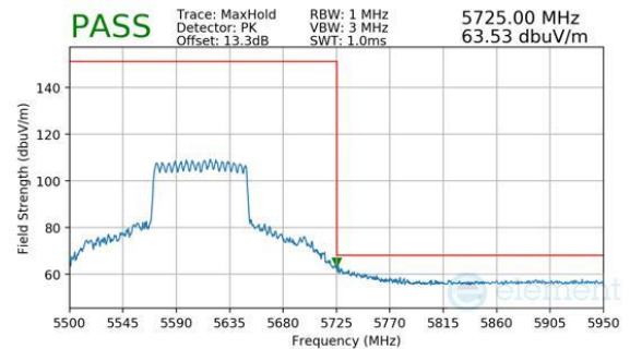
Plot 7-948. (FCC Only) CDD Primary (Peak, RU996, Index 67, Ch.122, MCS11)
