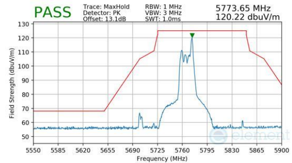
Plot 7-1045. CDD Diversity (Peak, RU26, Index 17, Ch.151, MCS11)
