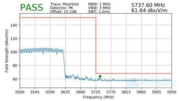
Plot 7-998. (FCC Only) CDD Primary (Peak, RU996+484+242, Index 99 (H), Ch.114, MCS11)
