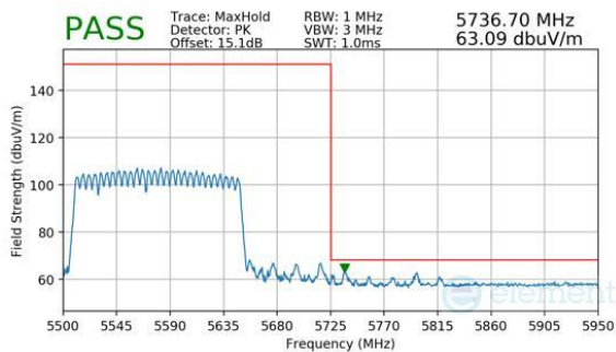
Plot 7-991. (FCC Only) CDD Primary (Peak, RU996+484+242, Index 96 (L), Ch.114, MCS11)
