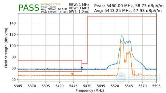
Plot 7-1052. CDD Diversity (Peak & Average, RU52, Index 37, Ch.110, MCS11)
