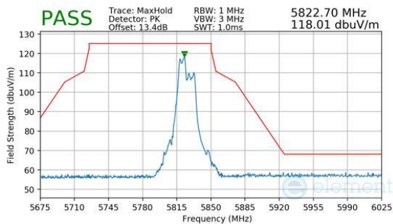
Plot 7-1029. CDD Diversity (Peak, RU52+26, Index 70, Ch.165, MCS11)
