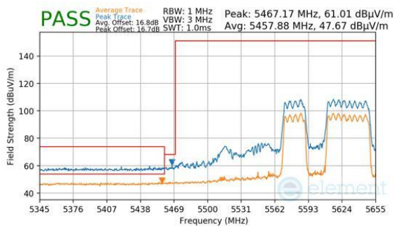
Plot 7-929. (FCC Only) CDD Primary (Peak & Average, RU484+242, Index 91, Ch.122, MCS11)
