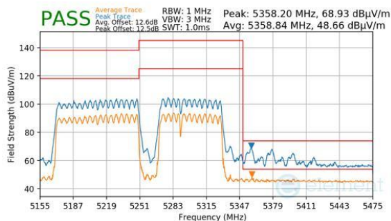
Plot 7-979. CDD Primary (Peak & Average, RU996+484+242, Index 96, Ch.50, MCS11)
