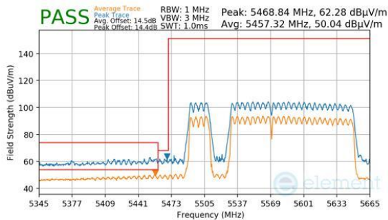
Plot 7-985. (FCC Only) CDD Primary (Peak & Average, RU996+484+242, Index 97 (L), Ch.114, MCS11)
