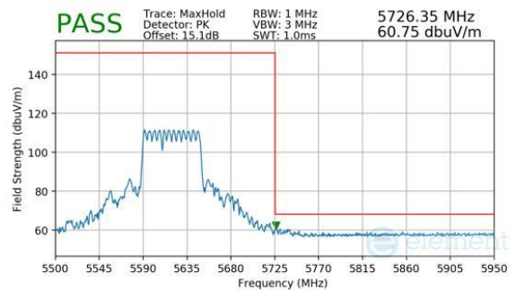
Plot 7-932. (FCC Only) CDD Primary (Peak, RU484+242, Index 90, Ch.122, MCS11)
