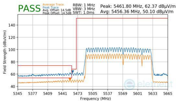
Plot 7-990. (FCC Only) CDD Primary (Peak & Average, RU996+484+242, Index 99 (H), Ch.114, MCS11)
