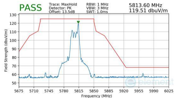
Plot 7-909. CDD Primary (Peak, RU26, Index 36, Ch.155, MCS11)
