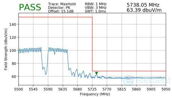
Plot 7-992. (FCC Only) CDD Primary (Peak, RU996+484+242, Index 96 (H), Ch.114, MCS11)
