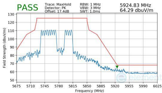
Plot 7-942. CDD Primary (Peak, RU484+242, Index 92, Ch.155, MCS11)
