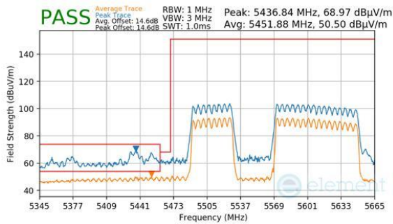
Plot 7-965. (FCC Only) CDD Primary (Peak & Average, RU996+484, Index 95 (L), Ch.114, MCS11)
