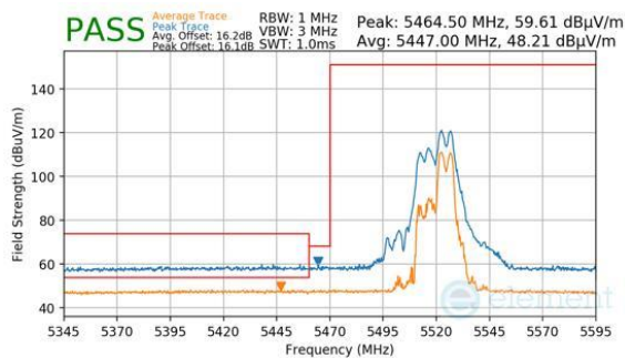
Plot 7-1022. CDD Diversity (Peak & Average, RU52+26, Index 72, Ch.104, MCS11)
