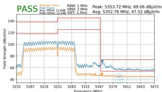
Plot 7-978. CDD Primary (Peak & Average, RU996+484+242, Index 95, Ch.50, MCS11)
