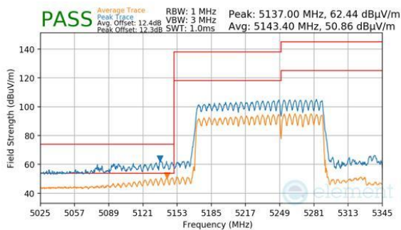
Plot 7-972. CDD Primary (Peak & Average, RU996+484+242, Index 95, Ch.50, MCS11)
