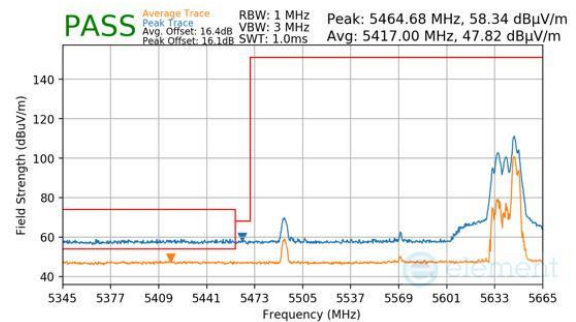
Plot 7-956. (FCC Only) CDD Primary (Peak & Average, RU52, Index 52 (H), Ch.114, MCS11)
