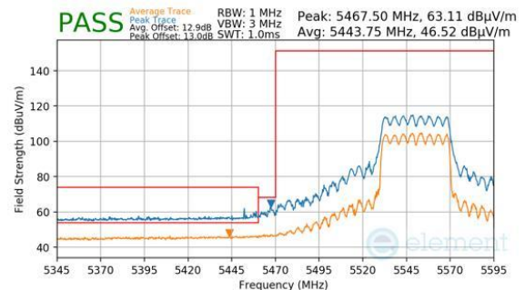
Plot 7-1061. CDD Diversity (Peak & Average, RU484, Index 65, Ch.110, MCS11)
