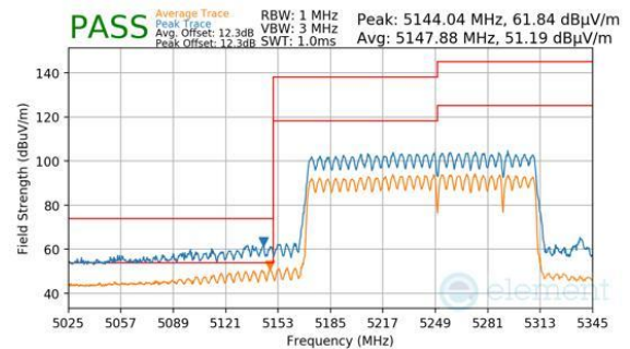
Plot 7-976. CDD Primary (Peak & Average, RU996+484+242, Index 99, Ch.50, MCS11)
