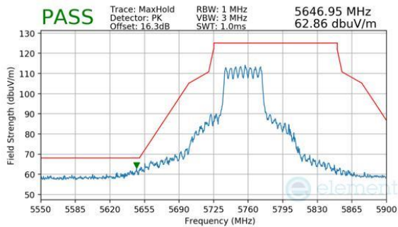
Plot 7-902. CDD Primary (Peak, RU484, Index 65, Ch.151, MCS11)
