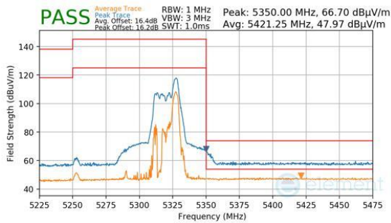
Plot 7-911. CDD Primary (Peak & Average, RU52, Index 52, Ch.58, MCS11)
