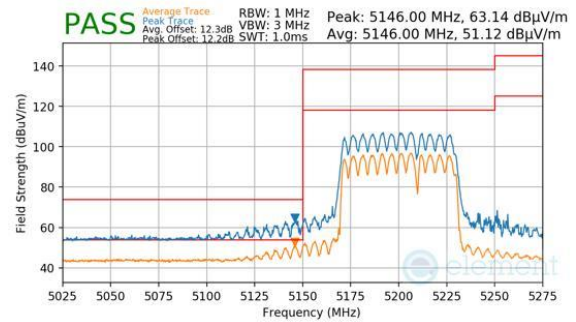
Plot 7-919. CDD Primary (Peak & Average, RU484+242, Index 93, Ch.42, MCS11)
