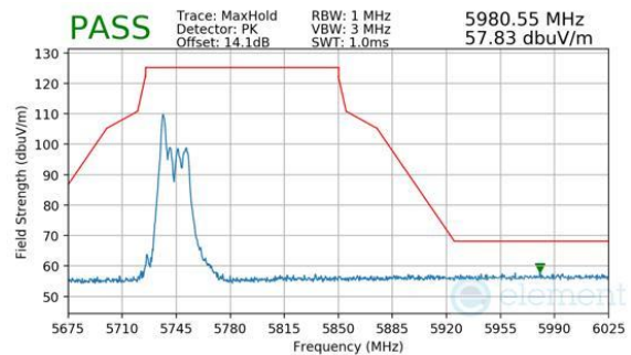
Plot 7-908. CDD Primary (Peak, RU26, Index 0, Ch.155, MCS11)
