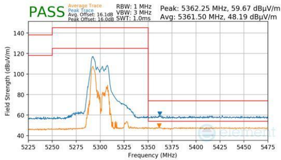
Plot 7-1048. CDD Diversity (Peak & Average, RU52, Index 37, Ch.62, MCS11)
