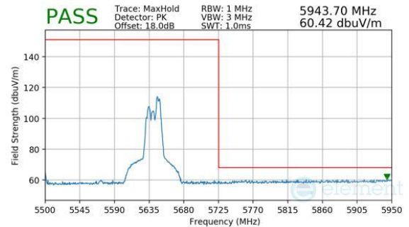
Plot 7-915. (FCC Only) CDD Primary (Peak, RU52, Index 52, Ch.122, MCS11)
