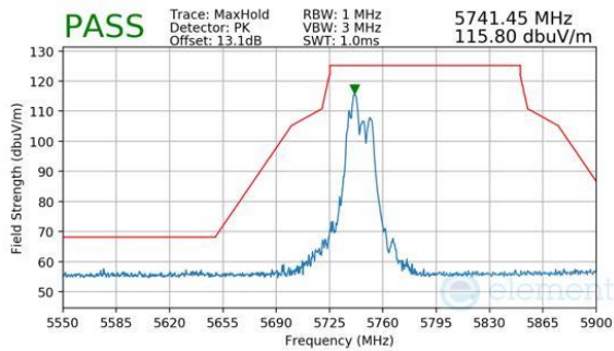
Plot 7-1027. CDD Diversity (Peak, RU52+26, Index 70, Ch.149, MCS11)
