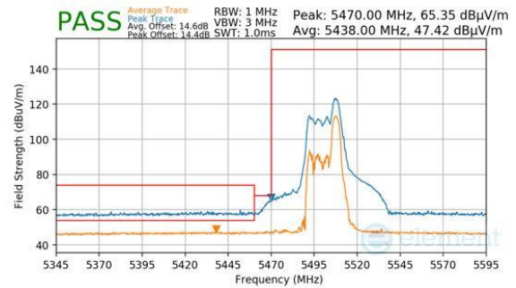
Plot 7-1051. CDD Diversity (Peak & Average, RU52, Index 40, Ch.102, MCS11)
