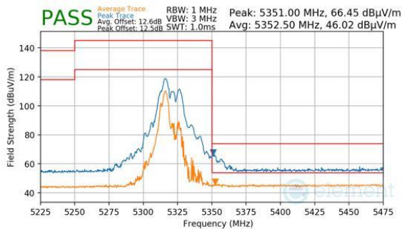
Plot 7-1017. CDD Diversity (Peak & Average, RU52+26, Index 70, Ch.64, MCS11)
