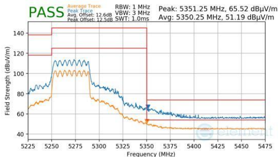
Plot 7-1058. CDD Diversity (Peak & Average, RU484, Index 65, Ch.54, MCS11)
