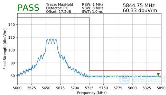
Plot 7-1037. CDD Diversity (Peak, RU242, Index 61, Ch.132, MCS11)
