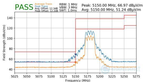
Plot 7-1031. CDD Diversity (Peak & Average, RU242, Index 61, Ch.36, MCS11)
