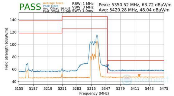
Plot 7-954. CDD Primary (Peak & Average, RU52, Index 52 (H), Ch.50, MCS11)
