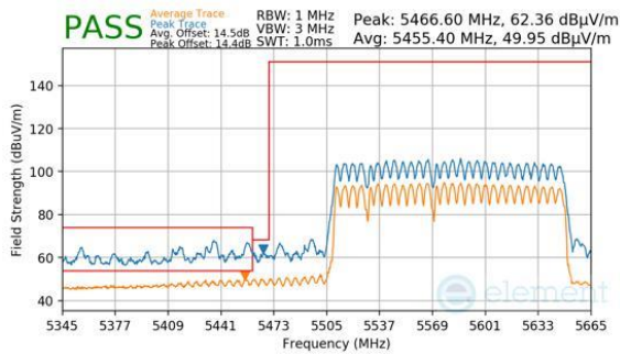
Plot 7-983. (FCC Only) CDD Primary (Peak & Average, RU996+484+242, Index 96 (L), Ch.114, MCS11)
