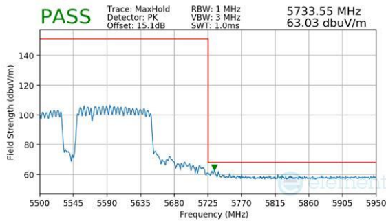
Plot 7-995. (FCC Only) CDD Primary (Peak, RU996+484+242, Index 98 (L), Ch.114, MCS11)
