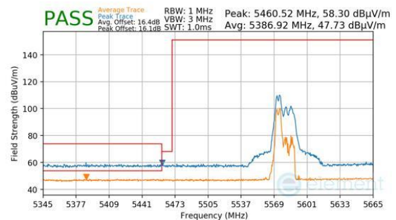
Plot 7-955. (FCC Only) CDD Primary (Peak & Average, RU52, Index 37, Ch.114, MCS11)
