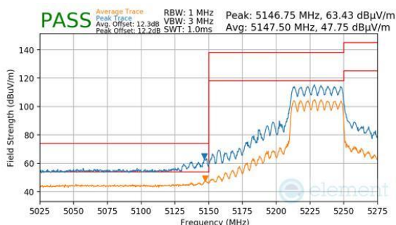
Plot 7-895. CDD Primary (Peak & Average, RU484, Index 65, Ch.46, MCS11)
