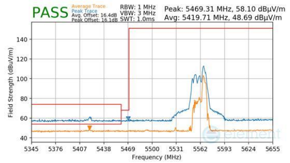
Plot 7-913. CDD Primary (Peak & Average, RU52, Index 52, Ch.106, MCS11)
