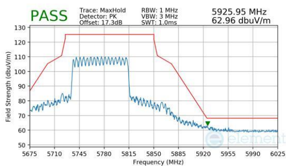
Plot 7-950. CDD Primary (Peak, RU996, Index 67, Ch.155, MCS11)
