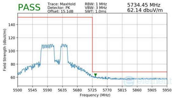
Plot 7-934. (FCC Only) CDD Primary (Peak, RU484+242, Index 92, Ch.122, MCS11)
