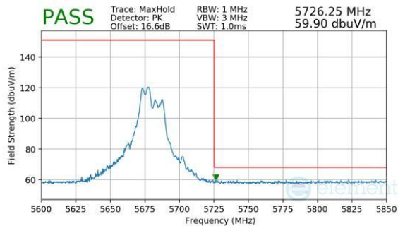
Plot 7-1023. CDD Diversity (Peak, RU52+26, Index 70, Ch.136, MCS11)
