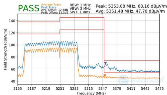
Plot 7-962. CDD Primary (Peak & Average, RU996+484, Index 95, Ch.50. MCS11)
