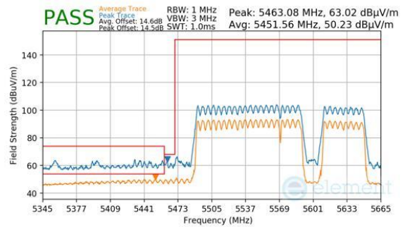
Plot 7-986. (FCC Only) CDD Primary (Peak & Average, RU996+484+242, Index 97 (H), Ch.114, MCS11)
