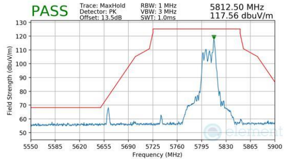
Plot 7-907. CDD Primary (Peak, RU26, Index 36, Ch.155, MCS11)
