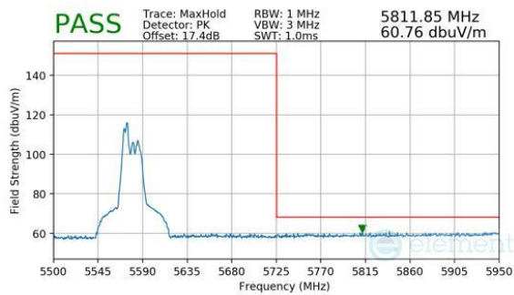
Plot 7-957. (FCC Only) CDD Primary (Peak, RU52, Index 37, Ch.114, MCS11)
