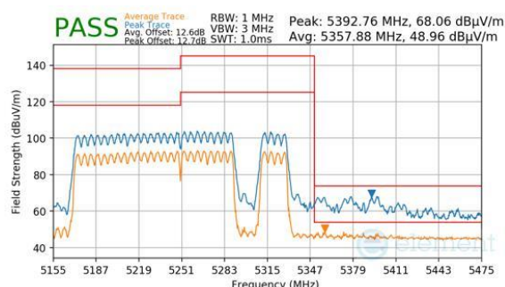
Plot 7-981. CDD Primary (Peak & Average, RU996+484+242, Index 98, Ch.50, MCS11)
