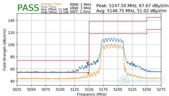
Plot 7-894. CDD Primary (Peak & Average, RU484, Index 65, Ch.38, MCS11)
