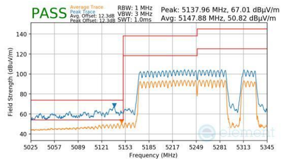
Plot 7-975. CDD Primary (Peak & Average, RU996+484+242, Index 98, Ch.50, MCS11)
