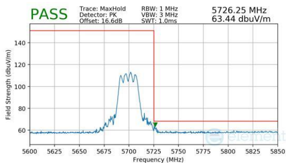
Plot 7-1039. CDD Diversity (Peak, RU242, Index 61, Ch.140, MCS11)
