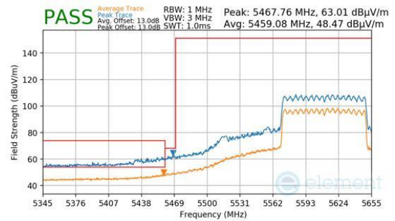
Plot 7-947. (FCC Only) CDD Primary (Peak & Average, RU996, Index 67, Ch.122, MCS11)
