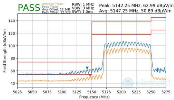
Plot 7-944. CDD Primary (Peak & Average, RU996, Index 67, Ch.42, MCS11)
