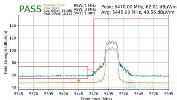
Plot 7-1035. CDD Diversity (Peak & Average, RU242, Index 61, Ch.100, MCS11)
