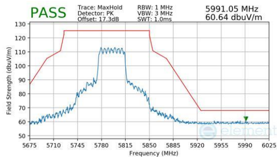
Plot 7-1065. CDD Diversity (Peak, RU484, Index 65, Ch.159, MCS11)
