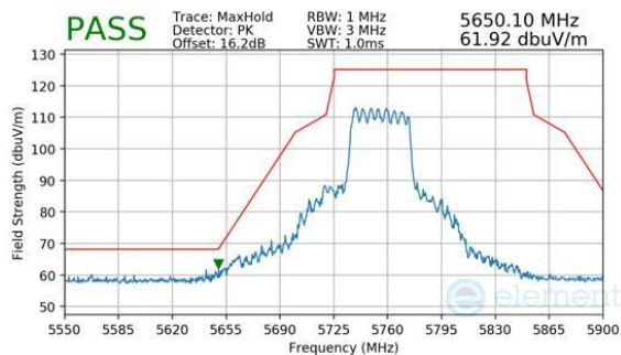
Plot 7-1064. CDD Diversity (Peak, RU484, Index 65, Ch.151, MCS11)
