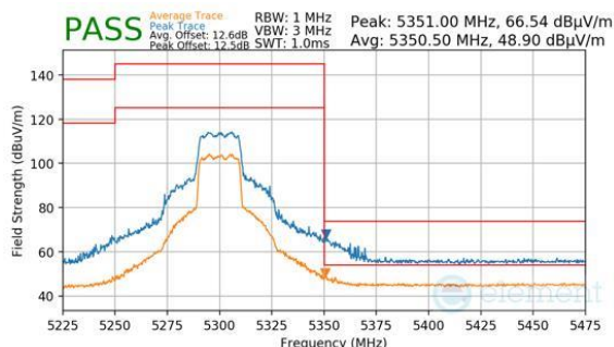
Plot 7-1033. CDD Diversity (Peak & Average, RU242, Index 61, Ch.60, MCS11)
