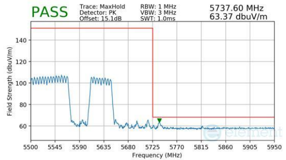
Plot 7-968. (FCC Only) CDD Primary (Peak, RU996+484, Index 94 (H), Ch.114, MCS11)
