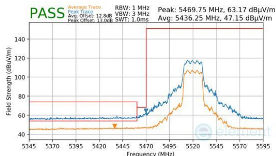
Plot 7-1036. CDD Diversity (Peak & Average, RU242, Index 61, Ch.104, MCS11)
