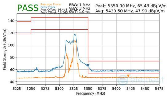
Plot 7-1049. CDD Diversity (Peak & Average, RU52, Index 44, Ch.62, MCS11)
