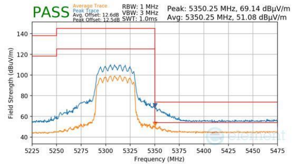
Plot 7-1059. CDD Diversity (Peak & Average, RU484, Index 65, Ch.62, MCS11)
