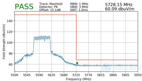
Plot 7-935. (FCC Only) CDD Primary (Peak, RU484+242, Index 93, Ch.122, MCS11)
