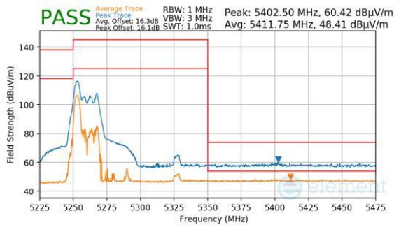
Plot 7-910. CDD Primary (Peak & Average, RU52, Index 37, Ch.58, MCS11)
