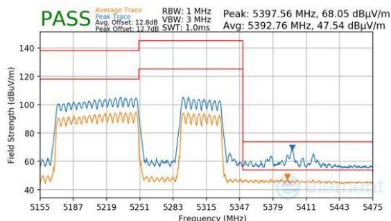
Plot 7-961. CDD Primary (Peak & Average, RU996+484, Index 94, Ch.50, MCS11)
