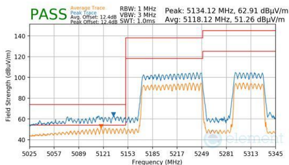
Plot 7-959. CDD Primary (Peak & Average, RU996+484, Index 94, Ch.50. MCS11)
