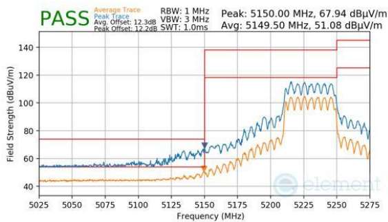
Plot 7-1057. CDD Diversity (Peak & Average, RU484, Index 65, Ch.46, MCS11)
