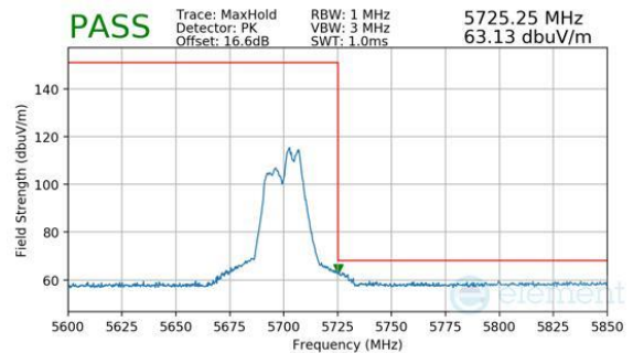
Plot 7-1026. CDD Diversity (Peak, RU52+26, Index 72, Ch.140, MCS11)
