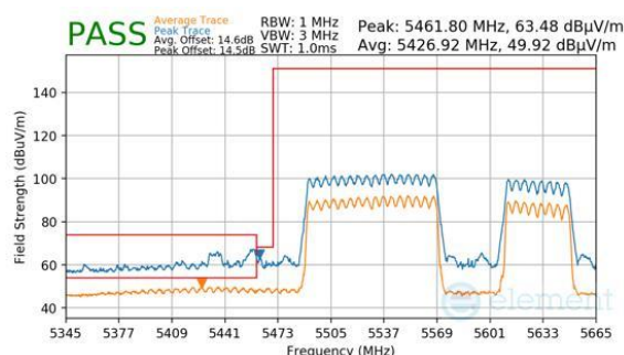
Plot 7-963. (FCC Only) CDD Primary (Peak & Average, RU996+484, Index 94 (H), Ch.114, MCS11)
