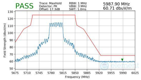
Plot 7-903. CDD Primary (Peak, RU484, Index 65, Ch.159, MCS11)
