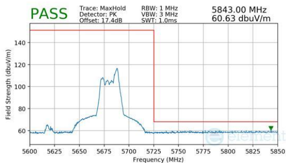
Plot 7-1055. CDD Diversity (Peak, RU52, Index 44, Ch.134, MCS11)
