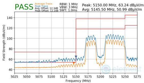
Plot 7-917. CDD Primary (Peak & Average, RU484+242, Index 91, Ch.42, MCS11)
