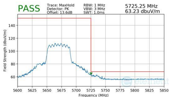
Plot 7-1063. CDD Diversity (Peak, RU484, Index 65, Ch.134, MCS11)
