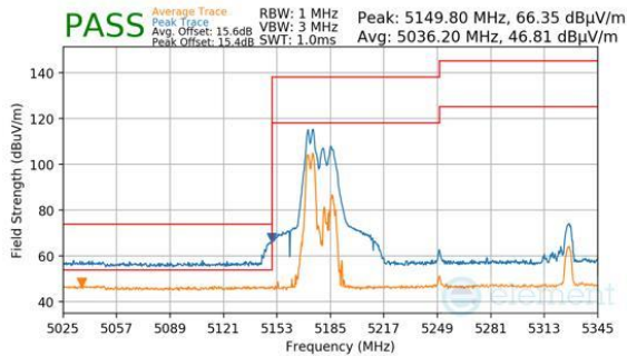
Plot 7-951. CDD Primary (Peak & Average, RU52, Index 37, Ch.50, MCS11)
