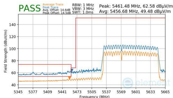
Plot 7-964. (FCC Only) CDD Primary (Peak & Average, RU996+484, Index 94 (L), Ch.114, MCS11)
