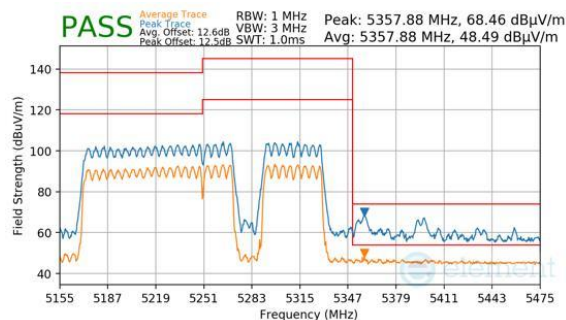
Plot 7-980. CDD Primary (Peak & Average, RU996+484+242, Index 97, Ch.50, MCS11)
