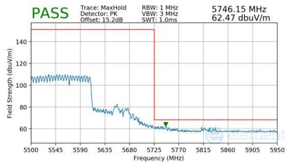
Plot 7-969. (FCC Only) CDD Primary (Peak, RU996+484, Index 95 (H), Ch.114, MCS11)
