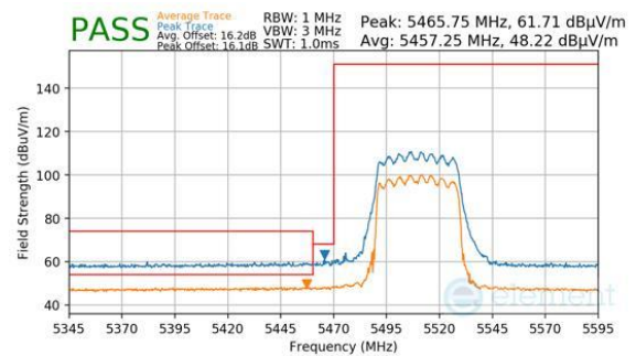
Plot 7-1060. CDD Diversity (Peak & Average, RU484, Index 65, Ch.102, MCS11)
