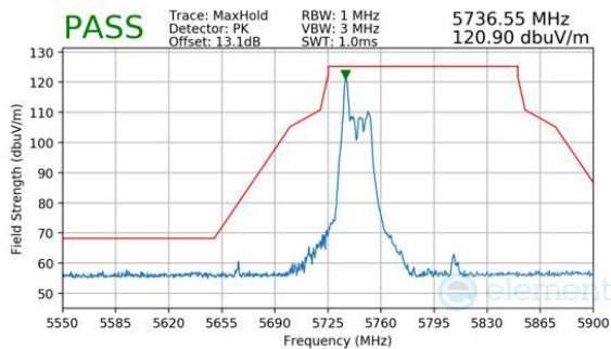
Plot 7-1044. CDD Diversity (Peak, RU26, Index 0, Ch.151, MCS11)
