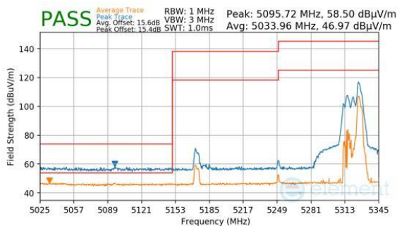
Plot 7-952. CDD Primary (Peak & Average, RU52, Index 52 (H), Ch.50, MCS11)
