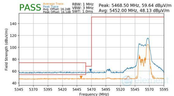
Plot 7-1053. CDD Diversity (Peak & Average, RU52, Index 44, Ch.110, MCS11)
