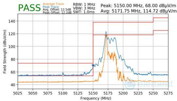
Plot 7-1042. CDD Diversity (Peak & Average, RU26, Index 0, Ch.38, MCS11)
