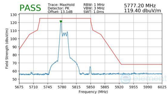
Plot 7-1046. CDD Diversity (Peak, RU26, Index 0, Ch.159, MCS11)
