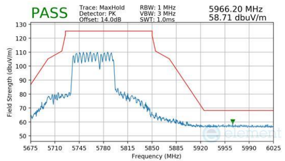
Plot 7-943. CDD Primary (Peak, RU484+242, Index 93, Ch.155, MCS11)
