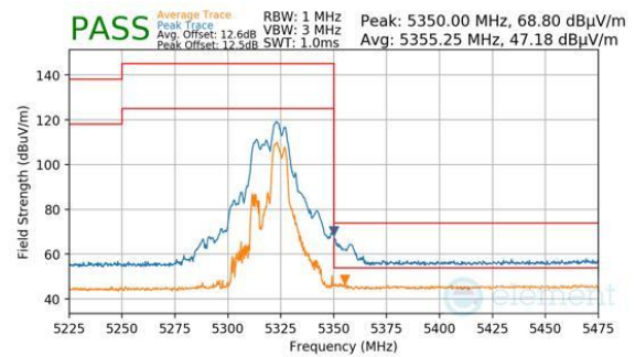
Plot 7-1018. CDD Diversity (Peak & Average, RU52+26, Index 72, Ch.64, MCS11)
