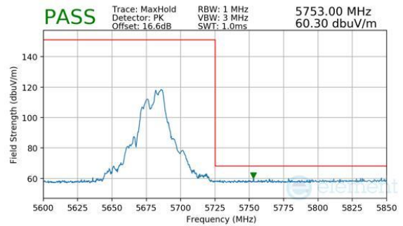
Plot 7-1024. CDD Diversity (Peak, RU52+26, Index 72, Ch.136, MCS11)
