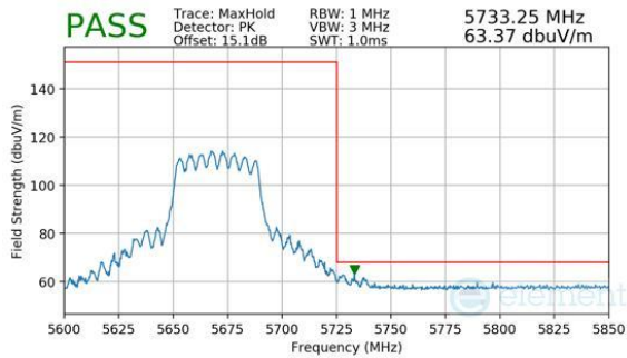
Plot 7-901. CDD Primary (Peak, RU484, Index 65, Ch.134, MCS11)
