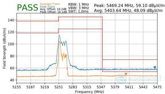
Plot 7-953. CDD Primary (Peak & Average, RU52, Index 37, Ch.50, MCS11)
