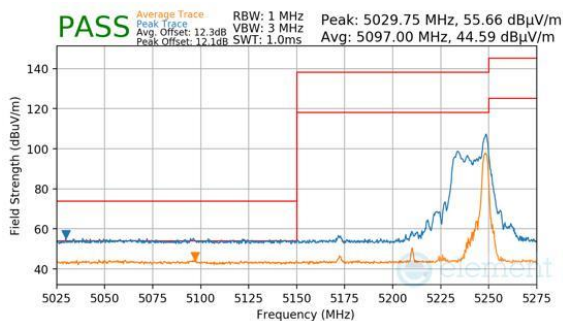
Plot 7-905. CDD Primary (Peak & Average, RU26, Index 36, Ch.42, MCS11)
