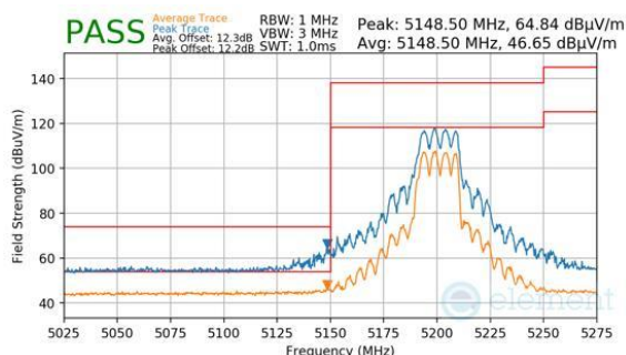
Plot 7-1032. CDD Diversity (Peak & Average, RU242, Index 61, Ch.40, MCS11)
