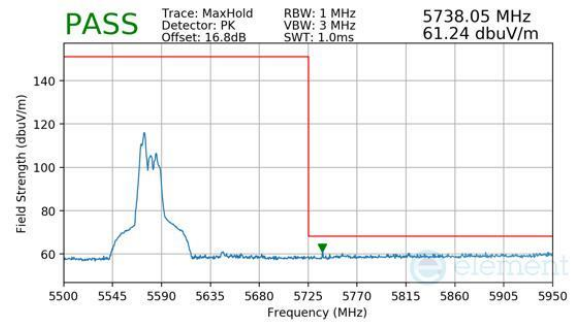
Plot 7-914. (FCC Only) CDD Primary (Peak, RU52, Index 37, Ch.122, MCS11)
