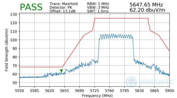
Plot 7-949. CDD Primary (Peak, RU996, Index 67, Ch.155, MCS11)
