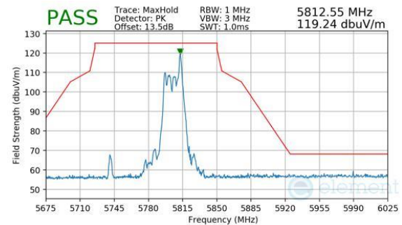
Plot 7-1047. CDD Diversity (Peak, RU26, Index 17, Ch.159, MCS11)
