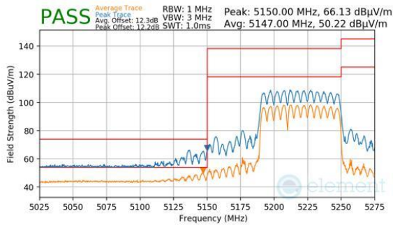
Plot 7-916. CDD Primary (Peak & Average, RU484+242, Index 90, Ch.42, MCS11)
