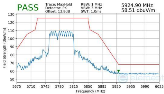
Plot 7-940. CDD Primary (Peak, RU484+242, Index 90, Ch.155, MCS11)
