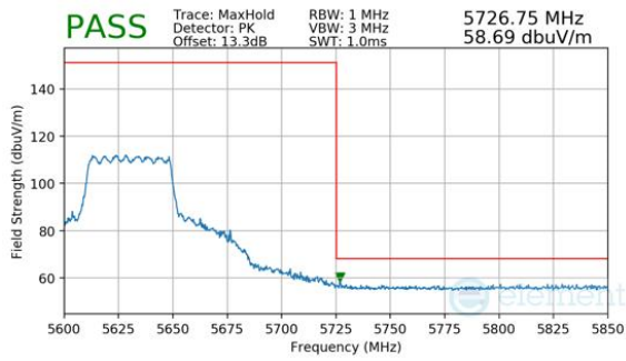
Plot 7-900. (FCC Only) CDD Primary (Peak, RU484, Index 65, Ch.126, MCS11)
