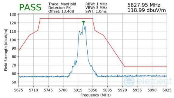
Plot 7-1030. CDD Diversity (Peak, RU52+26, Index 72, Ch.165, MCS11)
