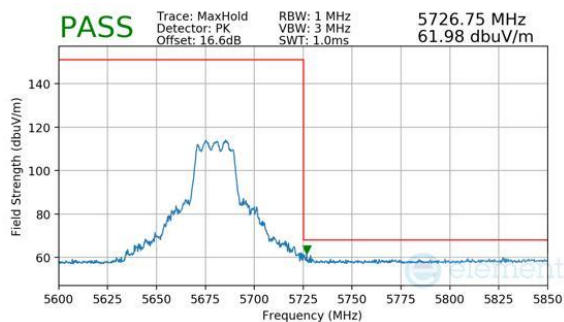
Plot 7-1038. CDD Diversity (Peak, RU242, Index 61, Ch.136, MCS11)
