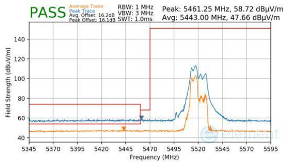
Plot 7-1021. CDD Diversity (Peak & Average, RU52+26, Index 70, Ch.104, MCS11)
