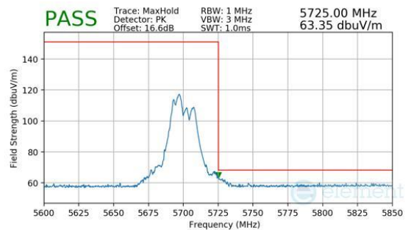
Plot 7-1025. CDD Diversity (Peak, RU52+26, Index 70, Ch.140, MCS11)
