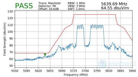
Plot 7-937. CDD Primary (Peak, RU484+242, Index 91, Ch.155, MCS11)
