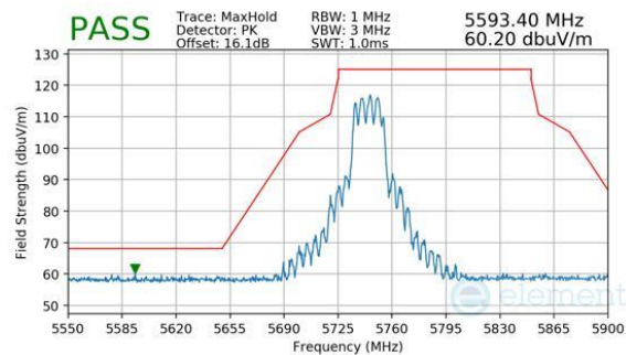
Plot 7-1040. CDD Diversity (Peak, RU242, Index 61, Ch.149, MCS11)
