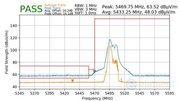
Plot 7-1019. CDD Diversity (Peak & Average, RU52+26, Index 70, Ch.100, MCS11)
