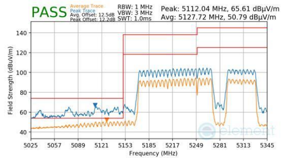
Plot 7-974. CDD Primary (Peak & Average, RU996+484+242, Index 97, Ch.50, MCS11)
