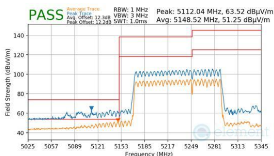
Plot 7-960. CDD Primary (Peak & Average, RU996+484, Index 95, Ch.50, MCS11)
