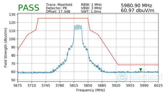
Plot 7-1041. CDD Diversity (Peak, RU242, Index 61, Ch.165, MCS11)
