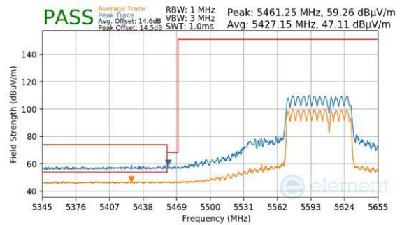
Plot 7-931. (FCC Only) CDD Primary (Peak & Average, RU484+242, Index 93, Ch.122, MCS11)
