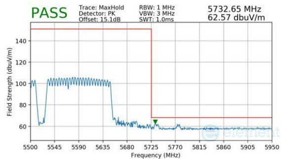
Plot 7-993. (FCC Only) CDD Primary (Peak, RU996+484+242, Index 97 (L), Ch.114, MCS11)
