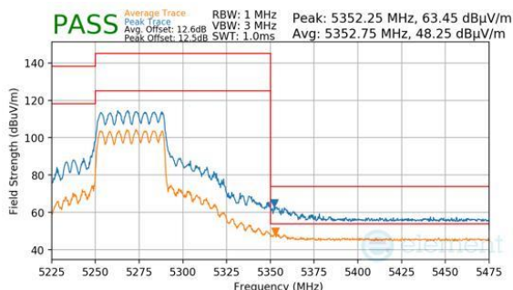
Plot 7-896. CDD Primary (Peak & Average, RU484, Index 65, Ch.54, MCS11)
