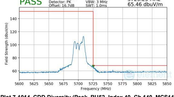
Plot 7-1014. CDD Diversity (Peak, RU52, Index 40, Ch.140, MCS11)
