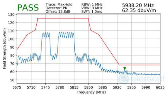
Plot 7-941. CDD Primary (Peak, RU484+242, Index 91, Ch.155, MCS11)
