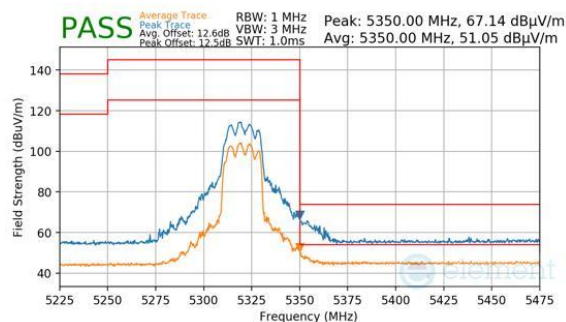
Plot 7-1034. CDD Diversity (Peak & Average, RU242, Index 61, Ch.64, MCS11)
