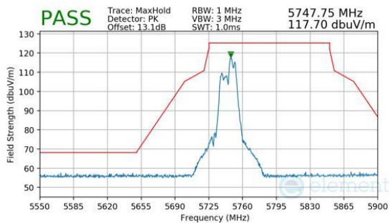
Plot 7-1028. CDD Diversity (Peak, RU52+26, Index 72, Ch.149, MCS11)
