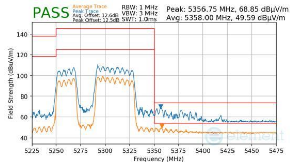
Plot 7-921. CDD Primary (Peak & Average, RU484+242, Index 91, Ch.58, MCS11)
