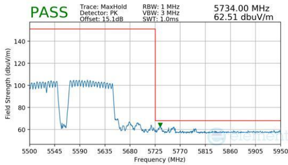
Plot 7-997. (FCC Only) CDD Primary (Peak, RU996+484+242, Index 99 (L), Ch.114, MCS11)
