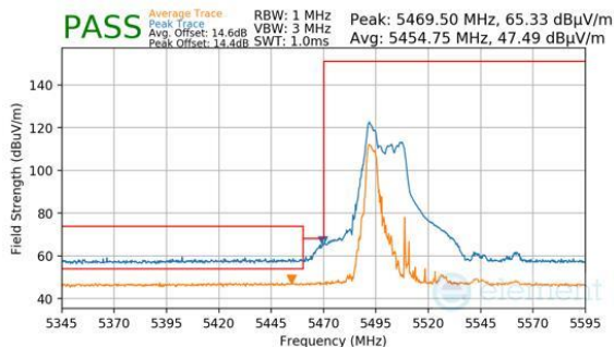
Plot 7-1050. CDD Diversity (Peak & Average, RU52, Index 37, Ch.102, MCS11)
