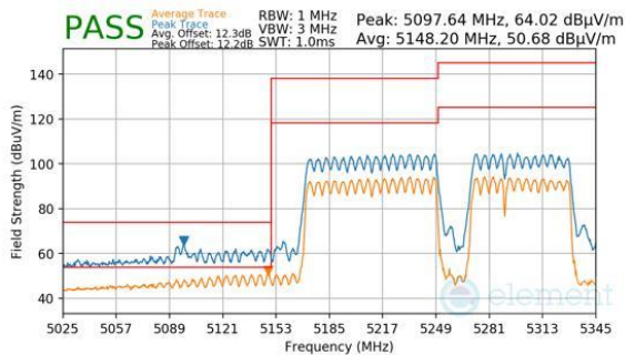
Plot 7-973. CDD Primary (Peak & Average, RU996+484+242, Index 96, Ch.50, MCS11)
