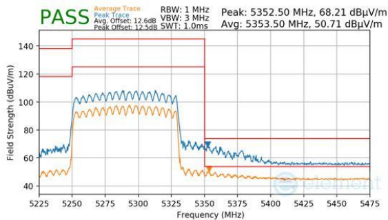
Plot 7-945. CDD Primary (Peak & Average, RU996, Index 67, Ch.58, MCS11)
