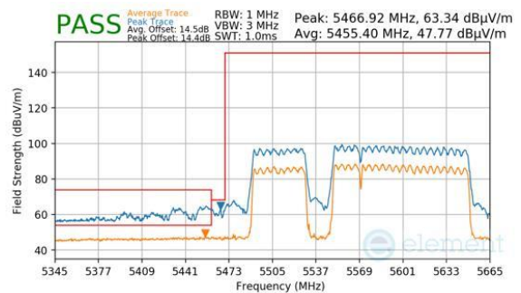
Plot 7-987. (FCC Only) CDD Primary (Peak & Average, RU996+484+242, Index 98 (L), Ch.114, MCS11)
