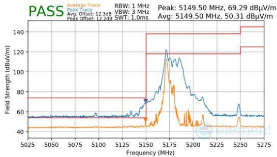
Plot 7-904. CDD Primary (Peak & Average, RU26, Index 0, Ch.42, MCS11)
