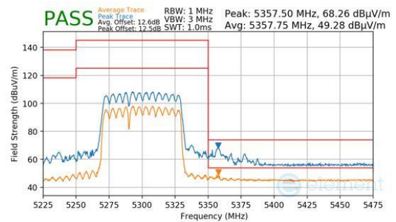
Plot 7-920. CDD Primary (Peak & Average, RU484+242, Index 90, Ch.58, MCS11)
