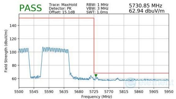
Plot 7-970. (FCC Only) CDD Primary (Peak, RU996+484, Index 95 (L), Ch.114, MCS11)
