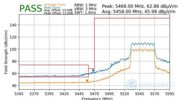
Plot 7-899. CDD Primary (Peak & Average, RU484, Index 65, Ch.110, MCS11)
