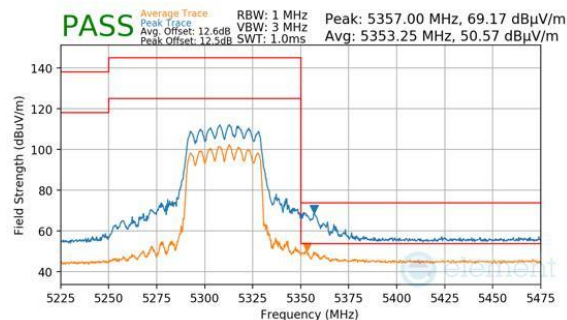
Plot 7-897. CDD Primary (Peak & Average, RU484, Index 65, Ch.62, MCS11)
