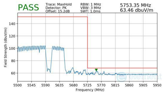
Plot 7-994. (FCC Only) CDD Primary (Peak, RU996+484+242, Index 97 (H), Ch.114, MCS11)
