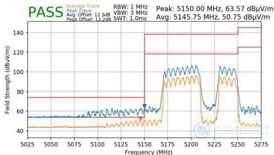
Plot 7-918. CDD Primary (Peak & Average, RU484+242, Index 92, Ch.42, MCS11)
