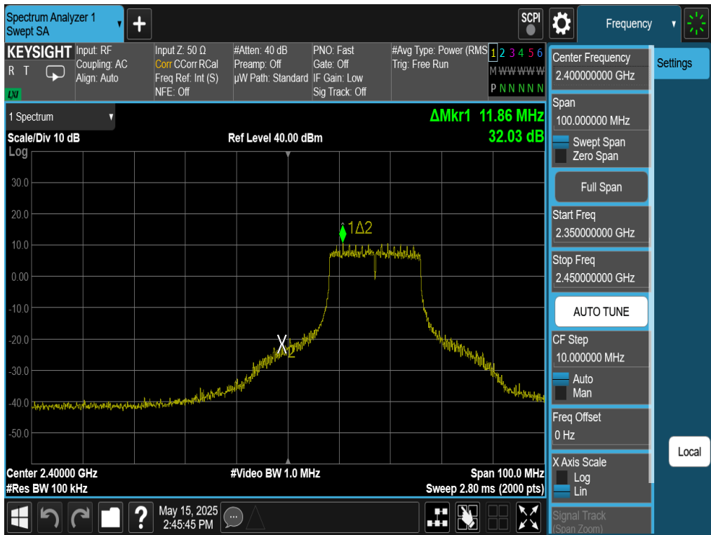
Plot 7-50. Band Edge Plot Antenna WF8 (802.11g – Ch. 2)
