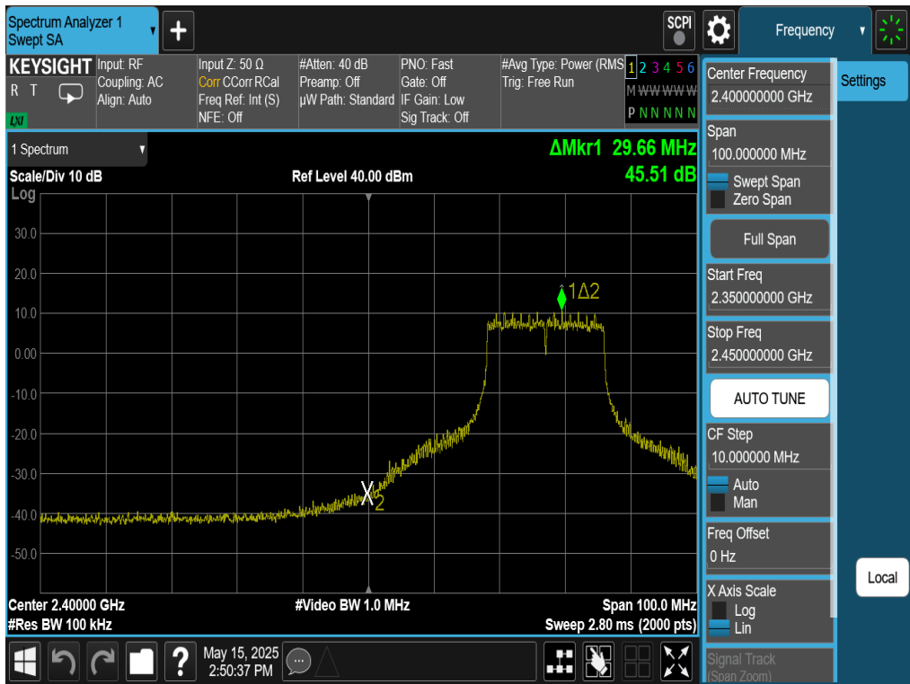
Plot 7-52. Band Edge Plot Antenna WF8 (802.11g – Ch. 4)
