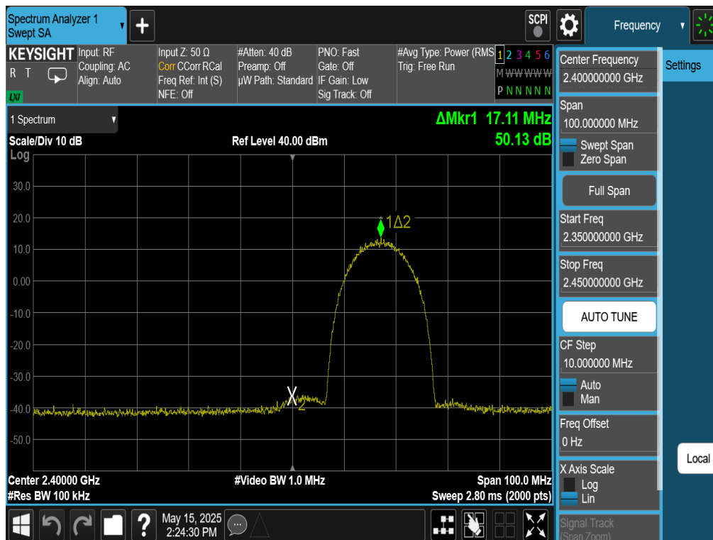
Plot 7-42. Band Edge Plot Antenna WF8 (802.11b – Ch. 2)
