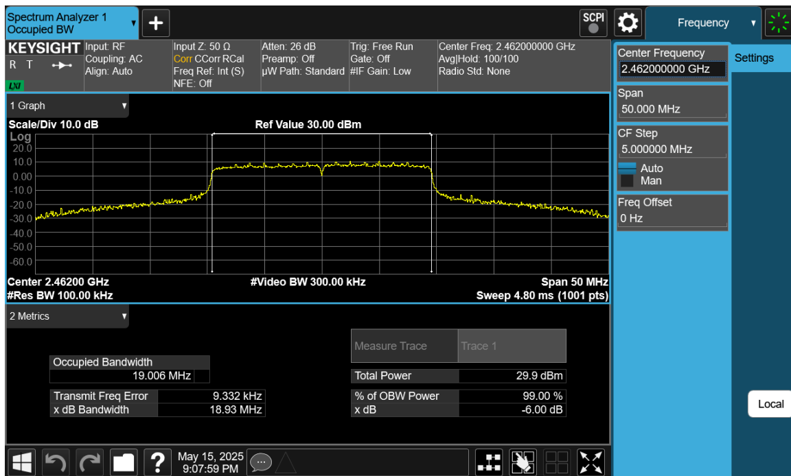
Plot 7-8 6dB BW & 99% OBW Antenna WF7 (20MHz BW 802.11be(SU) - Ch.11)
