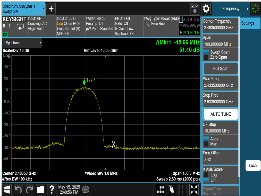
Plot 7-48. Band Edge Plot Antenna WF8 (802.11b – Ch. 13)
