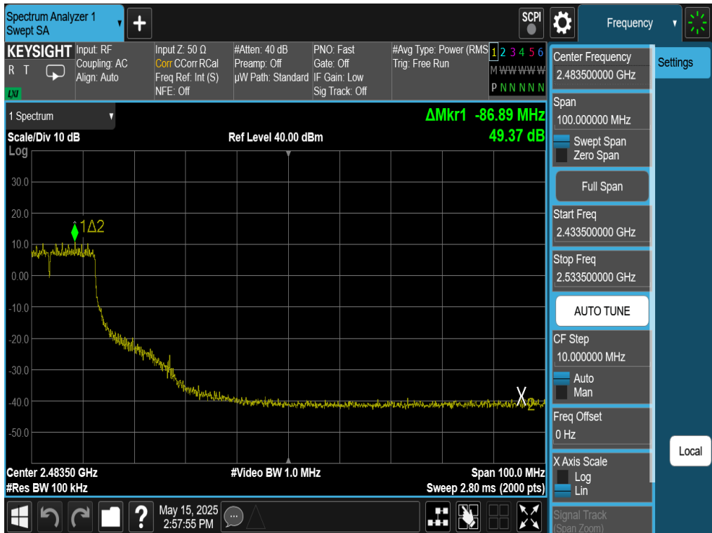
Plot 7-55. Band Edge Plot Antenna WF8 (802.11g – Ch. 6)
