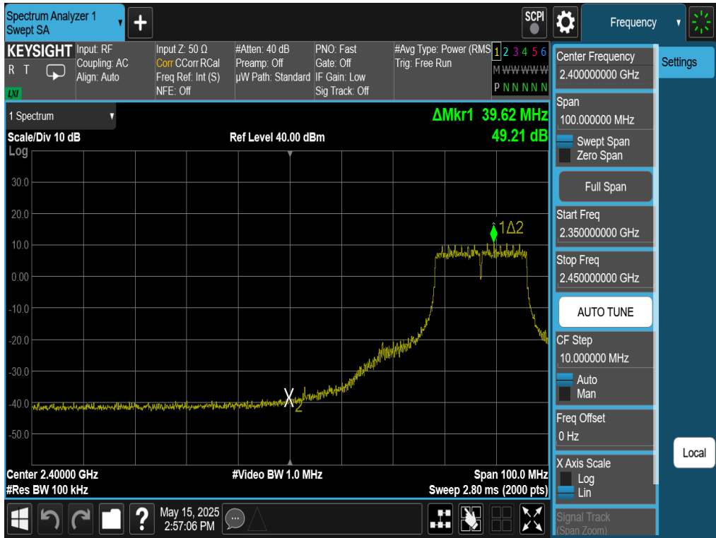
Plot 7-54. Band Edge Plot Antenna WF8 (802.11g – Ch. 6)
