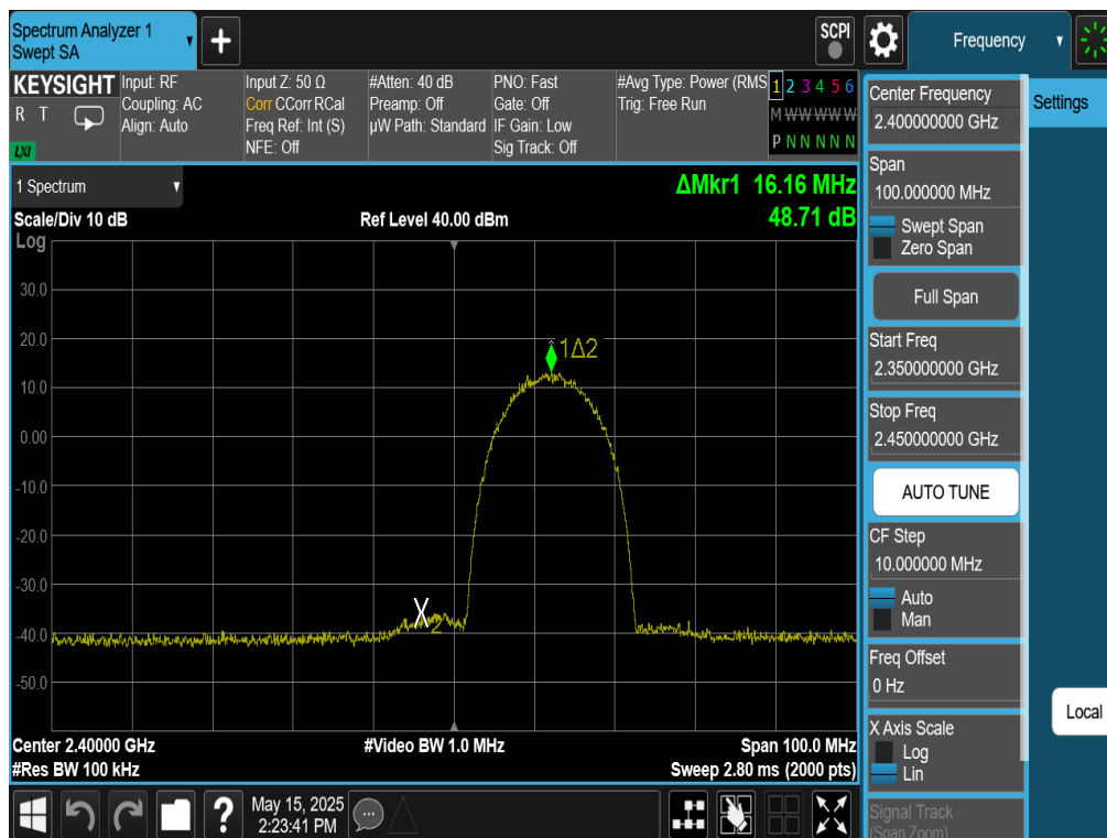
Plot 7-41. Band Edge Plot Antenna WF8 (802.11b – Ch. 1)
