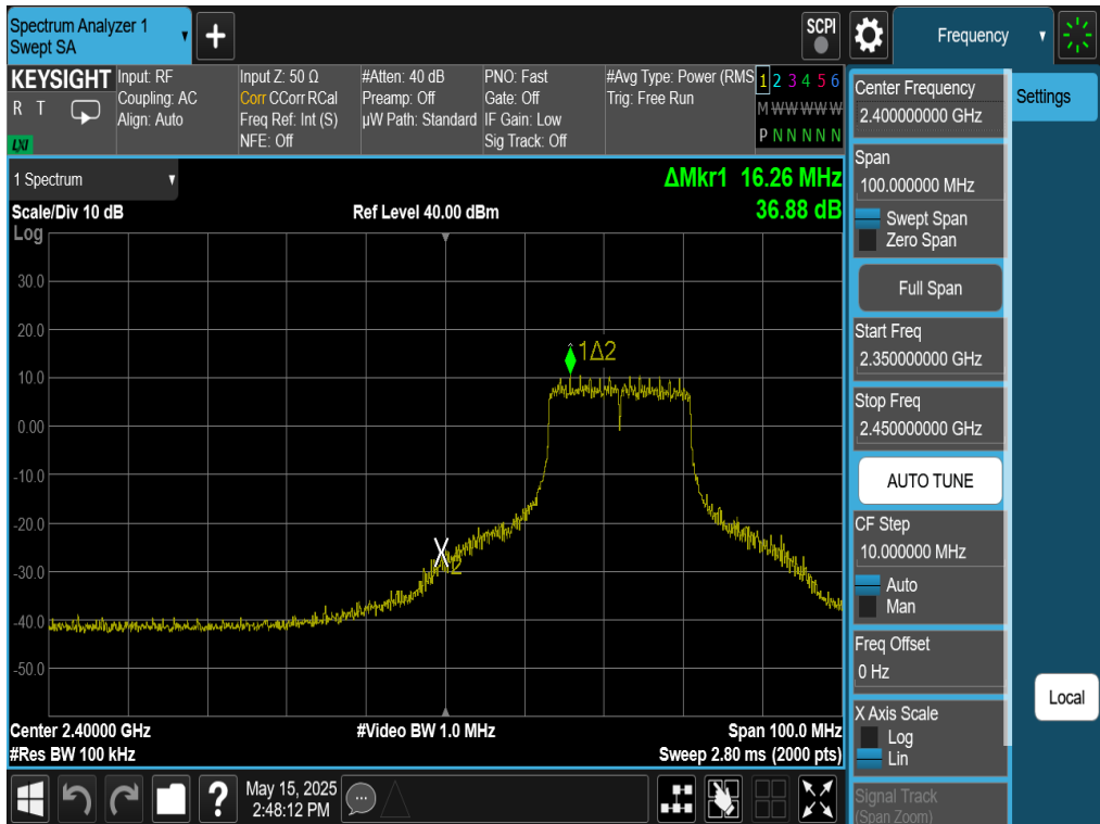
Plot 7-51. Band Edge Plot Antenna WF8 (802.11g – Ch. 3)
