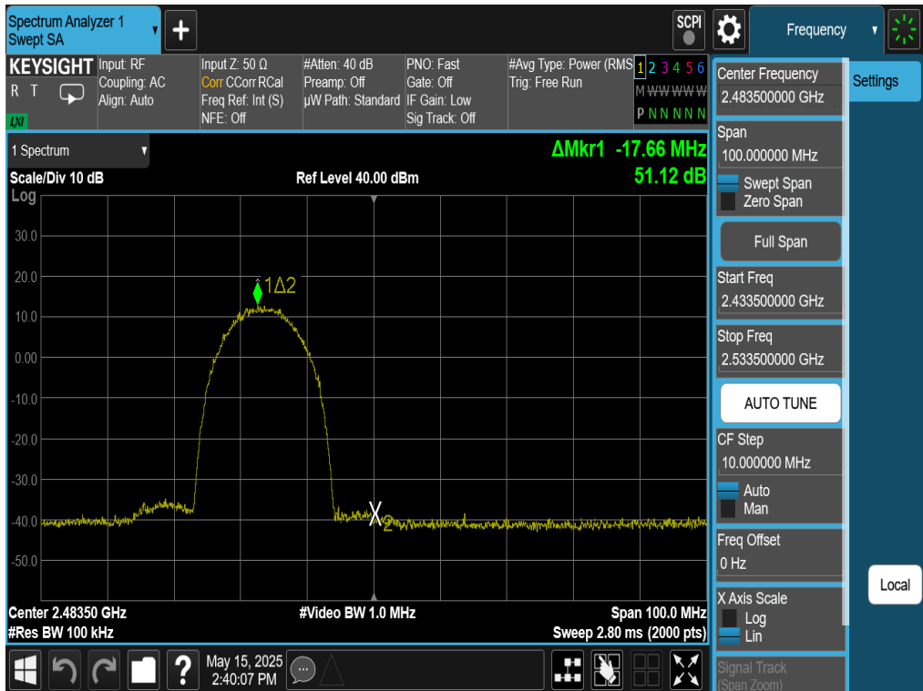
Plot 7-47. Band Edge Plot Antenna WF8 (802.11b – Ch. 12)
