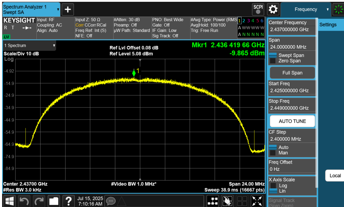
Plot 7-17 PSD Antenna WF7 (20MHz BW 802.11b - Ch.6)
