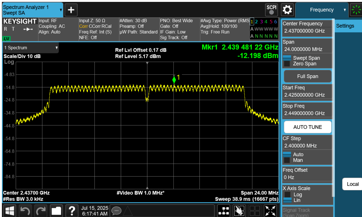
Plot 7-34 PSD CDD Diversity Antenna WF8 (20MHz BW 802.11g - Ch.6)
