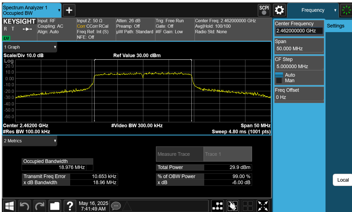
Plot 7-12 6dB BW & 99% OBW Antenna WF9 (20MHz BW 802.11be(SU) - Ch.11)
