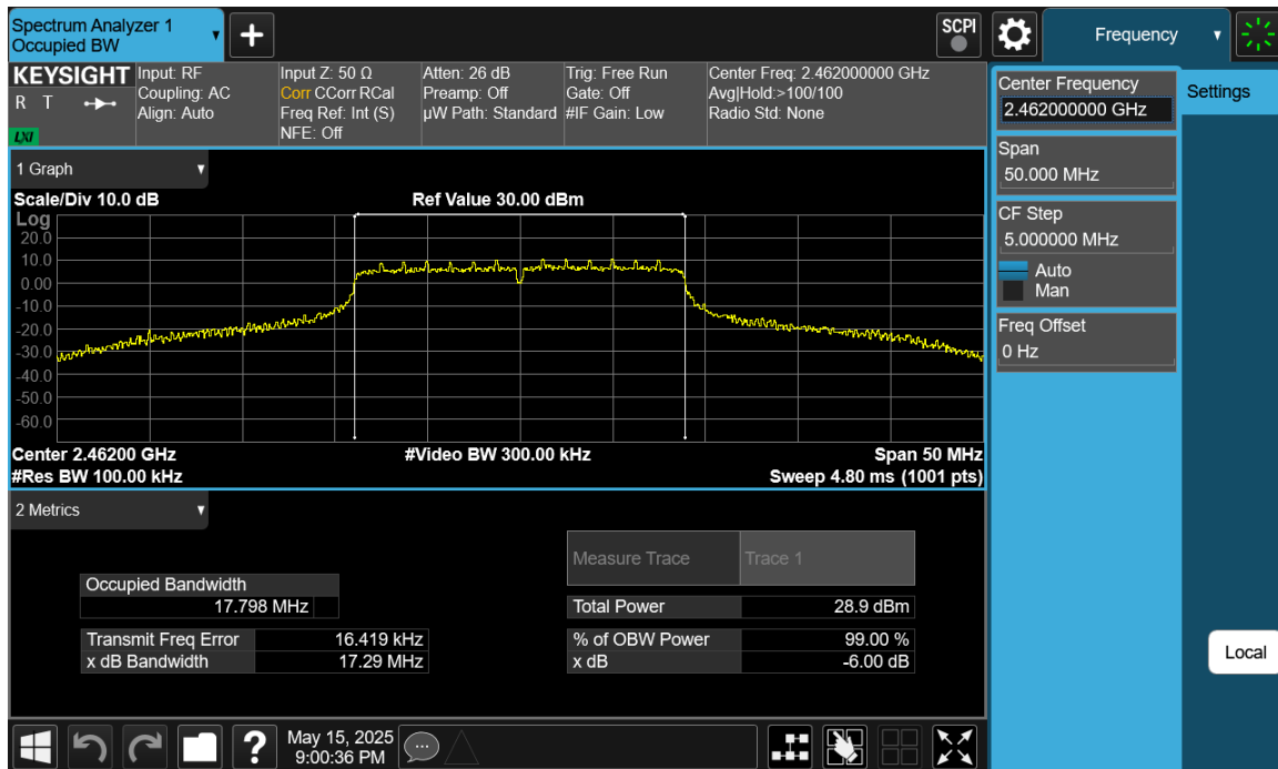
Plot 7-7 6dB BW & 99% OBW Antenna WF7 (20MHz BW 802.11n - Ch.11)
