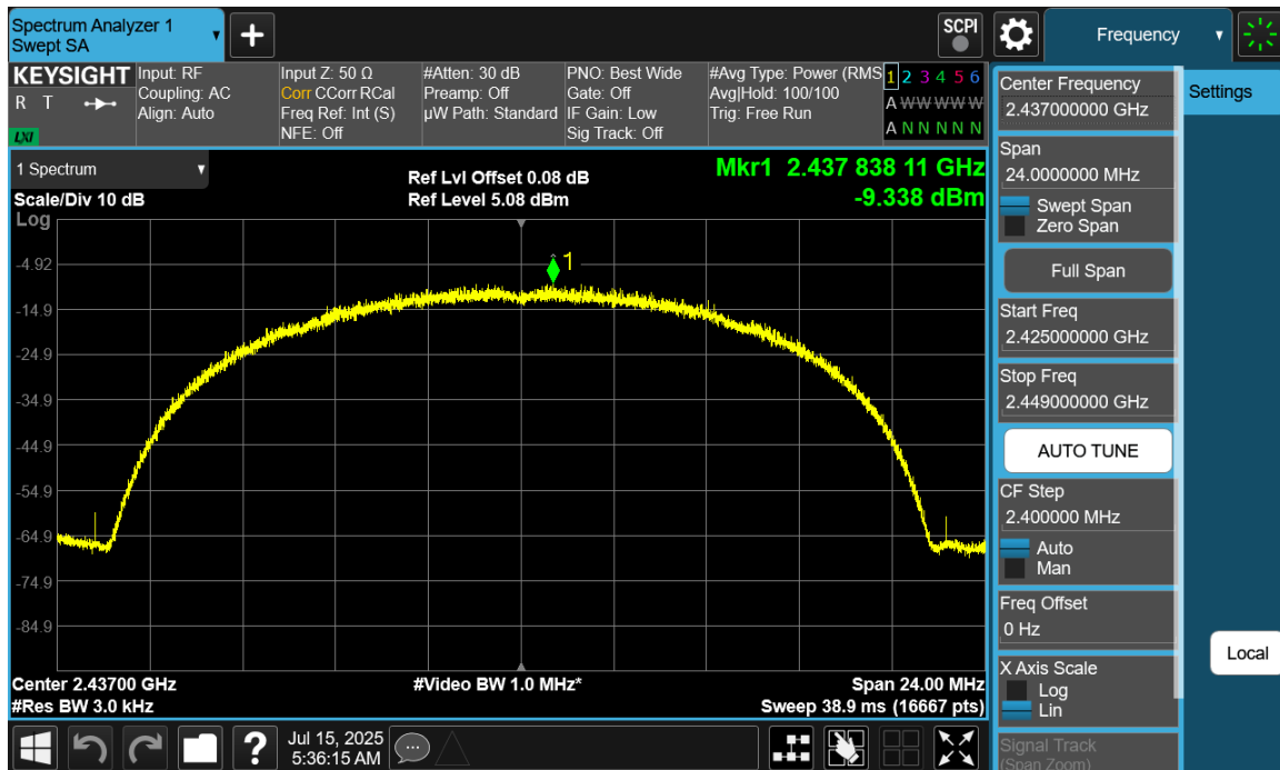
Plot 7-13 PSD Antenna WF8 (20MHz BW 802.11b - Ch.6)
