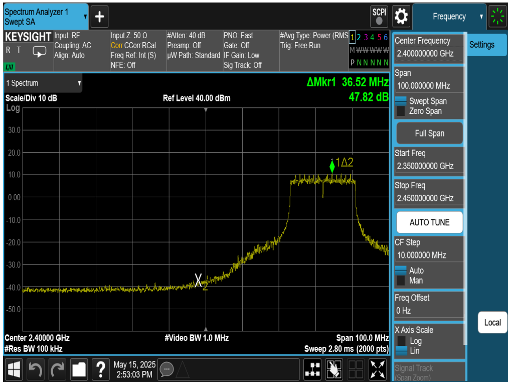
Plot 7-53. Band Edge Plot Antenna WF8 (802.11g – Ch. 5)
