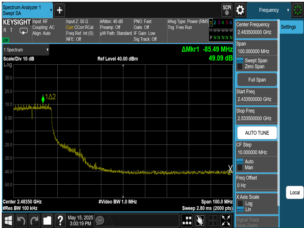
Plot 7-56. Band Edge Plot Antenna WF8 (802.11g – Ch. 7)
