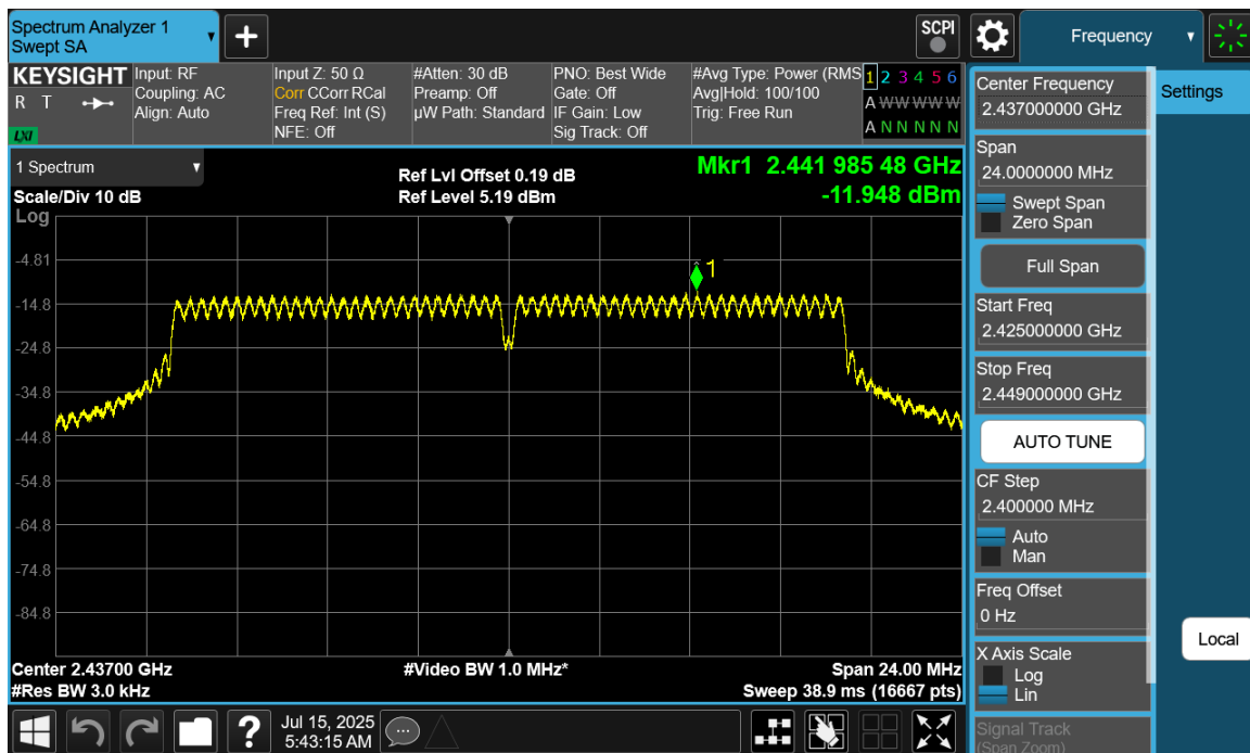
Plot 7-14 PSD Antenna WF8 (20MHz BW 802.11g - Ch.6)
