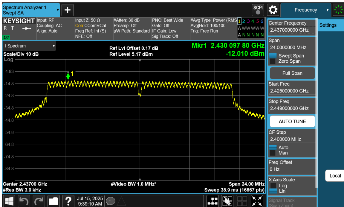
Plot 7-38 PSD CDD Diversity Antenna WF9 (20MHz BW 802.11g - Ch.6)
