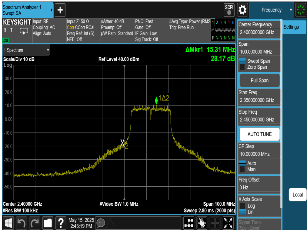
Plot 7-49. Band Edge Plot Antenna WF8 (802.11g – Ch. 1)
