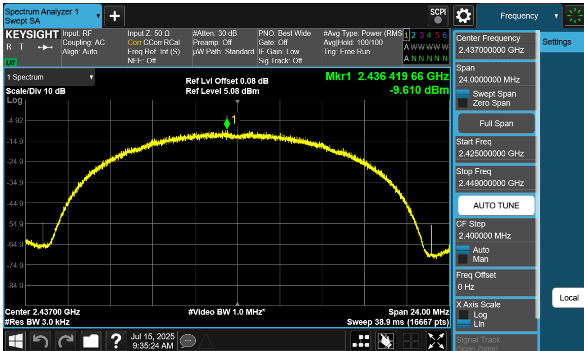
Plot 7-37 PSD CDD Diversity Antenna WF9 (20MHz BW 802.11b - Ch.6)
