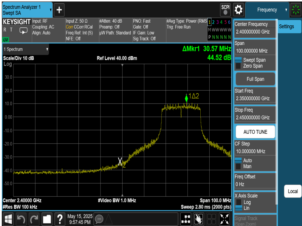
Plot 7-99. Band Edge Plot Antenna WF7 (802.11g – Ch. 4)
