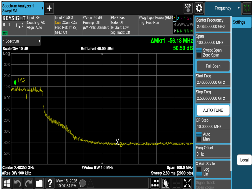
Plot 7-101. Band Edge Plot Antenna WF7 (802.11g – Ch. 7)
