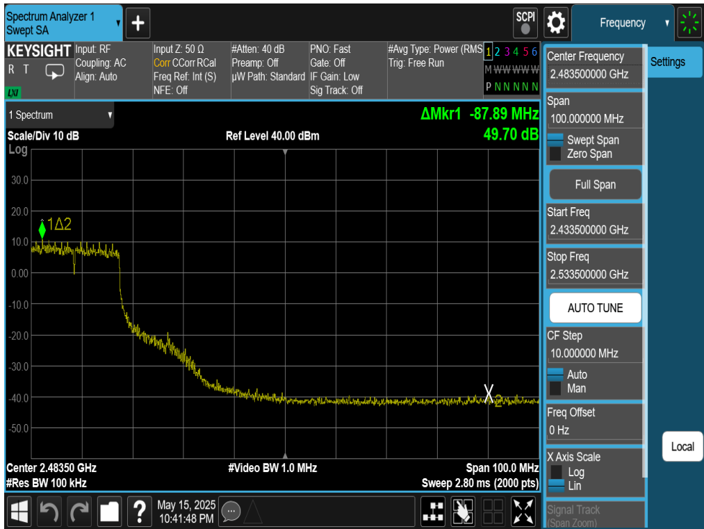
Plot 7-113. Band Edge Plot Antenna WF7 (802.11n (2.4GHz) – Ch. 7)
