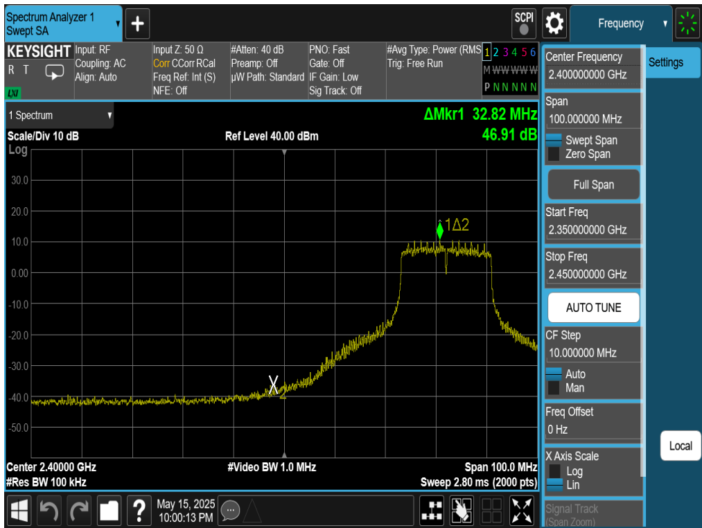
Plot 7-100. Band Edge Plot Antenna WF7 (802.11g – Ch. 5)
