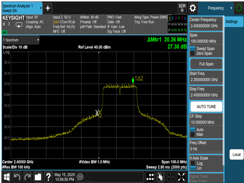
Plot 7-120. Band Edge Plot Antenna WF7 (802.11be (SU - 2.4GHz) – Ch. 1)
