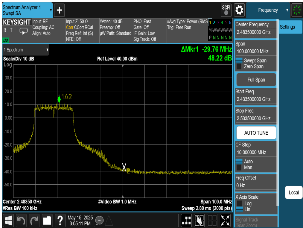
Plot 7-58. Band Edge Plot Antenna WF8 (802.11g – Ch. 9)
