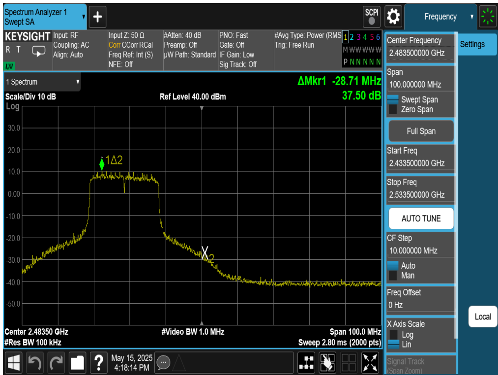
Plot 7-88. Band Edge Plot Antenna WF8 (802.11be (SU - 2.4GHz) – Ch. 11)
