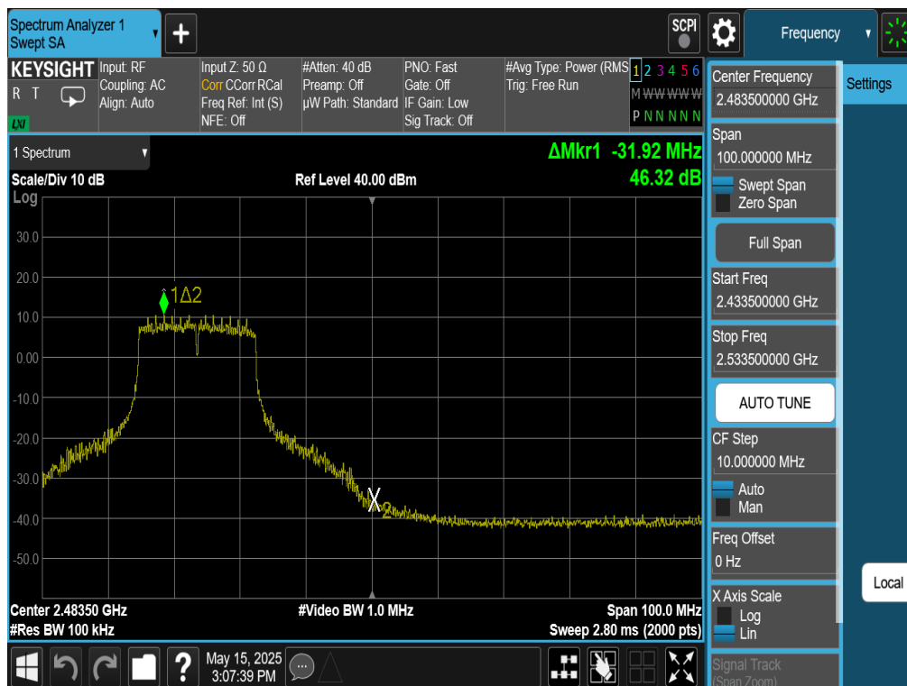
Plot 7-59. Band Edge Plot Antenna WF8 (802.11g – Ch. 10)
