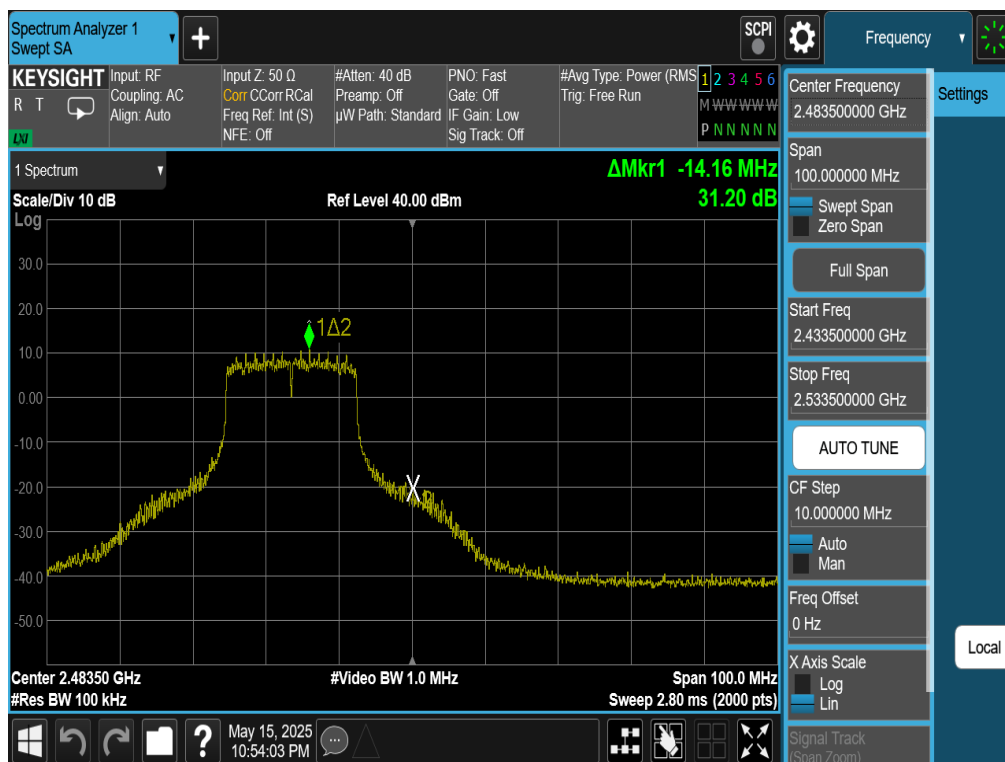
Plot 7-118. Band Edge Plot Antenna WF7 (802.11n (2.4GHz) – Ch. 12)
