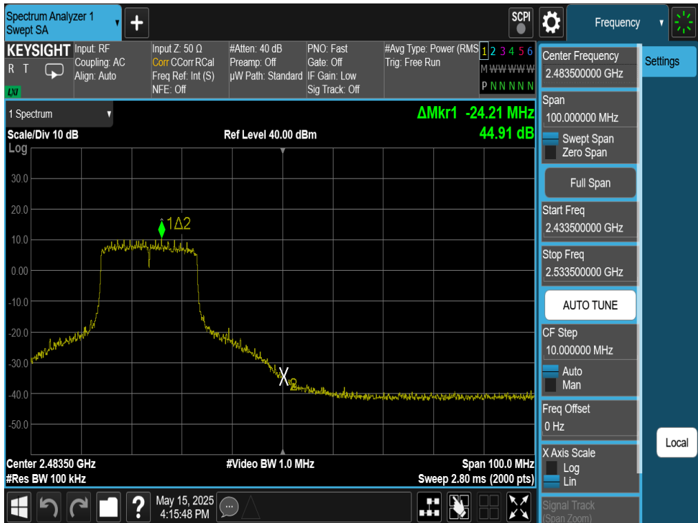
Plot 7-87. Band Edge Plot Antenna WF8 (802.11be (SU - 2.4GHz) – Ch. 10)
