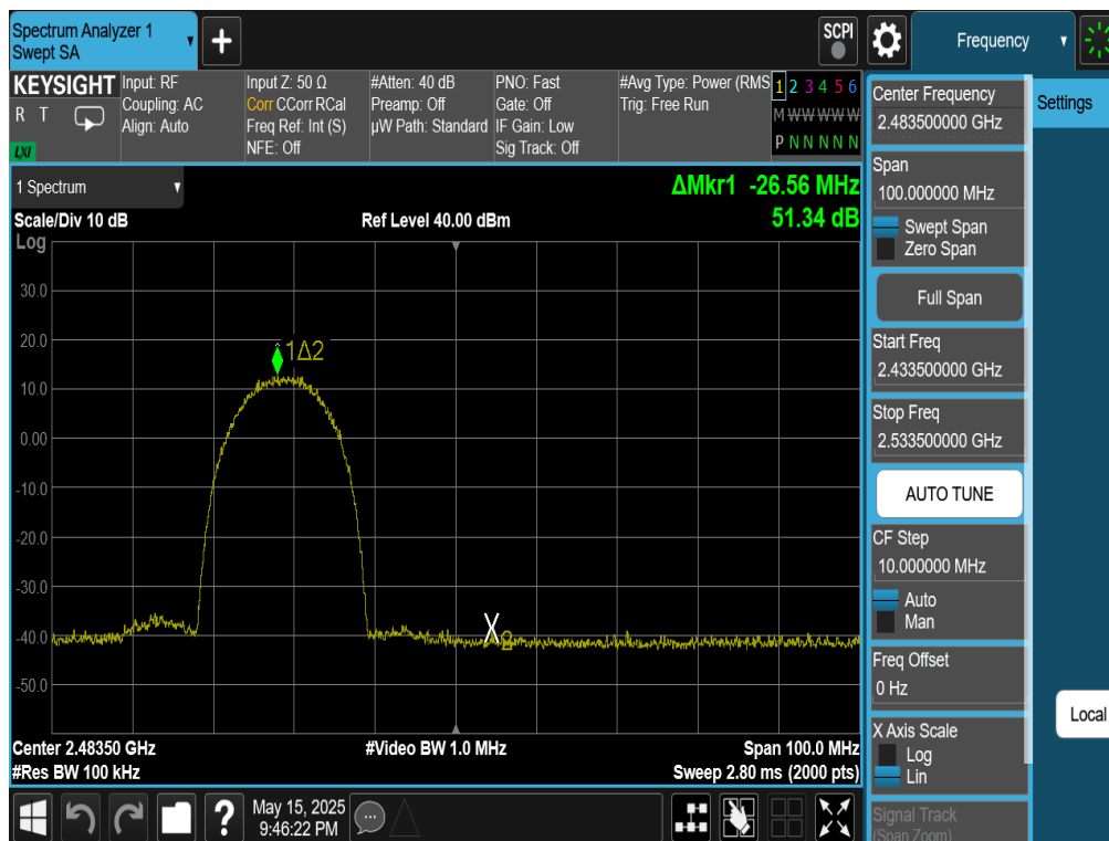
Plot 7-93. Band Edge Plot Antenna WF7 (802.11b – Ch. 11)
