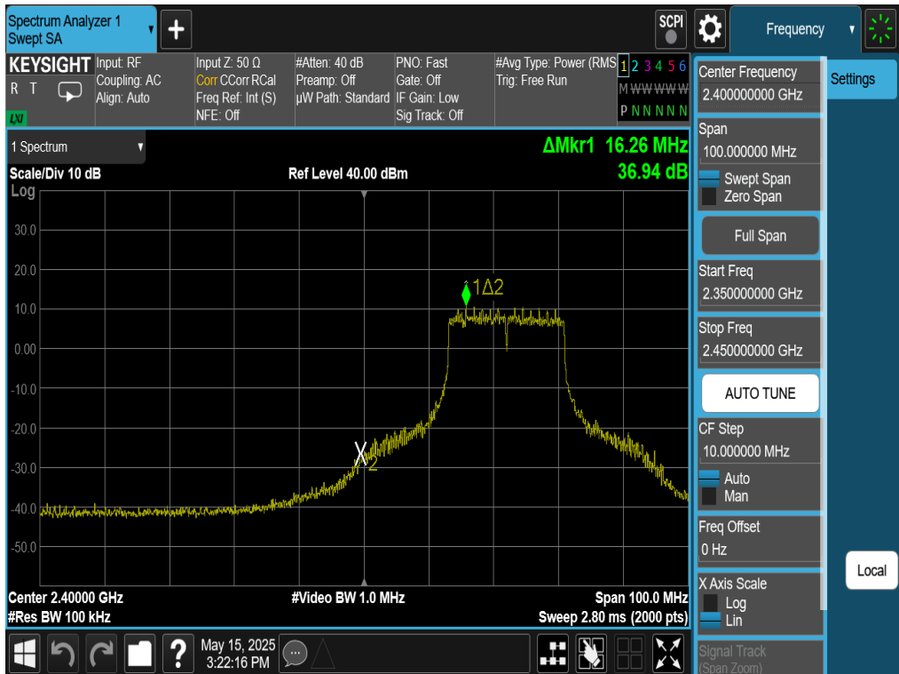
Plot 7-65. Band Edge Plot Antenna WF8 (802.11n (2.4GHz) – Ch. 3)
