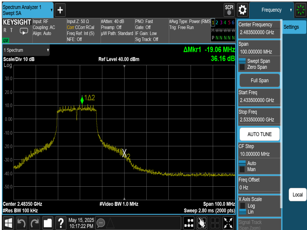
Plot 7-105. Band Edge Plot Antenna WF7 (802.11g – Ch. 11)
