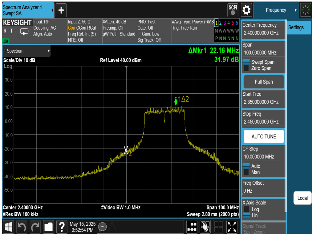
Plot 7-97. Band Edge Plot Antenna WF7 (802.11g – Ch. 2)
