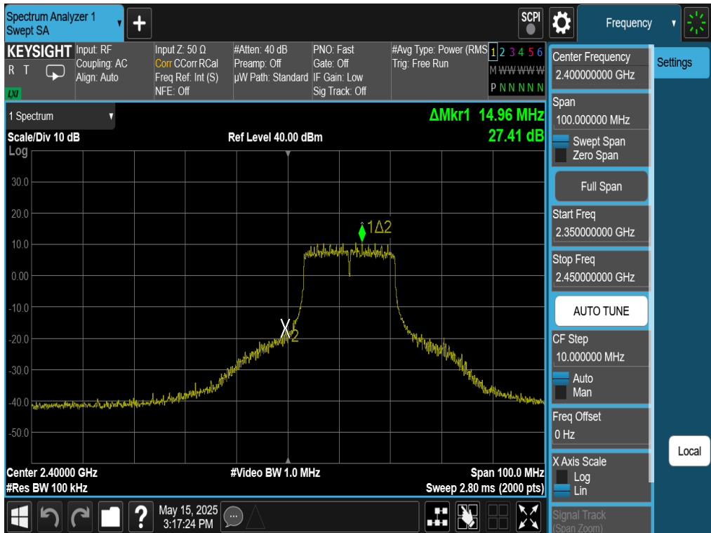
Plot 7-63. Band Edge Plot Antenna WF8 (802.11n (2.4GHz) – Ch. 1)
