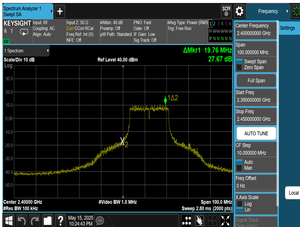
Plot 7-108. Band Edge Plot Antenna WF7 (802.11n (2.4GHz) – Ch. 1)
