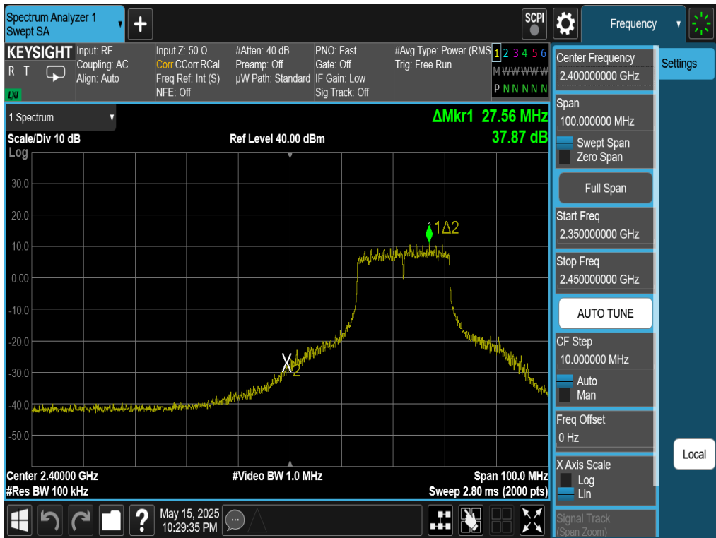
Plot 7-110. Band Edge Plot Antenna WF7 (802.11n (2.4GHz) – Ch. 3)
