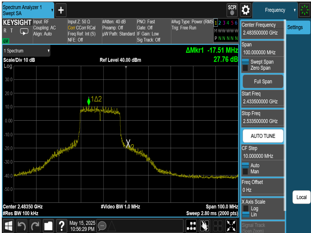
Plot 7-119. Band Edge Plot Antenna WF7 (802.11n (2.4GHz) – Ch. 13)
