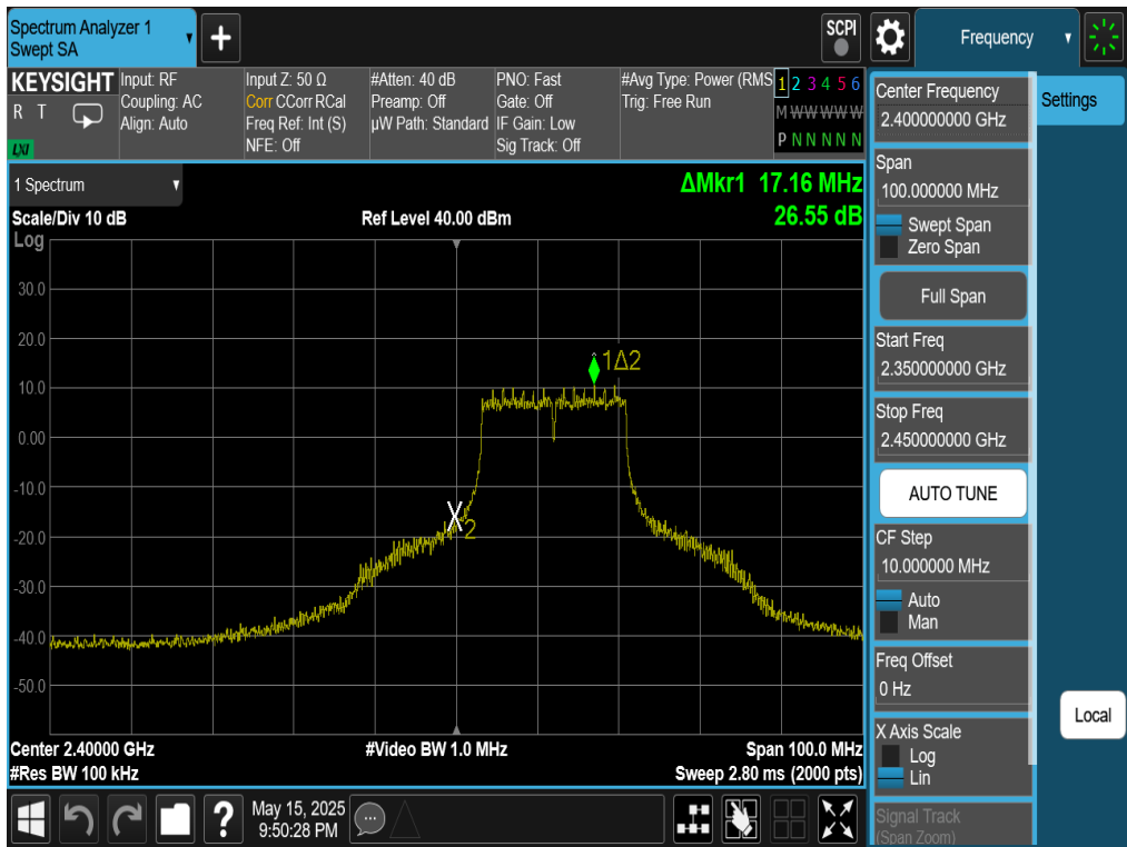
Plot 7-96. Band Edge Plot Antenna WF7 (802.11g – Ch. 1)
