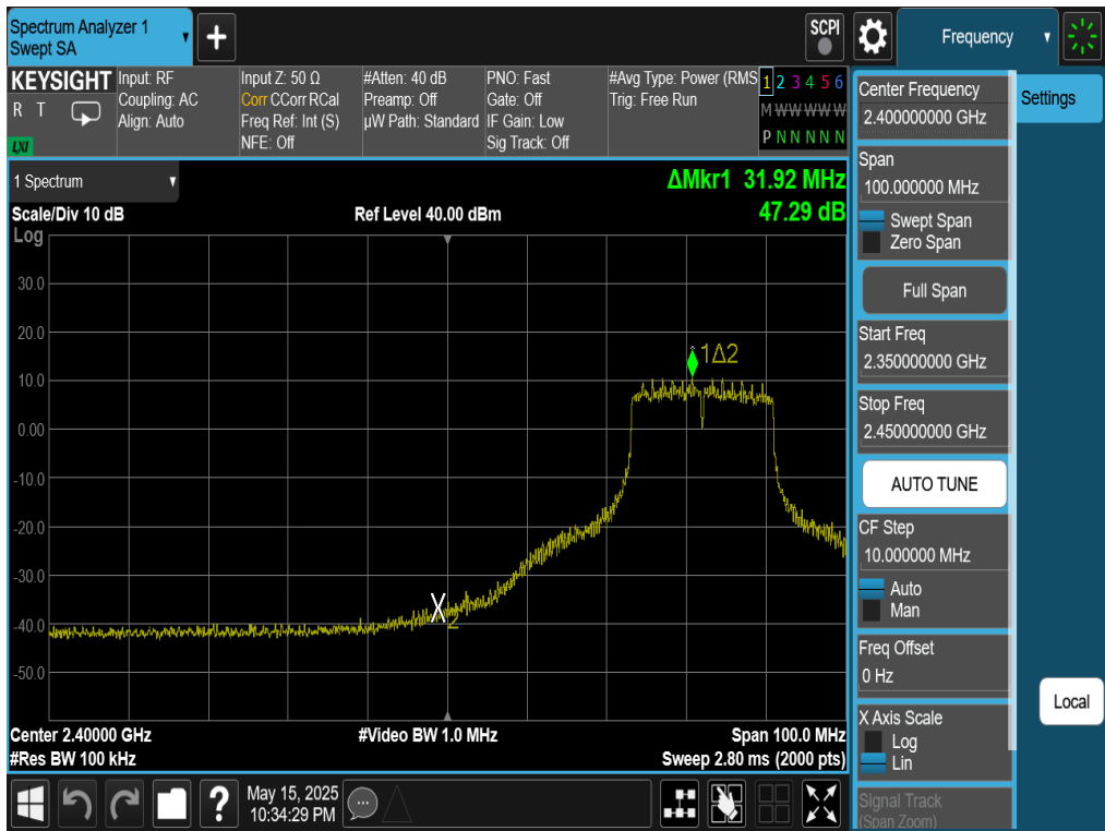
Plot 7-112. Band Edge Plot Antenna WF7 (802.11n (2.4GHz) – Ch. 5)
