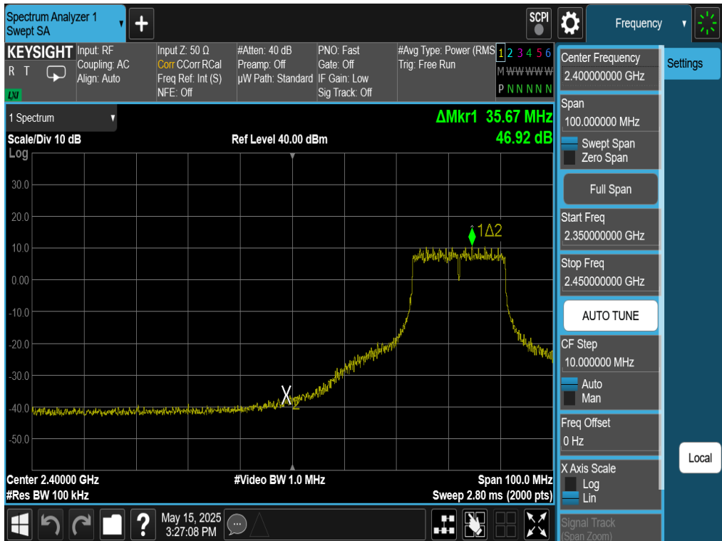
Plot 7-67. Band Edge Plot Antenna WF8 (802.11n (2.4GHz) – Ch. 5)
