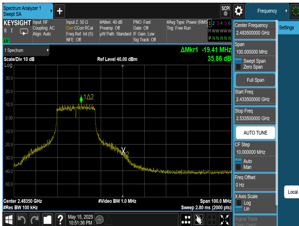
Plot 7-117. Band Edge Plot Antenna WF7 (802.11n (2.4GHz) – Ch. 11)
