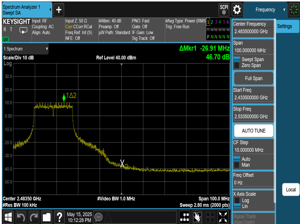
Plot 7-103. Band Edge Plot Antenna WF7 (802.11g – Ch. 9)
