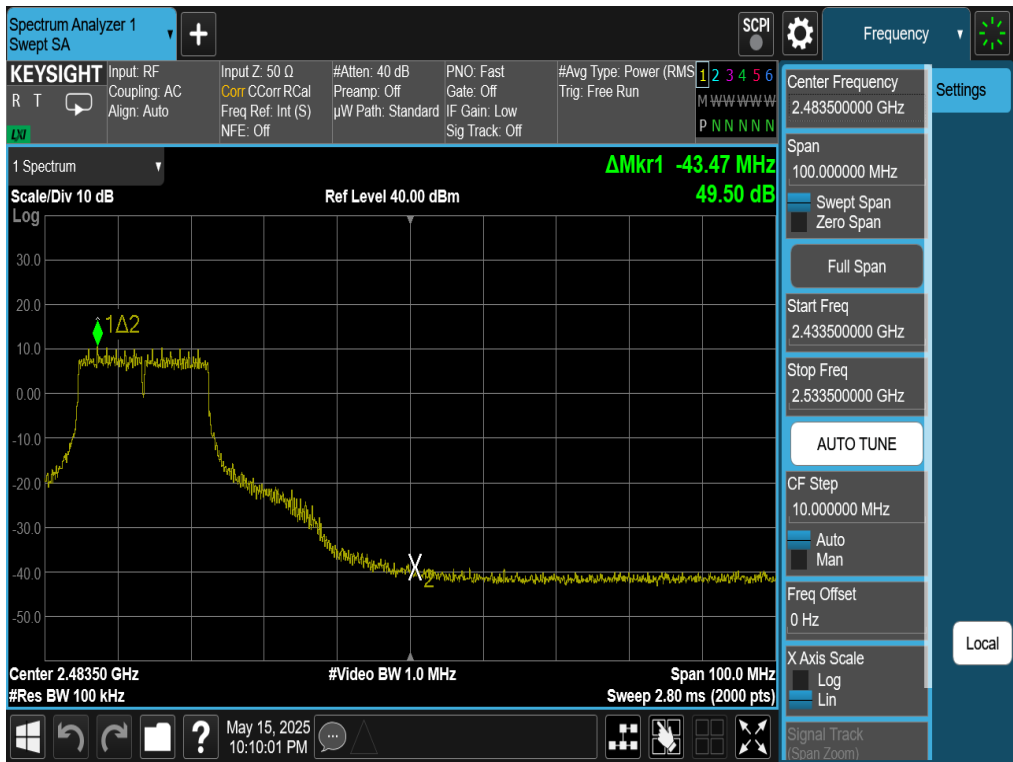
Plot 7-102. Band Edge Plot Antenna WF7 (802.11g – Ch. 8)
