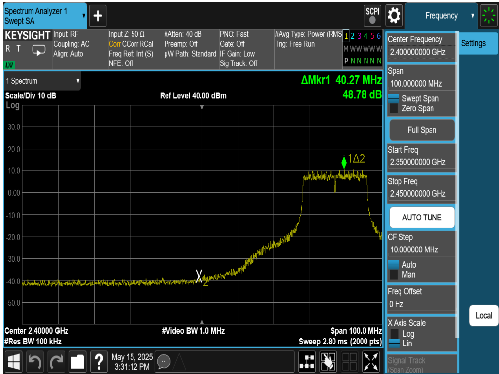
Plot 7-68. Band Edge Plot Antenna WF8 (802.11n (2.4GHz) – Ch. 6)
