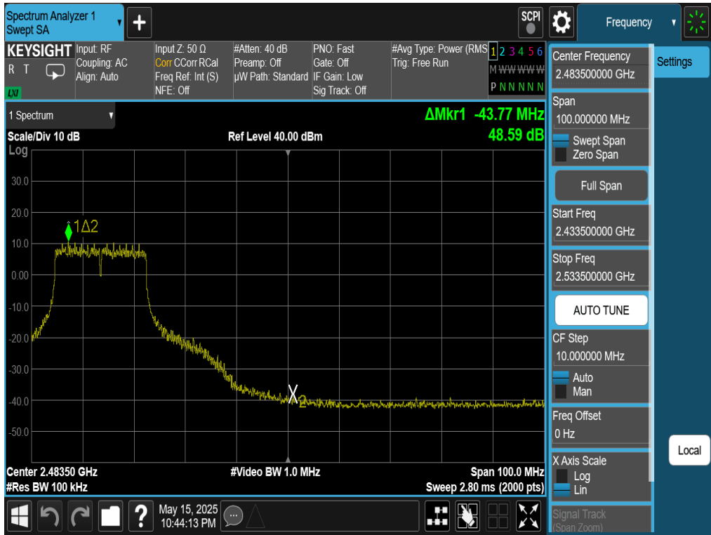
Plot 7-114. Band Edge Plot Antenna WF7 (802.11n (2.4GHz) – Ch. 8)
