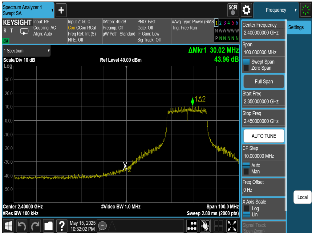
Plot 7-111. Band Edge Plot Antenna WF7 (802.11n (2.4GHz) – Ch. 4)
