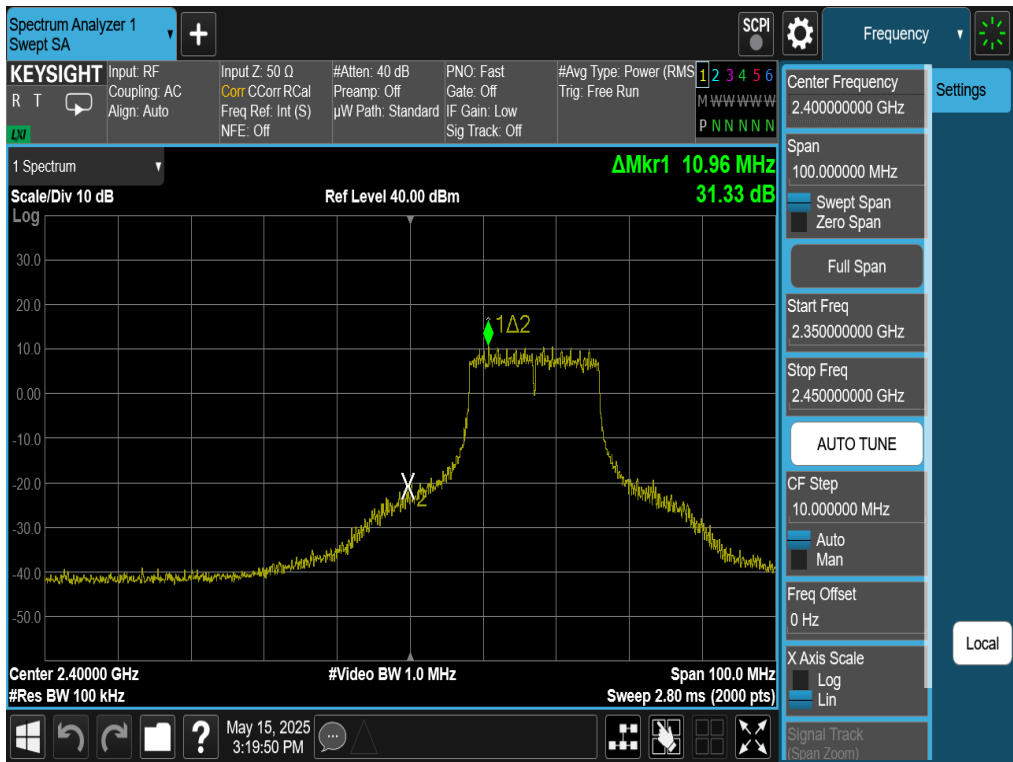
Plot 7-64. Band Edge Plot Antenna WF8 (802.11n (2.4GHz) – Ch. 2)
