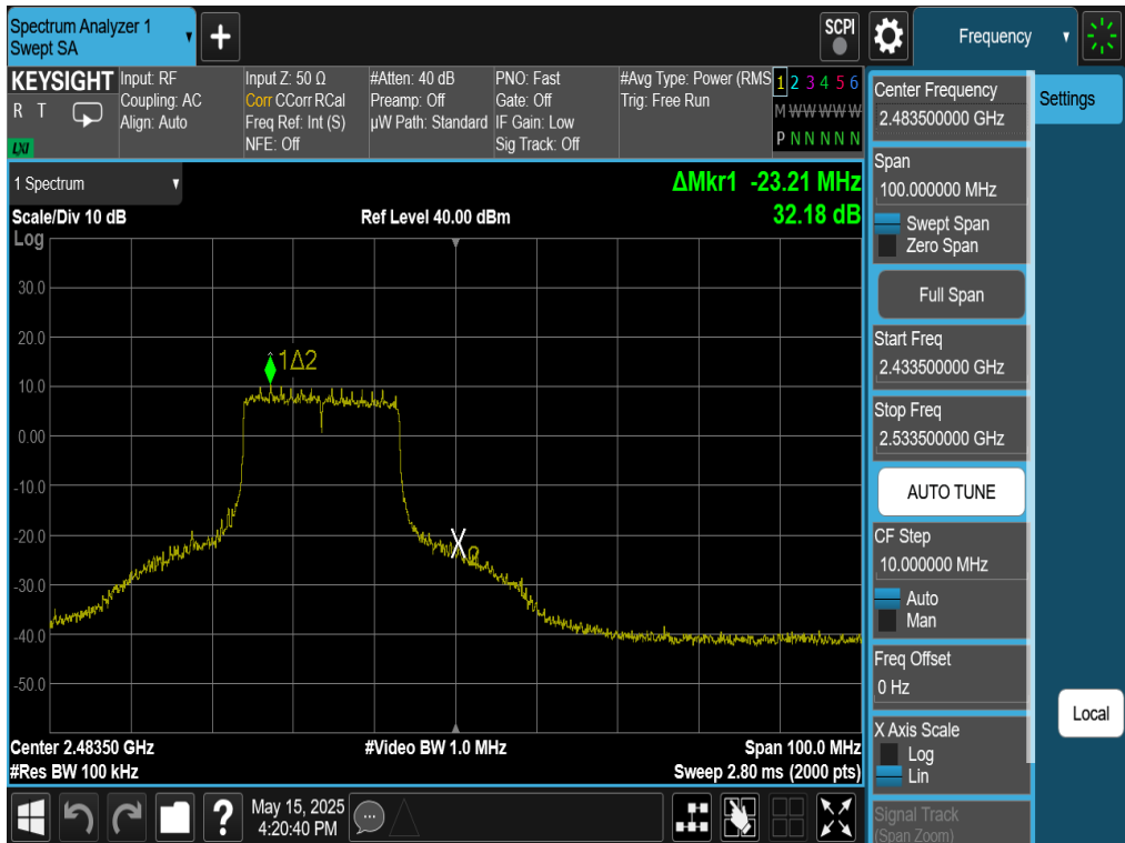
Plot 7-89. Band Edge Plot Antenna WF8 (802.11be (SU - 2.4GHz) – Ch. 12)
