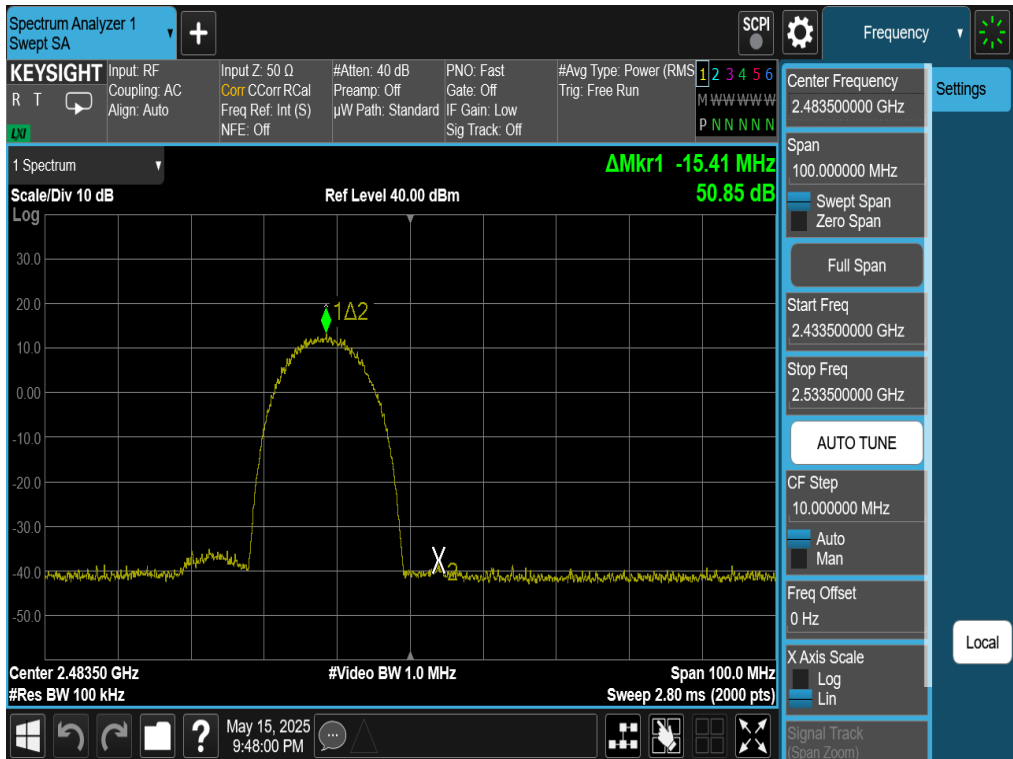
Plot 7-95. Band Edge Plot Antenna WF7 (802.11b – Ch. 13)
