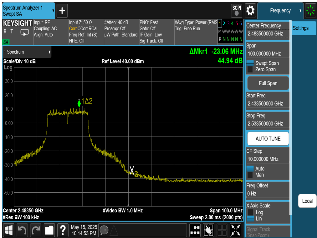
Plot 7-104. Band Edge Plot Antenna WF7 (802.11g – Ch. 10)
