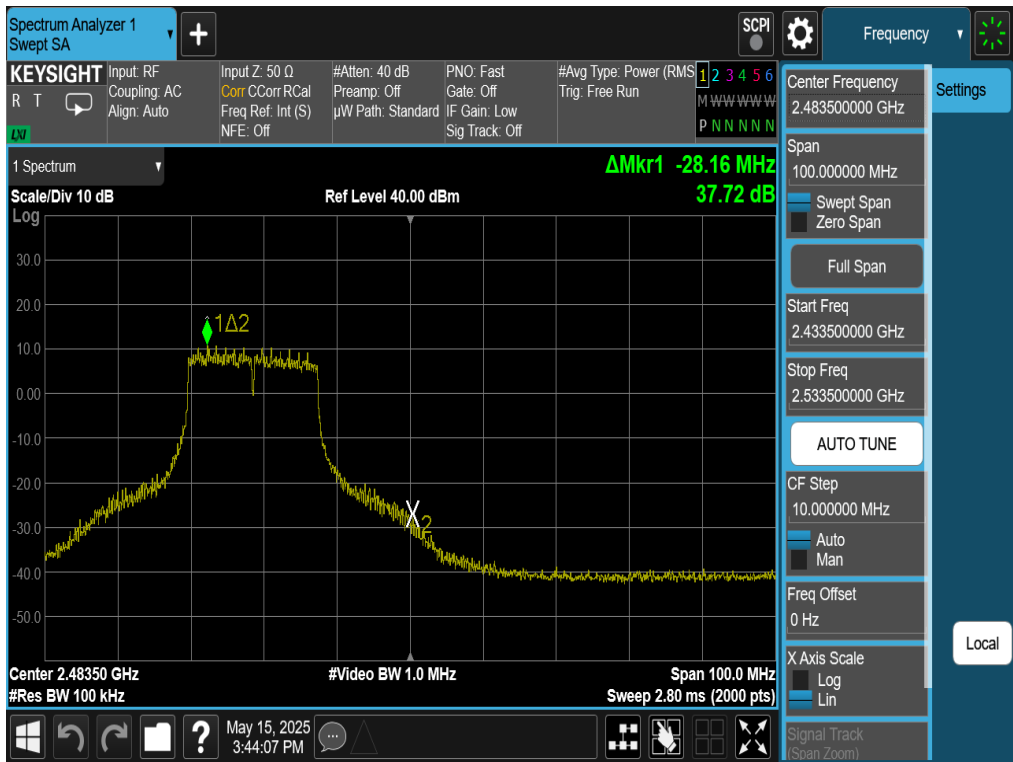
Plot 7-74. Band Edge Plot Antenna WF8 (802.11n (2.4GHz) – Ch. 11)
