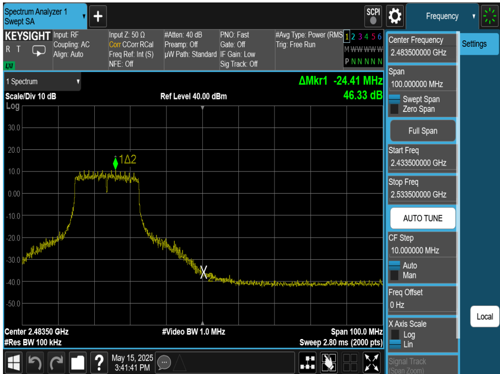
Plot 7-73. Band Edge Plot Antenna WF8 (802.11n (2.4GHz) – Ch. 10)
