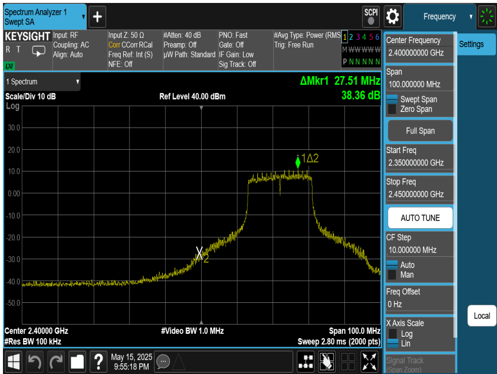
Plot 7-98. Band Edge Plot Antenna WF7 (802.11g – Ch. 3)
