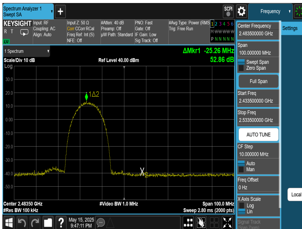
Plot 7-94. Band Edge Plot Antenna WF7 (802.11b – Ch. 12)
