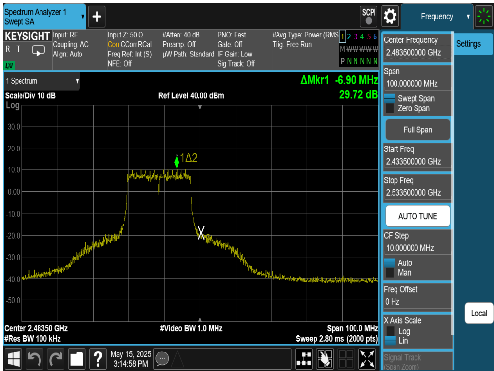
Plot 7-62. Band Edge Plot Antenna WF8 (802.11g – Ch. 13)
