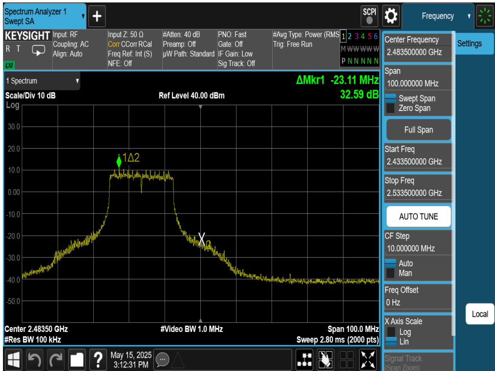
Plot 7-61. Band Edge Plot Antenna WF8 (802.11g – Ch. 12)
