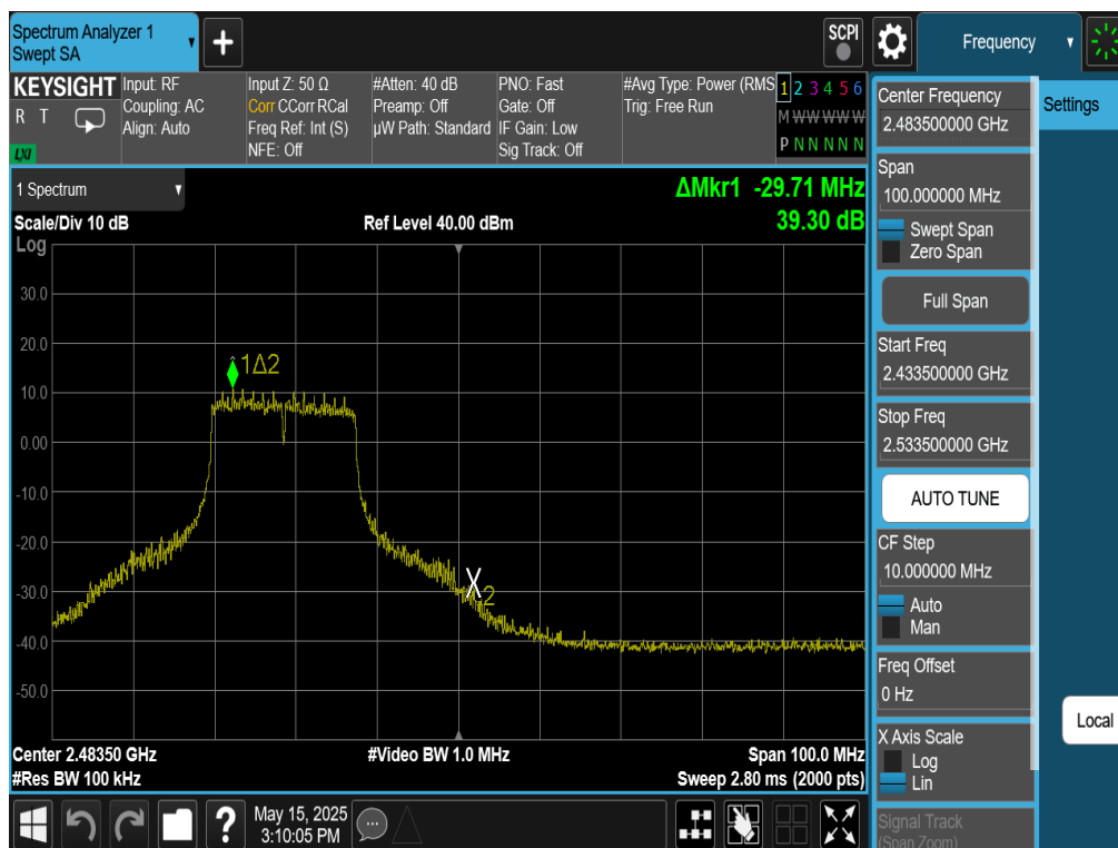
Plot 7-60. Band Edge Plot Antenna WF8 (802.11g – Ch. 11)
