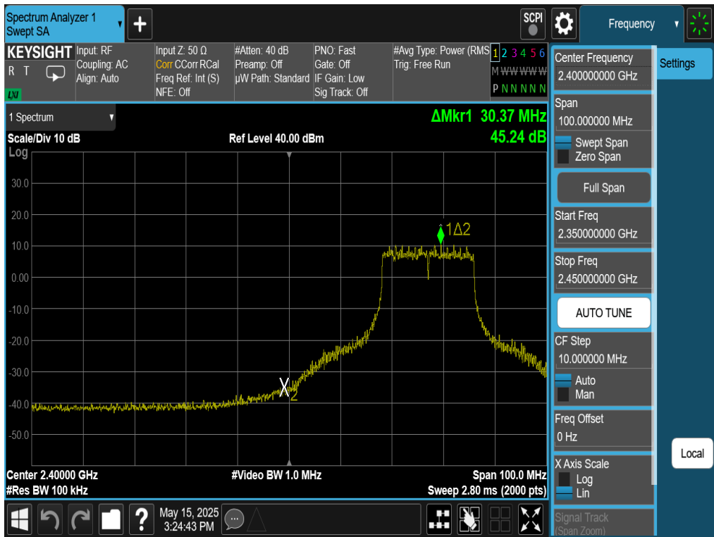
Plot 7-66. Band Edge Plot Antenna WF8 (802.11n (2.4GHz) – Ch. 4)
