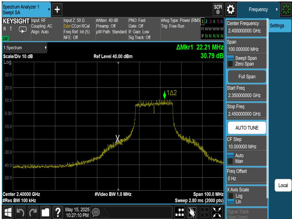
Plot 7-109. Band Edge Plot Antenna WF7 (802.11n (2.4GHz) – Ch. 2)
