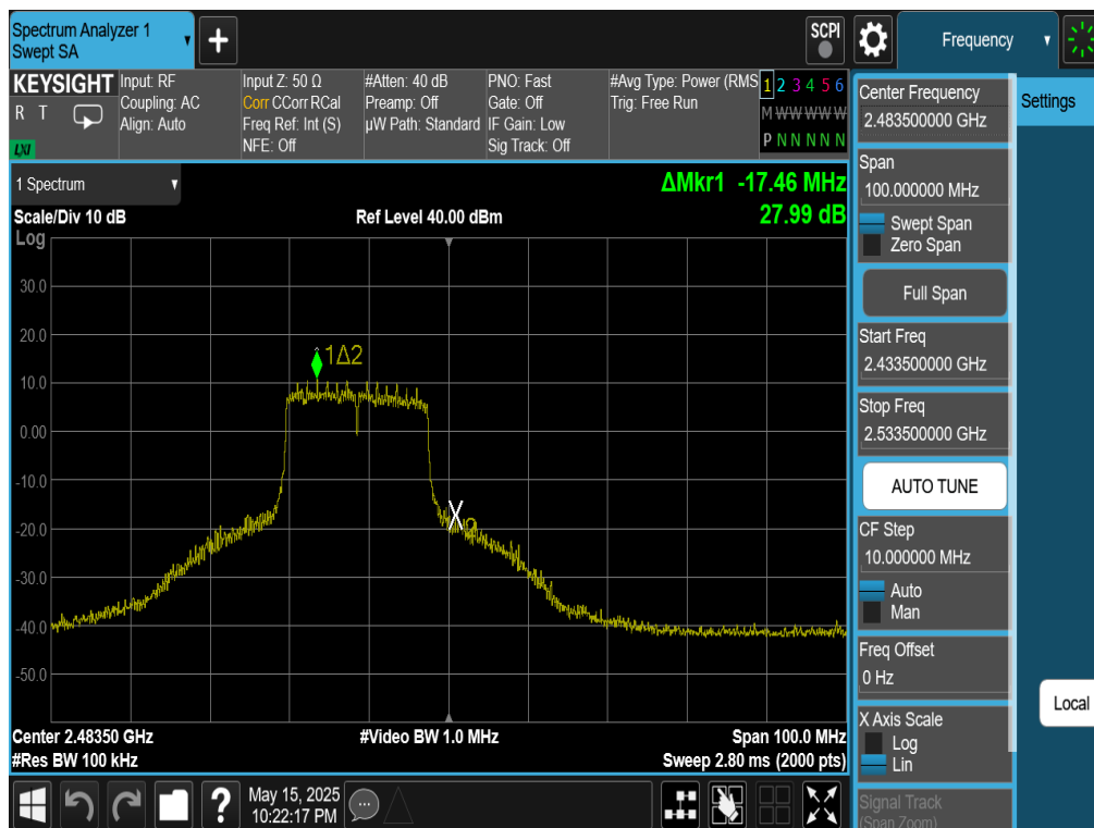
Plot 7-107. Band Edge Plot Antenna WF7 (802.11g – Ch. 13)
