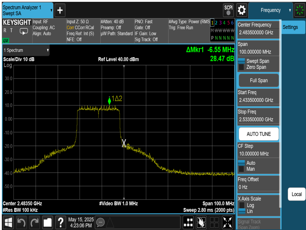
Plot 7-90. Band Edge Plot Antenna WF8 (802.11be (SU - 2.4GHz) – Ch. 13)
