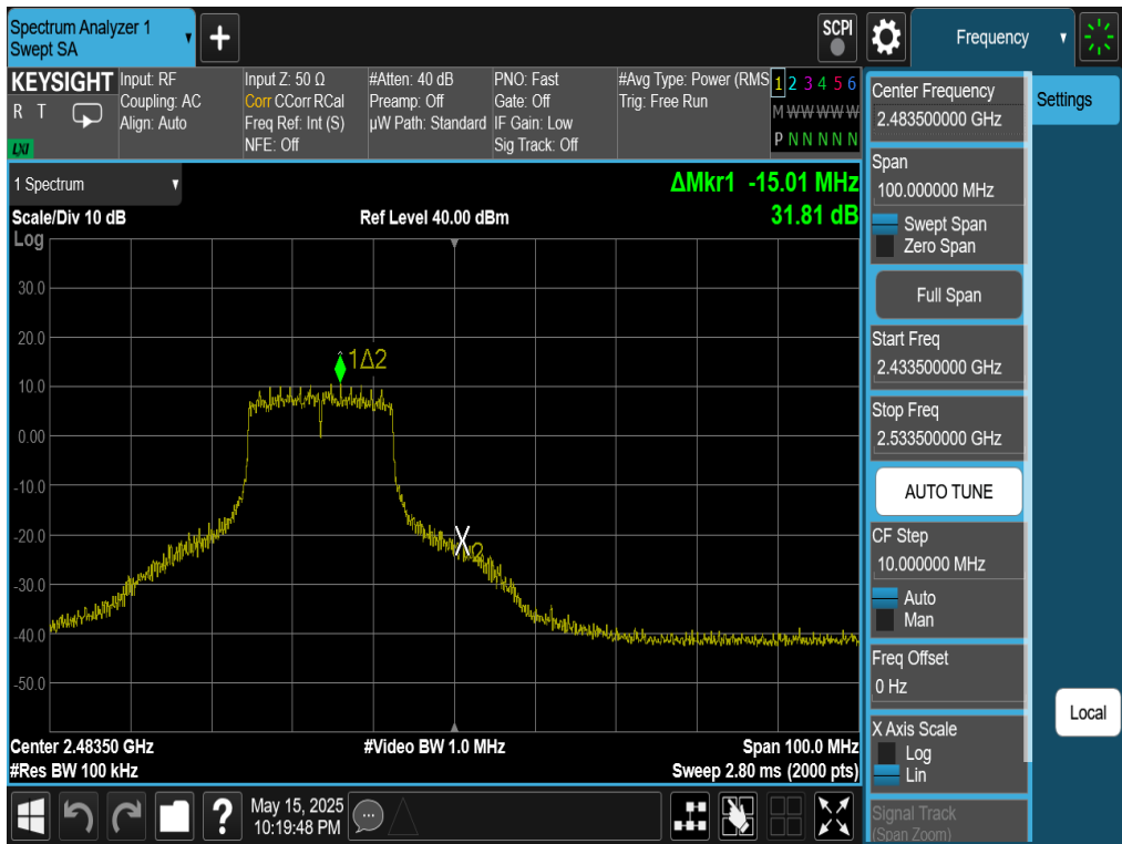
Plot 7-106. Band Edge Plot Antenna WF7 (802.11g – Ch. 12)
