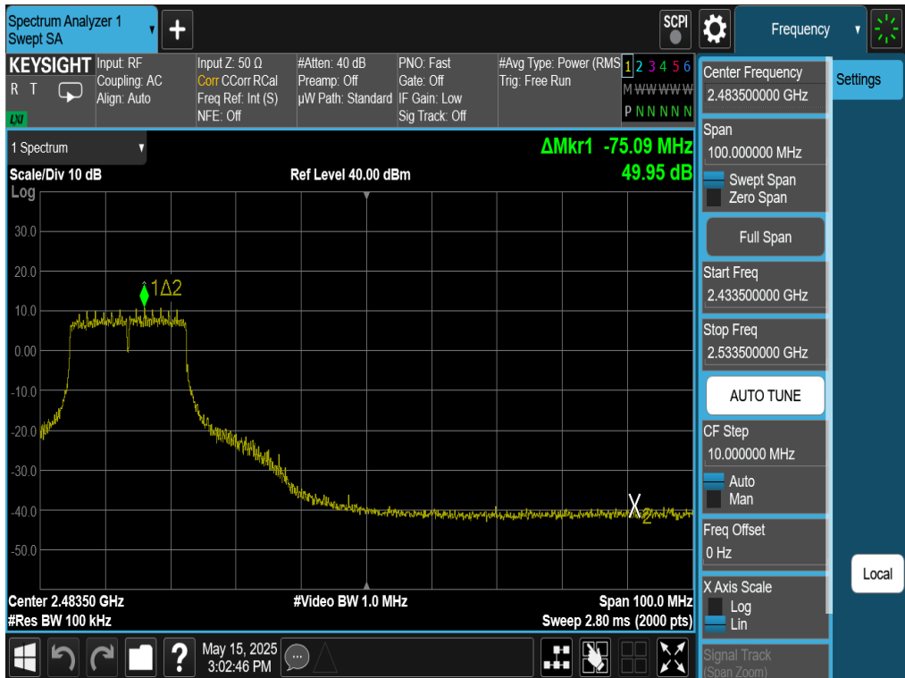
Plot 7-57. Band Edge Plot Antenna WF8 (802.11g – Ch. 8)
