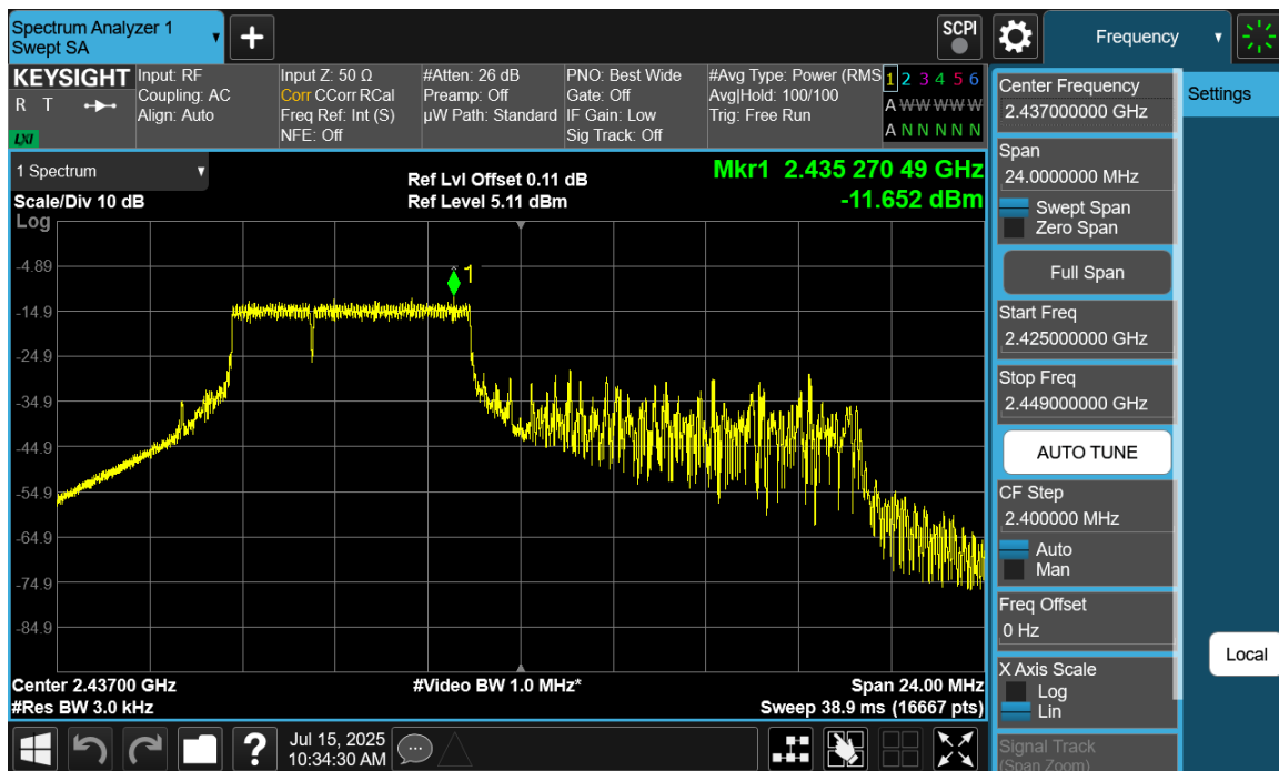
Plot 7-23 PSD Antenna WF9 (20MHz BW 802.11be(RU) RU52+26 Index70 - Ch.6)
