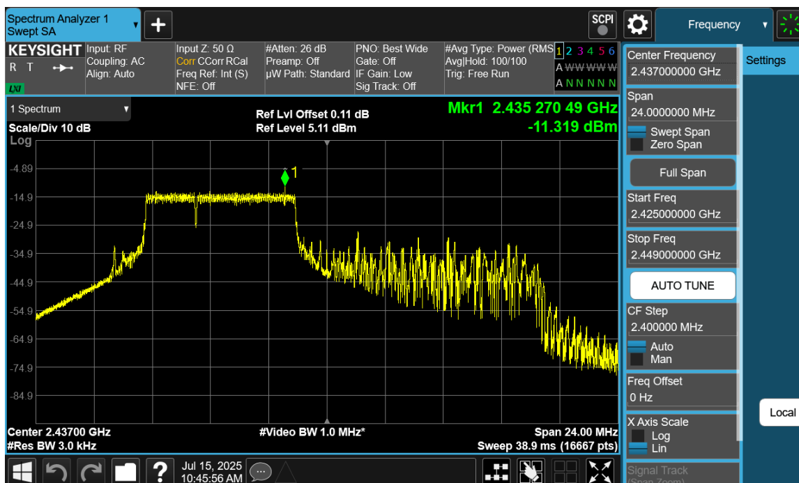
Plot 7-39 PSD CDD Diversity Antenna WF9 (20MHz BW 802.11be(RU) RU52+26 Index70 - Ch.6)
