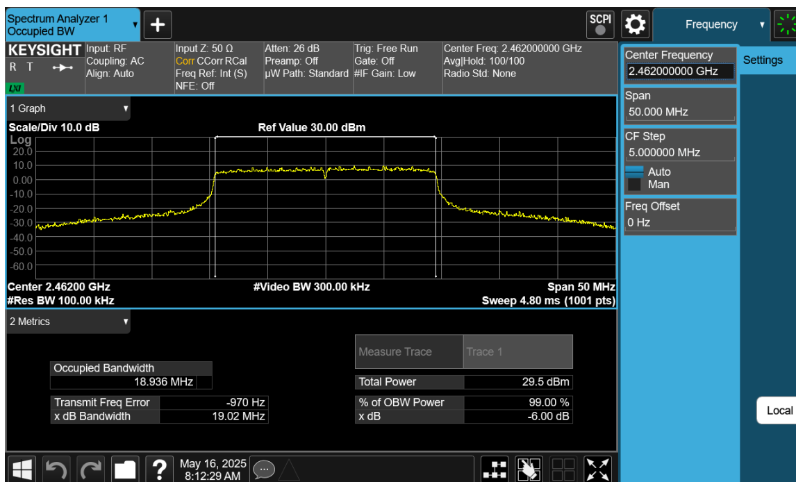
Plot 7-10 6dB BW & 99% OBW Antenna WF9 (20MHz BW 802.11be(RU) RU242 Index61 - Ch.11)
