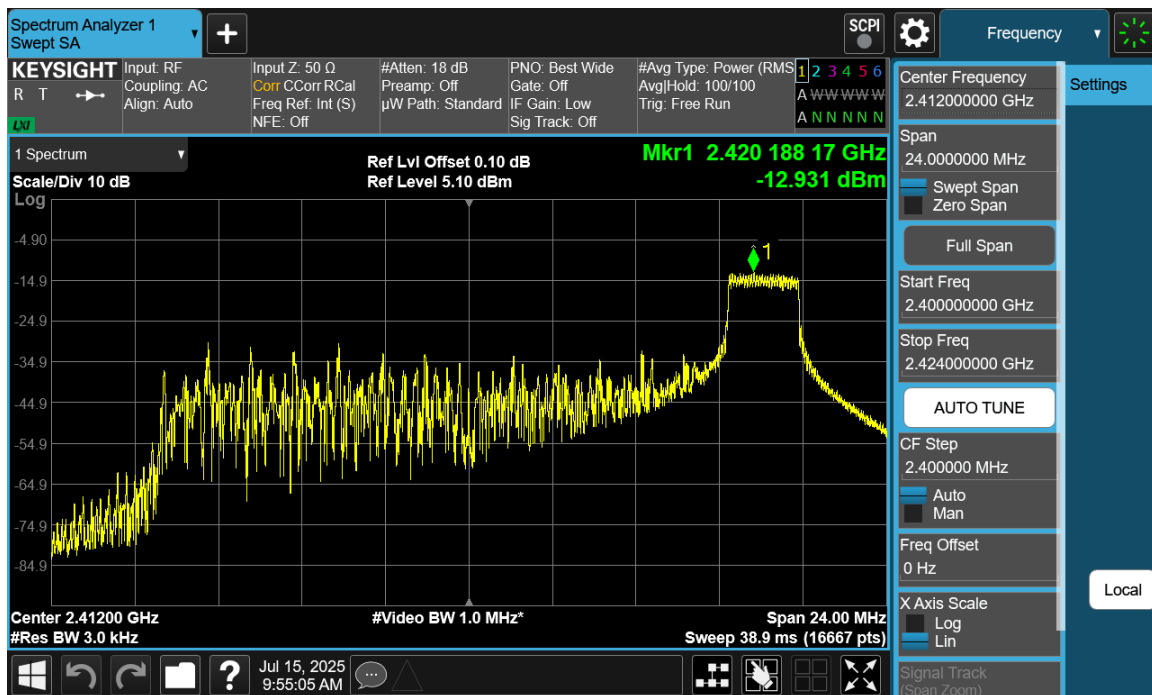
Plot 7-37 PSD CDD Diversity Antenna WF9 (20MHz BW 802.11be(RU) RU26 Index8 - Ch.1)
