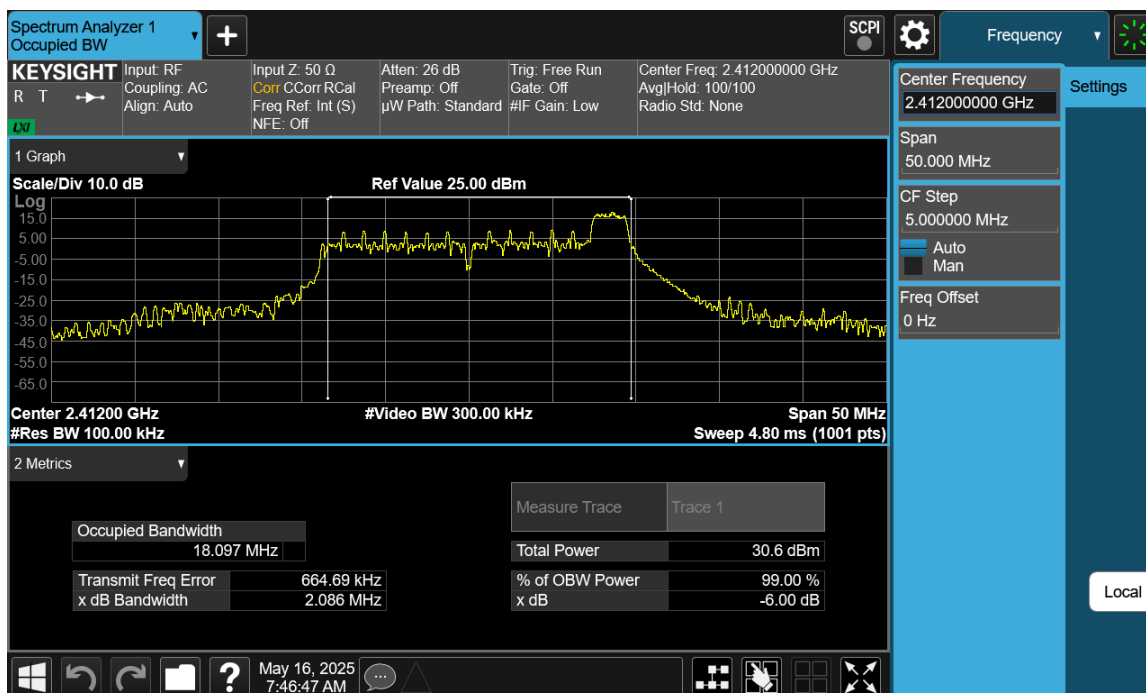
Plot 7-9 6dB BW & 99% OBW Antenna WF9 (20MHz BW 802.11be(RU) RU26 Index8 - Ch.1)
