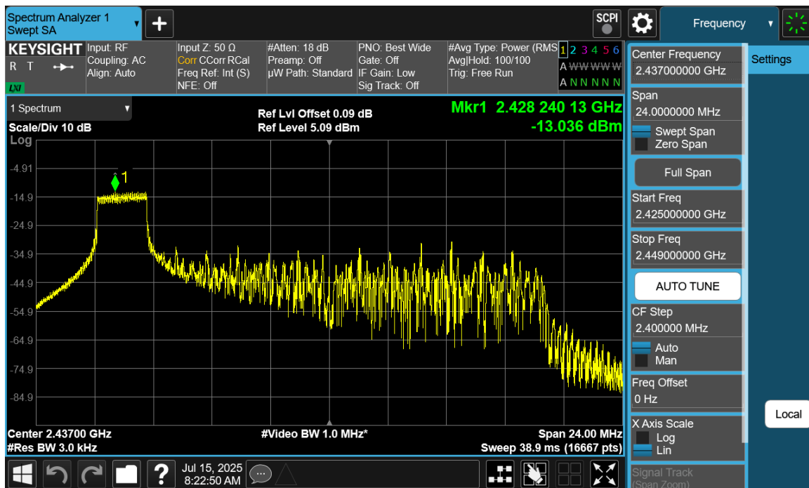
Plot 7-29 PSD CDD Primary Antenna WF7 (20MHz BW 802.11be(RU) RU26 Index0 - Ch.6)
