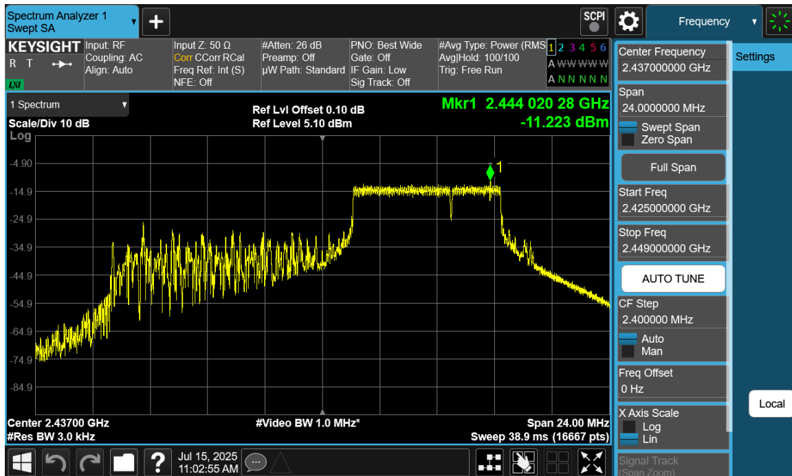
Plot 7-15 PSD Antenna WF8 (20MHz BW 802.11be(RU) RU52+26 Index72 - Ch.6)
