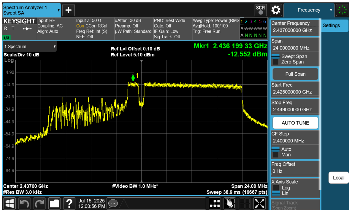
Plot 7-32 PSD CDD Primary Antenna WF7 (20MHz BW 802.11be(RU) RU106+26 Index83 - Ch.6)
