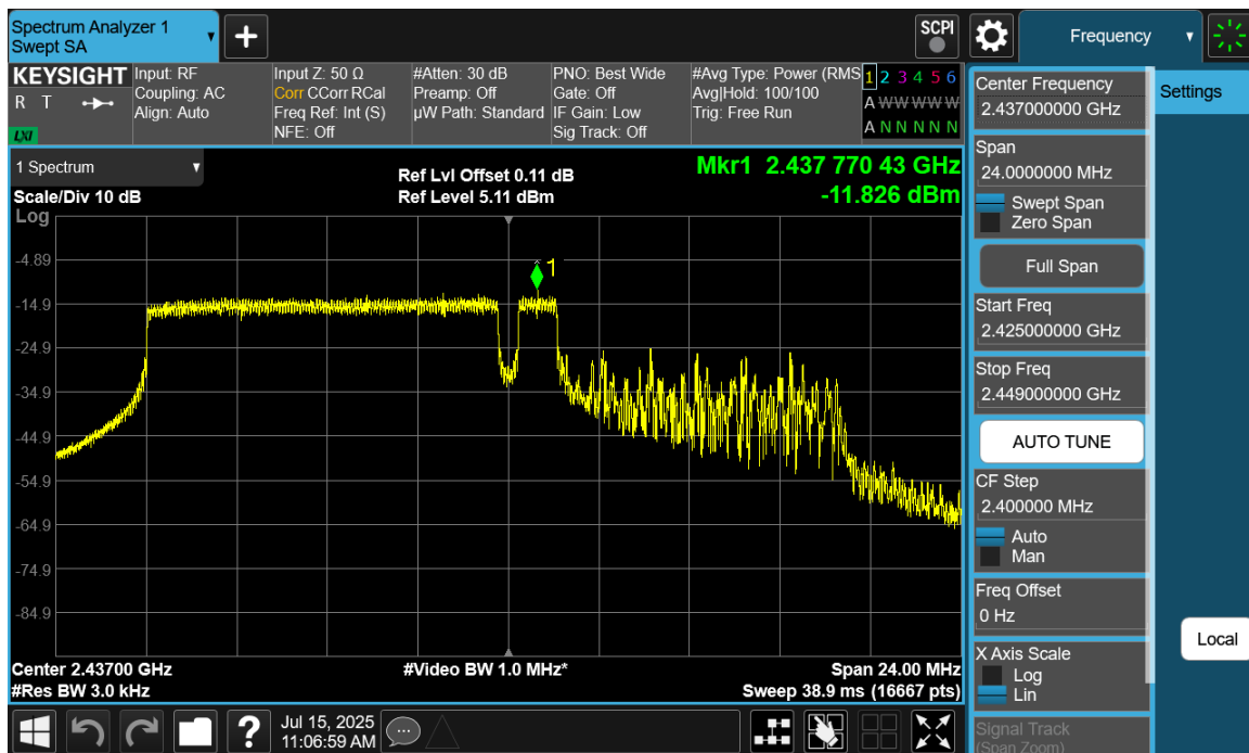
Plot 7-16 PSD Antenna WF8 (20MHz BW 802.11be(RU) RU106+26 Index82 - Ch.6)
