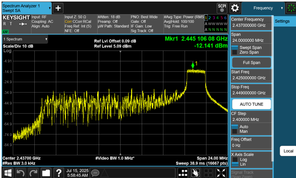
Plot 7-13 PSD Antenna WF8 (20MHz BW 802.11be(RU) RU26 Index8 - Ch.6)
