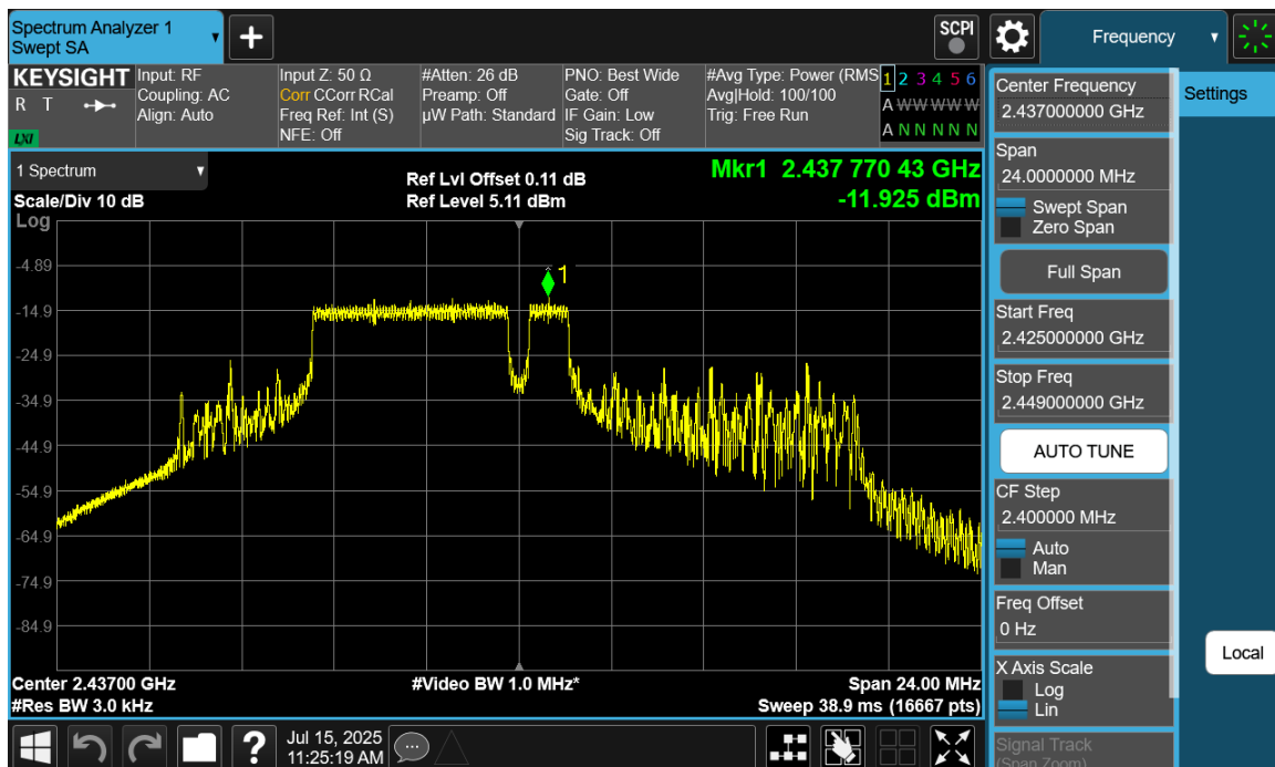
Plot 7-27 PSD CDD Primary Antenna WF8 (20MHz BW 802.11be(RU) RU52+26 Index71 - Ch.6)
