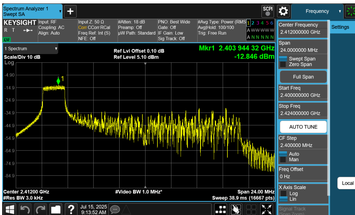
Plot 7-21 PSD Antenna WF9 (20MHz BW 802.11be(RU) RU26 Index0 - Ch.1)
