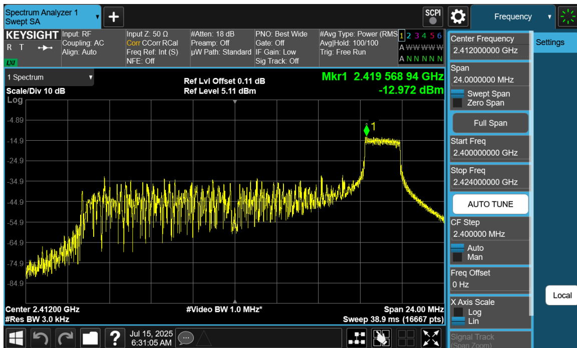
Plot 7-33 PSD CDD Diversity Antenna WF8 (20MHz BW 802.11be(RU) RU26 Index8 - Ch.1)
