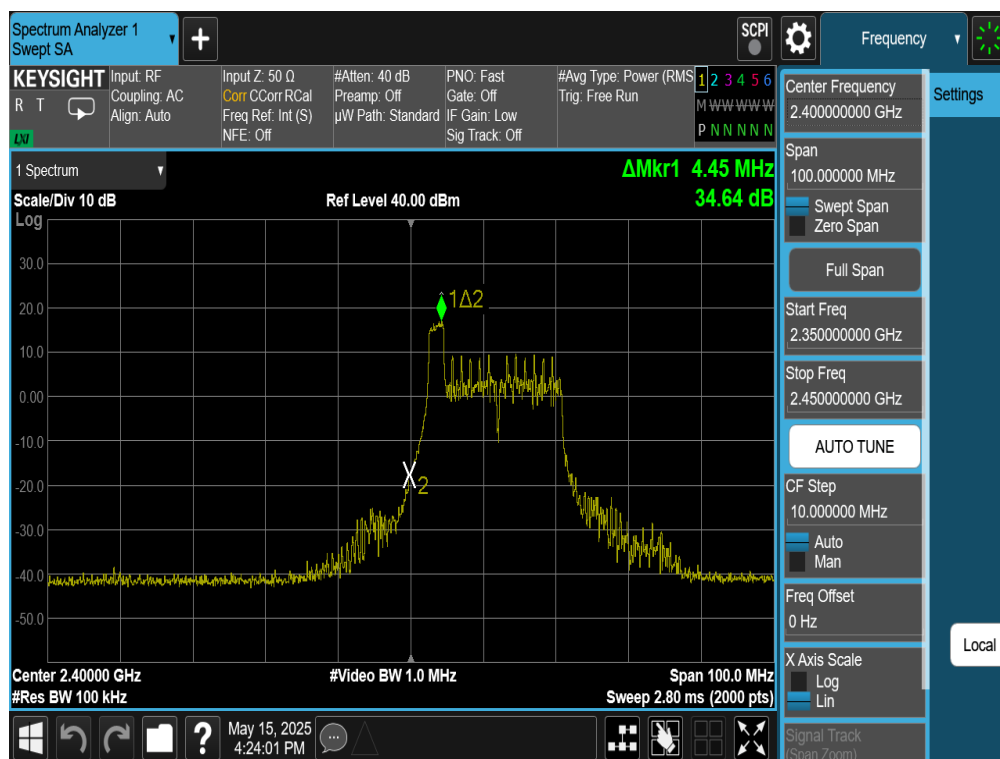
Plot 7-41. Band Edge Antenna WF8 (802.11be OFDMA – RU26 Index 0 – Ch. 1)
