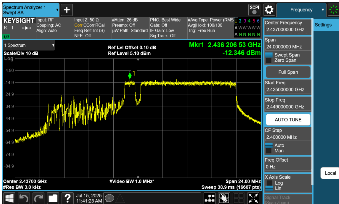
Plot 7-28 PSD CDD Primary Antenna WF8 (20MHz BW 802.11be(RU) RU106+26 Index83 - Ch.6)
