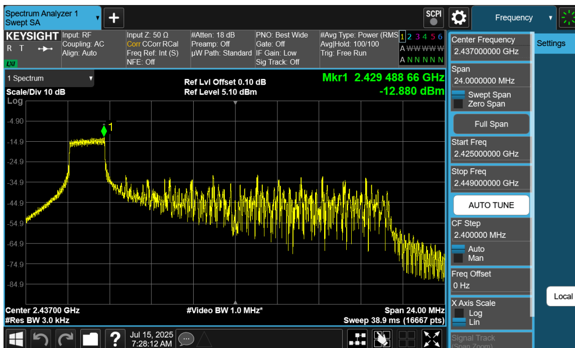
Plot 7-17 PSD Antenna WF7 (20MHz BW 802.11be(RU) RU26 Index0 - Ch.6)
