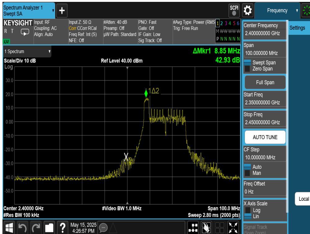
Plot 7-42. Band Edge Antenna WF8 (802.11be OFDMA – RU26 Index 0 – Ch. 2)
