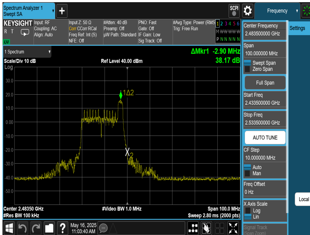
Plot 7-80. Band Edge Antenna WF9 (802.11be OFDMA – RU26 Index 8 – Ch. 13)
