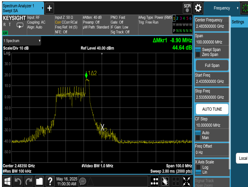
Plot 7-79. Band Edge Antenna WF9 (802.11be OFDMA – RU26 Index 8 – Ch. 12)
