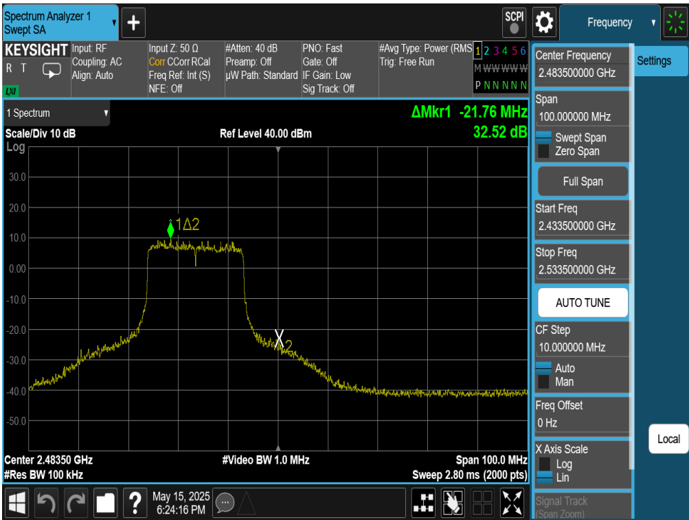
Plot 7-57. Band Edge Antenna WF8 (802.11be OFDMA – RU242 – Ch. 12)
