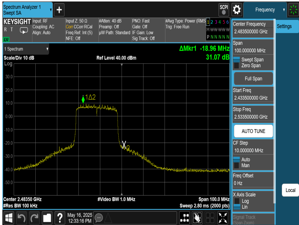
Plot 7-94. Band Edge Antenna WF9 (802.11be OFDMA – RU242 – Ch. 13)
