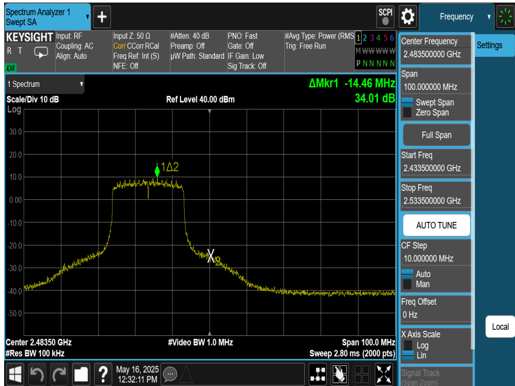
Plot 7-93. Band Edge Antenna WF9 (802.11be OFDMA – RU242 – Ch. 12)
