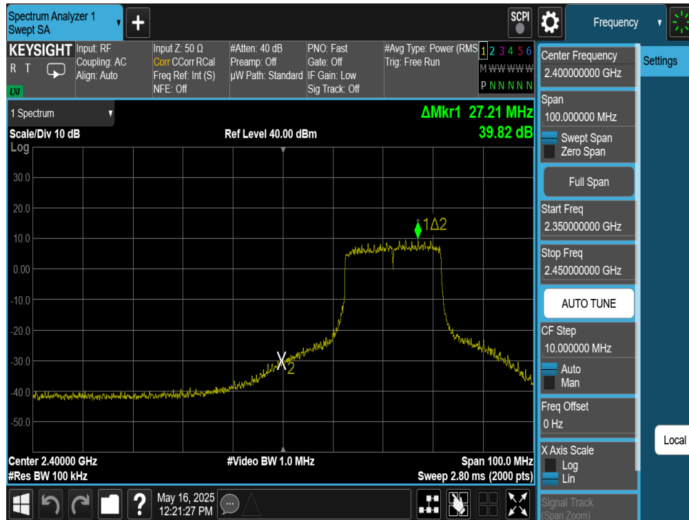
Plot 7-83. Band Edge Antenna WF9 (802.11be OFDMA – RU242 – Ch. 3)
