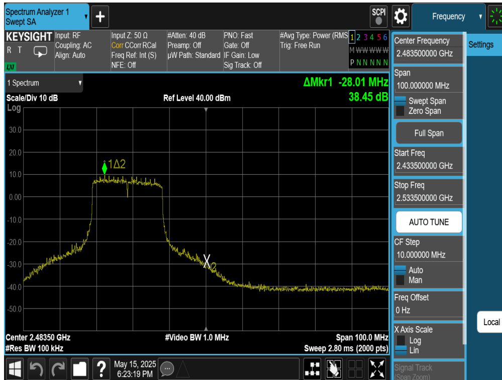
Plot 7-56. Band Edge Antenna WF8 (802.11be OFDMA – RU242 – Ch. 11)
