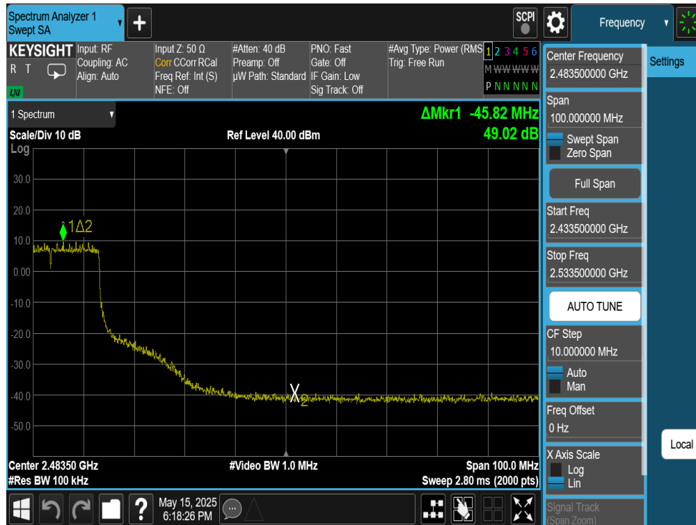
Plot 7-51. Band Edge Antenna WF8 (802.11be OFDMA – RU242 – Ch. 6(High Channel))
