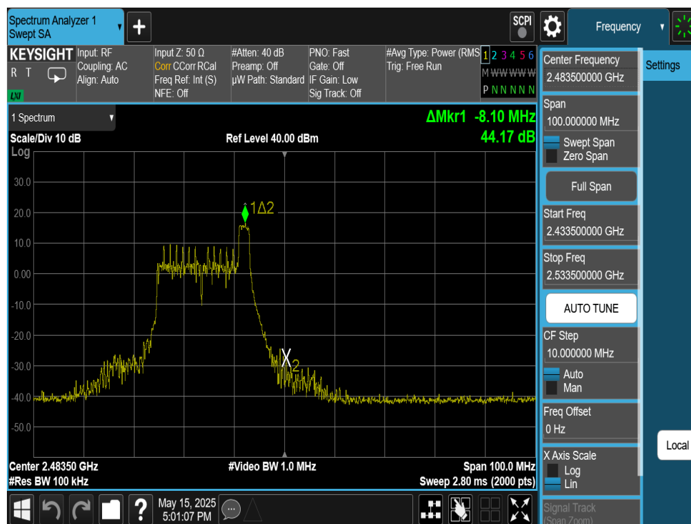
Plot 7-43. Band Edge Antenna WF8 (802.11be OFDMA – RU26 Index 8 – Ch. 12)
