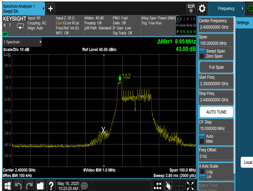
Plot 7-78. Band Edge Antenna WF9 (802.11be OFDMA – RU26 Index 0 – Ch. 2)
