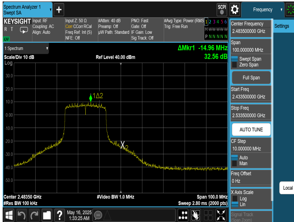
Plot 7-75. Band Edge Antenna WF7 (802.11be OFDMA – RU242 – Ch. 12)
