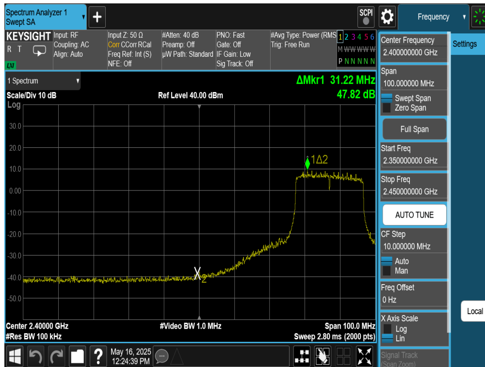
Plot 7-86. Band Edge Antenna WF9 (802.11be OFDMA – RU242 – Ch. 6(Low Channel))
