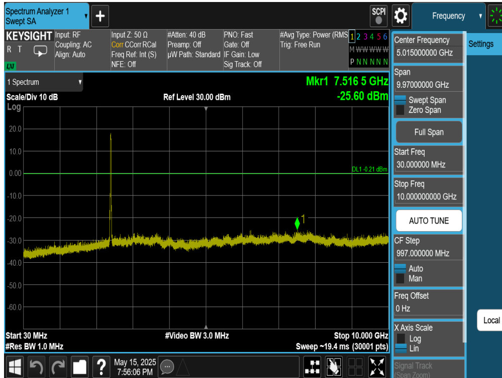
Plot 7-101. Conducted Spurious Plot Antenna WF8 (802.11be OFDMA – RU242 – Ch. 1)
