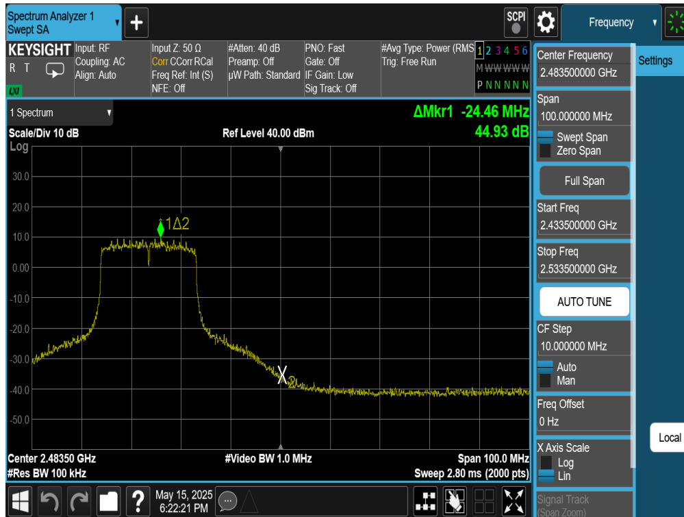
Plot 7-55. Band Edge Antenna WF8 (802.11be OFDMA – RU242 – Ch. 10)
