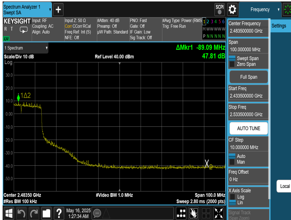
Plot 7-69. Band Edge Antenna WF7 (802.11be OFDMA – RU242 – Ch. 6(High Channel))
