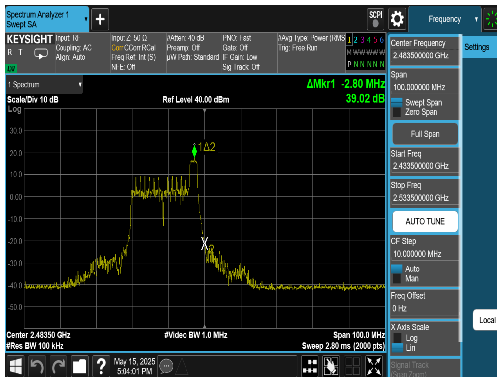
Plot 7-44. Band Edge Antenna WF8 (802.11be OFDMA – RU26 Index 8 – Ch. 13)
