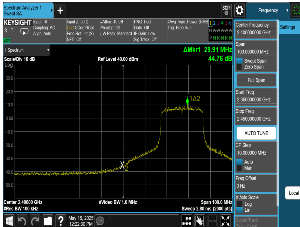
Plot 7-84. Band Edge Antenna WF9 (802.11be OFDMA – RU242 – Ch. 4)
