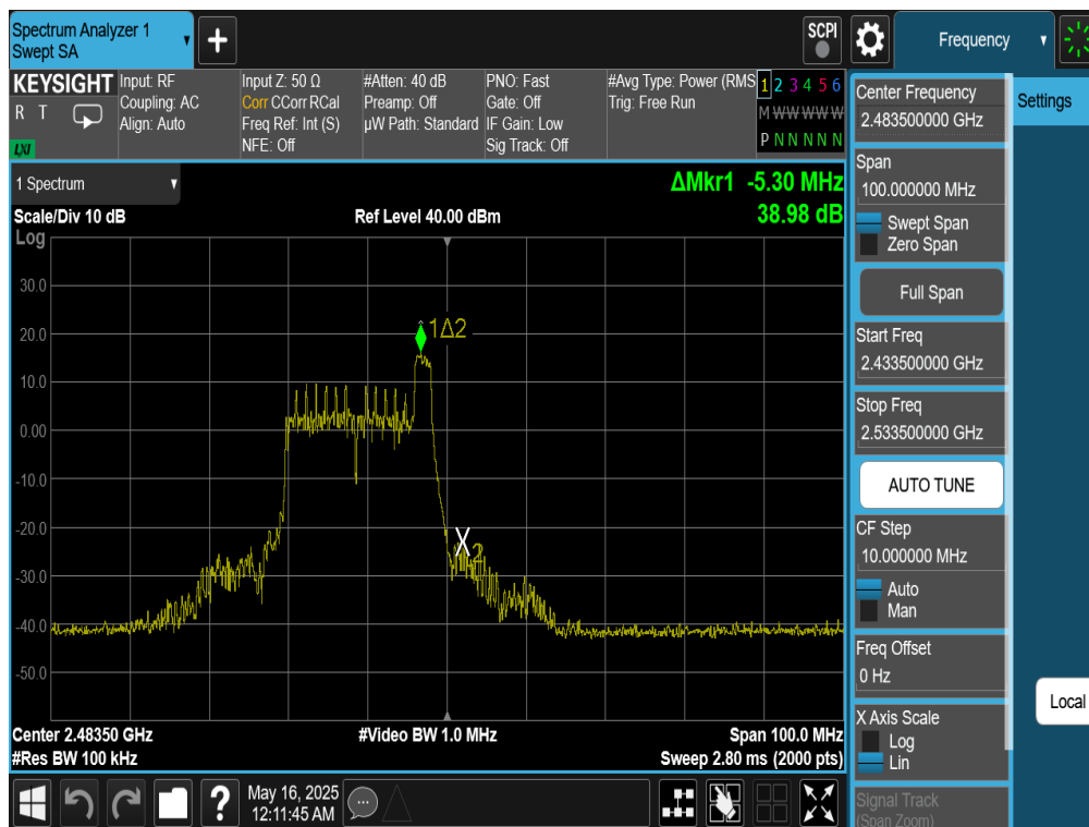
Plot 7-62. Band Edge Antenna WF7 (802.11be OFDMA – RU26 Index 8 – Ch. 13)
