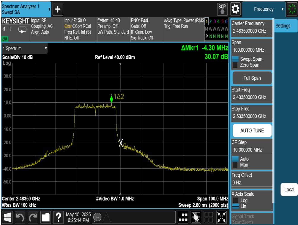
Plot 7-58. Band Edge Antenna WF8 (802.11be OFDMA – RU242 – Ch. 13)
