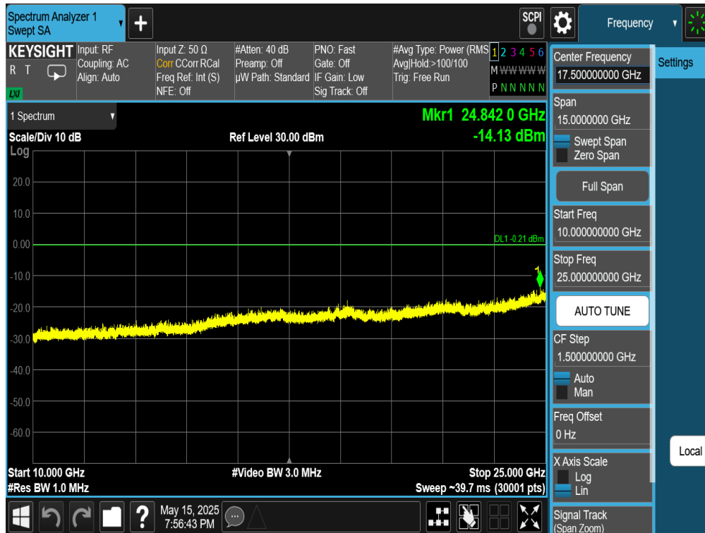
Plot 7-102. Conducted Spurious Plot Antenna WF8 (802.11be OFDMA – RU242 – Ch. 1)
