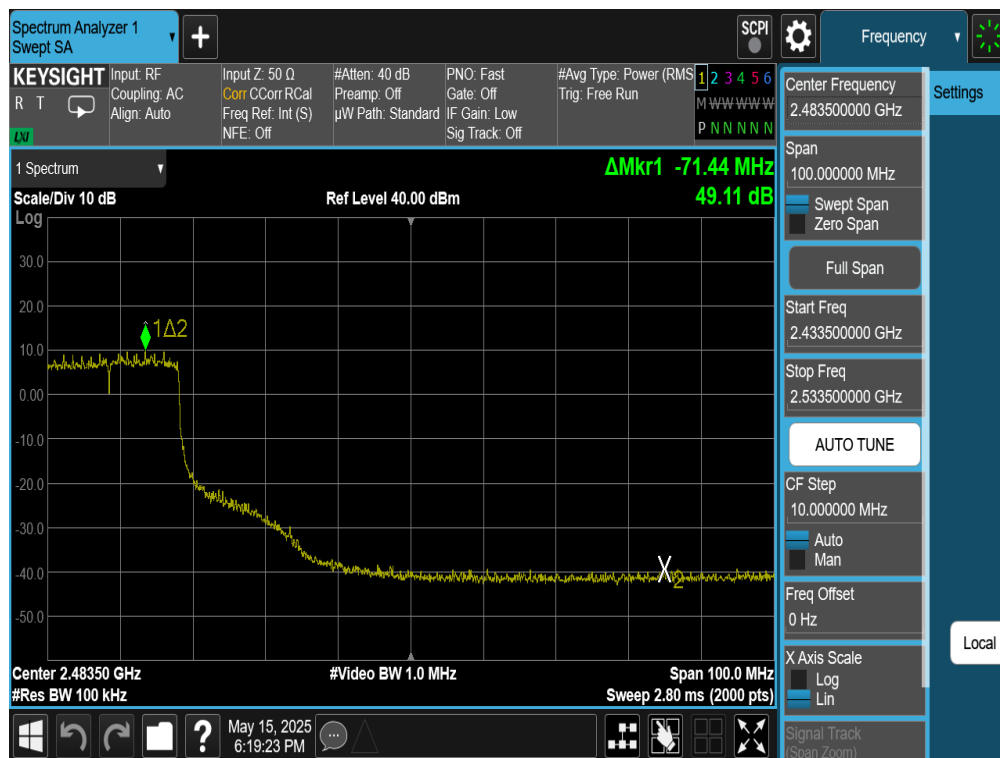
Plot 7-52. Band Edge Antenna WF8 (802.11be OFDMA – RU242 – Ch. 7)
