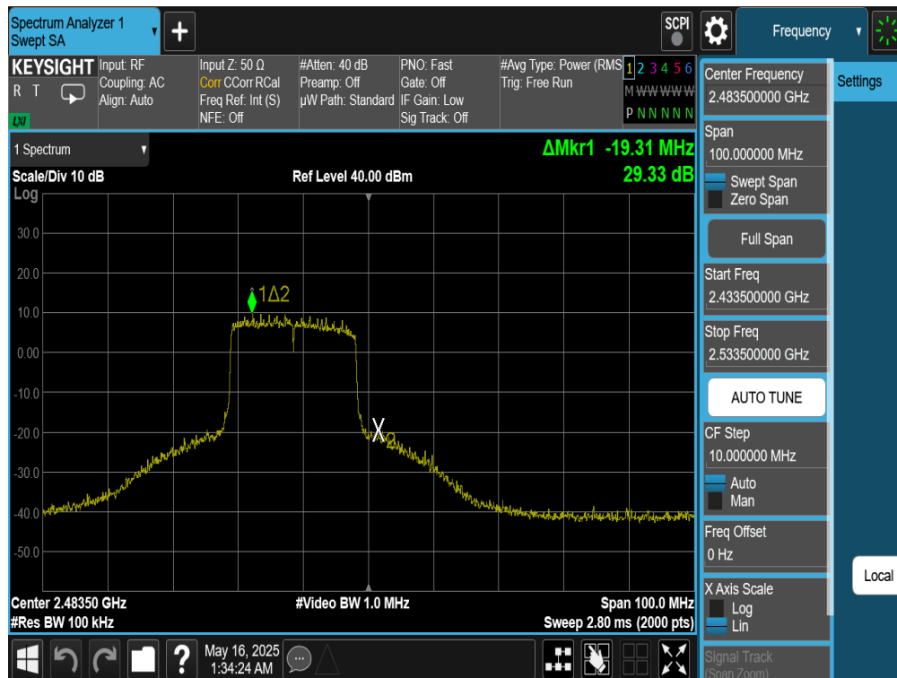
Plot 7-76. Band Edge Antenna WF7 (802.11be OFDMA – RU242 – Ch. 13)
