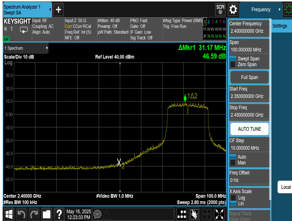
Plot 7-85. Band Edge Antenna WF9 (802.11be OFDMA – RU242 – Ch. 5)
