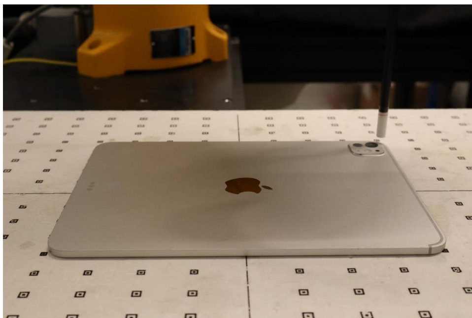
Near Field Power Density Test Setup 14: Back Side at 2mm – Antenna WF8
