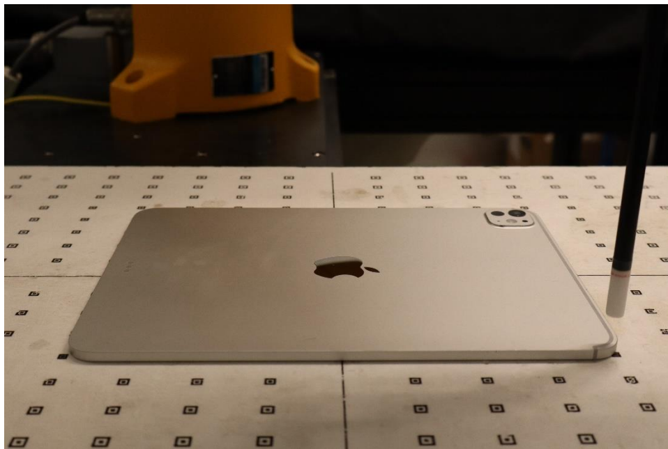
Near Field Power Density Test Setup 17: Back Side at 9.82mm – Antenna WF7
