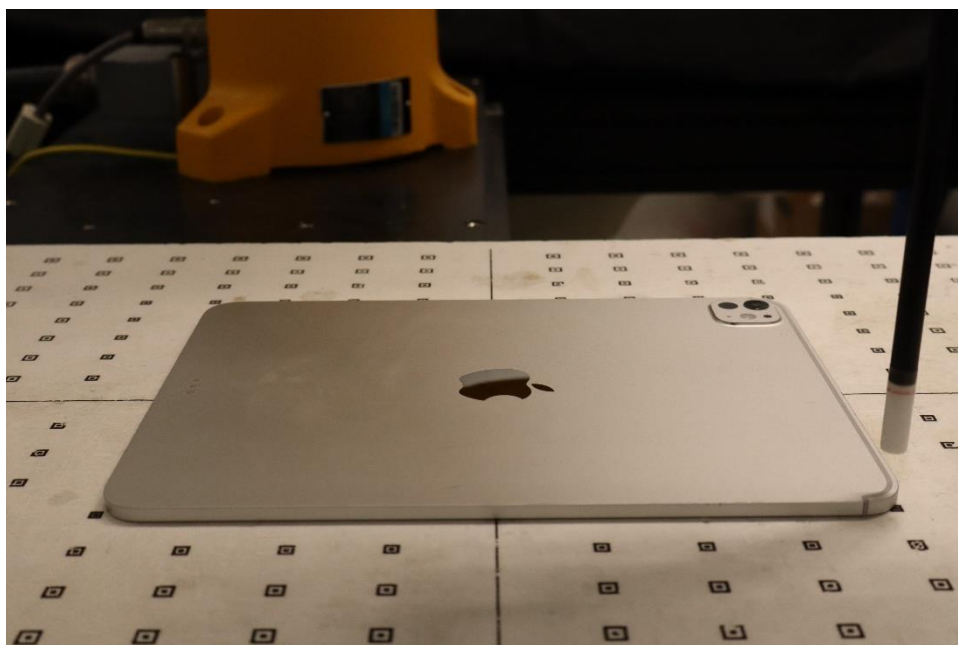
Near Field Power Density Test Setup 16: Back Side at 9.45mm – Antenna WF7
