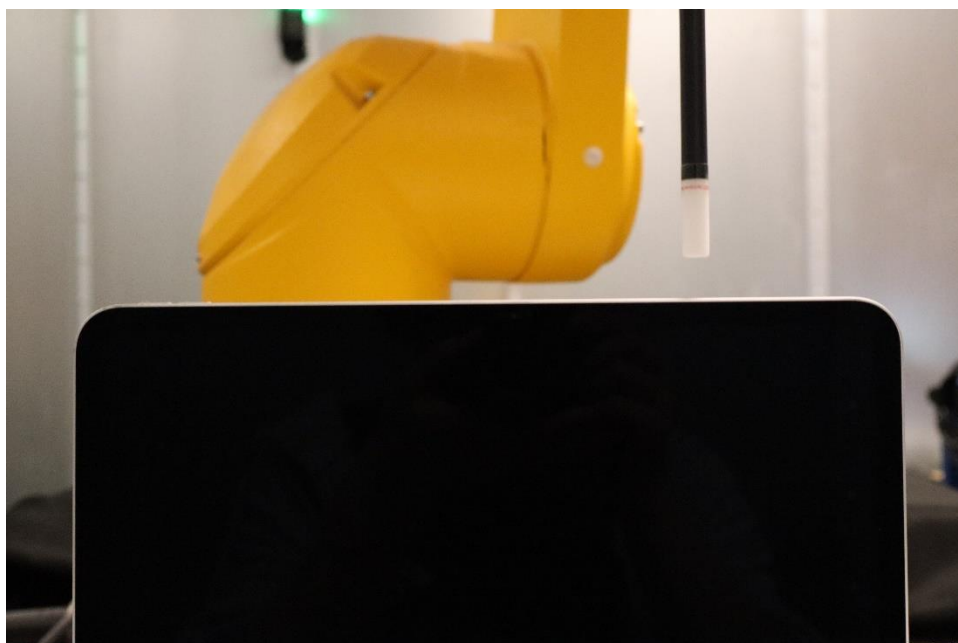
Near Field Power Density Test Setup 20: Right Edge at 9.69mm – Antenna WF5B
