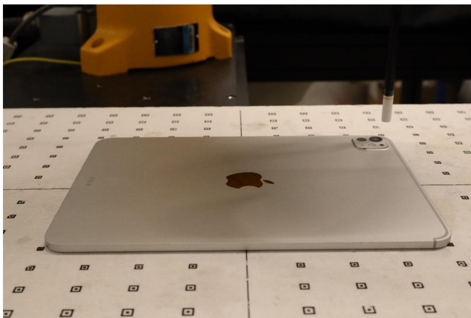
Near Field Power Density Test Setup 16: Back Side at 9.45mm – Antenna WF8
