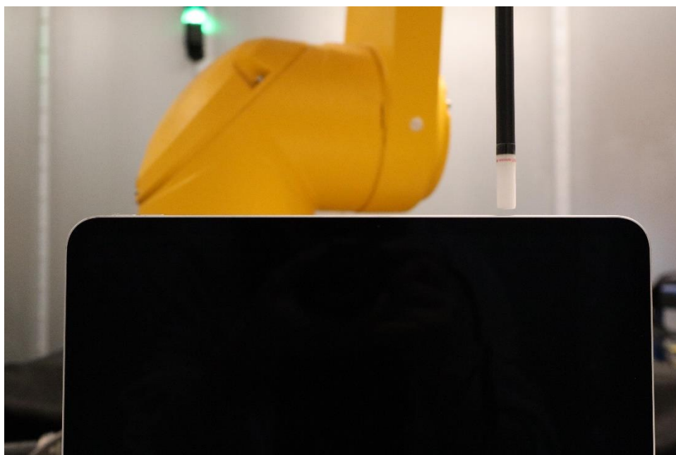
Near Field Power Density Test Setup 18: Right Edge at 2mm – Antenna WF5B
