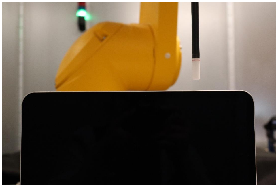
Near Field Power Density Test Setup 19: Right Edge at 9mm – Antenna WF5B
