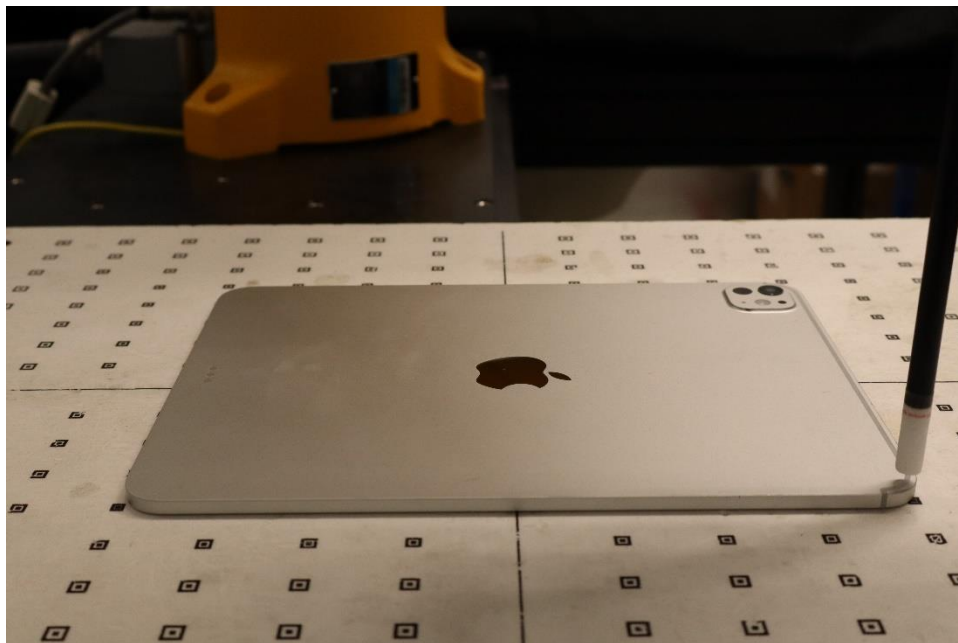
Near Field Power Density Test Setup 14: Back Side at 2mm – Antenna WF7
