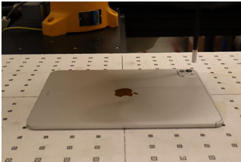
Near Field Power Density Test Setup 15: Back Side at 9mm – Antenna WF8
