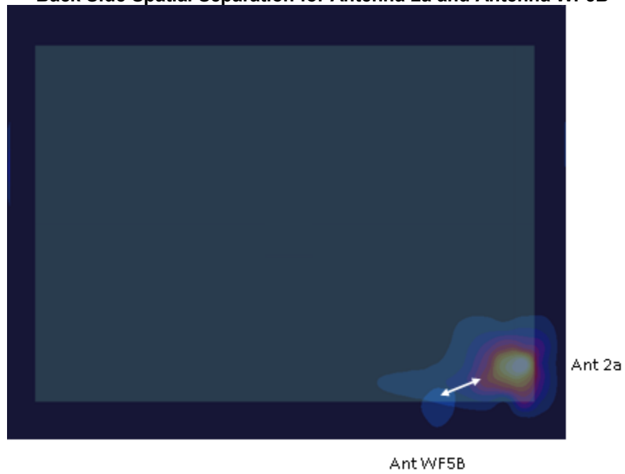
Figure F-7 Back Side Spatial Separation for Antenna 2a and Antenna WF5B
