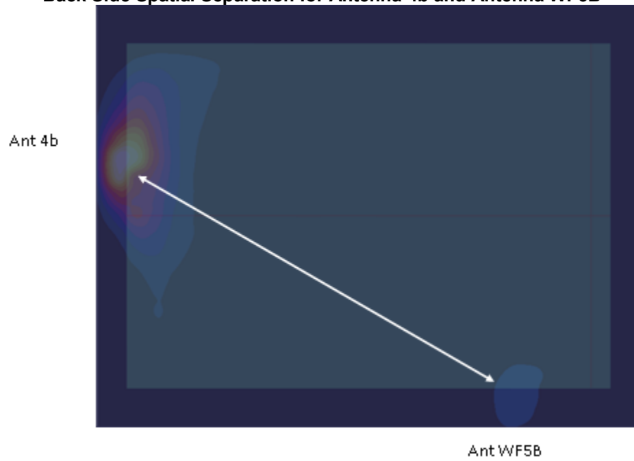
Figure F-13 Back Side Spatial Separation for Antenna 4b and Antenna WF5B
