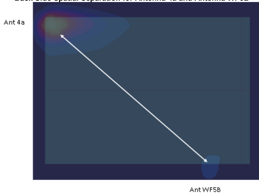
Figure F-12 Back Side Spatial Separation for Antenna 4a and Antenna WF5B
