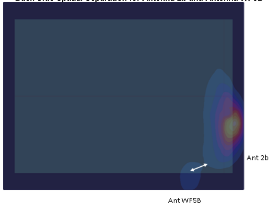
Figure F-9 Back Side Spatial Separation for Antenna 2b and Antenna WF5B
