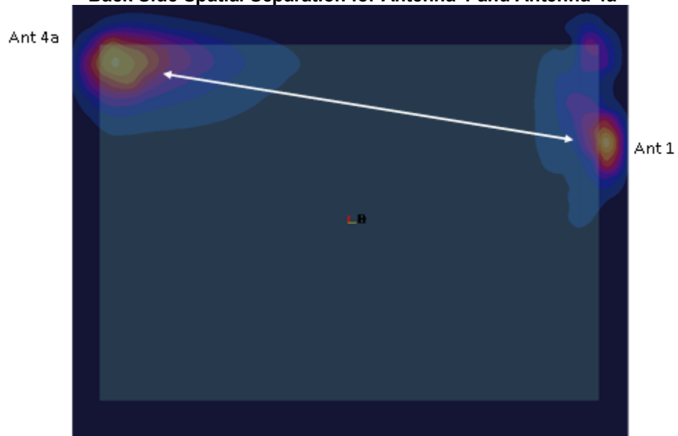
Figure F-2 Back Side Spatial Separation for Antenna 1 and Antenna 4a
