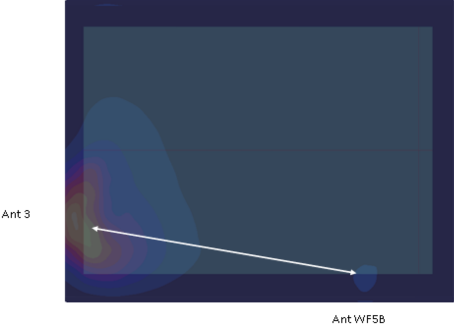
Figure F-11 Back Side Spatial Separation for Antenna 3 and Antenna WF5B
