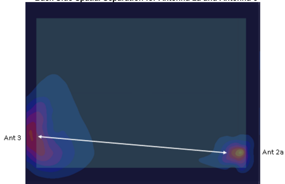
Figure F-4 Back Side Spatial Separation for Antenna 2a and Antenna 3
