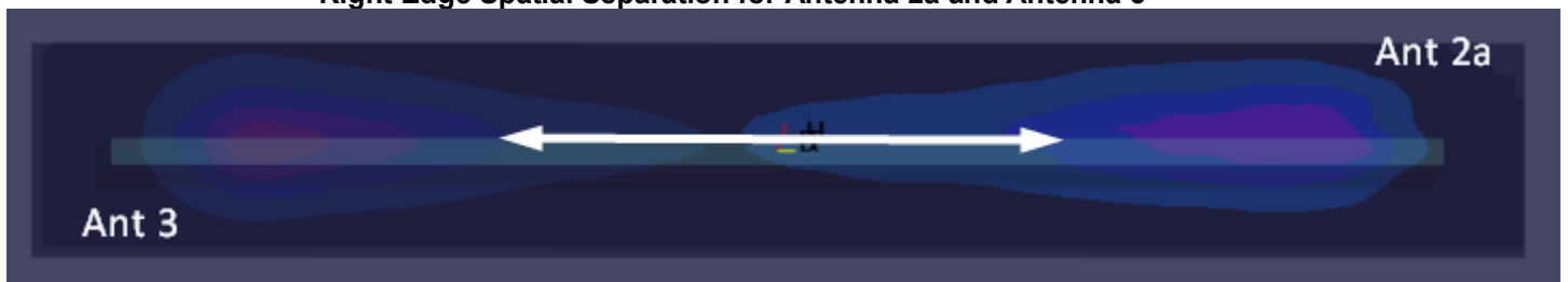
Figure F-17 Right Edge Spatial Separation for Antenna 2a and Antenna 3
