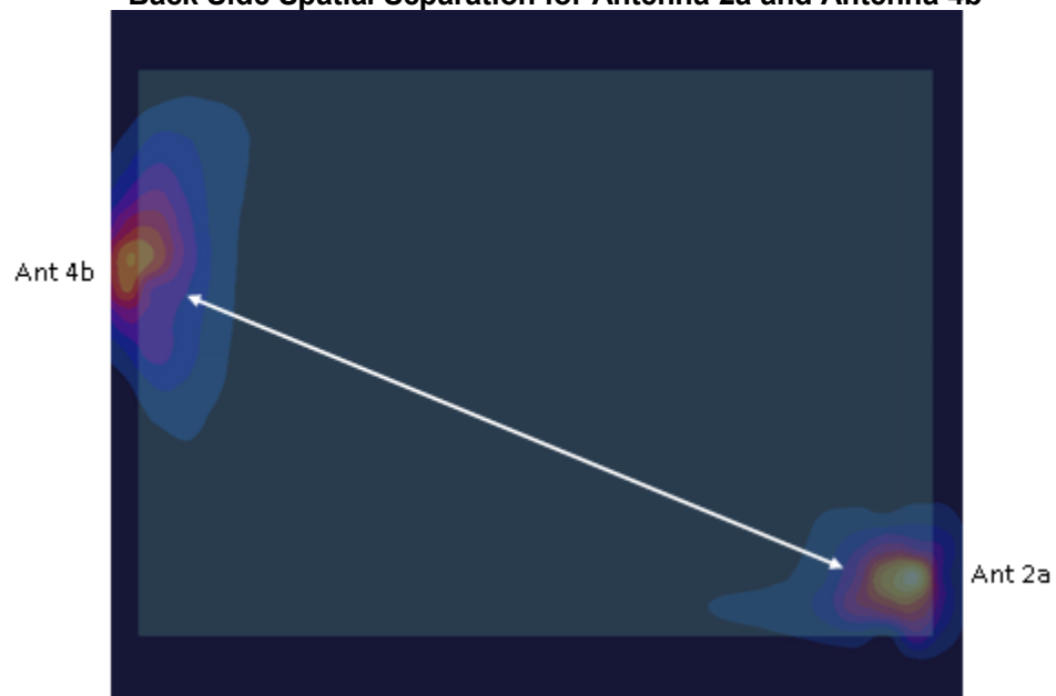
Figure F-6 Back Side Spatial Separation for Antenna 2a and Antenna 4b
