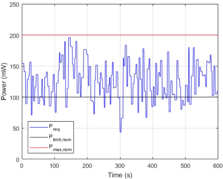
Figure E-1 Example of Pseudo-random sequence waveform
