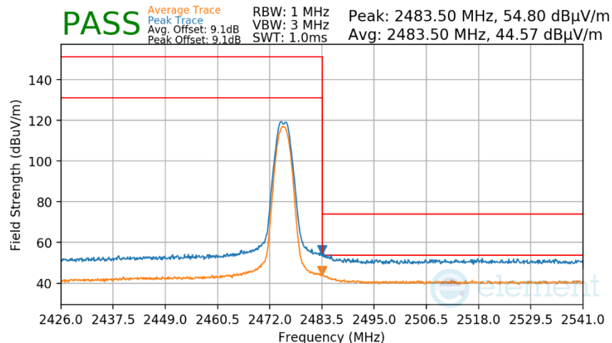
Plot 7-44. Radiated Restricted Upper Band Edge Measurement Antenna 4a
