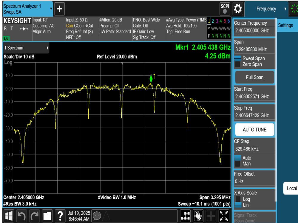
Plot 7-7. Power Spectral Density Antenna 4a (802.15.4, ePA – Ch. 11)
