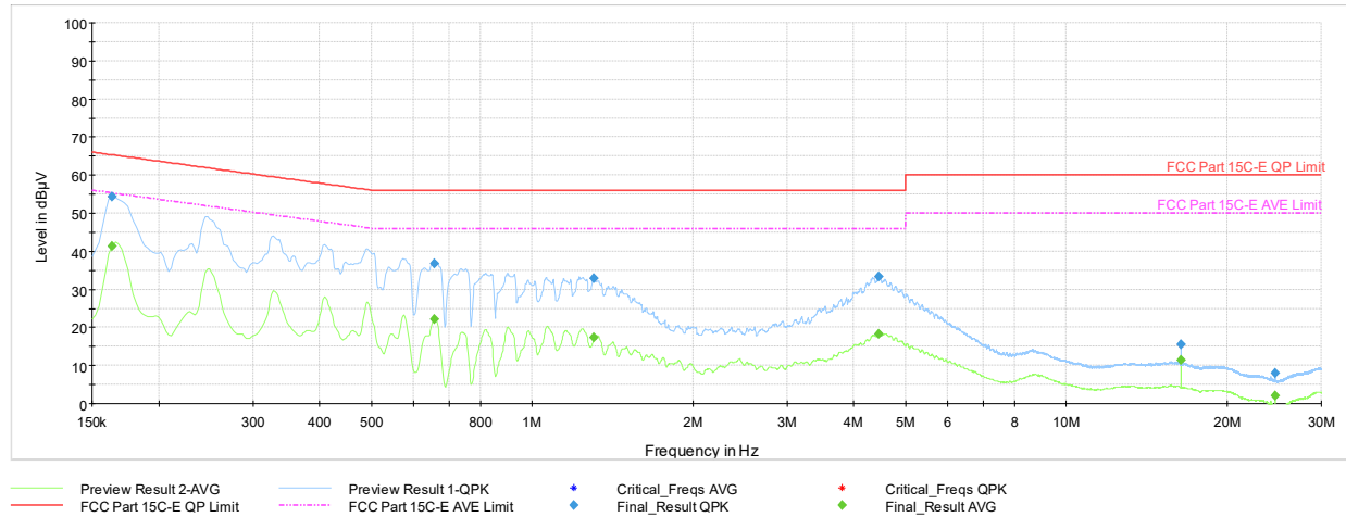
Plot 7-48. AC Line Conducted Emission with 802.15.4 Antenna 4a (L1, Ch.18 - ePA, with AC/DC Adaptor)
