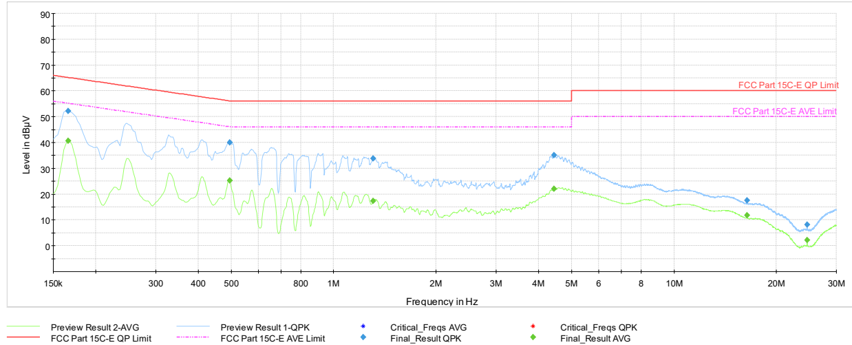
Plot 7-49. AC Line Conducted Emission with 802.15.4 Antenna 4a (N, Ch.18 - ePA, with AC/DC Adapter)
