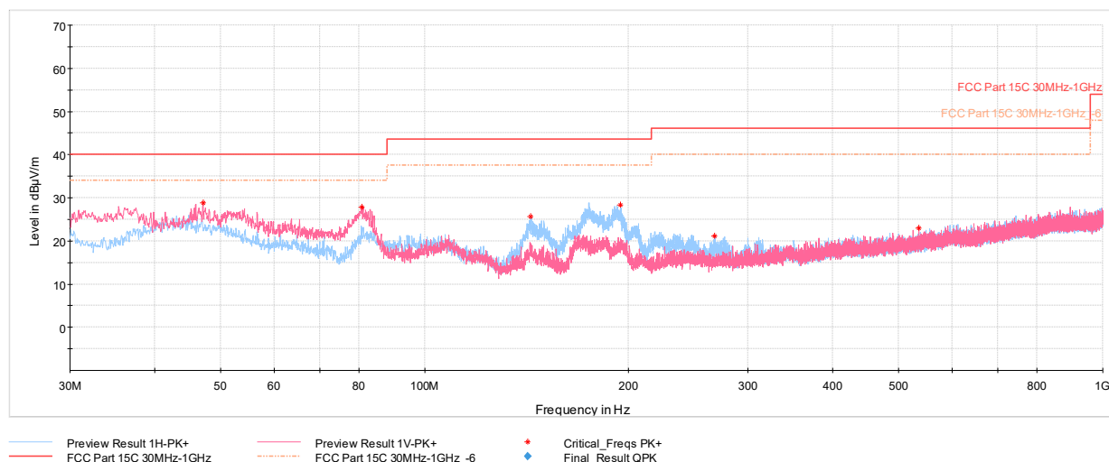
Plot 7-47. Radiated Spurious Emissions 30MHz-1GHz Antenna 4a (ePA - Ch.18, with AC/DC Adaptor)
