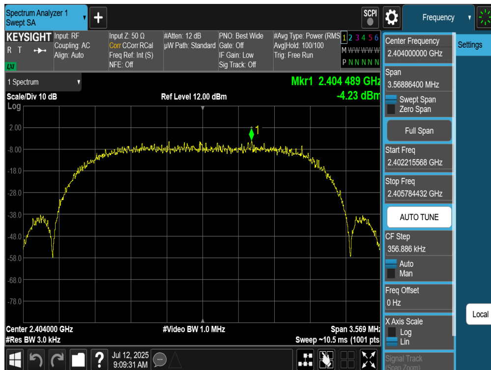
Plot 7-133. Power Spectral Density Plot TxBF Antenna 4a (Bluetooth (HDRPS2), 2Mbps, ePA – Ch. 1)
