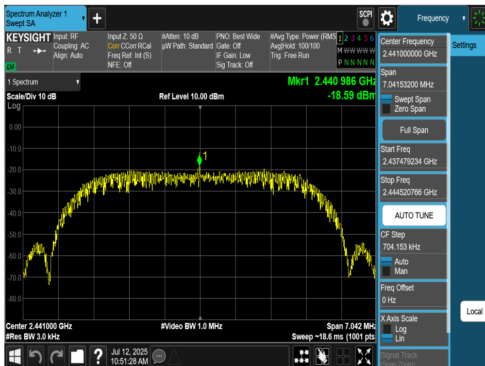
Plot 7-166. Power Spectral Density Plot Tx BF Antenna 2a (Bluetooth (HDRPM16), 16Mbps, iPA – Ch. 38)
