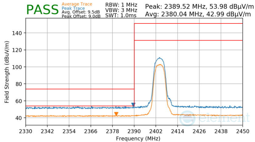
Plot 7-297. Radiated Restricted Lower Band Edge Measurement Antenna 2a
