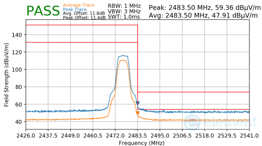
Plot 7-314. Radiated Restricted Upper Band Edge Measurement TxBF
