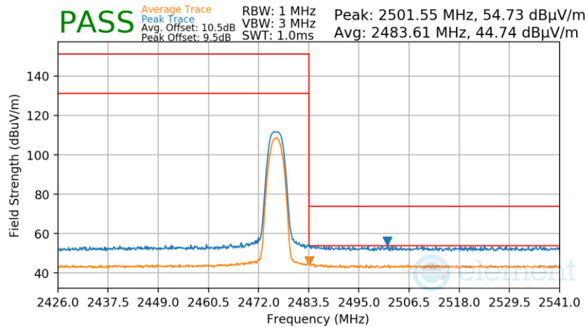
Plot 7-311. Radiated Restricted Upper Band Edge Measurement TxBF
