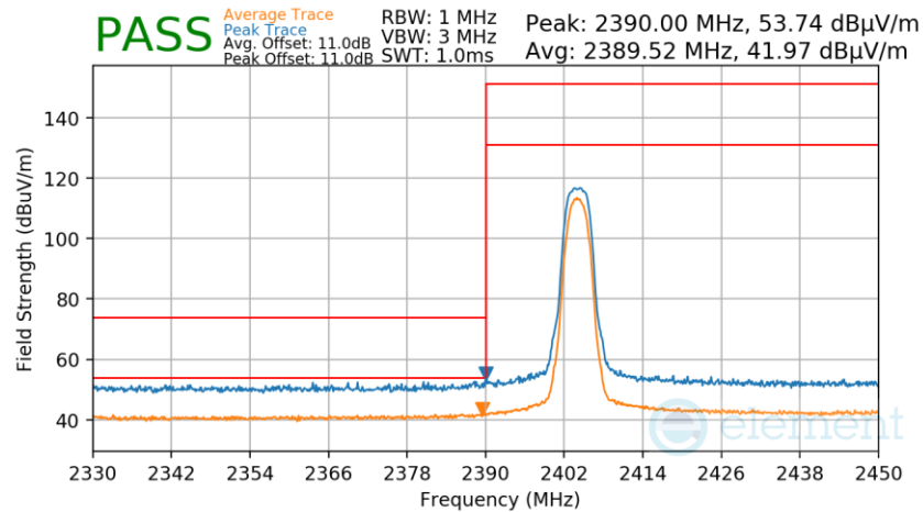
Plot 7-307. Radiated Restricted Lower Band Edge Measurement TxBF
