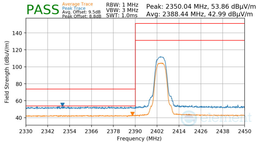
Plot 7-309. Radiated Restricted Lower Band Edge Measurement TxBF
