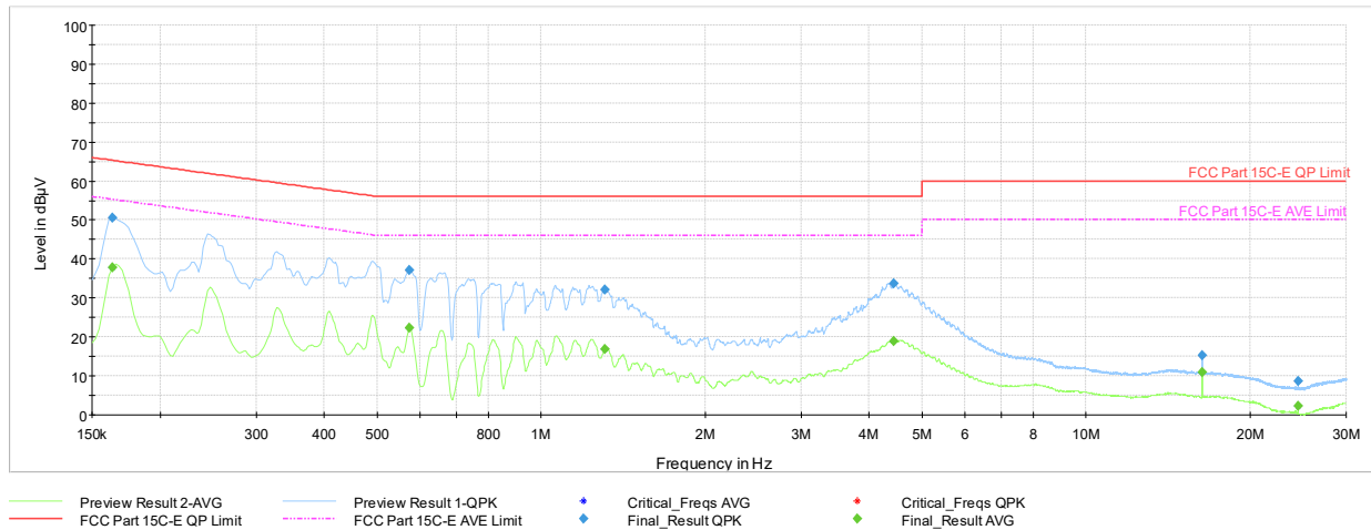
Plot 7-318. AC Line Conducted Plot with Bluetooth HDR TxBF (L1, HDR4, 4Mbps ePA - Ch.38 with AC/DC Adapter)
