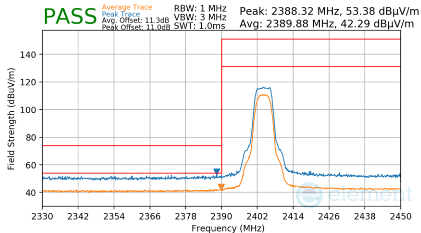
Plot 7-308. Radiated Restricted Lower Band Edge Measurement TxBF
