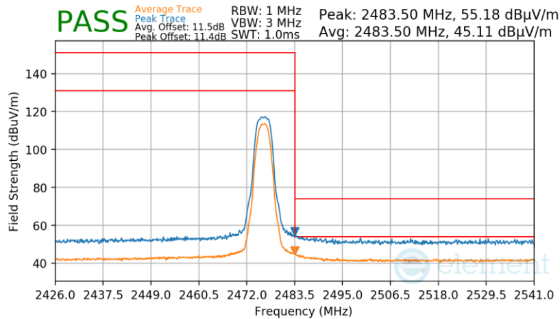
Plot 7-313. Radiated Restricted Upper Band Edge Measurement TxBF
