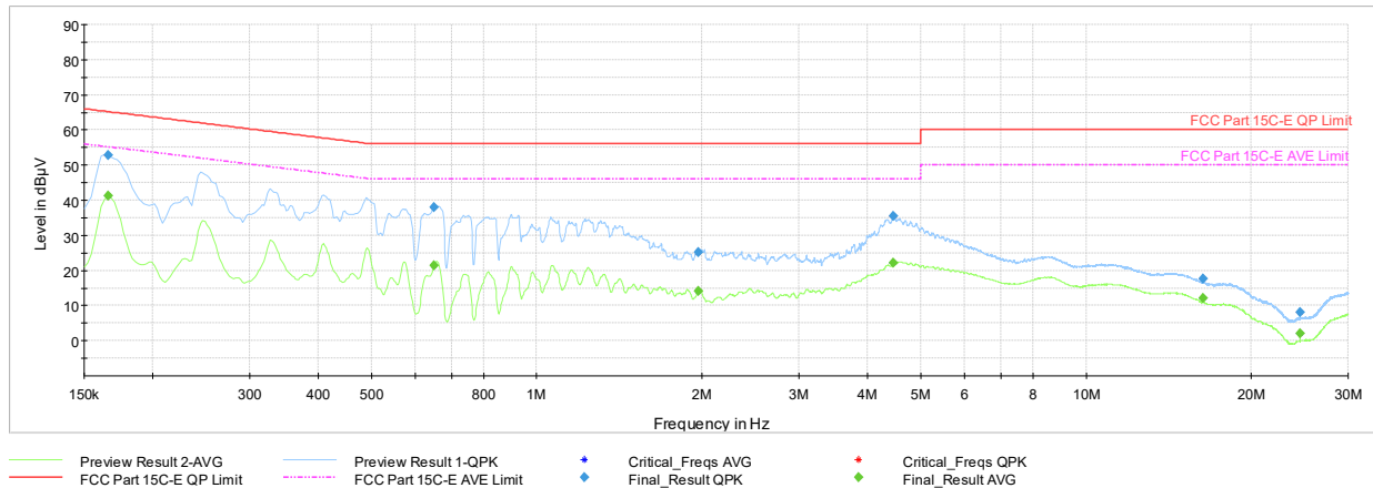
Plot 7-319. AC Line Conducted Plot with Bluetooth HDR TxBF (N, HDR4, 4Mbps ePA - Ch.38 with AC/DC Adapter)
