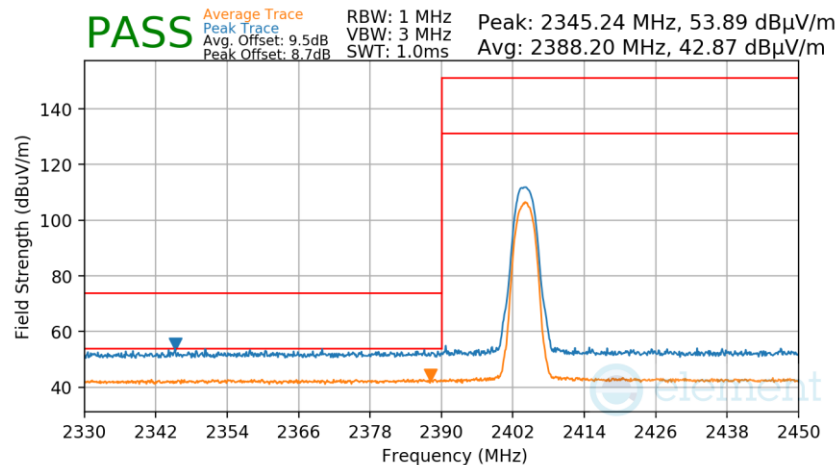
Plot 7-298. Radiated Restricted Lower Band Edge Measurement Antenna 2a
