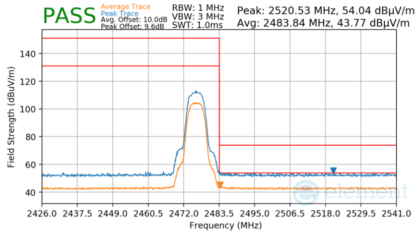
Plot 7-315. Radiated Restricted Upper Band Edge Measurement TxBF
