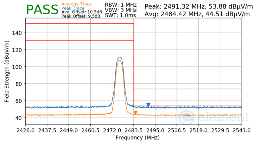
Plot 7-299. Radiated Restricted Upper Band Edge Measurement Antenna 2a
