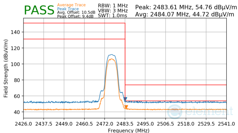
Plot 7-312. Radiated Restricted Upper Band Edge Measurement TxBF
