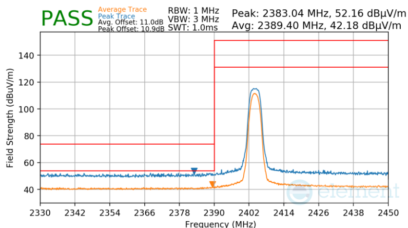
Plot 7-295. Radiated Restricted Lower Band Edge Measurement Antenna 2a
