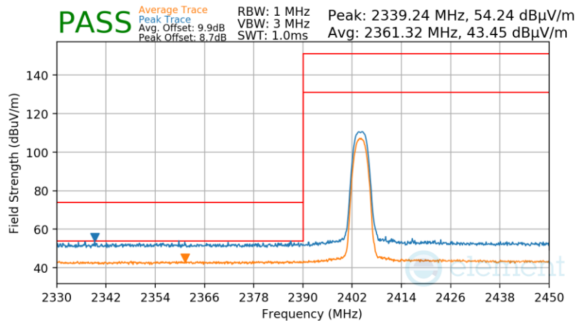
Plot 7-293. Radiated Restricted Lower Band Edge Measurement Antenna 2a
