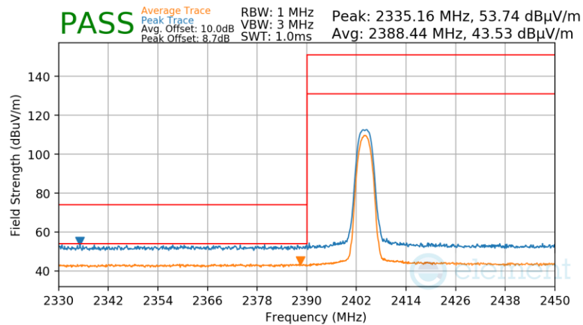
Plot 7-305. Radiated Restricted Lower Band Edge Measurement TxBF
