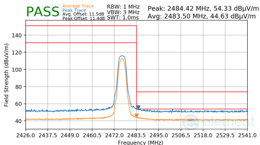
Plot 7-301. Radiated Restricted Upper Band Edge Measurement Antenna 2a
