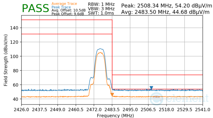
Plot 7-300. Radiated Restricted Upper Band Edge Measurement Antenna 2a
