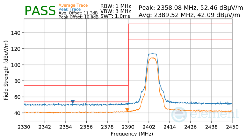
Plot 7-296. Radiated Restricted Lower Band Edge Measurement Antenna 2a
