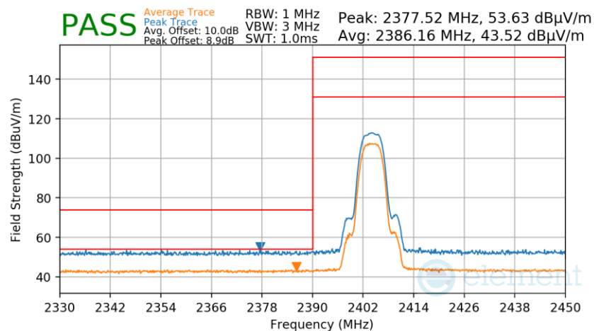
Plot 7-306. Radiated Restricted Lower Band Edge Measurement TxBF
