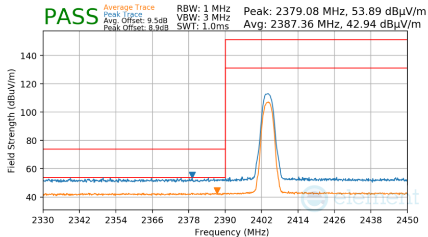
Plot 7-310. Radiated Restricted Lower Band Edge Measurement TxBF
