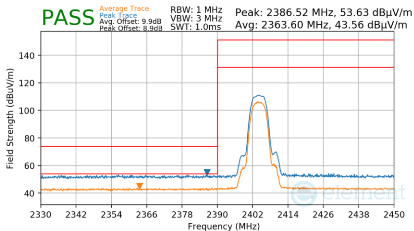
Plot 7-294. Radiated Restricted Lower Band Edge Measurement Antenna 2a
