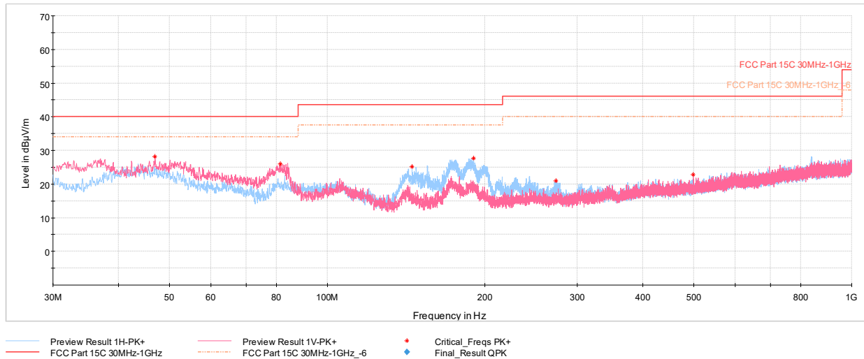
Plot 7-317. Radiated Spurious Emissions Below 1GHz TxBF (HDR4, 4Mbps, ePA – Ch.38 with AC/DC Adapter)
