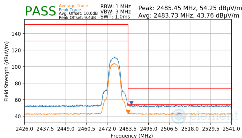
Plot 7-303. Radiated Restricted Upper Band Edge Measurement Antenna 2a
