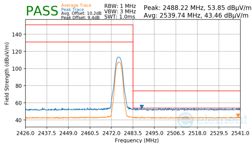
Plot 7-316. Radiated Restricted Upper Band Edge Measurement TxBF
