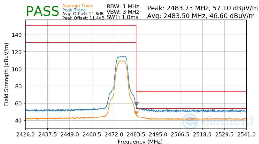
Plot 7-302. Radiated Restricted Upper Band Edge Measurement Antenna 2a
