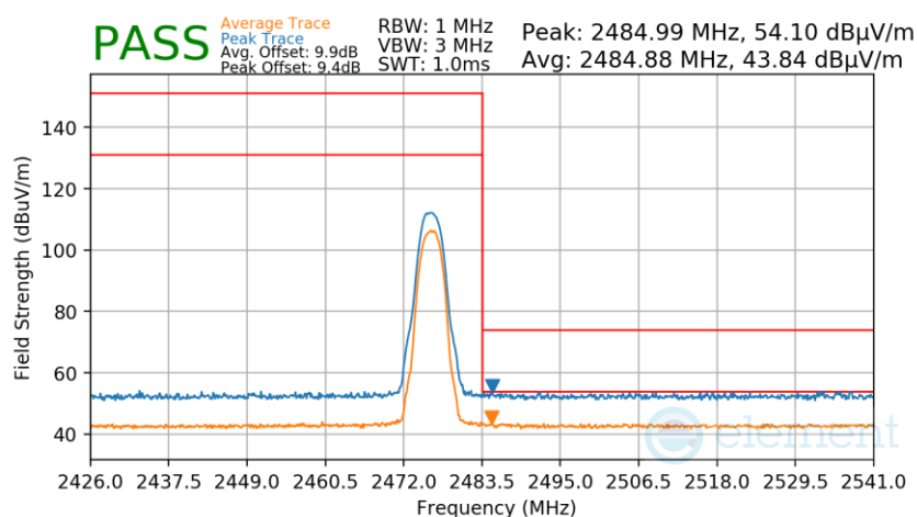
Plot 7-304. Radiated Restricted Upper Band Edge Measurement Antenna 2a
