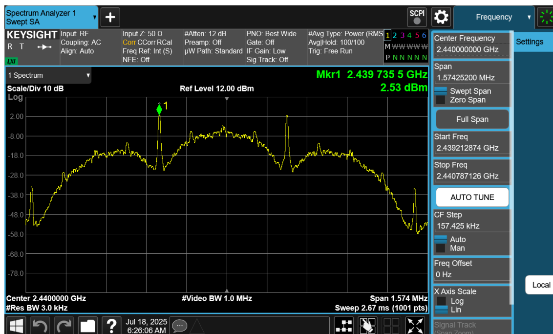
Plot 7-81. Power Spectral Density Plot Antenna 4a (Bluetooth (LE), 125kbps, iPA – Ch. 19)
