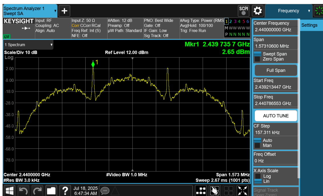
Plot 7-82. Power Spectral Density Plot Antenna 2a (Bluetooth (LE), 125kbps, iPA – Ch. 19)
