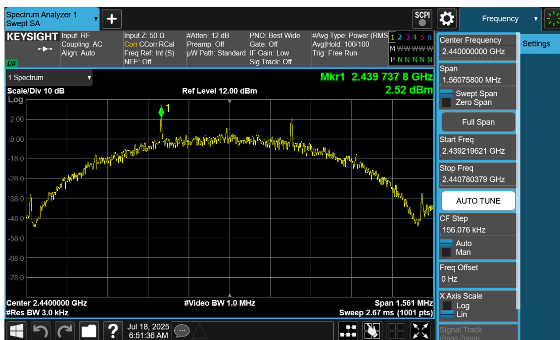
Plot 7-94. Power Spectral Density Plot Antenna 2a (Bluetooth (LE), 500kbps, iPA – Ch. 19)
