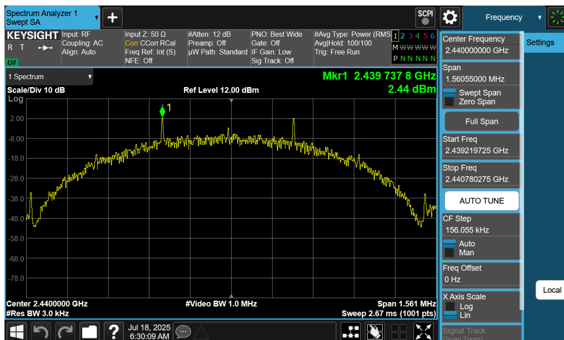
Plot 7-93. Power Spectral Density Plot Antenna 4a (Bluetooth (LE), 500kbps, iPA – Ch. 19)
