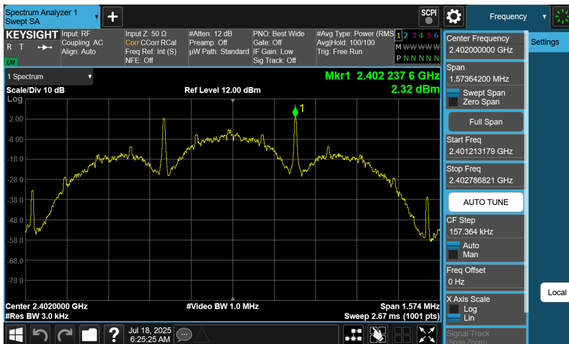
Plot 7-79. Power Spectral Density Plot Antenna 4a (Bluetooth (LE), 125kbps, iPA – Ch. 0)
