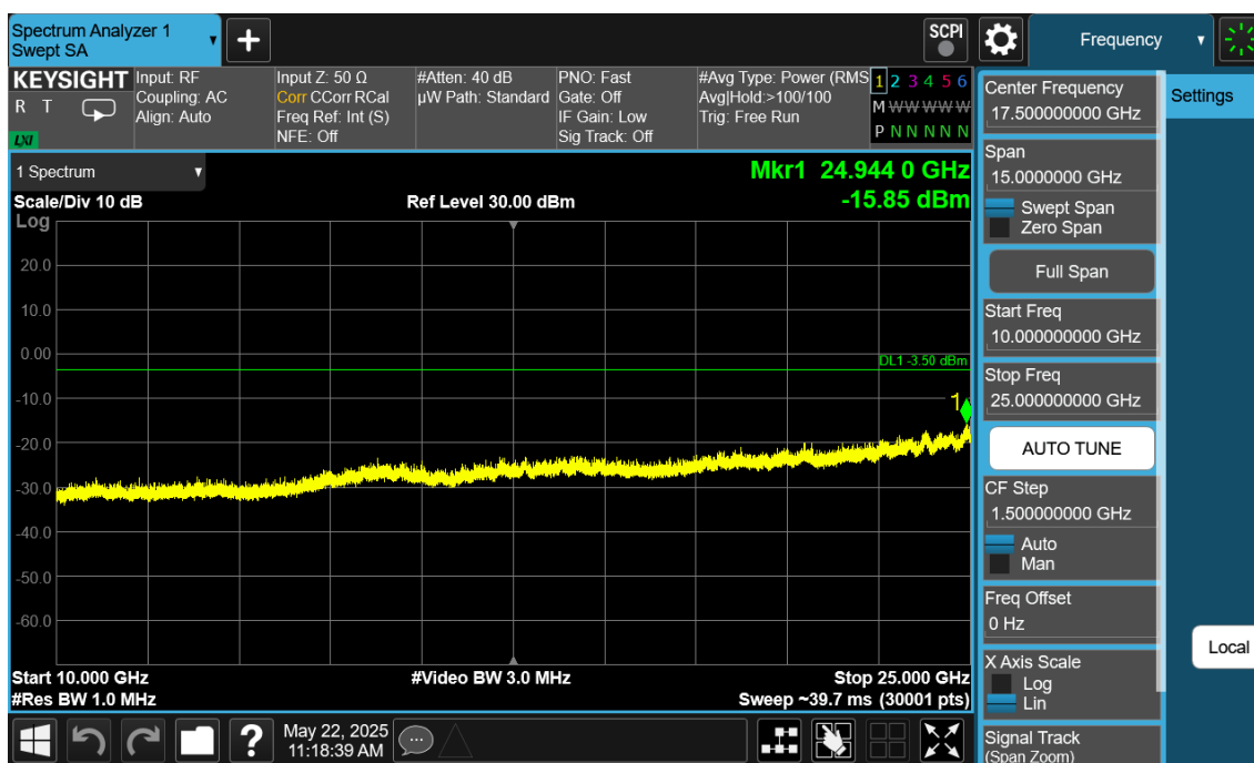
Plot 7-142. Conducted Spurious Plot Antenna 4a (Bluetooth (LE), 2Mbps, ePA – Ch. 38)
