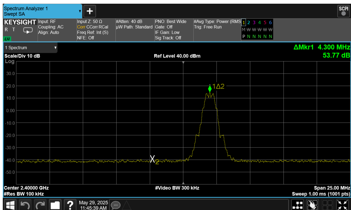
Plot 7-129. Band Edge Plot Antenna 2a (Bluetooth (LE), 125kbps, ePA – Ch.0)
