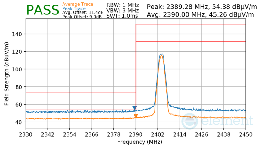
Plot 7-159. Radiated Restricted Lower Band Edge Measurement Antenna 4a (Average & Peak)
