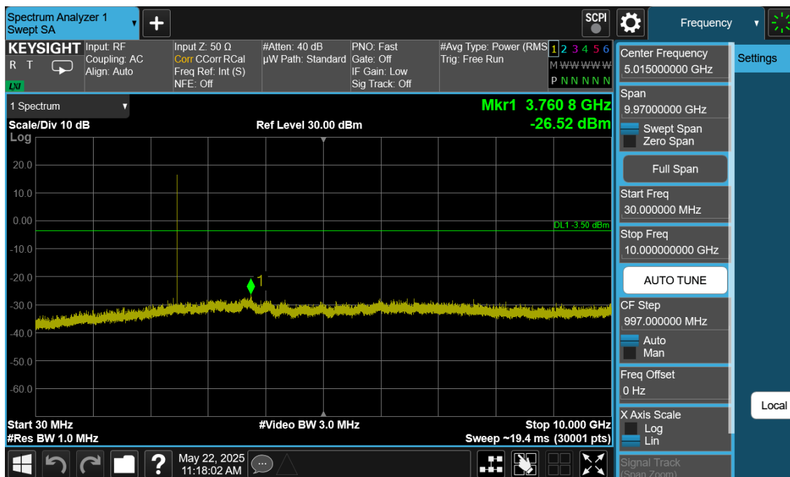
Plot 7-141. Conducted Spurious Plot Antenna 4a (Bluetooth (LE), 2Mbps, ePA – Ch. 38)
