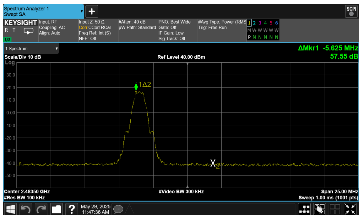
Plot 7-132. Band Edge Plot Antenna 2a (Bluetooth (LE), 500kbps, ePA – Ch. 39)
