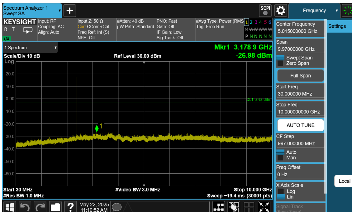
Plot 7-137. Conducted Spurious Plot Antenna 4a (Bluetooth (LE), 1Mbps, ePA – Ch. 0)
