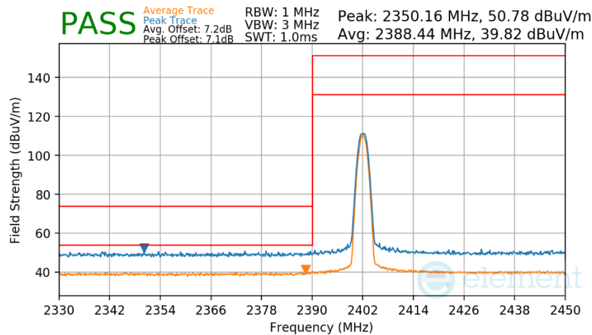
Plot 7-153. Radiated Restricted Lower Band Edge Measurement Antenna 4a (Average & Peak)
