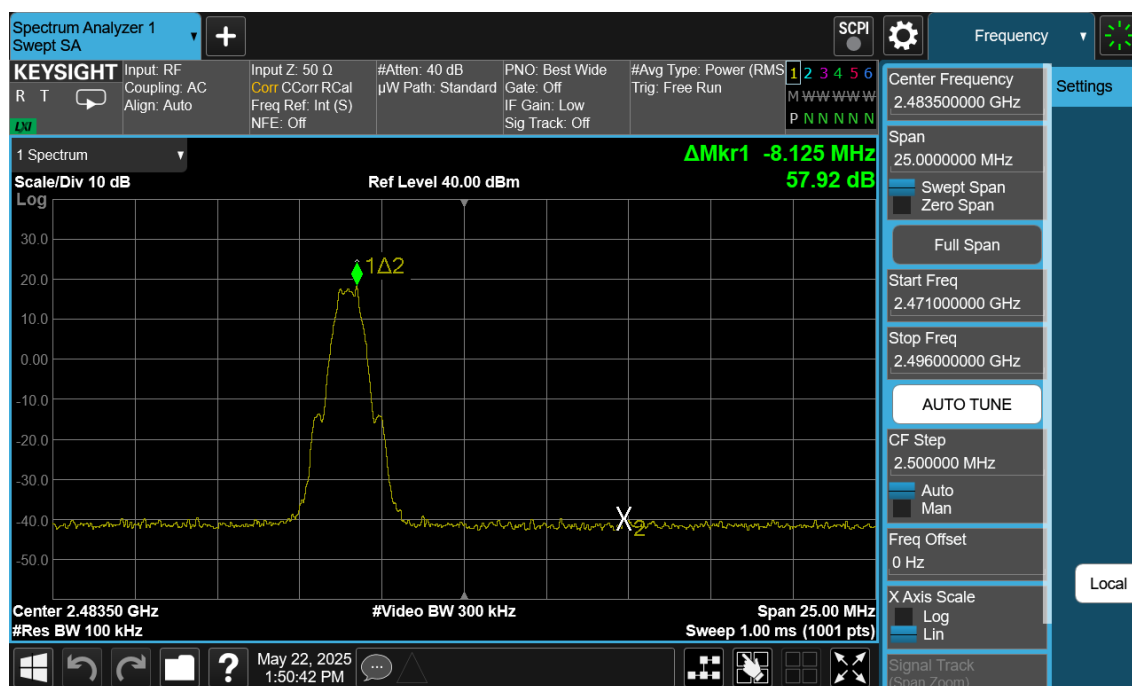
Plot 7-134. Band Edge Plot Antenna 2a (Bluetooth (LE), 1Mbps, ePA – Ch. 39)
