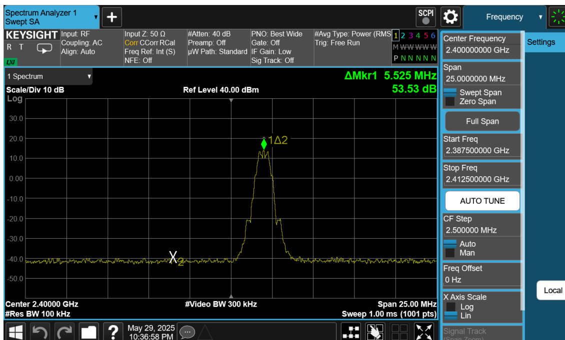
Plot 7-121. Band Edge Plot Antenna 4a (Bluetooth (LE), 125kbps, ePA – Ch.0)
