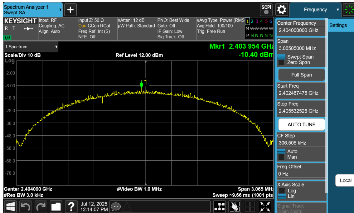
Plot 7-115. Power Spectral Density Plot Antenna 4a (Bluetooth (LE), 2Mbps, iPA – Ch. 1)
