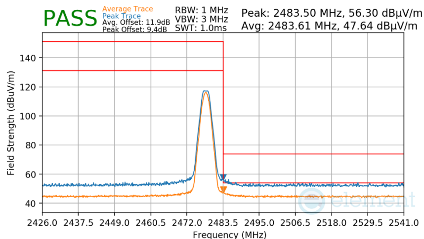
Plot 7-160. Radiated Restricted Upper Band Edge Measurement Antenna 4a (Average & Peak)
