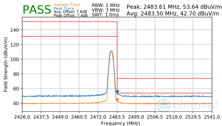
Plot 7-154. Radiated Restricted Upper Band Edge Measurement Antenna 4a (Average & Peak)
