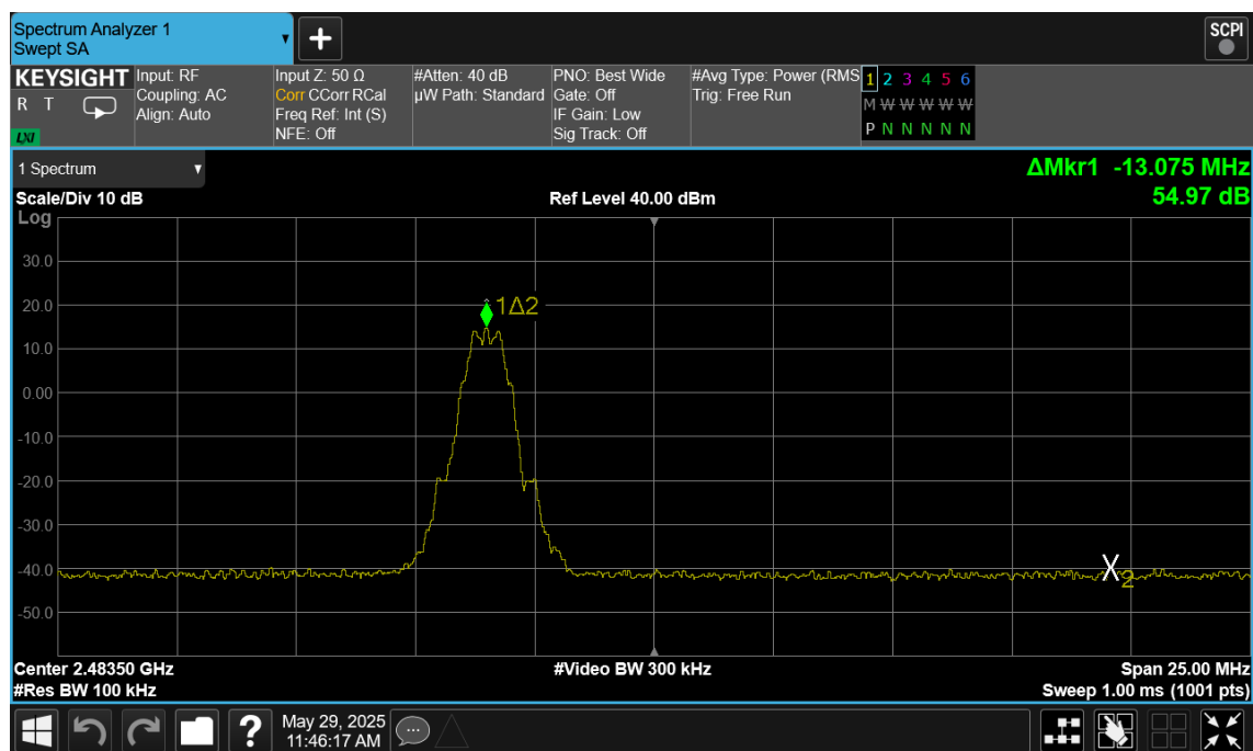
Plot 7-130. Band Edge Plot Antenna 2a (Bluetooth (LE), 125kbps, ePA – Ch. 39)
