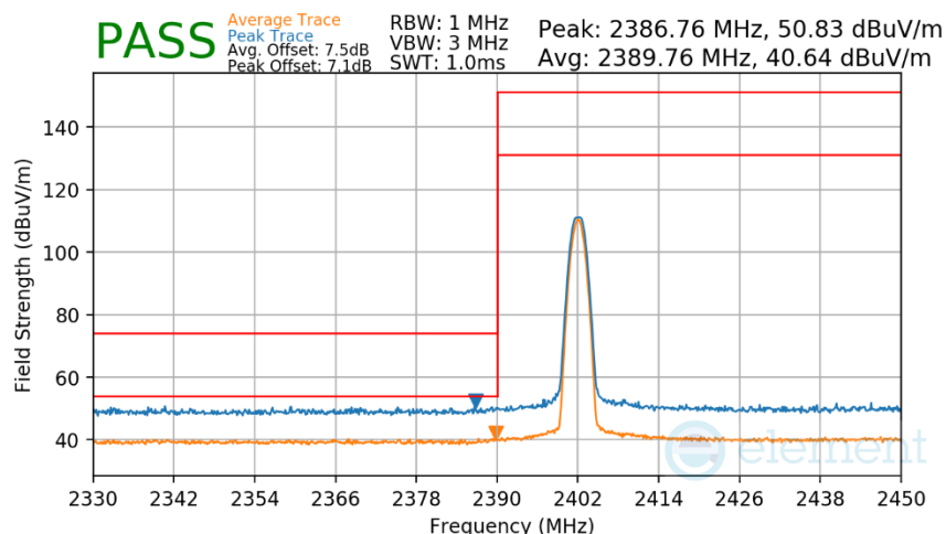
Plot 7-155. Radiated Restricted Lower Band Edge Measurement Antenna 4a (Average & Peak)
