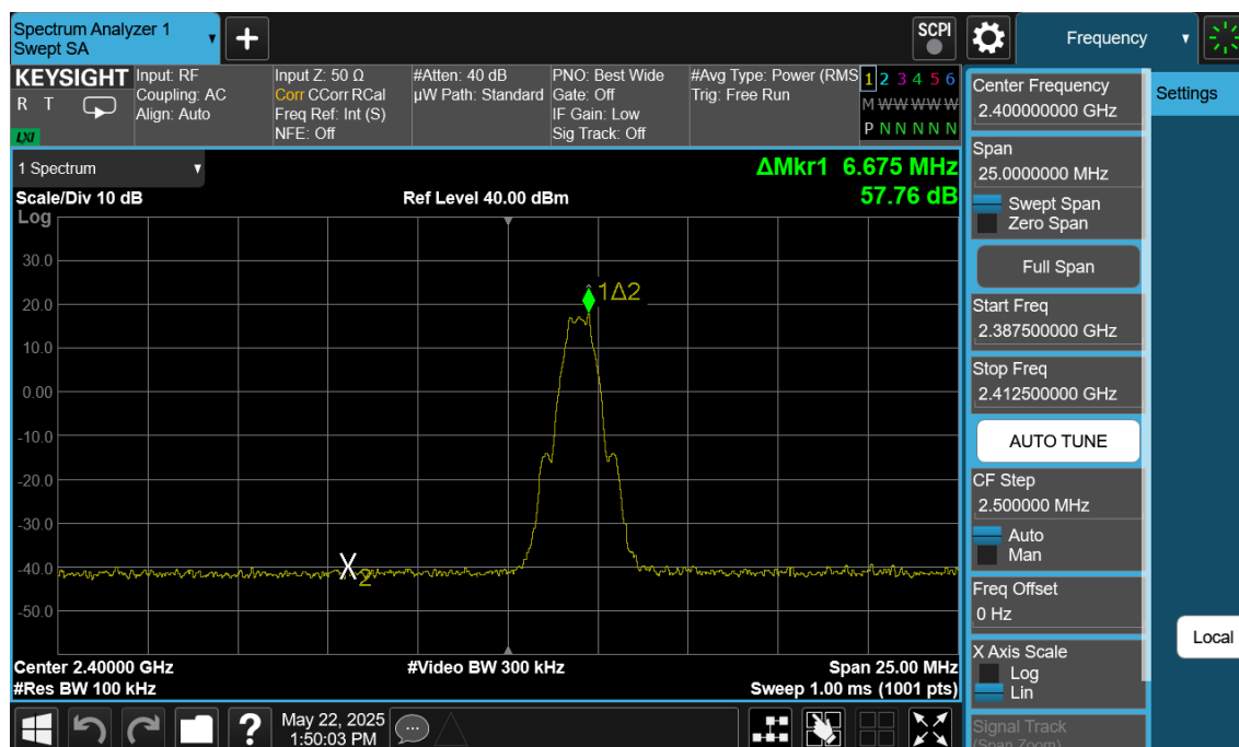
Plot 7-133. Band Edge Plot Antenna 2a (Bluetooth (LE), 1Mbps, ePA – Ch.0)
