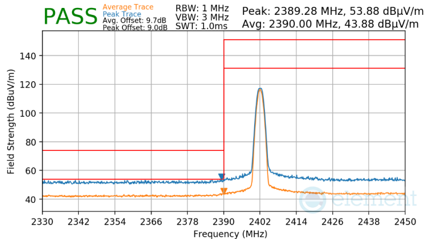
Plot 7-157. Radiated Restricted Lower Band Edge Measurement Antenna 4a (Average & Peak)
