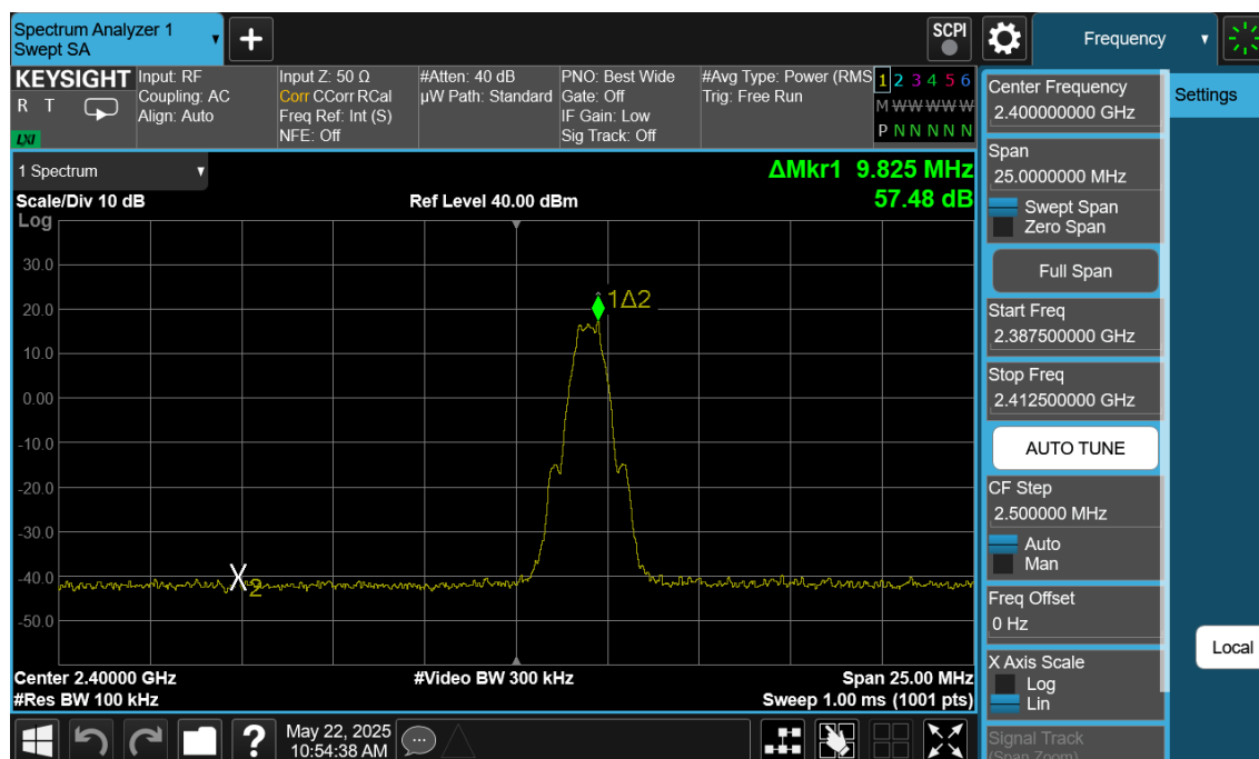
Plot 7-125. Band Edge Plot Antenna 4a (Bluetooth (LE), 1Mbps, ePA – Ch.0)
