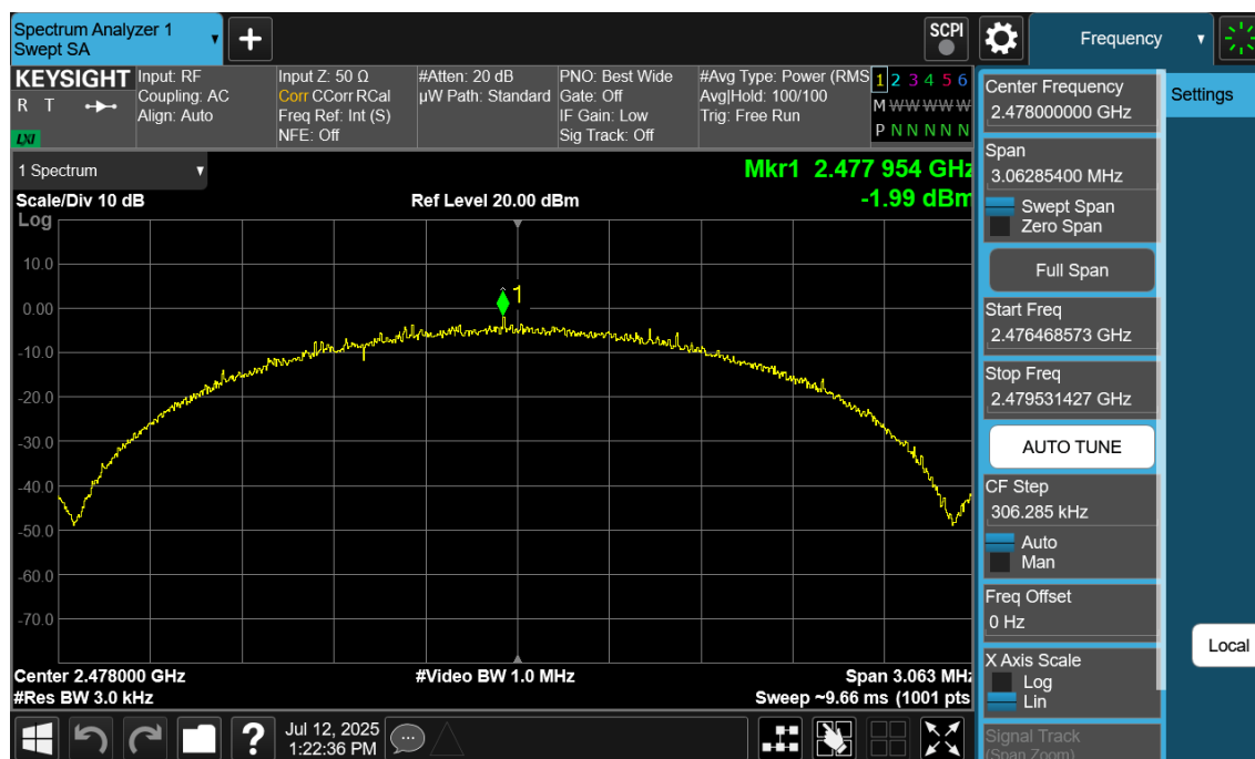
Plot 7-114. Power Spectral Density Plot Antenna 2a (Bluetooth (LE), 2Mbps, ePA – Ch. 38)
