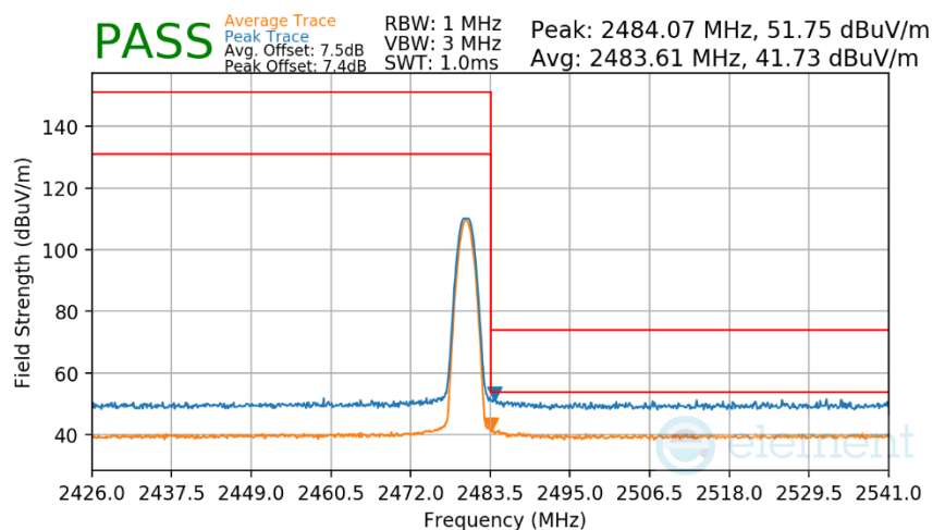
Plot 7-162. Radiated Restricted Upper Band Edge Measurement Antenna 2a (Average & Peak)
