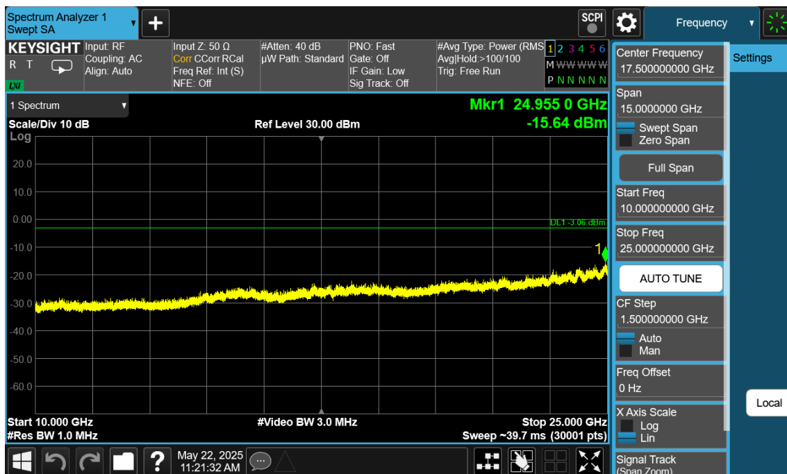
Plot 7-140. Conducted Spurious Plot Antenna 4a (Bluetooth (LE), 125kbps, ePA – Ch. 19)
