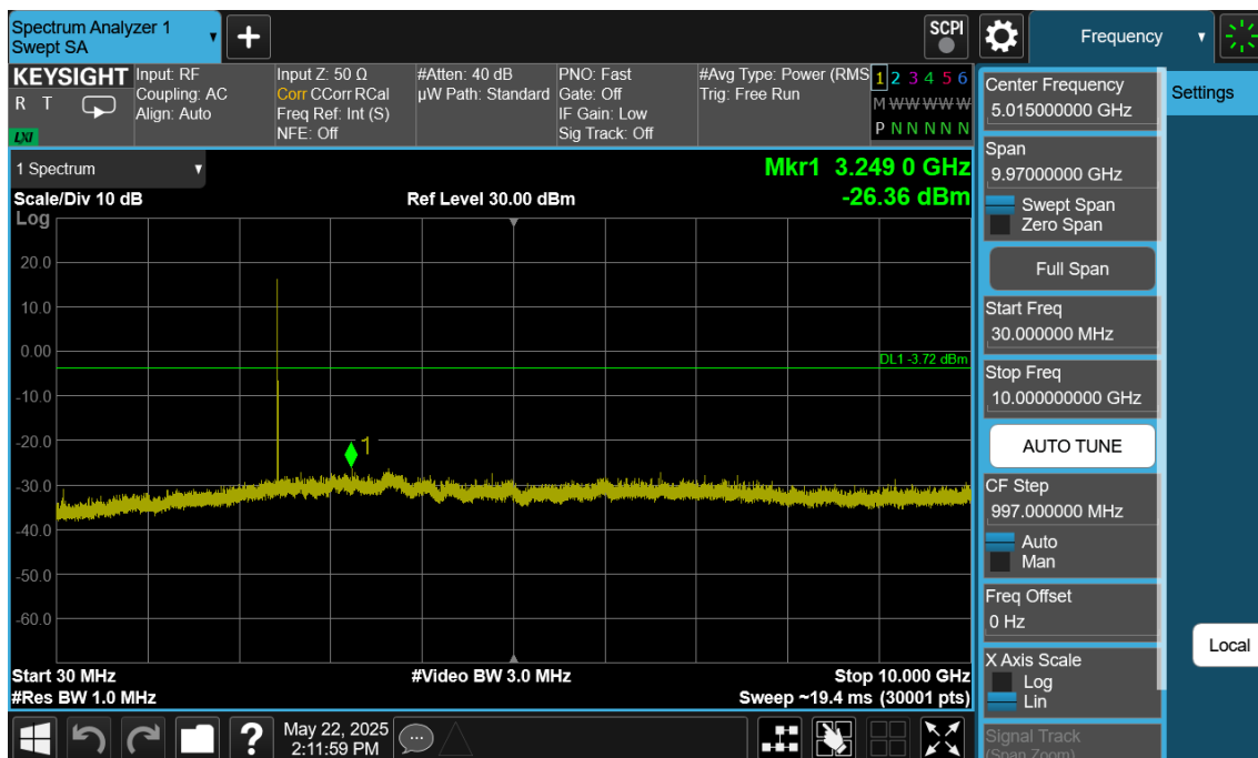
Plot 7-145. Conducted Spurious Plot Antenna 2a (Bluetooth (LE), 2Mbps, ePA – Ch. 19)
