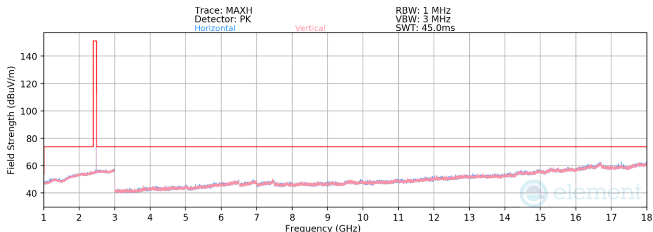
Plot 7-152. Radiated Spurious Emissions 1-18GHz TxBF (1Mbps ePA – Ch. 39)
