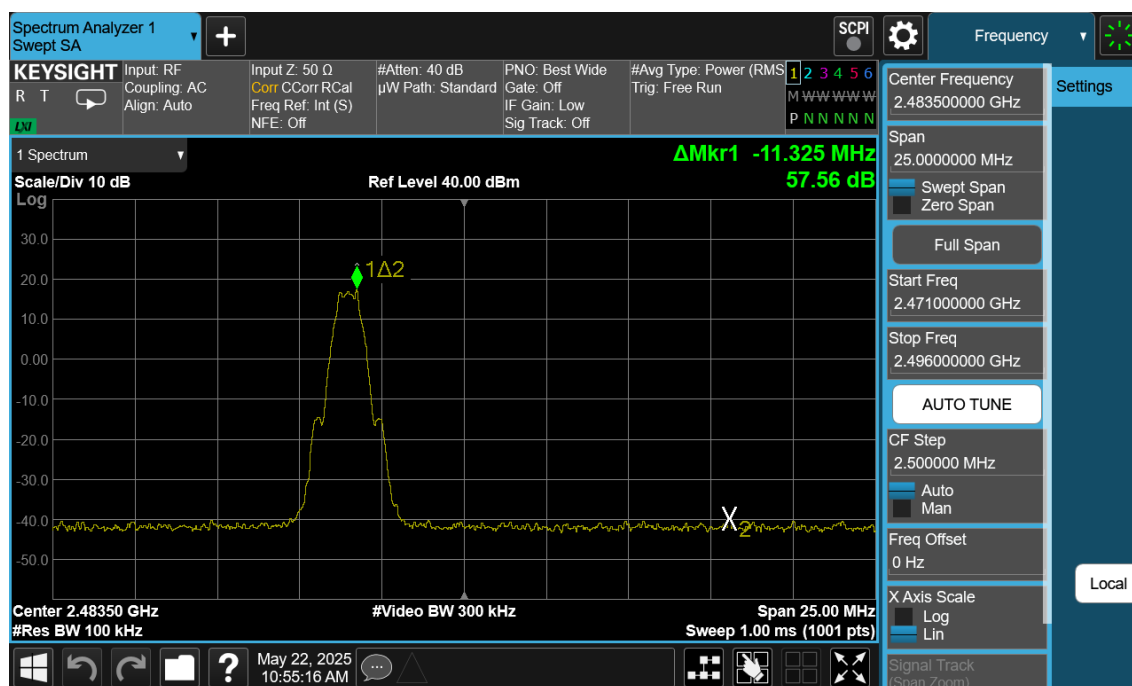
Plot 7-126. Band Edge Plot Antenna 4a (Bluetooth (LE), 1Mbps, ePA – Ch. 39)
