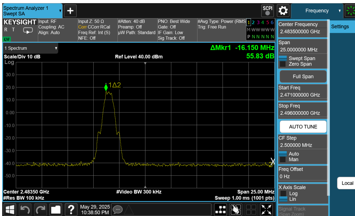
Plot 7-124. Band Edge Plot Antenna 4a (Bluetooth (LE), 500kbps, ePA – Ch. 39)
