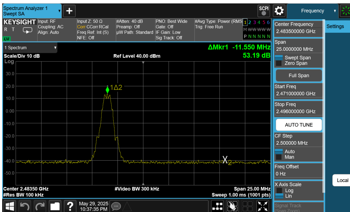
Plot 7-122. Band Edge Plot Antenna 4a (Bluetooth (LE), 125kbps, ePA – Ch. 39)
