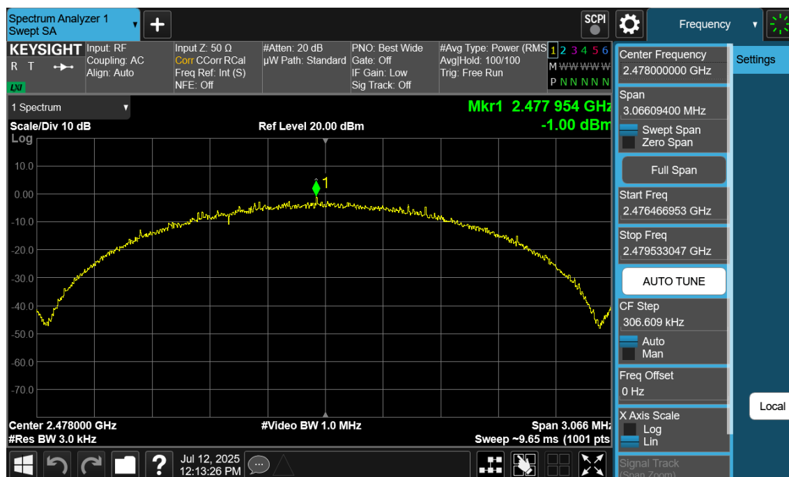
Plot 7-113. Power Spectral Density Plot Antenna 4a (Bluetooth (LE), 2Mbps, ePA – Ch. 38)
