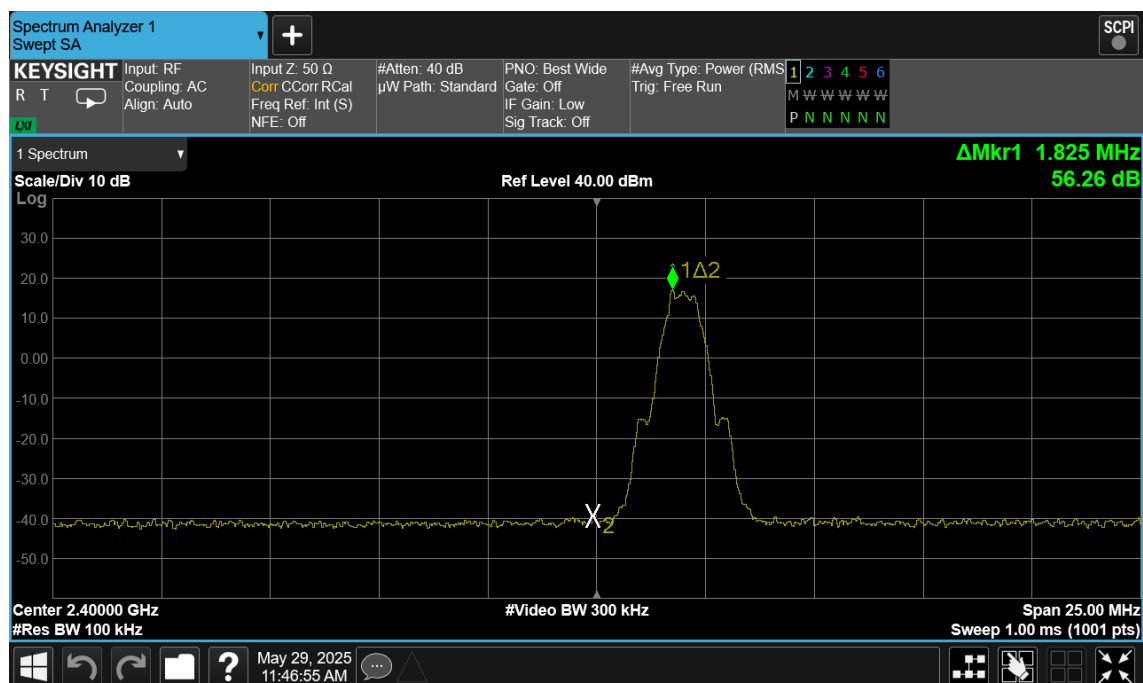
Plot 7-131. Band Edge Plot Antenna 2a (Bluetooth (LE), 500kbps, ePA – Ch.0)
