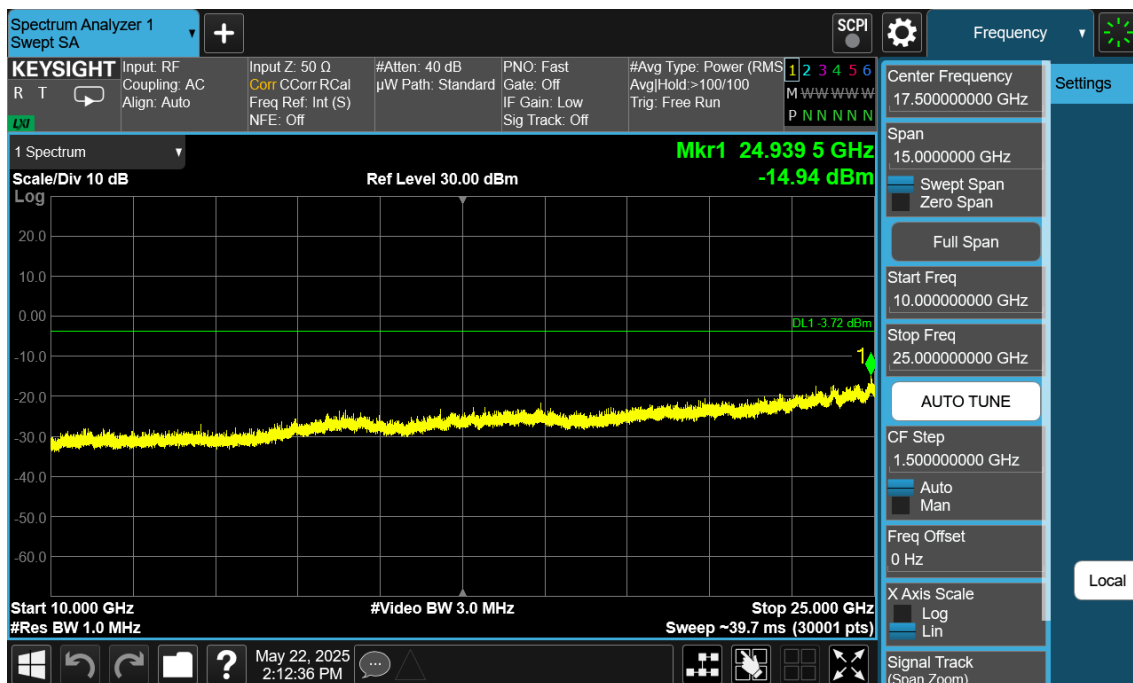
Plot 7-146. Conducted Spurious Plot Antenna 2a (Bluetooth (LE), 2Mbps, ePA – Ch. 19)
