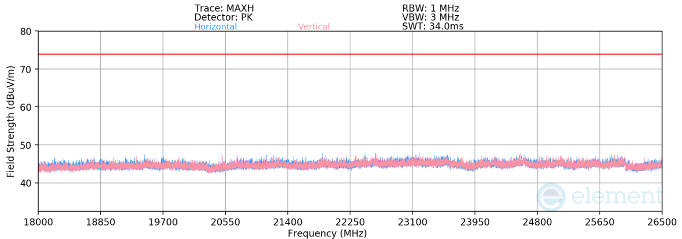
Plot 7-151. Radiated Spurious Emissions Above 18GHz TxBF (1Mbps ePA – Ch. 19)
