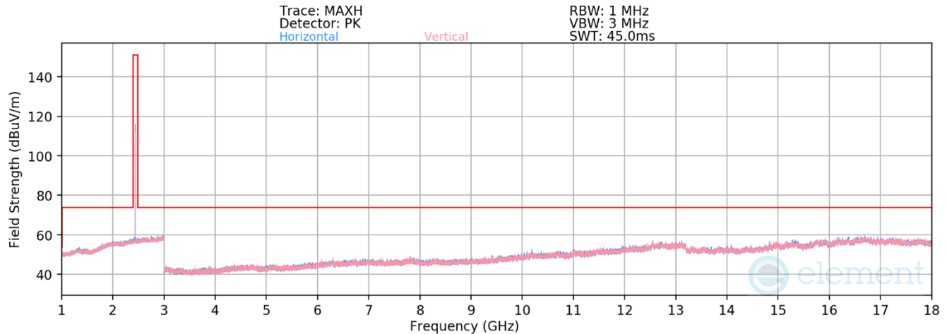
Plot 7-150. Radiated Spurious Emissions 1-18GHz TxBF (1Mbps, ePA – Ch. 19)
