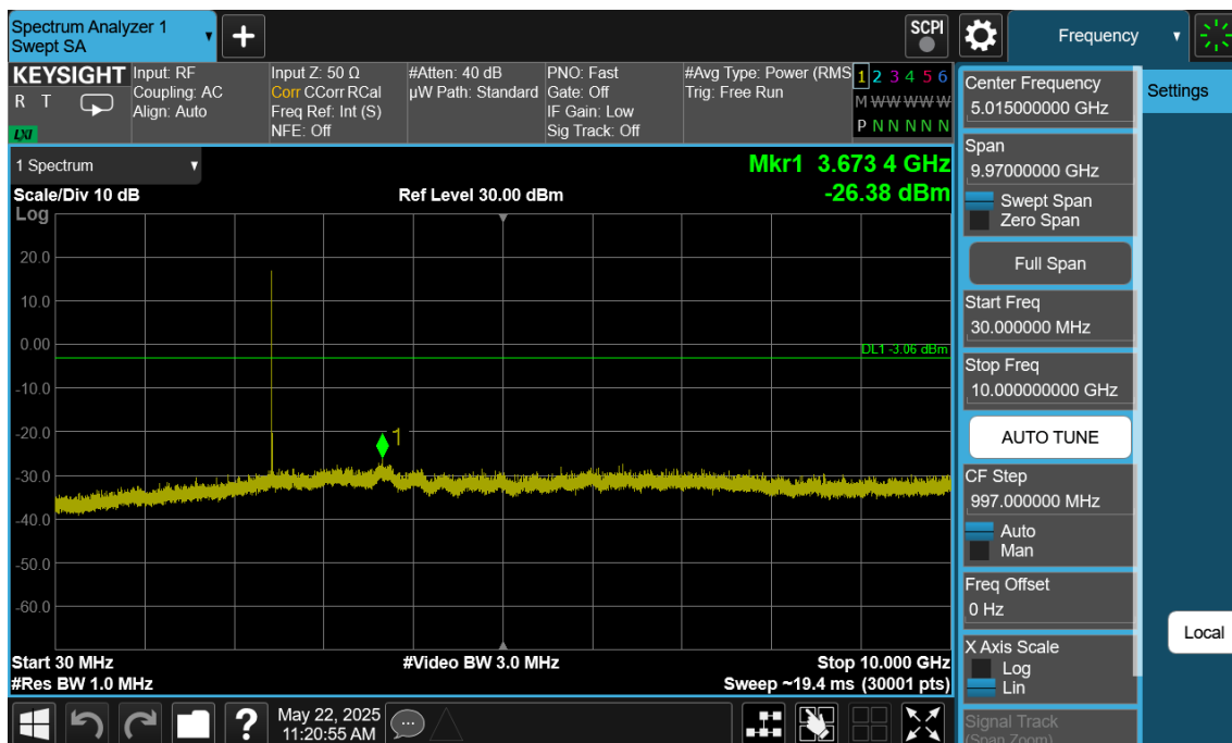
Plot 7-139. Conducted Spurious Plot Antenna 4a (Bluetooth (LE), 125kbps, ePA – Ch. 19)
