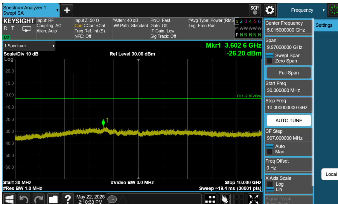
Plot 7-143. Conducted Spurious Plot Antenna 2a (Bluetooth (LE), 2Mbps, ePA – Ch. 1)
