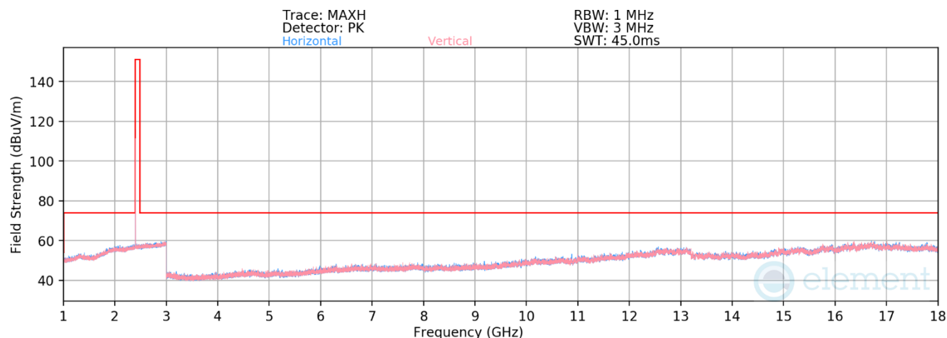
Plot 7-149. Radiated Spurious Emissions 1-18GHz TxBF (1Mbps, ePA – Ch. 0)
