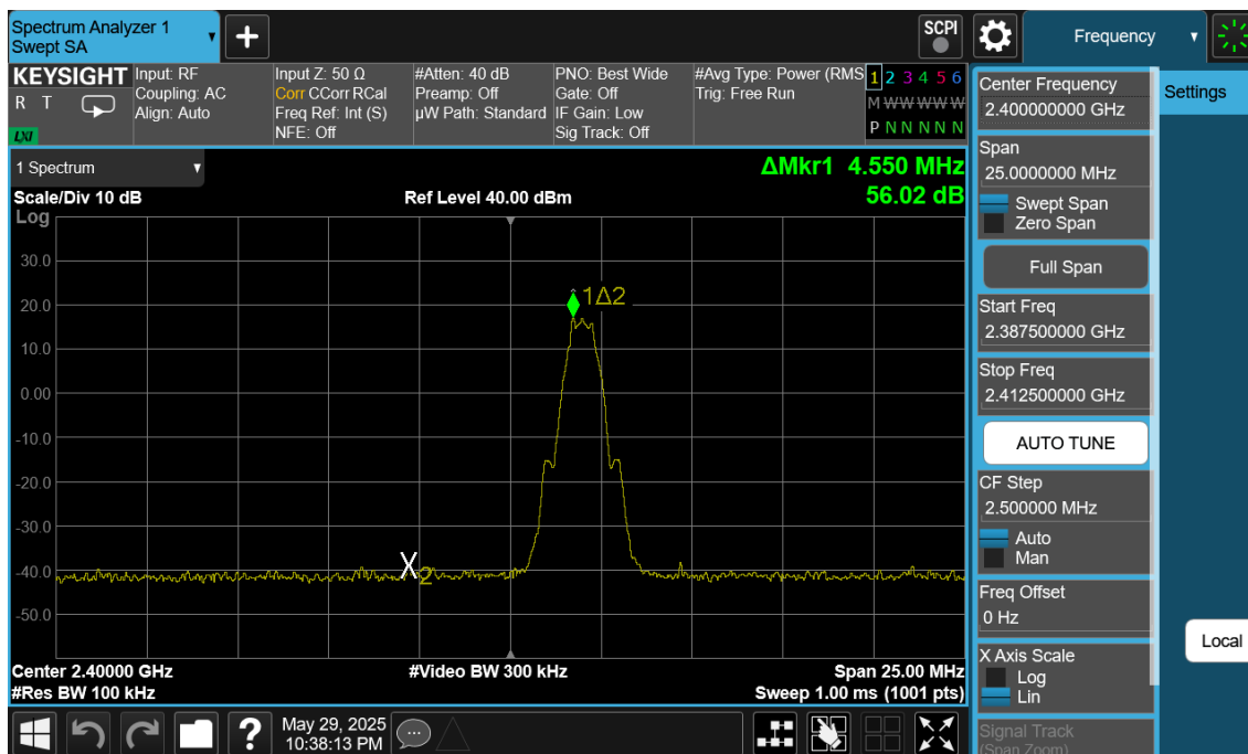
Plot 7-123. Band Edge Plot Antenna 4a (Bluetooth (LE), 500kbps, ePA – Ch.0)
