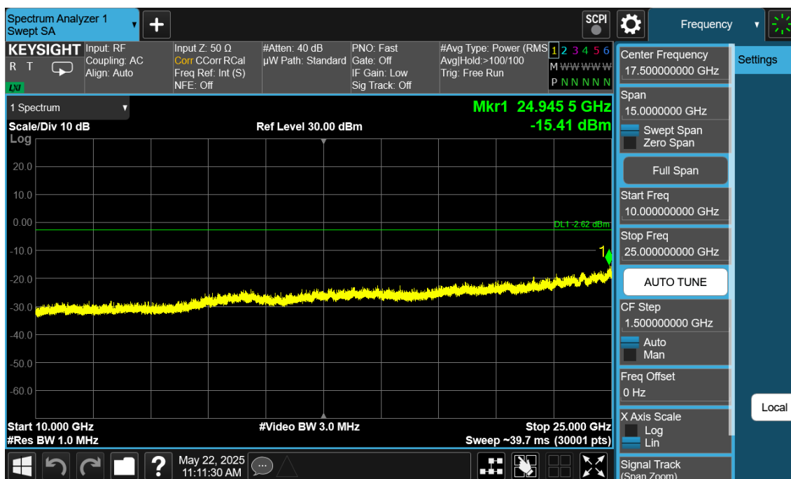
Plot 7-138. Conducted Spurious Plot Antenna 4a (Bluetooth (LE), 1Mbps, ePA – Ch. 0)
