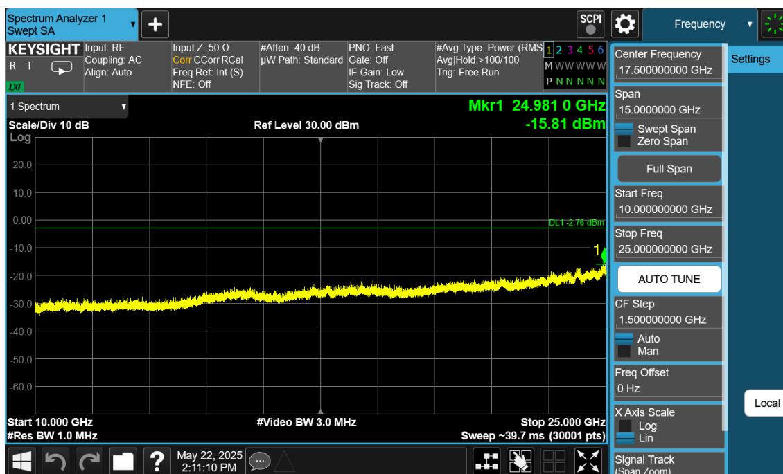
Plot 7-144. Conducted Spurious Plot Antenna 2a (Bluetooth (LE), 2Mbps, ePA – Ch. 1)
