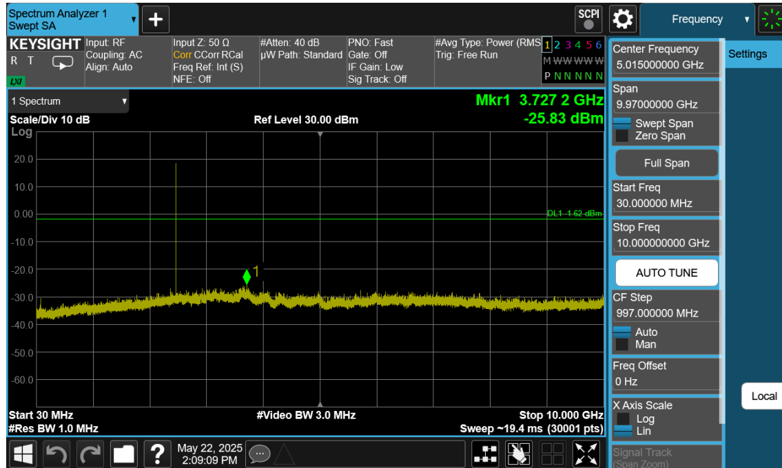
Plot 7-147. Conducted Spurious Plot Antenna 2a (Bluetooth (LE), 1Mbps, ePA – Ch. 39)
