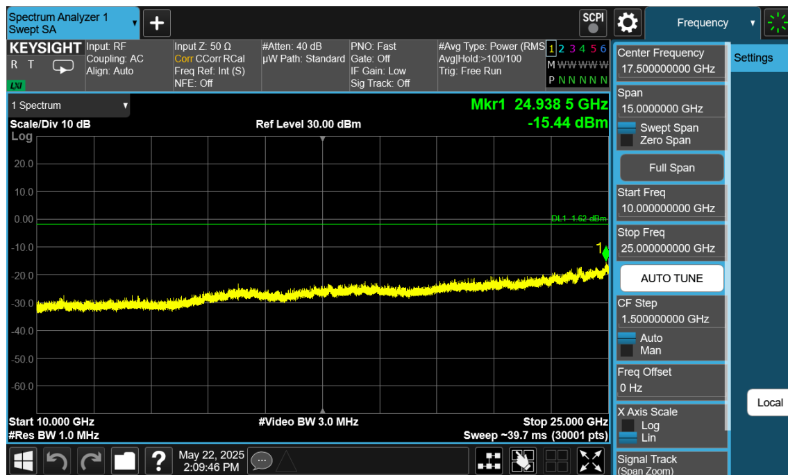
Plot 7-148. Conducted Spurious Plot Antenna 2a (Bluetooth (LE), 1Mbps, ePA – Ch. 39)
