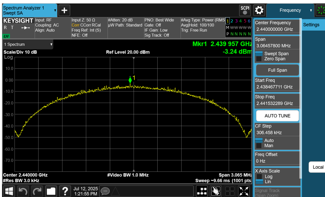
Plot 7-112. Power Spectral Density Plot Antenna 2a (Bluetooth (LE), 2Mbps, ePA – Ch. 19)
