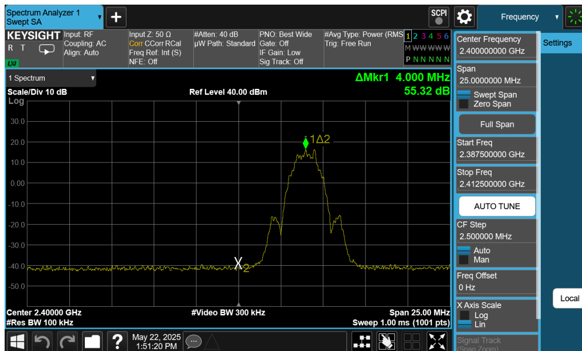
Plot 7-135. Band Edge Plot Antenna 2a (Bluetooth (LE), 2Mbps, ePA – Ch. 1)
