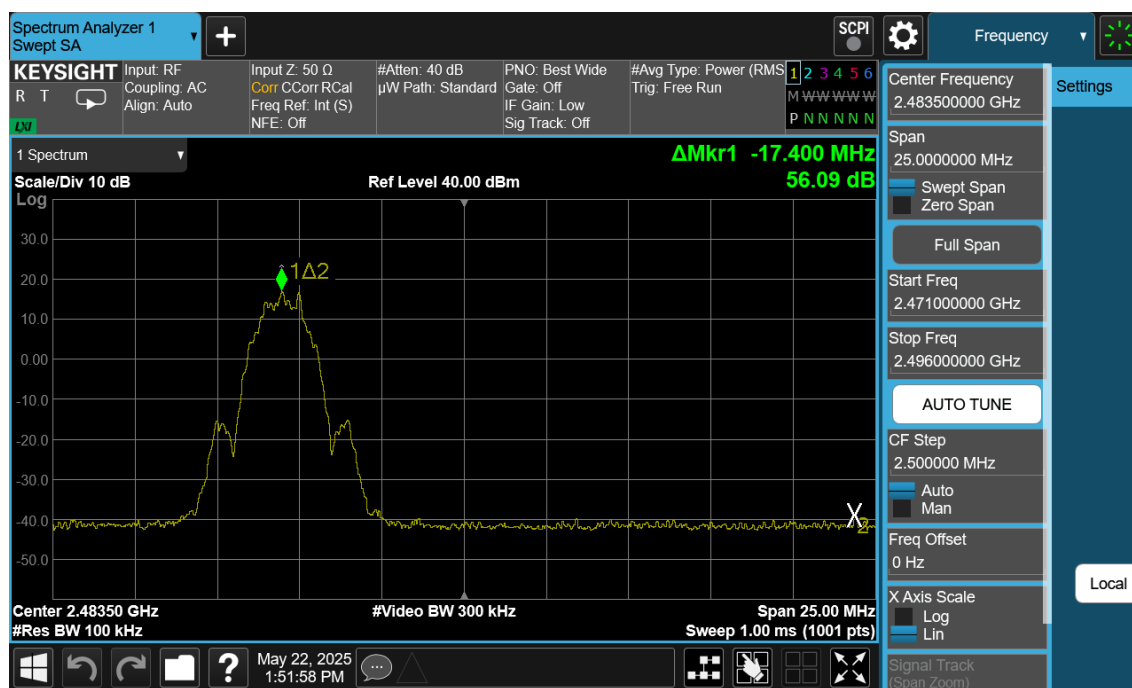
Plot 7-136. Band Edge Plot Antenna 2a (Bluetooth (LE), 2Mbps, ePA – Ch. 38)
