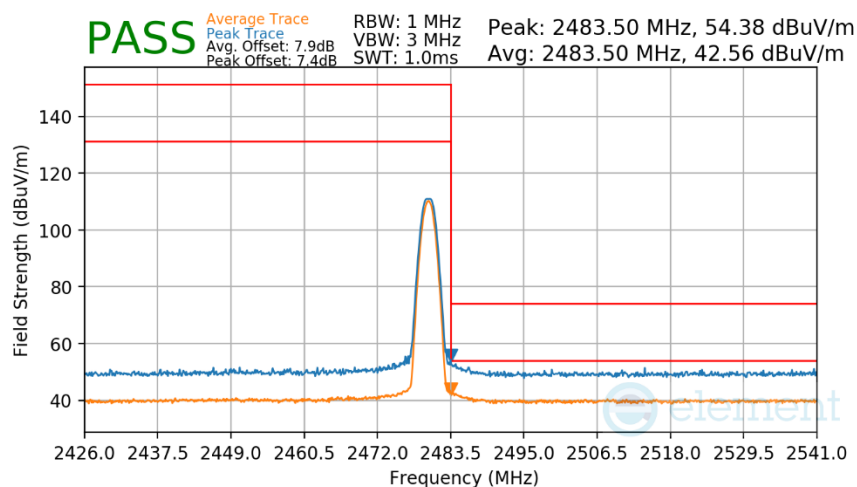
Plot 7-156. Radiated Restricted Upper Band Edge Measurement Antenna 4a (Average & Peak)
