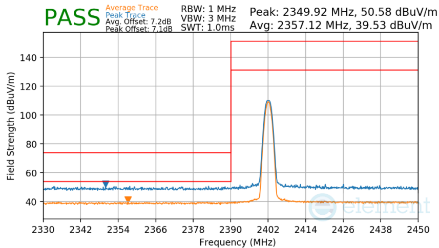
Plot 7-161. Radiated Restricted Lower Band Edge Measurement Antenna 2a (Average & Peak)
