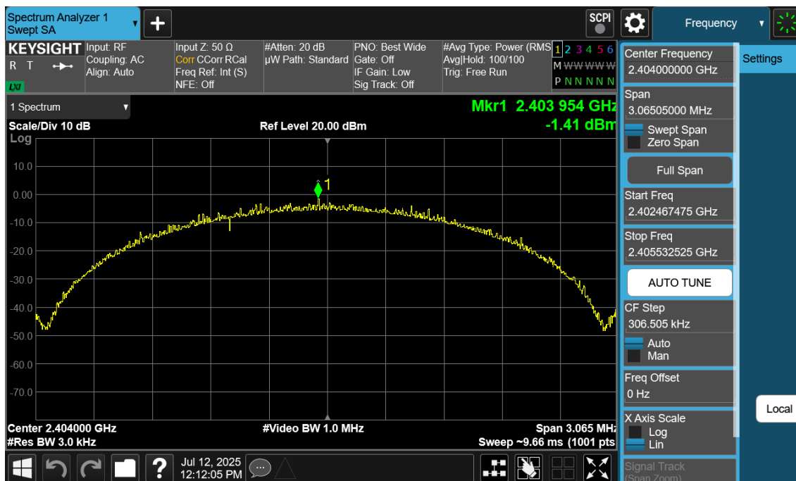
Plot 7-109. Power Spectral Density Plot Antenna 4a (Bluetooth (LE), 2Mbps, ePA – Ch. 1)
