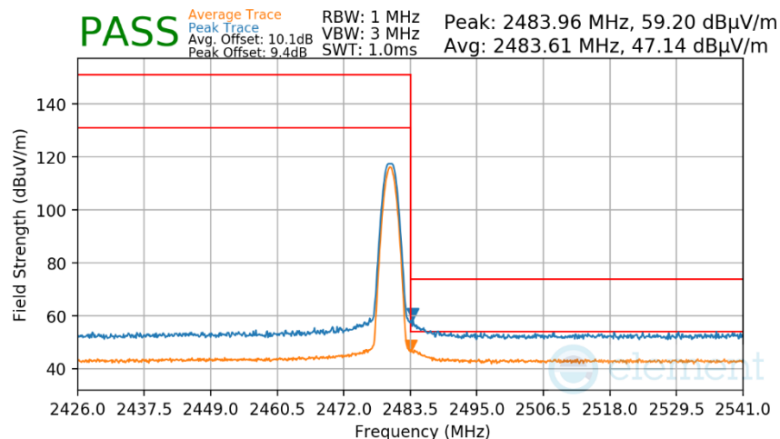
Plot 7-158. Radiated Restricted Upper Band Edge Measurement Antenna 4a (Average & Peak)
