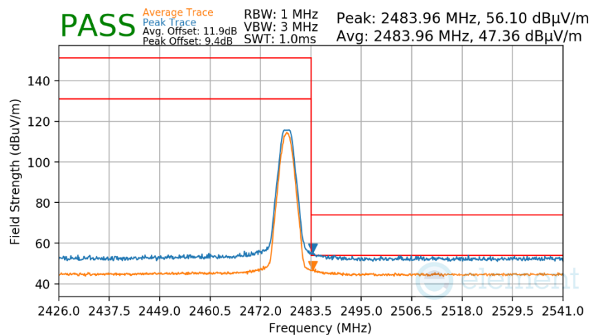
Plot 7-168. Radiated Restricted Upper Band Edge Measurement Antenna 2a (Average & Peak)
