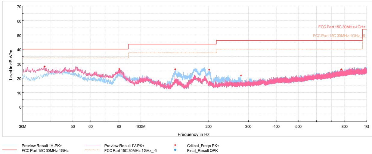
Plot 7-177. Radiated Spurious Emissions Below 1GHz TxBF (1Mbps, ePA – Ch.19, Pol. H & V, with AC/DC Adapter)
