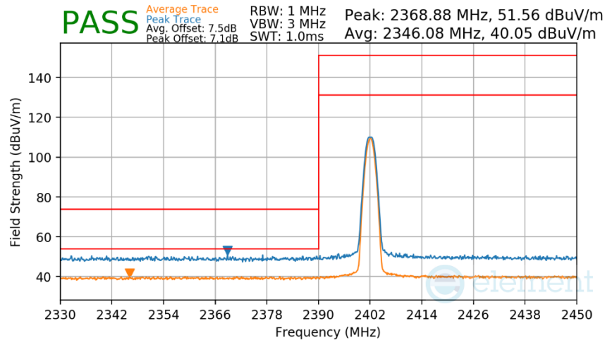
Plot 7-163. Radiated Restricted Lower Band Edge Measurement Antenna 2a (Average & Peak)
