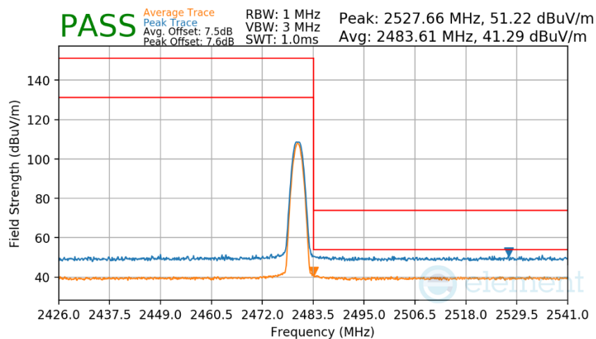
Plot 7-170. Radiated Restricted Upper Band Edge Measurement TxBF (Average & Peak)
