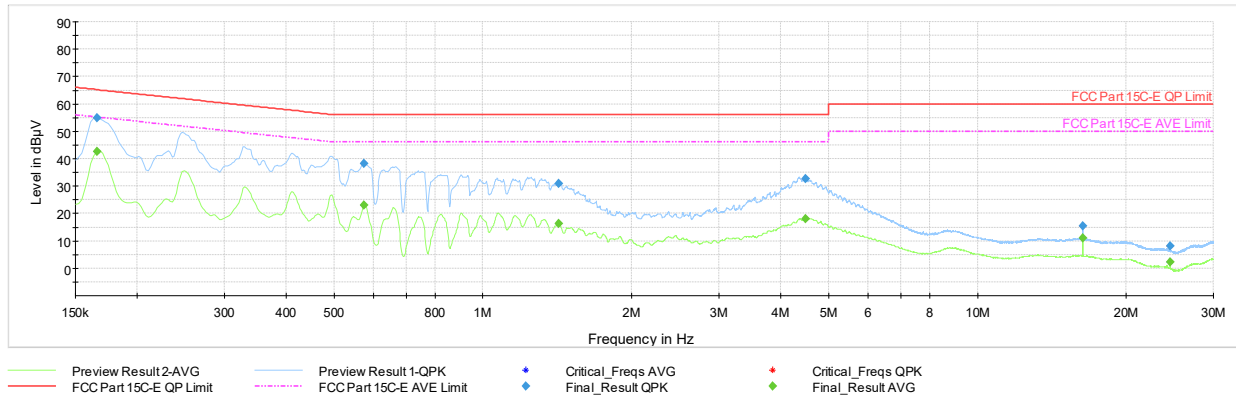
Plot 7-178. AC Line Conducted Plot with Bluetooth LE Tx BF (L1, 1Mbps ePA – Ch.19 with AC/DC Adapter)
