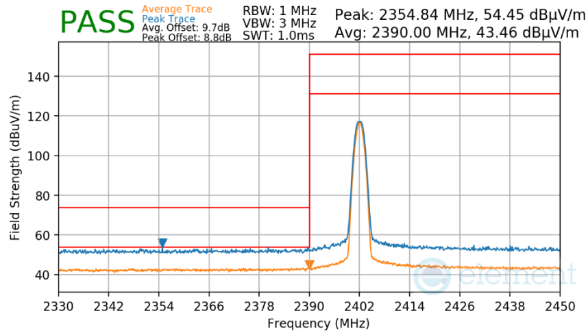
Plot 7-173. Radiated Restricted Lower Band Edge Measurement TxBF (Average & Peak)
