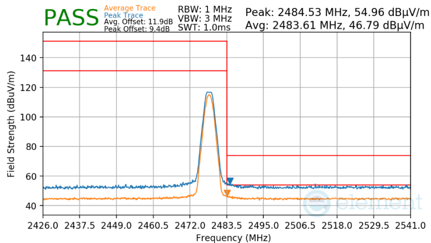
Plot 7-176. Radiated Restricted Upper Band Edge Measurement TxBF (Average & Peak)
