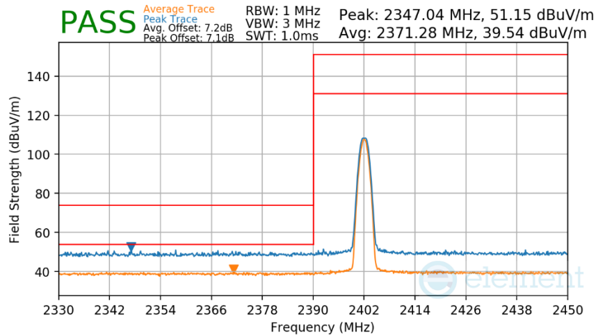
Plot 7-169. Radiated Restricted Lower Band Edge Measurement TxBF (Average & Peak)
