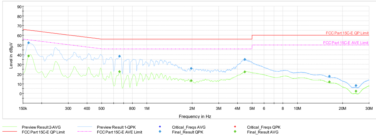
Plot 7-179. AC Line Conducted Plot with Bluetooth LE Tx BF (N, 1Mbps ePA – Ch.19, with AC/DC Adapter)
