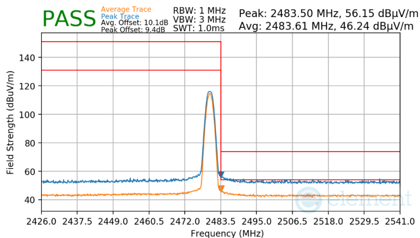
Plot 7-166. Radiated Restricted Upper Band Edge Measurement Antenna 2a (Average & Peak)
