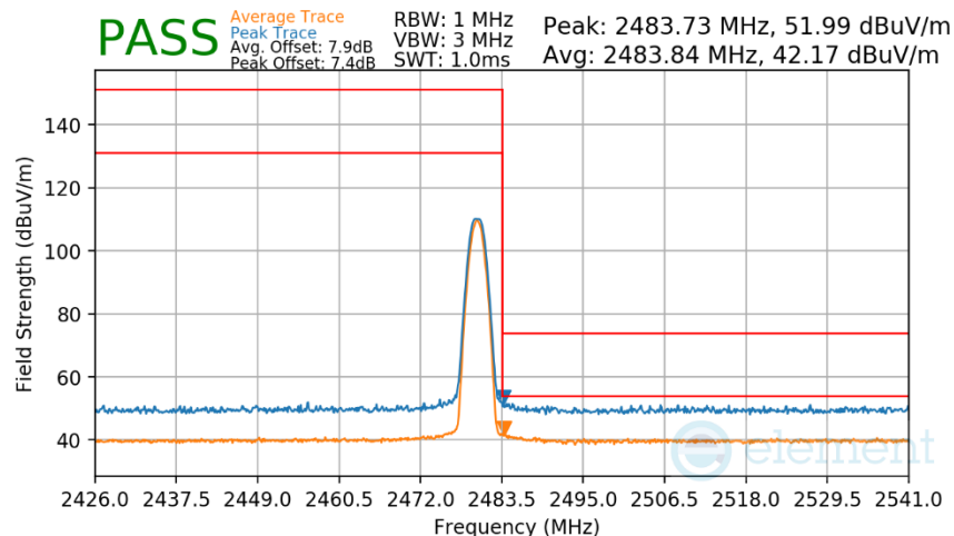
Plot 7-164. Radiated Restricted Upper Band Edge Measurement Antenna 2a (Average & Peak)
