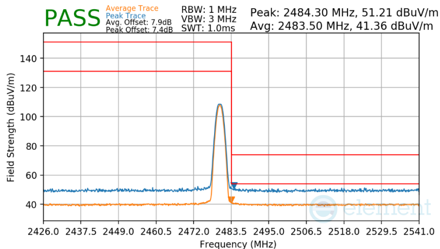
Plot 7-172. Radiated Restricted Upper Band Edge Measurement TxBF (Average & Peak)
