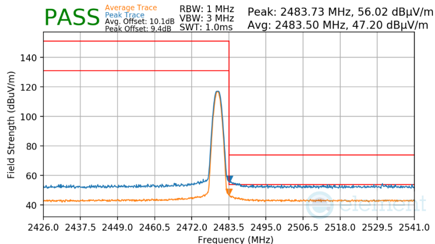
Plot 7-174. Radiated Restricted Upper Band Edge Measurement TxBF (Average & Peak)
