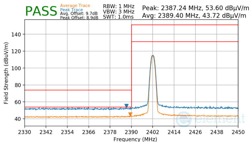
Plot 7-165. Radiated Restricted Lower Band Edge Measurement Antenna 2a (Average & Peak)
