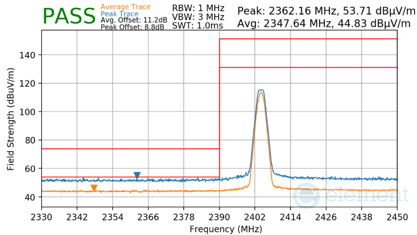
Plot 7-167. Radiated Restricted Lower Band Edge Measurement Antenna 2a (Average & Peak)
