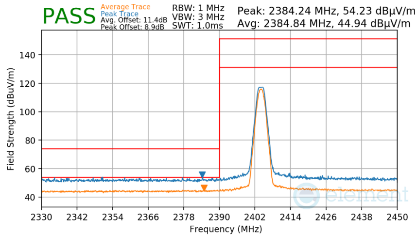
Plot 7-175. Radiated Restricted Lower Band Edge Measurement TxBF (Average & Peak)
