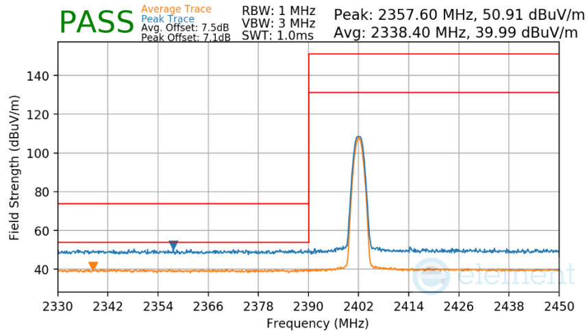
Plot 7-171. Radiated Restricted Lower Band Edge Measurement TxBF (Average & Peak)
