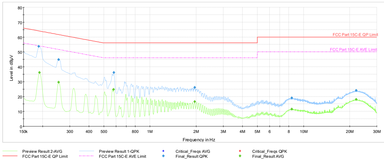
Plot 7-80. AC Line-Conducted Test Plot TxBF (N, GFSK ePA – Ch.39, with AC/DC Adapter)
