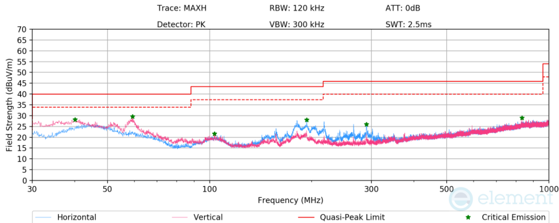
Plot 7-78. Radiated Spurious Emissions Simultaneous Transmission Below 1GHz (with AC/DC Adapter)
