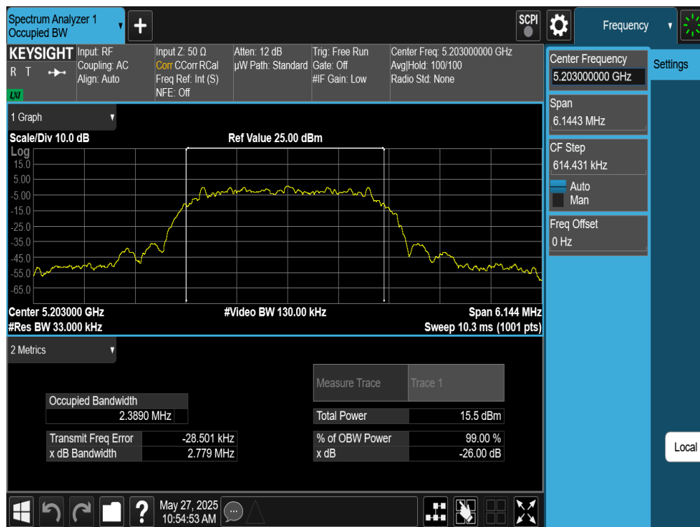
Plot 7-39. 26dB BW & 99% OBW Antenna 2a (NB UNII HDT6, ePA– 5203MHz)
