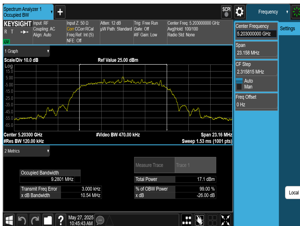
Plot 7-36. 26dB BW & 99% OBW Antenna 2a (NB UNII HDRPL32, ePA- 5203MHz)
