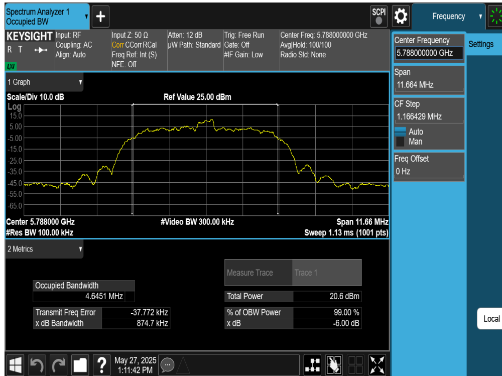
Plot 7-44. 6dB BW & 99% OBW Antenna WF5B (NB UNII HDR8, ePA – 5788MHz)
