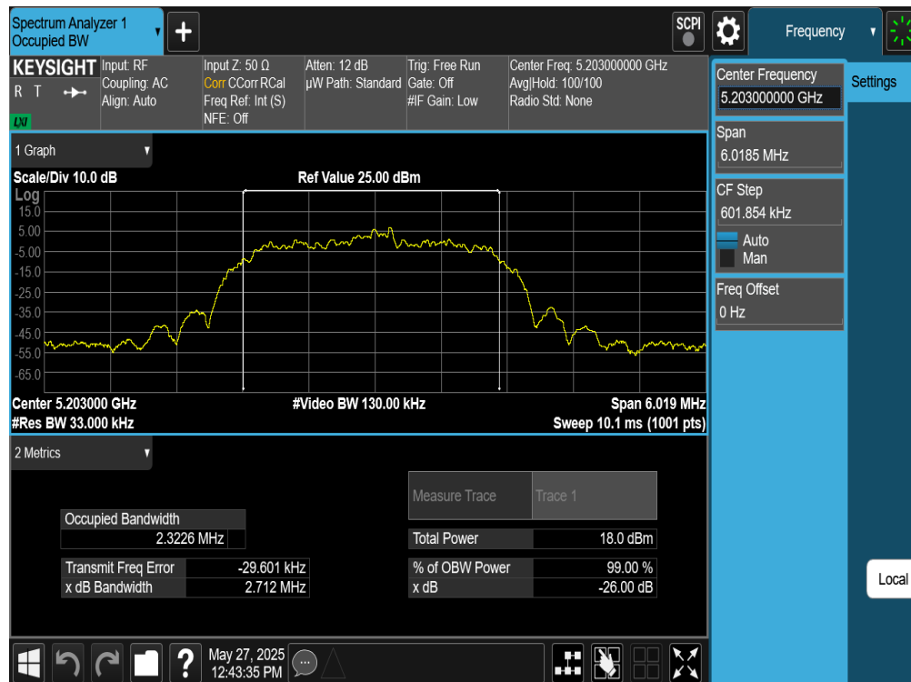
Plot 7-4. 26dB BW & 99% OBW Antenna WF5B (NB UNII HDR4, ePA- 5203MHz)
