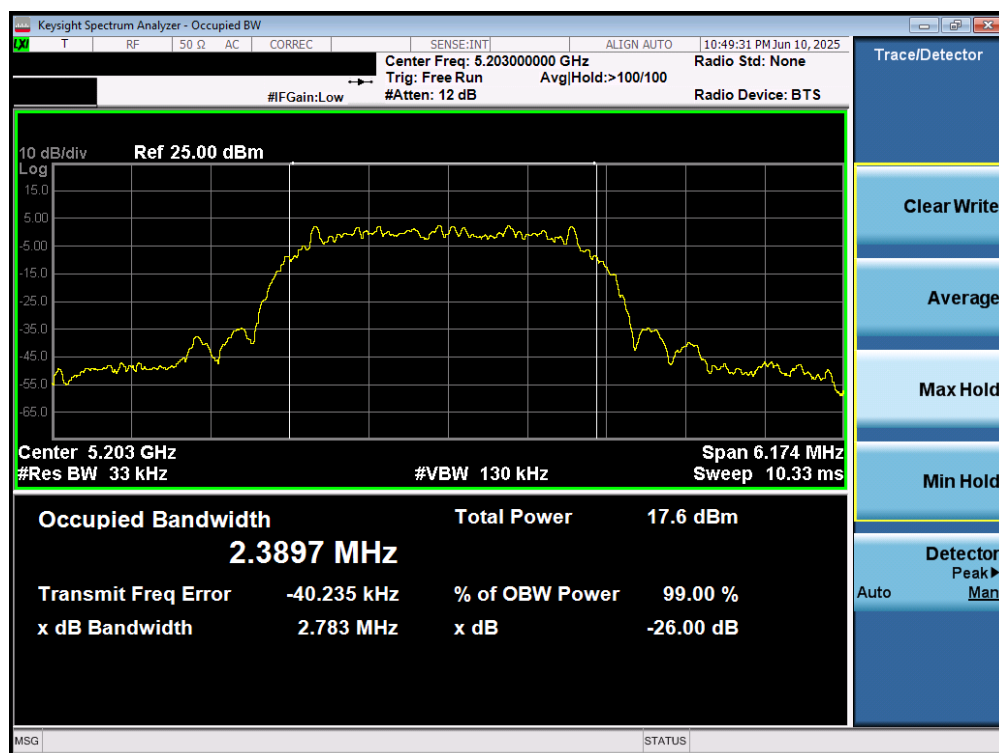
Plot 7-26. 26dB BW & 99% OBW Antenna 4a (NB UNII HDT6, ePA- 5203MHz)
