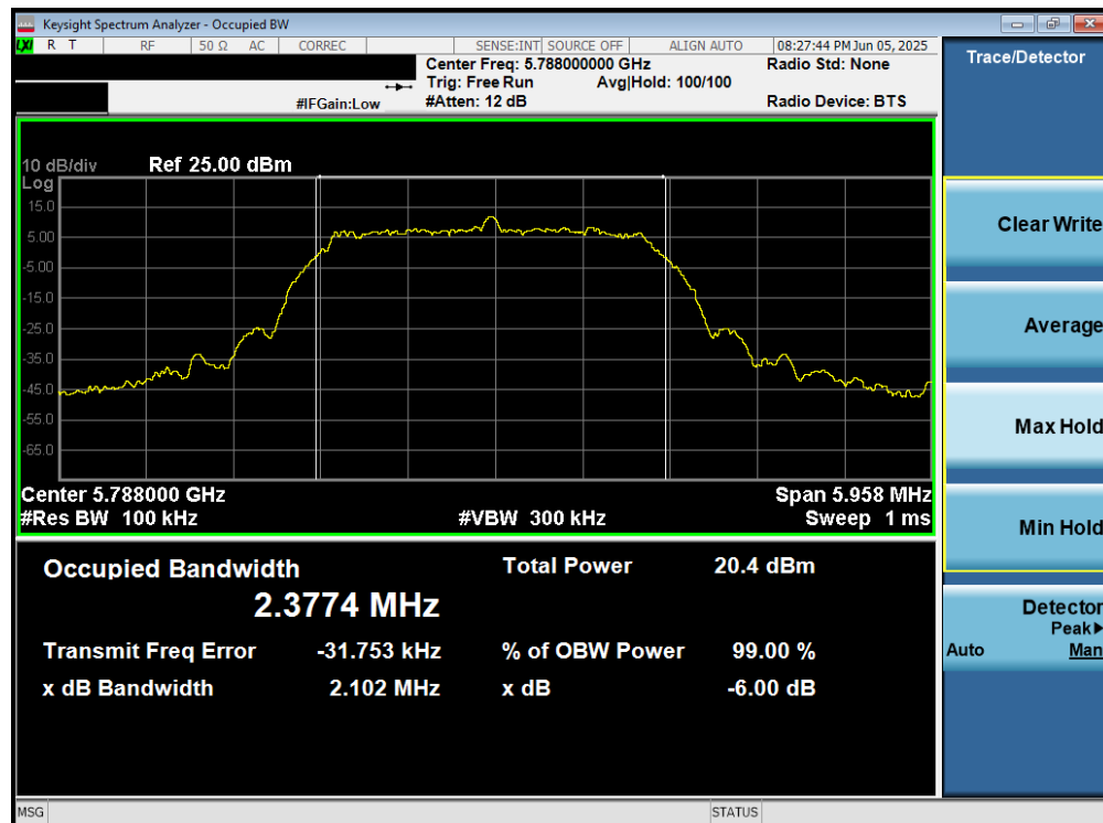
Plot 7-45. 6dB BW & 99% OBW Antenna WF5B (NB UNII HDRPS2, ePA – 5788MHz)
