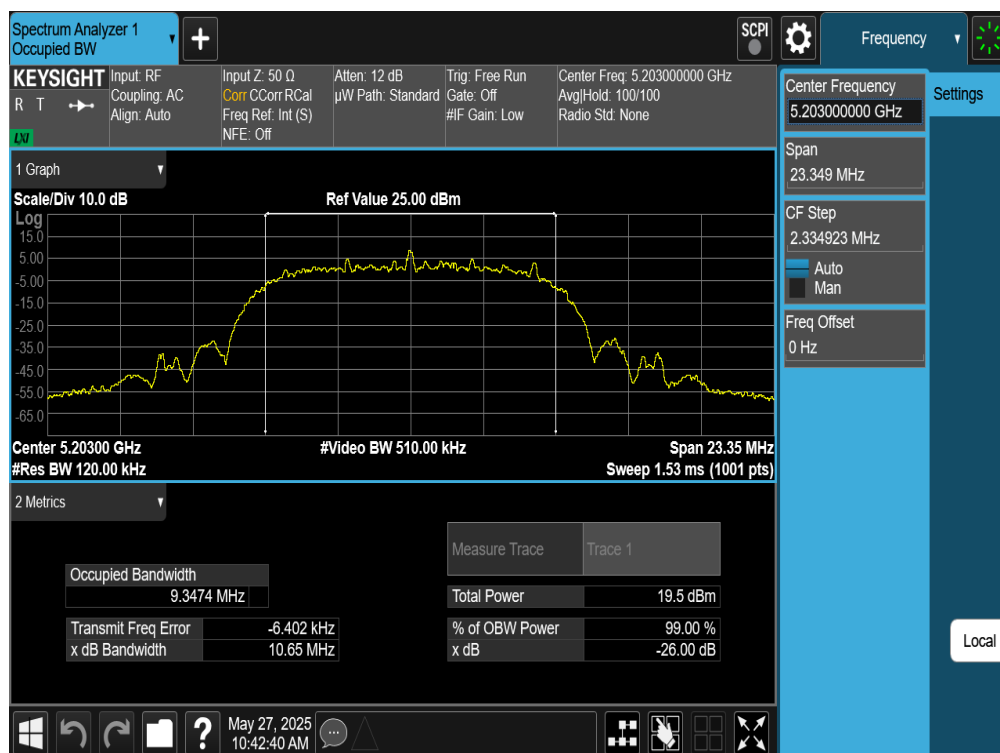
Plot 7-35. 26dB BW & 99% OBW Antenna 2a (NB UNII HDRPL12, ePA- 5203MHz)
