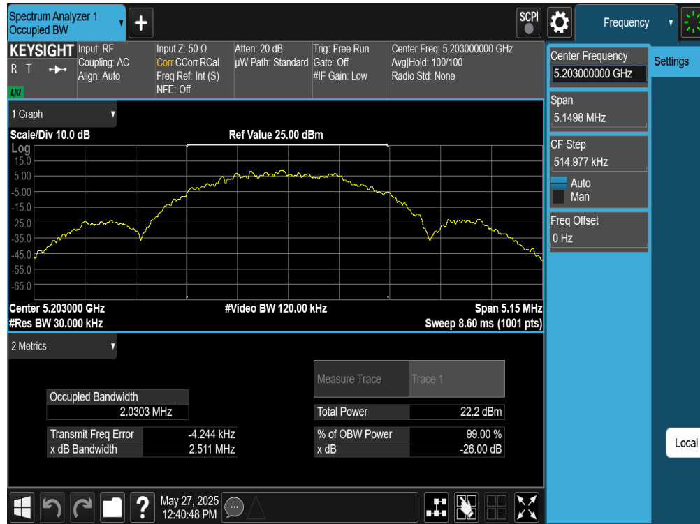
Plot 7-3. 26dB BW & 99% OBW Antenna WF5B (NB UNII LE2M, ePA- 5203MHz)
