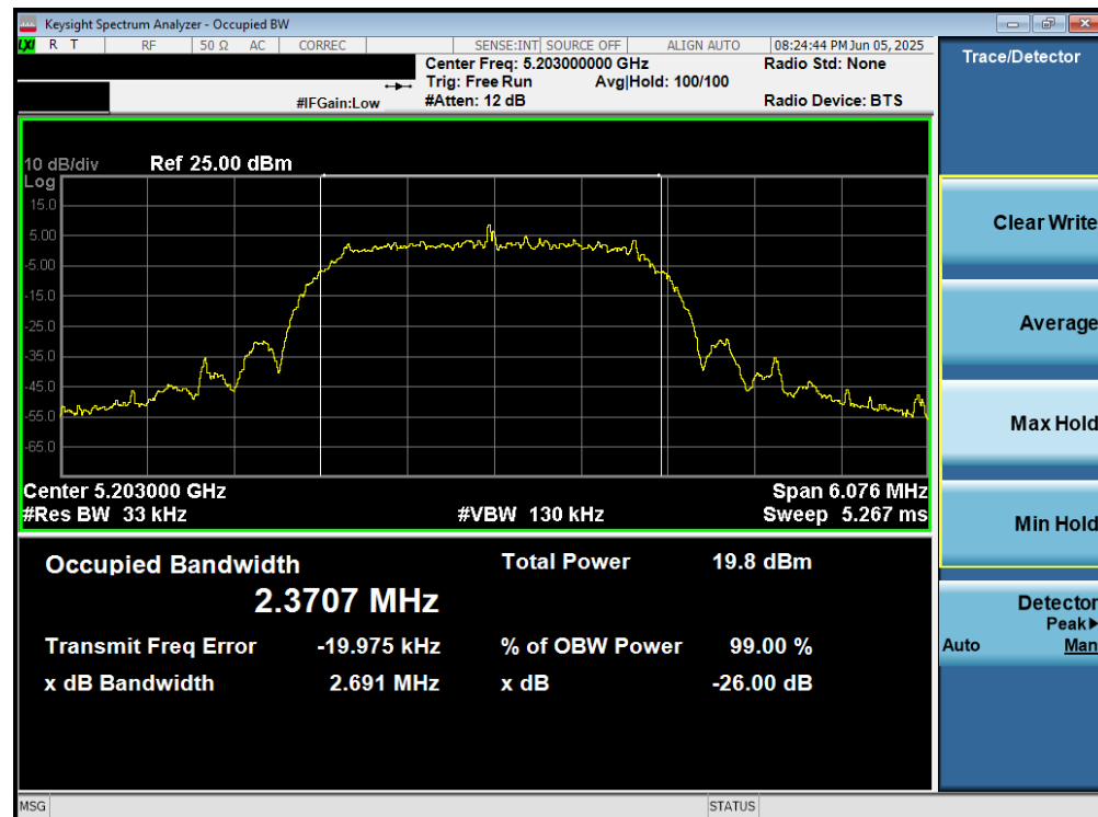
Plot 7-6. 26dB BW & 99% OBW Antenna WF5B (NB UNII HDRPS2, ePA- 5203MHz)
