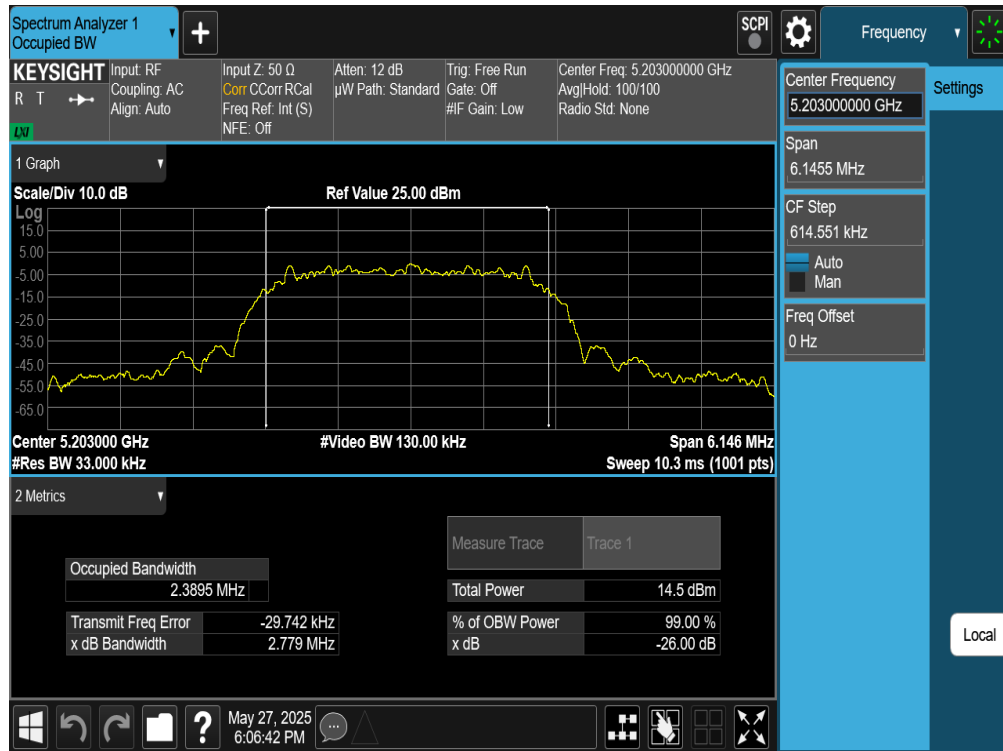
Plot 7-13. 26dB BW & 99% OBW Antenna WF5B (NB UNII HDT6, ePA– 5203MHz)
