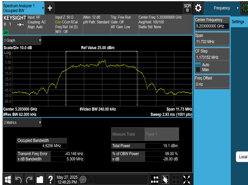
Plot 7-5. 26dB BW & 99% OBW Antenna WF5B (NB UNII HDR8, ePA- 5203MHz)
