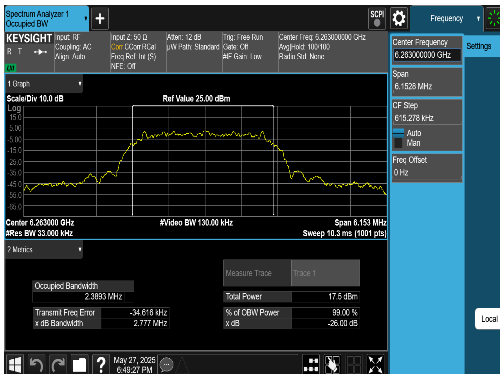
Plot 7-13. 26dB BW & 99% OBW Antenna WF5B (NB UNII HDT6, ePA– 6263MHz)
