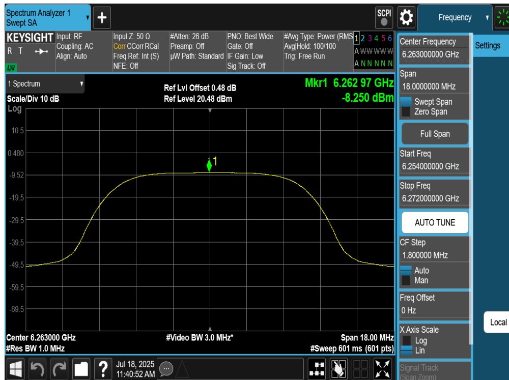
Plot 7-56. PSD Antenna WF5B (NB UNII HDRPL12, ePA – 6263MHz)
