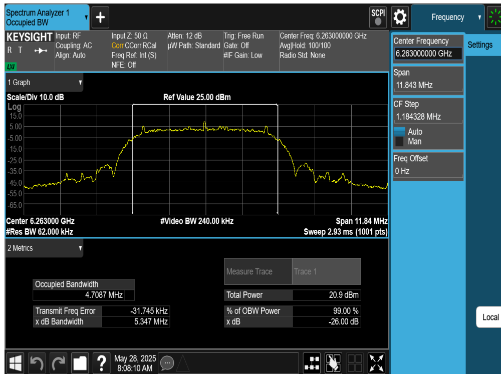
Plot 7-20. 26dB BW & 99% OBW Antenna 4a (NB UNII XHDRPM6, ePA- 6263MHz)
