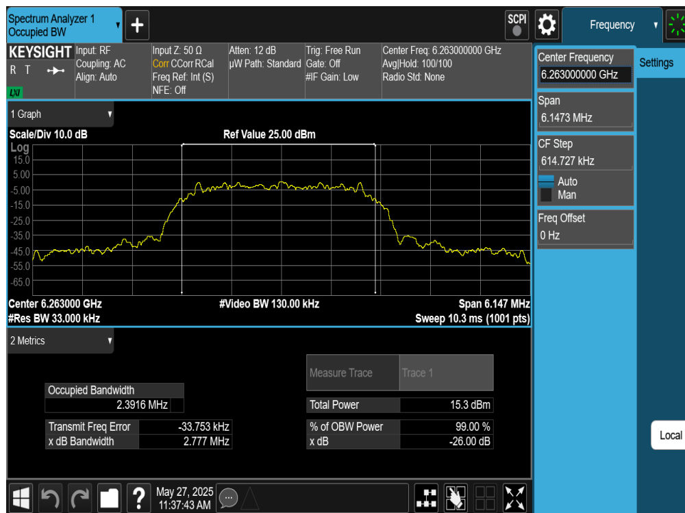
Plot 7-39. 26dB BW & 99% OBW Antenna 2a (NB UNII HDT6, ePA– 6263MHz)
