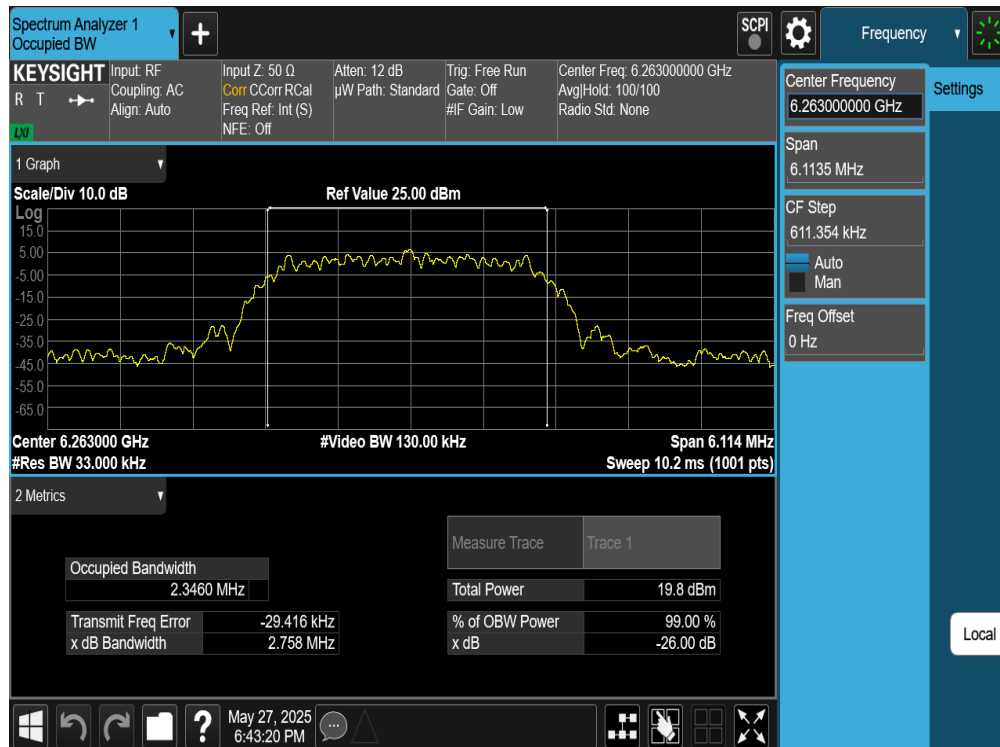
Plot 7-11. 26dB BW & 99% OBW Antenna WF5B (NB UNII HDT2, ePA- 6263MHz)
