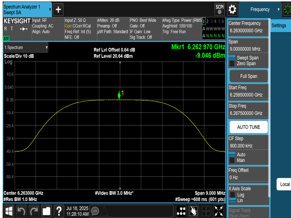
Plot 7-52. PSD Antenna WF5B (NB UNII XHDRPM6, ePA – 6263MHz)
