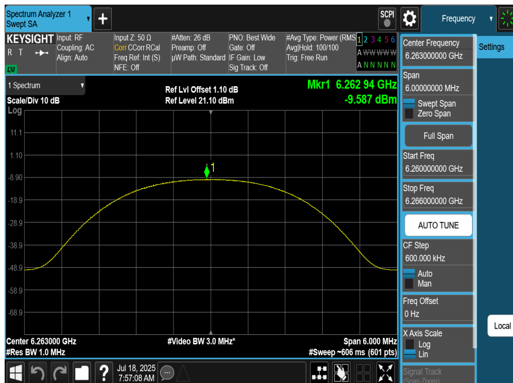
Plot 7-46. PSD Antenna WF5B (NB UNII HDR4, ePA – 6263MHz)
