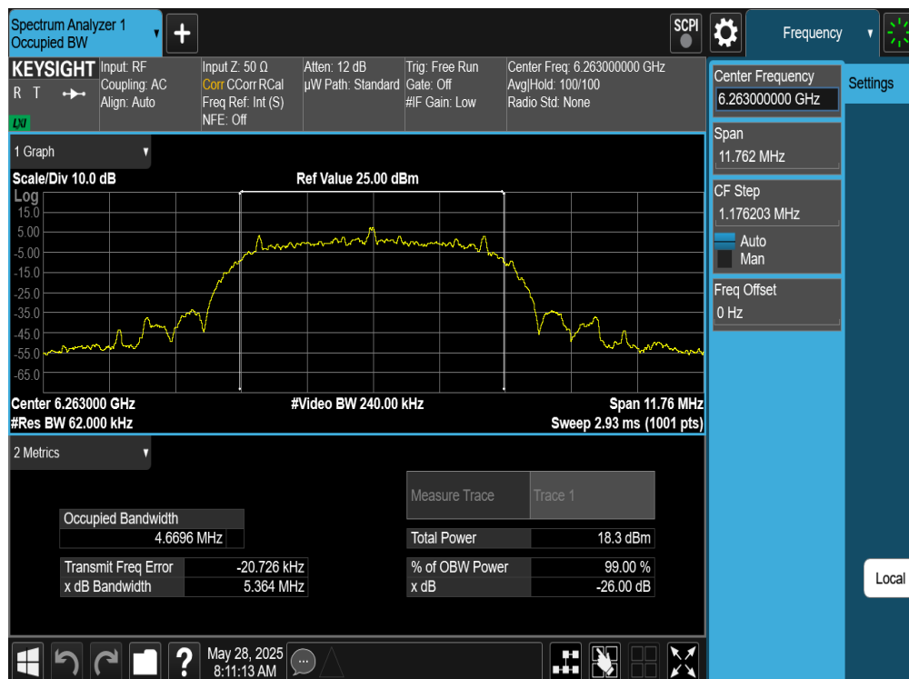
Plot 7-21. 26dB BW & 99% OBW Antenna 4a (NB UNII HDRPM16, ePA- 6263MHz)
