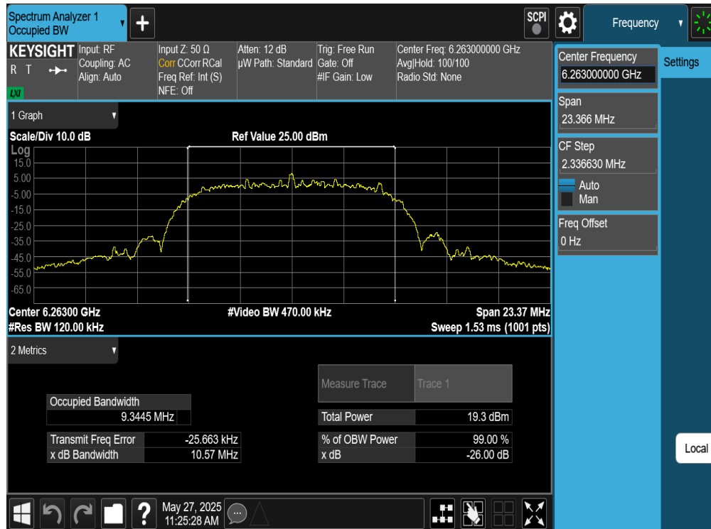
Plot 7-35. 26dB BW & 99% OBW Antenna 2a (NB UNII HDRPL12, ePA- 6263MHz)
