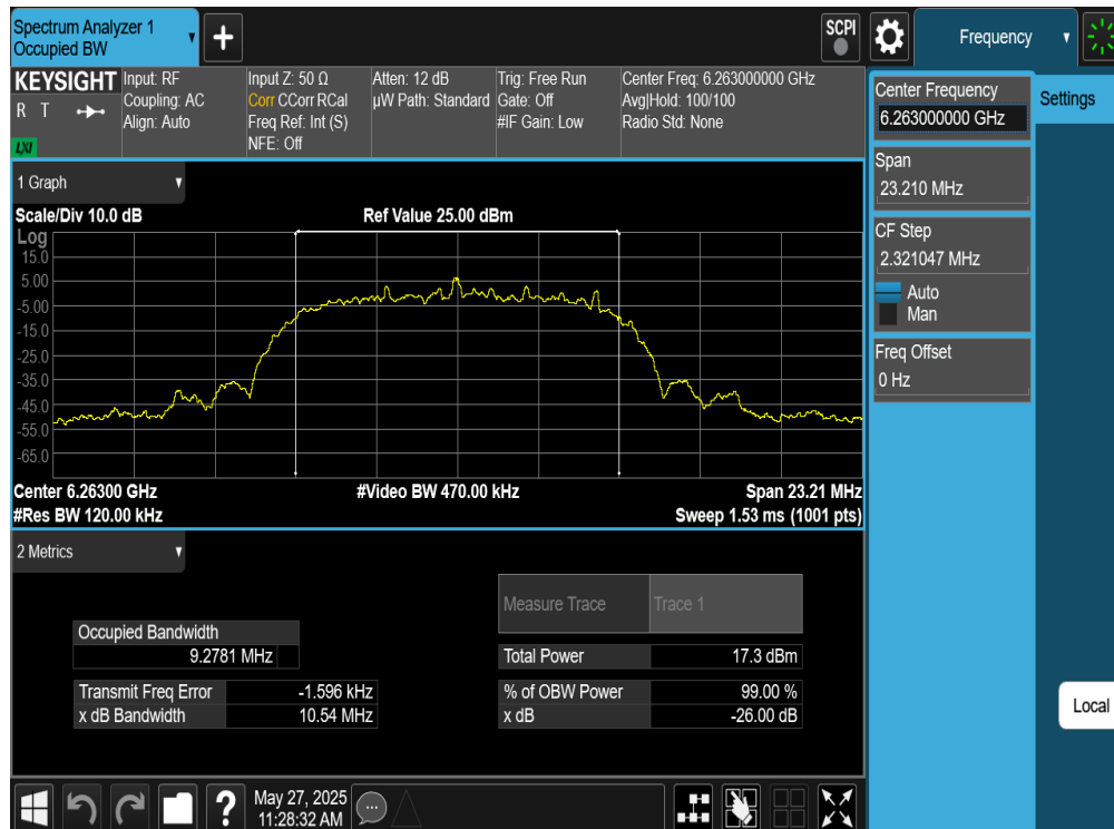
Plot 7-36. 26dB BW & 99% OBW Antenna 2a (NB UNII HDRPL32, ePA- 6263MHz)
