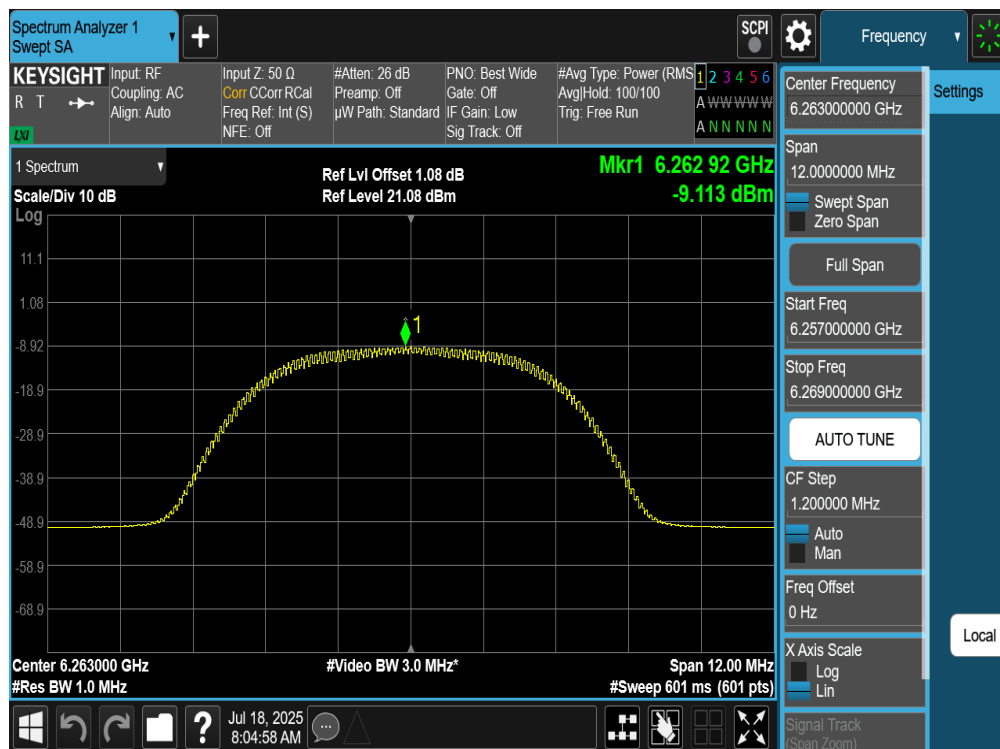
Plot 7-48. PSD Antenna WF5B (NB UNII HDR8, ePA – 6263MHz)
