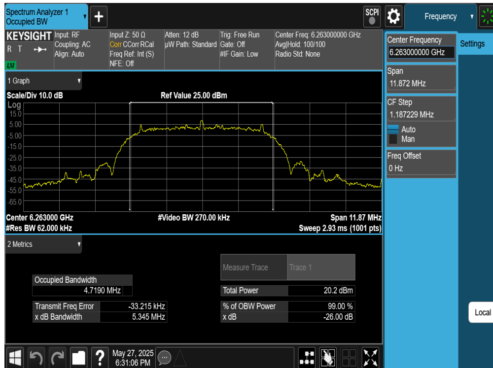
Plot 7-7. 26dB BW & 99% OBW Antenna WF5B (NB UNII XHDRPM6, ePA– 6263MHz)
