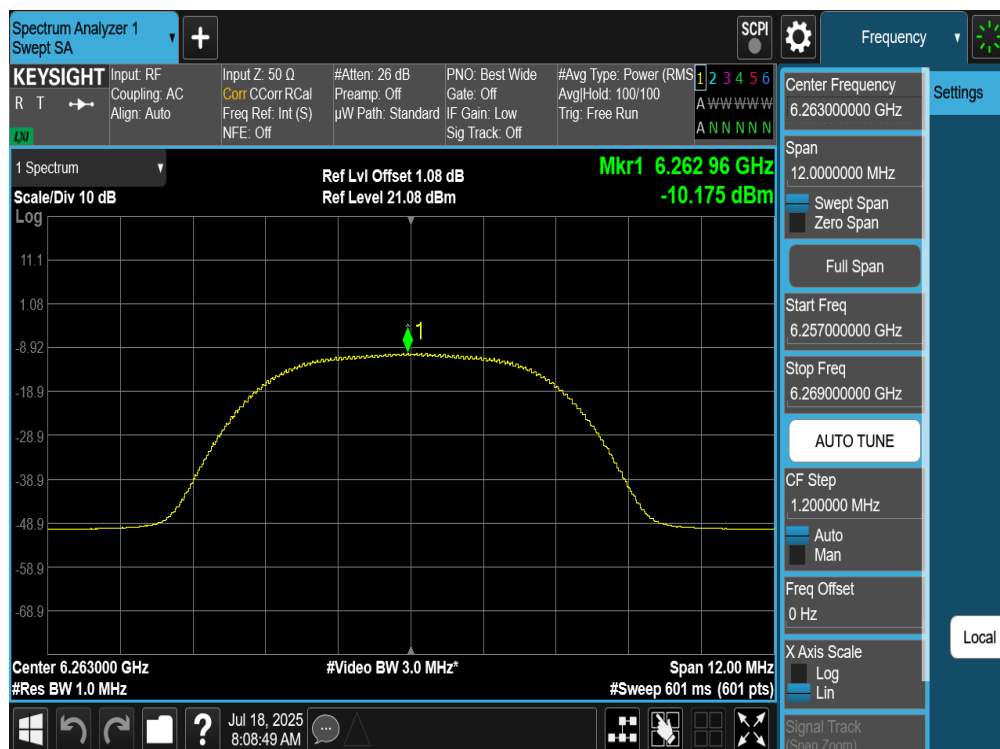
Plot 7-49. PSD Antenna WF5B (NB UNII HDR8, iPA – 6263MHz)
