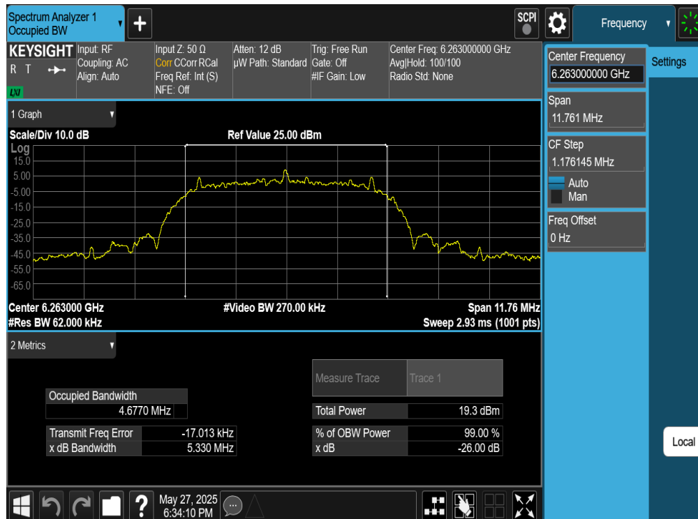
Plot 7-8. 26dB BW & 99% OBW Antenna WF5B (NB UNII HDRPM16, ePA– 6263MHz)
