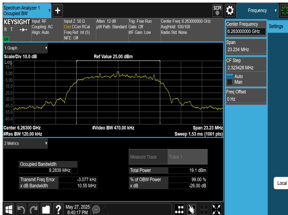
Plot 7-10. 26dB BW & 99% OBW Antenna WF5B (NB UNII HDRPL32, ePA- 6263MHz)
