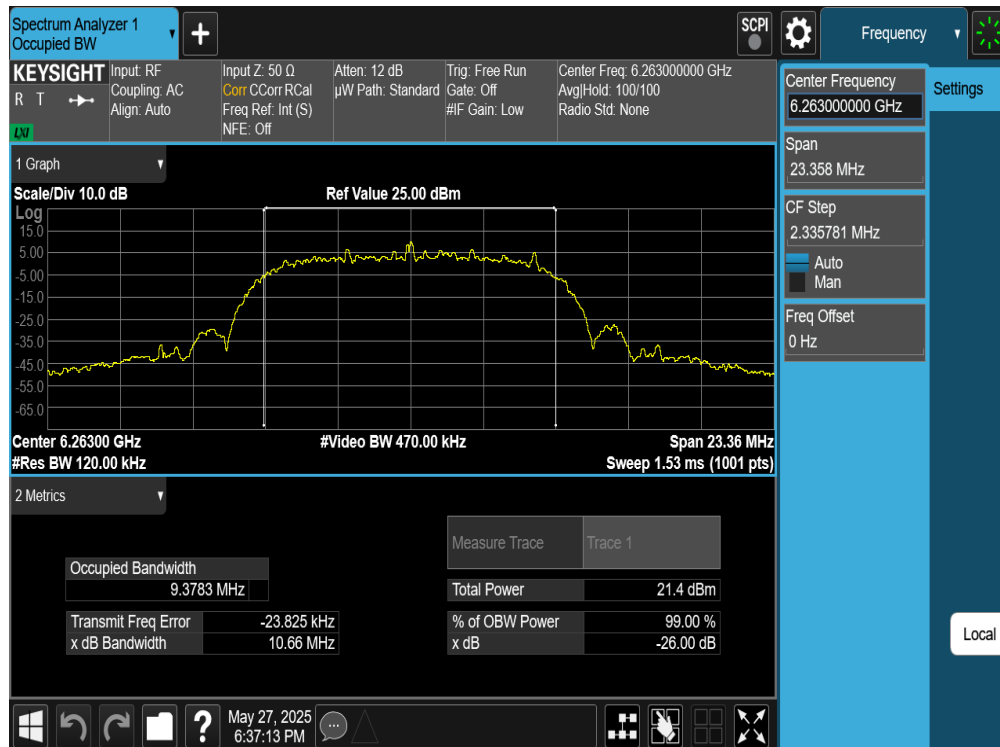
Plot 7-9. 26dB BW & 99% OBW Antenna WF5B (NB UNII HDRPL12, ePA- 6263MHz)
