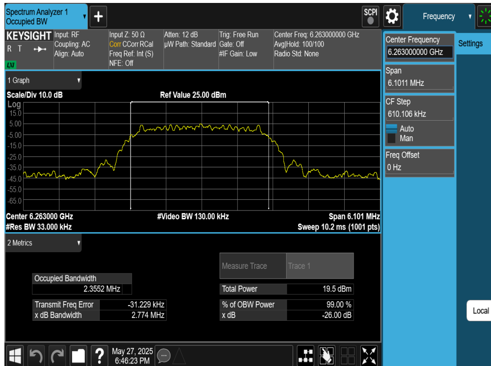
Plot 7-12. 26dB BW & 99% OBW Antenna WF5B (NB UNII HDT4, ePA- 6263MHz)
