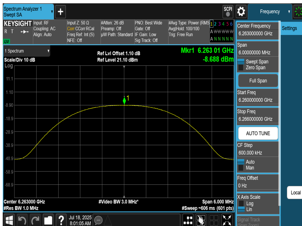
Plot 7-47. PSD Antenna WF5B (NB UNII HDR4, iPA – 6263MHz)
