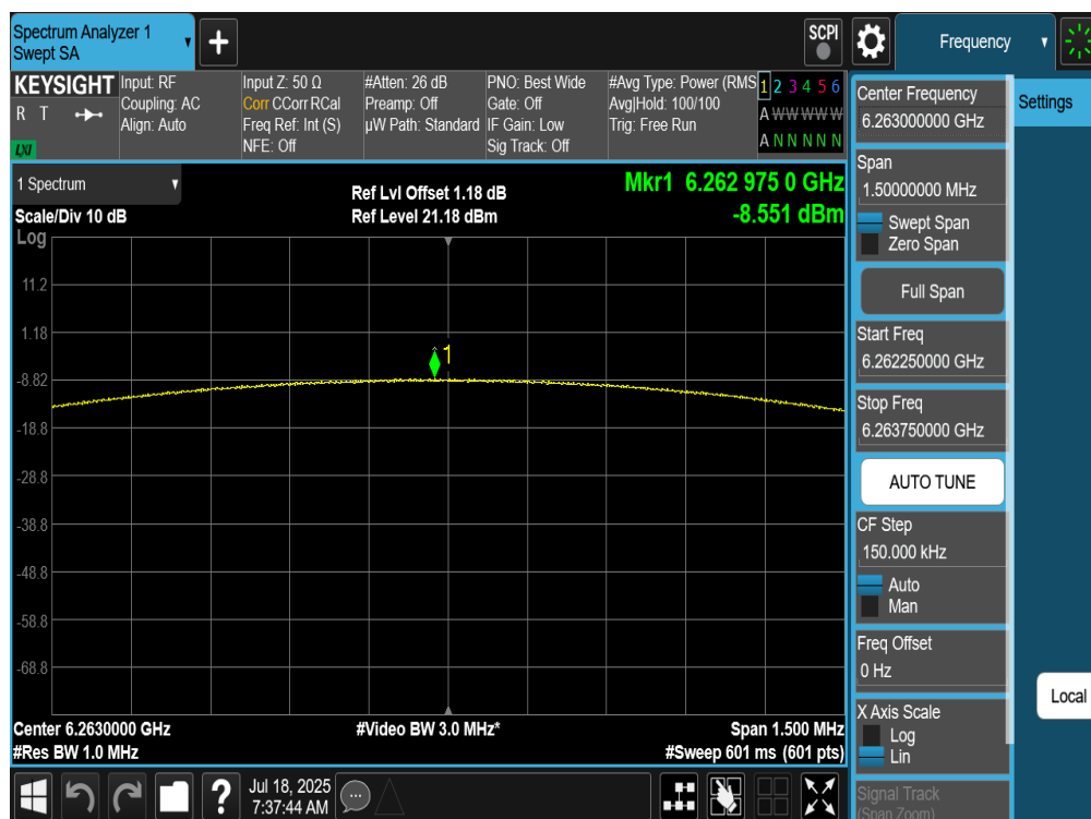
Plot 7-41. PSD Antenna WF5B (NB UNII BDR, iPA – 6263MHz)
