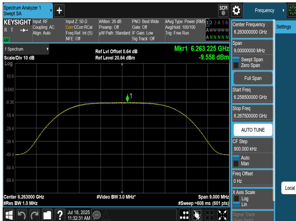
Plot 7-53. PSD Antenna WF5B (NB UNII XHDRPM6, iPA – 6263MHz)
