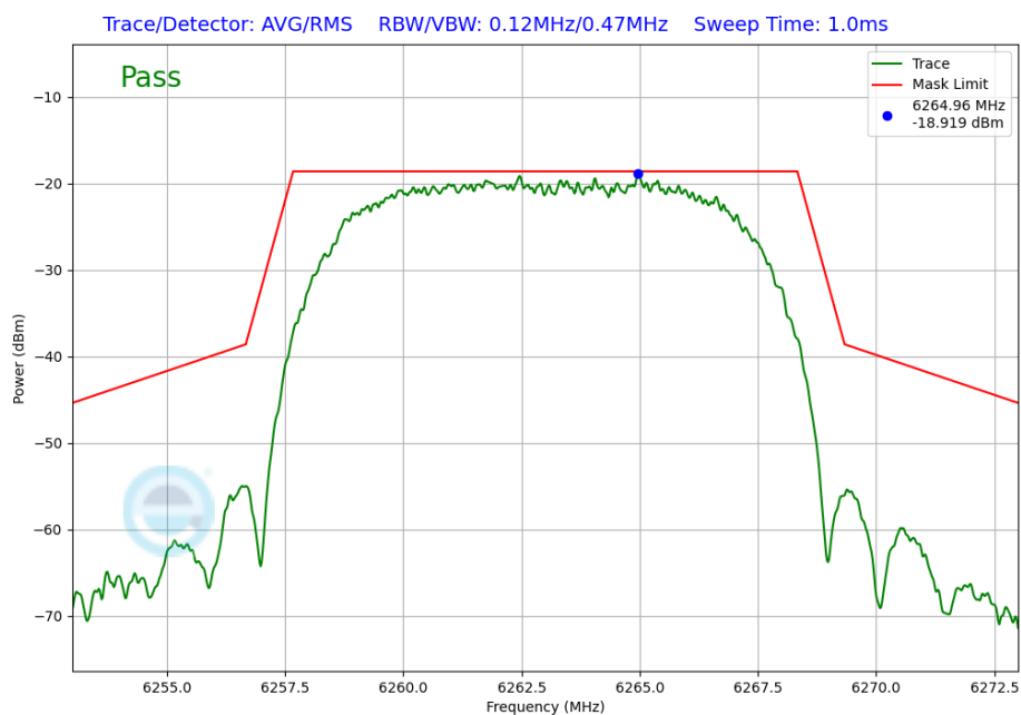
Plot 7-239. In-Band Emission Plot Antenna WF5B (NB UNII HDRPL12, iPA – 6263MHz)
