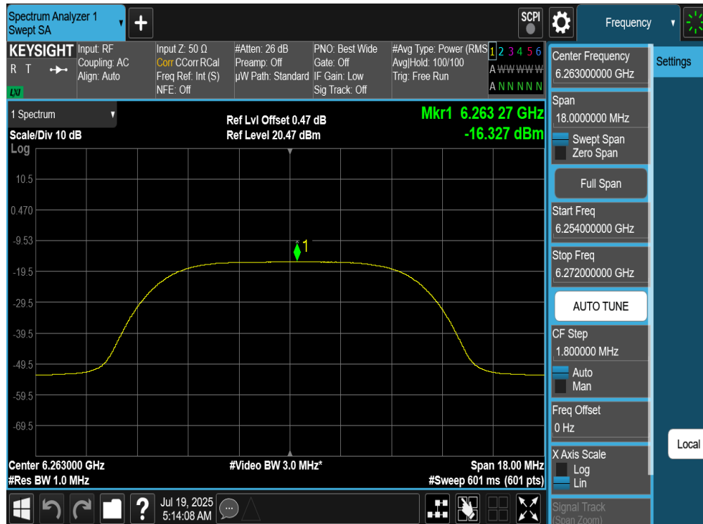
Plot 7-202. PSD TxBF Diversity Antenna 4a (NB UNII HDRPL12, ePA – 6263MHz)
