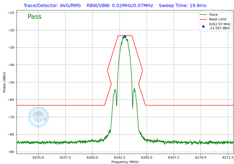
Plot 7-225. In-Band Emission Plot Antenna WF5B (NB UNII LE1M, iPA – 6263MHz)
