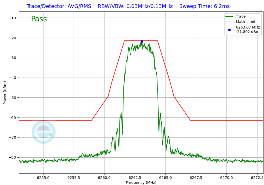
Plot 7-229. In-Band Emission Plot Antenna WF5B (NB UNII HDR4, iPA – 6263MHz)
