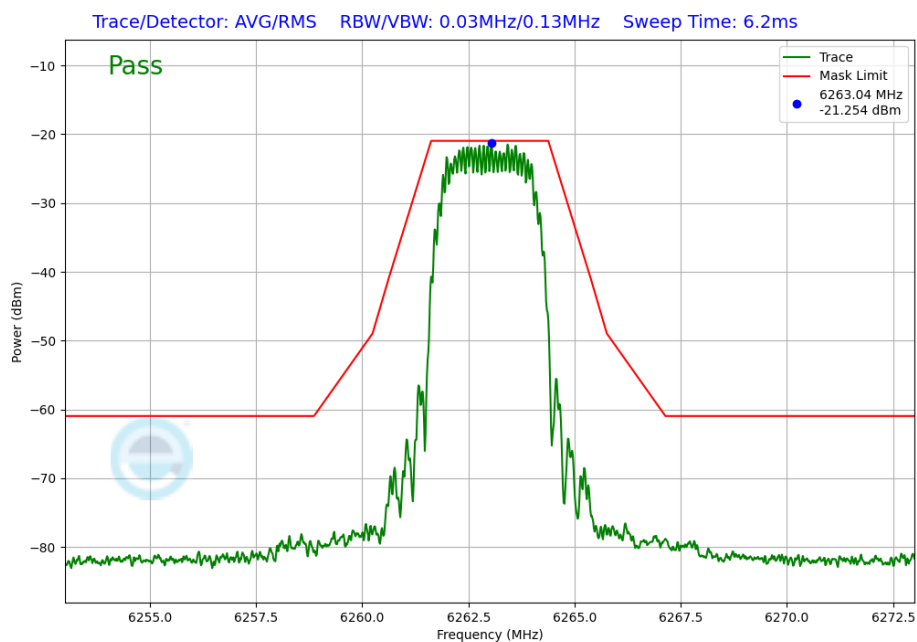
Plot 7-243. In-Band Emission Plot Antenna WF5B (NB UNII HDT2, iPA – 6263MHz)
