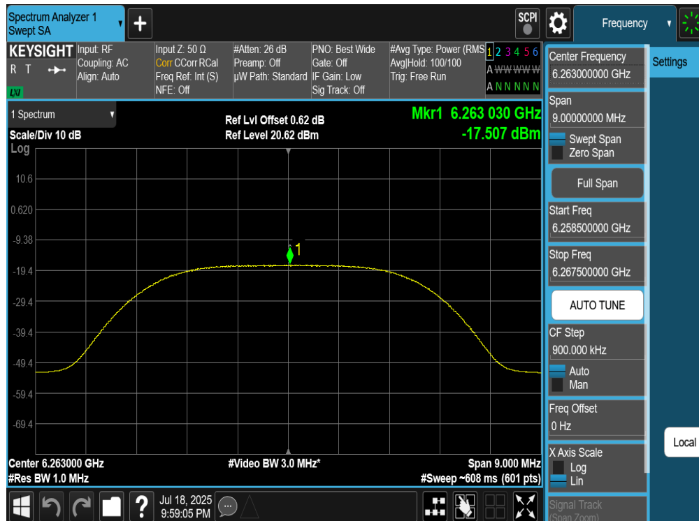
Plot 7-197. PSD TxBF Diversity Antenna 2a (NB UNII XHDRPM6, iPA – 6263MHz)
