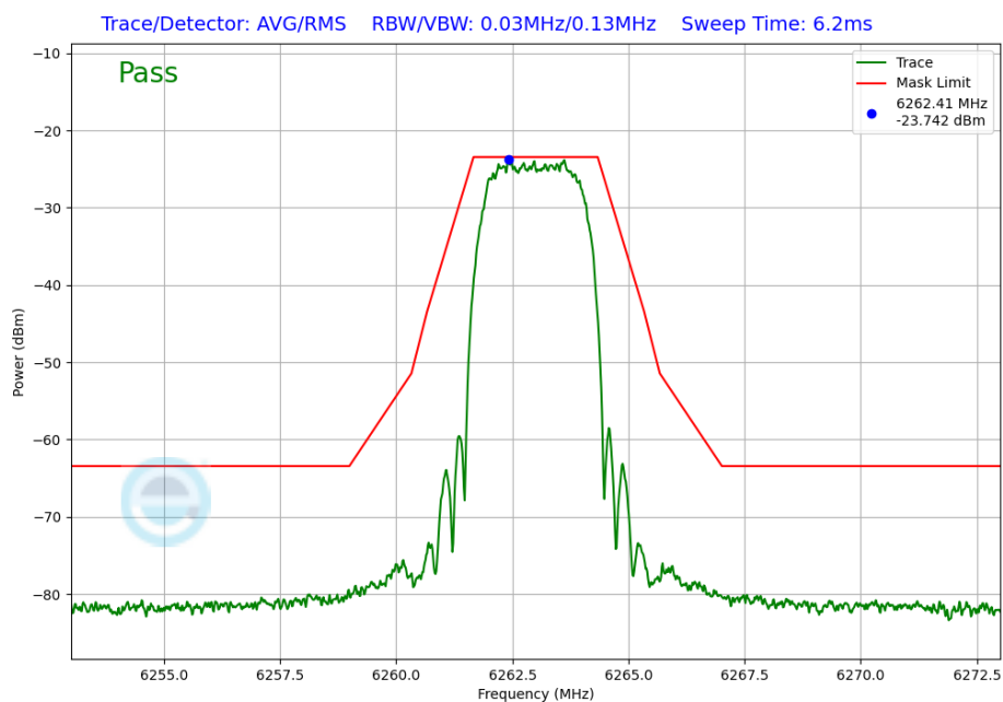
Plot 7-233. In-Band Emission Plot Antenna WF5B (NB UNII HDRPS2, iPA – 6263MHz)
