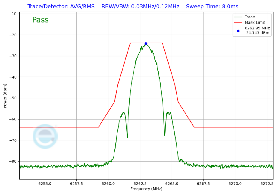
Plot 7-227. In-Band Emission Plot Antenna WF5B (NB UNII LE2M, iPA – 6263MHz)
