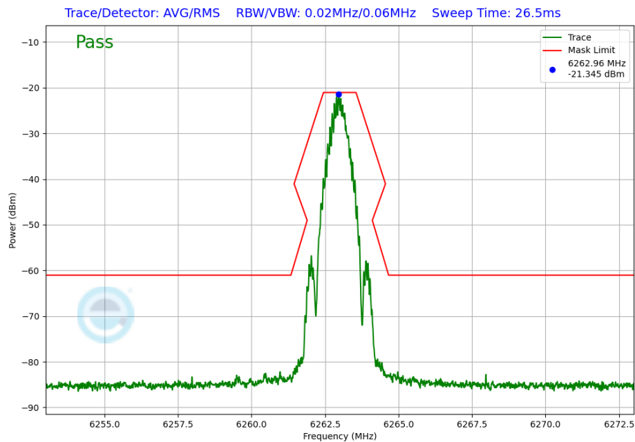
Plot 7-223. In-Band Emission Plot Antenna WF5B (NB UNII BDR, iPA – 6263MHz)
