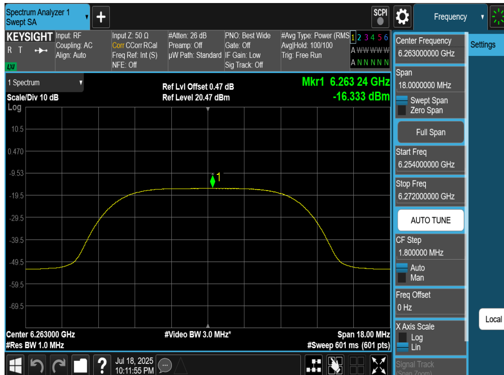
Plot 7-203. PSD TxBF Diversity Antenna 2a (NB UNII HDRPL12, ePA – 6263MHz)
