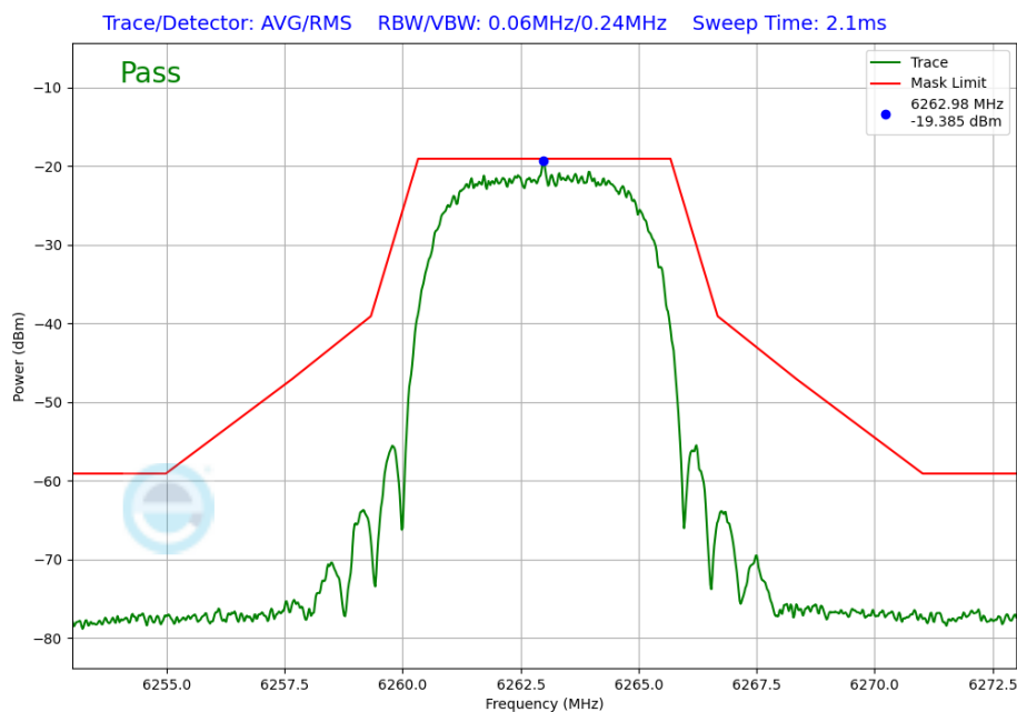
Plot 7-234. In-Band Emission Plot Antenna WF5B (NB UNII XHDRPM6, ePA – 6263MHz)
