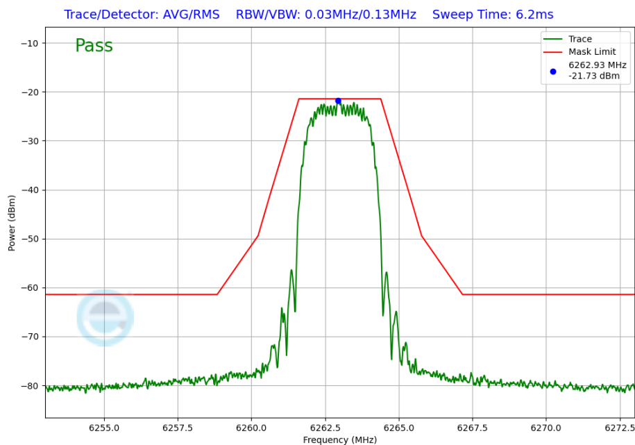
Plot 7-244. In-Band Emission Plot Antenna WF5B (NB UNII HDT4, ePA – 6263MHz)
