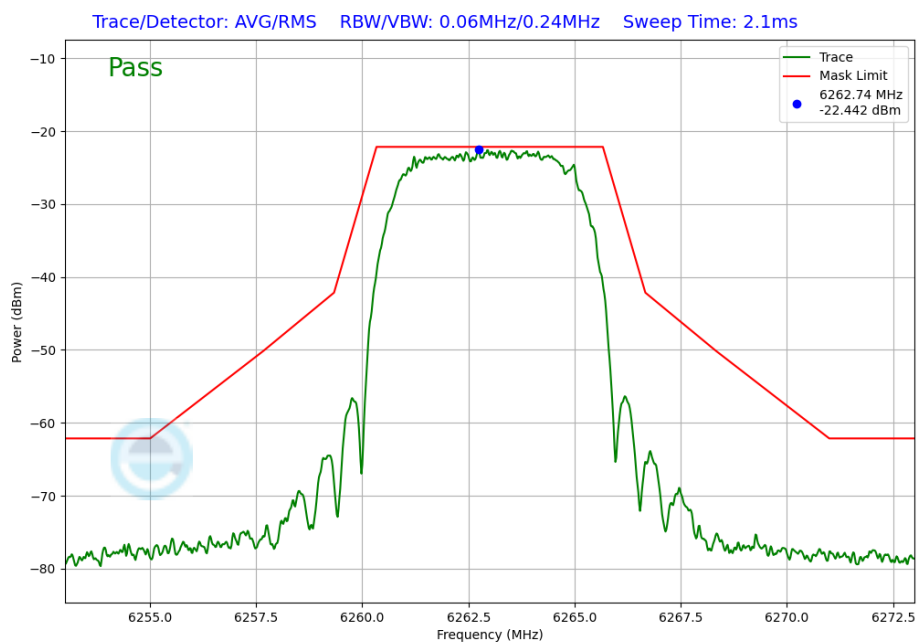
Plot 7-237. In-Band Emission Plot Antenna WF5B (NB UNII HDRPM16, iPA – 6263MHz)
