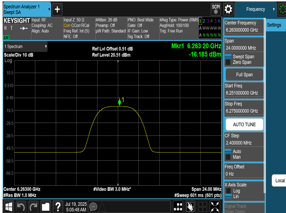
Plot 7-198. PSD TxBF Diversity Antenna 4a (NB UNII HDRPM16, ePA – 6263MHz)
