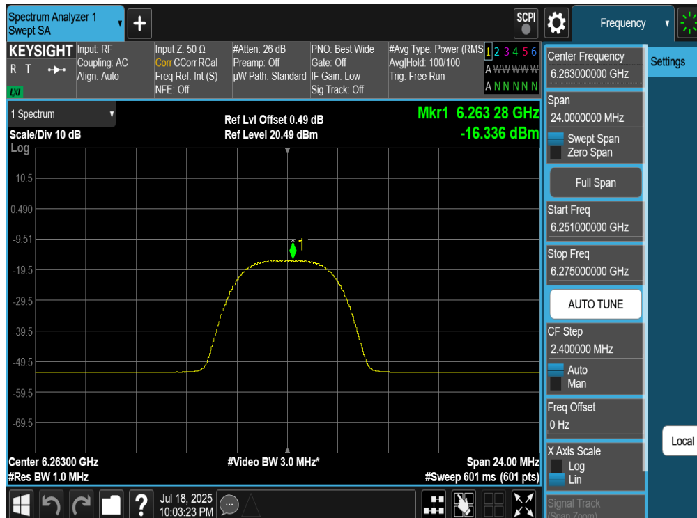
Plot 7-199. PSD TxBF Diversity Antenna 2a (NB UNII HDRPM16, ePA – 6263MHz)
