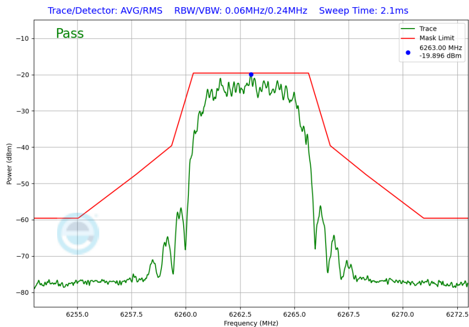
Plot 7-230. In-Band Emission Plot Antenna WF5B (NB UNII HDR8, ePA – 6263MHz)
