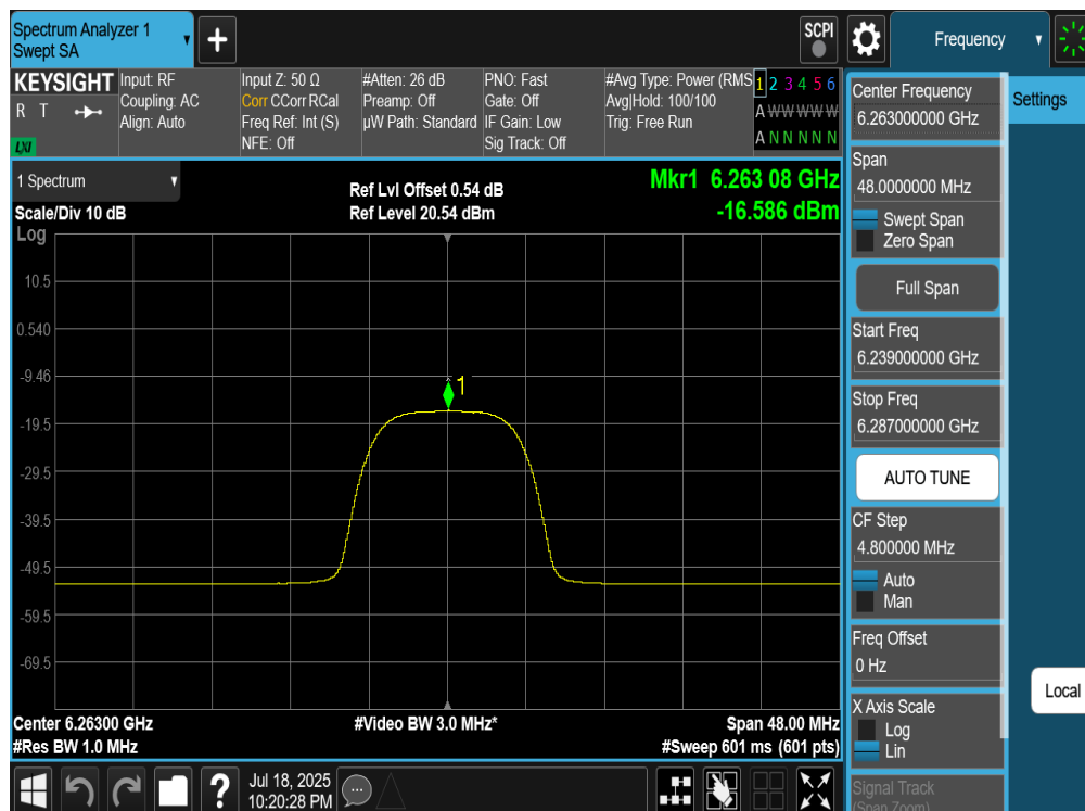
Plot 7-207. PSD TxBF Diversity Antenna 2a (NB UNII HDRPL32, ePA – 6263MHz)
