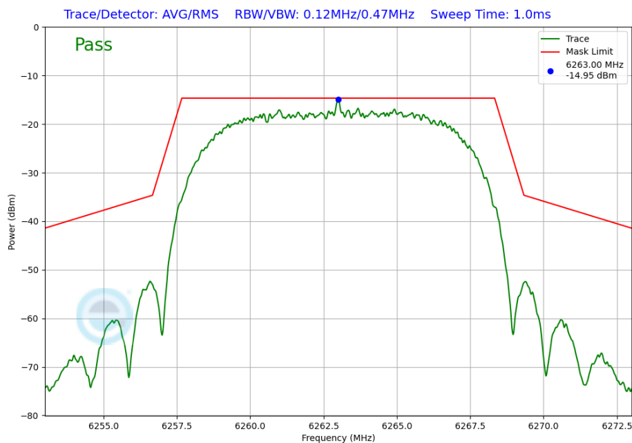
Plot 7-238. In-Band Emission Plot Antenna WF5B (NB UNII HDRPL12, ePA – 6263MHz)
