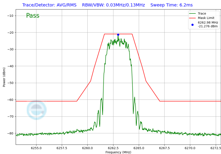
Plot 7-228. In-Band Emission Plot Antenna WF5B (NB UNII HDR4, ePA – 6263MHz)
