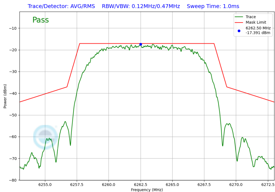
Plot 7-240. In-Band Emission Plot Antenna WF5B (NB UNII HDRPL32, ePA – 6263MHz)
