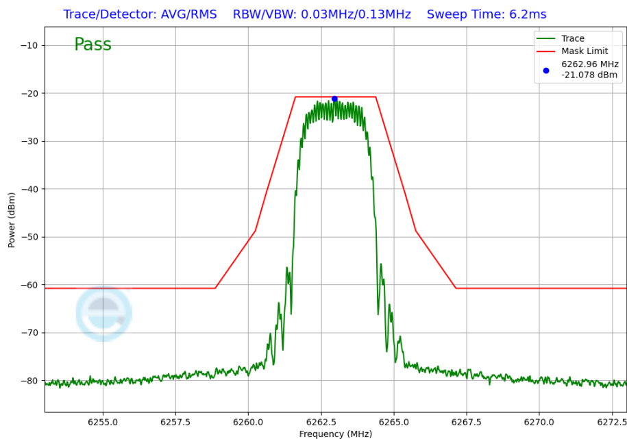
Plot 7-242. In-Band Emission Plot Antenna WF5B (NB UNII HDT2, ePA – 6263MHz)
