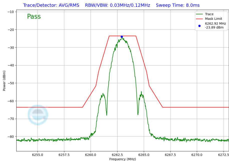
Plot 7-226. In-Band Emission Plot Antenna WF5B (NB UNII LE2M, ePA – 6263MHz)
