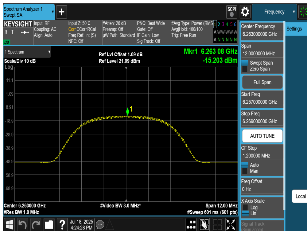
Plot 7-189. PSD TxBF Diversity Antenna 2a (NB UNII HDR8, iPA – 6263MHz)
