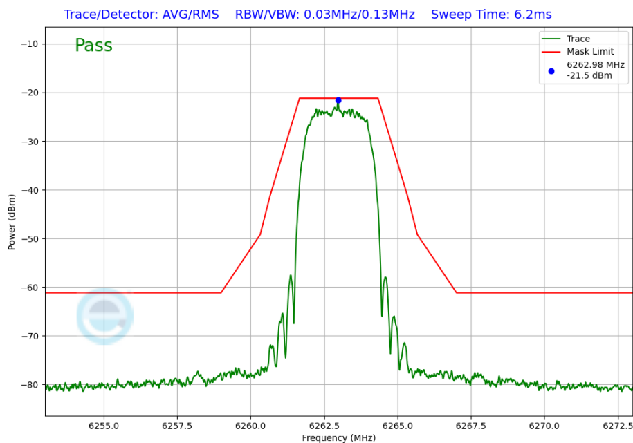
Plot 7-232. In-Band Emission Plot Antenna WF5B (NB UNII HDRPS2, ePA – 6263MHz)
