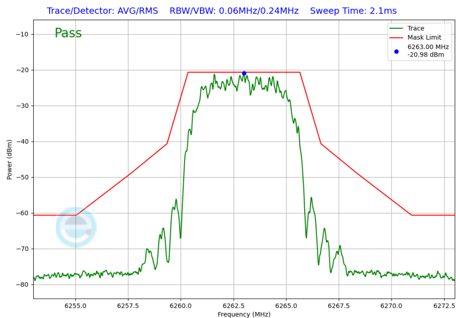
Plot 7-231. In-Band Emission Plot Antenna WF5B (NB UNII HDR8, iPA – 6263MHz)
