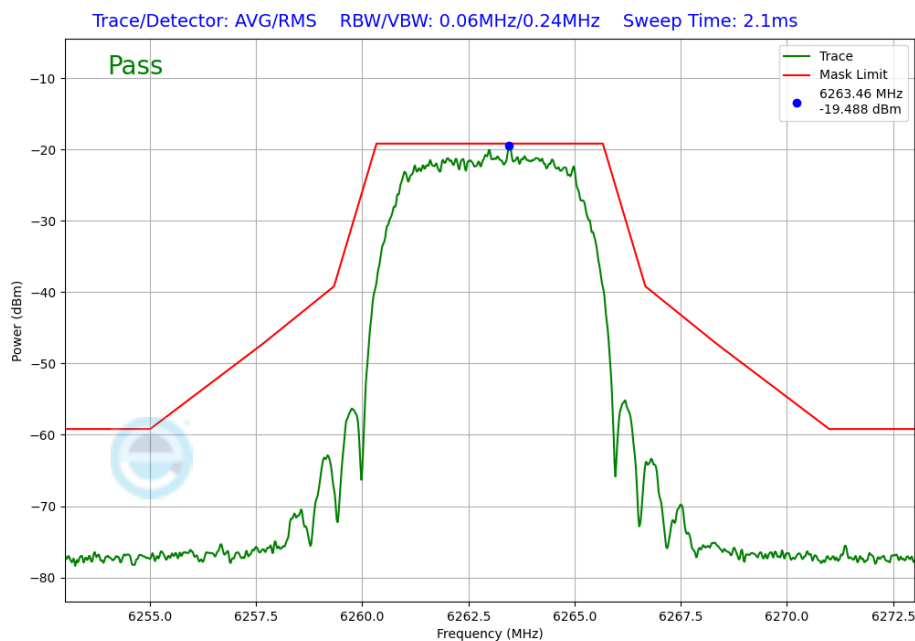
Plot 7-236. In-Band Emission Plot Antenna WF5B (NB UNII HDRPM16, ePA – 6263MHz)
