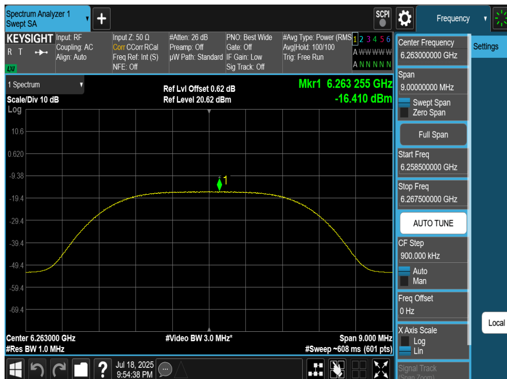
Plot 7-195. PSD TxBF Diversity Antenna 2a (NB UNII XHDRPM6, ePA – 6263MHz)
