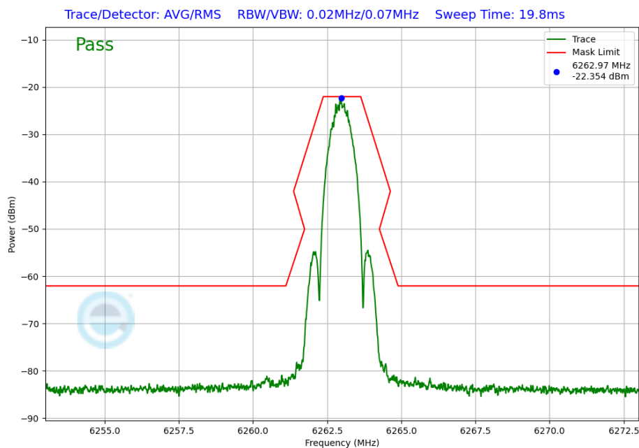
Plot 7-224. In-Band Emission Plot Antenna WF5B (NB UNII LE1M, ePA – 6263MHz)
