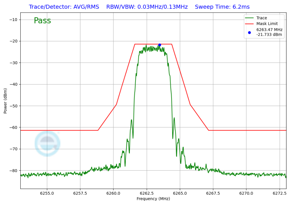
Plot 7-245. In-Band Emission Plot Antenna WF5B (NB UNII HDT4, iPA – 6263MHz)
