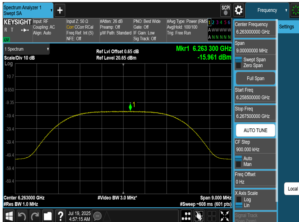
Plot 7-194. PSD TxBF Diversity Antenna 4a (NB UNII XHDRPM6, ePA – 6263MHz)
