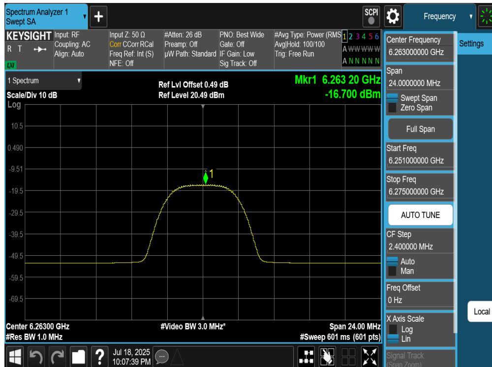
Plot 7-201. PSD TxBF Diversity Antenna 2a (NB UNII HDRPM16, iPA – 6263MHz)
