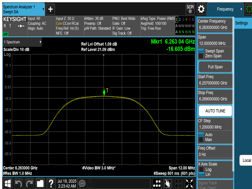
Plot 7-188. PSD TxBF Diversity Antenna 4a (NB UNII HDR8, iPA – 6263MHz)
