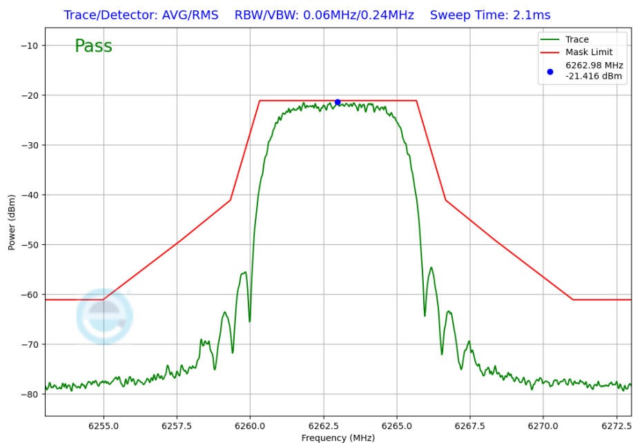
Plot 7-235. In-Band Emission Plot Antenna WF5B (NB UNII XHDRPM6, iPA – 6263MHz)
