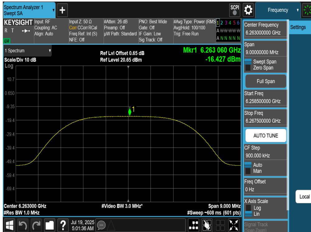
Plot 7-196. PSD TxBF Diversity Antenna 4a (NB UNII XHDRPM6, iPA – 6263MHz)
