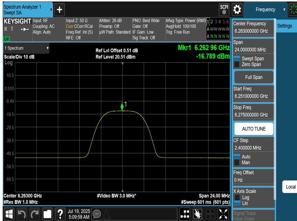
Plot 7-200. PSD TxBF Diversity Antenna 4a (NB UNII HDRPM16, iPA – 6263MHz)
