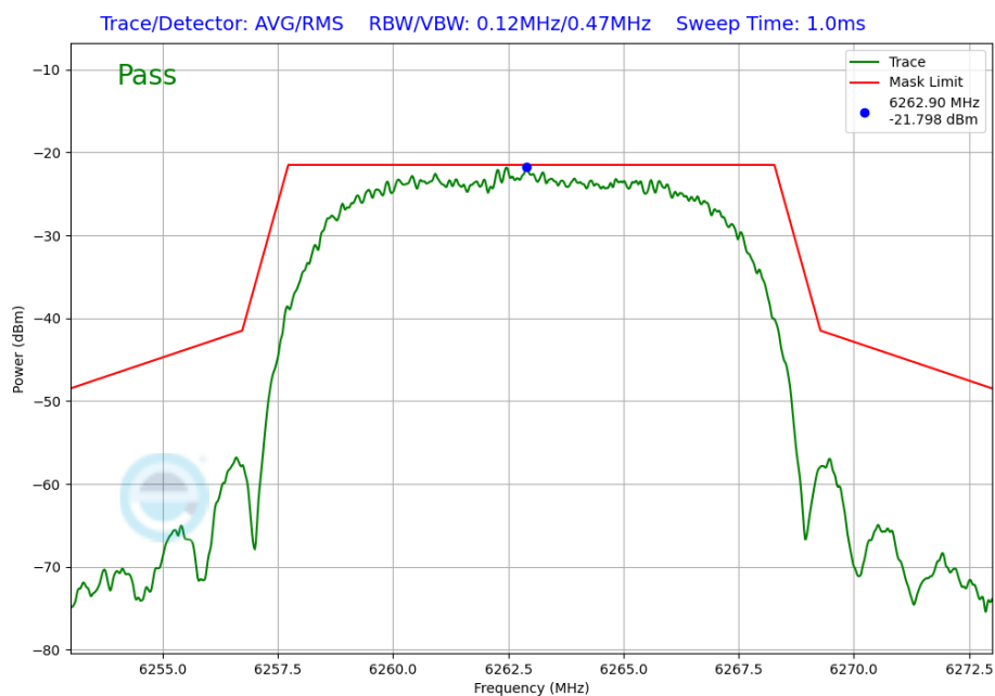
Plot 7-241. In-Band Emission Plot Antenna WF5B (NB UNII HDRPL32, iPA – 6263MHz)
