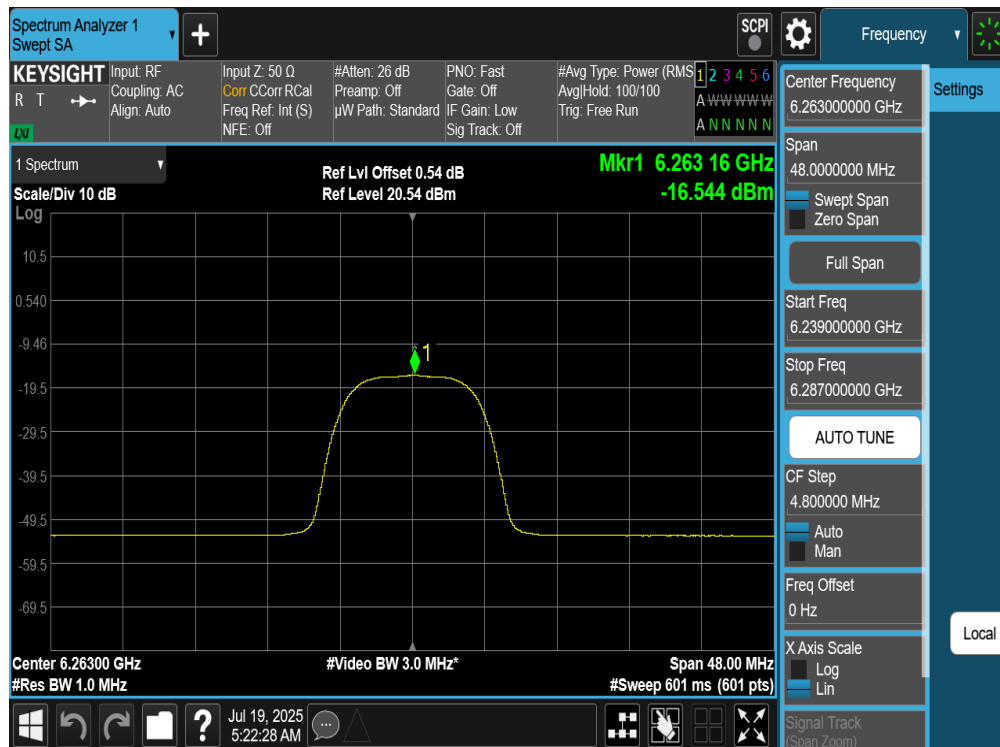
Plot 7-206. PSD TxBF Diversity Antenna 4a (NB UNII HDRPL32, ePA – 6263MHz)
