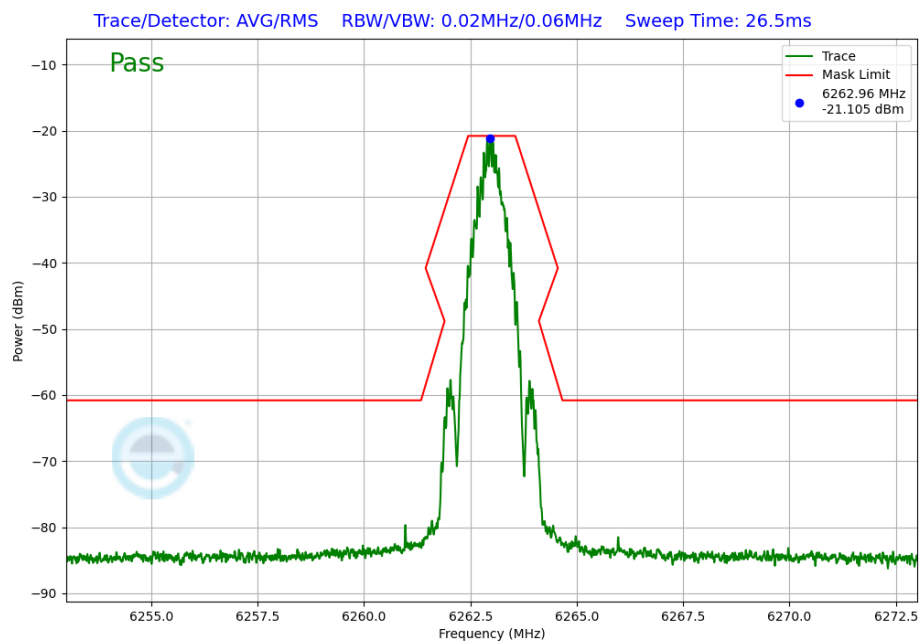
Plot 7-222. In-Band Emission Plot Antenna WF5B (NB UNII BDR, ePA – 6263MHz)
