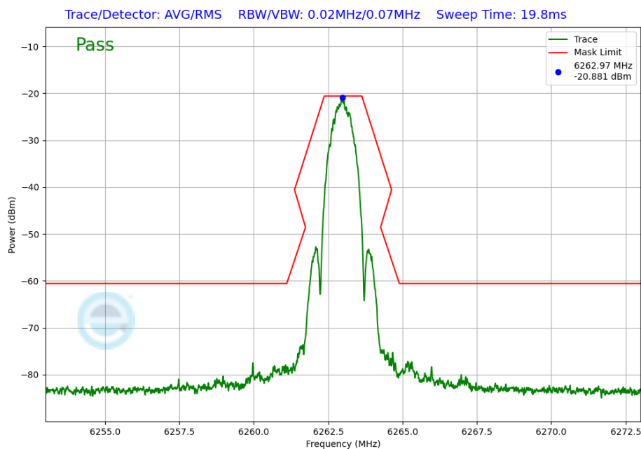
Plot 7-276. In-Band Emission Plot Antenna 2a (NB UNII LE1M, ePA – 6263MHz)
