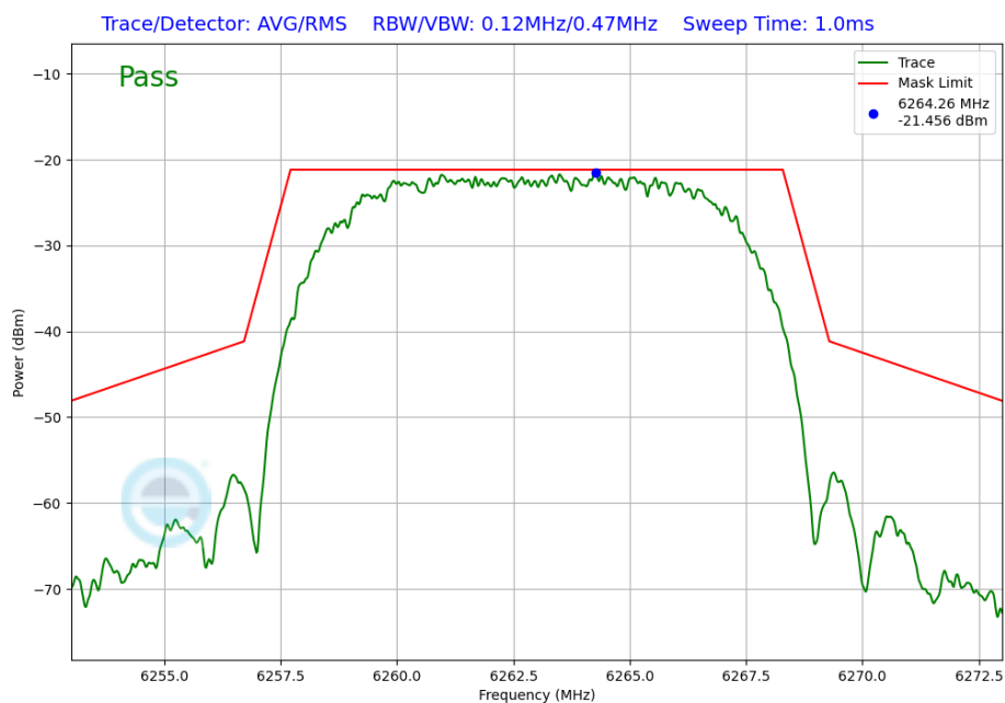
Plot 7-291. In-Band Emission Plot Antenna 2a (NB UNII HDRPL12, iPA – 6263MHz)
