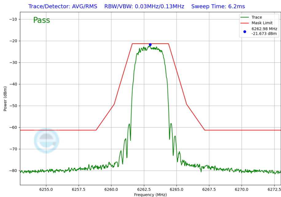
Plot 7-246. In-Band Emission Plot Antenna WF5B (NB UNII HDT6, ePA – 6263MHz)
