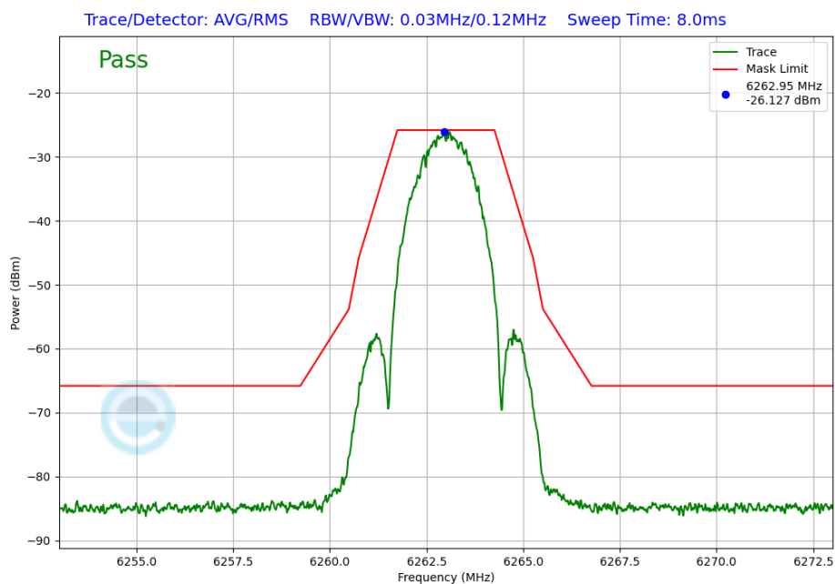
Plot 7-253. In-Band Emission Plot Antenna 4a (NB UNII LE2M, iPA – 6263MHz)
