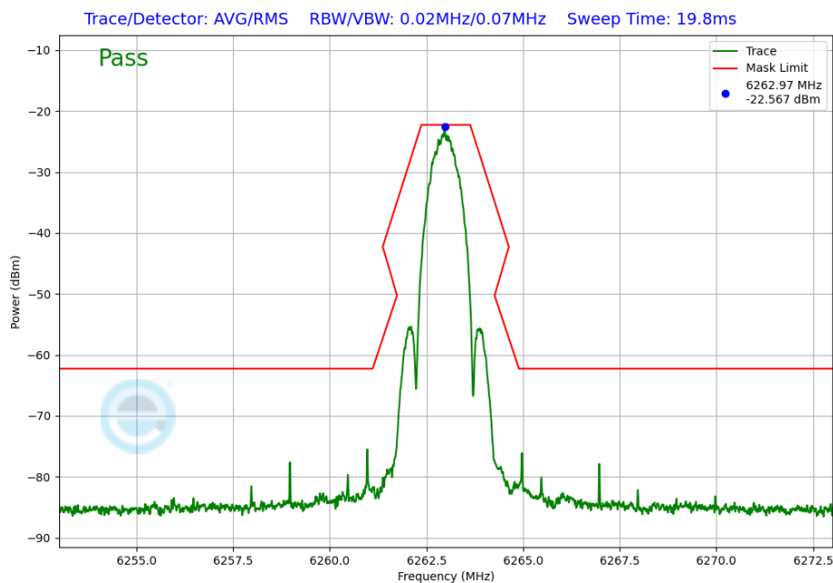
Plot 7-250. In-Band Emission Plot Antenna 4a (NB UNII LE1M, ePA – 6263MHz)
