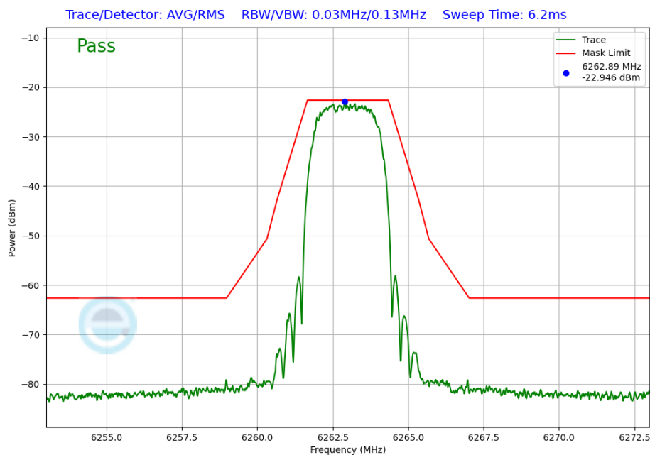
Plot 7-258. In-Band Emission Plot Antenna 4a (NB UNII HDRPS2, ePA – 6263MHz)
