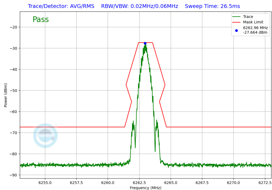
Plot 7-302. In-Band Emission Plot TxBF Primary Antenna WF5B (NB UNII BDR, iPA – 6263MHz)
