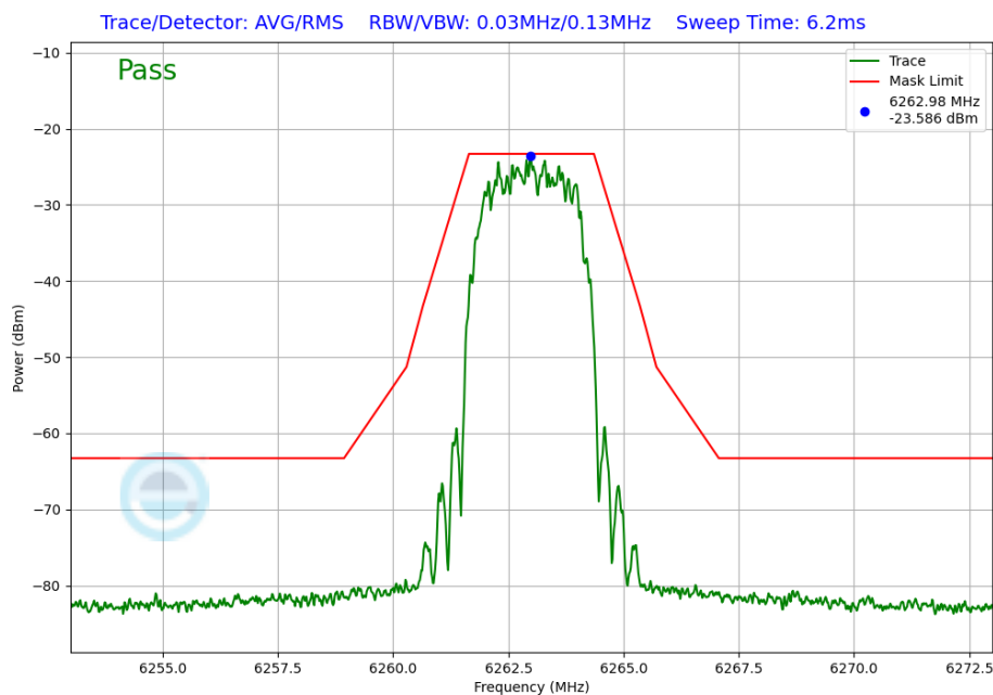
Plot 7-254. In-Band Emission Plot Antenna 4a (NB UNII HDR4, ePA – 6263MHz)
