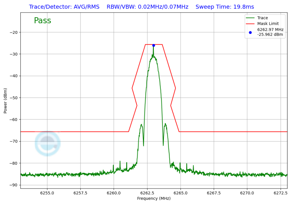
Plot 7-305. In-Band Emission Plot TxBF Primary Antenna 4a (NB UNII LE1M, ePA – 6263MHz)
