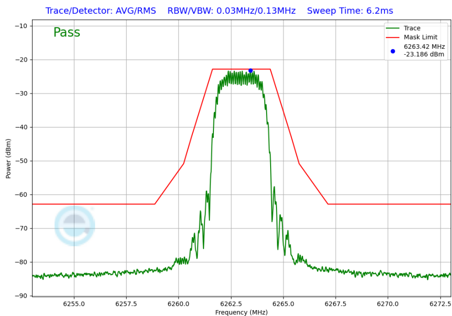
Plot 7-269. In-Band Emission Plot Antenna 4a (NB UNII HDT2, iPA – 6263MHz)
