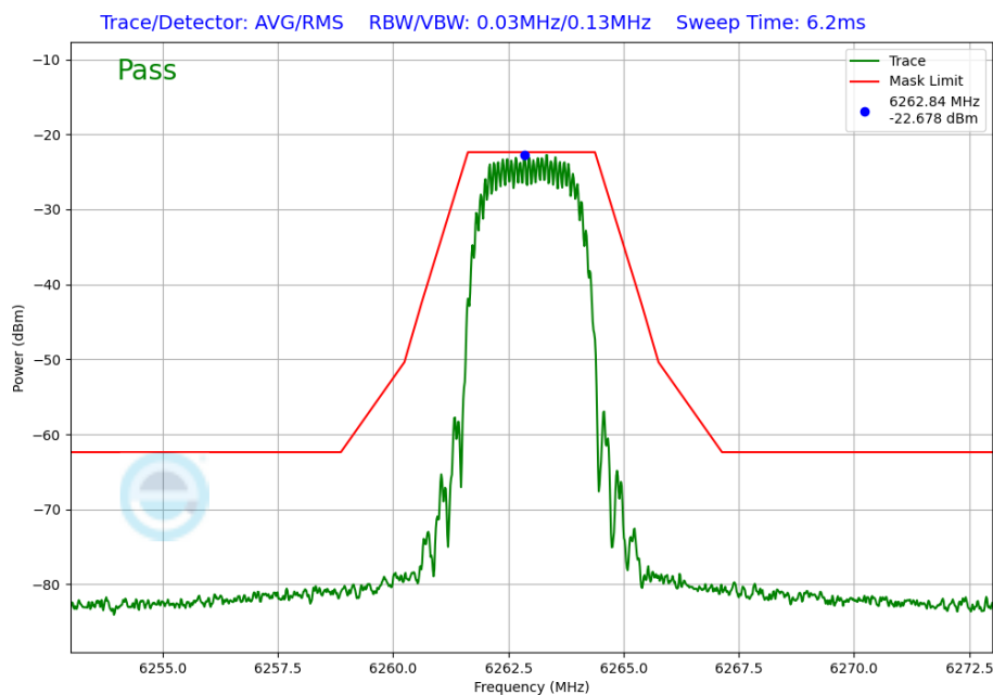
Plot 7-294. In-Band Emission Plot Antenna 2a (NB UNII HDT2, ePA – 6263MHz)
