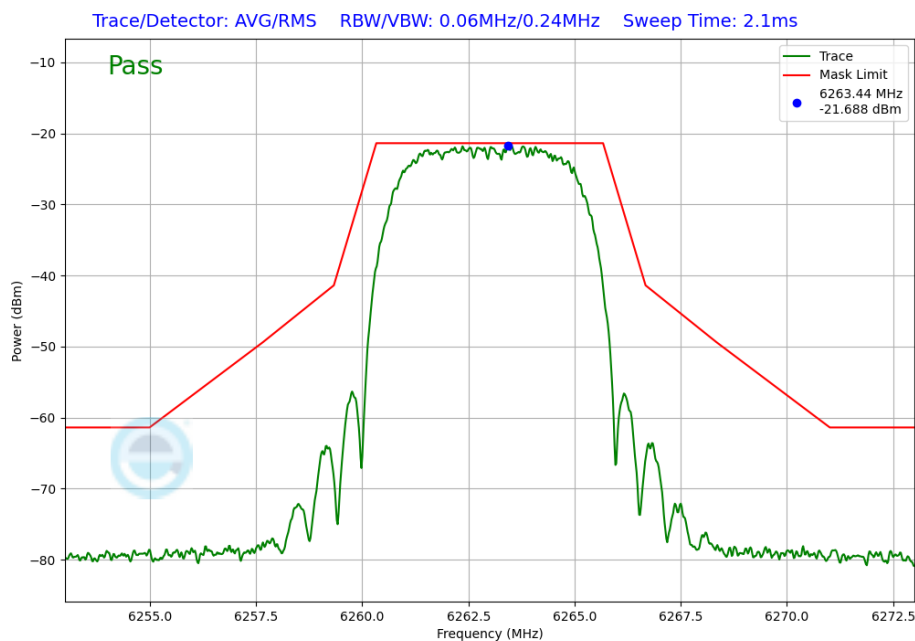
Plot 7-288. In-Band Emission Plot Antenna 2a (NB UNII HDRPM16, ePA – 6263MHz)
