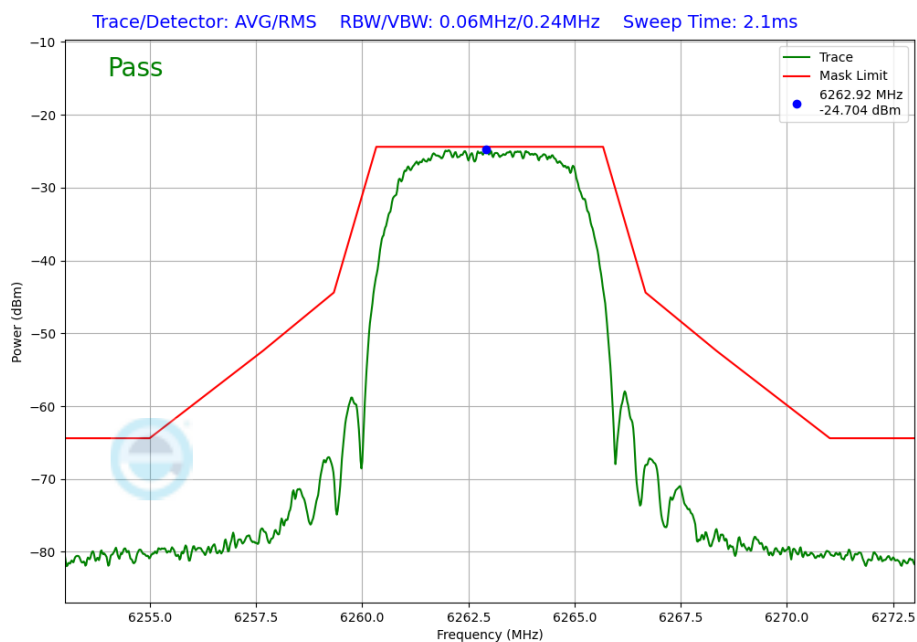
Plot 7-289. In-Band Emission Plot Antenna 2a (NB UNII HDRPM16, iPA – 6263MHz)
