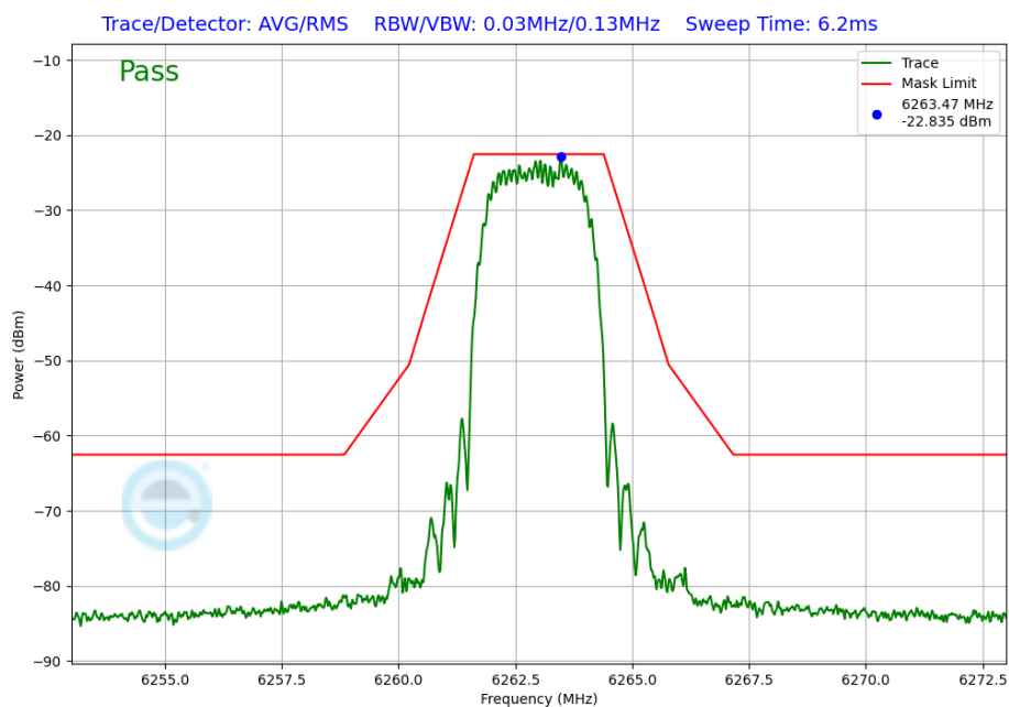
Plot 7-271. In-Band Emission Plot Antenna 4a (NB UNII HDT4, iPA – 6263MHz)
