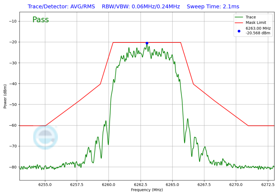
Plot 7-257. In-Band Emission Plot Antenna 4a (NB UNII HDR8, iPA – 6263MHz)
