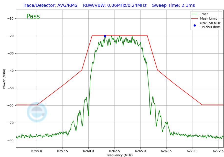
Plot 7-283. In-Band Emission Plot Antenna 2a (NB UNII HDR8, iPA – 6263MHz)
