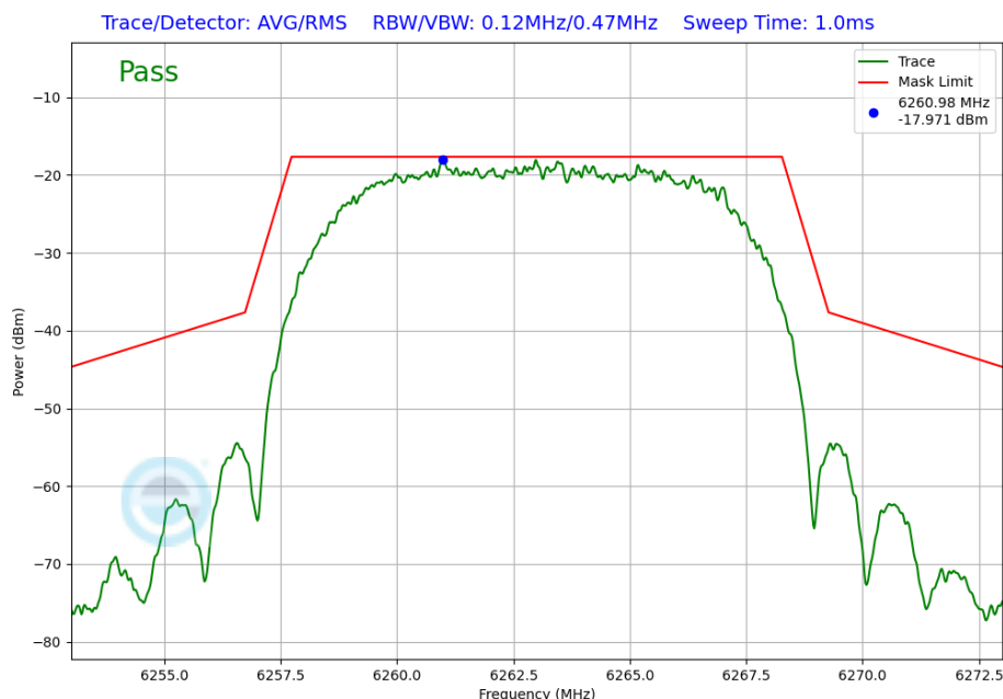
Plot 7-292. In-Band Emission Plot Antenna 2a (NB UNII HDRPL32, ePA – 6263MHz)
