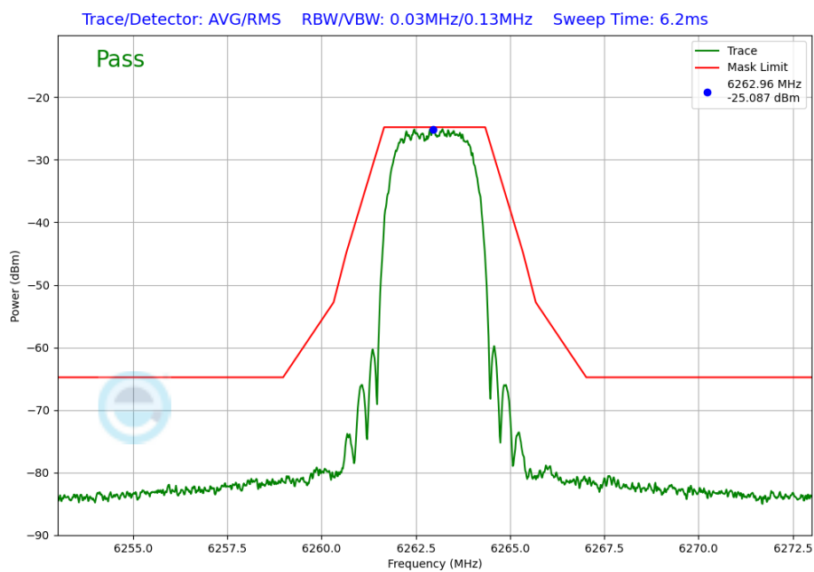
Plot 7-259. In-Band Emission Plot Antenna 4a (NB UNII HDRPS2, iPA – 6263MHz)
