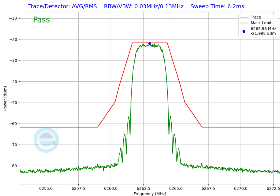
Plot 7-284. In-Band Emission Plot Antenna 2a (NB UNII HDRPS2, ePA – 6263MHz)
