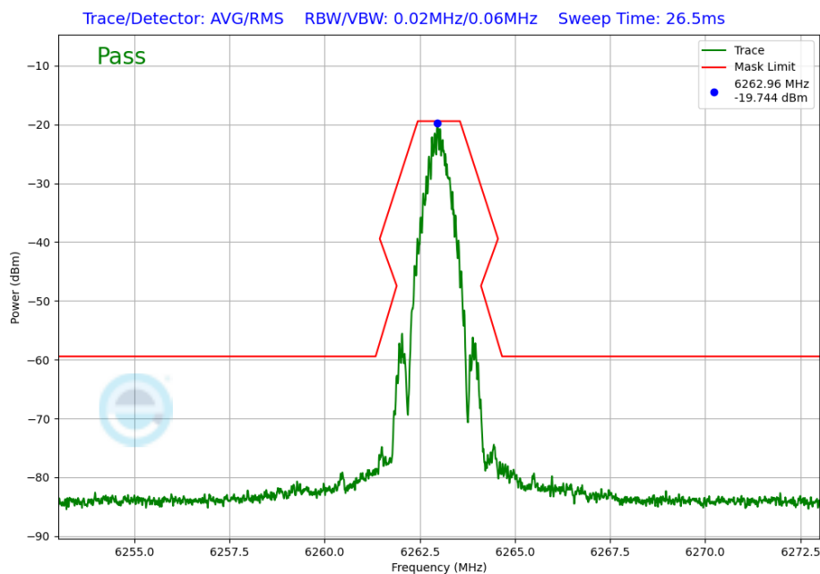
Plot 7-274. In-Band Emission Plot Antenna 2a (NB UNII BDR, ePA – 6263MHz)
