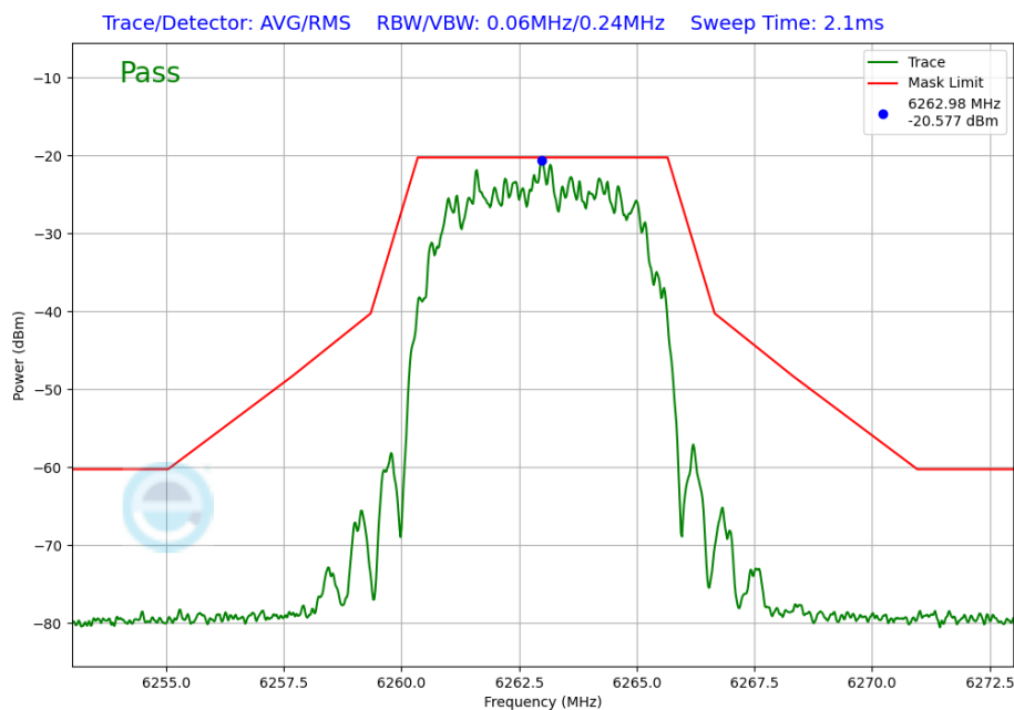
Plot 7-256. In-Band Emission Plot Antenna 4a (NB UNII HDR8, ePA – 6263MHz)
