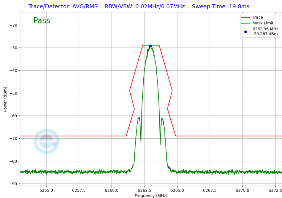
Plot 7-306. In-Band Emission Plot Tx BF Primary Antenna WF5B (NB UNII LE1M, iPA – 6263MHz)
