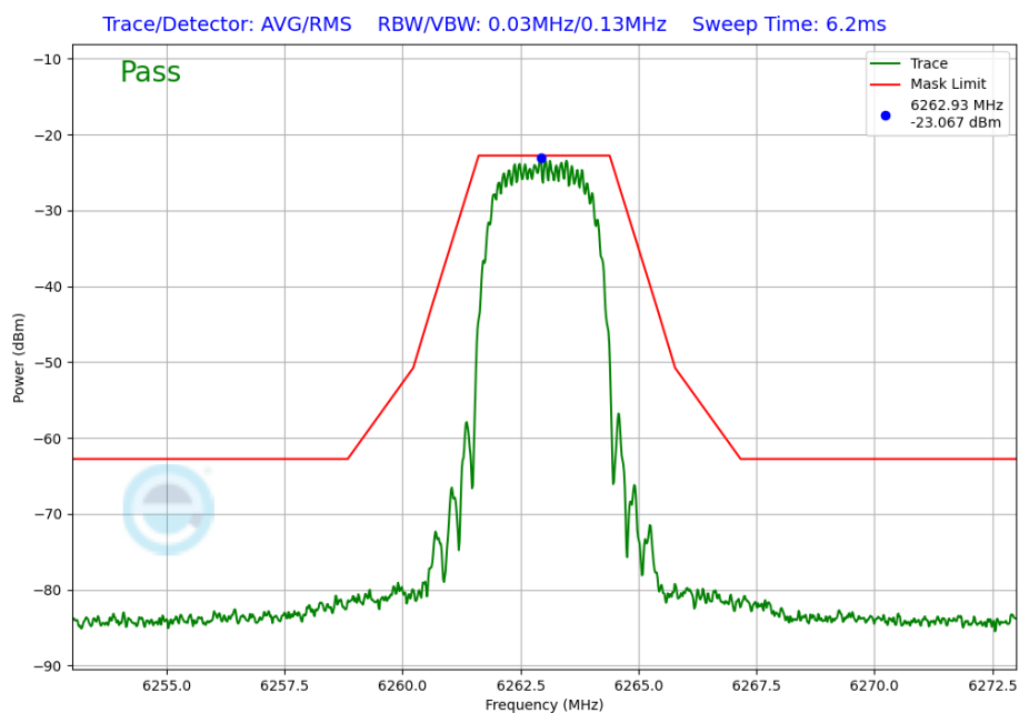
Plot 7-297. In-Band Emission Plot Antenna 2a (NB UNII HDT4, iPA – 6263MHz)
