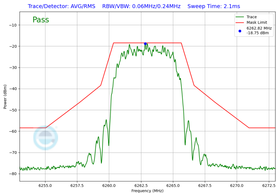
Plot 7-282. In-Band Emission Plot Antenna 2a (NB UNII HDR8, ePA – 6263MHz)
