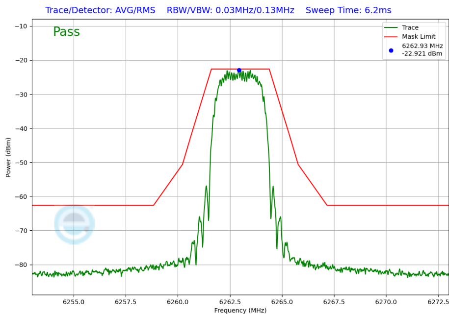
Plot 7-296. In-Band Emission Plot Antenna 2a (NB UNII HDT4, ePA – 6263MHz)
