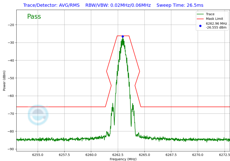
Plot 7-300. In-Band Emission Plot TxBF Primary Antenna WF5B (NB UNII BDR, ePA – 6263MHz)
