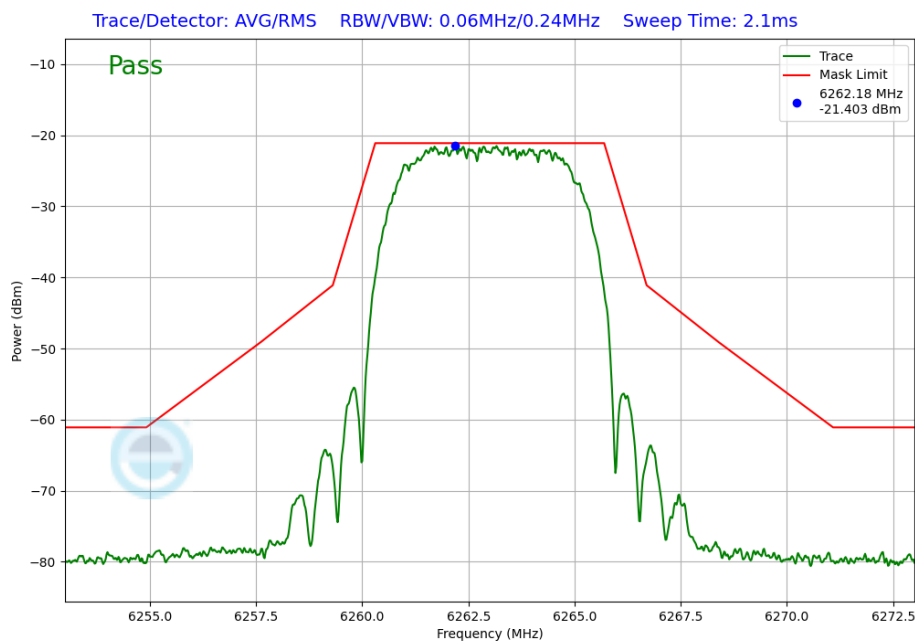
Plot 7-286. In-Band Emission Plot Antenna 2a (NB UNII XHDRPM6, ePA – 6263MHz)
