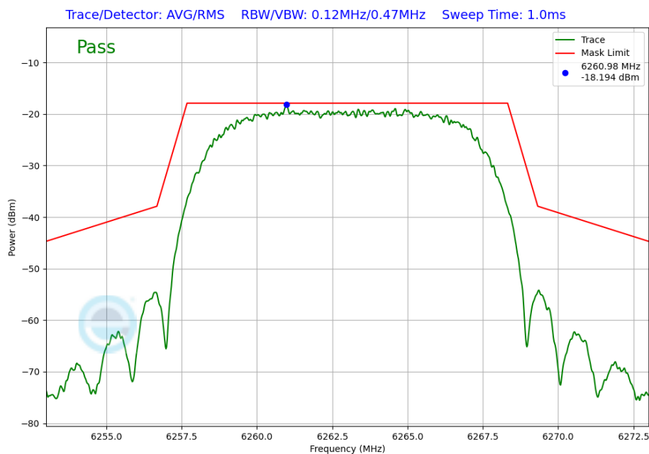
Plot 7-264. In-Band Emission Plot Antenna 4a (NB UNII HDRPL12, ePA – 6263MHz)
