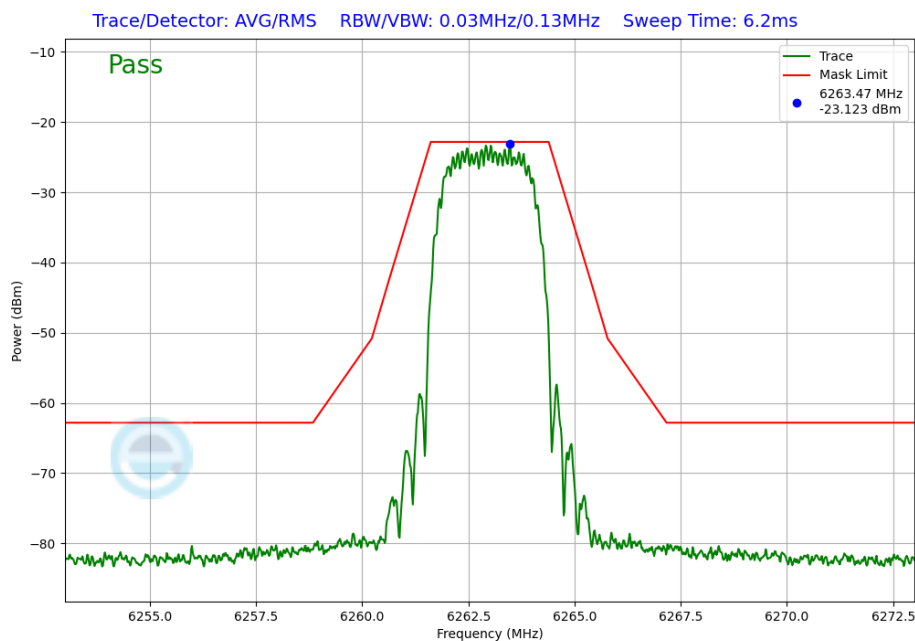
Plot 7-270. In-Band Emission Plot Antenna 4a (NB UNII HDT4, ePA – 6263MHz)
