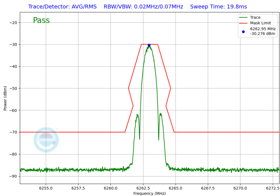
Plot 7-307. In-Band Emission Plot Tx BF Primary Antenna 4a (NB UNII LE1M, iPA – 6263MHz)
