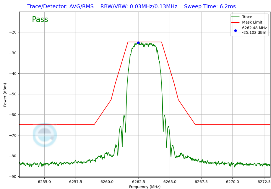
Plot 7-285. In-Band Emission Plot Antenna 2a (NB UNII HDRPS2, iPA – 6263MHz)
