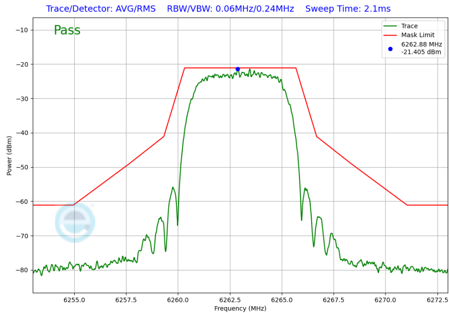
Plot 7-263. In-Band Emission Plot Antenna 4a (NB UNII HDRPM16, iPA – 6263MHz)
