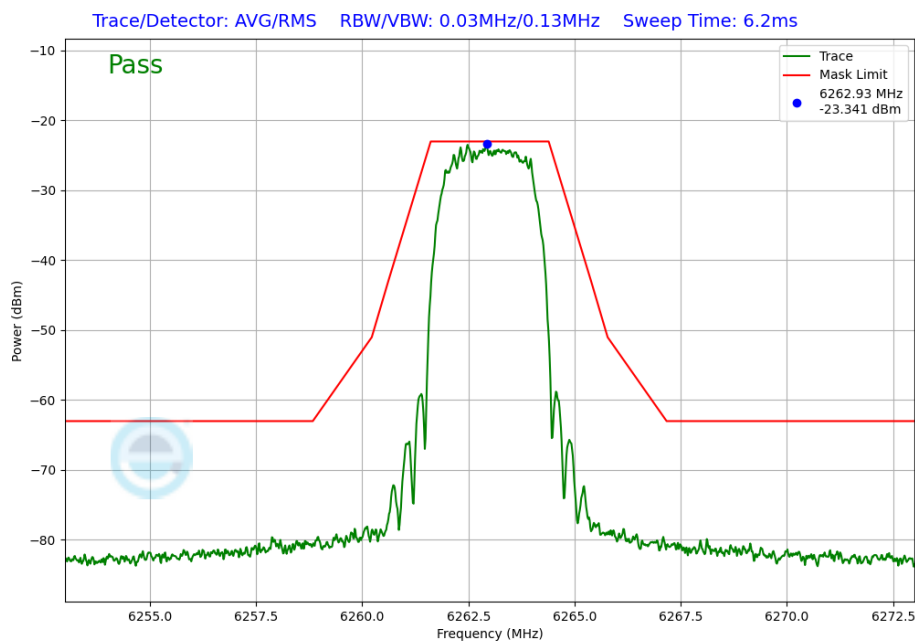
Plot 7-298. In-Band Emission Plot Antenna 2a (NB UNII HDT6, ePA – 6263MHz)
