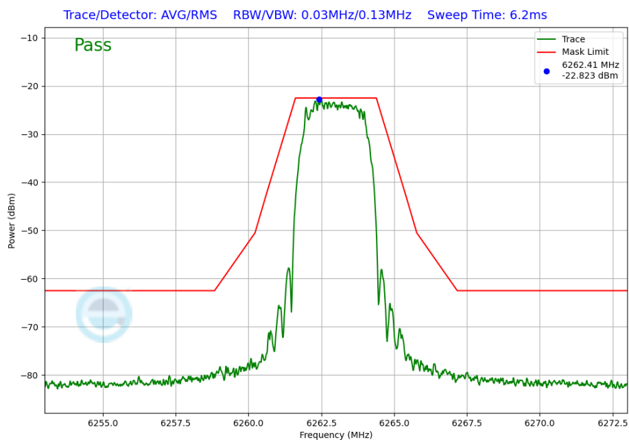
Plot 7-247. In-Band Emission Plot Antenna WF5B (NB UNII HDT6, iPA – 6263MHz)
