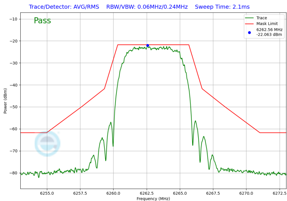
Plot 7-261. In-Band Emission Plot Antenna 4a (NB UNII XHDRPM6, iPA – 6263MHz)
