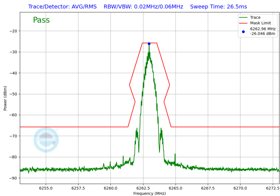
Plot 7-301. In-Band Emission Plot TxBF Primary Antenna 4a (NB UNII BDR, ePA – 6263MHz)
