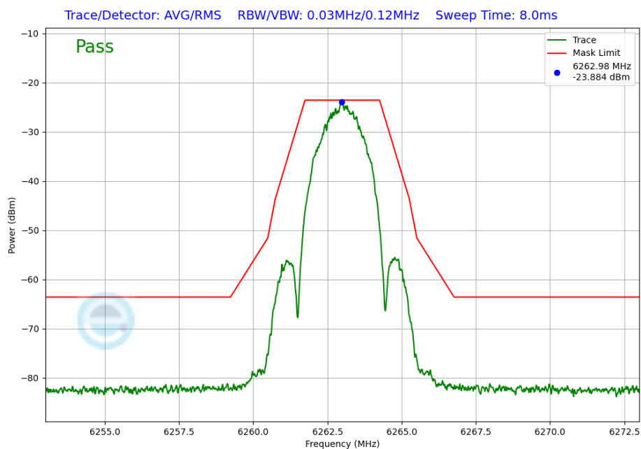
Plot 7-279. In-Band Emission Plot Antenna 2a (NB UNII LE2M, iPA – 6263MHz)
