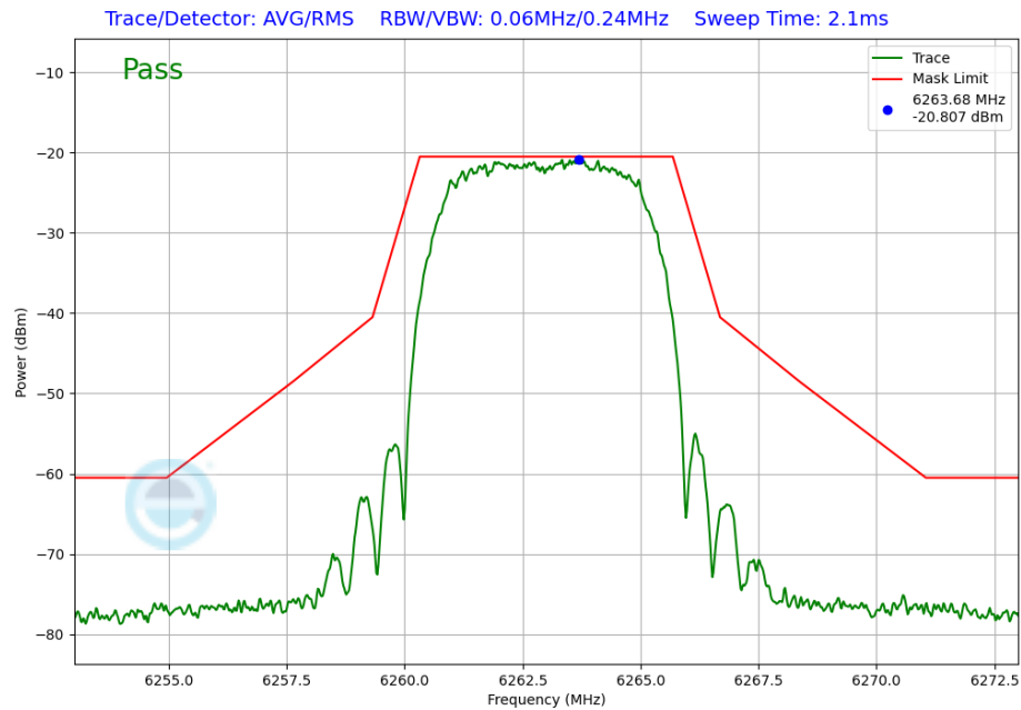
Plot 7-262. In-Band Emission Plot Antenna 4a (NB UNII HDRPM16, ePA – 6263MHz)
