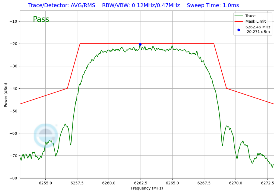
Plot 7-267. In-Band Emission Plot Antenna 4a (NB UNII HDRPL32, iPA – 6263MHz)
