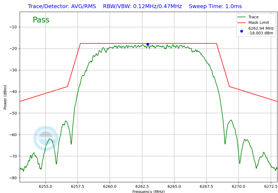
Plot 7-290. In-Band Emission Plot Antenna 2a (NB UNII HDRPL12, ePA – 6263MHz)
