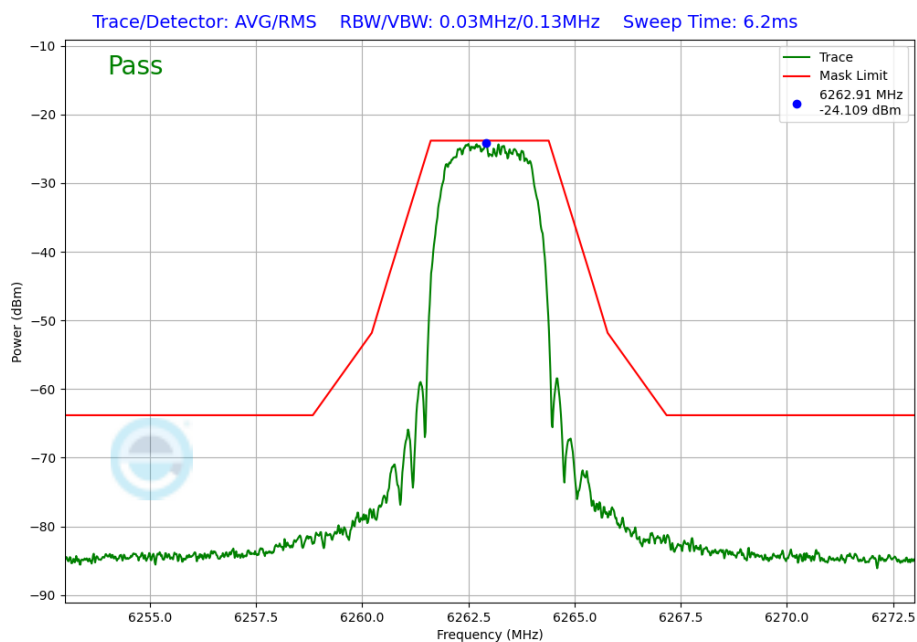
Plot 7-299. In-Band Emission Plot Antenna 2a (NB UNII HDT6, iPA – 6263MHz)
