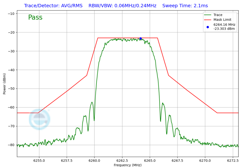
Plot 7-287. In-Band Emission Plot Antenna 2a (NB UNII XHDRPM6, iPA – 6263MHz)
