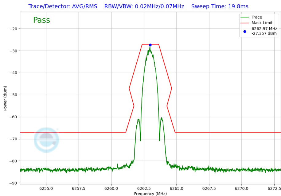
Plot 7-304. In-Band Emission Plot TxBF Primary Antenna WF5B (NB UNII LE1M, ePA – 6263MHz)
