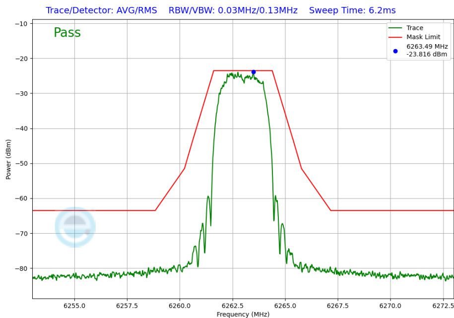
Plot 7-272. In-Band Emission Plot Antenna 4a (NB UNII HDT6, ePA – 6263MHz)
