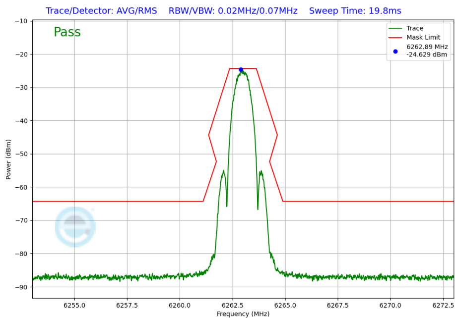
Plot 7-251. In-Band Emission Plot Antenna 4a (NB UNII LE1M, iPA – 6263MHz)
