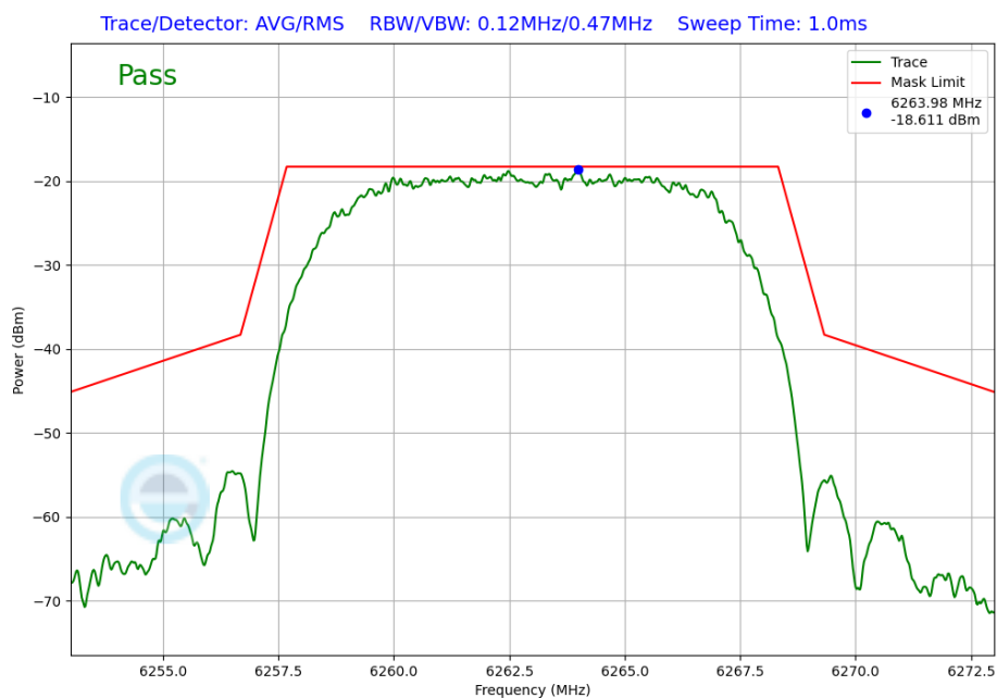
Plot 7-265. In-Band Emission Plot Antenna 4a (NB UNII HDRPL12, iPA – 6263MHz)
