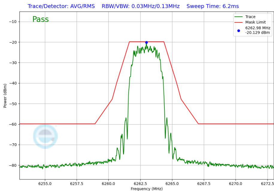
Plot 7-280. In-Band Emission Plot Antenna 2a (NB UNII HDR4, ePA – 6263MHz)
