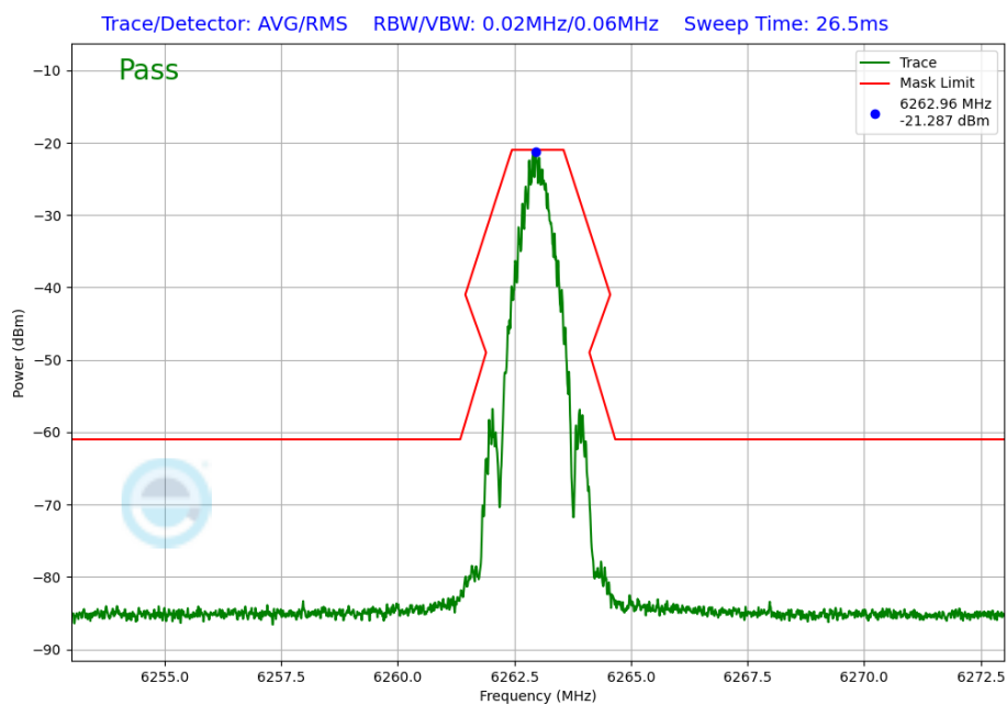
Plot 7-275. In-Band Emission Plot Antenna 2a (NB UNII BDR, iPA – 6263MHz)
