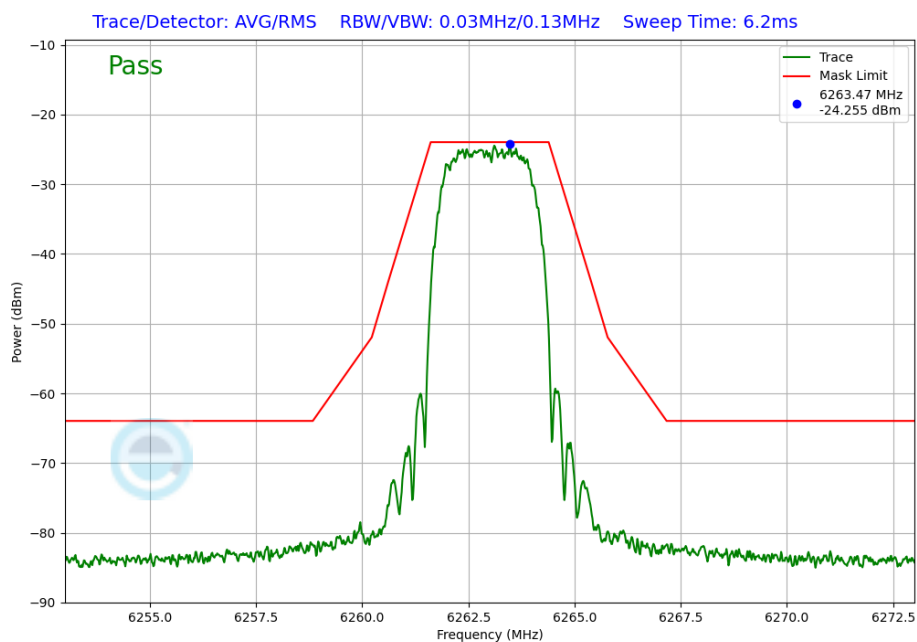
Plot 7-273. In-Band Emission Plot Antenna 4a (NB UNII HDT6, iPA – 6263MHz)
