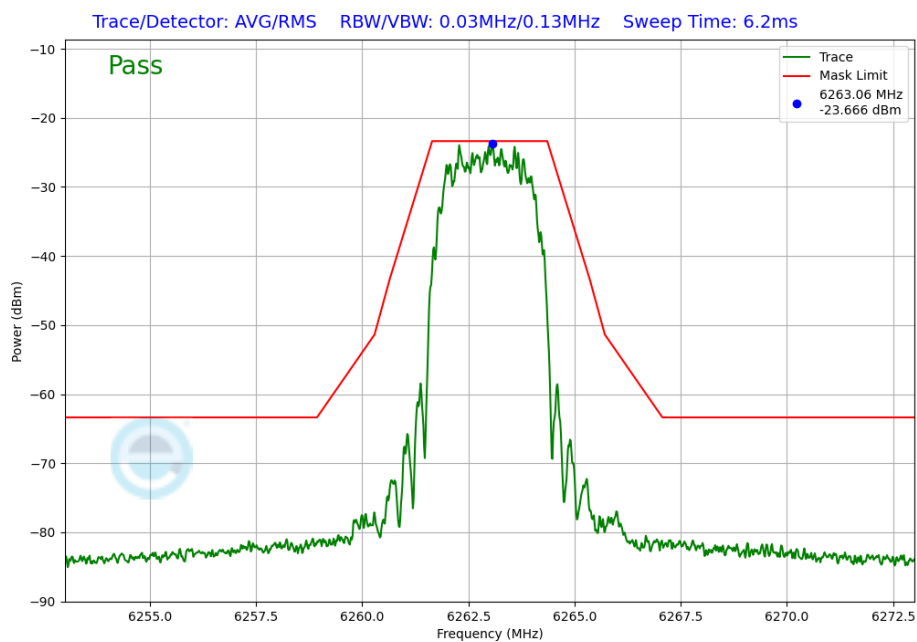
Plot 7-255. In-Band Emission Plot Antenna 4a (NB UNII HDR4, iPA – 6263MHz)
