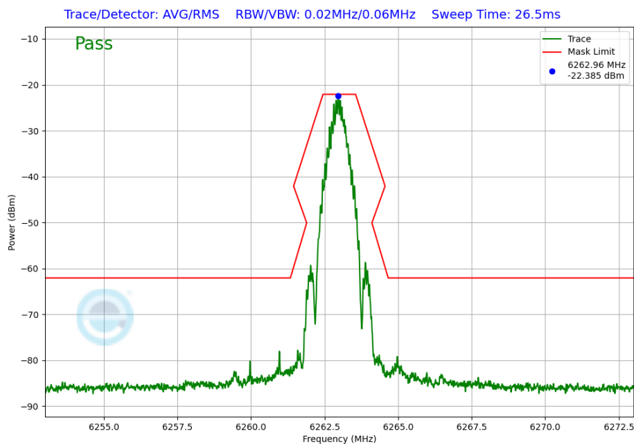
Plot 7-248. In-Band Emission Plot Antenna 4a (NB UNII BDR, ePA – 6263MHz)
