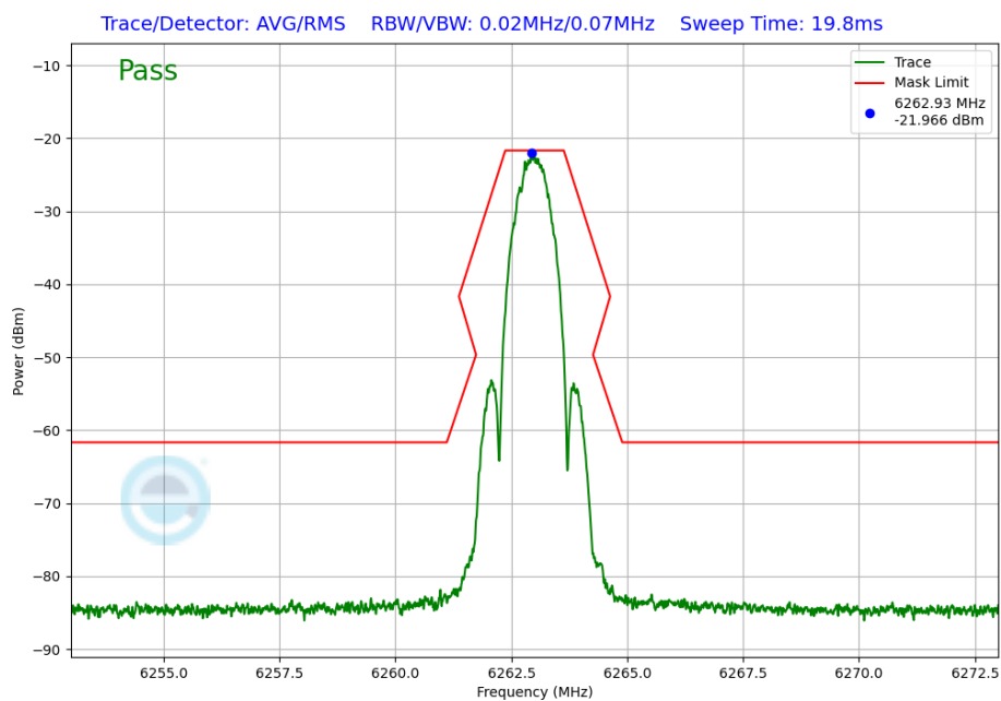
Plot 7-277. In-Band Emission Plot Antenna 2a (NB UNII LE1M, iPA – 6263MHz)
