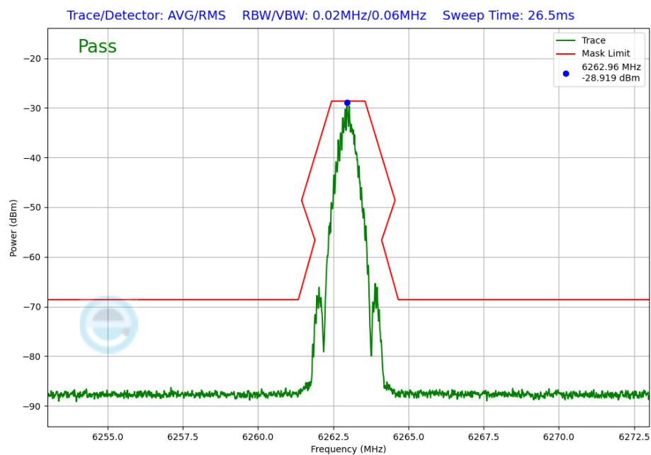
Plot 7-303. In-Band Emission Plot TxBF Primary Antenna 4a (NB UNII BDR, iPA – 6263MHz)
