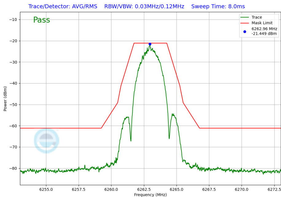
Plot 7-278. In-Band Emission Plot Antenna 2a (NB UNII LE2M, ePA – 6263MHz)
