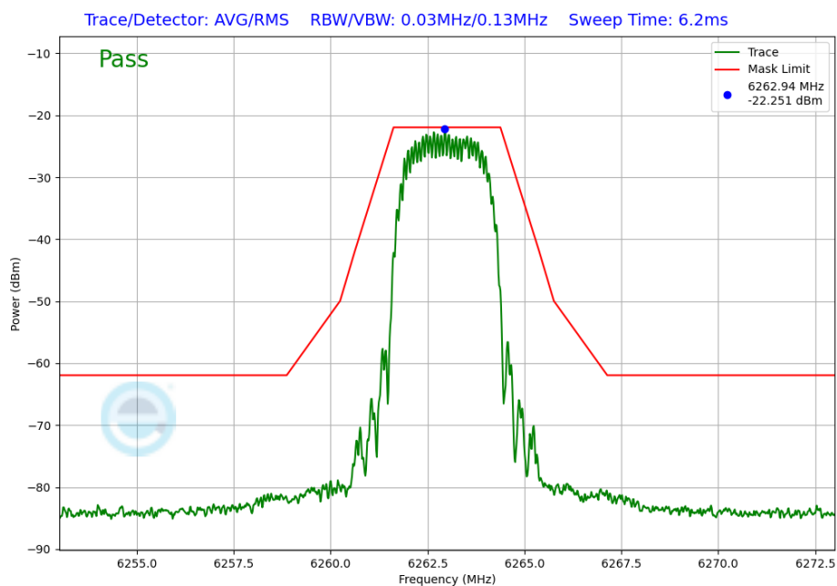
Plot 7-295. In-Band Emission Plot Antenna 2a (NB UNII HDT2, iPA – 6263MHz)
