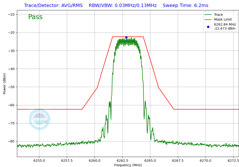
Plot 7-268. In-Band Emission Plot Antenna 4a (NB UNII HDT2, ePA – 6263MHz)
