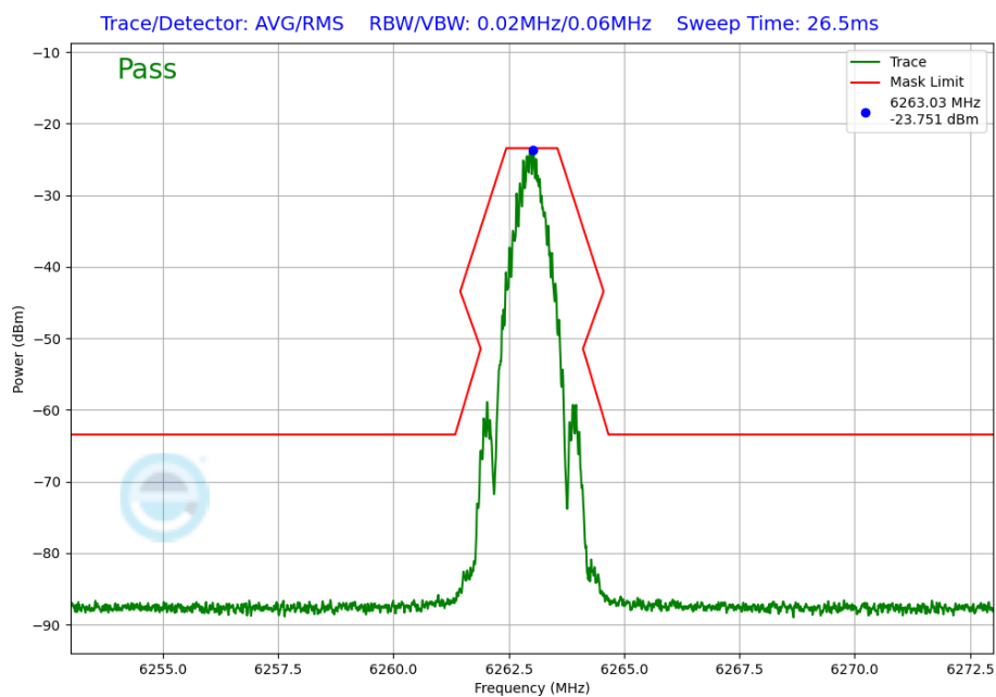
Plot 7-249. In-Band Emission Plot Antenna 4a (NB UNII BDR, iPA – 6263MHz)
