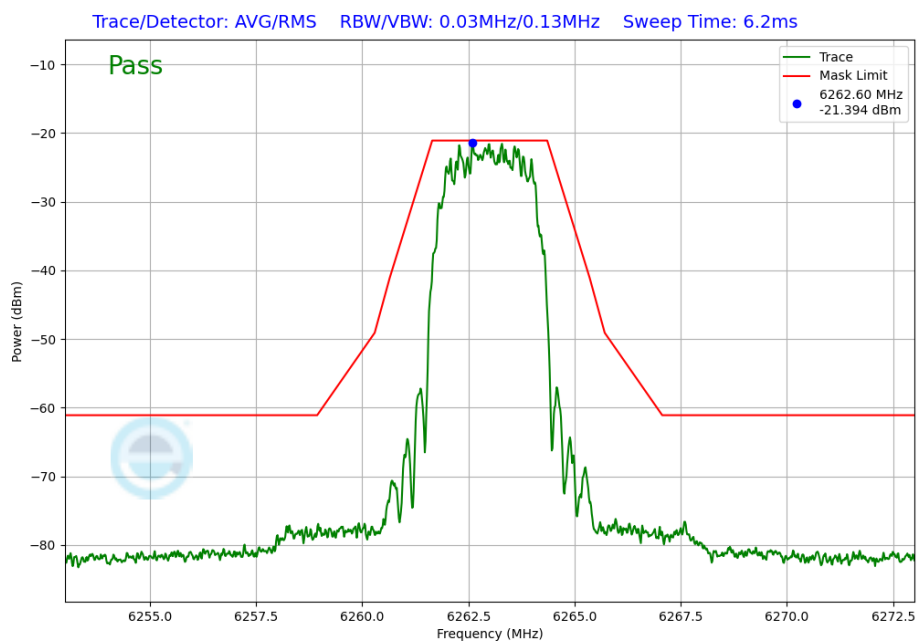
Plot 7-281. In-Band Emission Plot Antenna 2a (NB UNII HDR4, iPA – 6263MHz)
