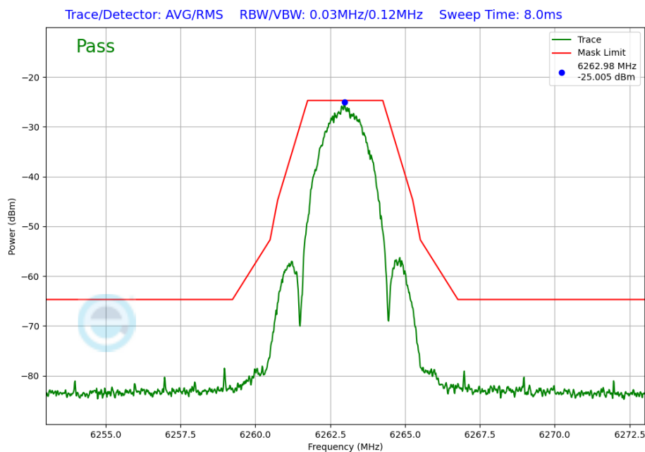
Plot 7-252. In-Band Emission Plot Antenna 4a (NB UNII LE2M, ePA – 6263MHz)
