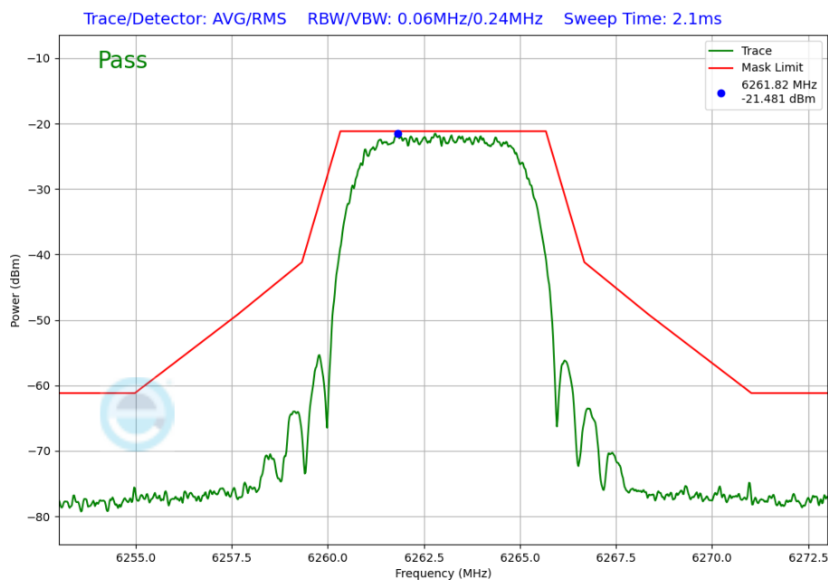
Plot 7-260. In-Band Emission Plot Antenna 4a (NB UNII XHDRPM6, ePA – 6263MHz)
