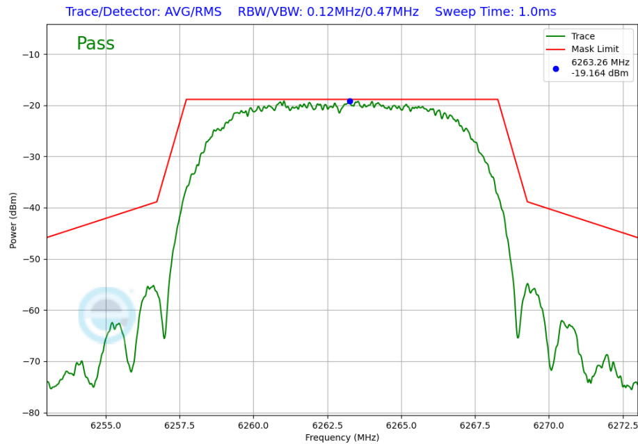
Plot 7-266. In-Band Emission Plot Antenna 4a (NB UNII HDRPL32, ePA – 6263MHz)
