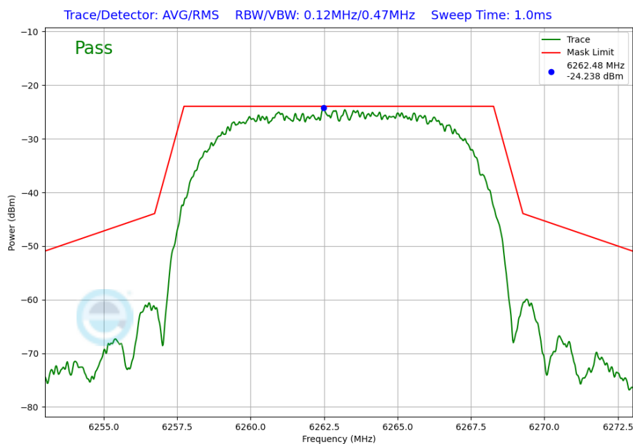
Plot 7-293. In-Band Emission Plot Antenna 2a (NB UNII HDRPL32, iPA – 6263MHz)
