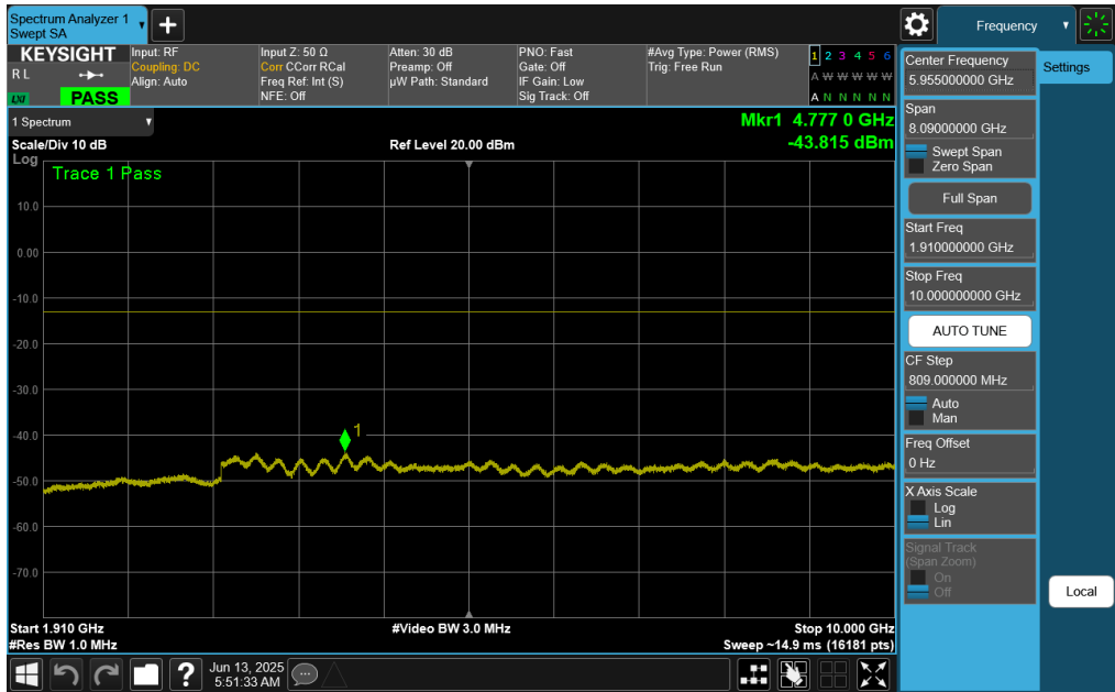
Plot 7-85. Conducted Spurious Plot (WCDMA Ch. 9262)
