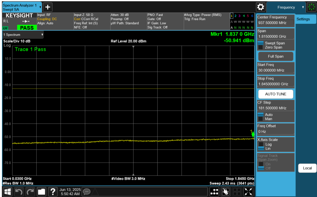
Plot 7-84. Conducted Spurious Plot (WCDMA Ch. 9262)
