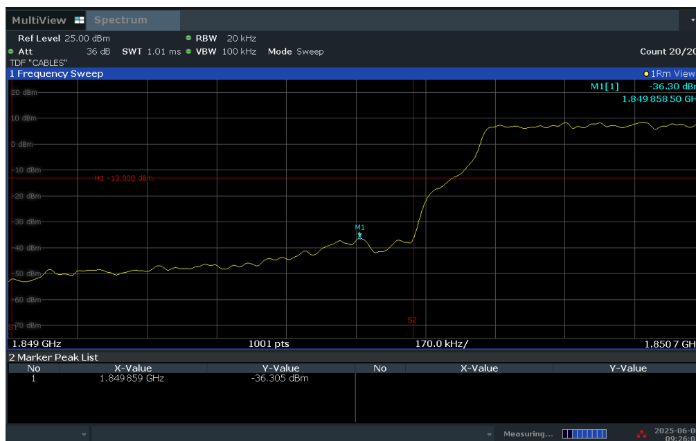
lot 7-93. Lower Band Edge Plot (LTE Band 25 – 1.4MHz QPSK – Full RB Configuration)
