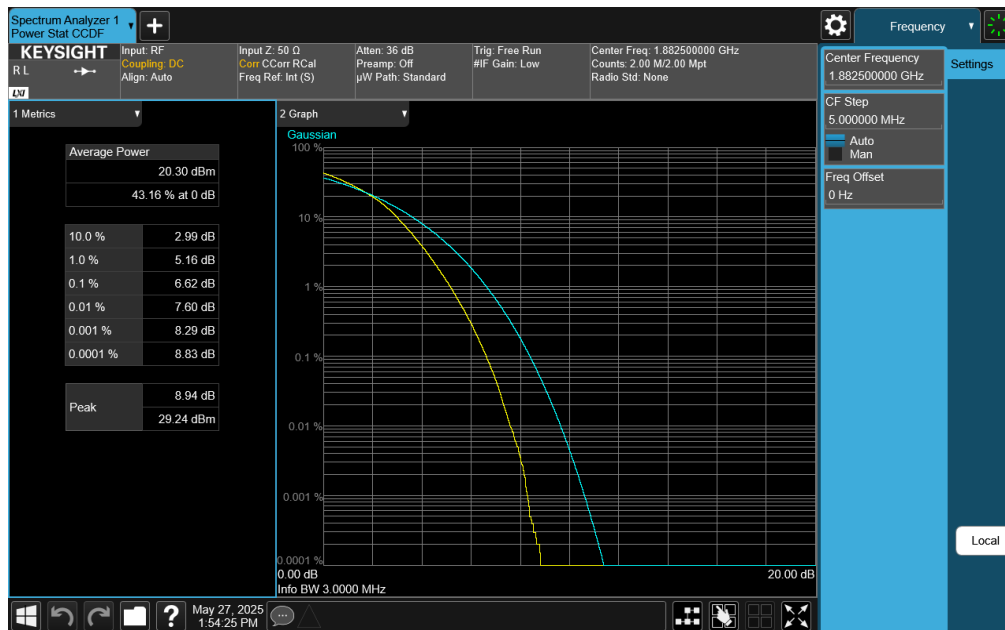
Plot 7-216. PAR Plot (LTE Band 25 - 3MHz 256-QAM - Full RB Configuration)
