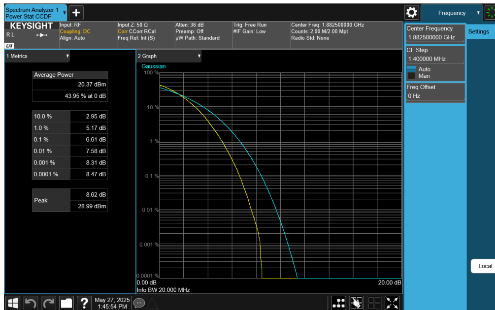
Plot 7-232. PAR Plot (LTE Band 25 - 20MHz 256-QAM - Full RB Configuration)
