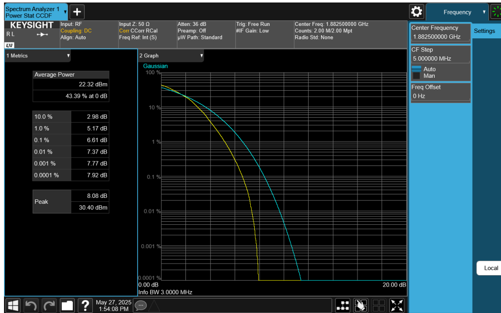
Plot 7-215. PAR Plot (LTE Band 25 - 3MHz 64-QAM - Full RB Configuration)
