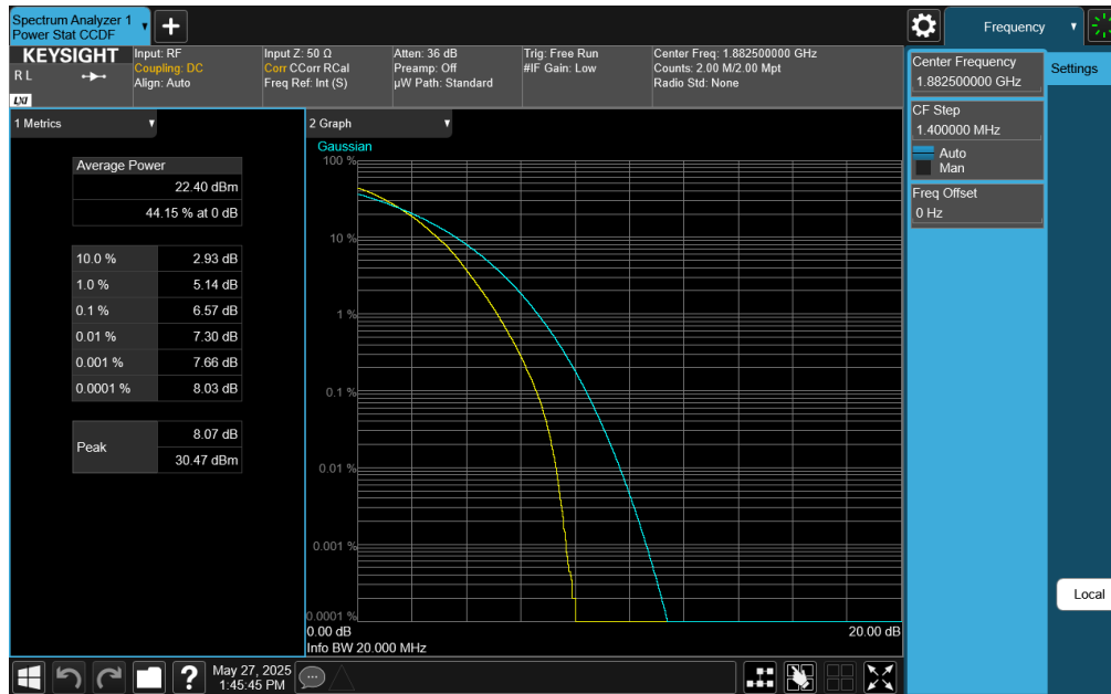
Plot 7-231. PAR Plot (LTE Band 25 - 20MHz 64-QAM - Full RB Configuration)
