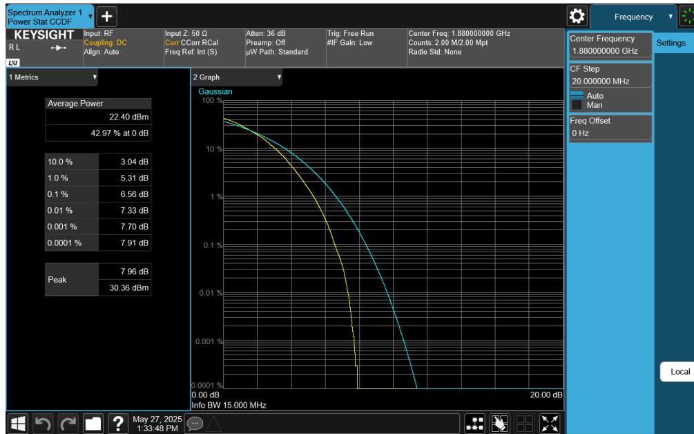
Plot 7-251. PAR Plot (LTE Band 2 - 15MHz 64-QAM - Full RB Configuration)
