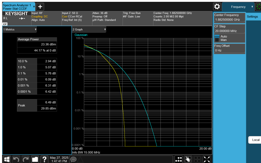
Plot 7-226. PAR Plot (LTE Band 25 - 15MHz 16-QAM - Full RB Configuration)
