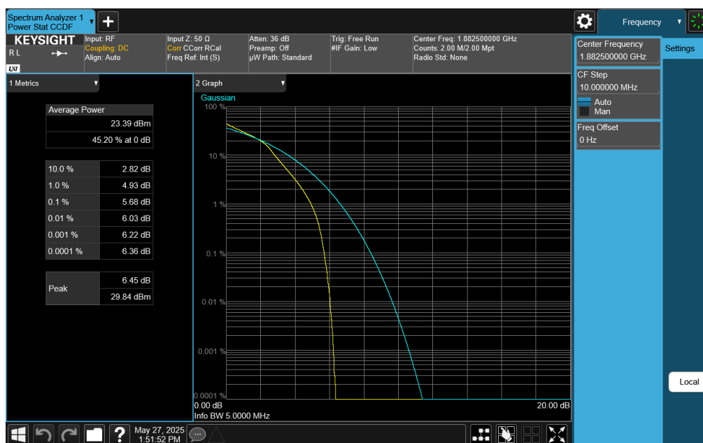
Plot 7-218. PAR Plot (LTE Band 25 - 5MHz 16-QAM - Full RB Configuration)
