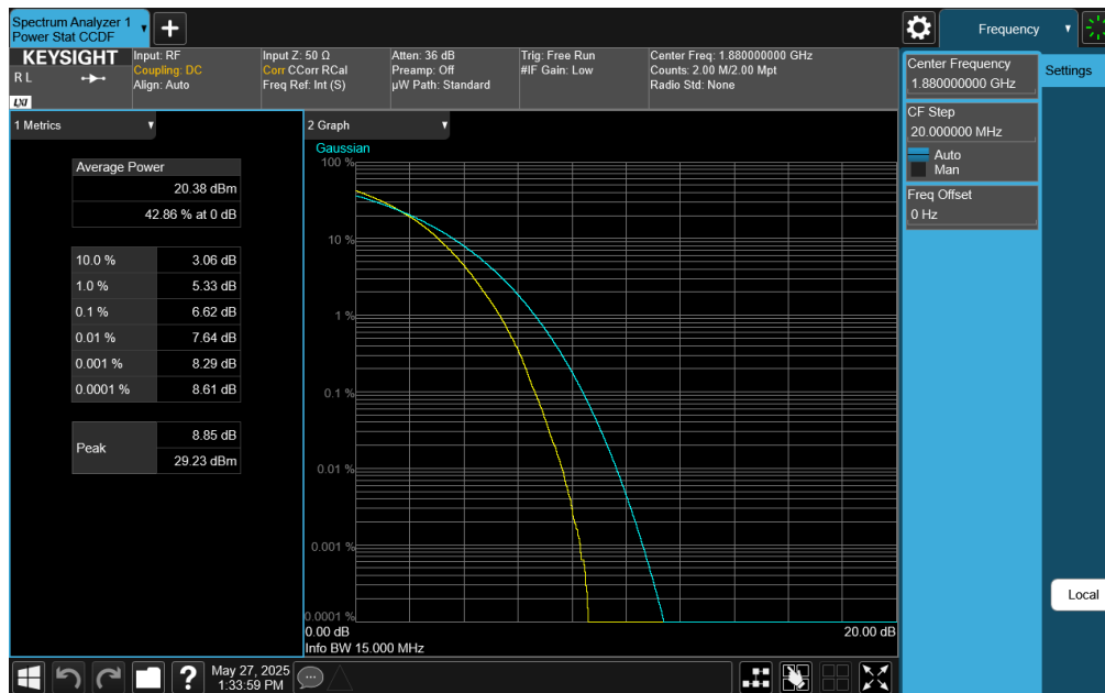
Plot 7-252. PAR Plot (LTE Band 2 - 15MHz 256-QAM - Full RB Configuration)
