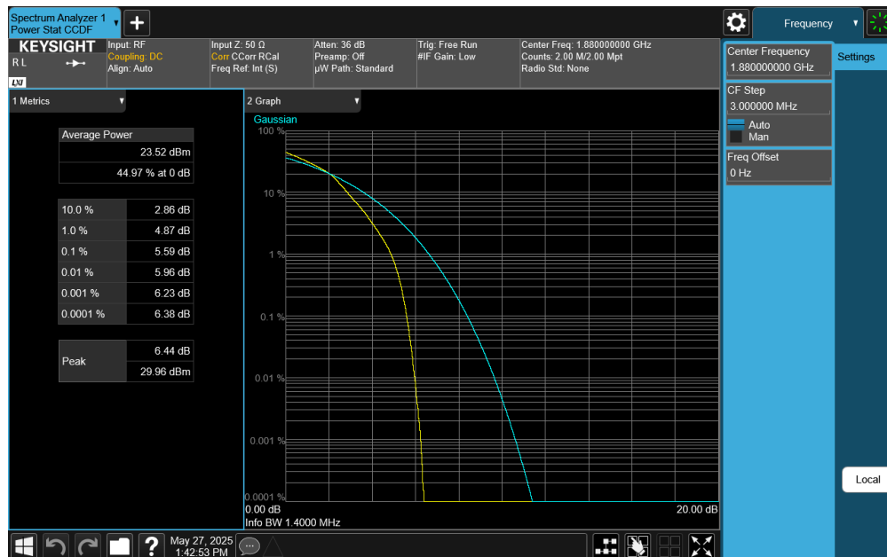
Plot 7-234. PAR Plot (LTE Band 2 - 1.4MHz 16-QAM - Full RB Configuration)
