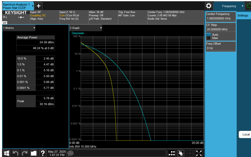
Plot 7-225. PAR Plot (LTE Band 25 - 15MHz QPSK - Full RB Configuration)
