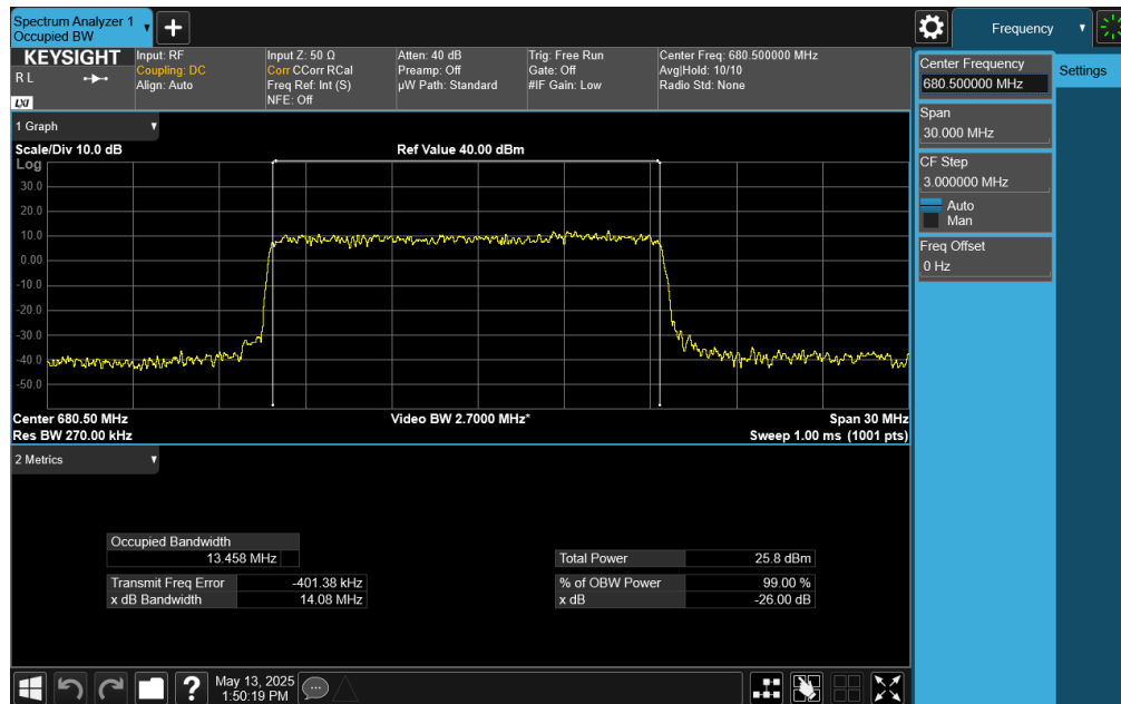
Plot 7-135. Occupied Bandwidth Plot (NR Band n71 - 15MHz DFT-s-OFDM \pi/2 BPSK - Full RB)
