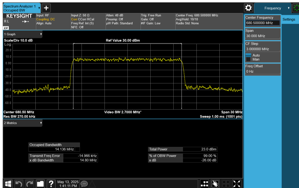
Plot 7-136. Occupied Bandwidth Plot (NR Band n71 - 15MHz CP-OFDM QPSK - Full RB)
