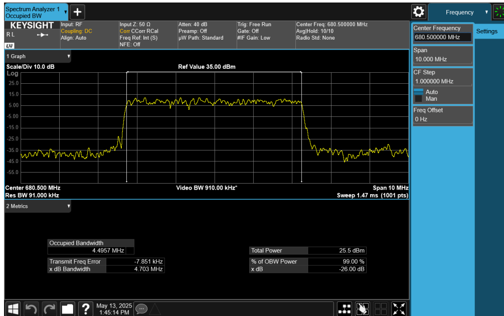
Plot 7-125. Occupied Bandwidth Plot (NR Band n71 - 5MHz DFT-s-OFDM \pi/2 BPSK - Full RB)
