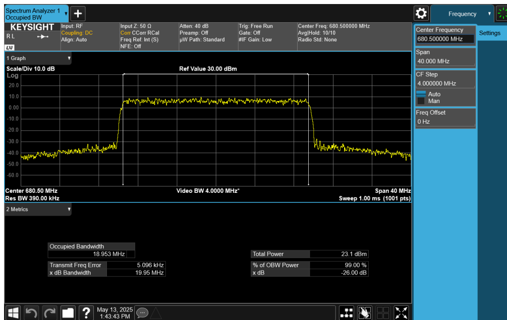
Plot 7-142. Occupied Bandwidth Plot (NR Band n71 - 20MHz CP-OFDM 16-QAM - Full RB)
