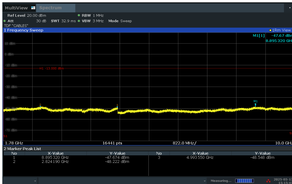
Plot 7-162. Conducted Spurious Plot (LTE Band 66/4 - 20MHz QPSK - RB Size 1, RB Offset 0 - Low Channel)
