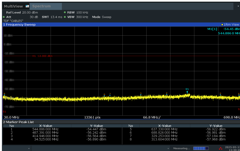
Plot 7-182. Conducted Spurious Plot (LTE Band 12/17 - 10MHz QPSK - RB Size 1, RB Offset 0 - Mid Channel)
