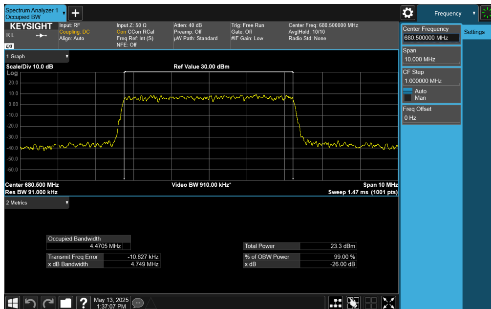
Plot 7-126. Occupied Bandwidth Plot (NR Band n71 - 5MHz CP-OFDM QPSK - Full RB)
