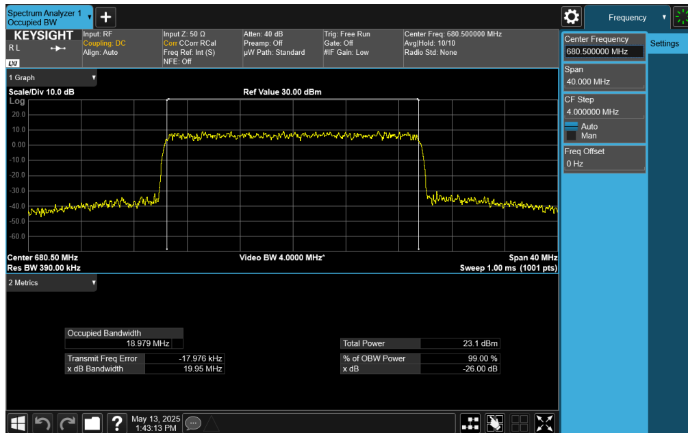
Plot 7-141. Occupied Bandwidth Plot (NR Band n71 - 20MHz CP-OFDM QPSK - Full RB)
