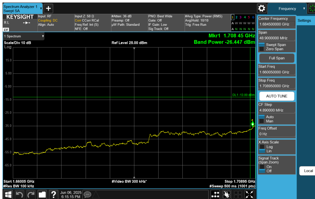
Plot 7-334. Lower Extended Band Edge Plot (NR Band n66 – 25.0MHz DFT-s-OFDM QPSK - Full RB)
