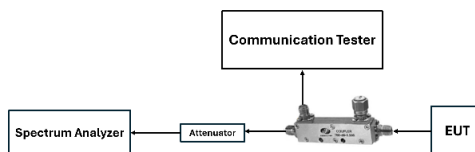
Figure 7-7. LTE Test Instrument & Measurement Setup
