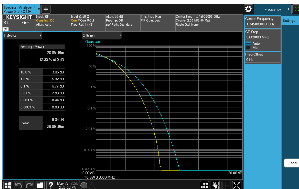
Plot 7-390. PAR Plot (LTE Band 66 - 3MHz 256-QAM - Full RB)
