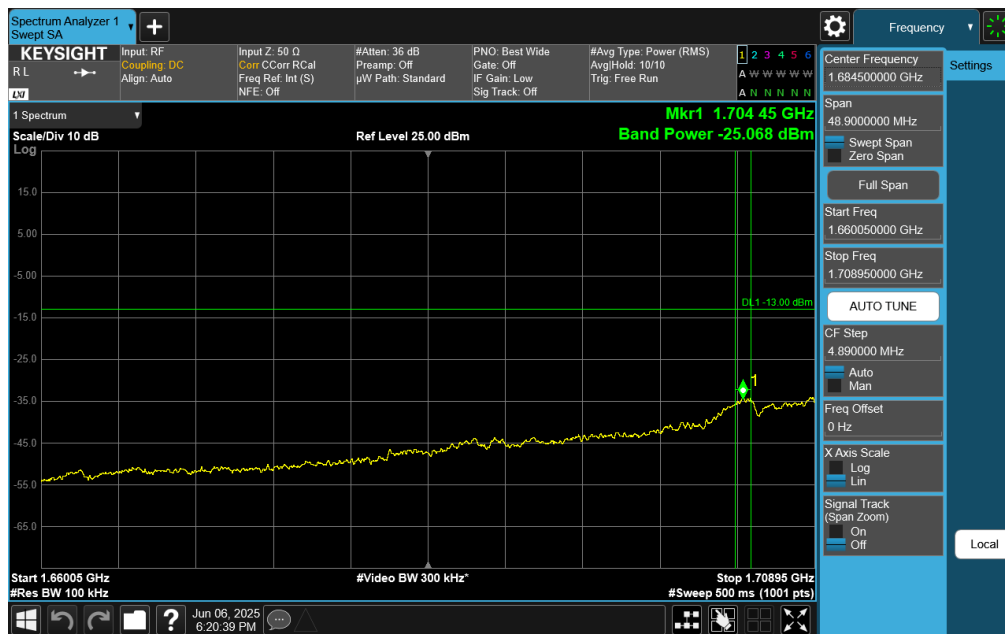
Plot 7-338. Lower Extended Band Edge Plot (NR Band n66 – 30.0MHz DFT-s-OFDM QPSK - Full RB)
