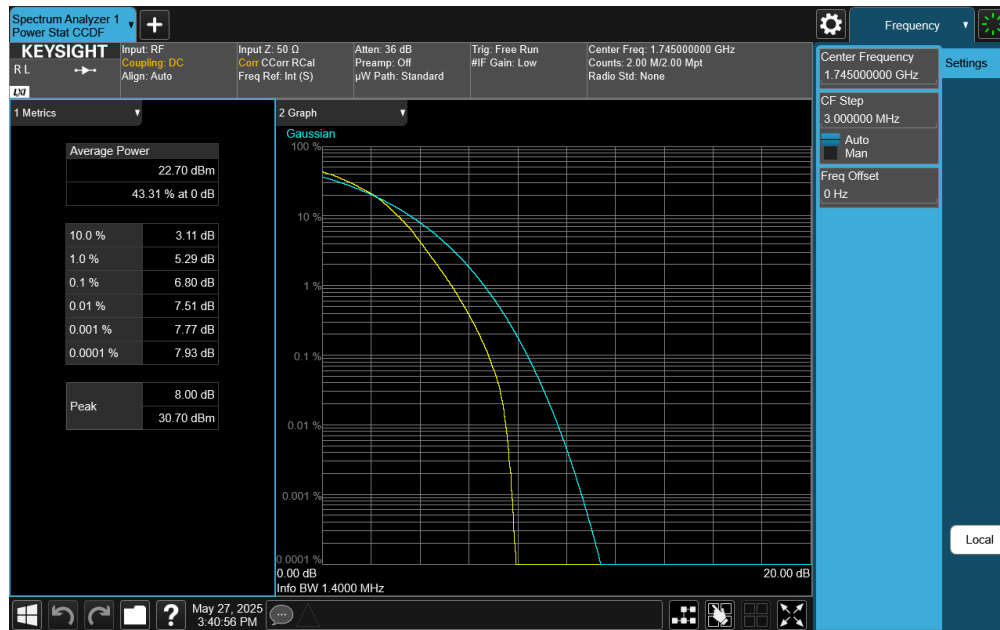
Plot 7-385. PAR Plot (LTE Band 66 - 1.4MHz 64-QAM - Full RB)
