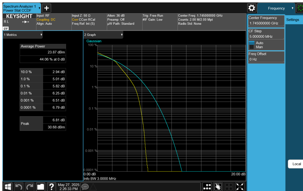
Plot 7-388. PAR Plot (LTE Band 66 - 3MHz 16-QAM - Full RB)
