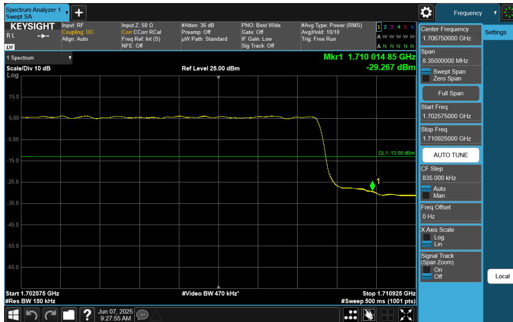
Plot 7-363. High Dand Edge Plot (NR Band n70 – 15.0MHz DFT-s-OFDM QPSK - Full RB)
