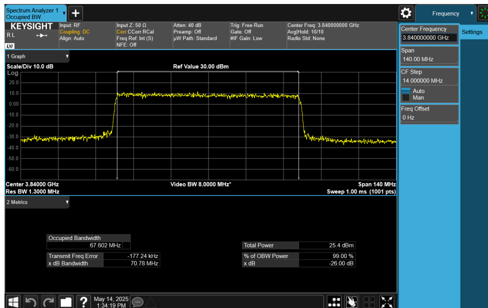
Plot 7-102. Occupied Bandwidth Plot (NR Band n77 C-Band - 70MHz CP-OFDM QPSK - Full RB)
