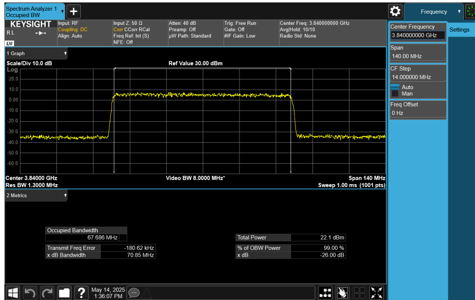
Plot 7-105. Occupied Bandwidth Plot (NR Band n77 C-Band - 70MHz CP-OFDM 256-QAM - Full RB)
