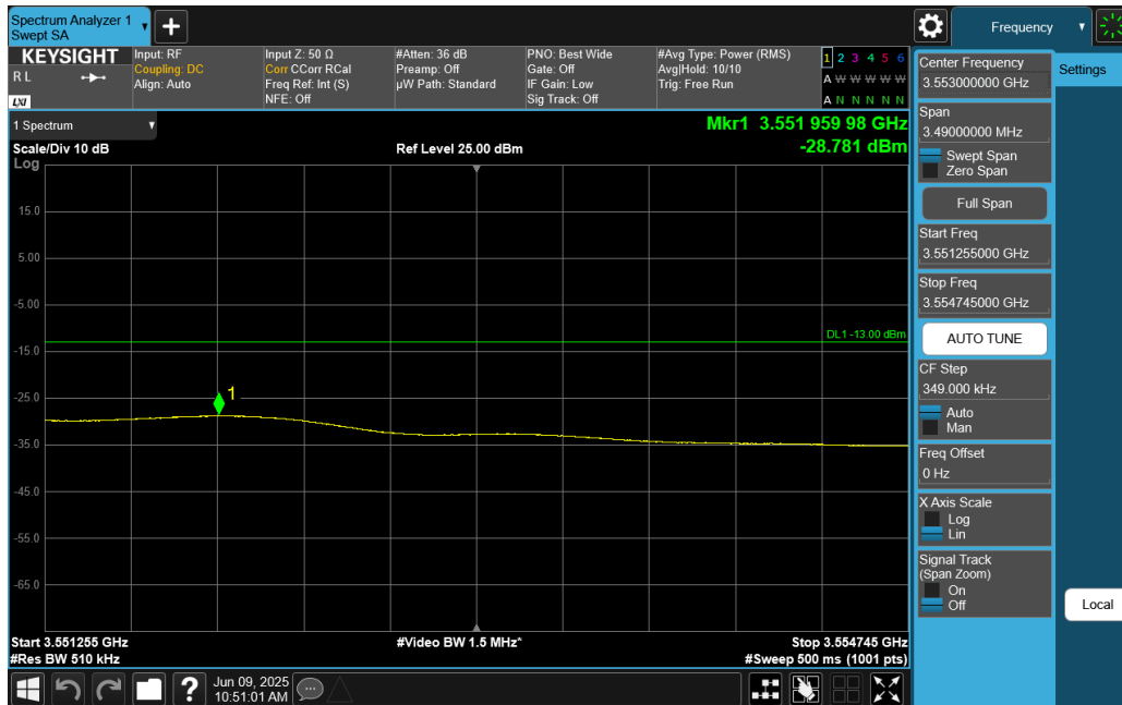
Plot 7-143. Extended Upper Band Edge Plot (NR Band n77 DoD-Band - 10MHz DFT-s-OFDM QPSK – Full RB)
