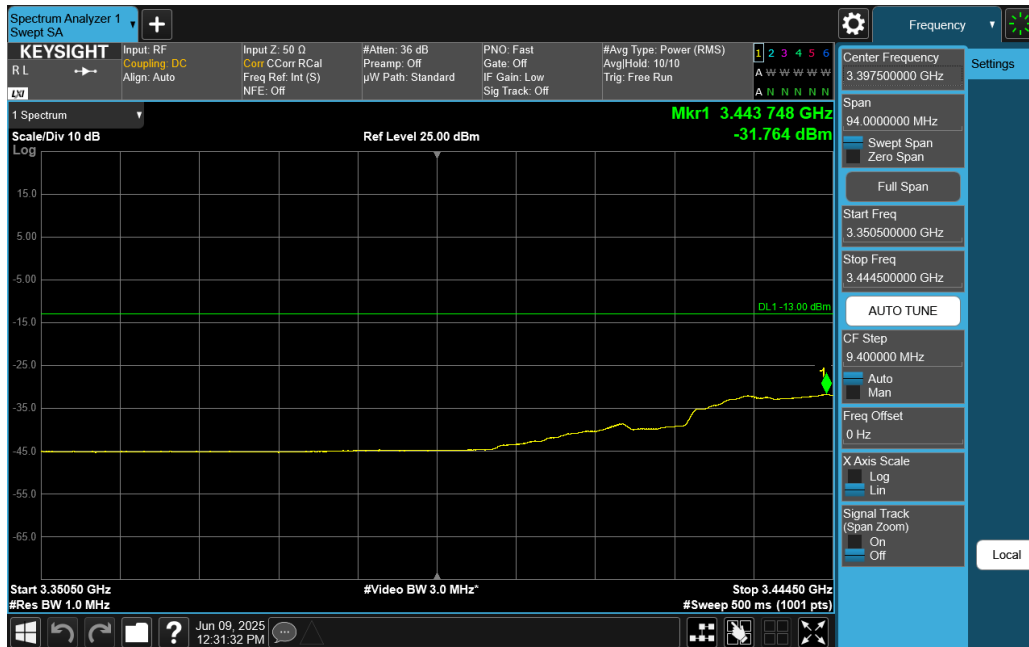
Plot 7-157. Lower Band Edge Plot (NR Band n77 DoD-Band - 25MHz DFT-s-OFDM QPSK – Full RB)
