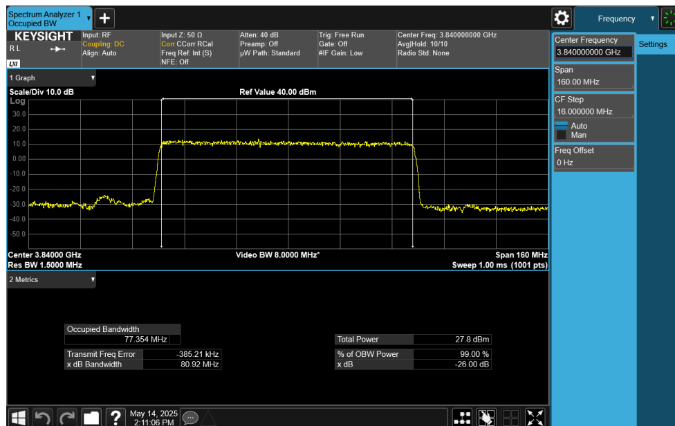
Plot 7-106. Occupied Bandwidth Plot (NR Band n77 C-Band - 80MHz DFT-s-OFDM \pi/2 BPSK - Full RB)
