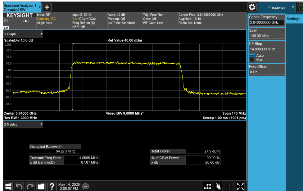
Plot 7-101. Occupied Bandwidth Plot (NR Band n77 C-Band - 70MHz DFT-s-OFDM \pi/2 BPSK - Full RB)
