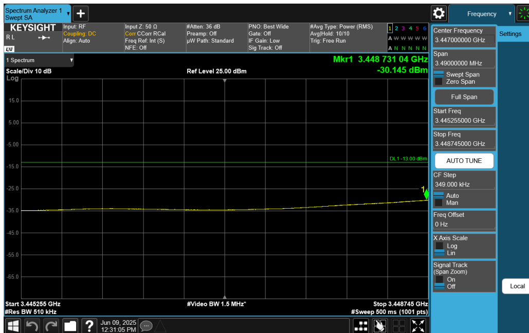
Plot 7-158. Lower Band Edge Plot (NR Band n77 DoD-Band - 25MHz DFT-s-OFDM QPSK – Full RB)
