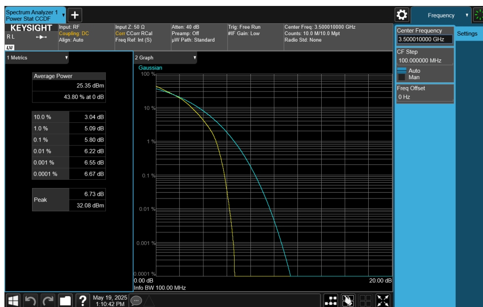
Plot 7-340. PAR Plot (NR Band n77 DoD-Band - 100MHz DFT-s-OFDM 16-QAM - Full RB)
