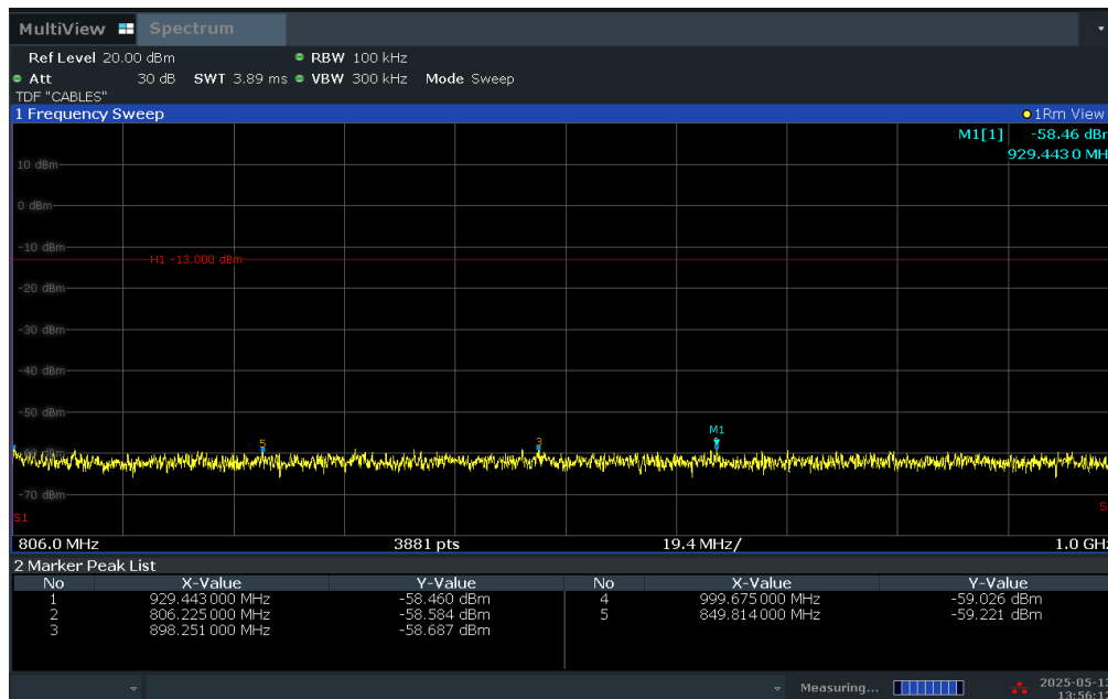
Plot 7-61. Conducted Spurious Plot (LTE Band 14 - 5MHz QPSK - RB Size 1, RB Offset 0 - High Channel)
