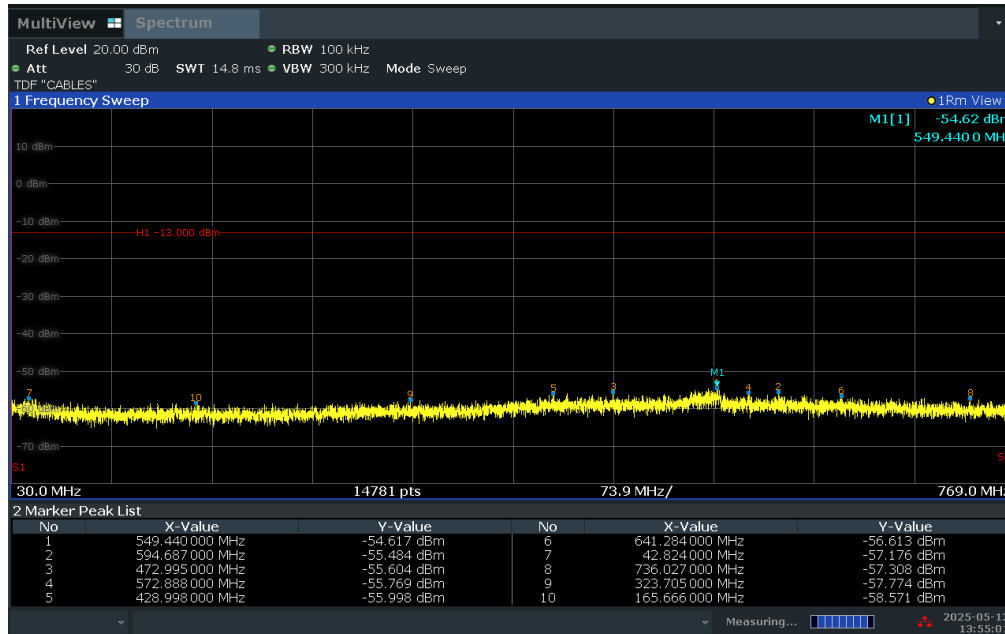
Plot 7-60. Conducted Spurious Plot (LTE Band 14 - 5MHz QPSK - RB Size 1, RB Offset 0 - High Channel)
