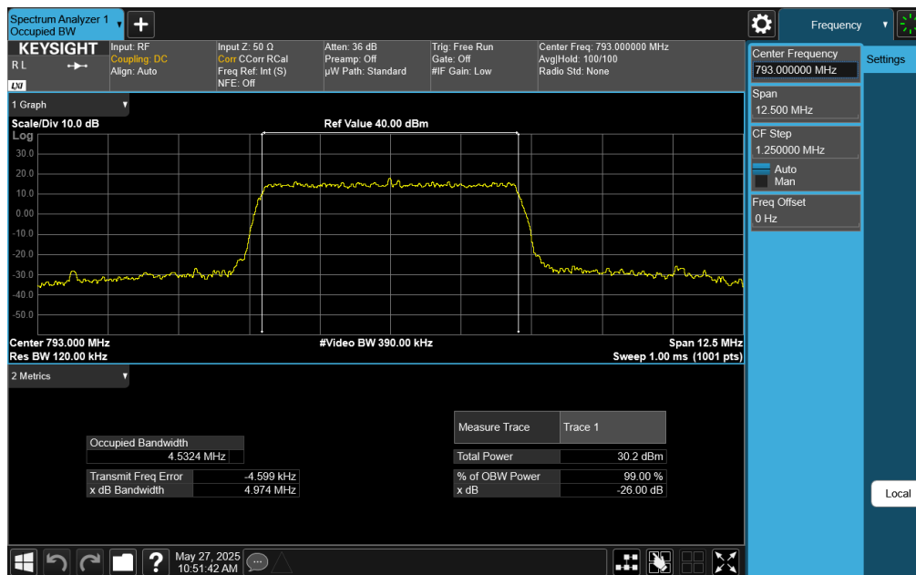
Plot 7-20. Occupied Bandwidth Plot (LTE Band 14 - 5MHz 256-QAM - Full RB)
