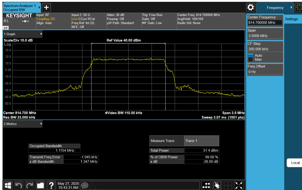
Plot 7-3. Occupied Bandwidth Plot (LTE Band 26 - 1.4MHz 64-QAM - Full RB)
