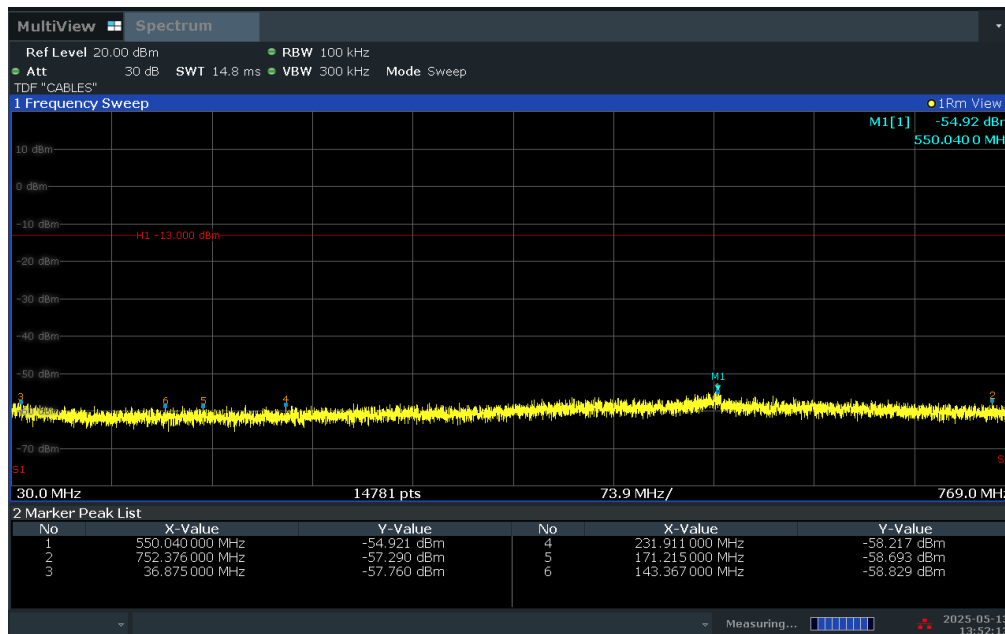
Plot 7-57. Conducted Spurious Plot (LTE Band 14 - 10MHz QPSK - RB Size 1, RB Offset 0 - Mid Channel)
