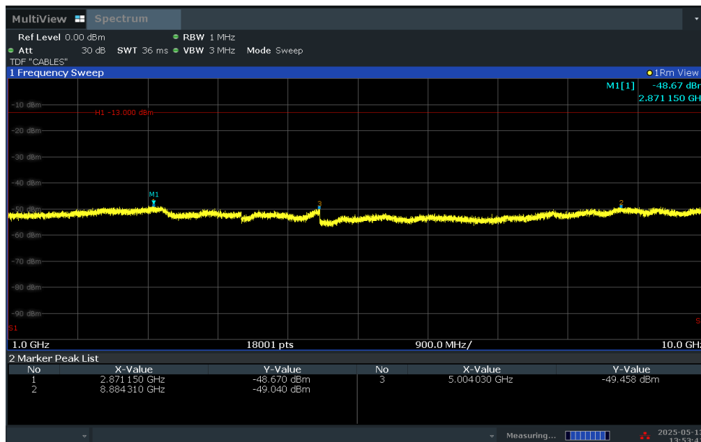
Plot 7-59. Conducted Spurious Plot (LTE Band 14 - 10MHz QPSK - RB Size 1, RB Offset 0 - Mid Channel)
