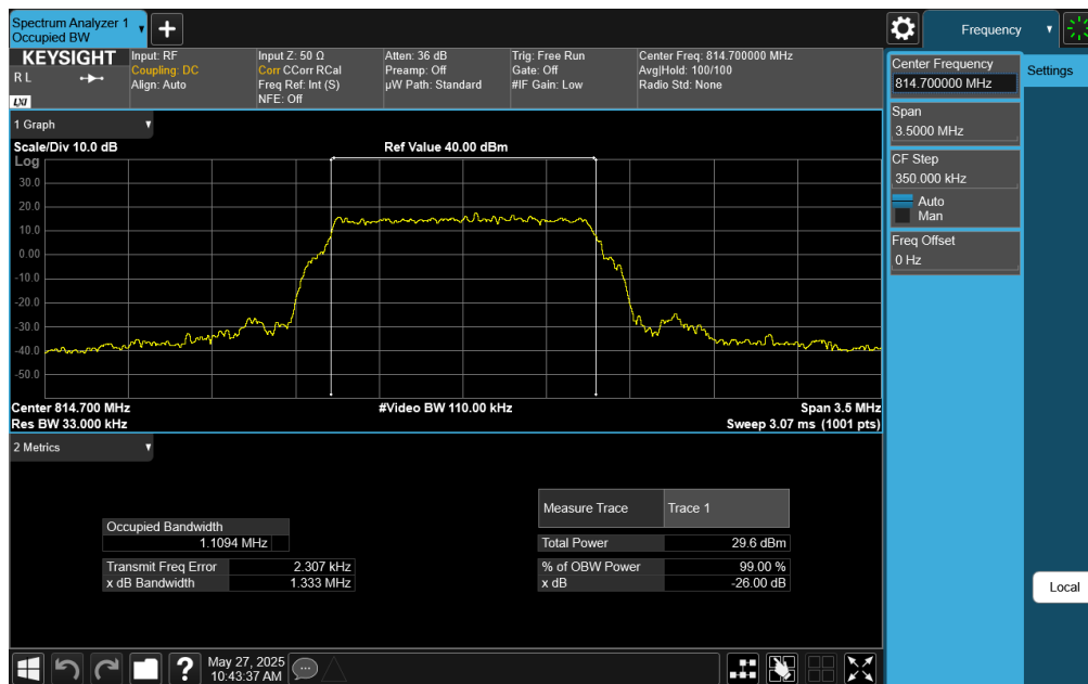
Plot 7-4. Occupied Bandwidth Plot (LTE Band 26 - 1.4MHz 256-QAM - Full RB)
