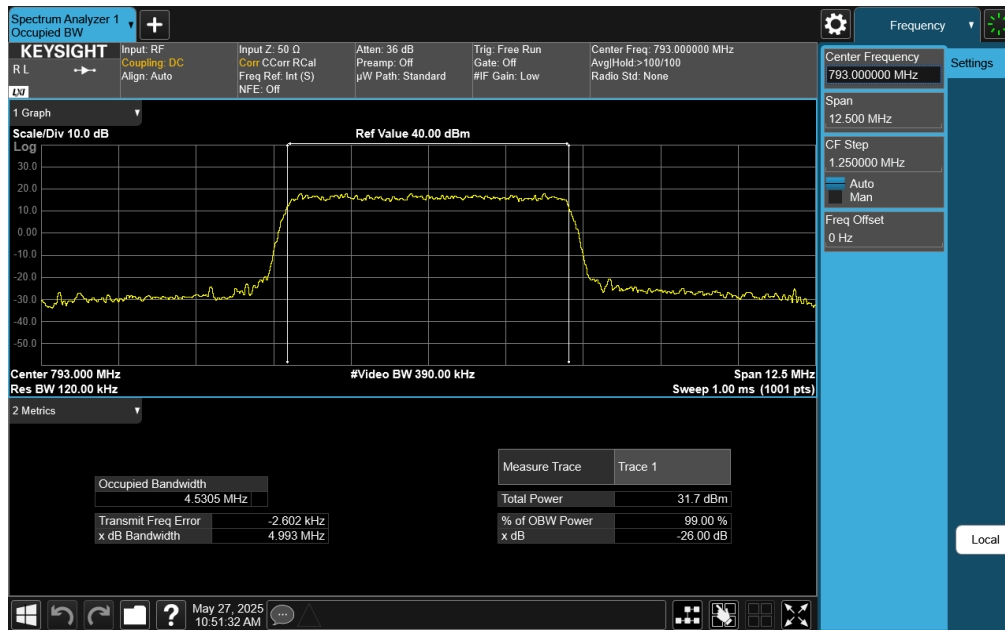
Plot 7-19. Occupied Bandwidth Plot (LTE Band 14 - 5MHz 64-QAM - Full RB)
