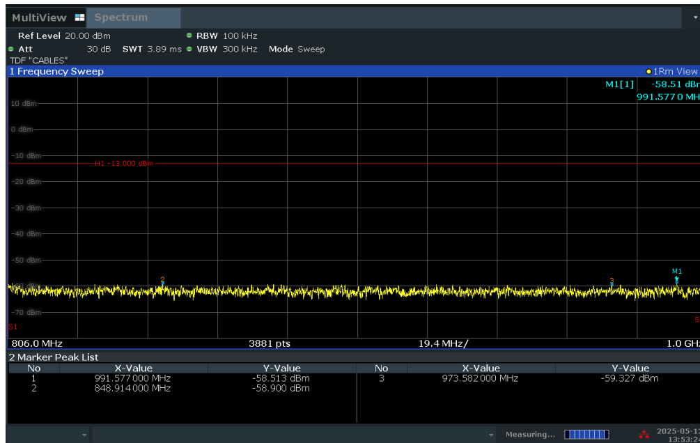
Plot 7-58. Conducted Spurious Plot (LTE Band 14 - 10MHz QPSK - RB Size 1, RB Offset 0 - Mid Channel)
