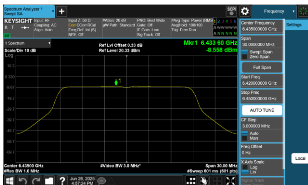
Plot 7-69 PSD Antenna 4a (20MHz BW 802.11a - Ch.97)
