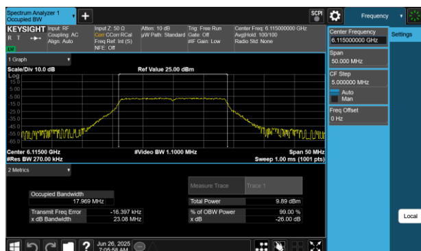
Plot 7-33 26dB BW & 99% OBW Antenna 2a (20MHz BW 802.11a - Ch.33)
