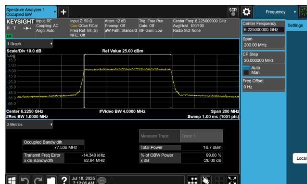
Plot 7-35 26dB BW & 99% OBW Antenna 2a (80MHz BW 802.11be(SU) - Ch.55)
