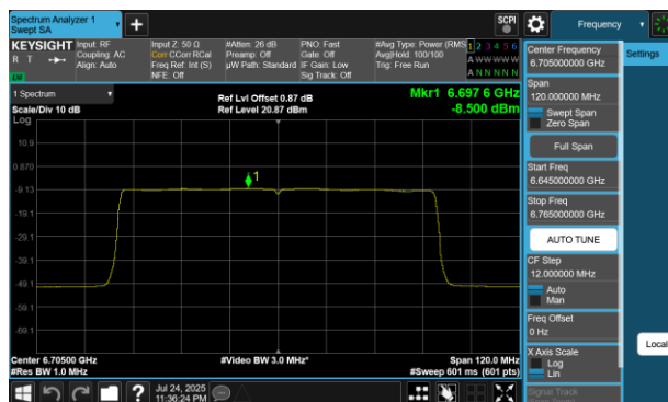
Plot 7-59 PSD Antenna WF5B (80MHz BW 802.11be(SU) - Ch.151)
