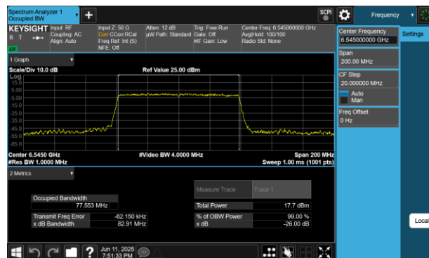
Plot 7-27 26dB BW & 99% OBW Antenna 4a (80MHz BW 802.11be(SU) - Ch.119)
