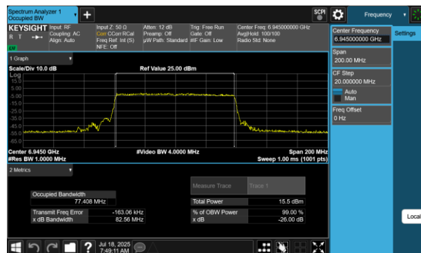
Plot 7-47 26dB BW & 99% OBW Antenna 2a (80MHz BW 802.11be(SU) - Ch.199)
