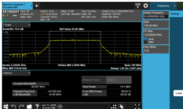
Plot 7-18 26dB BW & 99% OBW Antenna 4a (40MHz BW 802.11be(SU) - Ch.59)
