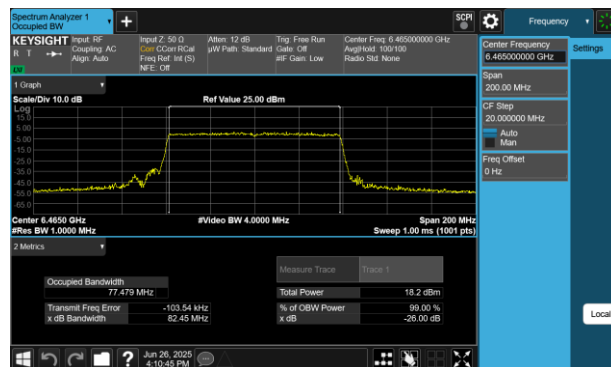
Plot 7-23 26dB BW & 99% OBW Antenna 4a (80MHz BW 802.11be(SU) - Ch.103)
