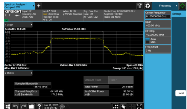
Plot 7-20 26dB BW & 99% OBW Antenna 4a (160MHz BW 802.11be(SU) - Ch.47)
