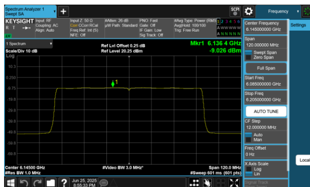
Plot 7-51 PSD Antenna WF5B (80MHz BW 802.11be(SU) - Ch.39)
