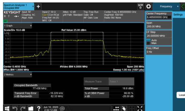
Plot 7-39 26dB BW & 99% OBW Antenna 2a (80MHz BW 802.11be(SU) - Ch.103)
