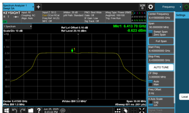
Plot 7-49 PSD Antenna WF5B (20MHz BW 802.11a - Ch.93)
