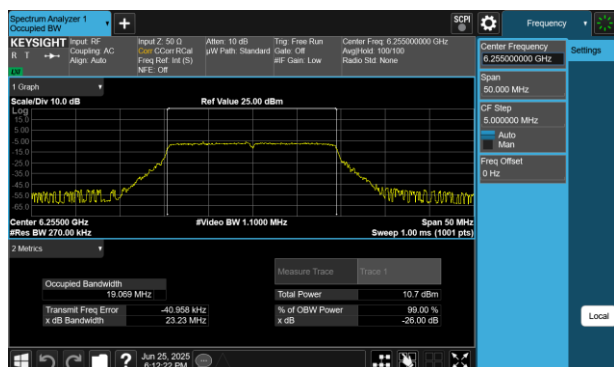
Plot 7-1 26dB BW & 99% OBW Antenna WF5B (20MHz BW 802.11be(SU) - Ch.61)
