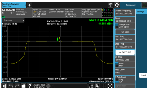
Plot 7-70 PSD Antenna 4a (40MHz BW 802.11be(SU) - Ch.99)
