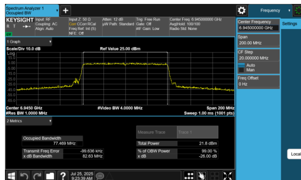
Plot 7-31 26dB BW & 99% OBW Antenna 4a (80MHz BW 802.11be(SU) - Ch.199)
