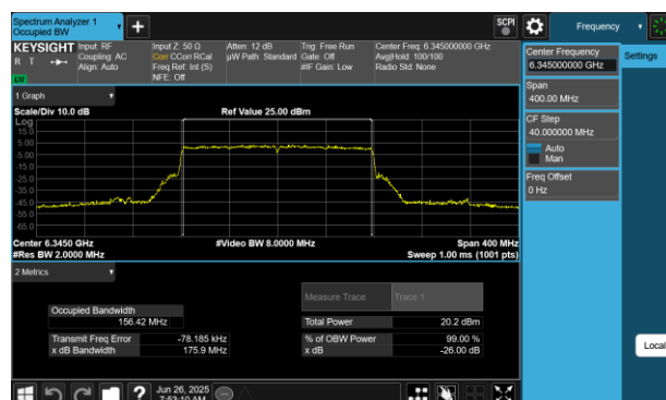
Plot 7-36 26dB BW & 99% OBW Antenna 2a (160MHz BW 802.11be(SU) - Ch.79)
