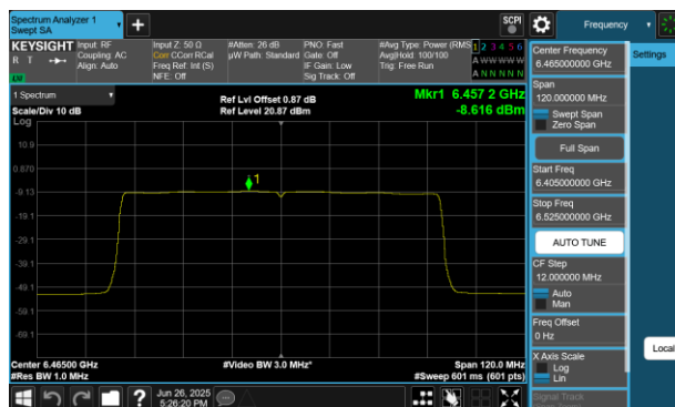
Plot 7-71 PSD Antenna 4a (80MHz BW 802.11be(SU) - Ch.103)
