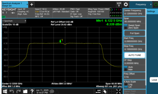
Plot 7-66 PSD Antenna 4a (40MHz BW 802.11b(SU) - Ch.35)
