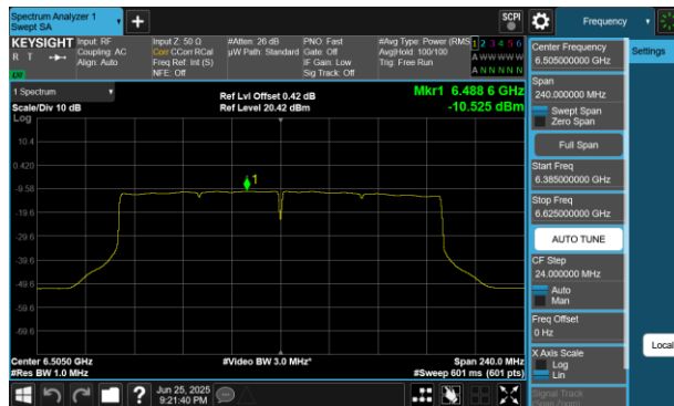
Plot 7-56 PSD Antenna WF5B (160MHz BW 802.11be(SU) - Ch.111)
