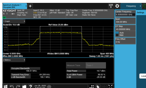
Plot 7-40 26dB BW & 99% OBW Antenna 2a (160MHz BW 802.11be(SU) - Ch.111)
