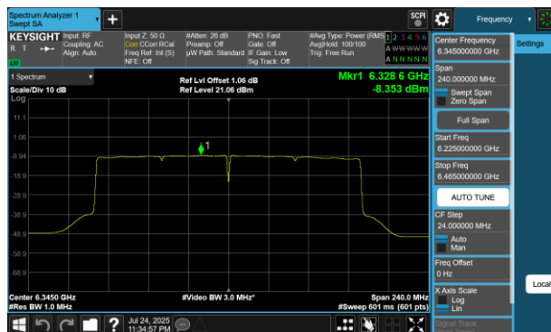
Plot 7-52 PSD Antenna WF5B (160MHz BW 802.11be(SU) - Ch.79)
