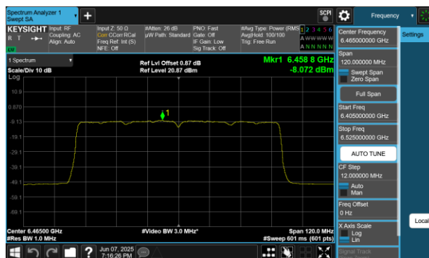
Plot 7-55 PSD Antenna WF5B (80MHz BW 802.11be(SU) - Ch.103)
