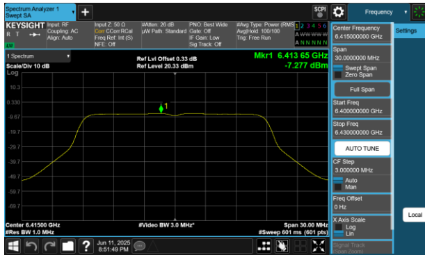
Plot 7-65 PSD Antenna 4a (20MHz BW 802.11a - Ch.93)
