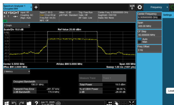
Plot 7-24 26dB BW & 99% OBW Antenna 4a (160MHz BW 802.11be(SU) - Ch.111)
