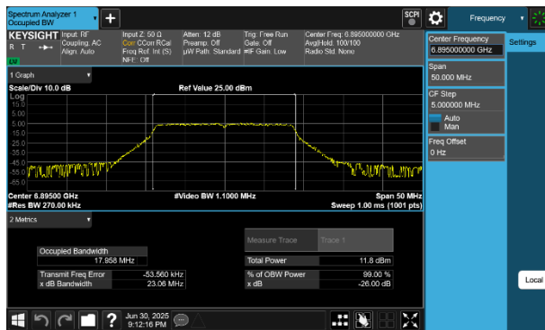
Plot 7-25 26dB BW & 99% OBW Antenna WF5B (20MHz BW 802.11a - Ch.189)
