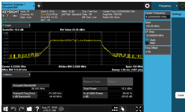
Plot 7-46 26dB BW & 99% OBW Antenna 4a (40MHz BW 802.11be(SU) - Ch.115)
