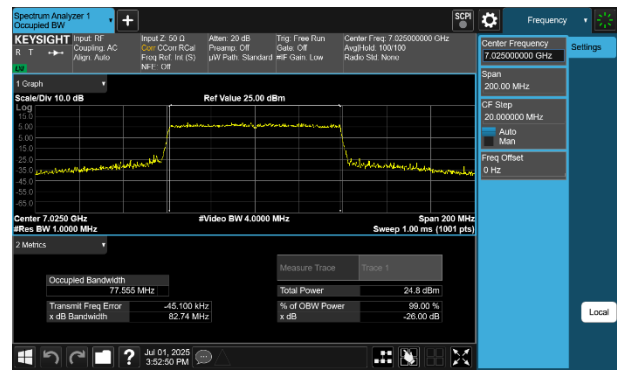
Plot 7-55 26dB BW & 99% OBW Antenna 4a (80MHz BW 802.11be(SU) - Ch.215)
