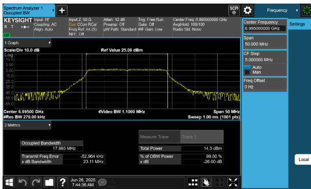
Plot 7-53 26dB BW & 99% OBW Antenna 4a (20MHz BW 802.11a - Ch.209)
