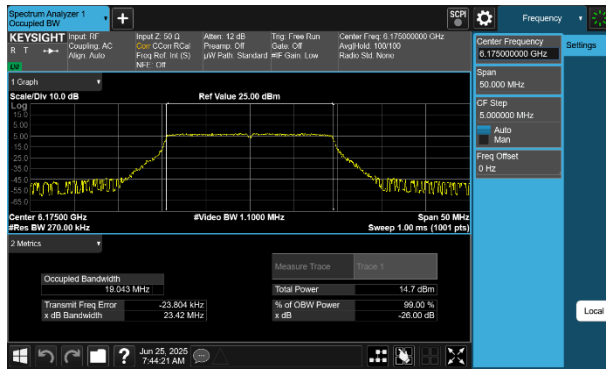
Plot 7-13 26dB BW & 99% OBW Antenna WF5B (20MHz BW 802.11be(SU) - Ch.45)
