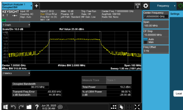
Plot 7-54 26dB BW & 99% OBW Antenna 4a (40MHz BW 802.11be(SU) - Ch.211)
