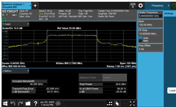
Plot 7-10 26dB BW & 99% OBW Antenna WF5B (40MHz BW 802.11be(SU) - Ch.179)
