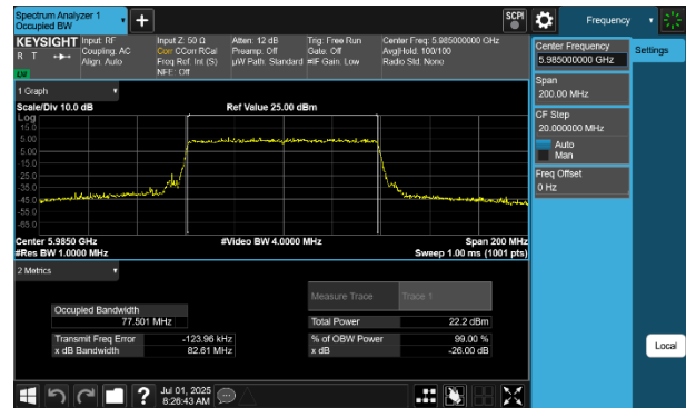
Plot 7-71 26dB BW & 99% OBW Antenna 2a (80MHz BW 802.11be(SU) - Ch.7)
