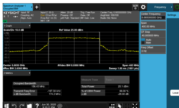
Plot 7-24 26dB BW & 99% OBW Antenna WF5B (160MHz BW 802.11be(SU) - Ch.143)
