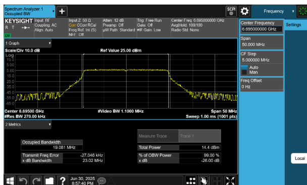
Plot 7-21 26dB BW & 99% OBW Antenna WF5B (20MHz BW 802.11be(SU) - Ch.149)
