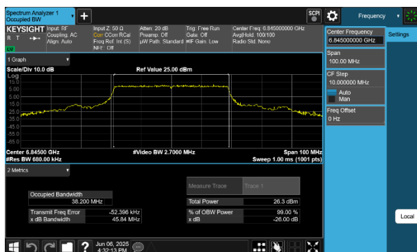
Plot 7-66 26dB BW & 99% OBW Antenna 2a (40MHz BW 802.11be(SU) - Ch.179)
