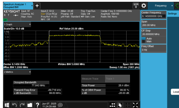
Plot 7-31 26dB BW & 99% OBW Antenna 4a (80MHz BW 802.11be(SU) - Ch.39)
