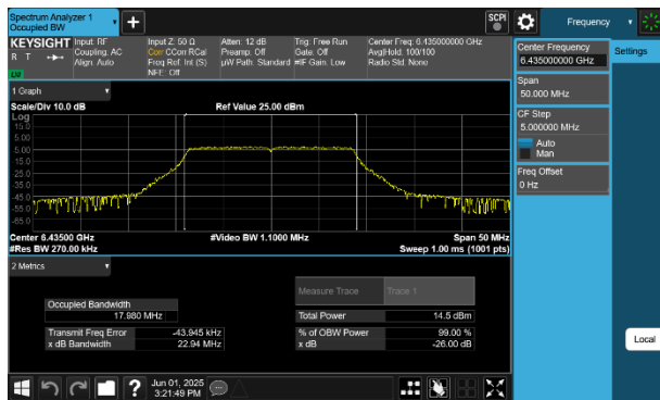
Plot 7-73 26dB BW & 99% OBW Antenna 2a (20MHz BW 802.11a - Ch.97)
