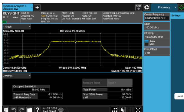
Plot 7-22 26dB BW & 99% OBW Antenna WF5B (40MHz BW 802.11be(SU) - Ch.179)
