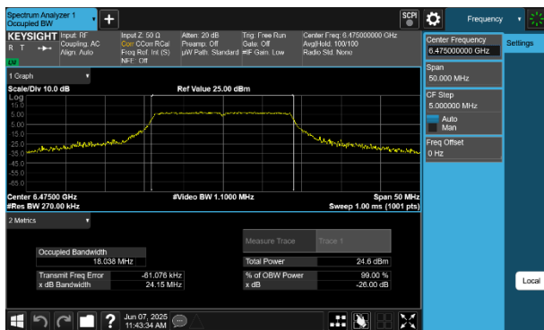
Plot 7-33 26dB BW & 99% OBW Antenna 4a (20MHz BW 802.11a - Ch.105)
