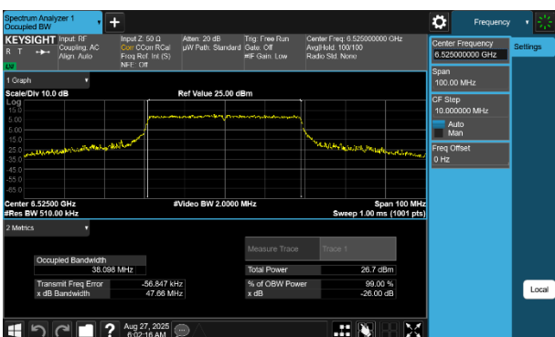
Plot 7-34 26dB BW & 99% OBW Antenna 4a (40MHz BW 802.11be(SU) - Ch.115)
