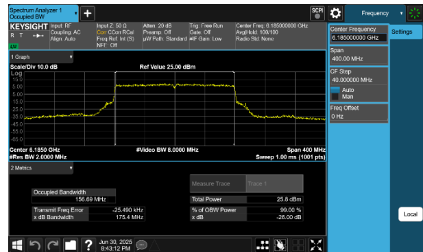
Plot 7-16 26dB BW & 99% OBW Antenna WF5B (160MHz BW 802.11be(SU) - Ch.47)
