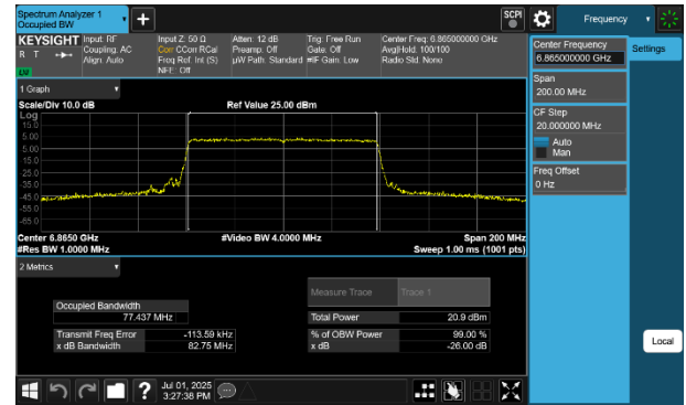
Plot 7-51 26dB BW & 99% OBW Antenna 4a (80MHz BW 802.11be(SU) - Ch.183)
