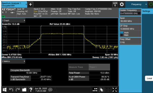
Plot 7-45 26dB BW & 99% OBW Antenna 4a (20MHz BW 802.11be(SU) - Ch.105)
