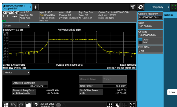
Plot 7-42 26dB BW & 99% OBW Antenna 4a (40MHz BW 802.11be(SU) - Ch.43)
