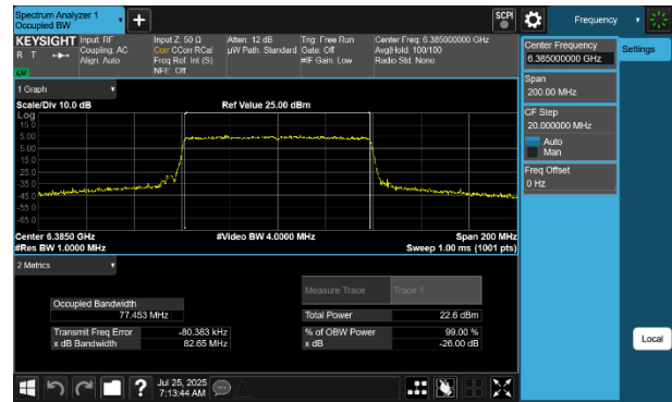
Plot 7-15 26dB BW & 99% OBW Antenna WF5B (80MHz BW 802.11be(SU) - Ch.87)
