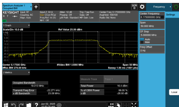
Plot 7-41 26dB BW & 99% OBW Antenna 4a (20MHz BW 802.11be(SU) - Ch.45)
