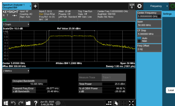
Plot 7-1 26dB BW & 99% OBW Antenna WF5B (20MHz BW 802.11a - Ch.1)
