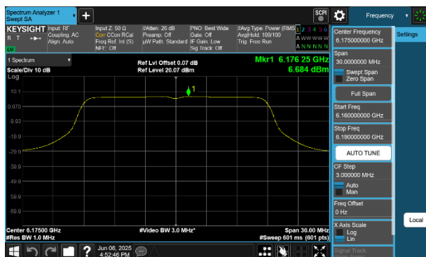
Plot 7-141 PSD Antenna 2a (20MHz BW 802.11a - Ch.45)
