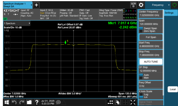
Plot 7-139 PSD Antenna 4a (80MHz BW 802.11be(SU) - Ch.215)
