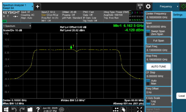
Plot 7-126 PSD Antenna 4a (40MHz BW 802.11be(SU) - Ch.43)
