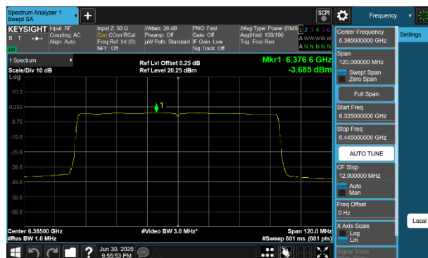
Plot 7-99 PSD Antenna WF5B (80MHz BW 802.11be(SU) - Ch.87)
