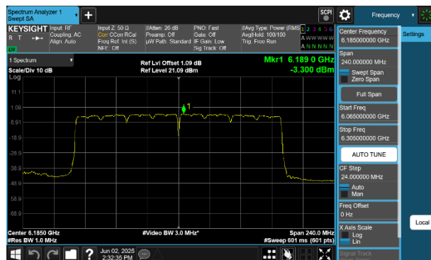
Plot 7-128 PSD Antenna 4a (160MHz BW 802.11be(SU) - Ch.47)
