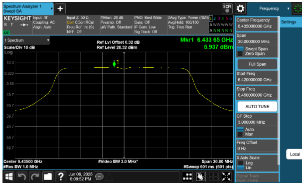
Plot 7-145 PSD Antenna 2a (20MHz BW 802.11a - Ch.97)
