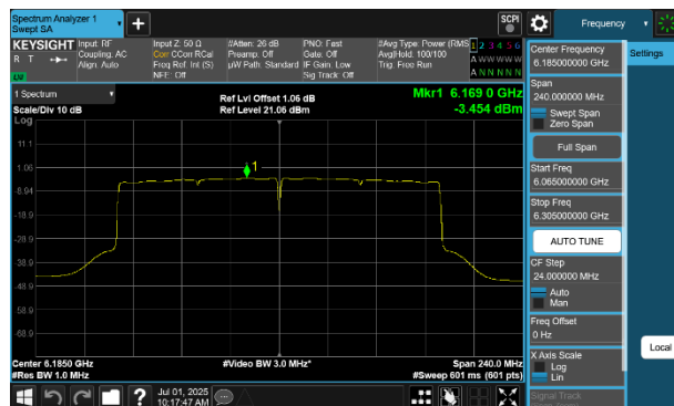
Plot 7-156 PSD Antenna 2a (160MHz BW 802.11be(SU) - Ch.47)
