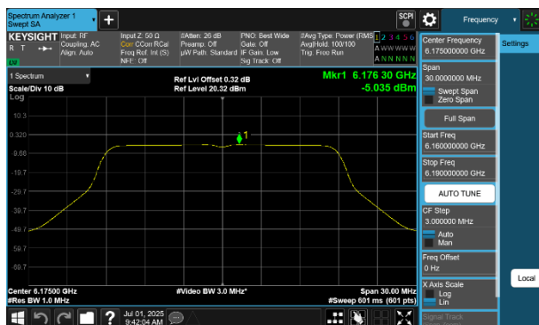
Plot 7-153 PSD Antenna 2a (20MHz BW 802.11a - Ch.45)
