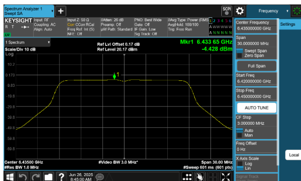
Plot 7-129 PSD Antenna 4a (20MHz BW 802.11a - Ch.97)
