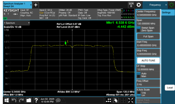
Plot 7-135 PSD Antenna 4a (80MHz BW 802.11be(SU) - Ch.119)
