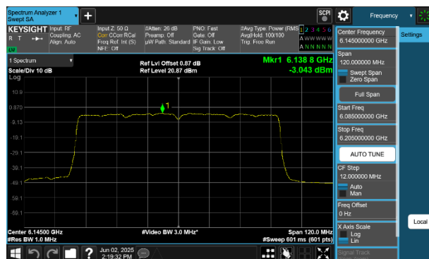
Plot 7-127 PSD Antenna 4a (80MHz BW 802.11be(SU) - Ch.39)
