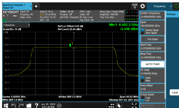
Plot 7-98 PSD Antenna WF5B (40MHz BW 802.11be(SU) - Ch.91)
