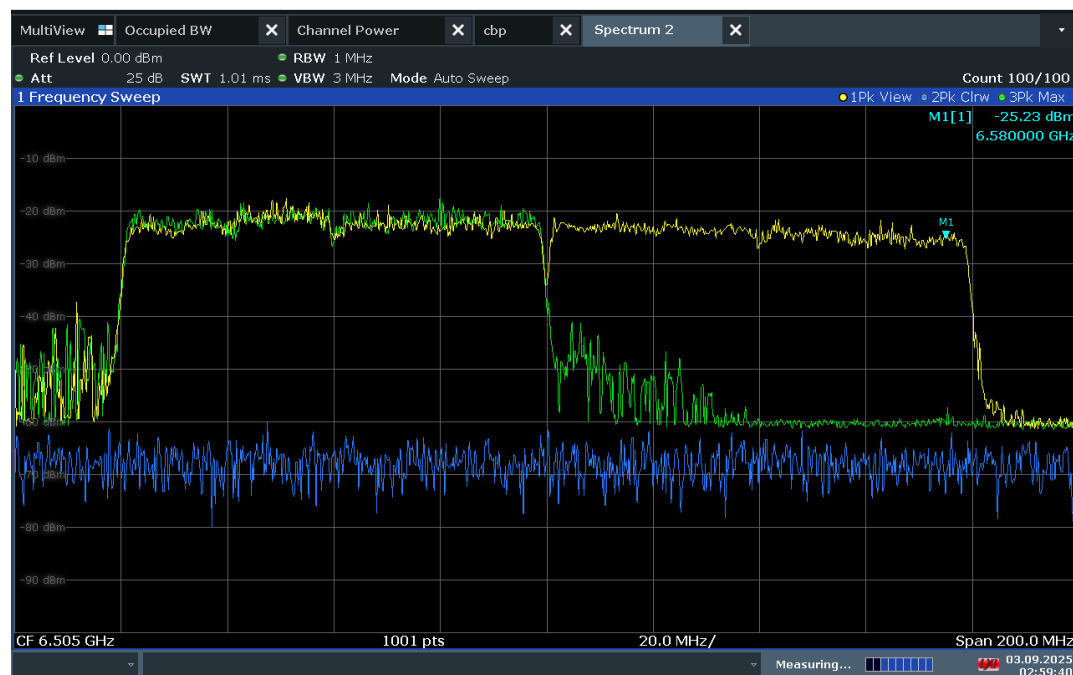
Plot 7-307. 160MHz Bandwidth, AWGN Signal Injected – 6580MHz
