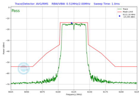
Plot 7-242 In-Band Emission Plot SDM Diversity Antenna 2a (40MHz BW 802.11be(SU) (UNII Band 5) - Ch.35)
