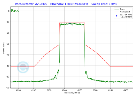
Plot 7-243 In-Band Emission Plot SDM Diversity Antenna 2a (80MHz BW 802.11be(SU) (UNII Band 5) - Ch.55)
