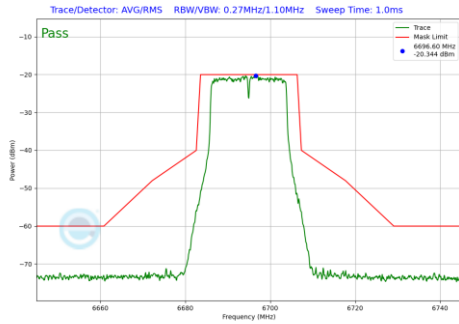
Plot 7-217 In-Band Emission Plot CDD Primary Antenna WF5B (20MHz BW 802.11a (UNII Band 7) - Ch.149)
