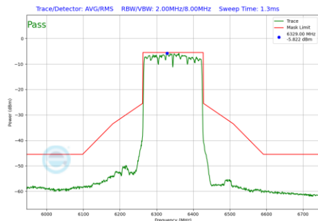
Plot 7-180 In-Band Emission Plot Antenna 4a (160MHz BW 802.11be(SU) (UNII Band 5) - Ch.79)
