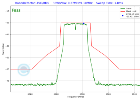
Plot 7-249 In-Band Emission Plot CDD Diversity Antenna 2a (20MHz BW 802.11a (UNII Band 7) - Ch.149)
