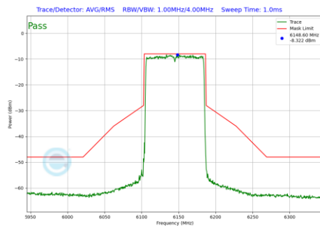
Plot 7-195 In-Band Emission Plot Antenna 2a (80MHz BW 802.11be(SU) (UNII Band 5) - Ch.39)
