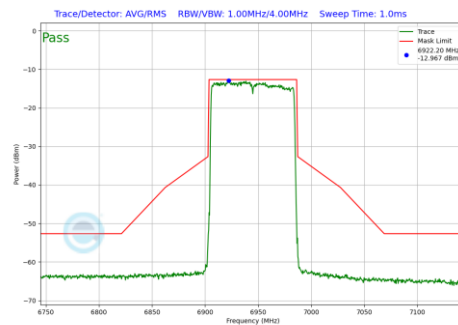
Plot 7-223 In-Band Emission Plot SDM Primary Antenna WF5B (80MHz BW 802.11be(SU) (UNII Band 8) - Ch.199)
