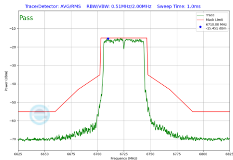
Plot 7-218 In-Band Emission Plot SDM Primary Antenna WF5B (40MHz BW 802.11be(SU) (UNII Band 7) - Ch.155)
