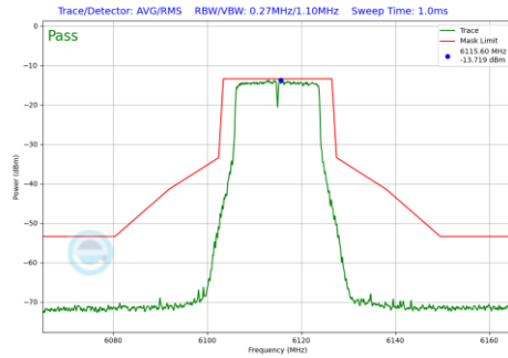
Plot 7-193 In-Band Emission Plot Antenna 2a (20MHz BW 802.11a (UNII Band 5) - Ch.33)
