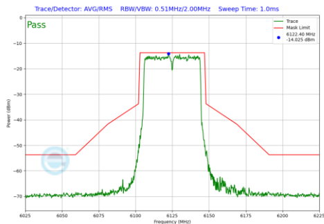
Plot 7-258 In-Band Emission Plot SDM Diversity Antenna 4a (40MHz BW 802.11be(SU) (UNII Band 5) - Ch.35)
