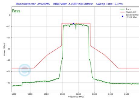
Plot 7-196 In-Band Emission Plot Antenna 2a (160MHz BW 802.11be(SU) (UNII Band 5) - Ch.47)
