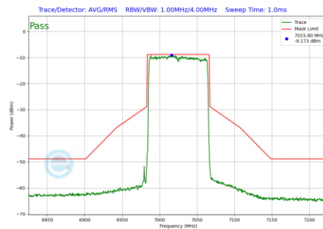
Plot 7-207 In-Band Emission Plot Antenna 2a (80MHz BW 802.11be(SU) (UNII Band 8) - Ch.215)
