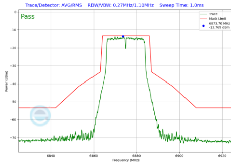
Plot 7-185 In-Band Emission Plot Antenna 4a (20MHz BW 802.11a (UNII Band 7) - Ch.185)
