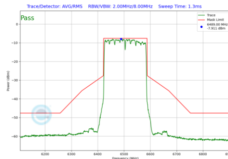
Plot 7-184 In-Band Emission Plot Antenna 4a (160MHz BW 802.11be(SU) (UNII Band 6) - Ch.111)
