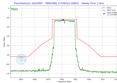
Plot 7-206 In-Band Emission Plot Antenna 2a (40MHz BW 802.11be(SU) (UNII Band 8) - Ch.211)
