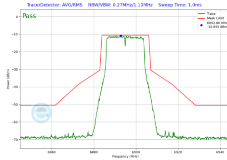
Plot 7-189 In-Band Emission Plot Antenna 4a (20MHz BW 802.11a (UNII Band 8) - Ch.189)
