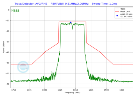
Plot 7-186 In-Band Emission Plot Antenna 4a (40MHz BW 802.11be(SU) (UNII Band 7) - Ch.179)
