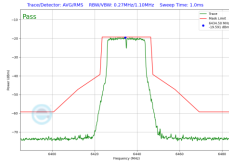
Plot 7-213 In-Band Emission Plot CDD Primary Antenna WF5B (20MHz BW 802.11a (UNII Band 6) - Ch.97)
