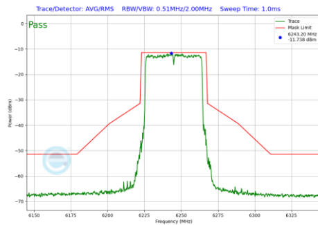
Plot 7-194 In-Band Emission Plot Antenna 2a (40MHz BW 802.11be(SU) (UNII Band 5) - Ch.59)
