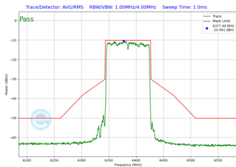
Plot 7-211 In-Band Emission Plot SDM Primary Antenna WF5B (80MHz BW 802.11be(SU) (UNII Band 5) - Ch.87)
