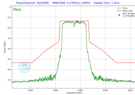
Plot 7-197 In-Band Emission Plot Antenna 2a (20MHz BW 802.11be(SU) (UNII Band 6) - Ch.105)
