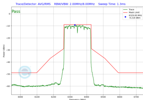
Plot 7-212 In-Band Emission Plot SDM Primary Antenna WF5B (160MHz BW 802.11be(SU) (UNII Band 5) - Ch.79)
