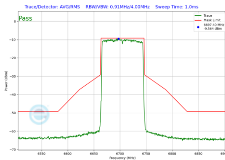
Plot 7-203 In-Band Emission Plot Antenna 2a (80MHz BW 802.11be(SU) (UNII Band 7) - Ch.151)
