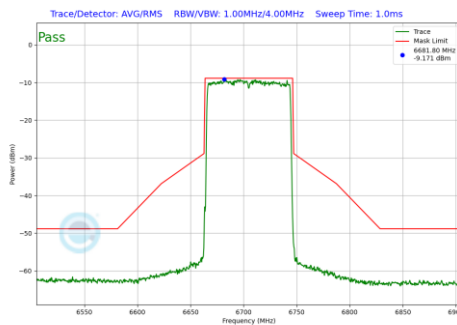
Plot 7-171 In-Band Emission Plot Antenna WF5B (80MHz BW 802.11be(SU) (UNII Band 7) - Ch.151)
