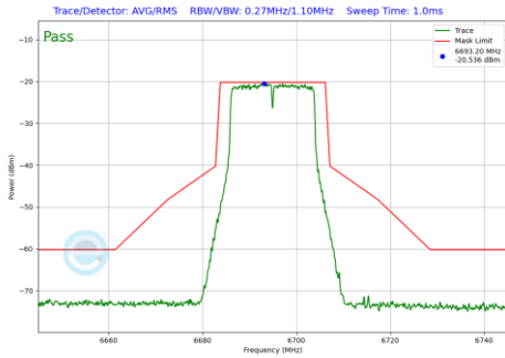
Plot 7-233 In-Band Emission Plot CDD Primary Antenna 4a (20MHz BW 802.11a (UNII Band 7) - Ch.149)
