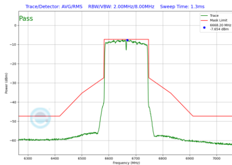
Plot 7-204 In-Band Emission Plot Antenna 2a (160MHz BW 802.11be(SU) (UNII Band 7) - Ch.143)
