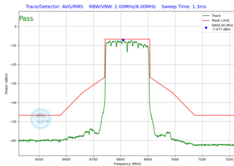
Plot 7-188 In-Band Emission Plot Antenna 4a (160MHz BW 802.11be(SU) (UNII Band 7) - Ch.175)
