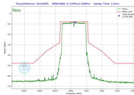
Plot 7-190 In-Band Emission Plot Antenna 4a (40MHz BW 802.11be(SU) (UNII Band 8) - Ch.211)
