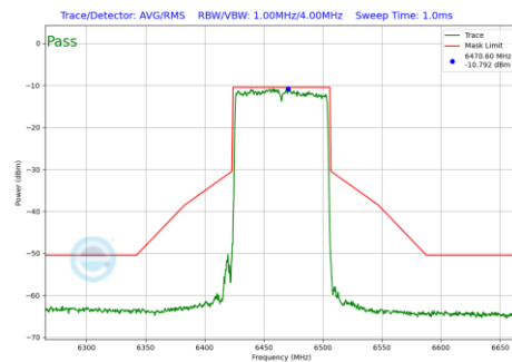
Plot 7-231 In-Band Emission Plot SDM Primary Antenna 4a (80MHz BW 802.11be(SU) (UNII Band 6) - Ch.103)
