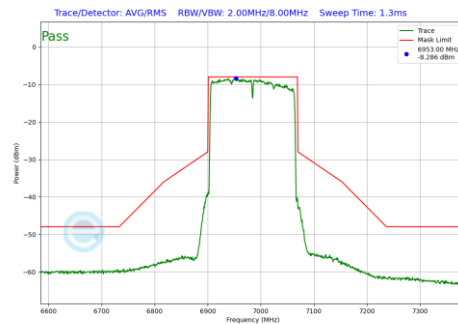
Plot 7-208 In-Band Emission Plot Antenna 2a (160MHz BW 802.11be(SU) (UNII Band 8) - Ch.207)
