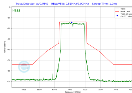
Plot 7-222 In-Band Emission Plot SDM Primary Antenna WF5B (40MHz BW 802.11be(SU) (UNII Band 8) - Ch.211)
