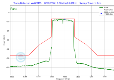
Plot 7-192 In-Band Emission Plot Antenna 4a (160MHz BW 802.11be(SU) (UNII Band 8) - Ch.207)
