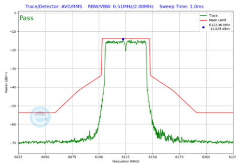
Plot 7-226 In-Band Emission Plot SDM Primary Antenna 4a (40MHz BW 802.11be(SU) (UNII Band 5) - Ch.35)
