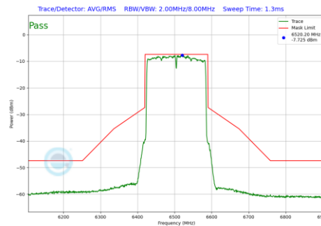
Plot 7-200 In-Band Emission Plot Antenna 2a (160MHz BW 802.11be(SU) (UNII Band 6) - Ch.111)
