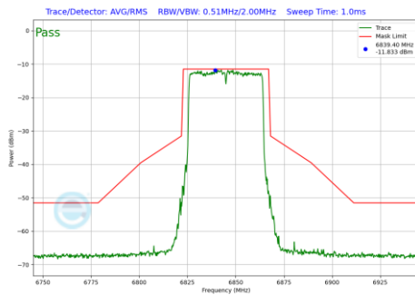
Plot 7-202 In-Band Emission Plot Antenna 2a (40MHz BW 802.11be(SU) (UNII Band 7) - Ch.179)
