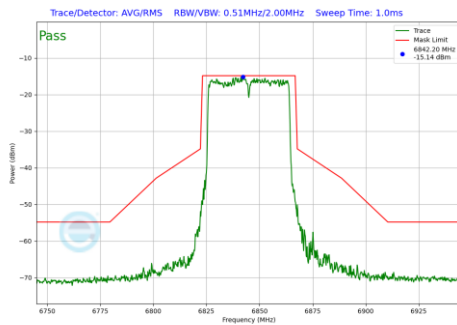
Plot 7-266 In-Band Emission Plot SDM Diversity Antenna 4a (40MHz BW 802.11be(SU) (UNII Band 7) - Ch.179)
