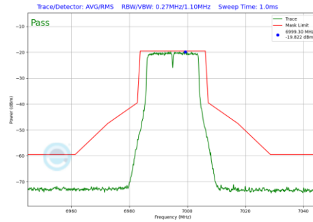
Plot 7-269 In-Band Emission Plot CDD Diversity Antenna 4a (20MHz BW 802.11a (UNII Band 8) - Ch.209)
