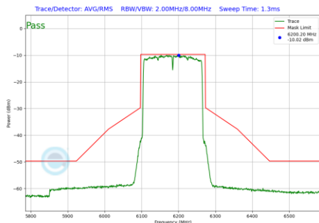
Plot 7-260 In-Band Emission Plot SDM Diversity Antenna 4a (160MHz BW 802.11be(SU) (UNII Band 5) - Ch.47)
