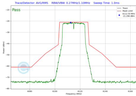
Plot 7-241 In-Band Emission Plot CDD Diversity Antenna 2a (20MHz BW 802.11a (UNII Band 5) - Ch.33)
