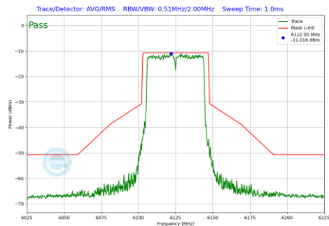
Plot 7-178 In-Band Emission Plot Antenna 4a (40MHz BW 802.11be(SU) (UNII Band 5) - Ch.35)
