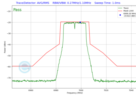
Plot 7-237 In-Band Emission Plot CDD Primary Antenna 4a (20MHz BW 802.11a (UNII Band 8) - Ch.209)
