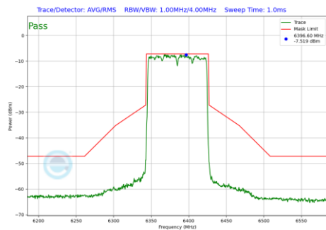
Plot 7-179 In-Band Emission Plot Antenna 4a (80MHz BW 802.11be(SU) (UNII Band 5) - Ch.87)
