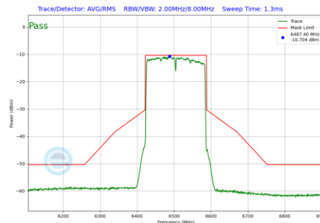
Plot 7-232 In-Band Emission Plot SDM Primary Antenna 4a (160MHz BW 802.11be(SU) (UNII Band 6) - Ch.111)
