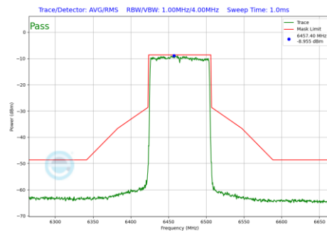
Plot 7-183 In-Band Emission Plot Antenna 4a (80MHz BW 802.11be(SU) (UNII Band 6) - Ch.103)
