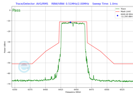
Plot 7-182 In-Band Emission Plot Antenna 4a (40MHz BW 802.11be(SU) (UNII Band 6) - Ch.99)
