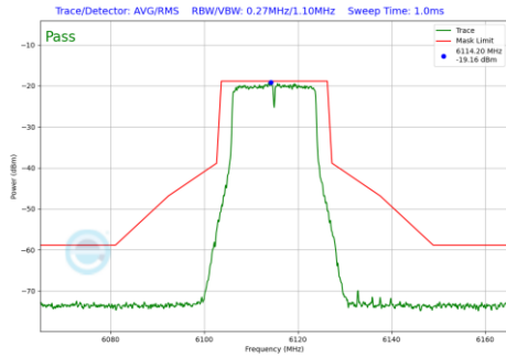
Plot 7-257 In-Band Emission Plot CDD Diversity Antenna 4a (20MHz BW 802.11a (UNII Band 5) - Ch.33)
