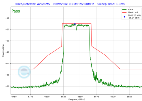
Plot 7-234 In-Band Emission Plot SDM Primary Antenna 4a (40MHz BW 802.11be(SU) (UNII Band 7) - Ch.179)
