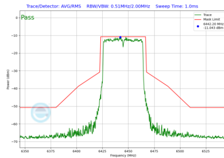
Plot 7-198 In-Band Emission Plot Antenna 2a (40MHz BW 802.11be(SU) (UNII Band 6) - Ch.99)
