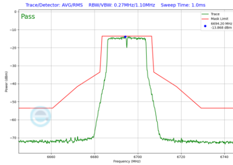
Plot 7-201 In-Band Emission Plot Antenna 2a (20MHz BW 802.11a (UNII Band 7) - Ch.149)
