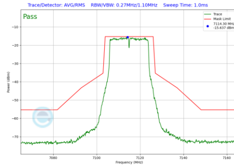
Plot 7-205 In-Band Emission Plot Antenna 2a (20MHz BW 802.11a (UNII Band 8) - Ch.233)
