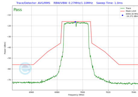
Plot 7-173 In-Band Emission Plot Antenna WF5B (20MHz BW 802.11be(SU) (UNII Band 8) - Ch.209)
