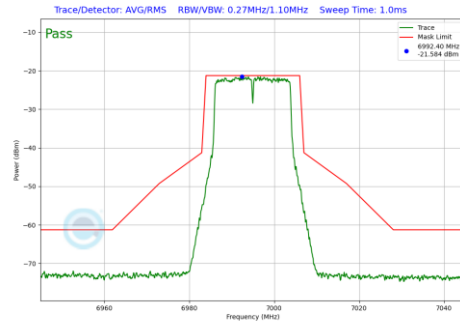
Plot 7-253 In-Band Emission Plot CDD Diversity Antenna 2a (20MHz BW 802.11a (UNII Band 8) - Ch.209)
