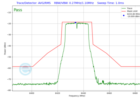
Plot 7-229 In-Band Emission Plot CDD Primary Antenna 4a (20MHz BW 802.11a (UNII Band 6) - Ch.97)
