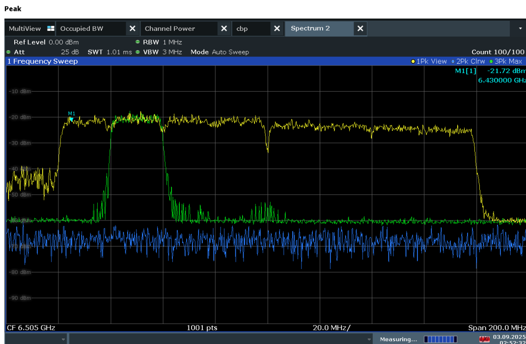
Plot 7-305. 160MHz Bandwidth, AWGN Signal Injected – 6430Mhz
