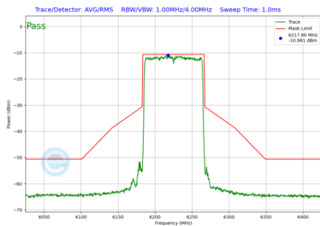
Plot 7-227 In-Band Emission Plot SDM Primary Antenna 4a (80MHz BW 802.11be(SU) (UNII Band 5) - Ch.55)
