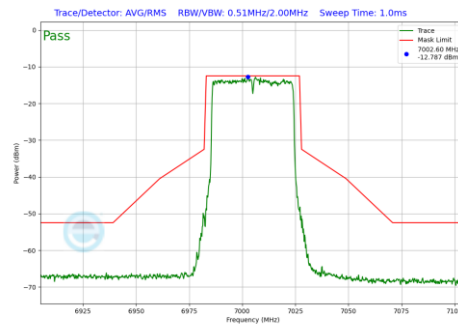
Plot 7-174 In-Band Emission Plot Antenna WF5B (40MHz BW 802.11be(SU) (UNII Band 8) - Ch.211)
