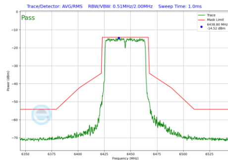
Plot 7-230 In-Band Emission Plot SDM Primary Antenna 4a (40MHz BW 802.11be(SU) (UNII Band 6) - Ch.99)
