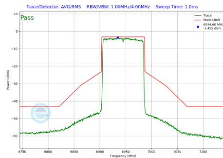
Plot 7-191 In-Band Emission Plot Antenna 4a (80MHz BW 802.11be(SU) (UNII Band 8) - Ch.199)
