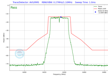
Plot 7-181 In-Band Emission Plot Antenna 4a (20MHz BW 802.11a (UNII Band 6) - Ch.97)
