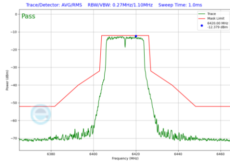
Plot 7-177 In-Band Emission Plot Antenna 4a (20MHz BW 802.11a (UNII Band 5) - Ch.93)
