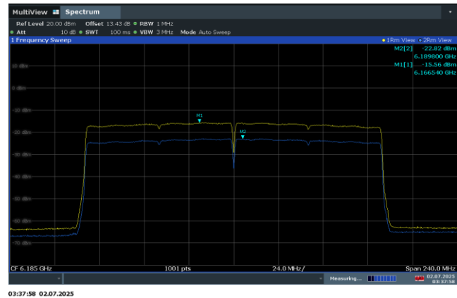
Plot 7-309. 160MHz Bandwidth – 6185MHz Antenna WF5B
