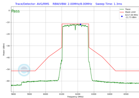
Plot 7-244 In-Band Emission Plot SDM Diversity Antenna 2a (160MHz BW 802.11be(SU) (UNII Band 5) - Ch.47)
