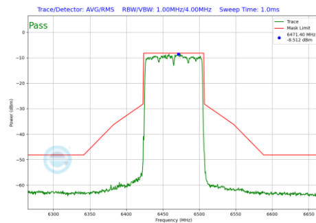
Plot 7-199 In-Band Emission Plot Antenna 2a (80MHz BW 802.11be(SU) (UNII Band 6) - Ch.103)
