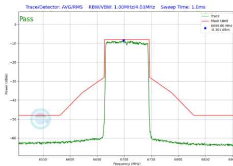
Plot 7-187 In-Band Emission Plot Antenna 4a (80MHz BW 802.11be(SU) (UNII Band 7) - Ch.151)
