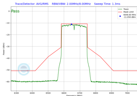
Plot 7-220 In-Band Emission Plot SDM Primary Antenna WF5B (160MHz BW 802.11be(SU) (UNII Band 7) - Ch.143)
