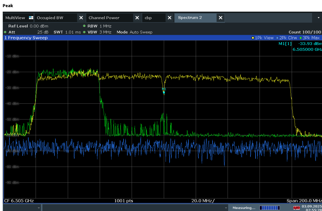
Plot 7-306. 160MHz Bandwidth, AWGN Signal Injected – 6505MHz
