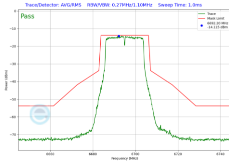
Plot 7-169 In-Band Emission Plot Antenna WF5B (20MHz BW 802.11a (UNII Band 7) - Ch.149)
