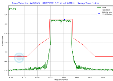
Plot 7-250 In-Band Emission Plot SDM Diversity Antenna 2a (40MHz BW 802.11be(SU) (UNII Band 7) - Ch.179)
