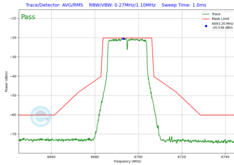
Plot 7-265 In-Band Emission Plot CDD Diversity Antenna 4a (20MHz BW 802.11a (UNII Band 7) - Ch.149)
