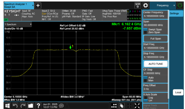
Plot 7-254 PSD SDM Diversity Antenna 2a (40MHz BW 802.11be(SU) - Ch.43)
