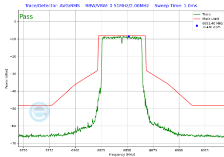
Plot 7-358 In-Band Emission Plot Antenna 2a (40MHz BW 802.11be(SU) (UNII Band 7) - Ch.179)
