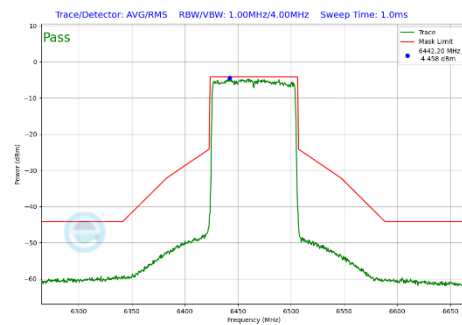
Plot 7-355 In-Band Emission Plot Antenna 2a (80MHz BW 802.11be(SU) (UNII Band 6) - Ch.103)
