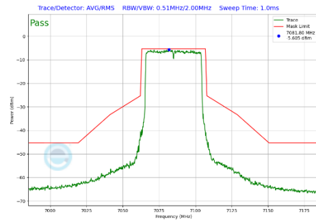
Plot 7-334 In-Band Emission Plot Antenna 4a (40MHz BW 802.11be(SU) (UNII Band 8) - Ch.227)
