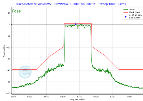
Plot 7-283 In-Band Emission Plot Antenna WF5B (80MHz BW 802.11be(SU) (UNII Band 5) - Ch.39)
