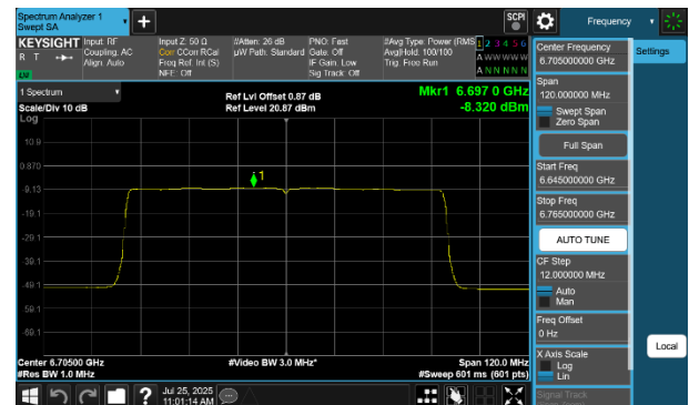
Plot 7-271 PSD SDM Diversity Antenna 2a (80MHz BW 802.11be(SU) - Ch.151)
