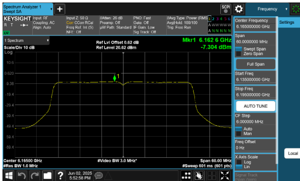
Plot 7-250 PSD SDM Diversity Antenna 4a (40MHz BW 802.11be(SU) - Ch.43)
