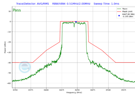
Plot 7-286 In-Band Emission Plot Antenna WF5B (40MHz BW 802.11be(SU) (UNII Band 6) - Ch.99)
