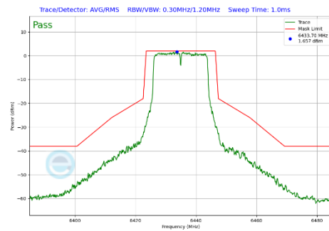
Plot 7-313 In-Band Emission Plot Antenna 4a (20MHz BW 802.11a (UNII Band 6) - Ch.97)
