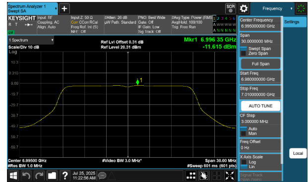
Plot 7-277 PSD CDD Diversity Antenna 2a (20MHz BW 802.11a - Ch.209)
