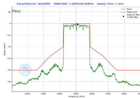
Plot 7-344 In-Band Emission Plot Antenna 2a (160MHz BW 802.11be(SU) (UNII Band 6) - Ch.111)
