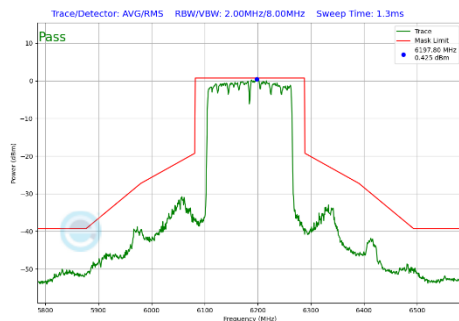
Plot 7-368 In-Band Emission Plot CDD Primary Antenna WF5B (160MHz BW 802.11be(SU) (UNII Band 5) - Ch.47)
