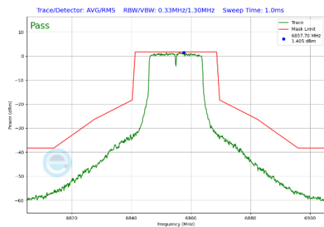
Plot 7-289 In-Band Emission Plot Antenna WF5B (20MHz BW 802.11a (UNII Band 7) - Ch.181)
