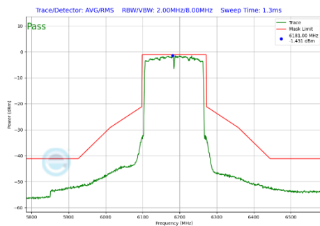
Plot 7-352 In-Band Emission Plot Antenna 2a (160MHz BW 802.11be(SU) (UNII Band 5) - Ch.47)
