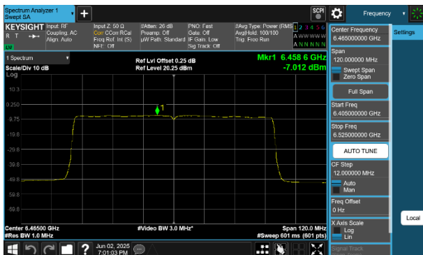
Plot 7-259 PSD SDM Diversity Antenna 4a (80MHz BW 802.11be(SU) - Ch.103)
