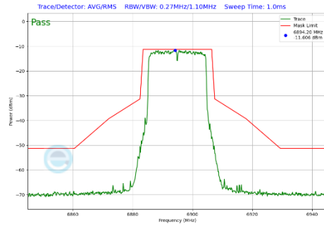
Plot 7-361 In-Band Emission Plot Antenna 2a (20MHz BW 802.11be(SU) (UNII Band 8) - Ch.189)
