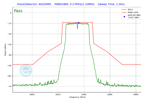
Plot 7-353 In-Band Emission Plot Antenna 2a (20MHz BW 802.11a (UNII Band 6) - Ch.97)
