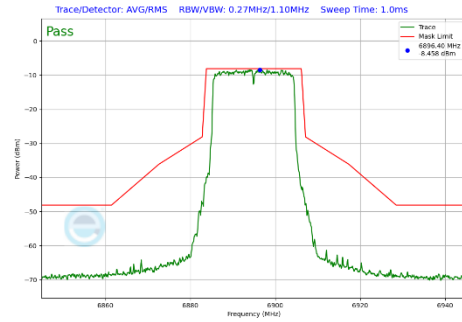
Plot 7-333 In-Band Emission Plot Antenna 4a (20MHz BW 802.11be(SU) (UNII Band 8) - Ch.189)
