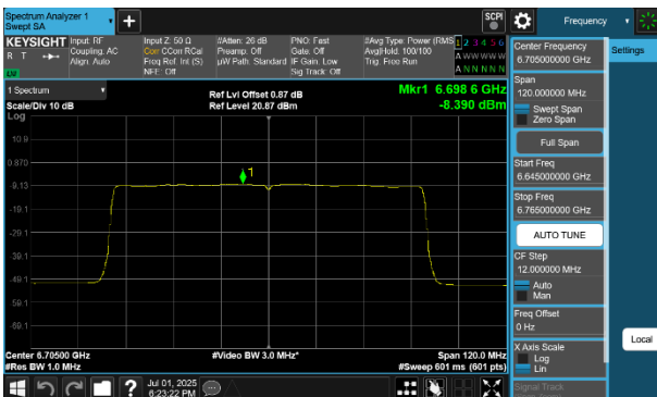
Plot 7-267 PSD SDM Diversity Antenna 4a (80MHz BW 802.11be(SU) - Ch.151)
