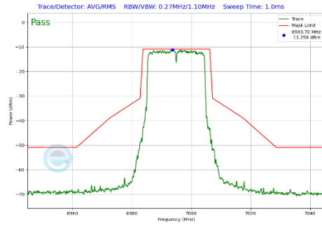
Plot 7-305 In-Band Emission Plot Antenna WF5B (20MHz BW 802.11be(SU) (UNII Band 8) - Ch.209)
