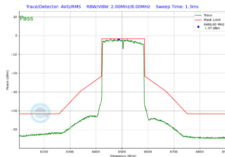
Plot 7-328 In-Band Emission Plot Antenna 4a (160MHz BW 802.11be(SU) (UNII Band 6) - Ch.111)
