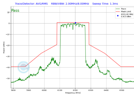
Plot 7-284 In-Band Emission Plot Antenna WF5B (160MHz BW 802.11be(SU) (UNII Band 5) - Ch.47)
