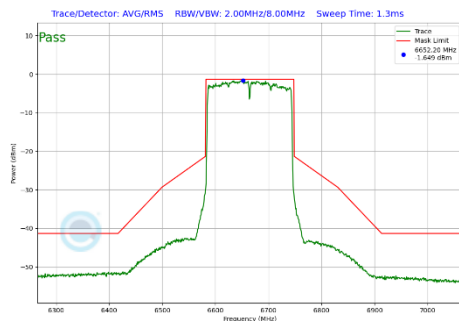
Plot 7-360 In-Band Emission Plot Antenna 2a (160MHz BW 802.11be(SU) (UNII Band 7) - Ch.143)
