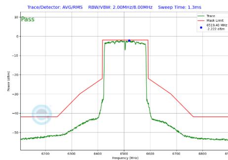
Plot 7-356 In-Band Emission Plot Antenna 2a (160MHz BW 802.11be(SU) (UNII Band 6) - Ch.111)
