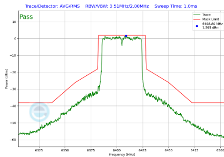
Plot 7-282 In-Band Emission Plot Antenna WF5B (40MHz BW 802.11be(SU) (UNII Band 5) - Ch.91)
