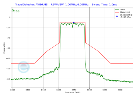
Plot 7-331 In-Band Emission Plot Antenna 4a (80MHz BW 802.11be(SU) (UNII Band 7) - Ch.119)
