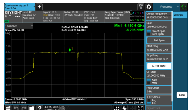
Plot 7-264 PSD SDM Diversity Antenna 2a (160MHz BW 802.11be(SU) - Ch.111)
