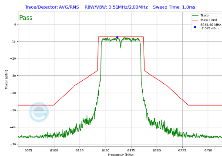
Plot 7-322 In-Band Emission Plot Antenna 4a (40MHz BW 802.11be(SU) (UNII Band 5) - Ch.43)
