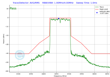
Plot 7-343 In-Band Emission Plot Antenna 2a (80MHz BW 802.11be(SU) (UNII Band 6) - Ch.103)
