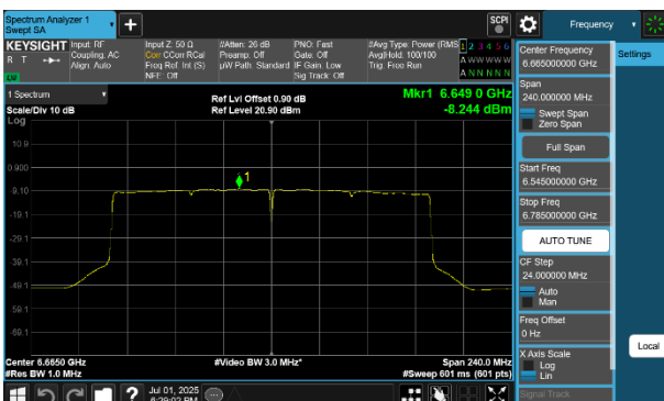
Plot 7-268 PSD SDM Diversity Antenna 4a (160MHz BW 802.11be(SU) - Ch.143)
