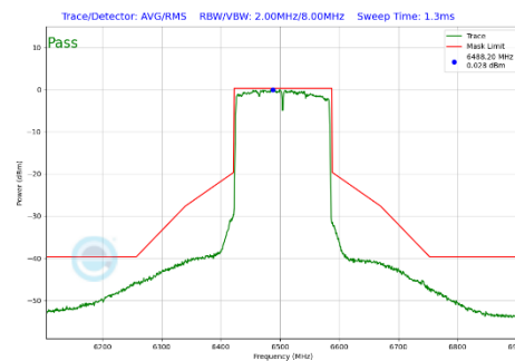
Plot 7-316 In-Band Emission Plot Antenna 4a (160MHz BW 802.11be(SU) (UNII Band 6) - Ch.111)
