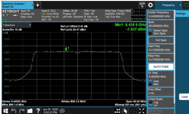
Plot 7-258 PSD SDM Diversity Antenna 4a (40MHz BW 802.11be(SU) - Ch.99)
