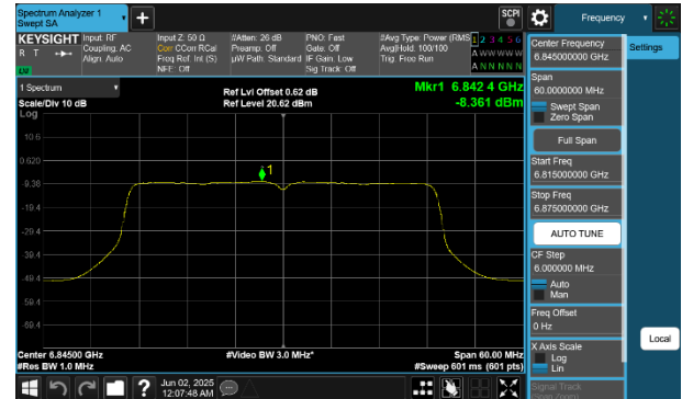
Plot 7-270 PSD SDM Diversity Antenna 2a (40MHz BW 802.11be(SU) - Ch.179)
