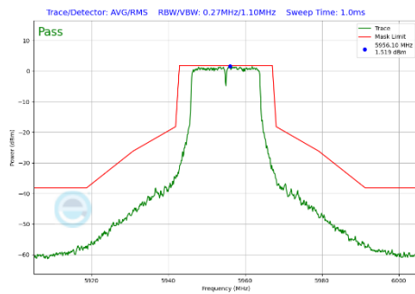
Plot 7-309 In-Band Emission Plot Antenna 4a (20MHz BW 802.11a (UNII Band 5) - Ch.1)
