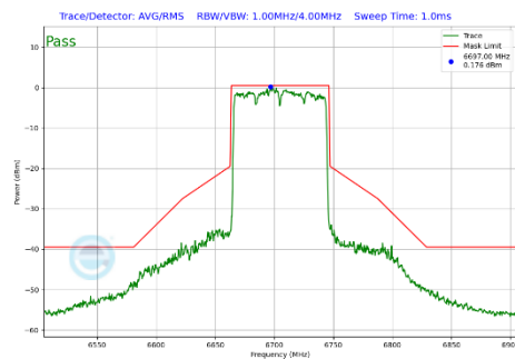
Plot 7-347 In-Band Emission Plot Antenna 2a (80MHz BW 802.11be(SU) (UNII Band 7) - Ch.151)
