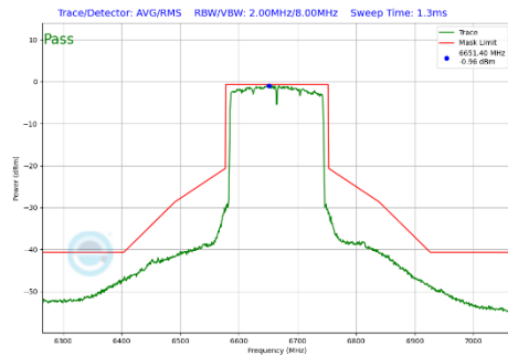
Plot 7-304 In-Band Emission Plot Antenna WF5B (160MHz BW 802.11be(SU) (UNII Band 7) - Ch.143)
