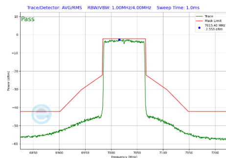
Plot 7-335 In-Band Emission Plot Antenna 4a (80MHz BW 802.11be(SU) (UNII Band 8) - Ch.215)
