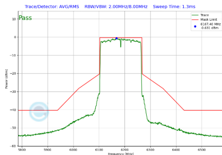
Plot 7-324 In-Band Emission Plot Antenna 4a (160MHz BW 802.11be(SU) (UNII Band 5) - Ch.47)
