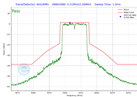
Plot 7-310 In-Band Emission Plot Antenna 4a (40MHz BW 802.11be(SU) (UNII Band 5) - Ch.3)
