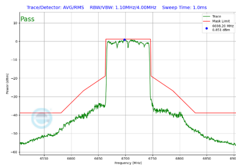
Plot 7-319 In-Band Emission Plot Antenna 4a (80MHz BW 802.11be(SU) (UNII Band 7) - Ch.151)
