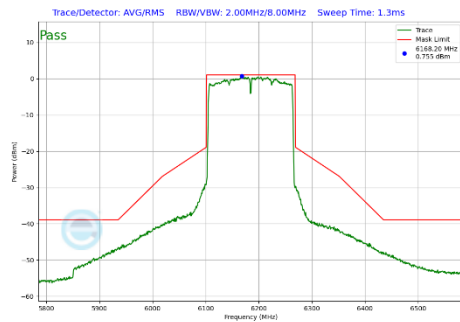
Plot 7-340 In-Band Emission Plot Antenna 2a (160MHz BW 802.11be(SU) (UNII Band 5) - Ch.47)
