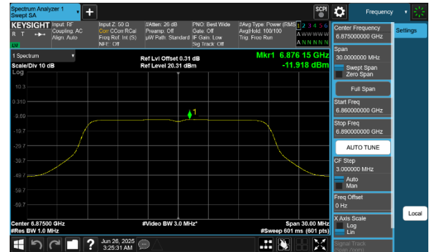
Plot 7-269 PSD CDD Diversity Antenna 2a (20MHz BW 802.11a - Ch.185)
