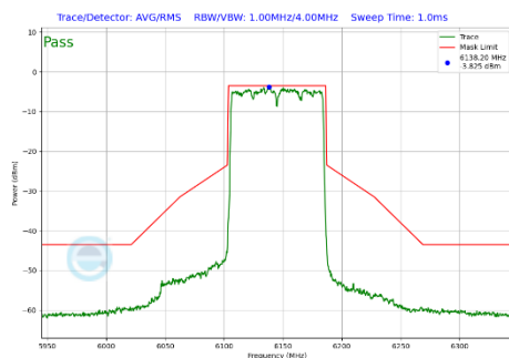
Plot 7-323 In-Band Emission Plot Antenna 4a (80MHz BW 802.11be(SU) (UNII Band 5) - Ch.39)
