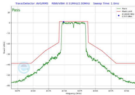
Plot 7-338 In-Band Emission Plot Antenna 2a (40MHz BW 802.11be(SU) (UNII Band 5) - Ch.43)
