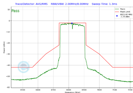
Plot 7-332 In-Band Emission Plot Antenna 4a (160MHz BW 802.11be(SU) (UNII Band 7) - Ch.175)
