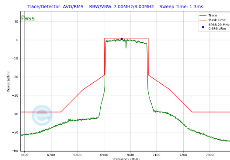
Plot 7-336 In-Band Emission Plot Antenna 4a (160MHz BW 802.11be(SU) (UNII Band 8) - Ch.207)
