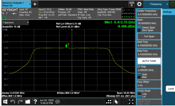
Plot 7-249 PSD CDD Diversity Antenna 4a (20MHz BW 802.11a - Ch.93)
