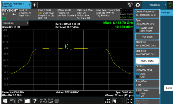
Plot 7-257 PSD CDD Diversity Antenna 4a (20MHz BW 802.11a - Ch.97)
