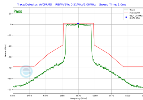
Plot 7-314 In-Band Emission Plot Antenna 4a (40MHz BW 802.11be(SU) (UNII Band 6) - Ch.115)
