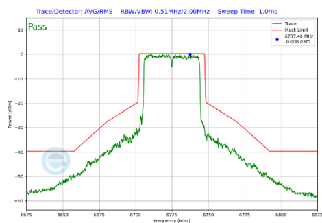
Plot 7-290 In-Band Emission Plot Antenna WF5B (40MHz BW 802.11be(SU) (UNII Band 7) - Ch.155)
