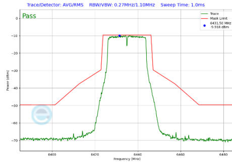
Plot 7-325 In-Band Emission Plot Antenna 4a (20MHz BW 802.11a (UNII Band 6) - Ch.97)
