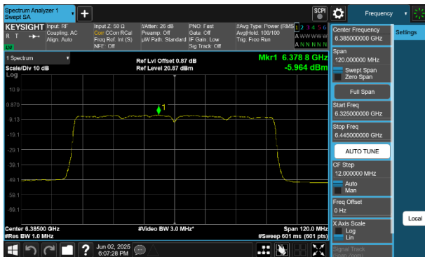
Plot 7-251 PSD SDM Diversity Antenna 4a (80MHz BW 802.11be(SU) - Ch.87)
