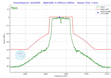
Plot 7-285 In-Band Emission Plot Antenna WF5B (20MHz BW 802.11a (UNII Band 6) - Ch.105)
