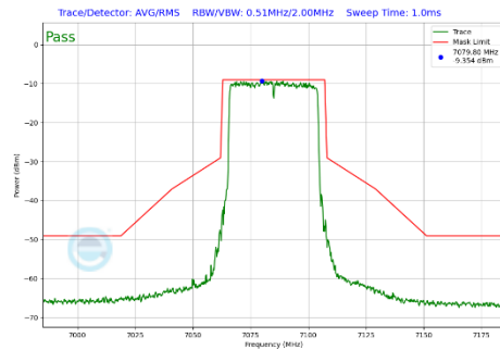
Plot 7-362 In-Band Emission Plot Antenna 2a (40MHz BW 802.11be(SU) (UNII Band 8) - Ch.227)
