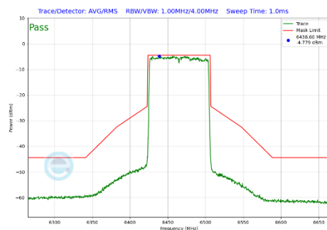
Plot 7-327 In-Band Emission Plot Antenna 4a (80MHz BW 802.11be(SU) (UNII Band 6) - Ch.103)
