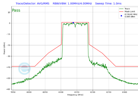
Plot 7-339 In-Band Emission Plot Antenna 2a (80MHz BW 802.11be(SU) (UNII Band 5) - Ch.39)
