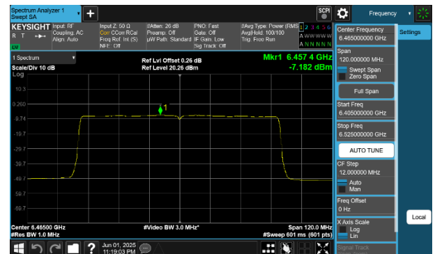
Plot 7-263 PSD SDM Diversity Antenna 2a (80MHz BW 802.11be(SU) - Ch.103)
