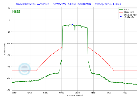
Plot 7-364 In-Band Emission Plot Antenna 2a (160MHz BW 802.11be(SU) (UNII Band 8) - Ch.207)
