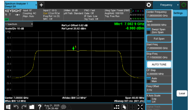
Plot 7-278 PSD SDM Diversity Antenna 2a (40MHz BW 802.11be(SU) - Ch.227)
