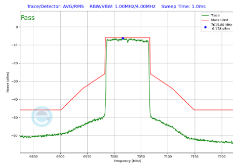
Plot 7-307 In-Band Emission Plot Antenna WF5B (80MHz BW 802.11be(SU) (UNII Band 8) - Ch.215)
