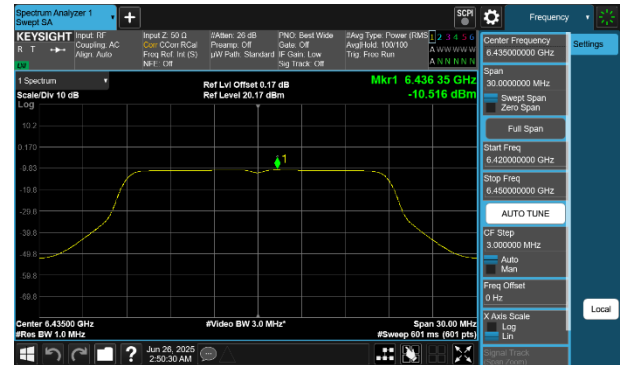
Plot 7-261 PSD CDD Diversity Antenna 2a (20MHz BW 802.11a - Ch.97)
