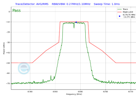
Plot 7-349 In-Band Emission Plot Antenna 2a (20MHz BW 802.11a (UNII Band 5) - Ch.45)
