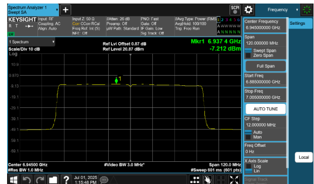
Plot 7-279 PSD SDM Diversity Antenna 2a (80MHz BW 802.11be(SU) - Ch.199)
