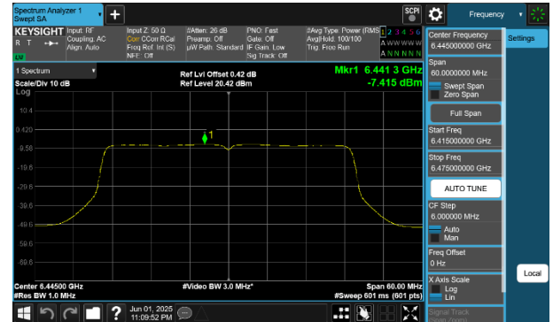
Plot 7-262 PSD SDM Diversity Antenna 2a (40MHz BW 802.11be(SU) - Ch.99)
