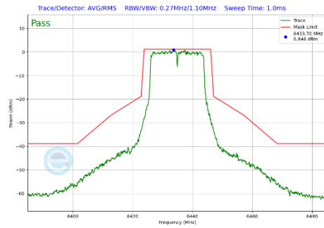
Plot 7-341 In-Band Emission Plot Antenna 2a (20MHz BW 802.11a (UNII Band 6) - Ch.97)
