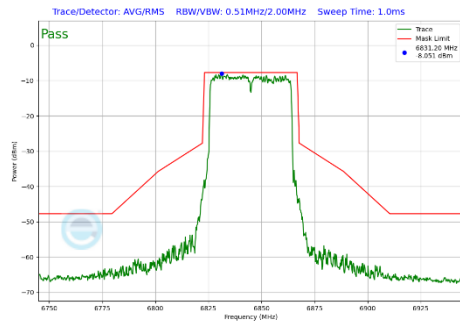
Plot 7-330 In-Band Emission Plot Antenna 4a (40MHz BW 802.11be(SU) (UNII Band 7) - Ch.179)
