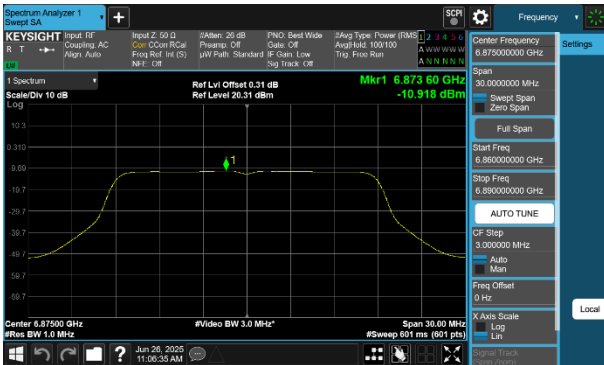
Plot 7-265 PSD CDD Diversity Antenna 4a (20MHz BW 802.11a - Ch.185)
