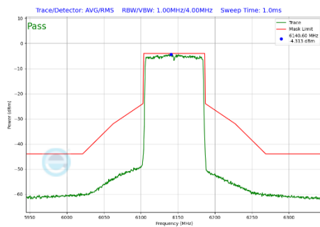
Plot 7-351 In-Band Emission Plot Antenna 2a (80MHz BW 802.11be(SU) (UNII Band 5) - Ch.39)
