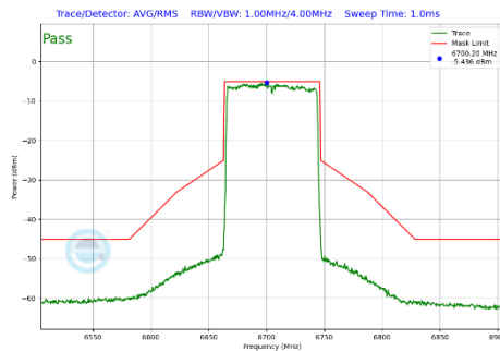
Plot 7-359 In-Band Emission Plot Antenna 2a (80MHz BW 802.11be(SU) (UNII Band 7) - Ch.151)
