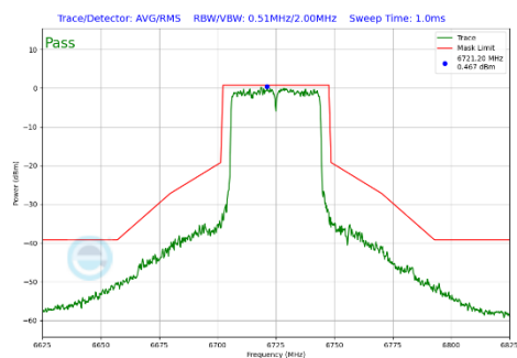
Plot 7-346 In-Band Emission Plot Antenna 2a (40MHz BW 802.11be(SU) (UNII Band 7) - Ch.155)
