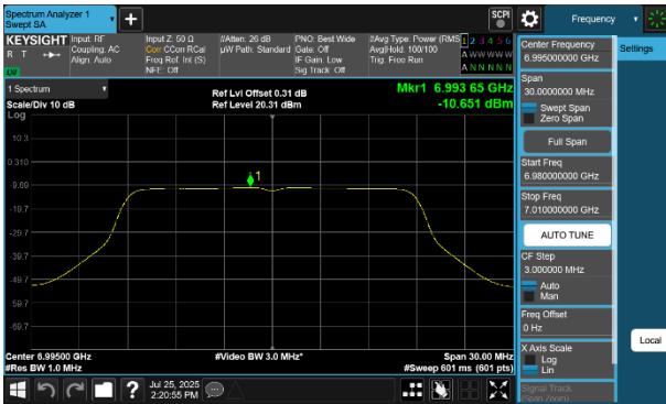
Plot 7-273 PSD CDD Diversity Antenna 4a (20MHz BW 802.11a - Ch.209)
