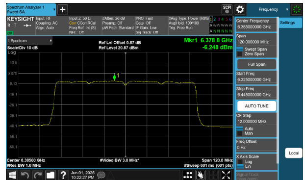
Plot 7-255 PSD SDM Diversity Antenna 2a (80MHz BW 802.11be(SU) - Ch.87)
