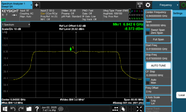
Plot 7-266 PSD SDM Diversity Antenna 4a (40MHz BW 802.11be(SU) - Ch.179)
