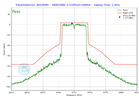
Plot 7-318 In-Band Emission Plot Antenna 4a (40MHz BW 802.11be(SU) (UNII Band 7) - Ch.155)
