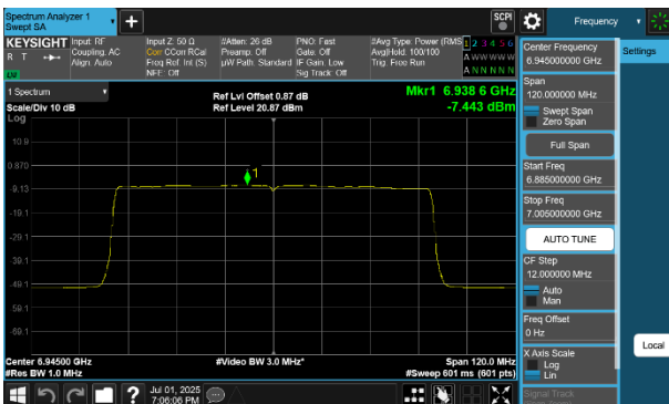
Plot 7-275 PSD SDM Diversity Antenna 4a (80MHz BW 802.11be(SU) - Ch.199)
