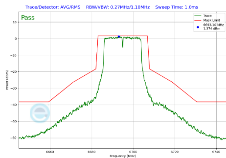
Plot 7-317 In-Band Emission Plot Antenna 4a (20MHz BW 802.11a (UNII Band 7) - Ch.149)
