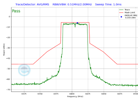
Plot 7-350 In-Band Emission Plot Antenna 2a (40MHz BW 802.11be(SU) (UNII Band 5) - Ch.91)
