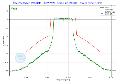
Plot 7-281 In-Band Emission Plot Antenna WF5B (20MHz BW 802.11a (UNII Band 5) - Ch.45)
