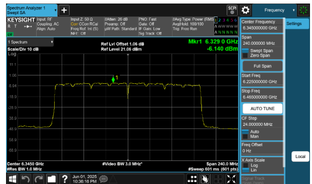
Plot 7-256 PSD SDM Diversity Antenna 2a (160MHz BW 802.11be(SU) - Ch.79)
