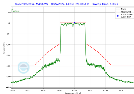
Plot 7-367 In-Band Emission Plot CDD Primary Antenna WF5B (80MHz BW 802.11be(SU) (UNII Band 5) - Ch.39)
