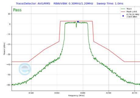
Plot 7-337 In-Band Emission Plot Antenna 2a (20MHz BW 802.11a (UNII Band 5) - Ch.45)
