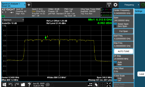
Plot 7-252 PSD SDM Diversity Antenna 4a (160MHz BW 802.11be(SU) - Ch.79)
