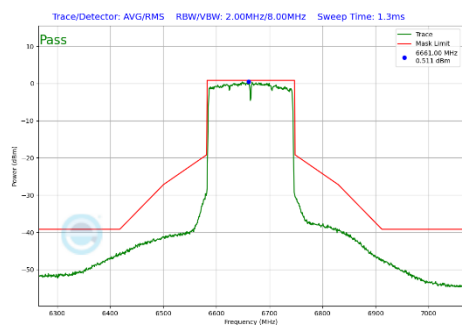
Plot 7-320 In-Band Emission Plot Antenna 4a (160MHz BW 802.11be(SU) (UNII Band 7) - Ch.143)
