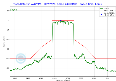
Plot 7-348 In-Band Emission Plot Antenna 2a (160MHz BW 802.11be(SU) (UNII Band 7) - Ch.143)
