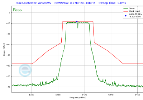
Plot 7-321 In-Band Emission Plot Antenna 4a (20MHz BW 802.11a (UNII Band 5) - Ch.93)
