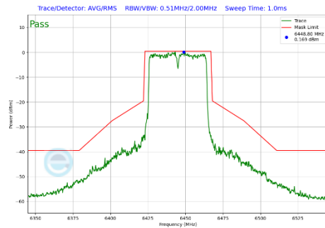
Plot 7-342 In-Band Emission Plot Antenna 2a (40MHz BW 802.11be(SU) (UNII Band 6) - Ch.99)
