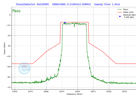
Plot 7-326 In-Band Emission Plot Antenna 4a (40MHz BW 802.11be(SU) (UNII Band 6) - Ch.99)
