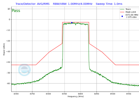
Plot 7-295 In-Band Emission Plot Antenna WF5B (80MHz BW 802.11be(SU) (UNII Band 5) - Ch.87)
