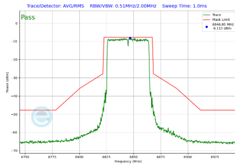
Plot 7-302 In-Band Emission Plot Antenna WF5B (40MHz BW 802.11be(SU) (UNII Band 7) - Ch.179)
