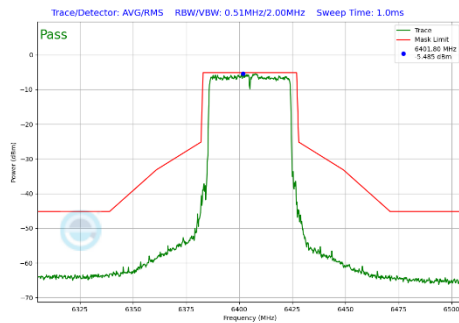
Plot 7-294 In-Band Emission Plot Antenna WF5B (40MHz BW 802.11be(SU) (UNII Band 5) - Ch.91)
