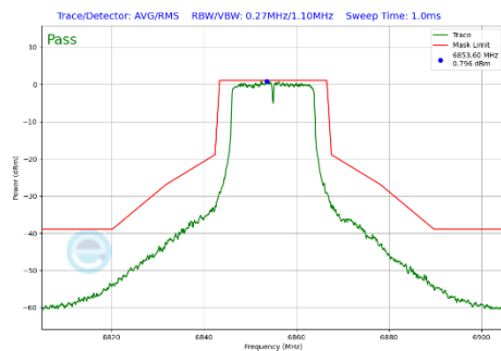
Plot 7-345 In-Band Emission Plot Antenna 2a (20MHz BW 802.11a (UNII Band 7) - Ch.181)
