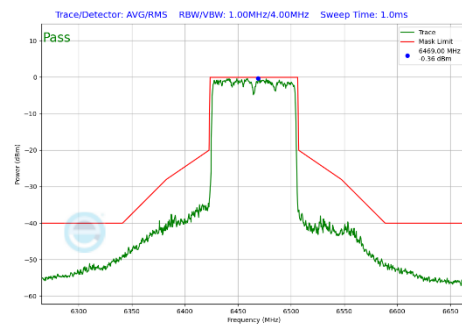
Plot 7-315 In-Band Emission Plot Antenna 4a (80MHz BW 802.11be(SU) (UNII Band 6) - Ch.103)
