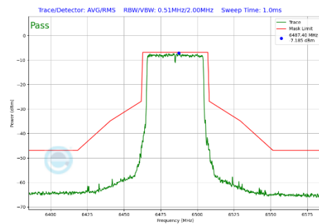
Plot 7-354 In-Band Emission Plot Antenna 2a (40MHz BW 802.11be(SU) (UNII Band 6) - Ch.107)
