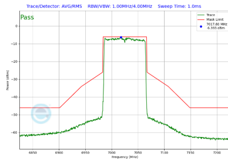
Plot 7-363 In-Band Emission Plot Antenna 2a (80MHz BW 802.11be(SU) (UNII Band 8) - Ch.215)
