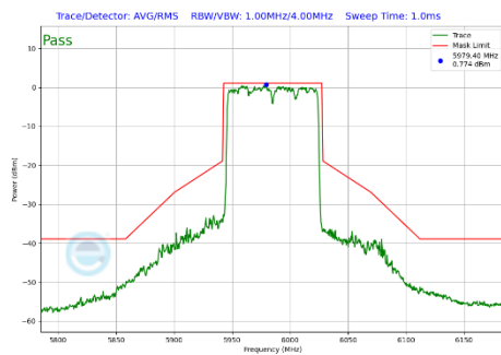
Plot 7-311 In-Band Emission Plot Antenna 4a (80MHz BW 802.11be(SU) (UNII Band 5) - Ch.7)
