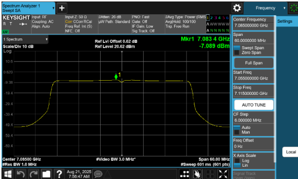
Plot 7-274 PSD SDM Diversity Antenna 4a (40MHz BW 802.11be(SU) - Ch.227)
