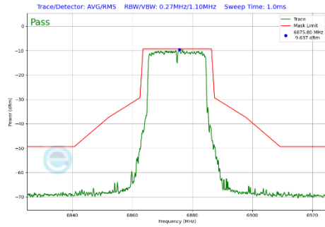
Plot 7-329 In-Band Emission Plot Antenna 4a (20MHz BW 802.11be(SU) (UNII Band 7) - Ch.185)
