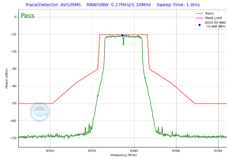
Plot 7-357 In-Band Emission Plot Antenna 2a (20MHz BW 802.11a (UNII Band 7) - Ch.117)
