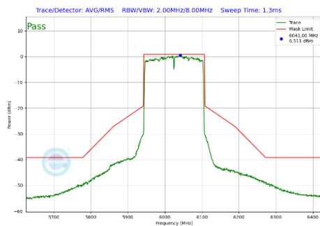
Plot 7-312 In-Band Emission Plot Antenna 4a (160MHz BW 802.11be(SU) (UNII Band 5) - Ch.15)
