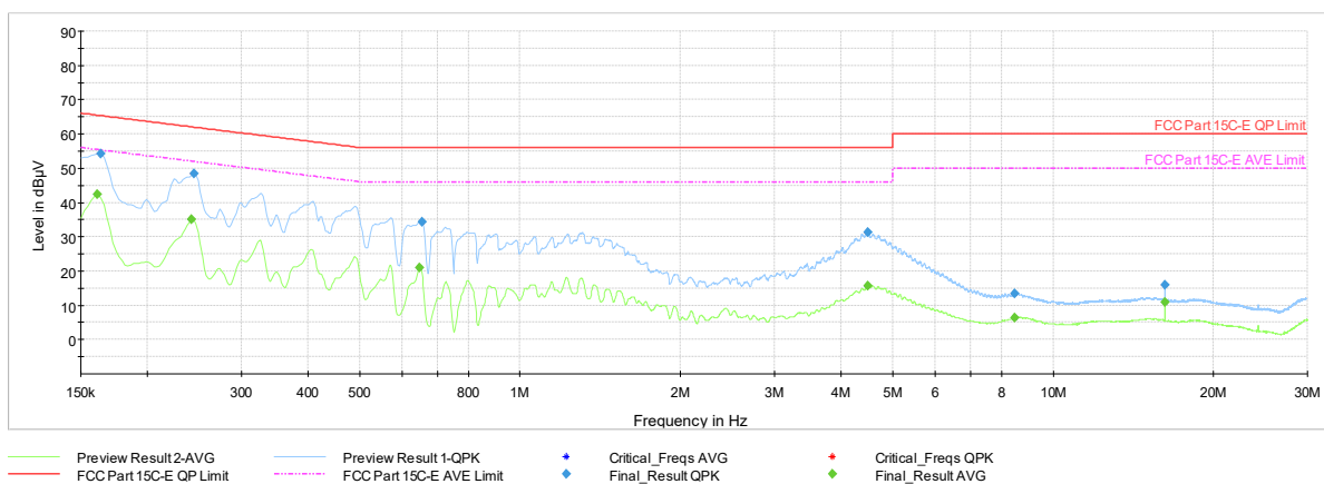
Plot 7-415. AC Line Conducted Plot with 802.11be SDM Primary – Ch.61 (L1), with AC/DC Adaptor
