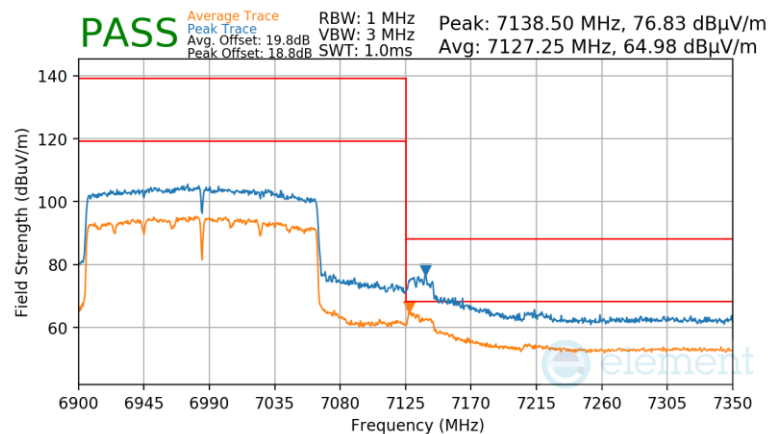
Plot 7-384 Antenna 2a Radiated Upper Band Edge (Peak & Average – UNII Band 8)
