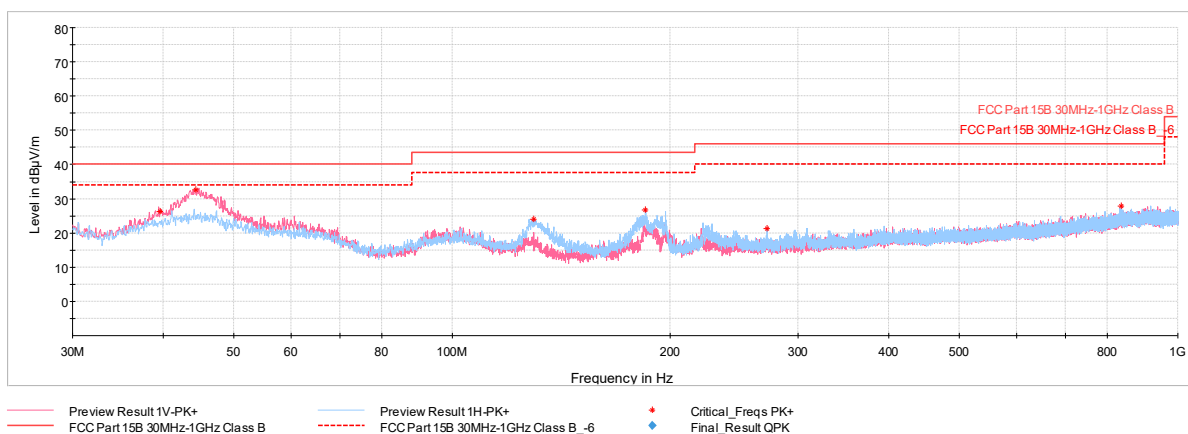
Plot 7-414. Radiated Spurious Emissions below 1GHz SDM Diversity, 802.11be, Ch.61 with AC/DC Adaptor
