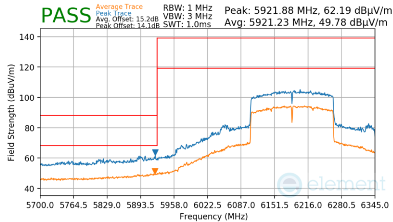
Plot 7-383 Antenna 2a Radiated Lower Band Edge (Peak & Average – UNII Band 5)
