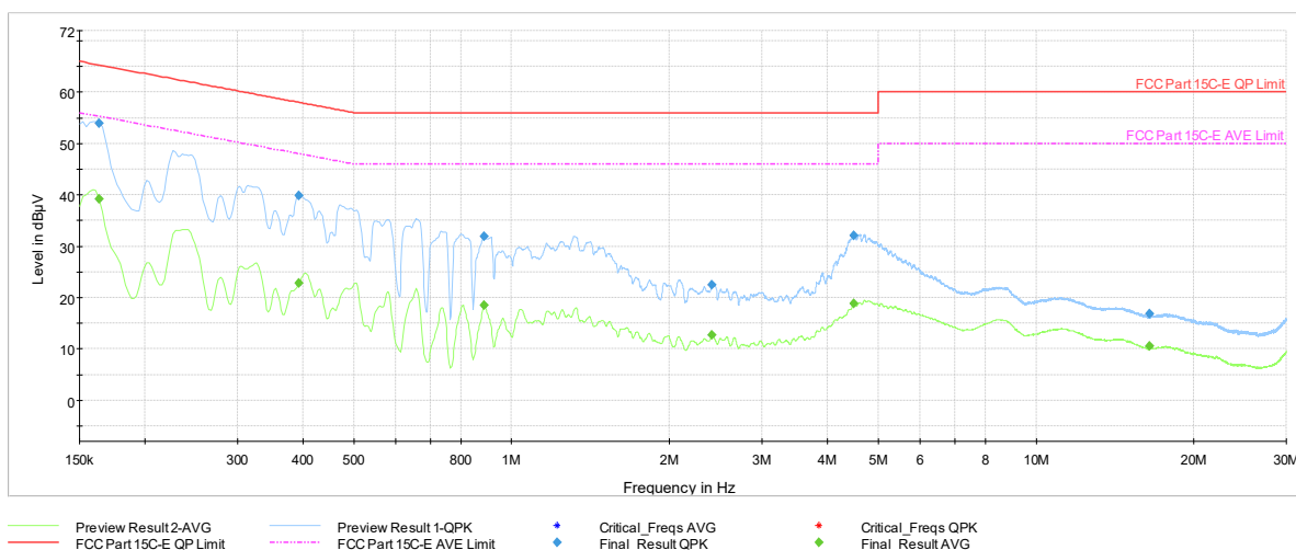
Plot 7-418. AC Line Conducted Plot with 802.11be SDM Diversity – Ch. 61 (N), with AC/DC Adaptor
