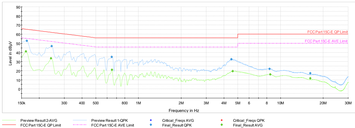
Plot 7-416. AC Line Conducted Plot with 802.11be SDM Primary – Ch. 61 (N), with AC/DC Adaptor
