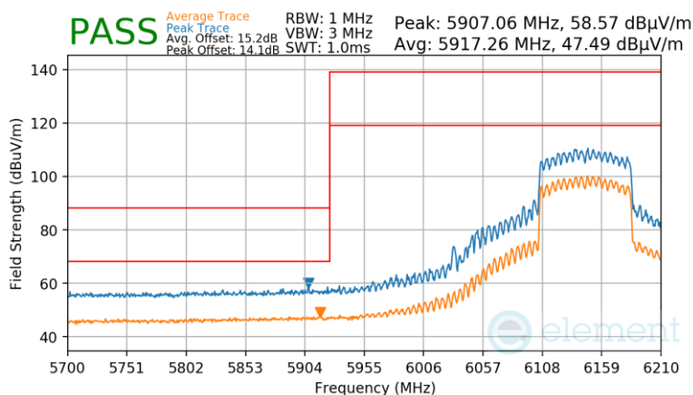
Plot 7-409 SDM Diversity Radiated Lower Band Edge (Peak & Average – UNII Band 5)
