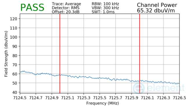
Plot 7-388 CDD Primary Radiated Upper Band Edge (Average – UNII Band 8)
