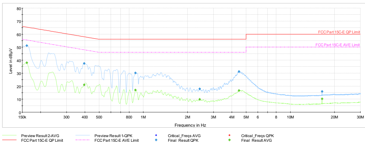
Plot 7-417. AC Line Conducted Plot with 802.11be SDM Diversity – Ch.61 (L1), with AC/DC Adaptor
