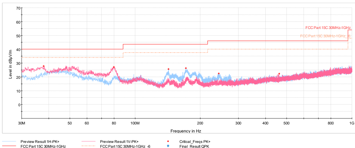
Plot 7-413. Radiated Spurious Emissions below 1GHz SDM Primary, 802.11be, Ch.61 with AC/DC Adaptor
