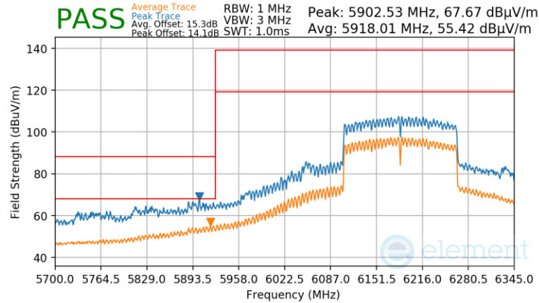
Plot 7-411 SDM Diversity Radiated Lower Band Edge (Peak & Average – UNII Band 5)
