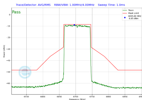
Plot 7-455 In-Band Emission Plot SDM Diversity Antenna 2a (80MHz BW 802.11be(SU) (UNII Band 7) - Ch.151)
