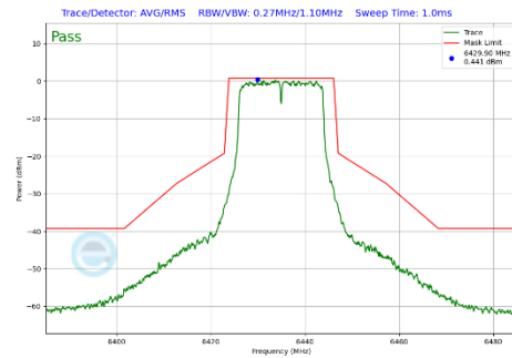
Plot 7-425 In-Band Emission Plot CDD Diversity Antenna 2a (20MHz BW 802.11a (UNII Band 6) - Ch.97)
