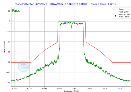
Plot 7-386 In-Band Emission Plot CDD Primary Antenna 4a (40MHz BW 802.11be(SU) (UNII Band 7) - Ch.179)
