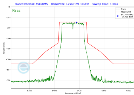
Plot 7-445 In-Band Emission Plot CDD Diversity Antenna 2a (20MHz BW 802.11a (UNII Band 5) - Ch.93)
