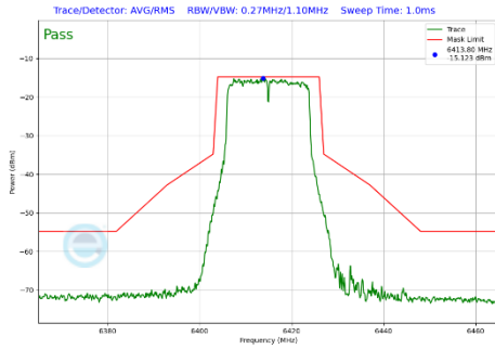
Plot 7-461 In-Band Emission Plot CDD Diversity Antenna 4a (20MHz BW 802.11a (UNII Band 5) - Ch.93)
