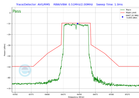
Plot 7-466 In-Band Emission Plot SDM Diversity Antenna 4a (40MHz BW 802.11be(SU) (UNII Band 6) - Ch.99)
