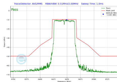
Plot 7-450 In-Band Emission Plot SDM Diversity Antenna 2a (40MHz BW 802.11be(SU) (UNII Band 6) - Ch.99)
