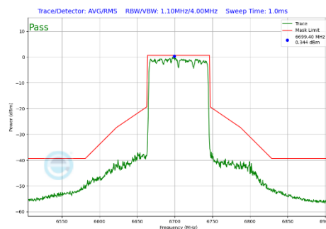
Plot 7-443 In-Band Emission Plot CDD Diversity Antenna 4a (80MHz BW 802.11be(SU) (UNII Band 7) - Ch.151)
