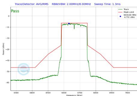
Plot 7-416 In-Band Emission Plot SDM Primary Antenna 4a (160MHz BW 802.11be(SU) (UNII Band 7) - Ch.143)
