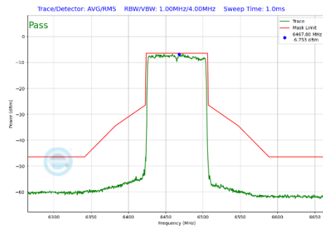
Plot 7-411 In-Band Emission Plot SDM Primary Antenna 4a (80MHz BW 802.11be(SU) (UNII Band 6) - Ch.103)
