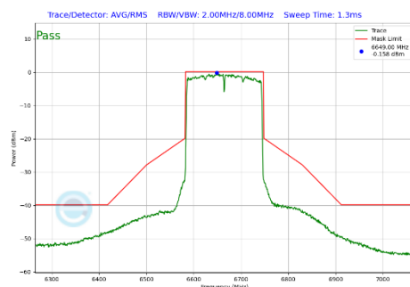
Plot 7-444 In-Band Emission Plot CDD Diversity Antenna 4a (160MHz BW 802.11be(SU) (UNII Band 7) - Ch.143)
