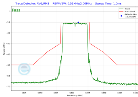
Plot 7-406 In-Band Emission Plot SDM Primary Antenna 4a (40MHz BW 802.11be(SU) (UNII Band 5) - Ch.91)
