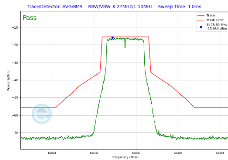
Plot 7-449 In-Band Emission Plot CDD Diversity Antenna 2a (20MHz BW 802.11a (UNII Band 6) - Ch.97)
