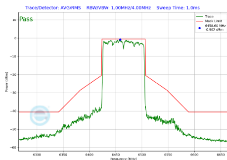
Plot 7-439 In-Band Emission Plot CDD Diversity Antenna 4a (80MHz BW 802.11be(SU) (UNII Band 6) - Ch.103)
