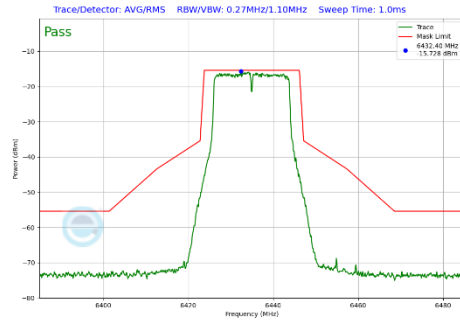
Plot 7-409 In-Band Emission Plot CDD Primary Antenna 4a (20MHz BW 802.11a (UNII Band 6) - Ch.97)
