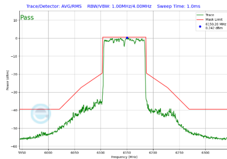
Plot 7-435 In-Band Emission Plot CDD Diversity Antenna 4a (80MHz BW 802.11be(SU) (UNII Band 5) - Ch.39)
