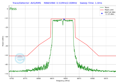
Plot 7-398 In-Band Emission Plot SDM Primary Antenna WF5B (40MHz BW 802.11be(SU) (UNII Band 7) - Ch.179)
