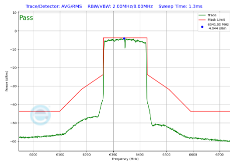
Plot 7-392 In-Band Emission Plot SDM Primary Antenna WF5B (160MHz BW 802.11be(SU) (UNII Band 5) - Ch.79)
