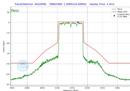
Plot 7-423 In-Band Emission Plot CDD Diversity Antenna 2a (80MHz BW 802.11be(SU) (UNII Band 5) - Ch.39)
