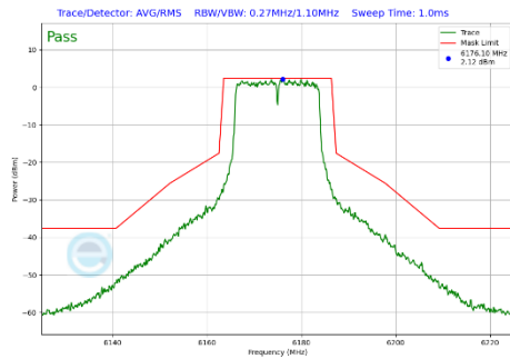
Plot 7-421 In-Band Emission Plot CDD Diversity Antenna 2a (20MHz BW 802.11a (UNII Band 5) - Ch.45)
