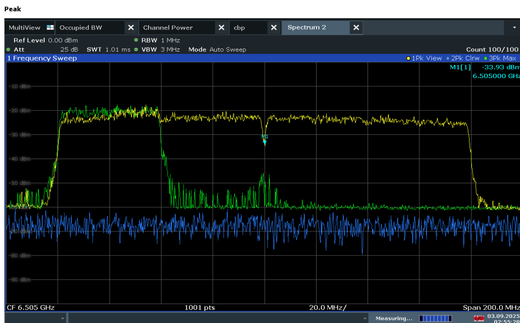
Plot 7-510. 160MHz Bandwidth, AWGN Signal Injected – 6505MHz
