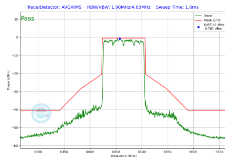
Plot 7-427 In-Band Emission Plot CDD Diversity Antenna 2a (80MHz BW 802.11be(SU) (UNII Band 6) - Ch.103)
