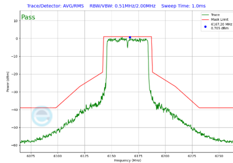
Plot 7-434 In-Band Emission Plot CDD Diversity Antenna 4a (40MHz BW 802.11be(SU) (UNII Band 5) - Ch.43)
