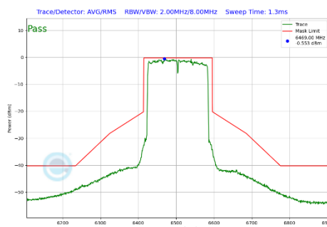
Plot 7-384 In-Band Emission Plot CDD Primary Antenna 4a (160MHz BW 802.11be(SU) (UNII Band 6) - Ch.111)
