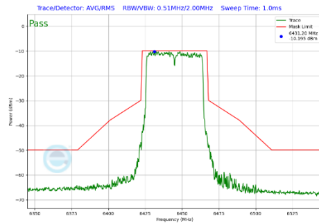
Plot 7-410 In-Band Emission Plot SDM Primary Antenna 4a (40MHz BW 802.11be(SU) (UNII Band 6) - Ch.99)
