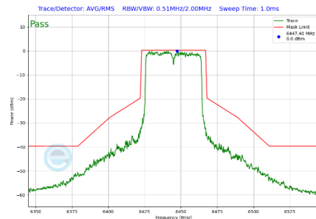
Plot 7-426 In-Band Emission Plot CDD Diversity Antenna 2a (40MHz BW 802.11be(SU) (UNII Band 6) - Ch.99)
