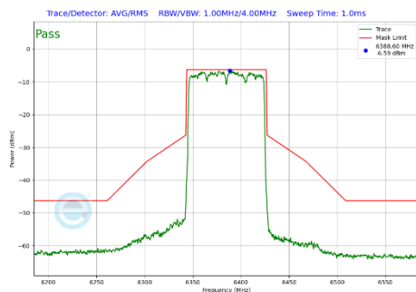
Plot 7-447 In-Band Emission Plot SDM Diversity Antenna 2a (80MHz BW 802.11be(SU) (UNII Band 5) - Ch.87)
