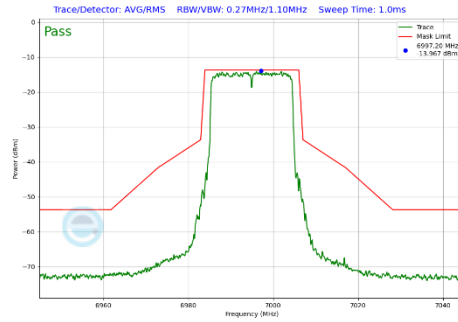
Plot 7-417 In-Band Emission Plot SDM Primary Antenna 4a (20MHz BW 802.11be(SU) (UNII Band 8) - Ch.209)
