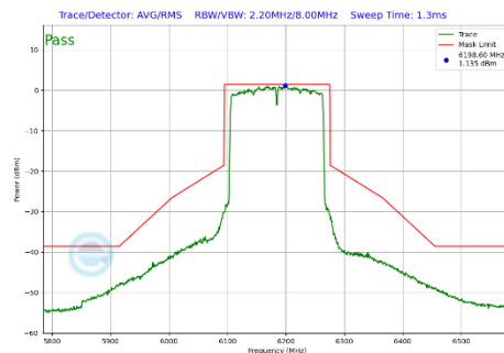
Plot 7-380 In-Band Emission Plot CDD Primary Antenna 4a (160MHz BW 802.11be(SU) (UNII Band 5) - Ch.47)
