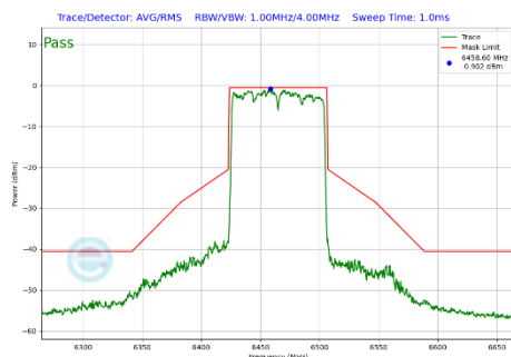
Plot 7-383 In-Band Emission Plot CDD Primary Antenna 4a (80MHz BW 802.11be(SU) (UNII Band 6) - Ch.103)
