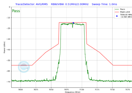
Plot 7-458 In-Band Emission Plot SDM Diversity Antenna 2a (40MHz BW 802.11be(SU) (UNII Band 8) - Ch.227)
