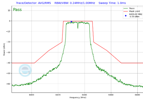
Plot 7-381 In-Band Emission Plot CDD Primary Antenna 4a (20MHz BW 802.11a (UNII Band 6) - Ch.97)
