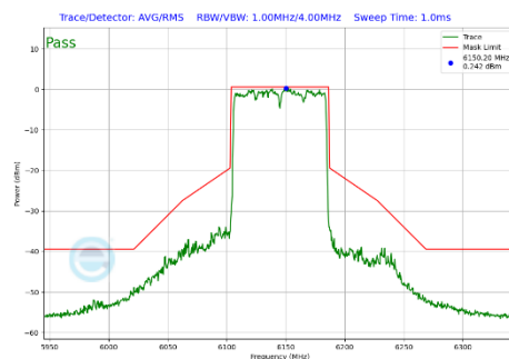
Plot 7-379 In-Band Emission Plot CDD Primary Antenna 4a (80MHz BW 802.11be(SU) (UNII Band 5) - Ch.39)
