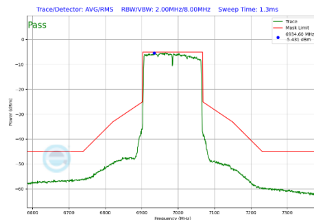
Plot 7-460 In-Band Emission Plot SDM Diversity Antenna 2a (160MHz BW 802.11be(SU) (UNII Band 8) - Ch.207)
