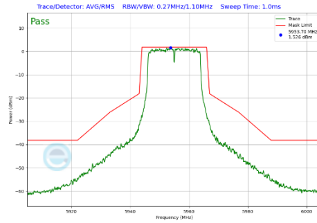
Plot 7-377 In-Band Emission Plot CDD Primary Antenna 4a (20MHz BW 802.11a (UNII Band 5) - Ch.1)
