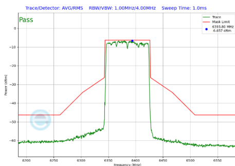
Plot 7-463 In-Band Emission Plot SDM Diversity Antenna 4a (80MHz BW 802.11be(SU) (UNII Band 5) - Ch.87)
