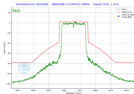
Plot 7-378 In-Band Emission Plot CDD Primary Antenna 4a (40MHz BW 802.11be(SU) (UNII Band 5) - Ch.3)
