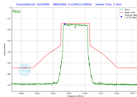
Plot 7-418 In-Band Emission Plot SDM Primary Antenna 4a (40MHz BW 802.11be(SU) (UNII Band 8) - Ch.227)
