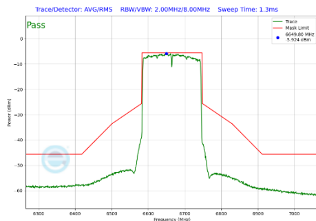
Plot 7-456 In-Band Emission Plot SDM Diversity Antenna 2a (160MHz BW 802.11be(SU) (UNII Band 7) - Ch.143)
