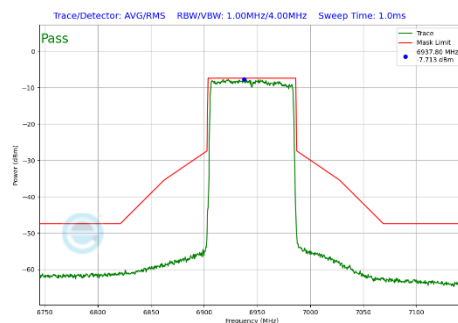
Plot 7-459 In-Band Emission Plot SDM Diversity Antenna 2a (80MHz BW 802.11be(SU) (UNII Band 8) - Ch.199)
