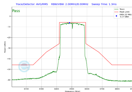
Plot 7-452 In-Band Emission Plot SDM Diversity Antenna 2a (160MHz BW 802.11be(SU) (UNII Band 6) - Ch.111)
