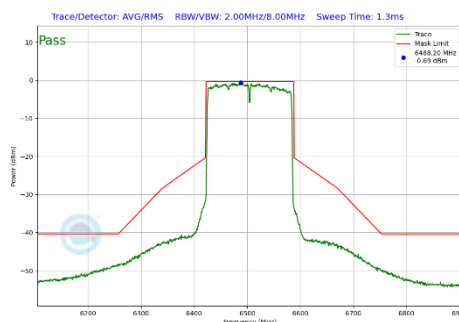
Plot 7-440 In-Band Emission Plot CDD Diversity Antenna 4a (160MHz BW 802.11be(SU) (UNII Band 6) - Ch.111)
