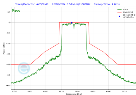
Plot 7-374 In-Band Emission Plot CDD Primary Antenna WF5B (40MHz BW 802.11be(SU) (UNII Band 7) - Ch.179)
