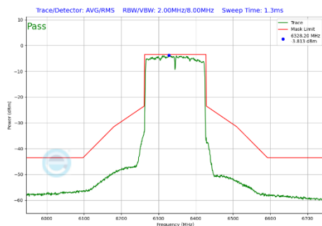
Plot 7-448 In-Band Emission Plot SDM Diversity Antenna 2a (160MHz BW 802.11be(SU) (UNII Band 5) - Ch.79)
