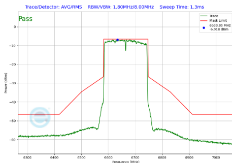
Plot 7-472 In-Band Emission Plot SDM Diversity Antenna 4a (160MHz BW 802.11be(SU) (UNII Band 7) - Ch.143)
