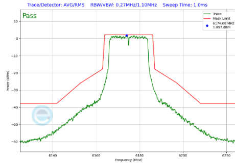
Plot 7-433 In-Band Emission Plot CDD Diversity Antenna 4a (20MHz BW 802.11a (UNII Band 5) - Ch.45)
