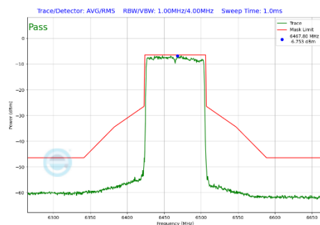
Plot 7-467 In-Band Emission Plot SDM Diversity Antenna 4a (80MHz BW 802.11be(SU) (UNII Band 6) - Ch.103)
