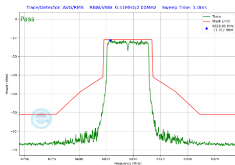
Plot 7-454 In-Band Emission Plot SDM Diversity Antenna 2a (40MHz BW 802.11be(SU) (UNII Band 7) - Ch.179)
