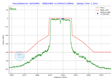
Plot 7-382 In-Band Emission Plot CDD Primary Antenna 4a (40MHz BW 802.11be(SU) (UNII Band 6) - Ch.99)
