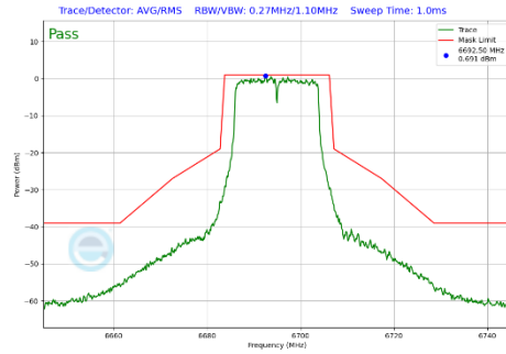
Plot 7-441 In-Band Emission Plot CDD Diversity Antenna 4a (20MHz BW 802.11a (UNII Band 7) - Ch.149)
