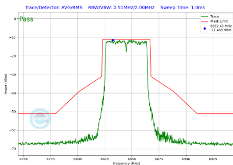
Plot 7-470 In-Band Emission Plot SDM Diversity Antenna 4a (40MHz BW 802.11be(SU) (UNII Band 7) - Ch.179)
