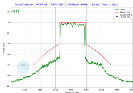
Plot 7-375 In-Band Emission Plot CDD Primary Antenna WF5B (80MHz BW 802.11be(SU) (UNII Band 7) - Ch.151)
