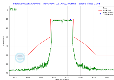
Plot 7-446 In-Band Emission Plot SDM Diversity Antenna 2a (40MHz BW 802.11be(SU) (UNII Band 5) - Ch.43)
