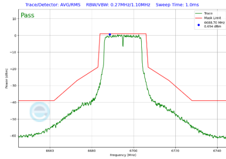
Plot 7-429 In-Band Emission Plot CDD Diversity Antenna 2a (20MHz BW 802.11a (UNII Band 7) - Ch.149)
