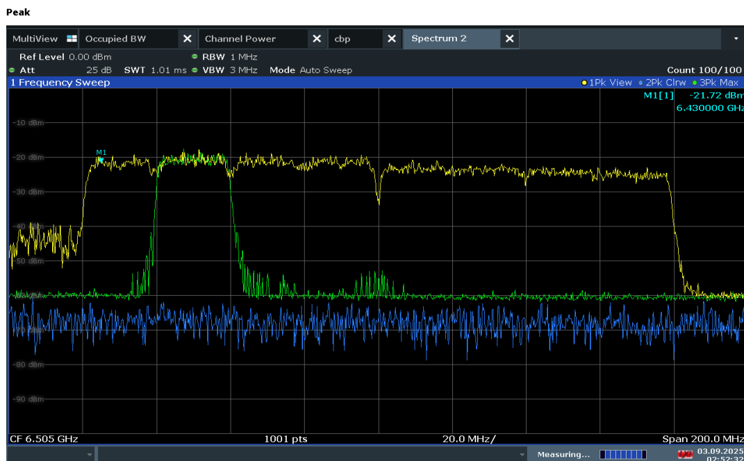
Plot 7-509. 160MHz Bandwidth, AWGN Signal Injected – 6430Mhz
