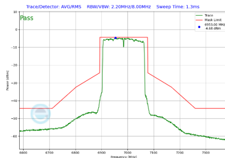
Plot 7-476 In-Band Emission Plot SDM Diversity Antenna 4a (160MHz BW 802.11be(SU) (UNII Band 8) - Ch.207)
