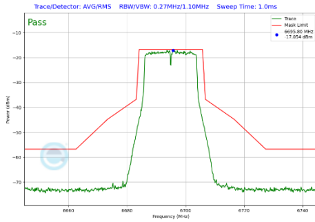
Plot 7-397 In-Band Emission Plot CDD Primary Antenna WF5B (20MHz BW 802.11a (UNII Band 7) - Ch.149)
