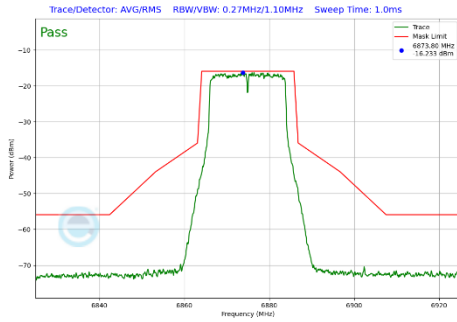
Plot 7-469 In-Band Emission Plot CDD Diversity Antenna 4a (20MHz BW 802.11a (UNII Band 7) - Ch.185)
