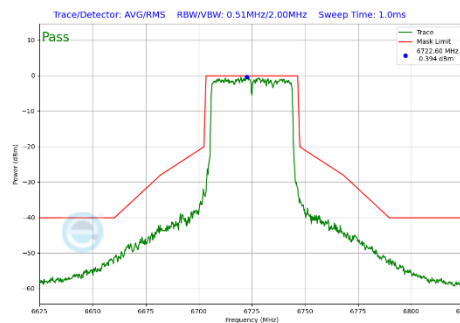
Plot 7-442 In-Band Emission Plot CDD Diversity Antenna 4a (40MHz BW 802.11be(SU) (UNII Band 7) - Ch.155)
