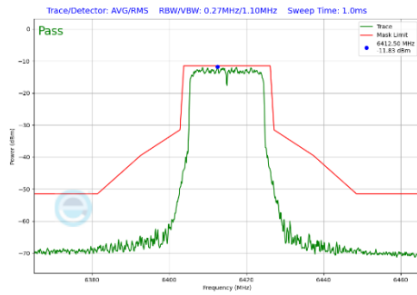
Plot 7-389 In-Band Emission Plot SDM Primary Antenna WF5B (20MHz BW 802.11be(SU) (UNII Band 5) - Ch.93)
