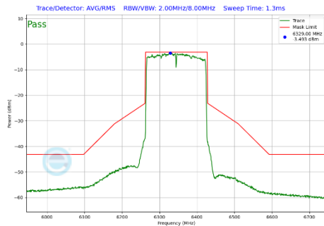
Plot 7-408 In-Band Emission Plot SDM Primary Antenna 4a (160MHz BW 802.11be(SU) (UNII Band 5) - Ch.79)
