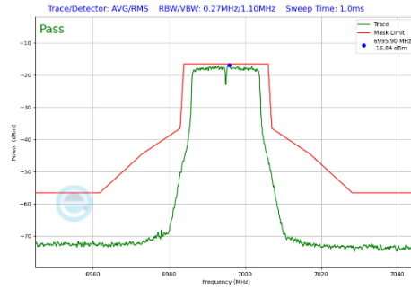
Plot 7-457 In-Band Emission Plot CDD Diversity Antenna 2a (20MHz BW 802.11a (UNII Band 8) - Ch.209)
