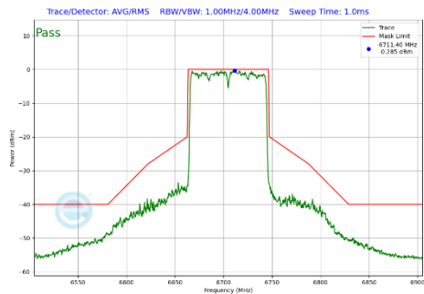
Plot 7-431 In-Band Emission Plot CDD Diversity Antenna 2a (80MHz BW 802.11be(SU) (UNII Band 7) - Ch.151)
