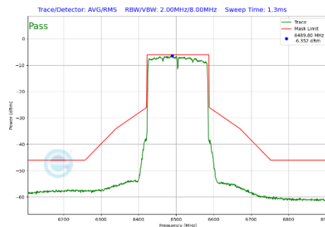
Plot 7-468 In-Band Emission Plot SDM Diversity Antenna 4a (160MHz BW 802.11be(SU) (UNII Band 6) - Ch.111)
