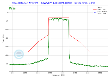
Plot 7-407 In-Band Emission Plot SDM Primary Antenna 4a (80MHz BW 802.11be(SU) (UNII Band 5) - Ch.87)
