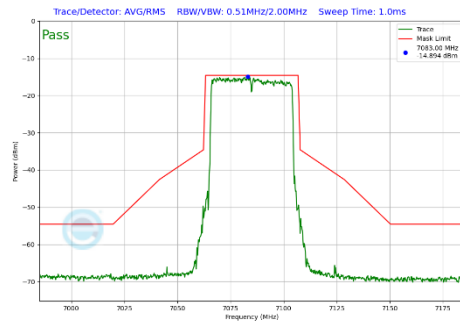
Plot 7-402 In-Band Emission Plot SDM Primary Antenna WF5B (40MHz BW 802.11be(SU) (UNII Band 8) - Ch.227)
