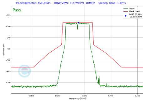
Plot 7-413 In-Band Emission Plot CDD Primary Antenna 4a (20MHz BW 802.11a (UNII Band 7) - Ch.149)
