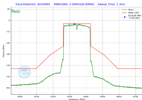
Plot 7-464 In-Band Emission Plot SDM Diversity Antenna 4a (160MHz BW 802.11be(SU) (UNII Band 5) - Ch.79)
