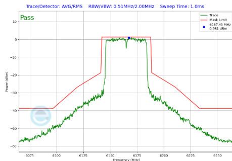
Plot 7-422 In-Band Emission Plot CDD Diversity Antenna 2a (40MHz BW 802.11be(SU) (UNII Band 5) - Ch.43)
