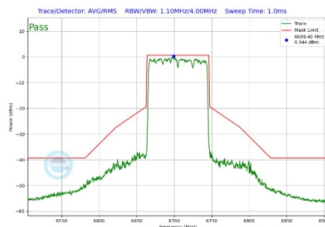
Plot 7-387 In-Band Emission Plot CDD Primary Antenna 4a (80MHz BW 802.11be(SU) (UNII Band 7) - Ch.151)
