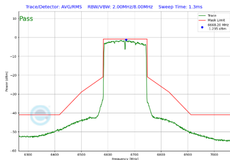
Plot 7-432 In-Band Emission Plot CDD Diversity Antenna 2a (160MHz BW 802.11be(SU) (UNII Band 7) - Ch.143)
