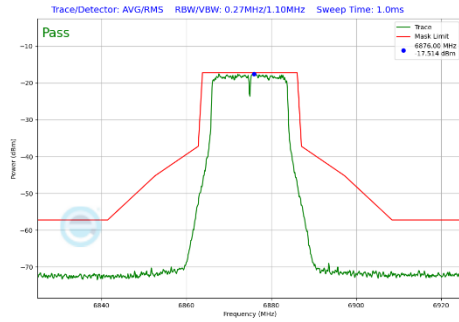
Plot 7-453 In-Band Emission Plot CDD Diversity Antenna 2a (20MHz BW 802.11a (UNII Band 7) - Ch.185)
