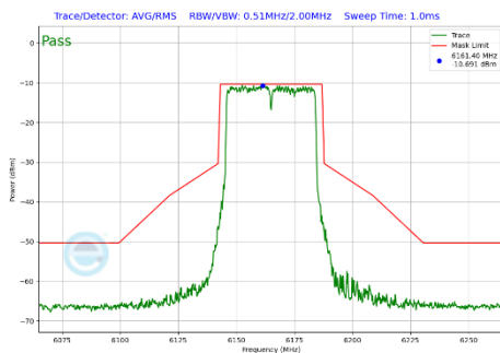
Plot 7-462 In-Band Emission Plot SDM Diversity Antenna 4a (40MHz BW 802.11be(SU) (UNII Band 5) - Ch.43)
