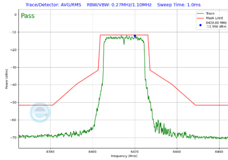
Plot 7-405 In-Band Emission Plot SDM Primary Antenna 4a (20MHz BW 802.11be(SU) (UNII Band 5) - Ch.93)
