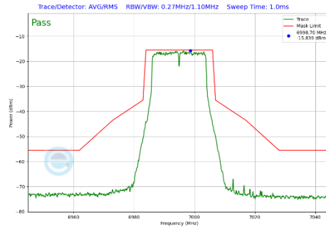
Plot 7-473 In-Band Emission Plot CDD Diversity Antenna 4a (20MHz BW 802.11a (UNII Band 8) - Ch.209)
