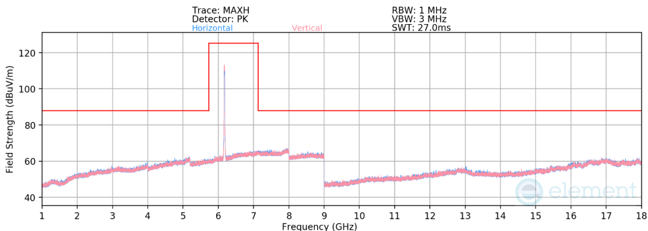
Plot 7-513. Radiated Spurious Emissions 1-18GHz CDD Primary (802.11be – Ch. 45)
