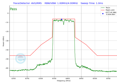
Plot 7-391 In-Band Emission Plot SDM Primary Antenna WF5B (80MHz BW 802.11be(SU) (UNII Band 5) - Ch.87)
