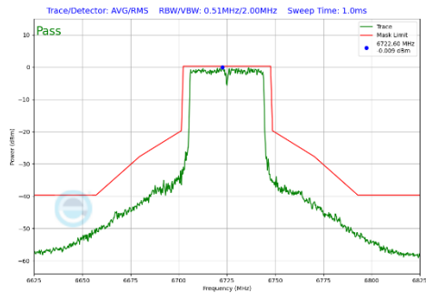
Plot 7-430 In-Band Emission Plot CDD Diversity Antenna 2a (40MHz BW 802.11be(SU) (UNII Band 7) - Ch.155)
