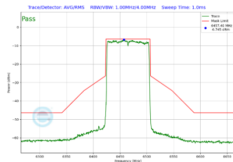
Plot 7-451 In-Band Emission Plot SDM Diversity Antenna 2a (80MHz BW 802.11be(SU) (UNII Band 6) - Ch.103)
