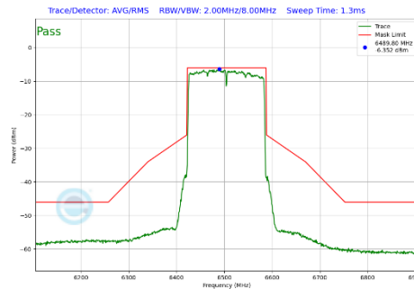
Plot 7-412 In-Band Emission Plot SDM Primary Antenna 4a (160MHz BW 802.11be(SU) (UNII Band 6) - Ch.111)
