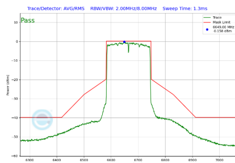
Plot 7-388 In-Band Emission Plot CDD Primary Antenna 4a (160MHz BW 802.11be(SU) (UNII Band 7) - Ch.143)
