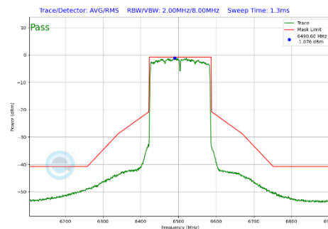
Plot 7-428 In-Band Emission Plot CDD Diversity Antenna 2a (160MHz BW 802.11be(SU) (UNII Band 6) - Ch.111)
