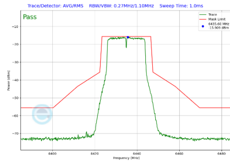
Plot 7-393 In-Band Emission Plot CDD Primary Antenna WF5B (20MHz BW 802.11a (UNII Band 6) - Ch.97)
