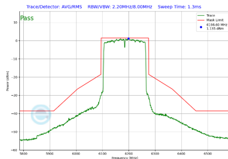
Plot 7-436 In-Band Emission Plot CDD Diversity Antenna 4a (160MHz BW 802.11be(SU) (UNII Band 5) - Ch.47)
