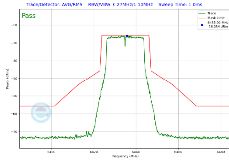
Plot 7-465 In-Band Emission Plot CDD Diversity Antenna 4a (20MHz BW 802.11a (UNII Band 6) - Ch.97)
