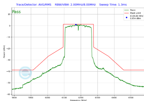
Plot 7-424 In-Band Emission Plot CDD Diversity Antenna 2a (160MHz BW 802.11be(SU) (UNII Band 5) - Ch.47)
