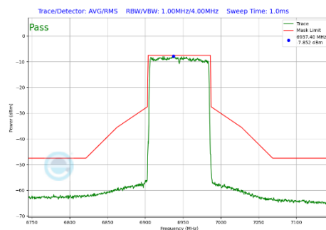
Plot 7-475 In-Band Emission Plot SDM Diversity Antenna 4a (80MHz BW 802.11be(SU) (UNII Band 8) - Ch.199)
