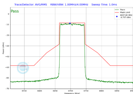
Plot 7-415 In-Band Emission Plot SDM Primary Antenna 4a (80MHz BW 802.11be(SU) (UNII Band 7) - Ch.151)
