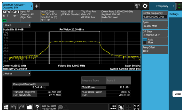
Plot 7-52 26dB BW & 99% OBW Antenna 4a (20MHz BW 802.11be(RU) RU242 Index61 - Ch.61)
