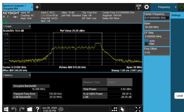
Plot 7-12 26dB BW & 99% OBW Antenna WF5B (20MHz BW 802.11be(RU) RU26 Index8 - Ch.113)
