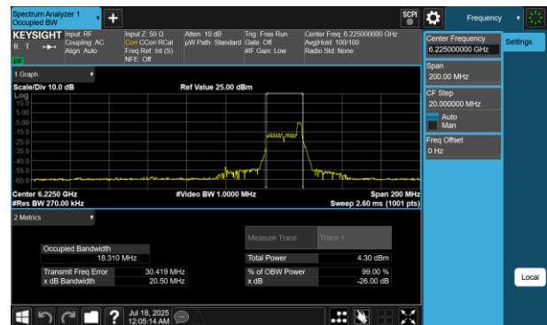
Plot 7-47 26dB BW & 99% OBW Antenna 4a (80MHz BW 802.11be(RU) RU26 Index36 - Ch.55)
