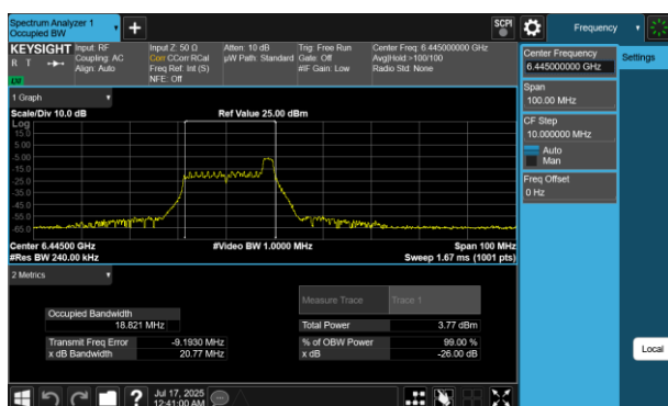
Plot 7-13 26dB BW & 99% OBW Antenna WF5B (40MHz BW 802.11be(RU) RU26 Index8 - Ch.99)
