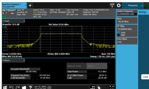
Plot 7-53 26dB BW & 99% OBW Antenna 4a (40MHz BW 802.11be(RU) RU484 Index65 - Ch.59)
