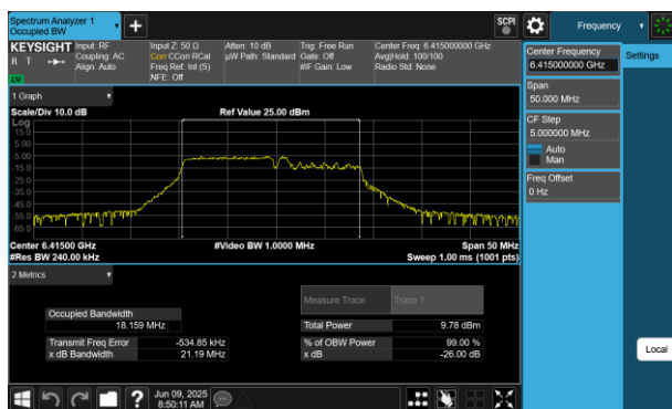
Plot 7-5 26dB BW & 99% OBW Antenna WF5B (20MHz BW 802.11be(RU) RU106+26 Index82 - Ch.93)
