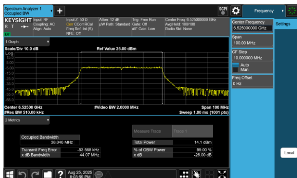
Plot 7-64 26dB BW & 99% OBW Antenna 4a (40MHz BW 802.11be(RU) RU484 Index65 - Ch.115)
