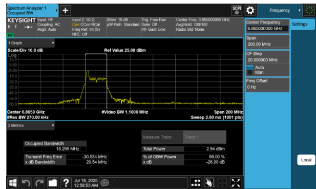
Plot 7-69 26dB BW & 99% OBW Antenna 4a (80MHz BW 802.11be(RU) RU26 Index0 - Ch.183)
