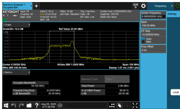
Plot 7-68 26dB BW & 99% OBW Antenna 4a (40MHz BW 802.11be(RU) RU26 Index8 - Ch.123)
