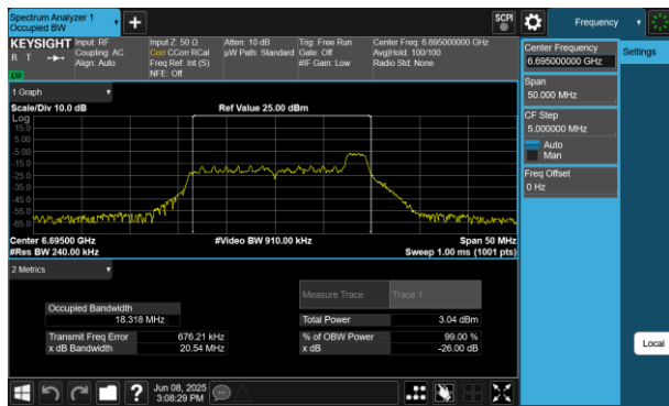
Plot 7-23 26dB BW & 99% OBW Antenna WF5B (20MHz BW 802.11be(RU) RU26 Index8 - Ch.149)
