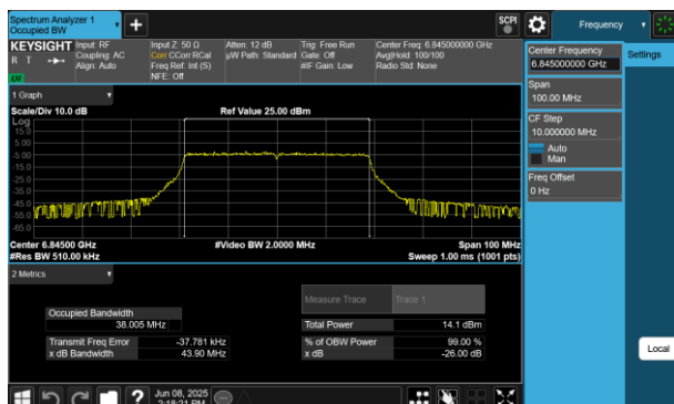
Plot 7-31 26dB BW & 99% OBW Antenna WF5B (40MHz BW 802.11be(RU) RU484 Index65 - Ch.179)
