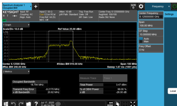
Plot 7-46 26dB BW & 99% OBW Antenna 4a (40MHz BW 802.11be(RU) RU26 Index8 - Ch.35)
