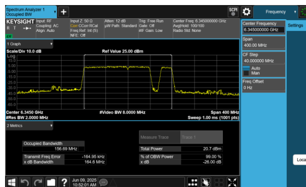
Plot 7-7 26dB BW & 99% OBW Antenna WF5B (160MHz BW 802.11be(RU) RU996+484+242 Index98 - Ch.79)
