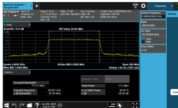
Plot 7-32 26dB BW & 99% OBW Antenna WF5B (80MHz BW 802.11be(RU) RU996 Index67 - Ch.183)
