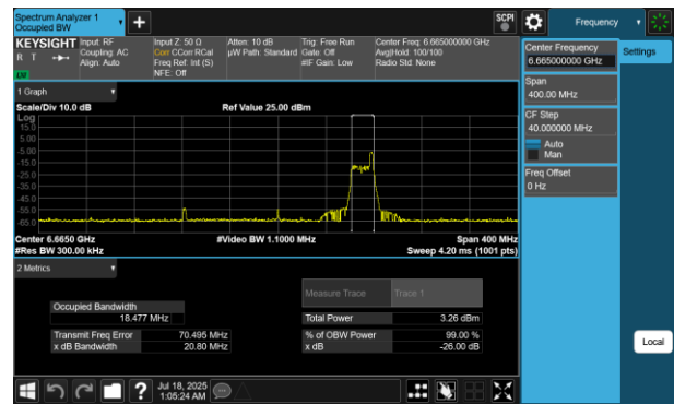
Plot 7-70 26dB BW & 99% OBW Antenna 4a (160MHz BW 802.11be(RU) RU26 Index36 - Ch.143)
