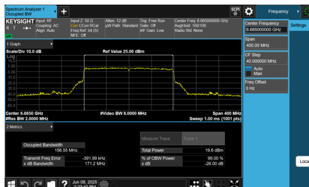
Plot 7-33 26dB BW & 99% OBW Antenna WF5B (160MHz BW 802.11be(RU) RU996X2 Index68 - Ch.143)
