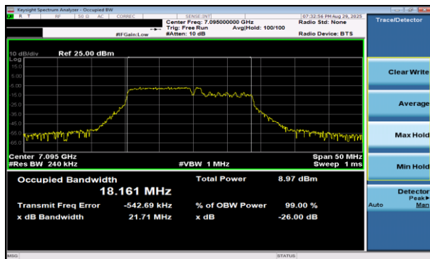
Plot 7-38 26dB BW & 99% OBW Antenna WF5B (20MHz BW 802.11be(RU) RU106+26 Index82 - Ch.229)
