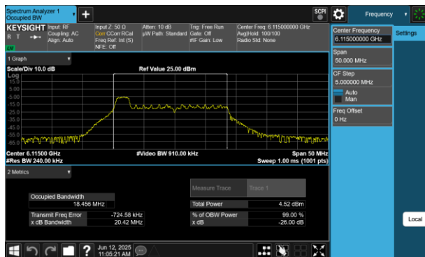
Plot 7-45 26dB BW & 99% OBW Antenna 4a (20MHz BW 802.11be(RU) RU26 Index0 - Ch.33)
