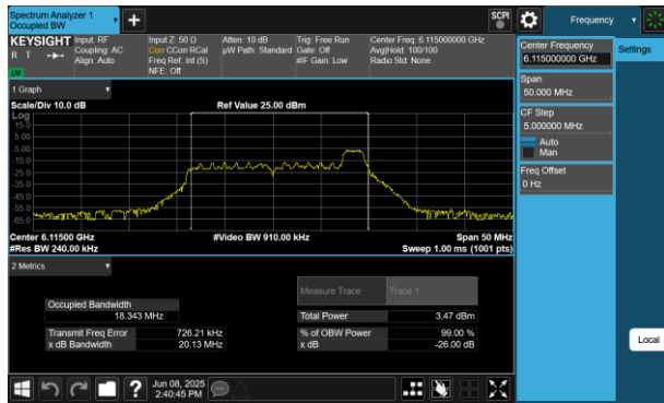
Plot 7-1 26dB BW & 99% OBW Antenna WF5B (20MHz BW 802.11be(RU) RU26 Index8 - Ch.33)
