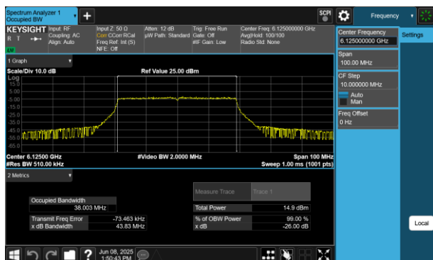
Plot 7-9 26dB BW & 99% OBW Antenna WF5B (40MHz BW 802.11be(RU) RU484 Index65 - Ch.35)
