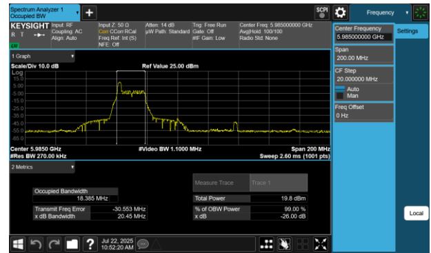
Plot 7-3 26dB BW & 99% OBW Antenna WF5B (80MHz BW 802.11be(RU) RU26 Index0 - Ch.7)
