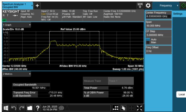
Plot 7-56 26dB BW & 99% OBW Antenna WF5B (20MHz BW 802.11be(RU) RU26 Index0 - Ch.117)
