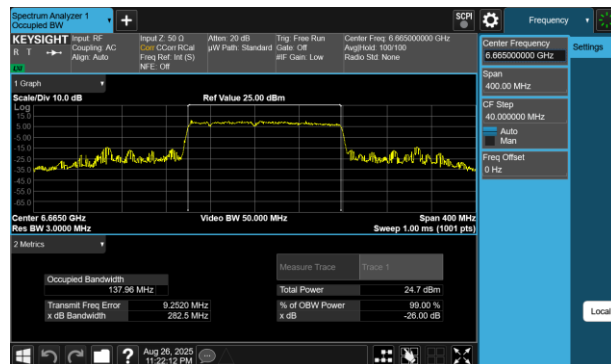
Plot 7-62 26dB BW & 99% OBW Antenna WF5B (160MHz BW 802.11be(RU) RU996+484+242 Index96 - Ch.143)
