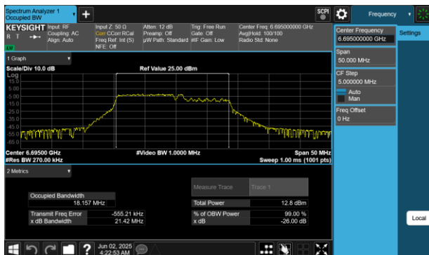
Plot 7-60 26dB BW & 99% OBW Antenna WF5B (20MHz BW 802.11be(RU) RU106+26 Index82 - Ch.149)
