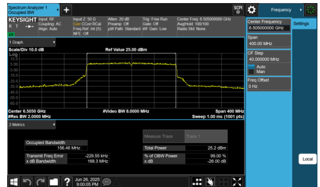
Plot 7-55 26dB BW & 99% OBW Antenna WF5B (160MHz BW 802.11be(RU) RU996X2 Index68 - Ch.111)
