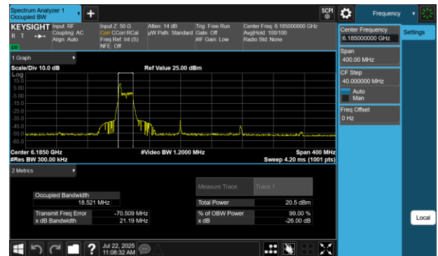
Plot 7-4 26dB BW & 99% OBW Antenna WF5B (160MHz BW 802.11be(RU) RU26 Index0 - Ch.47)
