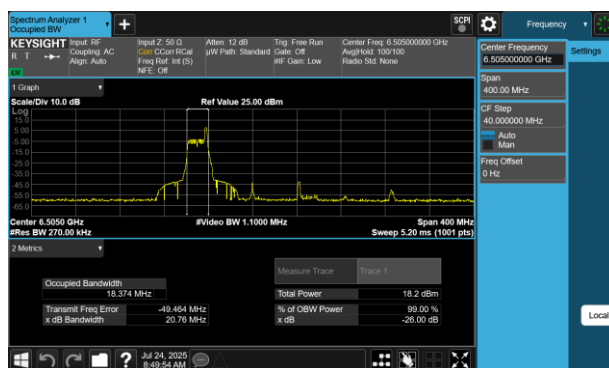
Plot 7-15 26dB BW & 99% OBW Antenna WF5B (160MHz BW 802.11be(RU) RU26 Index17 - Ch.111)
