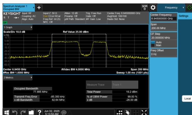
Plot 7-72 26dB BW & 99% OBW Antenna WF5B (80MHz BW 802.11be(RU) RU484+242 Index92 - Ch.199)
