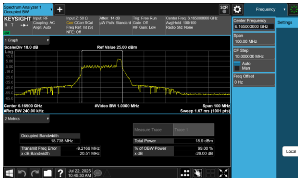
Plot 7-2 26dB BW & 99% OBW Antenna WF5B (40MHz BW 802.11be(RU) RU26 Index8 - Ch.43)
