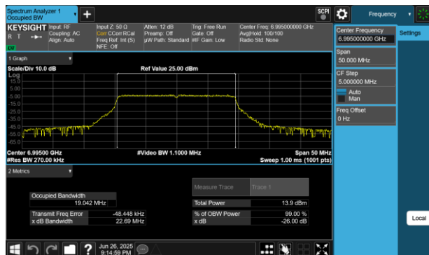
Plot 7-74 26dB BW & 99% OBW Antenna WF5B (20MHz BW 802.11be(RU) RU242 Index61 - Ch.209)
