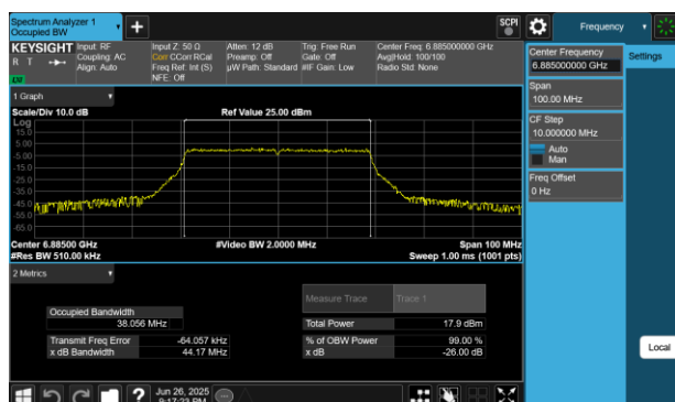
Plot 7-75 26dB BW & 99% OBW Antenna WF5B (40MHz BW 802.11be(RU) RU484 Index65 - Ch.187)
