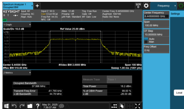
Plot 7-53 26dB BW & 99% OBW Antenna WF5B (40MHz BW 802.11be(RU) RU484 Index65 - Ch.99)
