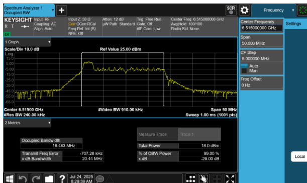
Plot 7-12 26dB BW & 99% OBW Antenna WF5B (20MHz BW 802.11be(RU) RU26 Index0 - Ch.113)
