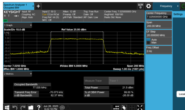
Plot 7-76 26dB BW & 99% OBW Antenna WF5B (80MHz BW 802.11be(RU) RU996 Index67 - Ch.215)
