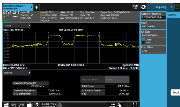
Plot 7-6 26dB BW & 99% OBW Antenna WF5B (80MHz BW 802.11be(RU) RU484+242 Index91 - Ch.87)
