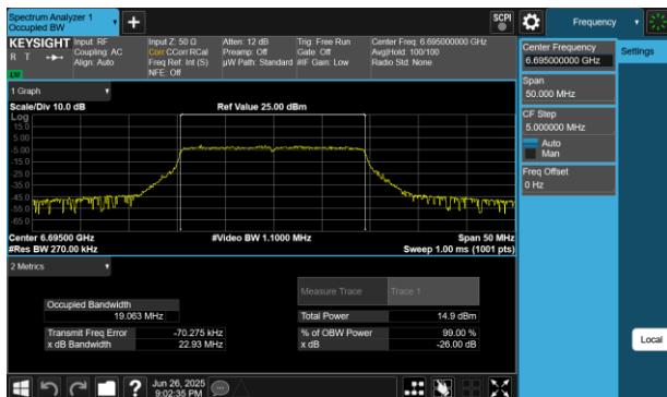
Plot 7-63 26dB BW & 99% OBW Antenna WF5B (20MHz BW 802.11be(RU) RU242 Index61 - Ch.149)
