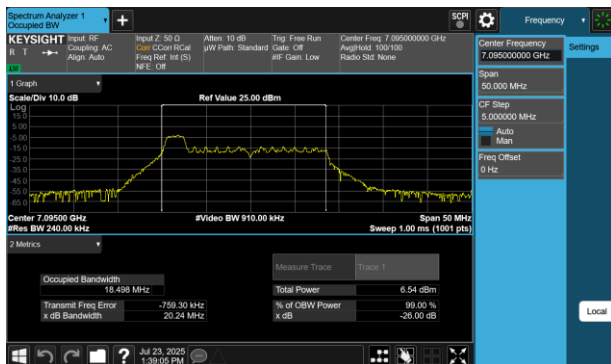
Plot 7-67 26dB BW & 99% OBW Antenna WF5B (20MHz BW 802.11be(RU) RU26 Index0 - Ch.229)
