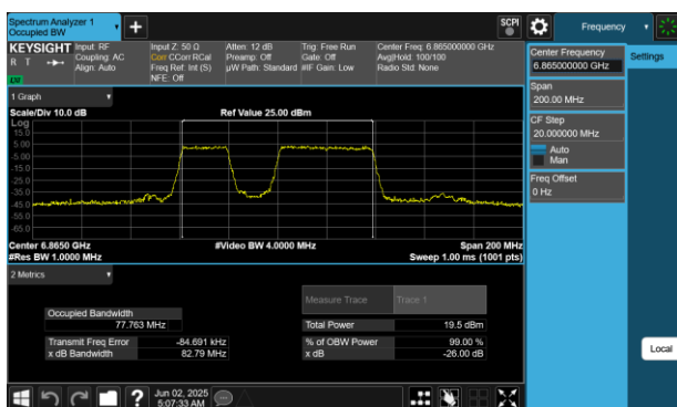
Plot 7-61 26dB BW & 99% OBW Antenna WF5B (80MHz BW 802.11be(RU) RU484+242 Index91 - Ch.183)
