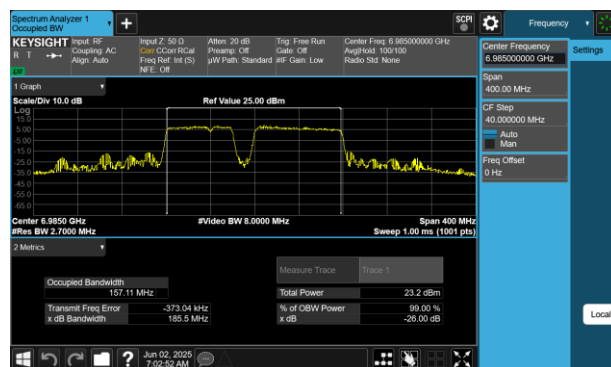
Plot 7-73 26dB BW & 99% OBW Antenna WF5B (160MHz BW 802.11be(RU) RU996+484+242 Index99 - Ch.207)
