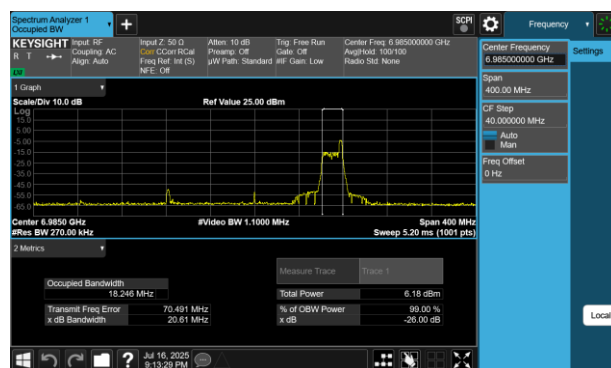
Plot 7-70 26dB BW & 99% OBW Antenna WF5B (160MHz BW 802.11be(RU) RU26 Index36 - Ch.207)
