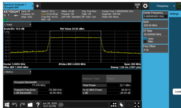
Plot 7-43 26dB BW & 99% OBW Antenna WF5B (80MHz BW 802.11be(RU) RU996 Index67 - Ch.7)
