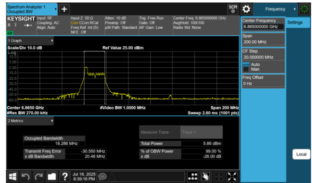
Plot 7-58 26dB BW & 99% OBW Antenna WF5B (80MHz BW 802.11be(RU) RU26 Index0 - Ch.183)
