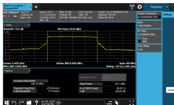
Plot 7-44 26dB BW & 99% OBW Antenna WF5B (160MHz BW 802.11be(RU) RU996X2 Index68 - Ch.79)
