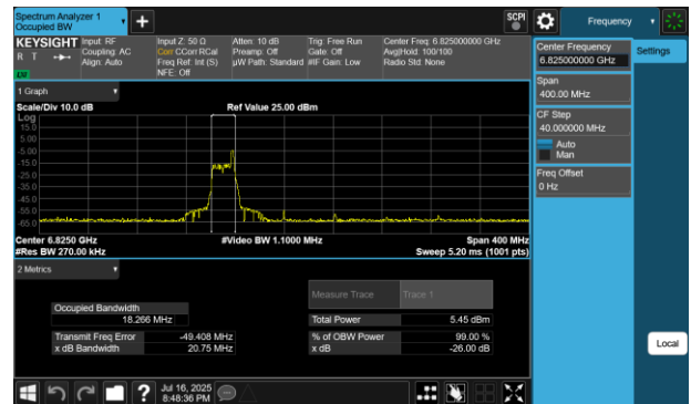
Plot 7-59 26dB BW & 99% OBW Antenna WF5B (160MHz BW 802.11be(RU) RU26 Index17 - Ch.175)
