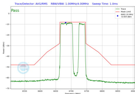
Plot 7-1118 In-Band Emission Plot SDM Primary Antenna 4a (80MHz BW 802.11be(RU) RU484+242 Index92 (UNII Band 7) - Ch.151)
