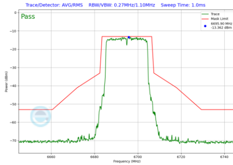
Plot 7-1131 In-Band Emission Plot SDM Primary Antenna WF5B (20MHz BW 802.11be(RU) RU242 Index61 (UNII Band 7) - Ch.149)
