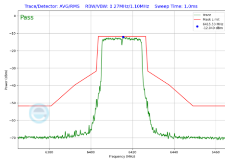
Plot 7-1123 In-Band Emission Plot SDM Primary Antenna WF5B (20MHz BW 802.11be(RU) RU242 Index61 (UNII Band 5) - Ch.93)
