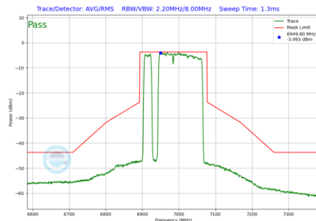
Plot 7-1122 In-Band Emission Plot SDM Primary Antenna 4a (160MHz BW 802.11be(RU) RU996+484+242 Index97 (UNII Band 8) - Ch.207)
