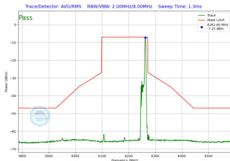
Plot 7-1086 In-Band Emission Plot SDM Primary Antenna 4a (160MHz BW 802.11be(RU) RU26 Index36 (UNII Band 5) - Ch.47)
