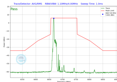
Plot 7-1023 In-Band Emission Plot CDD Primary Antenna 4a (80MHz BW 802.11be(RU) RU26 Index0 (UNII Band 7) - Ch.151)
