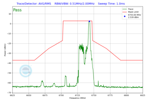
Plot 7-1022 In-Band Emission Plot CDD Primary Antenna 4a (40MHz BW 802.11be(RU) RU26 Index17 (UNII Band 7) - Ch.155)
