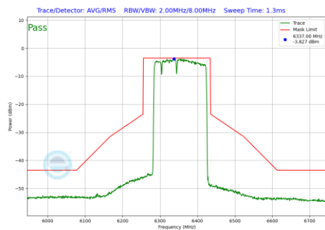
Plot 7-1101 In-Band Emission Plot SDM Primary Antenna WF5B (160MHz BW 802.11be(RU) RU996+484+242 Index96 (UNII Band 5) - Ch.79)
