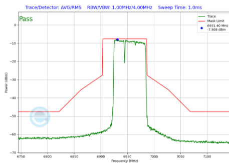
Plot 7-1109 In-Band Emission Plot SDM Primary Antenna WF5B (80MHz BW 802.11be(RU) RU484+242 Index90 (UNII Band 8) - Ch.199)
