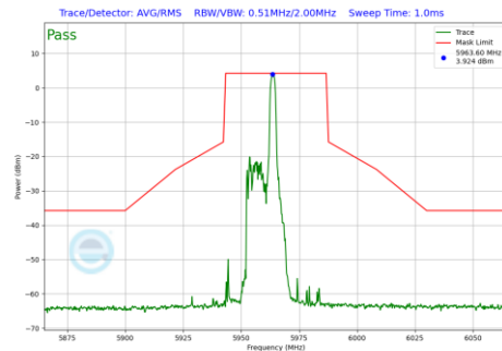
Plot 7-1014 In-Band Emission Plot CDD Primary Antenna 4a (40MHz BW 802.11be(RU) RU26 Index8 (UNII Band 5) - Ch.3)
