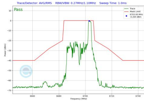
Plot 7-1021 In-Band Emission Plot CDD Primary Antenna 4a (20MHz BW 802.11be(RU) RU26 Index8 (UNII Band 7) - Ch.149)
