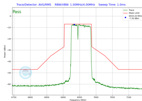
Plot 7-1121 In-Band Emission Plot SDM Primary Antenna 4a (80MHz BW 802.11be(RU) RU484+242 Index90 (UNII Band 8) - Ch.199)
