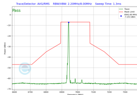
Plot 7-1098 In-Band Emission Plot SDM Primary Antenna 4a (160MHz BW 802.11be(RU) RU26 Index17 (UNII Band 8) - Ch.207)
