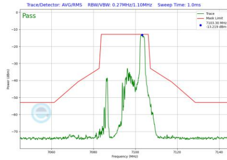
Plot 7-1079 In-Band Emission Plot SDM Primary Antenna WF5B (20MHz BW 802.11be(RU) RU26 Index8 (UNII Band 8) - Ch.229)
