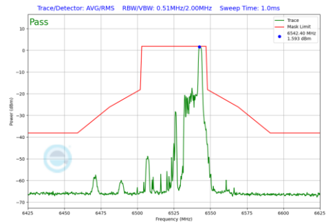
Plot 7-1006 In-Band Emission Plot CDD Primary Antenna WF5B (40MHz BW 802.11be(RU) RU26 Index17 (UNII Band 6) - Ch.115)
