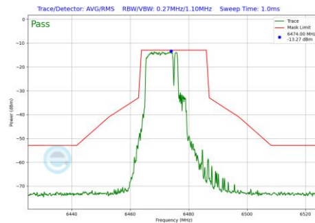
Plot 7-1114 In-Band Emission Plot SDM Primary Antenna 4a (20MHz BW 802.11be(RU) RU106+26 Index82 (UNII Band 6) - Ch.105)
