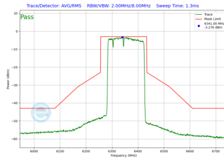
Plot 7-1113 In-Band Emission Plot SDM Primary Antenna 4a (160MHz BW 802.11be(RU) RU996+484+242 Index96 (UNII Band 5) - Ch.79)
