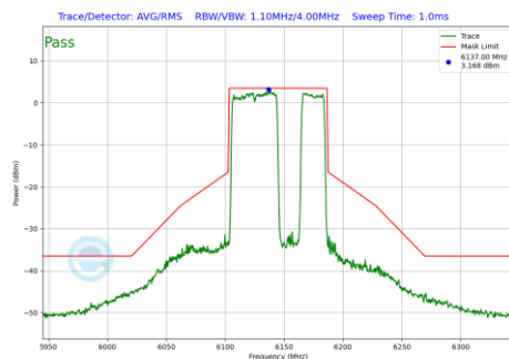
Plot 7-1035 In-Band Emission Plot CDD Primary Antenna 4a (80MHz BW 802.11be(RU) RU484+242 Index92 (UNII Band 5) - Ch.39)
