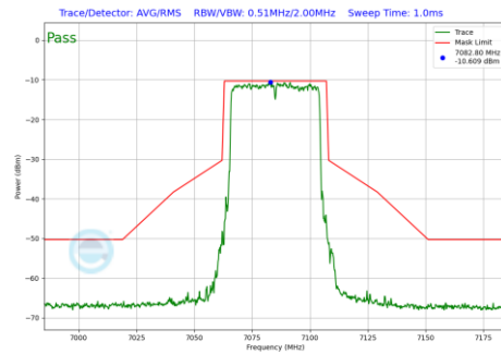
Plot 7-1152 In-Band Emission Plot SDM Primary Antenna 4a (40MHz BW 802.11be(RU) RU484 Index65 (UNII Band 8) - Ch.227)
