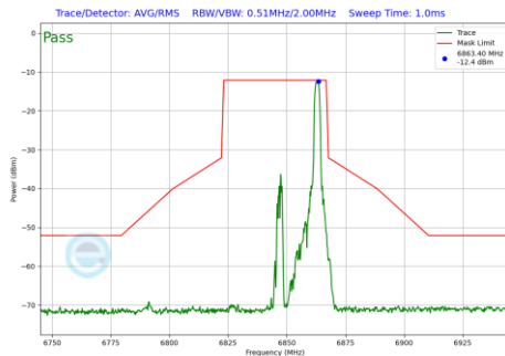
Plot 7-1092 In-Band Emission Plot SDM Primary Antenna 4a (40MHz BW 802.11be(RU) RU26 Index17 (UNII Band 7) - Ch.179)
