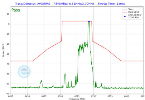
Plot 7-1010 In-Band Emission Plot CDD Primary Antenna WF5B (40MHz BW 802.11be(RU) RU26 Index17 (UNII Band 7) - Ch.155)
