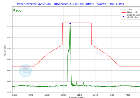
Plot 7-1082 In-Band Emission Plot SDM Primary Antenna WF5B (160MHz BW 802.11be(RU) RU26 Index17 (UNII Band 8) - Ch.207)
