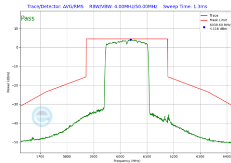
Plot 7-1058 In-Band Emission Plot CDD Primary Antenna 4a (160MHz BW 802.11be(RU) RU996X2 Index68 (UNII Band 5) - Ch.15)
