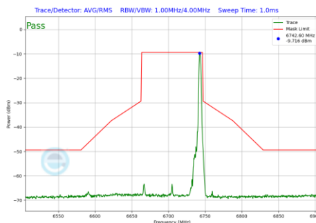
Plot 7-1093 In-Band Emission Plot SDM Primary Antenna 4a (80MHz BW 802.11be(RU) RU26 Index36 (UNII Band 7) - Ch.151)
