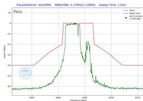
Plot 7-1028 In-Band Emission Plot CDD Primary Antenna WF5B (20MHz BW 802.11be(RU) RU106+26 Index82 (UNII Band 6) - Ch.105)
