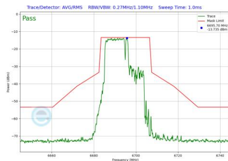
Plot 7-1105 In-Band Emission Plot SDM Primary Antenna WF5B (20MHz BW 802.11be(RU) RU106+26 Index82 (UNII Band 7) - Ch.149)
