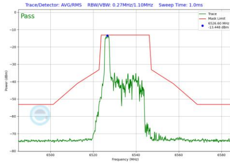
Plot 7-1091 In-Band Emission Plot SDM Primary Antenna 4a (20MHz BW 802.11be(RU) RU26 Index0 (UNII Band 7) - Ch.117)
