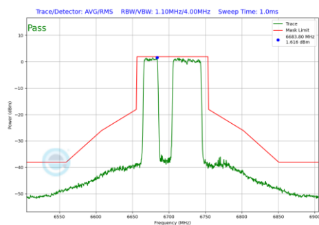
Plot 7-1041 In-Band Emission Plot CDD Primary Antenna 4a (80MHz BW 802.11be(RU) RU484+242 Index91 (UNII Band 7) - Ch.151)
