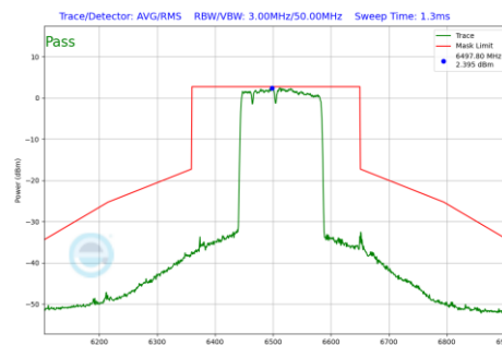
Plot 7-1030 In-Band Emission Plot CDD Primary Antenna WF5B (160MHz BW 802.11be(RU) RU996+484+242 Index96 (UNII Band 6) - Ch.111)
