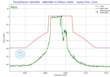
Plot 7-1031 In-Band Emission Plot CDD Primary Antenna WF5B (20MHz BW 802.11be(RU) RU106+26 Index82 (UNII Band 7) - Ch.149)
