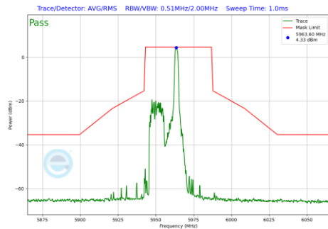
Plot 7-1002 In-Band Emission Plot CDD Primary Antenna WF5B (40MHz BW 802.11be(RU) RU26 Index8 (UNII Band 5) - Ch.3)
