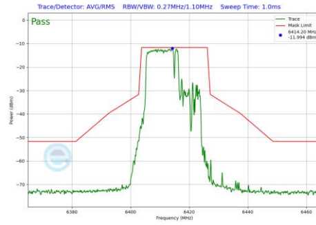
Plot 7-1111 In-Band Emission Plot SDM Primary Antenna 4a (20MHz BW 802.11be(RU) RU106+26 Index82 (UNII Band 5) - Ch.93)
