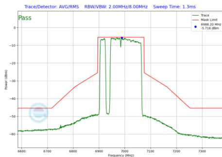
Plot 7-1110 In-Band Emission Plot SDM Primary Antenna WF5B (160MHz BW 802.11be(RU) RU996+484+242 Index97 (UNII Band 8) - Ch.207)
