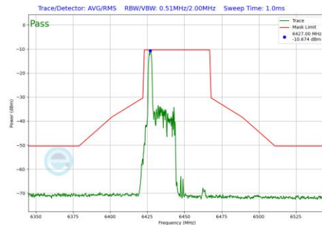
Plot 7-1088 In-Band Emission Plot SDM Primary Antenna 4a (40MHz BW 802.11be(RU) RU26 Index0 (UNII Band 6) - Ch.99)
