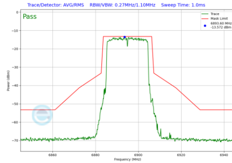
Plot 7-1151 In-Band Emission Plot SDM Primary Antenna 4a (20MHz BW 802.11be(RU) RU242 Index61 (UNII Band 8) - Ch.189)
