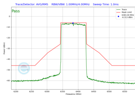
Plot 7-1141 In-Band Emission Plot SDM Primary Antenna 4a (80MHz BW 802.11be(RU) RU996 Index67 (UNII Band 5) - Ch.87)
