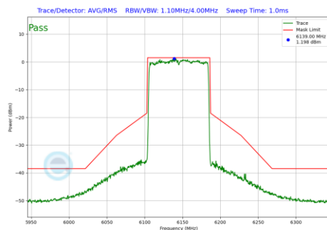
Plot 7-1045 In-Band Emission Plot CDD Primary Antenna WF5B (80MHz BW 802.11be(RU) RU996 Index67 (UNII Band 5) - Ch.39)
