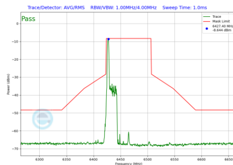
Plot 7-1073 In-Band Emission Plot SDM Primary Antenna WF5B (80MHz BW 802.11be(RU) RU26 Index0 (UNII Band 6) - Ch.103)
