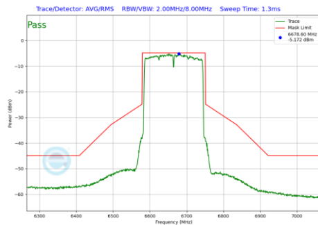
Plot 7-1150 In-Band Emission Plot SDM Primary Antenna 4a (160MHz BW 802.11be(RU) RU996X2 Index68 (UNII Band 7) - Ch.143)
