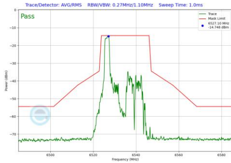
Plot 7-1075 In-Band Emission Plot SDM Primary Antenna WF5B (20MHz BW 802.11be(RU) RU26 Index0 (UNII Band 7) - Ch.117)
