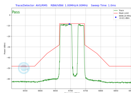
Plot 7-1106 In-Band Emission Plot SDM Primary Antenna WF5B (80MHz BW 802.11be(RU) RU484+242 Index92 (UNII Band 7) - Ch.151)
