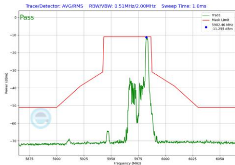
Plot 7-1084 In-Band Emission Plot SDM Primary Antenna 4a (40MHz BW 802.11be(RU) RU26 Index17 (UNII Band 5) - Ch.3)
