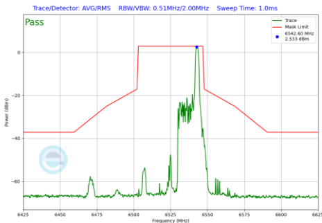
Plot 7-1018 In-Band Emission Plot CDD Primary Antenna 4a (40MHz BW 802.11be(RU) RU26 Index17 (UNII Band 6) - Ch.115)
