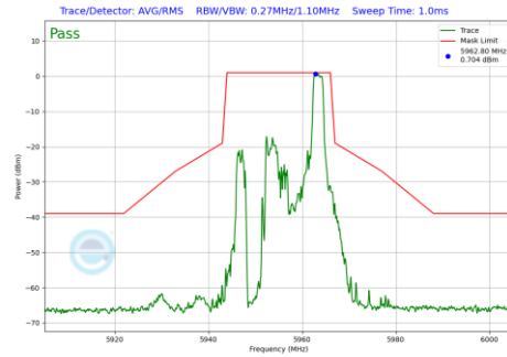
Plot 7-1013 In-Band Emission Plot CDD Primary Antenna 4a (20MHz BW 802.11be(RU) RU26 Index8 (UNII Band 5) - Ch.1)
