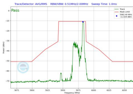
Plot 7-1068 In-Band Emission Plot SDM Primary Antenna WF5B (40MHz BW 802.11be(RU) RU26 Index17 (UNII Band 5) - Ch.3)
