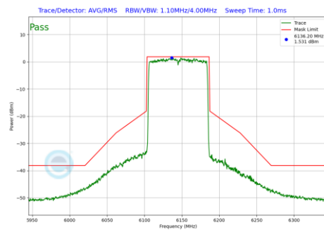
Plot 7-1057 In-Band Emission Plot CDD Primary Antenna 4a (80MHz BW 802.11be(RU) RU996 Index67 (UNII Band 5) - Ch.39)
