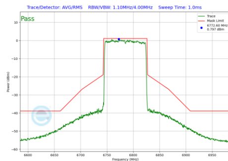
Plot 7-1065 In-Band Emission Plot CDD Primary Antenna 4a (80MHz BW 802.11be(RU) RU996 Index67 (UNII Band 7) - Ch.167)
