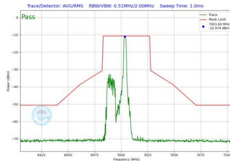
Plot 7-1096 In-Band Emission Plot SDM Primary Antenna 4a (40MHz BW 802.11be(RU) RU26 Index8 (UNII Band 8) - Ch.211)
