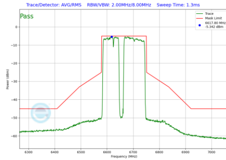
Plot 7-1119 In-Band Emission Plot SDM Primary Antenna 4a (160MHz BW 802.11be(RU) RU996+484+242 Index99 (UNII Band 7) - Ch.143)
