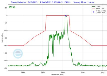
Plot 7-1017 In-Band Emission Plot CDD Primary Antenna 4a (20MHz BW 802.11be(RU) RU26 Index8 (UNII Band 6) - Ch.105)
