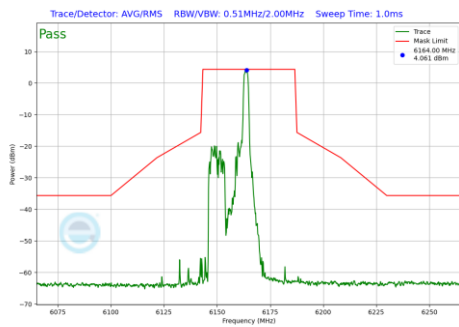
Plot 7-1156 In-Band Emission Plot CDD Diversity Antenna 2a (40MHz BW 802.11be(RU) RU26 Index8 (UNII Band 5) - Ch.43)
