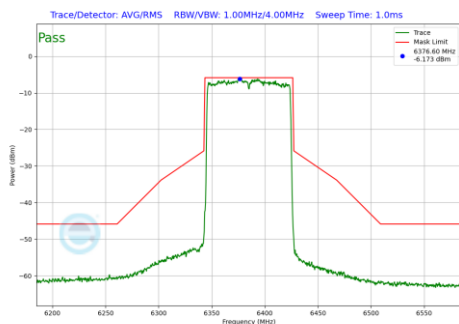
Plot 7-1125 In-Band Emission Plot SDM Primary Antenna WF5B (80MHz BW 802.11be(RU) RU996 Index67 (UNII Band 5) - Ch.87)
