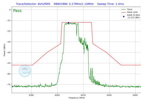
Plot 7-1099 In-Band Emission Plot SDM Primary Antenna WF5B (20MHz BW 802.11be(RU) RU106+26 Index82 (UNII Band 5) - Ch.93)
