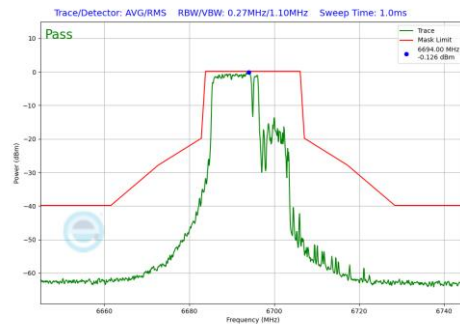
Plot 7-1040 In-Band Emission Plot CDD Primary Antenna 4a (20MHz BW 802.11be(RU) RU106+26 Index82 (UNII Band 7) - Ch.149)
