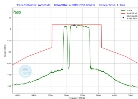
Plot 7-1042 In-Band Emission Plot CDD Primary Antenna 4a (160MHz BW 802.11be(RU) RU996+484+242 Index97 (UNII Band 7) - Ch.143)
