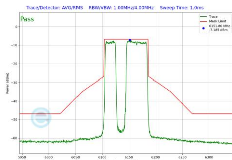
Plot 7-1100 In-Band Emission Plot SDM Primary Antenna WF5B (80MHz BW 802.11be(RU) RU484+242 Index91 (UNII Band 5) - Ch.39)
