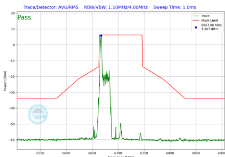
Plot 7-1011 In-Band Emission Plot CDD Primary Antenna WF5B (80MHz BW 802.11be(RU) RU26 Index0 (UNII Band 7) - Ch.151)
