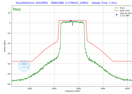
Plot 7-1055 In-Band Emission Plot CDD Primary Antenna 4a (20MHz BW 802.11be(RU) RU242 Index61 (UNII Band 5) - Ch.1)
