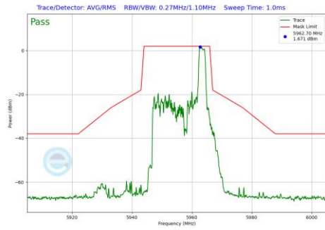
Plot 7-1001 In-Band Emission Plot SDM Primary Antenna WF5B (20MHz BW 802.11be(RU) RU26 Index8 (UNII Band 5) - Ch.1)
