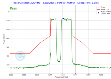
Plot 7-1112 In-Band Emission Plot SDM Primary Antenna 4a (80MHz BW 802.11be(RU) RU484+242 Index91 (UNII Band 5) - Ch.39)
