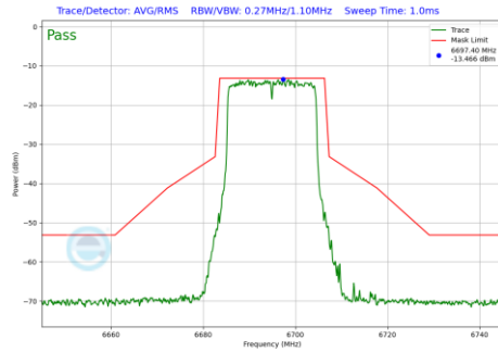
Plot 7-1147 In-Band Emission Plot SDM Primary Antenna 4a (20MHz BW 802.11be(RU) RU242 Index61 (UNII Band 7) - Ch.149)
