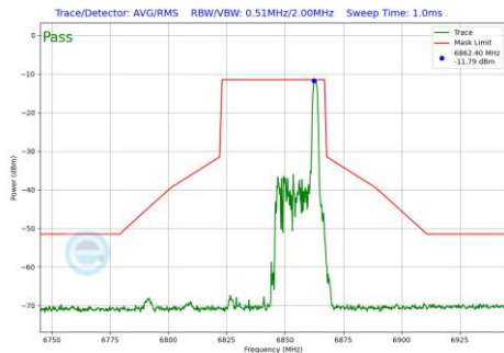
Plot 7-1076 In-Band Emission Plot SDM Primary Antenna WF5B (40MHz BW 802.11be(RU) RU26 Index17 (UNII Band 7) - Ch.179)
