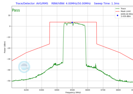
Plot 7-1039 In-Band Emission Plot CDD Primary Antenna 4a (160MHz BW 802.11be(RU) RU996+484+242 Index96 (UNII Band 6) - Ch.111)
