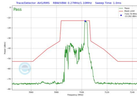
Plot 7-1095 In-Band Emission Plot SDM Primary Antenna 4a (20MHz BW 802.11be(RU) RU26 Index8 (UNII Band 8) - Ch.229)
