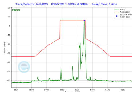
Plot 7-1015 In-Band Emission Plot CDD Primary Antenna 4a (80MHz BW 802.11be(RU) RU26 Index36 (UNII Band 5) - Ch.7)
