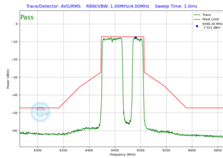
Plot 7-1103 In-Band Emission Plot SDM Primary Antenna WF5B (80MHz BW 802.11be(RU) RU484+242 Index92 (UNII Band 6) - Ch.103)
