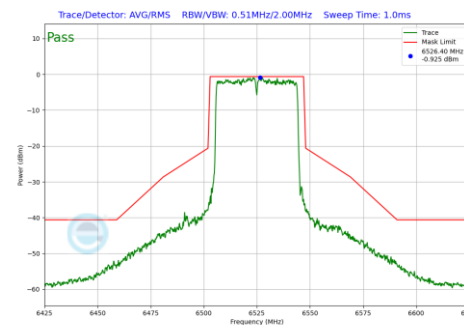
Plot 7-1048 In-Band Emission Plot CDD Primary Antenna WF5B (40MHz BW 802.11be(RU) RU484 Index65 (UNII Band 6) - Ch.115)
