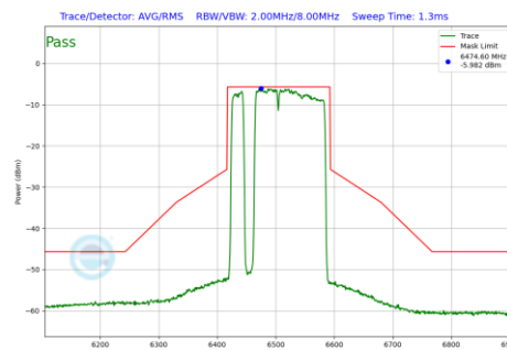
Plot 7-1104 In-Band Emission Plot SDM Primary Antenna WF5B (160MHz BW 802.11be(RU) RU996+484+242 Index97 (UNII Band 6) - Ch.111)
