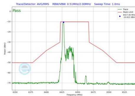
Plot 7-1072 In-Band Emission Plot SDM Primary Antenna WF5B (40MHz BW 802.11be(RU) RU26 Index0 (UNII Band 6) - Ch.99)
