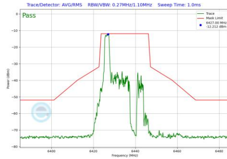
Plot 7-1087 In-Band Emission Plot SDM Primary Antenna 4a (20MHz BW 802.11be(RU) RU26 Index0 (UNII Band 6) - Ch.97)
