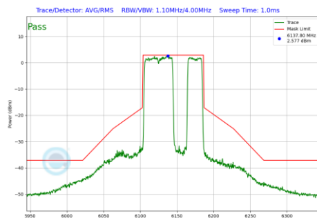
Plot 7-1026 In-Band Emission Plot CDD Primary Antenna WF5B (80MHz BW 802.11be(RU) RU484+242 Index92 (UNII Band 5) - Ch.39)
