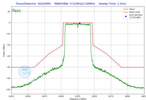
Plot 7-1060 In-Band Emission Plot CDD Primary Antenna 4a (40MHz BW 802.11be(RU) RU484 Index65 (UNII Band 6) - Ch.115)
