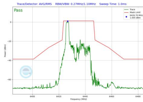
Plot 7-1159 In-Band Emission Plot CDD Diversity Antenna 2a (20MHz BW 802.11be(RU) RU26 Index0 (UNII Band 6) - Ch.97)
