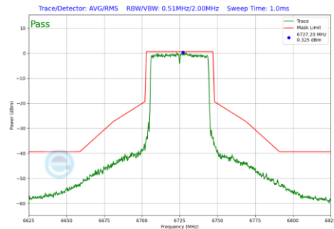
Plot 7-1064 In-Band Emission Plot CDD Primary Antenna 4a (40MHz BW 802.11be(RU) RU484 Index65 (UNII Band 7) - Ch.155)
