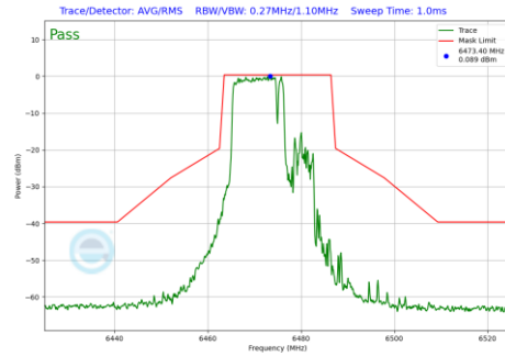
Plot 7-1037 In-Band Emission Plot CDD Primary Antenna 4a (20MHz BW 802.11be(RU) RU106+26 Index82 (UNII Band 6) - Ch.105)
