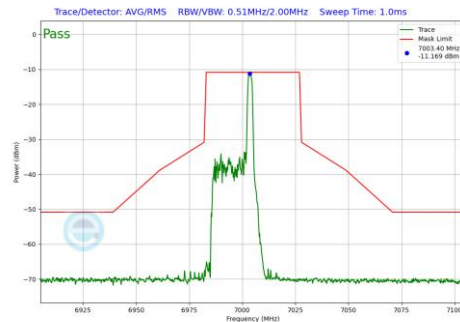
Plot 7-1080 In-Band Emission Plot SDM Primary Antenna WF5B (40MHz BW 802.11be(RU) RU26 Index8 (UNII Band 8) - Ch.211)
