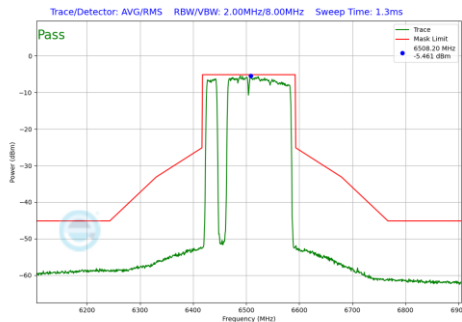
Plot 7-1116 In-Band Emission Plot SDM Primary Antenna 4a (160MHz BW 802.11be(RU) RU996+484+242 Index97 (UNII Band 6) - Ch.111)
