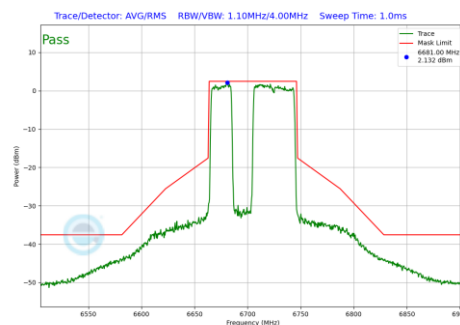
Plot 7-1032 In-Band Emission Plot CDD Primary Antenna WF5B (80MHz BW 802.11be(RU) RU484+242 Index91 (UNII Band 7) - Ch.151)
