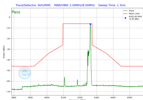
Plot 7-1070 In-Band Emission Plot SDM Primary Antenna WF5B (160MHz BW 802.11be(RU) RU26 Index36 (UNII Band 5) - Ch.47)
