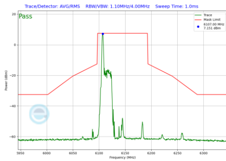
Plot 7-1157 In-Band Emission Plot CDD Diversity Antenna 2a (80MHz BW 802.11be(RU) RU26 Index0 (UNII Band 5) - Ch.39)
