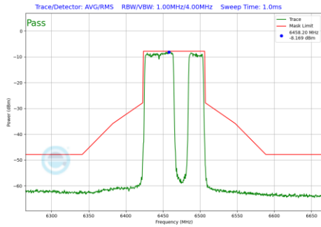
Plot 7-1115 In-Band Emission Plot SDM Primary Antenna 4a (80MHz BW 802.11be(RU) RU484+242 Index92 (UNII Band 6) - Ch.103)
