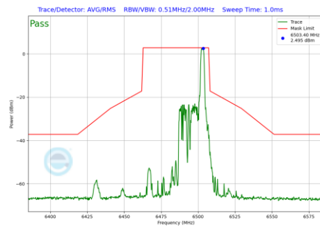
Plot 7-1160 In-Band Emission Plot CDD Diversity Antenna 2a (40MHz BW 802.11be(RU) RU26 Index17 (UNII Band 6) - Ch.107)
