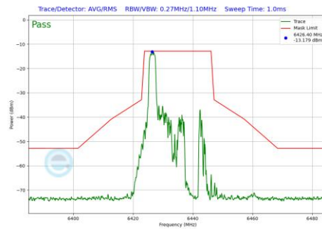
Plot 7-1071 In-Band Emission Plot SDM Primary Antenna WF5B (20MHz BW 802.11be(RU) RU26 Index0 (UNII Band 6) - Ch.97)
