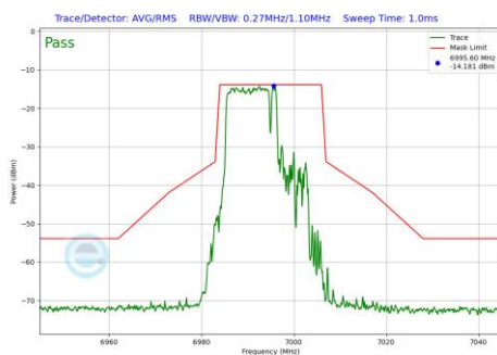
Plot 7-1108 In-Band Emission Plot SDM Primary Antenna WF5B (20MHz BW 802.11be(RU) RU106+26 Index82 (UNII Band 8) - Ch.209)
