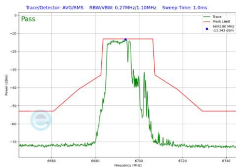
Plot 7-1117 In-Band Emission Plot SDM Primary Antenna 4a (20MHz BW 802.11be(RU) RU106+26 Index82 (UNII Band 7) - Ch.149)
