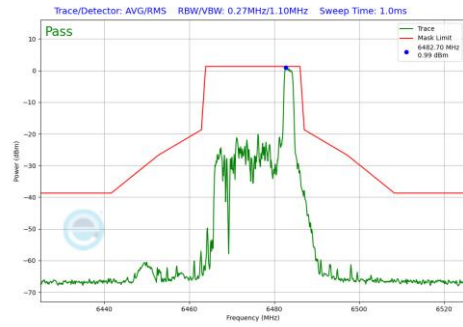
Plot 7-1005 In-Band Emission Plot CDD Primary Antenna WF5B (20MHz BW 802.11be(RU) RU26 Index8 (UNII Band 6) - Ch.105)
