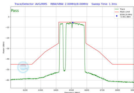
Plot 7-1270 In-Band Emission Plot SDM Diversity Antenna 4a (160MHz BW 802.11be(RU) RU996+484+242 Index97 (UNII Band 6) - Ch.111)
