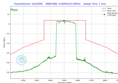
Plot 7-1193 In-Band Emission Plot CDD Diversity Antenna 4a (160MHz BW 802.11be(RU) RU996+484+242 Index96 (UNII Band 6) - Ch.111)
