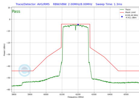
Plot 7-1280 In-Band Emission Plot SDM Diversity Antenna 2a (160MHz BW 802.11be(RU) RU996X2 Index68 (UNII Band 5) - Ch.47)
