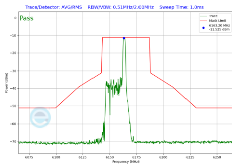
Plot 7-1222 In-Band Emission Plot SDM Diversity Antenna 2a (40MHz BW 802.11be(RU) RU26 Index8 (UNII Band 5) - Ch.43)
