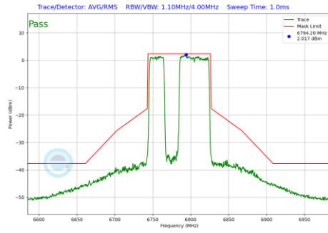
Plot 7-1195 In-Band Emission Plot CDD Diversity Antenna 4a (80MHz BW 802.11be(RU) RU484+242 Index91 (UNII Band 7) - Ch.167)
