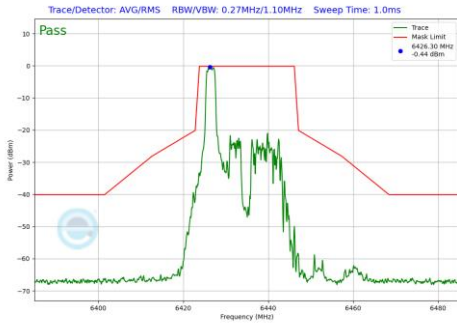
Plot 7-1171 In-Band Emission Plot CDD Diversity Antenna 4a (20MHz BW 802.11be(RU) RU26 Index0 (UNII Band 6) - Ch.97)
