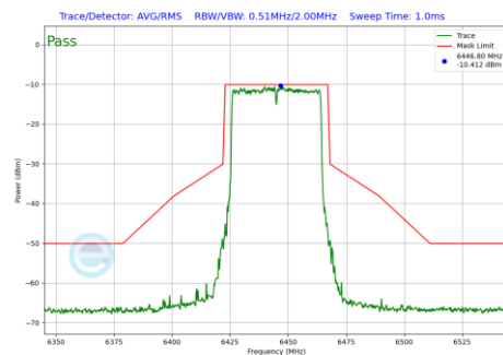
Plot 7-1282 In-Band Emission Plot SDM Diversity Antenna 2a (40MHz BW 802.11be(RU) RU484 Index65 (UNII Band 6) - Ch.99)
