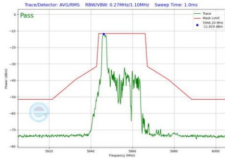
Plot 7-1237 In-Band Emission Plot SDM Diversity Antenna 4a (20MHz BW 802.11be(RU) RU26 Index0 (UNII Band 5) - Ch.1)
