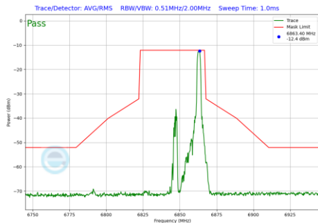
Plot 7-1246 In-Band Emission Plot SDM Diversity Antenna 4a (40MHz BW 802.11be(RU) RU26 Index17 (UNII Band 7) - Ch.179)
