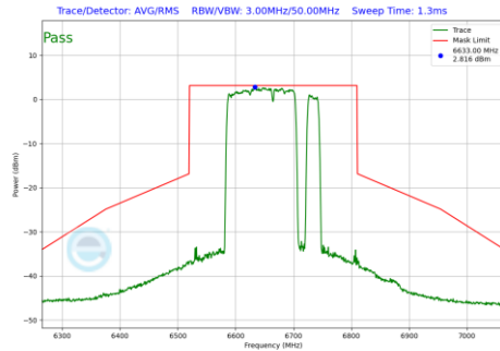
Plot 7-1187 In-Band Emission Plot CDD Diversity Antenna 2a (160MHz BW 802.11be(RU) RU996+484+242 Index98 (UNII Band 7) - Ch.143)
