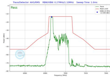
Plot 7-1249 In-Band Emission Plot SDM Diversity Antenna 4a (20MHz BW 802.11be(RU) RU26 Index0 (UNII Band 8) - Ch.209)
