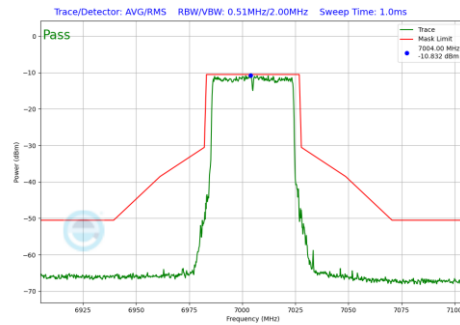
Plot 7-1306 In-Band Emission Plot SDM Diversity Antenna 4a (40MHz BW 802.11be(RU) RU484 Index65 (UNII Band 8) - Ch.211)
