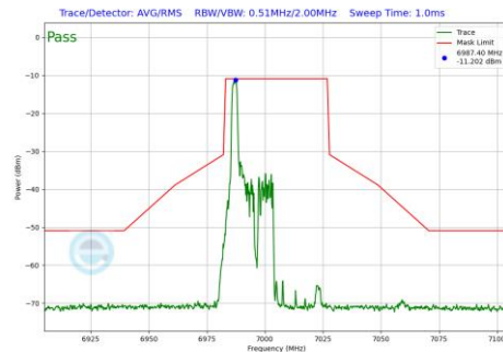
Plot 7-1250 In-Band Emission Plot SDM Diversity Antenna 4a (40MHz BW 802.11be(RU) RU26 Index0 (UNII Band 8) - Ch.211)
