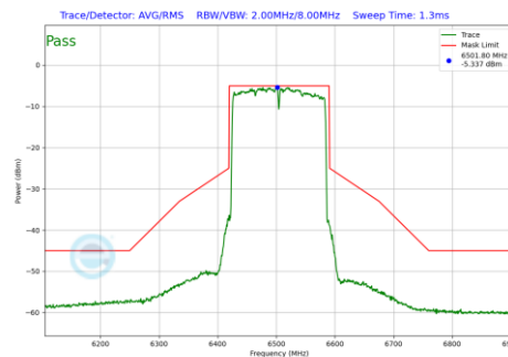
Plot 7-1284 In-Band Emission Plot SDM Diversity Antenna 2a (160MHz BW 802.11be(RU) RU996X2 Index68 (UNII Band 6) - Ch.111)
