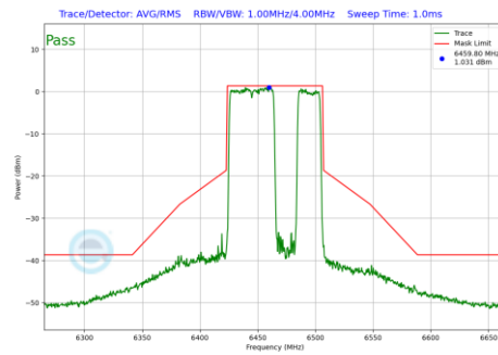
Plot 7-1183 In-Band Emission Plot CDD Diversity Antenna 2a (80MHz BW 802.11be(RU) RU484+242 Index92 (UNII Band 6) - Ch.103)
