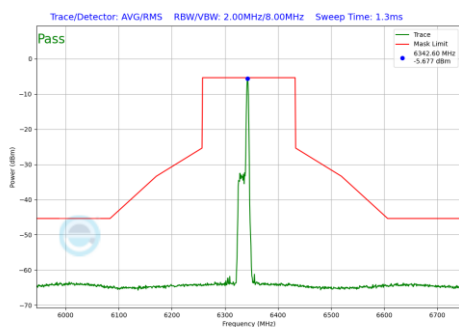
Plot 7-1224 In-Band Emission Plot SDM Diversity Antenna 2a (160MHz BW 802.11be(RU) RU26 Index36 (UNII Band 5) - Ch.79)
