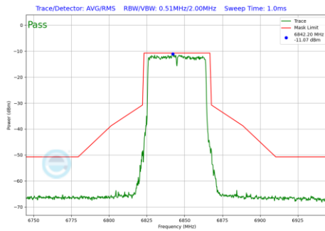
Plot 7-1302 In-Band Emission Plot SDM Diversity Antenna 4a (40MHz BW 802.11be(RU) RU484 Index65 (UNII Band 7) - Ch.179)
