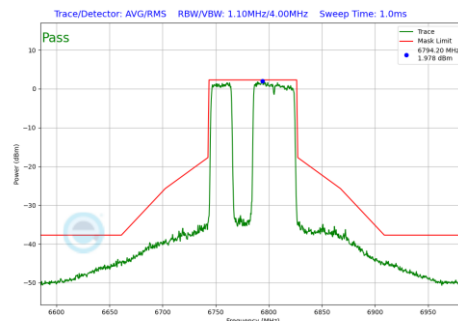
Plot 7-1186 In-Band Emission Plot CDD Diversity Antenna 2a (80MHz BW 802.11be(RU) RU484+242 Index91 (UNII Band 7) - Ch.167)
