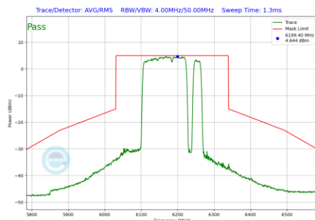
Plot 7-1190 In-Band Emission Plot CDD Diversity Antenna 4a (160MHz BW 802.11be(RU) RU996+484+242 Index98 (UNII Band 5) - Ch.47)
