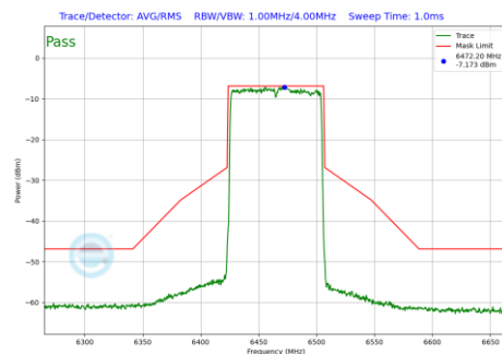
Plot 7-1283 In-Band Emission Plot SDM Diversity Antenna 2a (80MHz BW 802.11be(RU) RU996 Index67 (UNII Band 6) - Ch.103)
