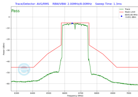
Plot 7-1288 In-Band Emission Plot SDM Diversity Antenna 2a (160MHz BW 802.11be(RU) RU996X2 Index68 (UNII Band 7) - Ch.143)
