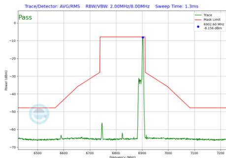
Plot 7-1248 In-Band Emission Plot SDM Diversity Antenna 4a (160MHz BW 802.11be(RU) RU26 Index36 (UNII Band 7) - Ch.175)
