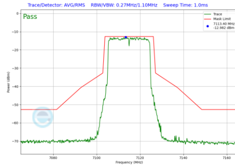
Plot 7-1305 In-Band Emission Plot SDM Diversity Antenna 4a (20MHz BW 802.11be(RU) RU242 Index61 (UNII Band 8) - Ch.233)
