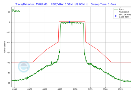
Plot 7-1202 In-Band Emission Plot CDD Diversity Antenna 2a (40MHz BW 802.11be(RU) RU484 Index65 (UNII Band 6) - Ch.99)
