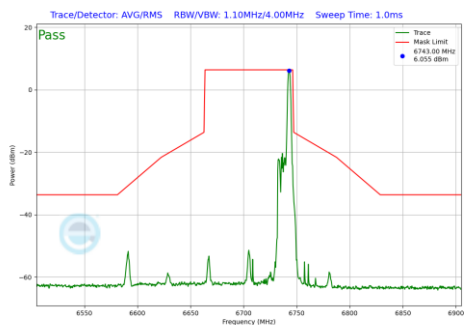
Plot 7-1165 In-Band Emission Plot CDD Diversity Antenna 2a (80MHz BW 802.11be(RU) RU26 Index36 (UNII Band 7) - Ch.151)
