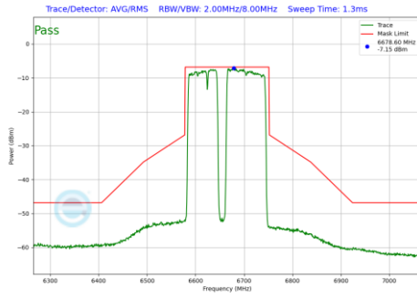
Plot 7-1261 In-Band Emission Plot SDM Diversity Antenna 2a (160MHz BW 802.11be(RU) RU996+484+242 Index99 (UNII Band 7) - Ch.143)
