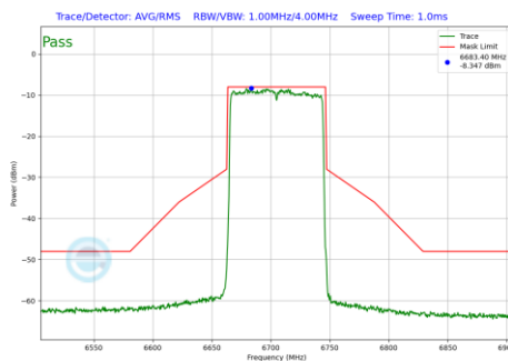
Plot 7-1303 In-Band Emission Plot SDM Diversity Antenna 4a (80MHz BW 802.11be(RU) RU996 Index67 (UNII Band 7) - Ch.151)
