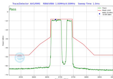
Plot 7-1272 In-Band Emission Plot SDM Diversity Antenna 4a (80MHz BW 802.11be(RU) RU484+242 Index92 (UNII Band 7) - Ch.151)
