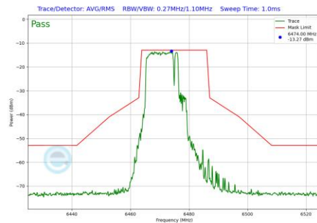
Plot 7-1268 In-Band Emission Plot SDM Diversity Antenna 4a (20MHz BW 802.11be(RU) RU106+26 Index82 (UNII Band 6) - Ch.105)
