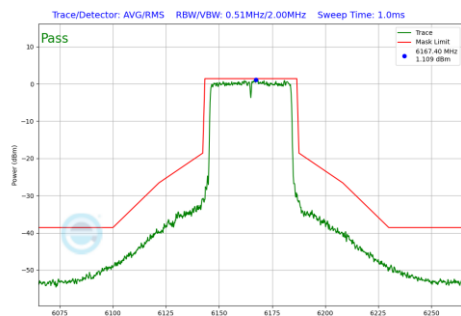
Plot 7-1198 In-Band Emission Plot CDD Diversity Antenna 2a (40MHz BW 802.11be(RU) RU484 Index65 (UNII Band 5) - Ch.43)
