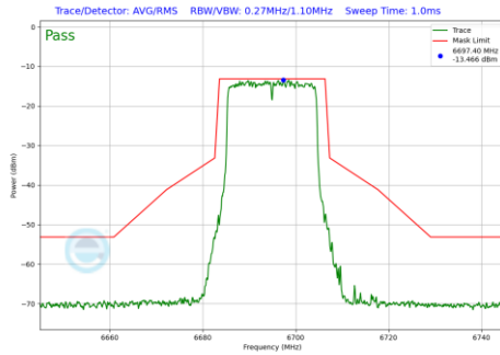
Plot 7-1301 In-Band Emission Plot SDM Diversity Antenna 4a (20MHz BW 802.11be(RU) RU242 Index61 (UNII Band 7) - Ch.149)
