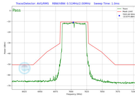
Plot 7-1290 In-Band Emission Plot SDM Diversity Antenna 2a (40MHz BW 802.11be(RU) RU484 Index65 (UNII Band 8) - Ch.211)
