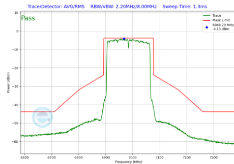
Plot 7-1308 In-Band Emission Plot SDM Diversity Antenna 4a (160MHz BW 802.11be(RU) RU996X2 Index68 (UNII Band 8) - Ch.207)
