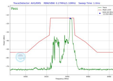
Plot 7-1225 In-Band Emission Plot SDM Diversity Antenna 2a (20MHz BW 802.11be(RU) RU26 Index8 (UNII Band 6) - Ch.97)
