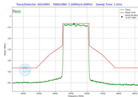
Plot 7-1299 In-Band Emission Plot SDM Diversity Antenna 4a (80MHz BW 802.11be(RU) RU996 Index67 (UNII Band 6) - Ch.103)
