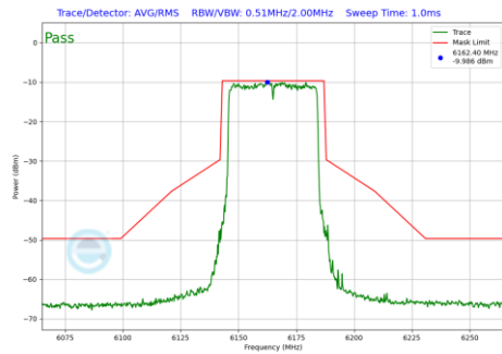
Plot 7-1294 In-Band Emission Plot SDM Diversity Antenna 4a (40MHz BW 802.11be(RU) RU484 Index65 (UNII Band 5) - Ch.43)
