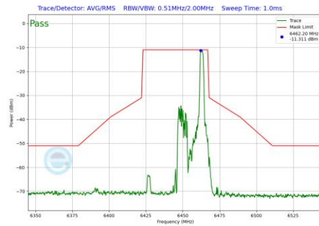
Plot 7-1242 In-Band Emission Plot SDM Diversity Antenna 4a (40MHz BW 802.11be(RU) RU26 Index17 (UNII Band 6) - Ch.99)
