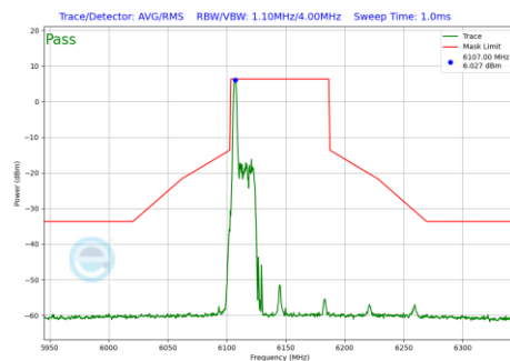
Plot 7-1169 In-Band Emission Plot CDD Diversity Antenna 4a (80MHz BW 802.11be(RU) RU26 Index0 (UNII Band 5) - Ch.39)
