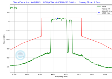
Plot 7-1196 In-Band Emission Plot CDD Diversity Antenna 4a (160MHz BW 802.11be(RU) RU996+484+242 Index98 (UNII Band 7) - Ch.143)
