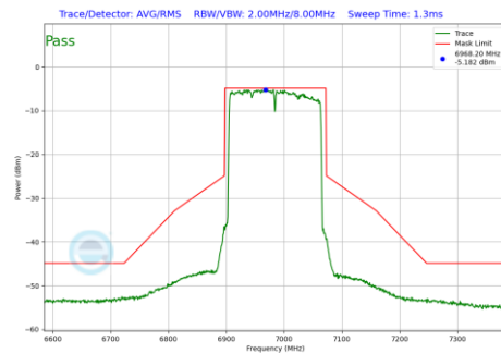
Plot 7-1292 In-Band Emission Plot SDM Diversity Antenna 2a (160MHz BW 802.11be(RU) RU996X2 Index68 (UNII Band 8) - Ch.207)
