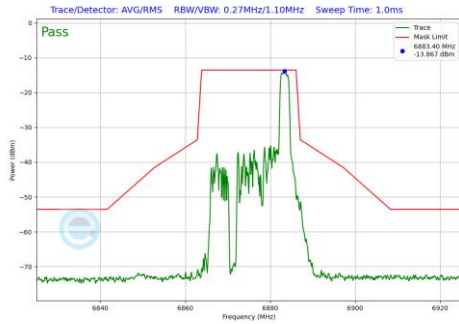
Plot 7-1245 In-Band Emission Plot SDM Diversity Antenna 4a (20MHz BW 802.11be(RU) RU26 Index8 (UNII Band 7) - Ch.185)
