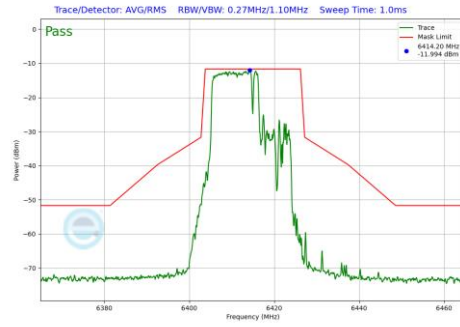
Plot 7-1265 In-Band Emission Plot SDM Diversity Antenna 4a (20MHz BW 802.11be(RU) RU106+26 Index82 (UNII Band 5) - Ch.93)
