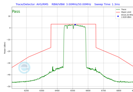
Plot 7-1184 In-Band Emission Plot CDD Diversity Antenna 2a (160MHz BW 802.11be(RU) RU996+484+242 Index96 (UNII Band 6) - Ch.111)
