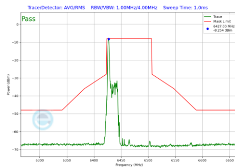
Plot 7-1227 In-Band Emission Plot SDM Diversity Antenna 2a (80MHz BW 802.11be(RU) RU26 Index0 (UNII Band 6) - Ch.103)
