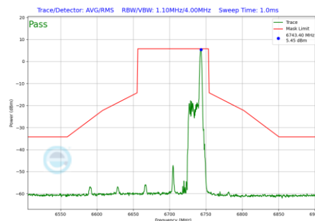
Plot 7-1177 In-Band Emission Plot CDD Diversity Antenna 4a (80MHz BW 802.11be(RU) RU26 Index36 (UNII Band 7) - Ch.151)
