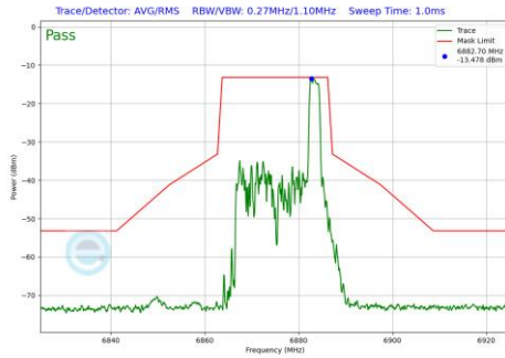
Plot 7-1229 In-Band Emission Plot SDM Diversity Antenna 2a (20MHz BW 802.11be(RU) RU26 Index8 (UNII Band 7) - Ch.185)
