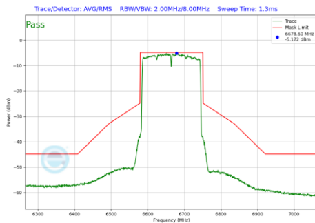
Plot 7-1304 In-Band Emission Plot SDM Diversity Antenna 4a (160MHz BW 802.11be(RU) RU996X2 Index68 (UNII Band 7) - Ch.143)
