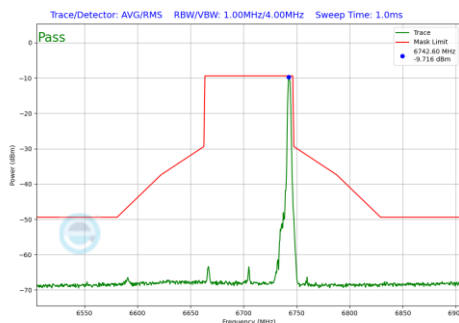
Plot 7-1247 In-Band Emission Plot SDM Diversity Antenna 4a (80MHz BW 802.11be(RU) RU26 Index36 (UNII Band 7) - Ch.151)
