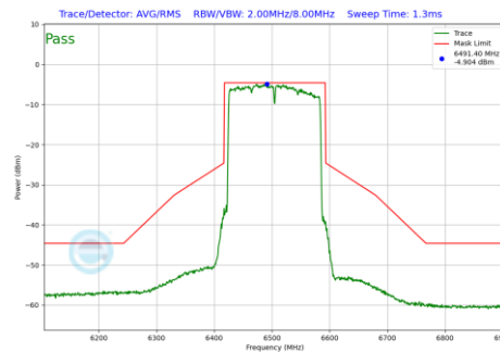
Plot 7-1300 In-Band Emission Plot SDM Diversity Antenna 4a (160MHz BW 802.11be(RU) RU996X2 Index68 (UNII Band 6) - Ch.111)
