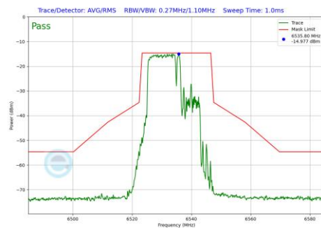
Plot 7-1259 In-Band Emission Plot SDM Diversity Antenna 2a (20MHz BW 802.11be(RU) RU106+26 Index82 (UNII Band 7) - Ch.117)
