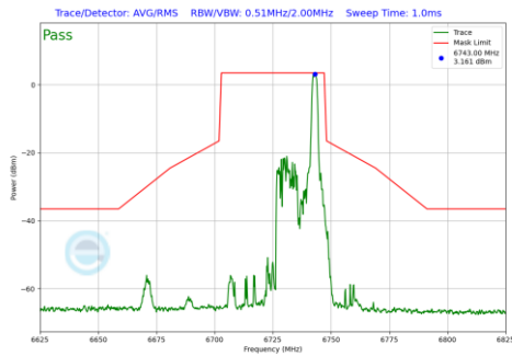
Plot 7-1164 In-Band Emission Plot CDD Diversity Antenna 2a (40MHz BW 802.11be(RU) RU26 Index17 (UNII Band 7) - Ch.155)
