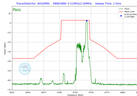
Plot 7-1176 In-Band Emission Plot CDD Diversity Antenna 4a (40MHz BW 802.11be(RU) RU26 Index17 (UNII Band 7) - Ch.155)
