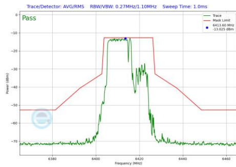
Plot 7-1253 In-Band Emission Plot SDM Diversity Antenna 2a (20MHz BW 802.11be(RU) RU106+26 Index82 (UNII Band 5) - Ch.93)
