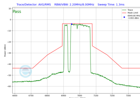
Plot 7-1276 In-Band Emission Plot SDM Diversity Antenna 4a (160MHz BW 802.11be(RU) RU996+484+242 Index97 (UNII Band 8) - Ch.207)
