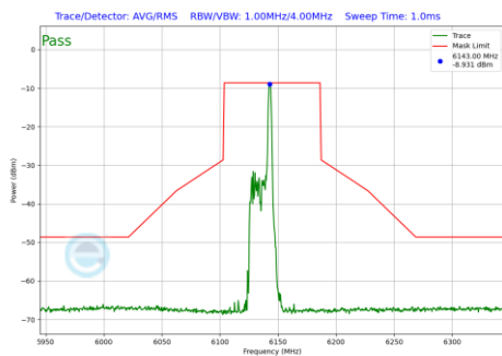
Plot 7-1223 In-Band Emission Plot SDM Diversity Antenna 2a (80MHz BW 802.11be(RU) RU26 Index17 (UNII Band 5) - Ch.39)
