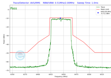
Plot 7-1298 In-Band Emission Plot SDM Diversity Antenna 4a (40MHz BW 802.11be(RU) RU484 Index65 (UNII Band 6) - Ch.99)
