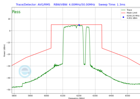
Plot 7-1181 In-Band Emission Plot CDD Diversity Antenna 2a (160MHz BW 802.11be(RU) RU996+484+242 Index98 (UNII Band 5) - Ch.47)
