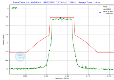
Plot 7-1293 In-Band Emission Plot SDM Diversity Antenna 4a (20MHz BW 802.11be(RU) RU242 Index61 (UNII Band 5) - Ch.93)
