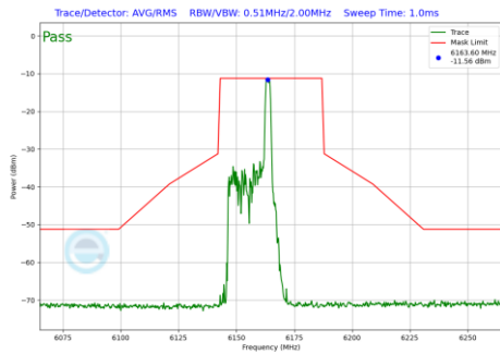
Plot 7-1238 In-Band Emission Plot SDM Diversity Antenna 4a (40MHz BW 802.11be(RU) RU26 Index8 (UNII Band 5) - Ch.43)
