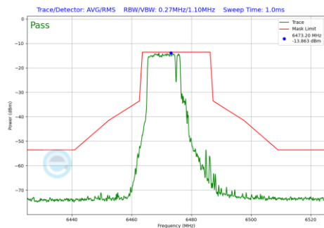
Plot 7-1256 In-Band Emission Plot SDM Diversity Antenna 2a (20MHz BW 802.11be(RU) RU106+26 Index82 (UNII Band 6) - Ch.105)
