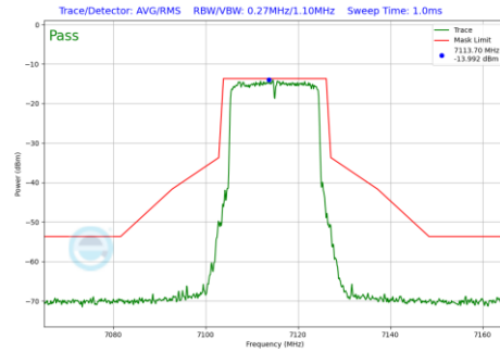
Plot 7-1289 In-Band Emission Plot SDM Diversity Antenna 2a (20MHz BW 802.11be(RU) RU242 Index61 (UNII Band 8) - Ch.233)
