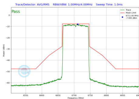
Plot 7-1287 In-Band Emission Plot SDM Diversity Antenna 2a (80MHz BW 802.11be(RU) RU996 Index67 (UNII Band 7) - Ch.151)
