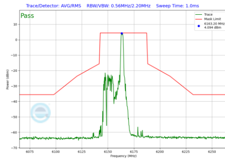
Plot 7-1168 In-Band Emission Plot CDD Diversity Antenna 4a (40MHz BW 802.11be(RU) RU26 Index8 (UNII Band 5) - Ch.43)
