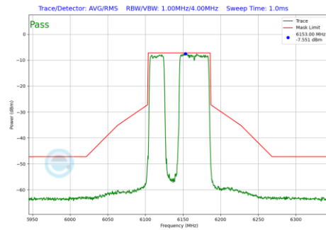
Plot 7-1266 In-Band Emission Plot SDM Diversity Antenna 4a (80MHz BW 802.11be(RU) RU484+242 Index91 (UNII Band 5) - Ch.39)
