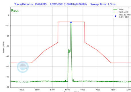
Plot 7-1232 In-Band Emission Plot SDM Diversity Antenna 2a (160MHz BW 802.11be(RU) RU26 Index36 (UNII Band 7) - Ch.175)
