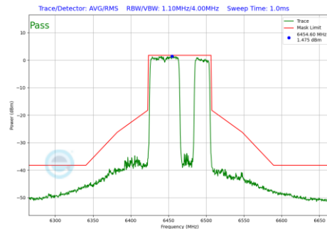
Plot 7-1192 In-Band Emission Plot CDD Diversity Antenna 4a (80MHz BW 802.11be(RU) RU484+242 Index92 (UNII Band 6) - Ch.103)
