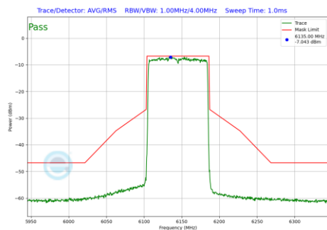
Plot 7-1295 In-Band Emission Plot SDM Diversity Antenna 4a (80MHz BW 802.11be(RU) RU996 Index67 (UNII Band 5) - Ch.39)
