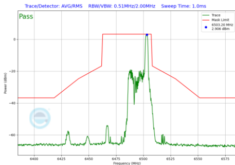
Plot 7-1172 In-Band Emission Plot CDD Diversity Antenna 4a (40MHz BW 802.11be(RU) RU26 Index17 (UNII Band 6) - Ch.107)
