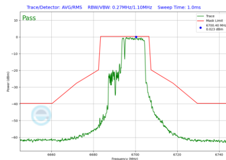
Plot 7-1185 In-Band Emission Plot CDD Diversity Antenna 2a (20MHz BW 802.11be(RU) RU106+26 Index83 (UNII Band 7) - Ch.149)
