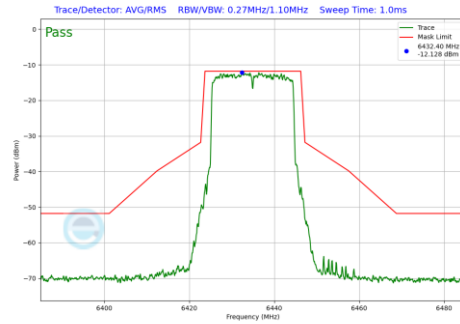
Plot 7-1297 In-Band Emission Plot SDM Diversity Antenna 4a (20MHz BW 802.11be(RU) RU242 Index61 (UNII Band 6) - Ch.97)
