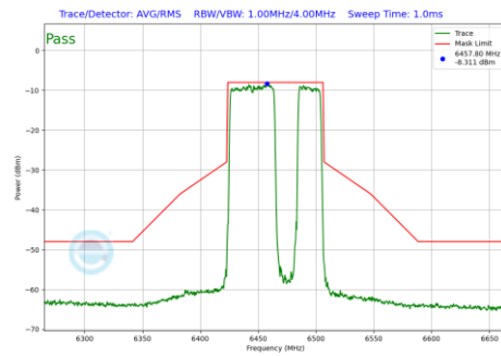
Plot 7-1257 In-Band Emission Plot SDM Diversity Antenna 2a (80MHz BW 802.11be(RU) RU484+242 Index92 (UNII Band 6) - Ch.103)
