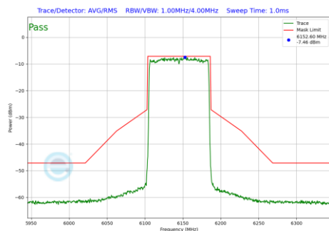
Plot 7-1279 In-Band Emission Plot SDM Diversity Antenna 2a (80MHz BW 802.11be(RU) RU996 Index67 (UNII Band 5) - Ch.39)
