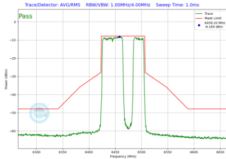
Plot 7-1269 In-Band Emission Plot SDM Diversity Antenna 4a (80MHz BW 802.11be(RU) RU484+242 Index92 (UNII Band 6) - Ch.103)
