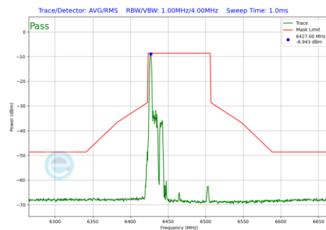
Plot 7-1243 In-Band Emission Plot SDM Diversity Antenna 4a (80MHz BW 802.11be(RU) RU26 Index0 (UNII Band 6) - Ch.103)
