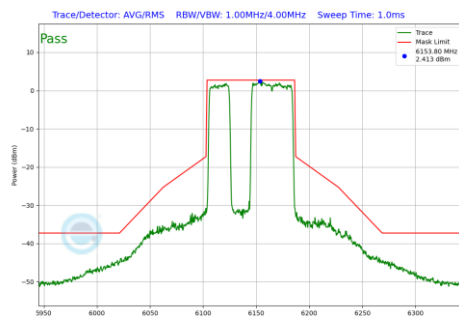
Plot 7-1180 In-Band Emission Plot CDD Diversity Antenna 2a (80MHz BW 802.11be(RU) RU484+242 Index91 (UNII Band 5) - Ch.39)
