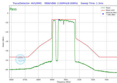
Plot 7-1264 In-Band Emission Plot SDM Diversity Antenna 2a (160MHz BW 802.11be(RU) RU996+484+242 Index97 (UNII Band 8) - Ch.207)
