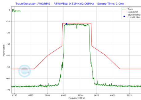
Plot 7-1286 In-Band Emission Plot SDM Diversity Antenna 2a (40MHz BW 802.11be(RU) RU484 Index65 (UNII Band 7) - Ch.179)
