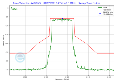
Plot 7-1277 In-Band Emission Plot SDM Diversity Antenna 2a (20MHz BW 802.11be(RU) RU242 Index61 (UNII Band 5) - Ch.93)
