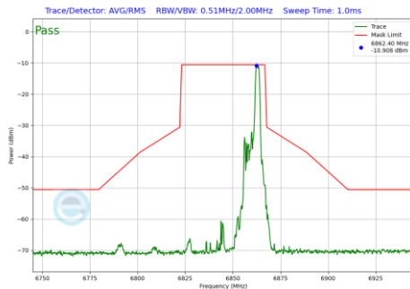
Plot 7-1230 In-Band Emission Plot SDM Diversity Antenna 2a (40MHz BW 802.11be(RU) RU26 Index17 (UNII Band 7) - Ch.179)
