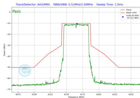
Plot 7-1278 In-Band Emission Plot SDM Diversity Antenna 2a (40MHz BW 802.11be(RU) RU484 Index65 (UNII Band 5) - Ch.43)
