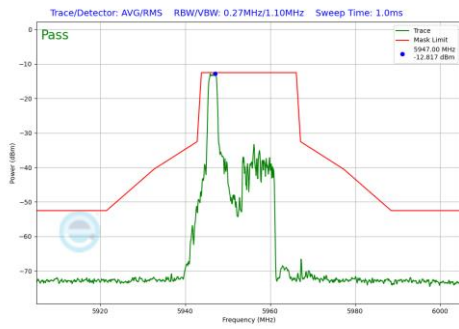
Plot 7-1221 In-Band Emission Plot SDM Diversity Antenna 2a (20MHz BW 802.11be(RU) RU26 Index0 (UNII Band 5) - Ch.1)
