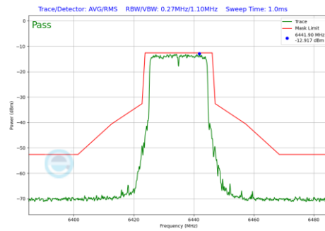
Plot 7-1281 In-Band Emission Plot SDM Diversity Antenna 2a (20MHz BW 802.11be(RU) RU242 Index61 (UNII Band 6) - Ch.97)
