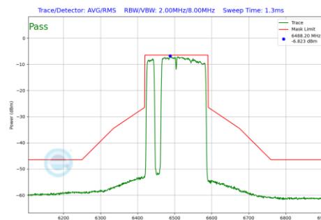
Plot 7-1258 In-Band Emission Plot SDM Diversity Antenna 2a (160MHz BW 802.11be(RU) RU996+484+242 Index97 (UNII Band 6) - Ch.111)
