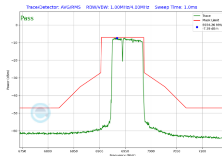
Plot 7-1275 In-Band Emission Plot SDM Diversity Antenna 4a (80MHz BW 802.11be(RU) RU484+242 Index90 (UNII Band 8) - Ch.199)
