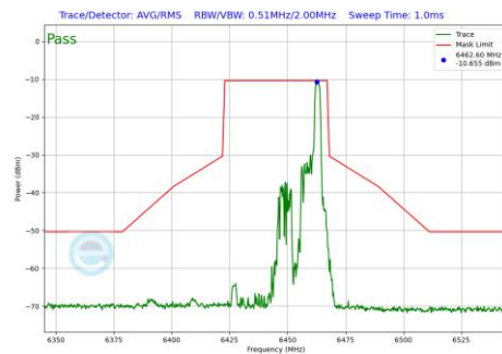
Plot 7-1226 In-Band Emission Plot SDM Diversity Antenna 2a (40MHz BW 802.11be(RU) RU26 Index17 (UNII Band 6) - Ch.99)
