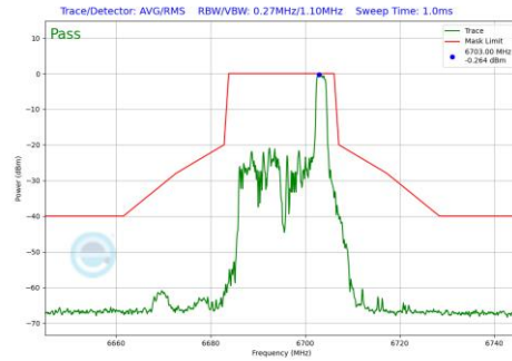
Plot 7-1175 In-Band Emission Plot CDD Diversity Antenna 4a (20MHz BW 802.11be(RU) RU26 Index8 (UNII Band 7) - Ch.149)
