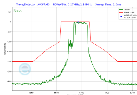
Plot 7-1194 In-Band Emission Plot CDD Diversity Antenna 4a (20MHz BW 802.11be(RU) RU106+26 Index83 (UNII Band 7) - Ch.149)
