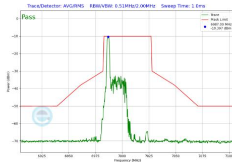
Plot 7-1234 In-Band Emission Plot SDM Diversity Antenna 2a (40MHz BW 802.11be(RU) RU26 Index0 (UNII Band 8) - Ch.211)
