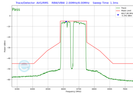
Plot 7-1273 In-Band Emission Plot SDM Diversity Antenna 4a (160MHz BW 802.11be(RU) RU996+484+242 Index99 (UNII Band 7) - Ch.143)
