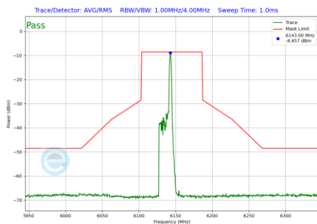
Plot 7-1239 In-Band Emission Plot SDM Diversity Antenna 4a (80MHz BW 802.11be(RU) RU26 Index17 (UNII Band 5) - Ch.39)
