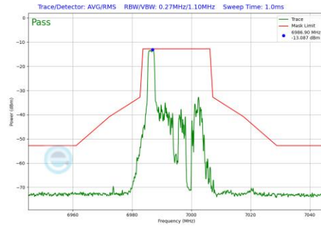
Plot 7-1233 In-Band Emission Plot SDM Diversity Antenna 2a (20MHz BW 802.11be(RU) RU26 Index0 (UNII Band 8) - Ch.209)
