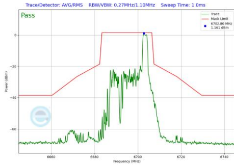
Plot 7-1163 In-Band Emission Plot CDD Diversity Antenna 2a (20MHz BW 802.11be(RU) RU26 Index8 (UNII Band 7) - Ch.149)
