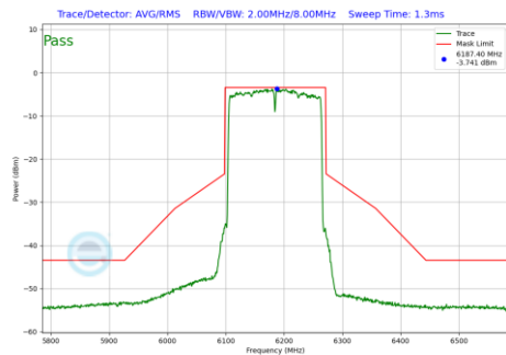
Plot 7-1296 In-Band Emission Plot SDM Diversity Antenna 4a (160MHz BW 802.11be(RU) RU996X2 Index68 (UNII Band 5) - Ch.47)
