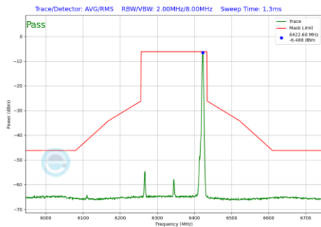
Plot 7-1240 In-Band Emission Plot SDM Diversity Antenna 4a (160MHz BW 802.11be(RU) RU26 Index36 (UNII Band 5) - Ch.79)
