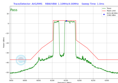
Plot 7-1189 In-Band Emission Plot CDD Diversity Antenna 4a (80MHz BW 802.11be(RU) RU484+242 Index91 (UNII Band 5) - Ch.39)
