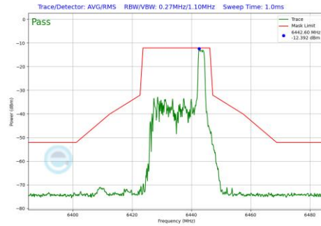
Plot 7-1241 In-Band Emission Plot SDM Diversity Antenna 4a (20MHz BW 802.11be(RU) RU26 Index8 (UNII Band 6) - Ch.97)
