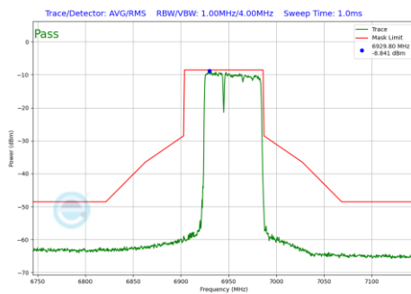
Plot 7-1263 In-Band Emission Plot SDM Diversity Antenna 2a (80MHz BW 802.11be(RU) RU484+242 Index90 (UNII Band 8) - Ch.199)
