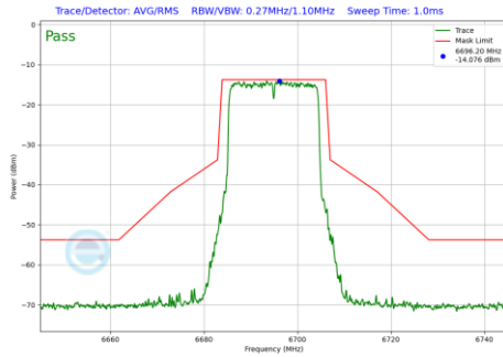
Plot 7-1285 In-Band Emission Plot SDM Diversity Antenna 2a (20MHz BW 802.11be(RU) RU242 Index61 (UNII Band 7) - Ch.149)
