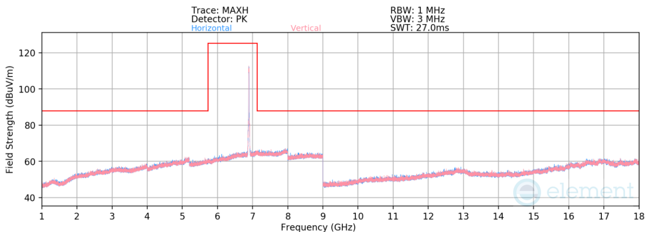
Plot 7-1372. Radiated Spurious Emissions above 1GHz CDD/SDM Primary (802.11be – Ch. 189 – RU242)
