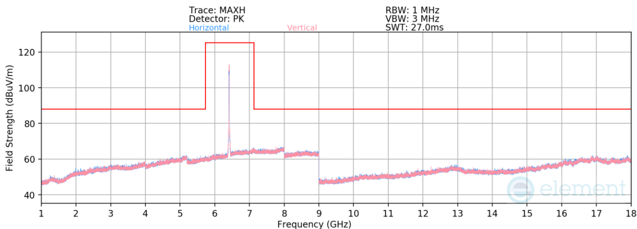
Plot 7-1363. Radiated Spurious Emissions above 1GHz CDD/SDM Primary (802.11be – Ch. 93 – RU242)
