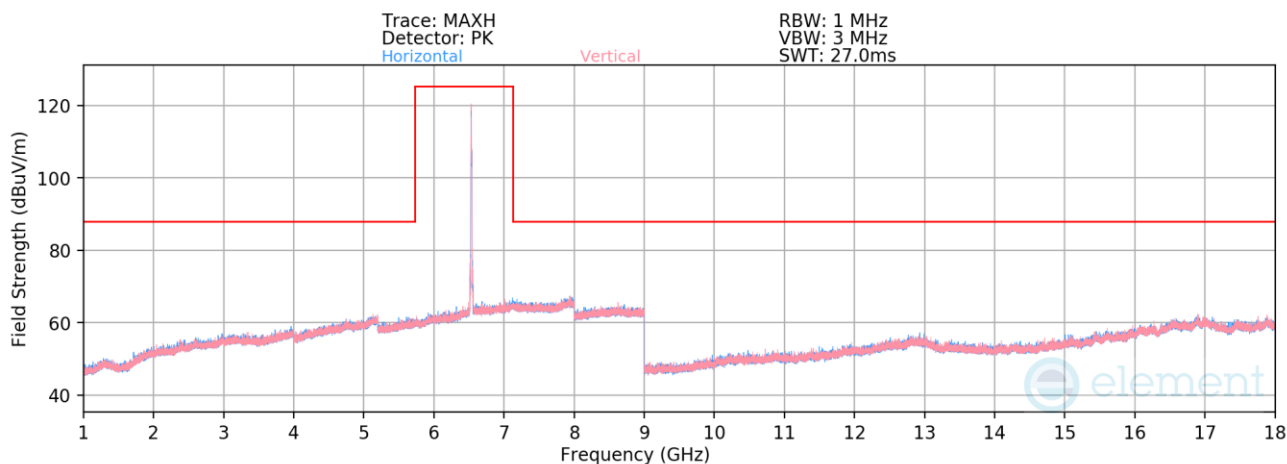
Plot 7-1384. Radiated Spurious Emissions above 1GHz CDD/SDM Diversity (802.11be – Ch. 117 – RU26)
