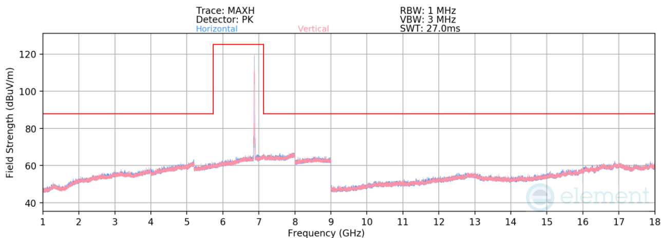
Plot 7-1387. Radiated Spurious Emissions above 1GHz CDD/SDM Diversity (802.11be – Ch. 185 – RU26)
