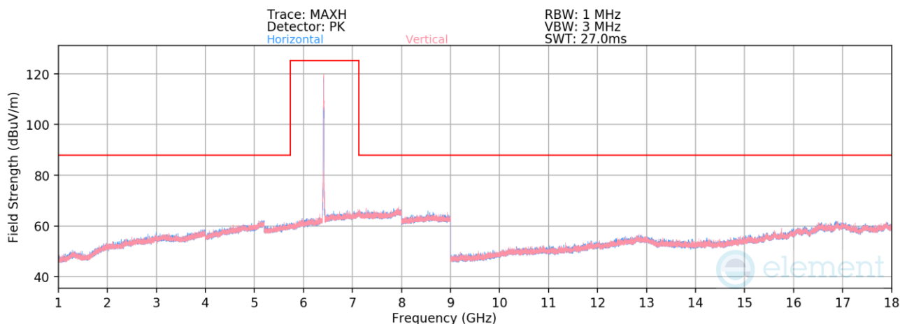
Plot 7-1379. Radiated Spurious Emissions above 1GHz CDD/SDM Diversity (802.11be – Ch. 93 – RU26)
