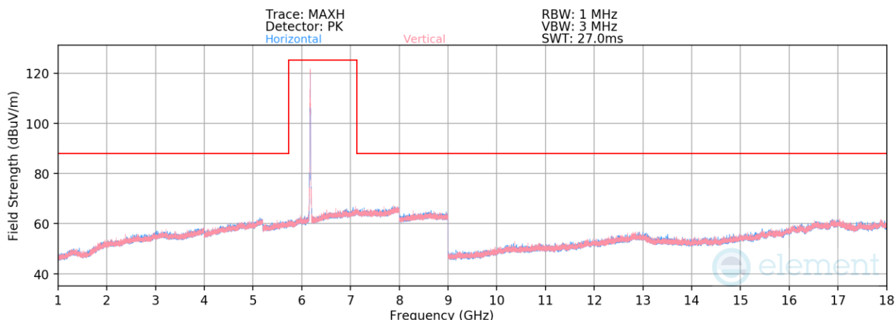
Plot 7-1345. Radiated Spurious Emissions above 1GHz CDD/SDM Primary (802.11be – Ch. 45 – RU26)
