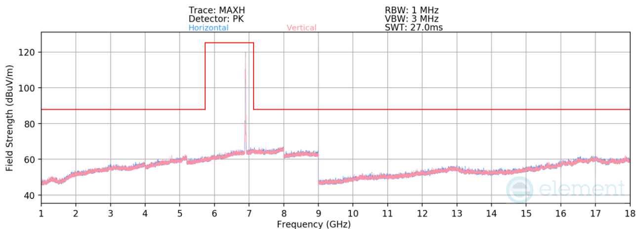
Plot 7-1388. Radiated Spurious Emissions above 1GHz CDD/SDM Diversity (802.11be – Ch. 189 – RU26)
