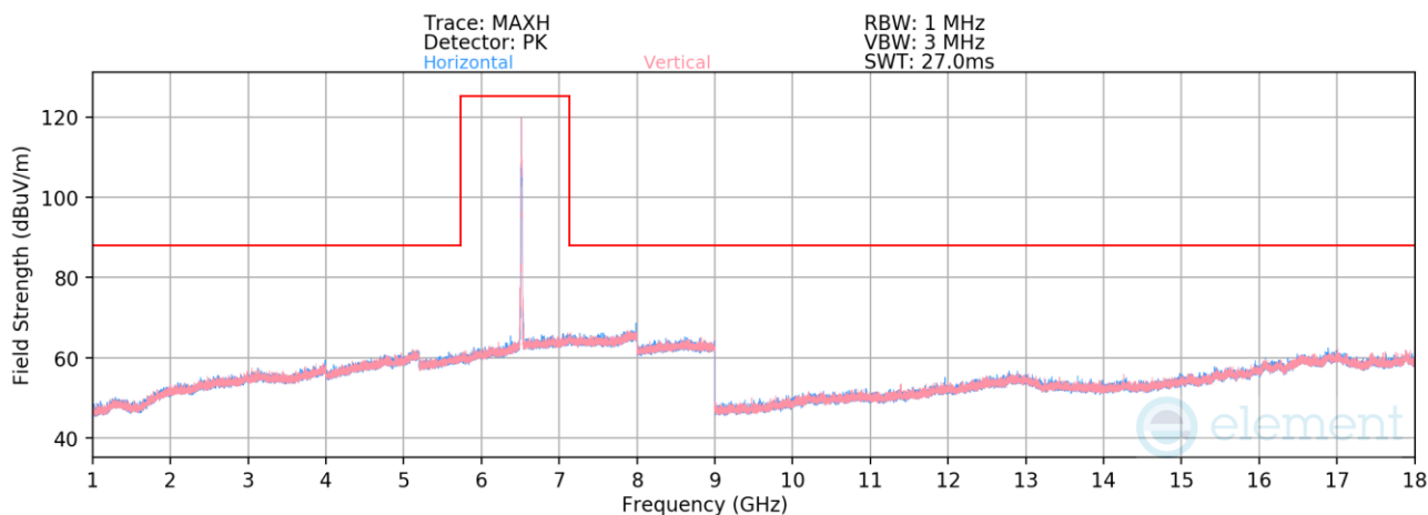
Plot 7-1383. Radiated Spurious Emissions above 1GHz CDD/SDM Diversity (802.11be – Ch. 113 – RU26)
