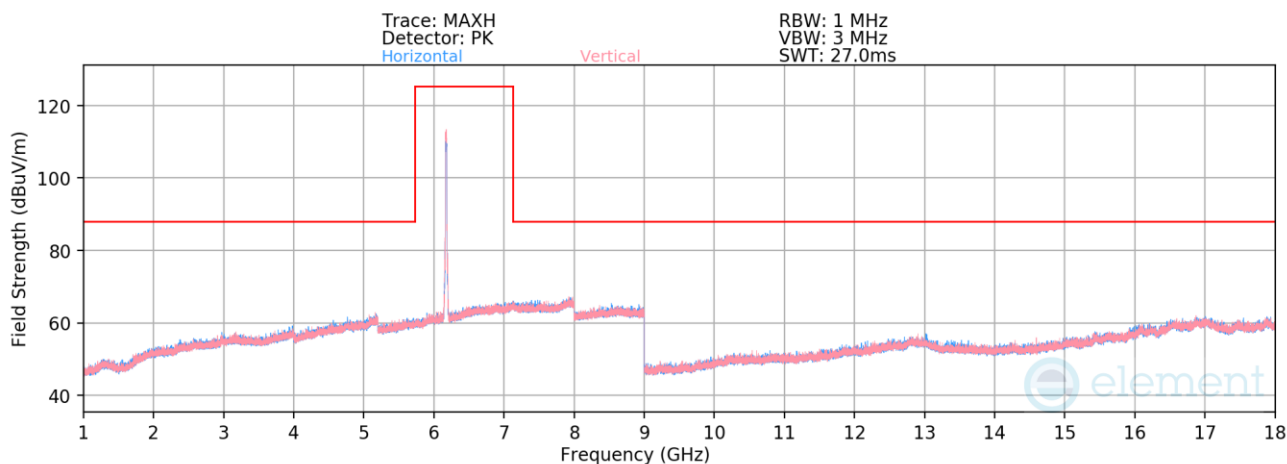
Plot 7-1362. Radiated Spurious Emissions above 1GHz CDD/SDM Primary (802.11be – Ch. 45 – RU242)
