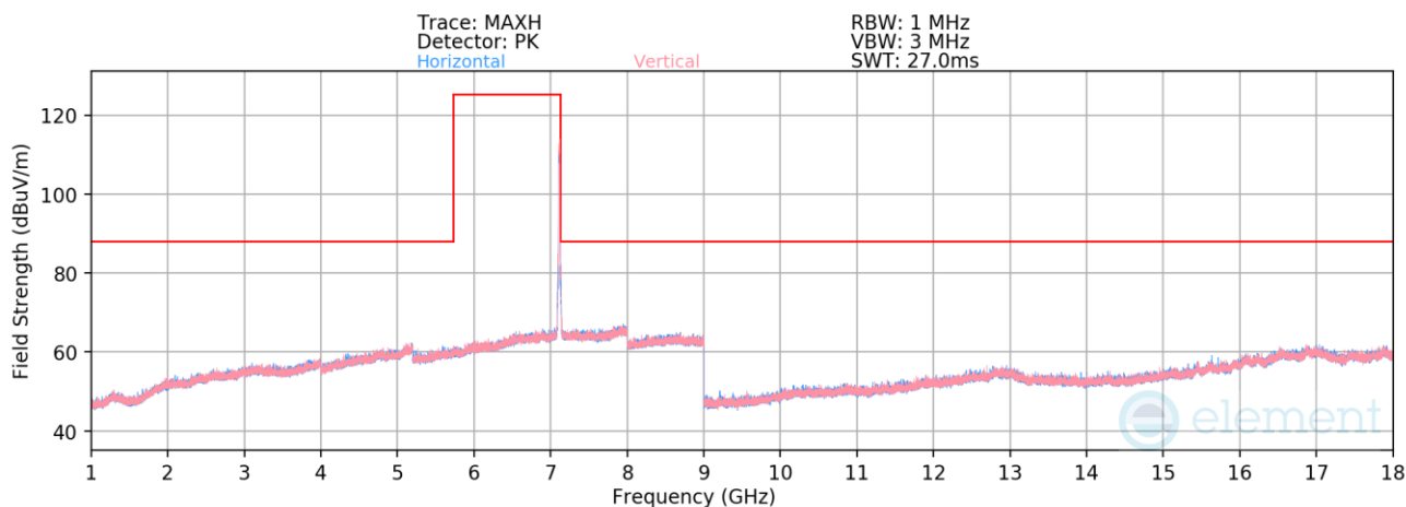
Plot 7-1375. Radiated Spurious Emissions above 1GHz CDD/SDM Primary (802.11be – Ch. 233 – RU242)
