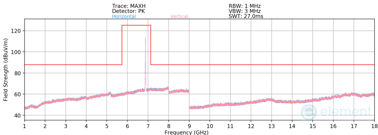
Plot 7-1371. Radiated Spurious Emissions above 1GHz CDD/SDM Primary (802.11be – Ch. 185 – RU242)
