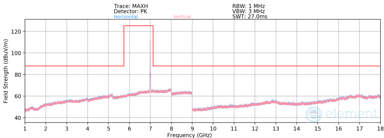
Plot 7-1373. Radiated Spurious Emissions above 1GHz CDD/SDM Primary (802.11be – Ch. 209 – RU242)
