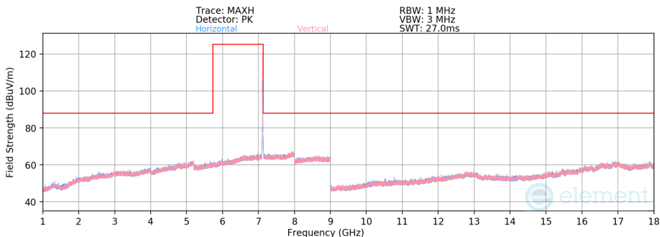
Plot 7-1359. Radiated Spurious Emissions above 1GHz CDD/SDM Primary (802.11be – Ch. 229 – RU26)
