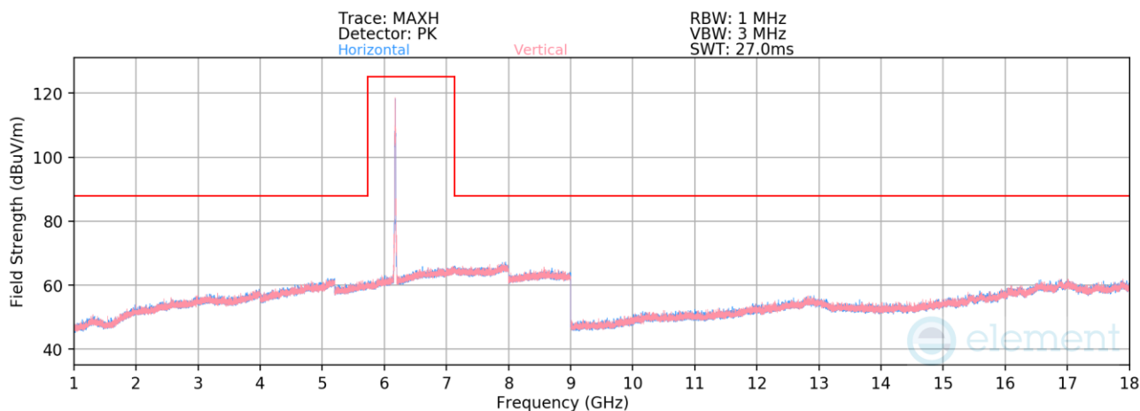
Plot 7-1377. Radiated Spurious Emissions above 1GHz CDD/SDM Diversity (802.11be – Ch. 45 – RU26)
