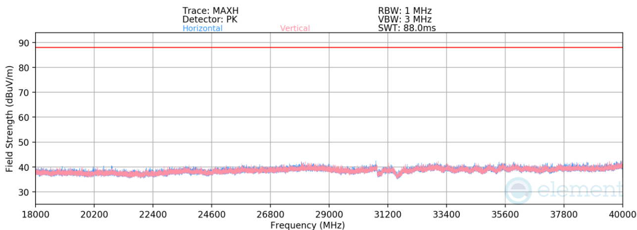
Plot 7-1350. Radiated Spurious Emissions 18-40GHz CDD/SDM Primary (802.11be – Ch. 105 – RU26)
