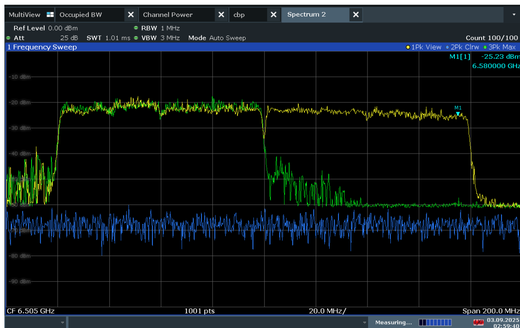
Plot 7-1343. 160MHz Bandwidth, AWGN Signal Injected – 6580MHz
