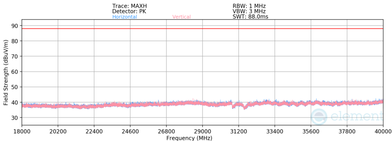
Plot 7-1386. Radiated Spurious Emissions 18-40GHz CDD/SDM Diversity (802.11be – Ch. 149 – RU26)
