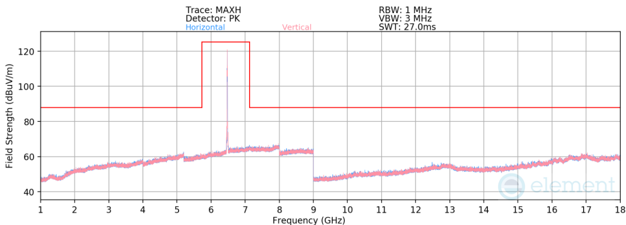
Plot 7-1349. Radiated Spurious Emissions above 1GHz CDD/SDM Primary (802.11be – Ch. 105 – RU26)
