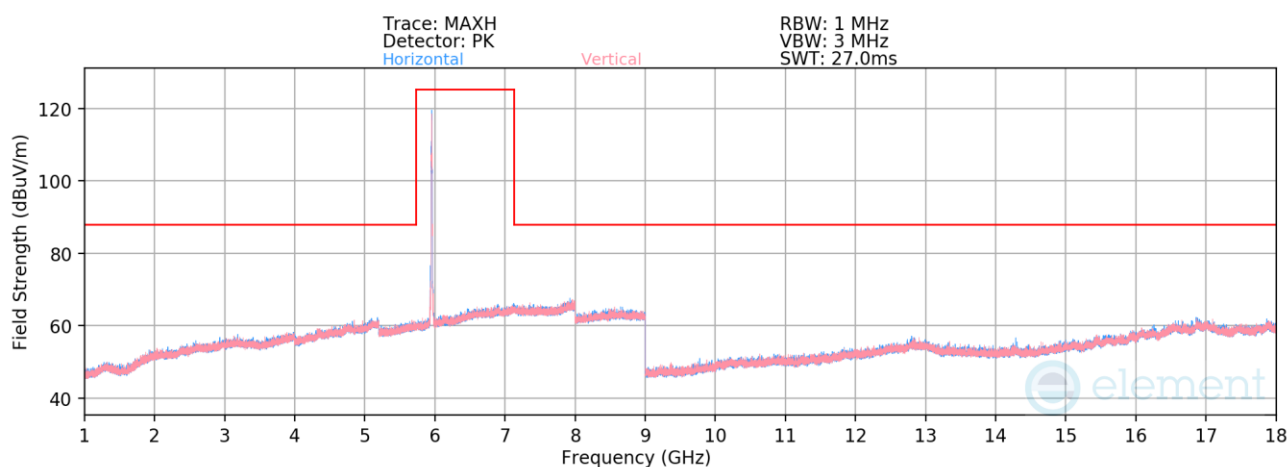
Plot 7-1376. Radiated Spurious Emissions above 1GHz CDD/SDM Diversity (802.11be – Ch. 1 – RU26)
