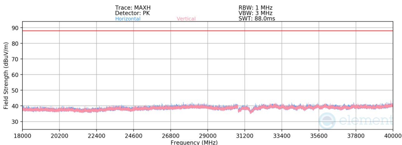
Plot 7-1354. Radiated Spurious Emissions 18-40GHz CDD/SDM Primary (802.11be – Ch. 149 – RU26)
