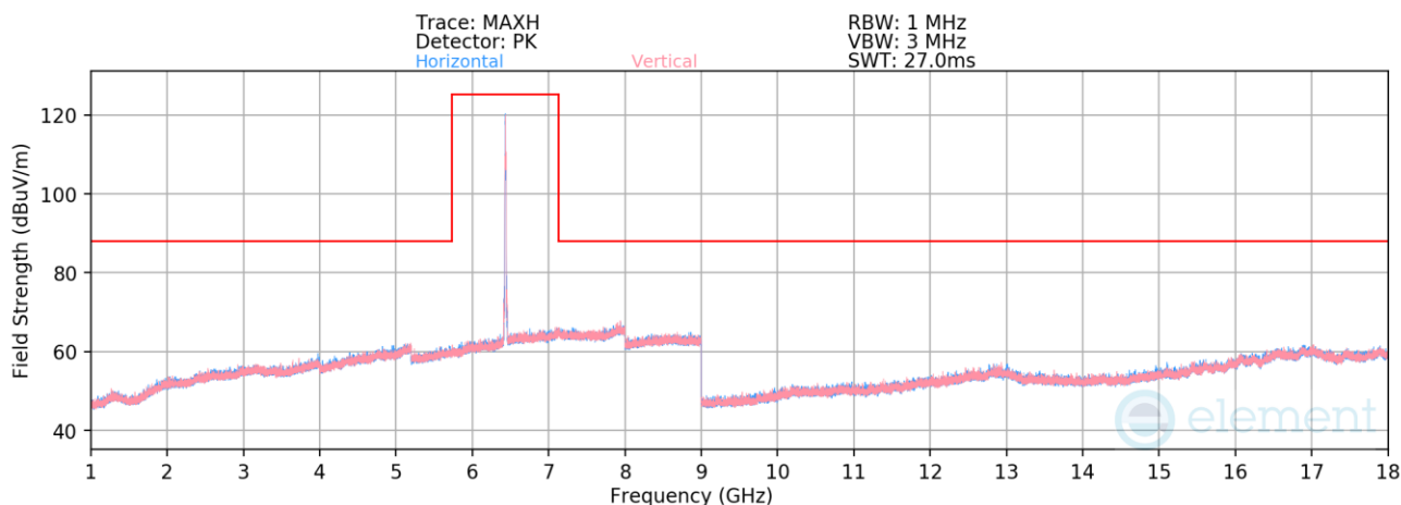
Plot 7-1348. Radiated Spurious Emissions above 1GHz CDD/SDM Primary (802.11be – Ch. 97 – RU26)
