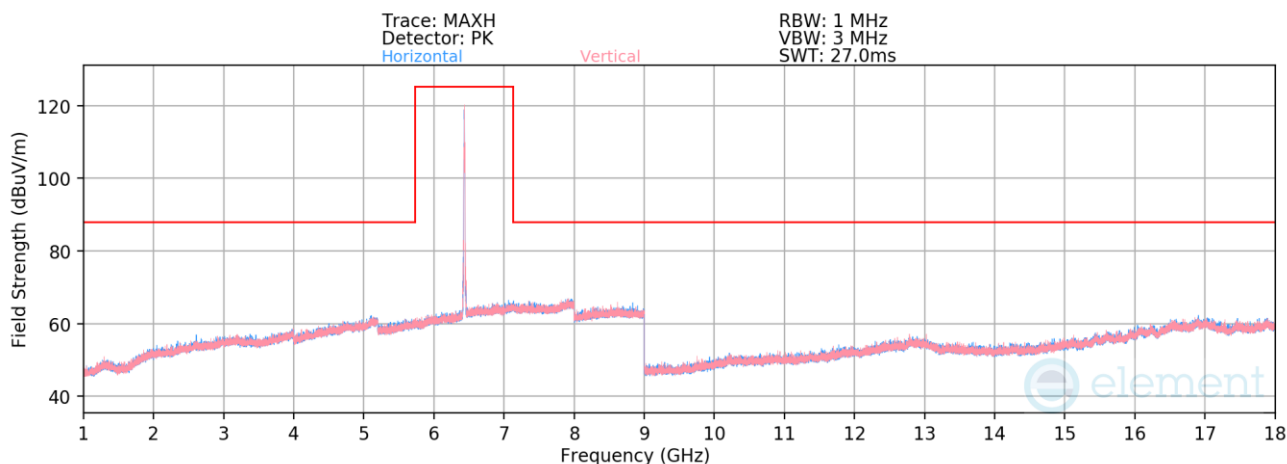
Plot 7-1380. Radiated Spurious Emissions above 1GHz CDD/SDM Diversity (802.11be – Ch. 97 – RU26)
