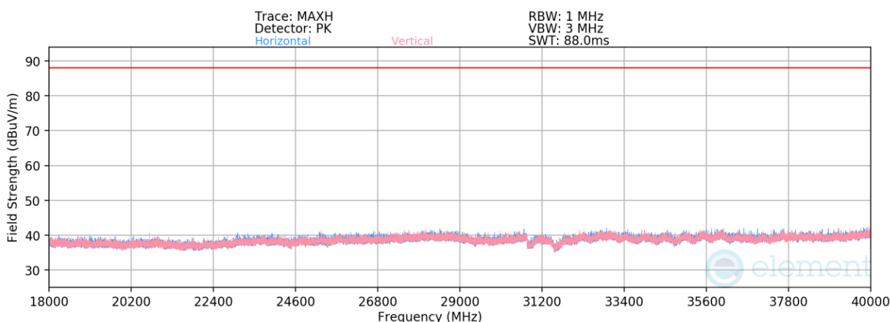
Plot 7-1361. Radiated Spurious Emissions 18-40GHz CDD/SDM Primary (802.11be – Ch. 1 – RU242)
