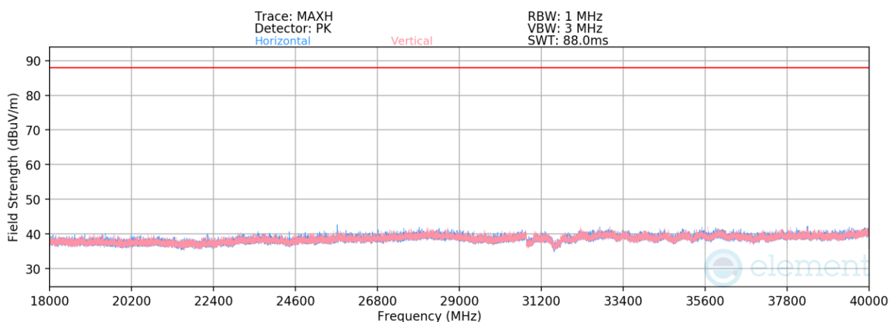
Plot 7-1346. Radiated Spurious Emissions 18-40GHz CDD/SDM Primary (802.11be – Ch. 45 – RU26)
