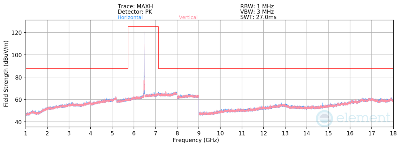
Plot 7-1381. Radiated Spurious Emissions above 1GHz CDD/SDM Diversity (802.11be – Ch. 105 – RU26)
