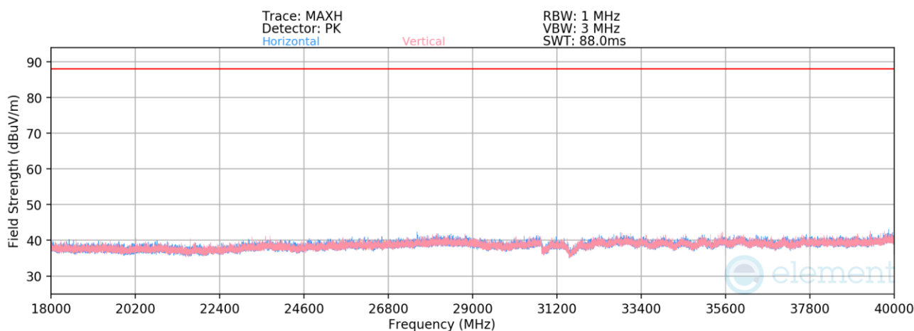
Plot 7-1366. Radiated Spurious Emissions 18-40GHz CDD/SDM Primary (802.11be – Ch. 105 – RU242)
