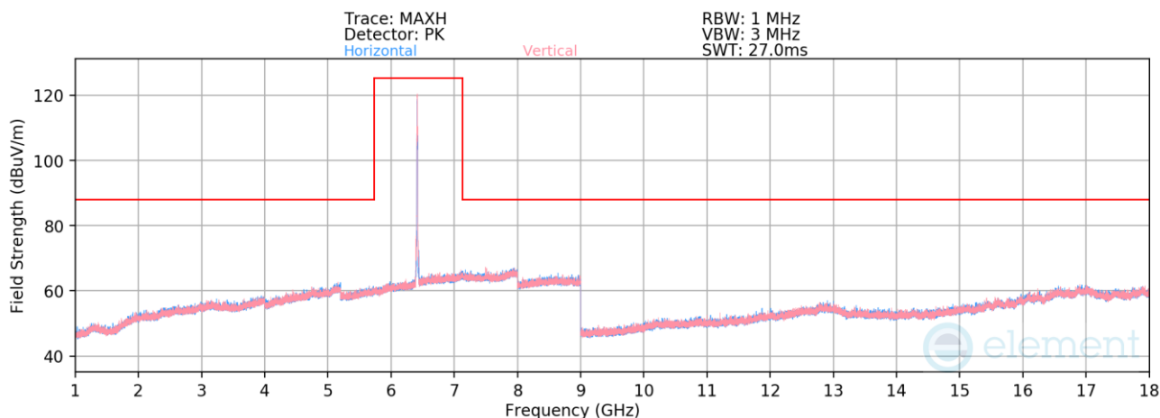
Plot 7-1347. Radiated Spurious Emissions above 1GHz CDD/SDM Primary (802.11be – Ch. 93 – RU26)
