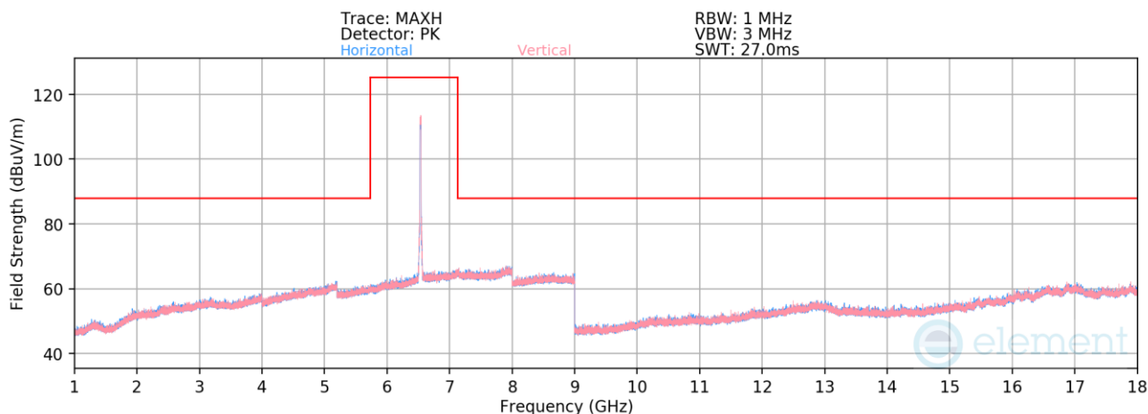
Plot 7-1368. Radiated Spurious Emissions above 1GHz CDD/SDM Primary (802.11be – Ch. 117 – RU242)
