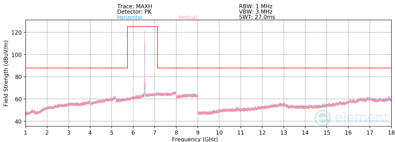
Plot 7-1352. Radiated Spurious Emissions above 1GHz CDD/SDM Primary (802.11be – Ch. 117 – RU26)
