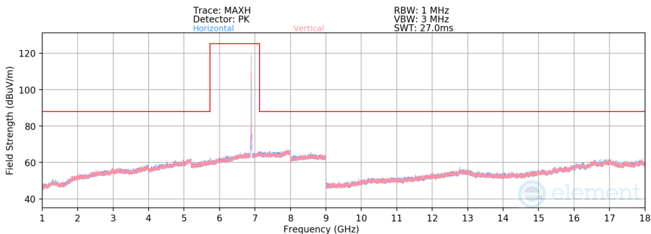
Plot 7-1356. Radiated Spurious Emissions above 1GHz CDD/SDM Primary (802.11be – Ch. 189 – RU26)
