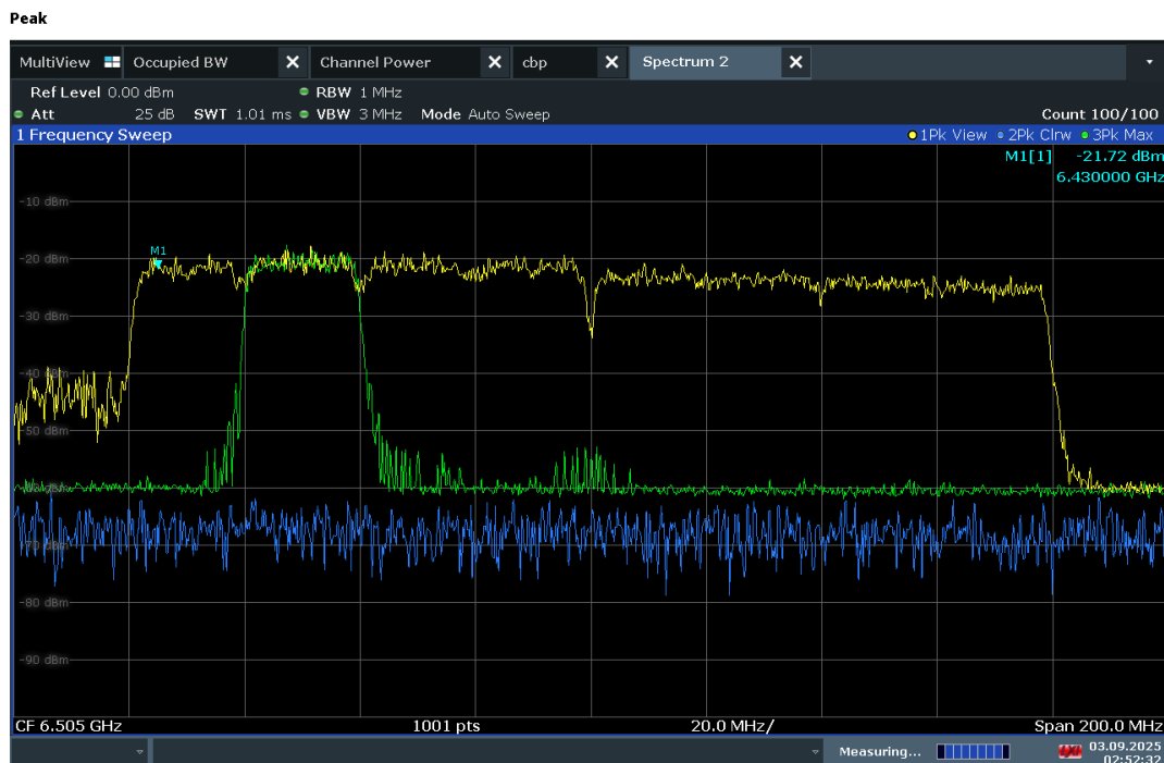
Plot 7-1341. 160MHz Bandwidth, AWGN Signal Injected – 6430Mhz
