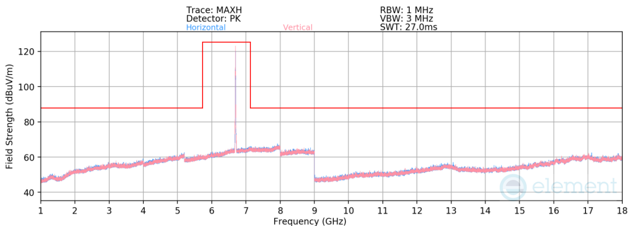
Plot 7-1385. Radiated Spurious Emissions above 1GHz CDD/SDM Diversity (802.11be – Ch. 149 – RU26)
