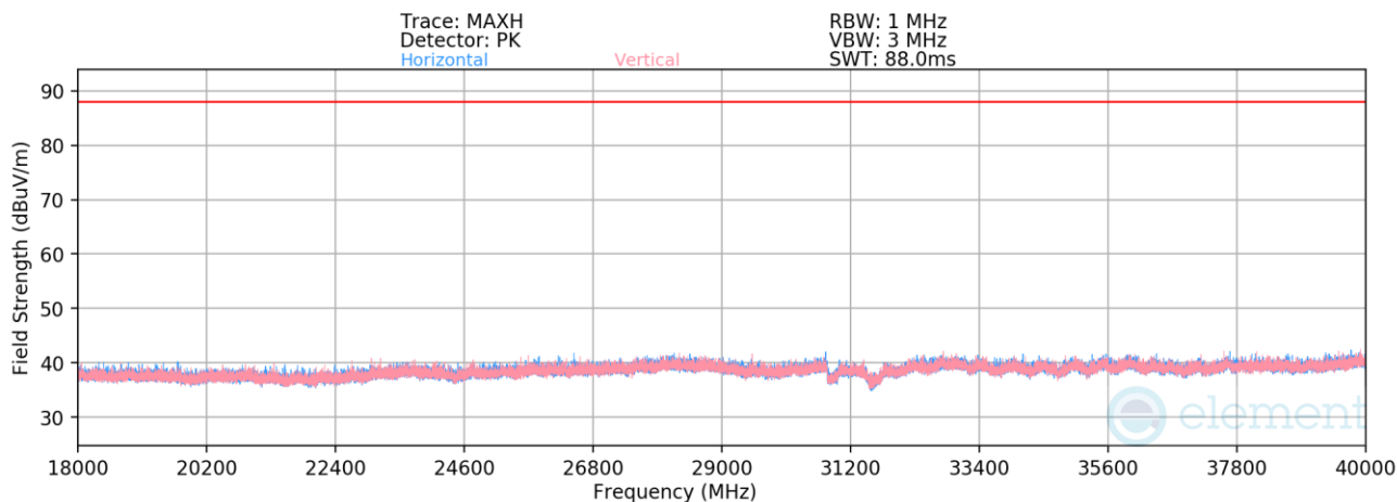
Plot 7-1382. Radiated Spurious Emissions 18-40GHz CDD/SDM Diversity (802.11be – Ch. 105 – RU26)
