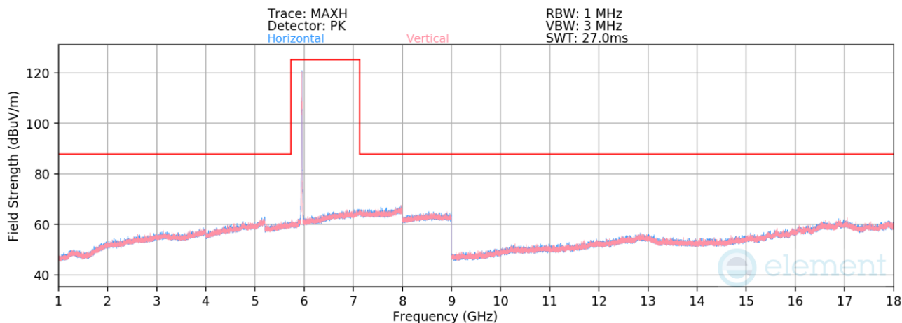
Plot 7-1344. Radiated Spurious Emissions above 1GHz CDD/SDM Primary (802.11be – Ch. 1 – RU26)
