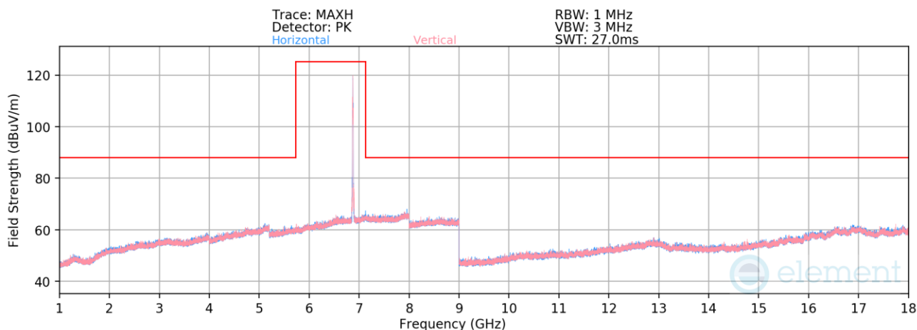
Plot 7-1355. Radiated Spurious Emissions above 1GHz CDD/SDM Primary (802.11be – Ch. 185 – RU26)
