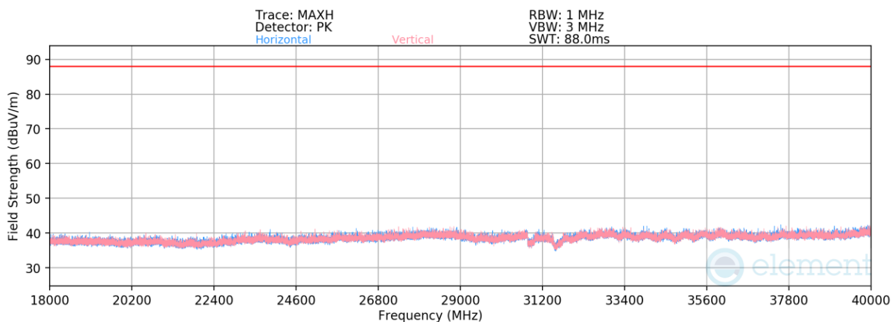
Plot 7-1378. Radiated Spurious Emissions 18-40GHz CDD/SDM Diversity (802.11be – Ch. 45 – RU26)
