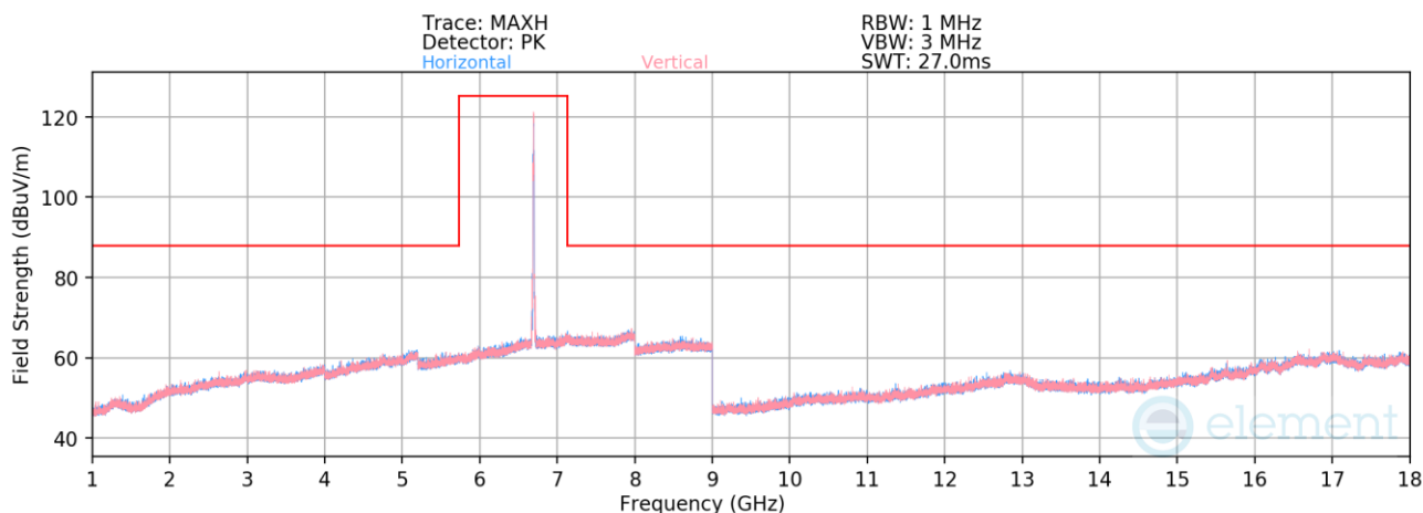
Plot 7-1353. Radiated Spurious Emissions above 1GHz CDD/SDM Primary (802.11be – Ch. 149 – RU26)
