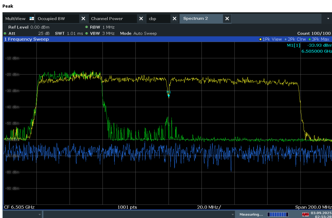
Plot 7-1342. 160MHz Bandwidth, AWGN Signal Injected – 6505MHz
