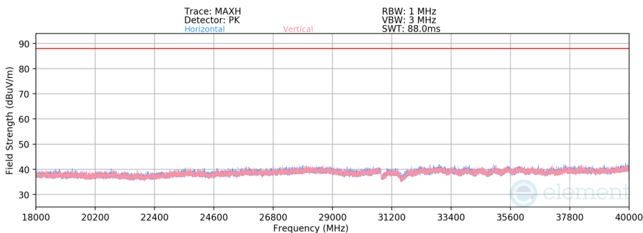
Plot 7-1374. Radiated Spurious Emissions 18-40GHz CDD/SDM Primary (802.11be – Ch. 209 – RU242)
