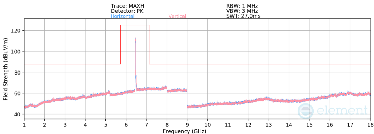
Plot 7-1365. Radiated Spurious Emissions above 1GHz CDD/SDM Primary (802.11be – Ch. 105 – RU242)
