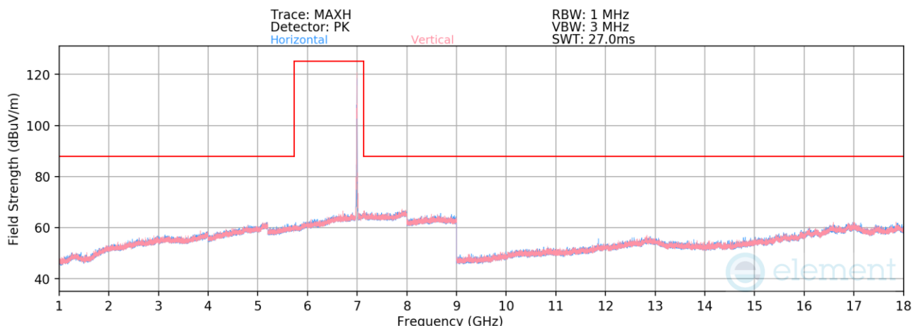
Plot 7-1357. Radiated Spurious Emissions above 1GHz CDD/SDM Primary (802.11be – Ch. 209 – RU26)
