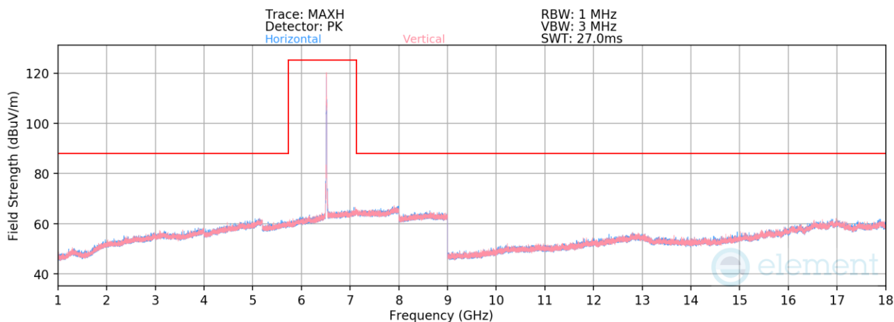
Plot 7-1351. Radiated Spurious Emissions above 1GHz CDD/SDM Primary (802.11be – Ch. 113 – RU26)
