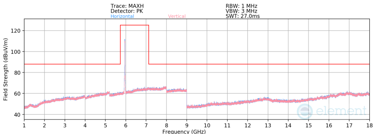
Plot 7-1360. Radiated Spurious Emissions above 1GHz CDD/SDM Primary (802.11be – Ch. 1 – RU242)
