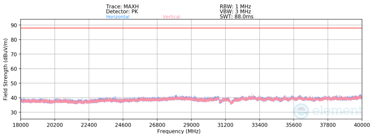
Plot 7-1370. Radiated Spurious Emissions 18-40GHz CDD/SDM Primary (802.11be – Ch. 149 – RU242)
