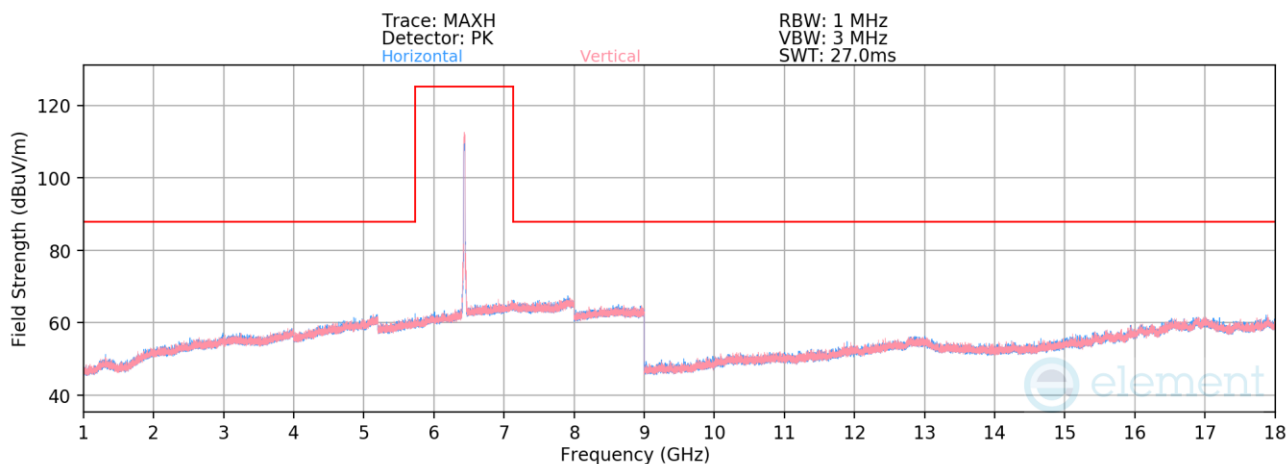
Plot 7-1364. Radiated Spurious Emissions above 1GHz CDD/SDM Primary (802.11be – Ch. 97 – RU242)
