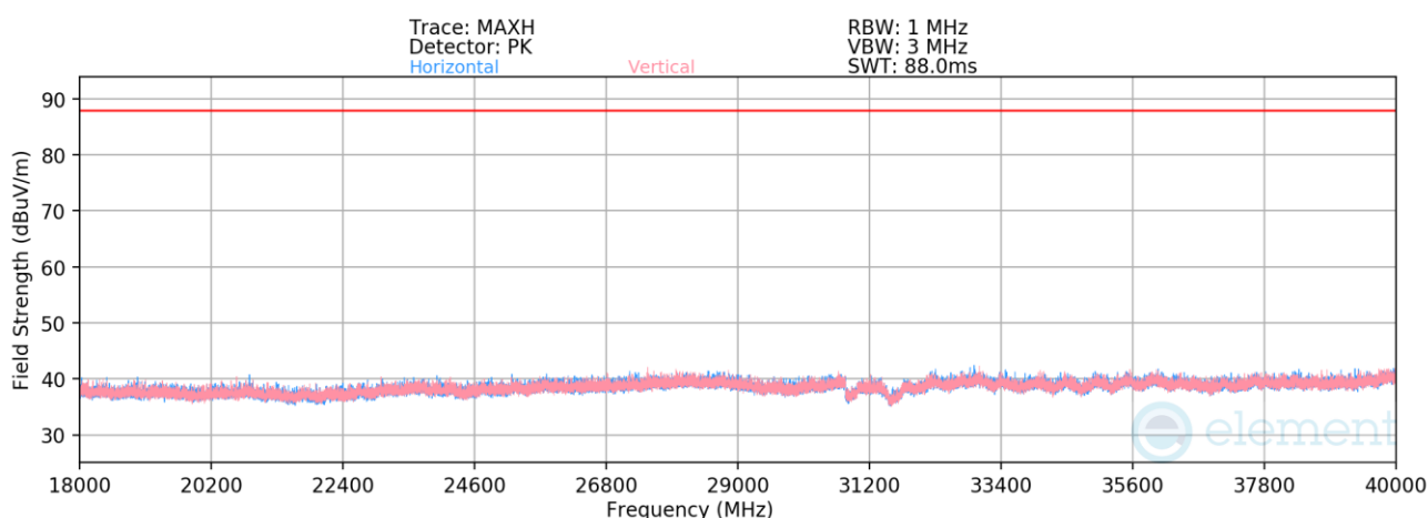
Plot 7-1358. Radiated Spurious Emissions 18-40GHz CDD/SDM Primary (802.11be – Ch. 209 – RU26)
