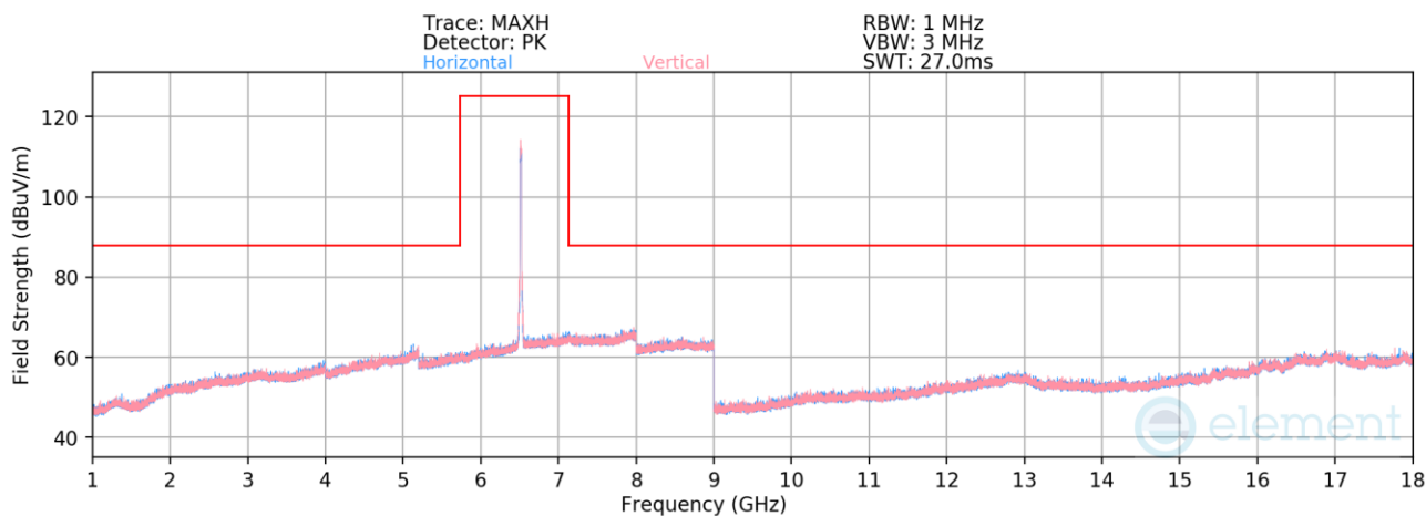
Plot 7-1367. Radiated Spurious Emissions above 1GHz CDD/SDM Primary (802.11be – Ch. 113 – RU242)
