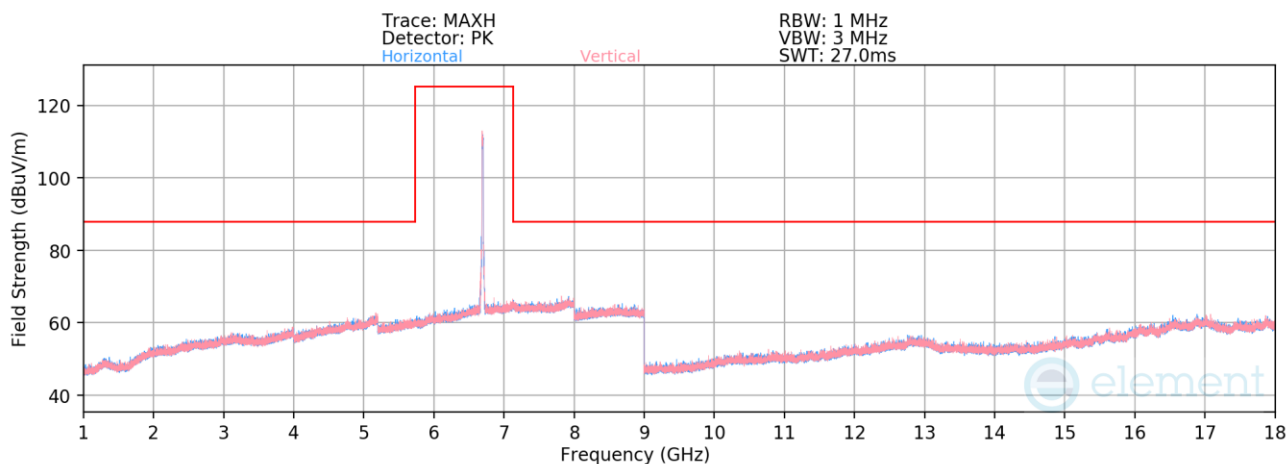
Plot 7-1369. Radiated Spurious Emissions above 1GHz CDD/SDM Primary (802.11be – Ch. 149 – RU242)
