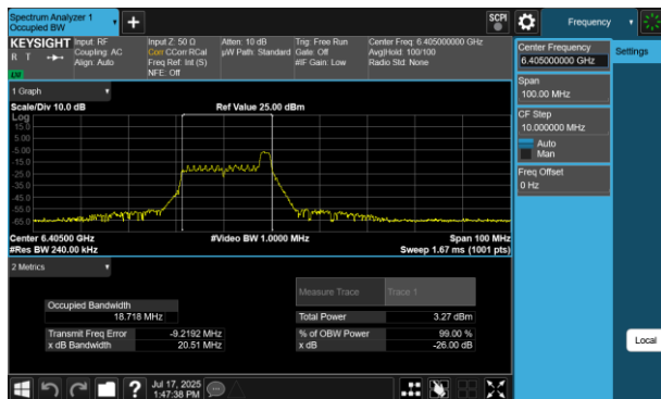
Plot 7-90 26dB BW & 99% OBW Antenna 2a (40MHz BW 802.11be(RU) RU26 Index8 - Ch.91)
