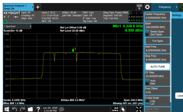
Plot 7-139 PSD Antenna WF5B (160MHz BW 802.11be(RU) RU996+484+242 Index96 - Ch.79)
