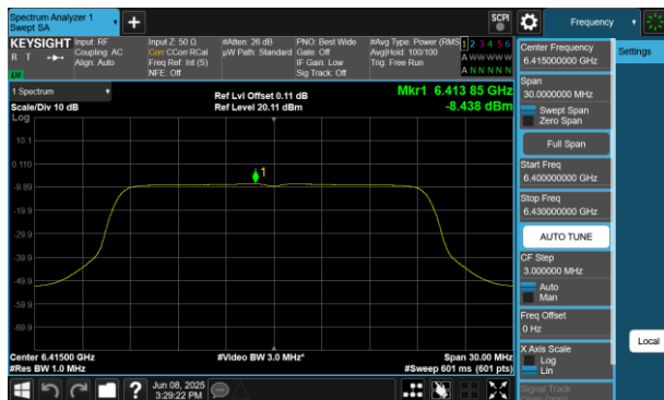
Plot 7-140 PSD Antenna WF5B (20MHz BW 802.11be(RU) RU242 Index61 - Ch.93)
