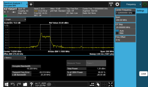
Plot 7-124 26dB BW & 99% OBW Antenna 2a (80MHz BW 802.11be(RU) RU26 Index0 - Ch.215)
