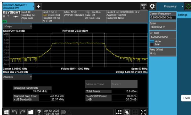
Plot 7-85 26dB BW & 99% OBW Antenna 4a (20MHz BW 802.11be(RU) RU242 Index61 - Ch.209)
