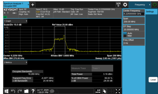
Plot 7-91 26dB BW & 99% OBW Antenna 2a (80MHz BW 802.11be(RU) RU26 Index17 - Ch.55)
