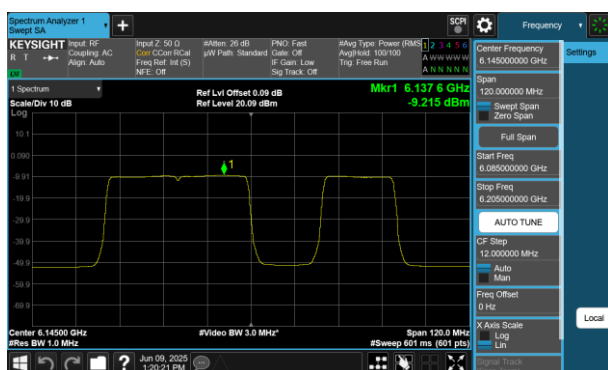
Plot 7-138 PSD Antenna WF5B (80MHz BW 802.11be(RU) RU484+242 Index92 - Ch.39)
