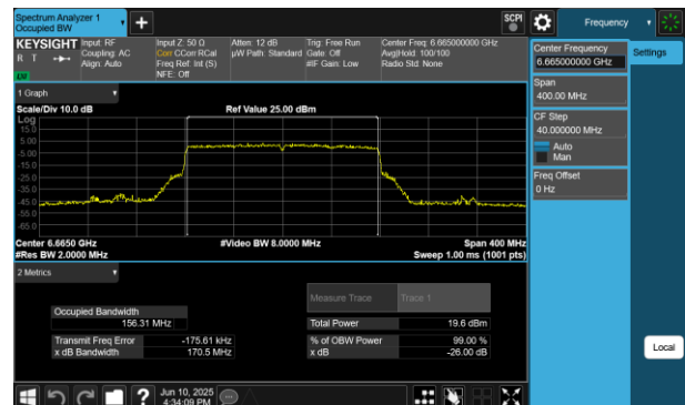
Plot 7-121 26dB BW & 99% OBW Antenna 2a (160MHz BW 802.11be(RU) RU996X2 Index68 - Ch.143)
