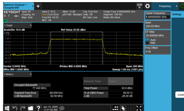
Plot 7-87 26dB BW & 99% OBW Antenna 4a (80MHz BW 802.11be(RU) RU996 Index67 - Ch.199)
