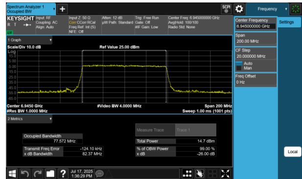
Plot 7-131 26dB BW & 99% OBW Antenna 2a (80MHz BW 802.11be(RU) RU996 Index67 - Ch.199)
