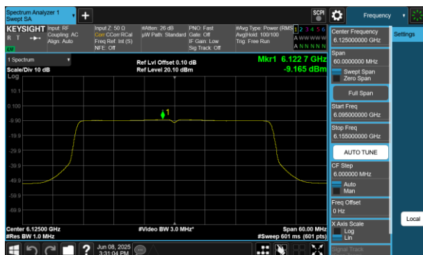
Plot 7-141 PSD Antenna WF5B (40MHz BW 802.11be(RU) RU484 Index65 - Ch.35)
