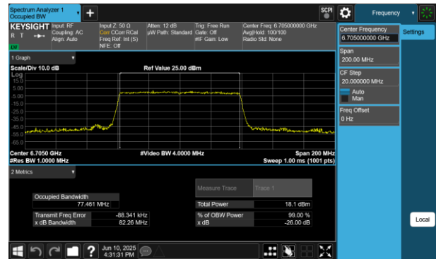
Plot 7-120 26dB BW & 99% OBW Antenna 2a (80MHz BW 802.11be(RU) RU996 Index67 - Ch.151)
