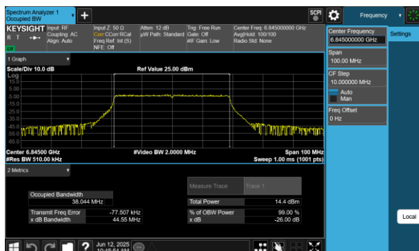
Plot 7-75 26dB BW & 99% OBW Antenna 4a (40MHz BW 802.11be(RU) RU484 Index65 - Ch.179)
