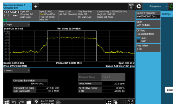
Plot 7-77 26dB BW & 99% OBW Antenna 4a (160MHz BW 802.11be(RU) RU996X2 Index68 - Ch.143)
