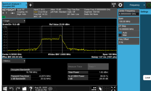
Plot 7-112 26dB BW & 99% OBW Antenna 2a (40MHz BW 802.11be(RU) RU26 Index8 - Ch.123)
