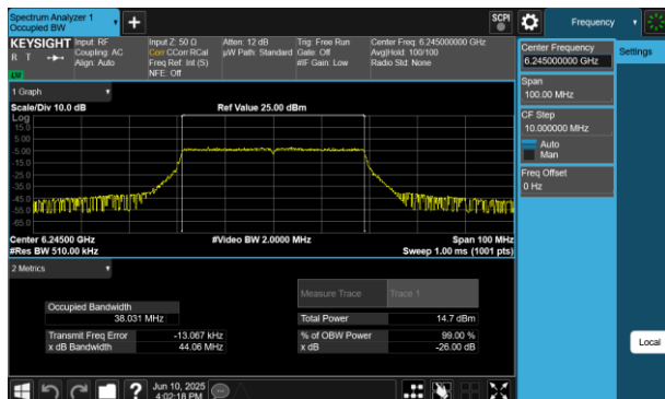
Plot 7-97 26dB BW & 99% OBW Antenna 2a (40MHz BW 802.11be(RU) RU484 Index65 - Ch.59)
