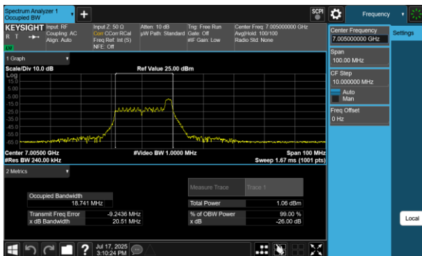
Plot 7-123 26dB BW & 99% OBW Antenna 2a (40MHz BW 802.11be(RU) RU26 Index8 - Ch.211)
