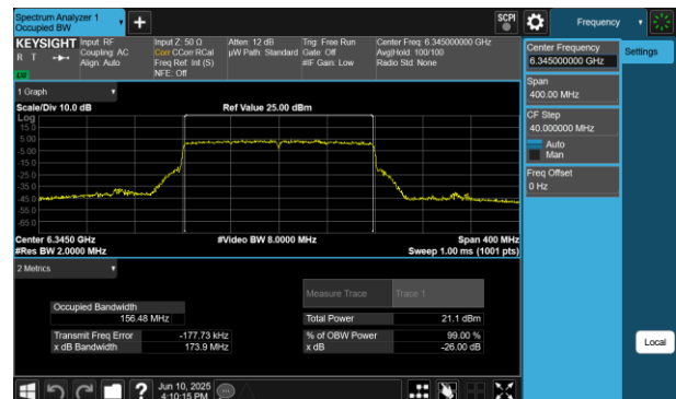
Plot 7-99 26dB BW & 99% OBW Antenna 2a (160MHz BW 802.11be(RU) RU996X2 Index68 - Ch.79)
