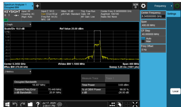
Plot 7-92 26dB BW & 99% OBW Antenna 2a (160MHz BW 802.11be(RU) RU26 Index36 - Ch.79)
