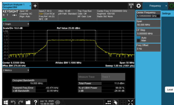
Plot 7-74 26dB BW & 99% OBW Antenna 4a (20MHz BW 802.11be(RU) RU242 Index61 - Ch.117)
