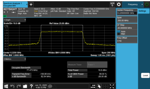
Plot 7-98 26dB BW & 99% OBW Antenna 2a (80MHz BW 802.11be(RU) RU996 Index67 - Ch.55)
