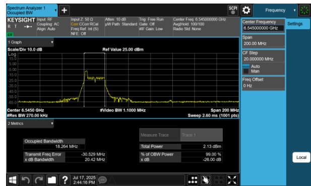
Plot 7-113 26dB BW & 99% OBW Antenna 2a (80MHz BW 802.11be(RU) RU26 Index0 - Ch.119)
