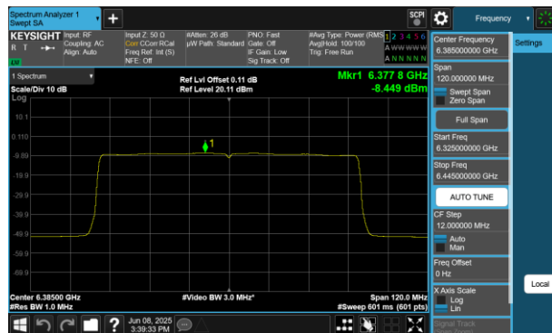
Plot 7-142 PSD Antenna WF5B (80MHz BW 802.11be(RU) RU996 Index67 - Ch.87)
