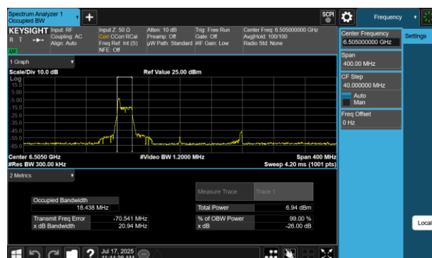
Plot 7-202 26dB BW & 99% OBW Antenna 2a (160MHz BW 802.11be(RU) RU26 Index0 - Ch.111)
