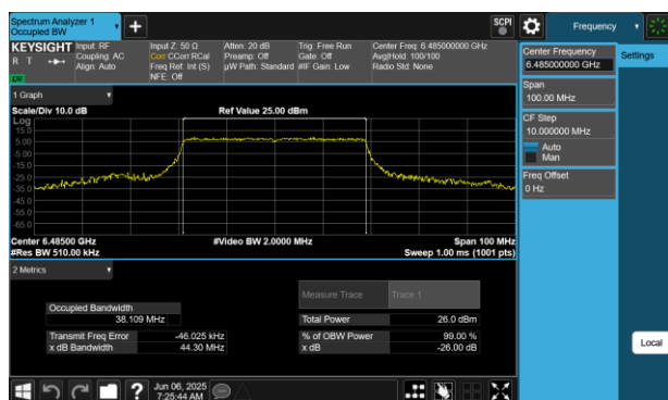
Plot 7-174 26dB BW & 99% OBW Antenna 2a (40MHz BW 802.11be(RU) RU484 Index65 - Ch.107)
