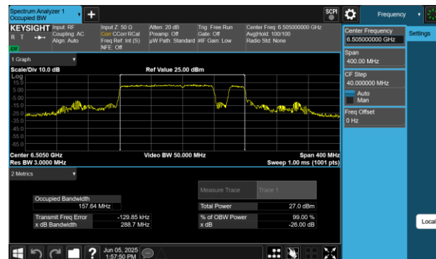
Plot 7-172 26dB BW & 99% OBW Antenna 2a (160MHz BW 802.11be(RU) RU996+484+242 Index98 - Ch.111)
