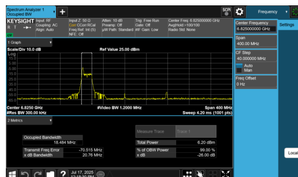
Plot 7-213 26dB BW & 99% OBW Antenna 2a (160MHz BW 802.11be(RU) RU26 Index0 - Ch.175)
