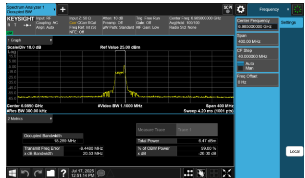
Plot 7-224 26dB BW & 99% OBW Antenna 2a (160MHz BW 802.11be(RU) RU26 Index36 - Ch.207)
