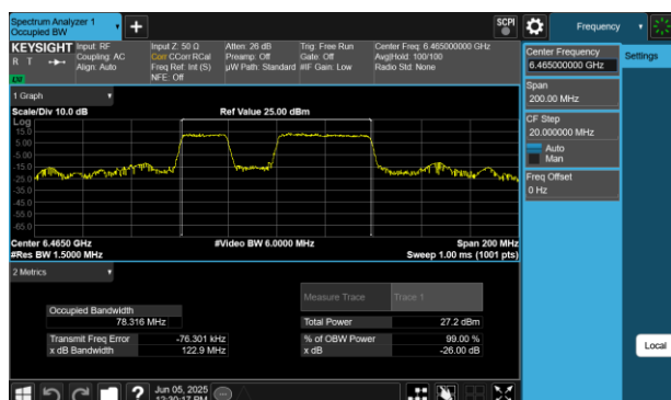
Plot 7-171 26dB BW & 99% OBW Antenna 2a (80MHz BW 802.11be(RU) RU484+242 Index91 - Ch.103)
