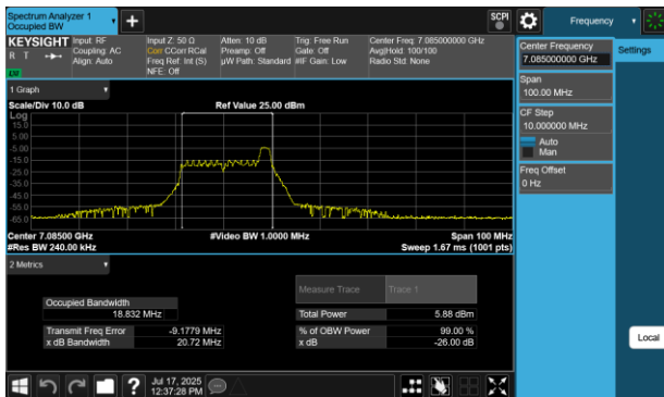
Plot 7-222 26dB BW & 99% OBW Antenna 2a (40MHz BW 802.11be(RU) RU26 Index8 - Ch.227)
