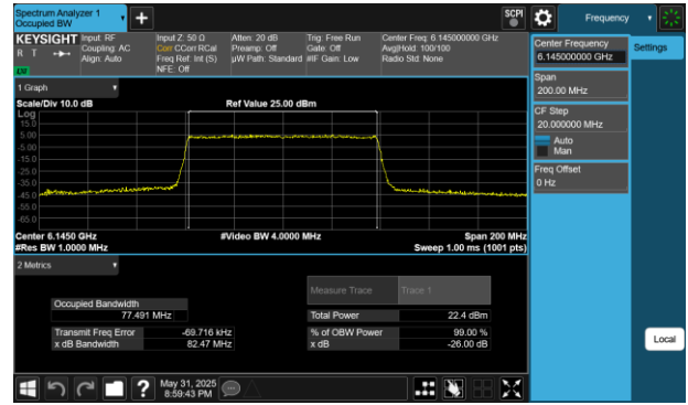
Plot 7-197 26dB BW & 99% OBW Antenna 2a (80MHz BW 802.11be(RU) RU996 Index67 - Ch.39)
