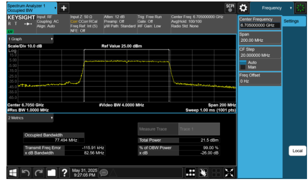
Plot 7-219 26dB BW & 99% OBW Antenna 2a (80MHz BW 802.11be(RU) RU996 Index67 - Ch.151)
