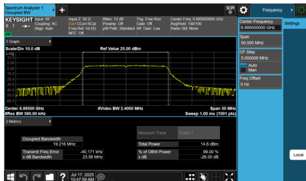
Plot 7-228 26dB BW & 99% OBW Antenna 2a (20MHz BW 802.11be(RU) RU242 Index61 - Ch.189)
