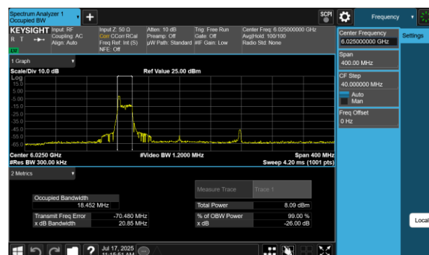
Plot 7-191 26dB BW & 99% OBW Antenna 2a (160MHz BW 802.11be(RU) RU26 Index0 - Ch.15)
