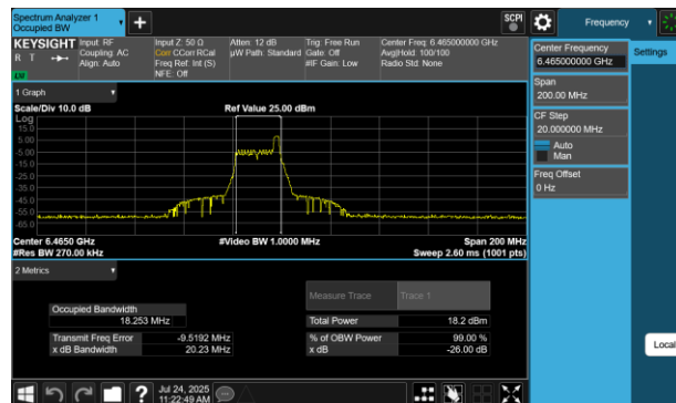
Plot 7-168 26dB BW & 99% OBW Antenna 2a (80MHz BW 802.11be(RU) RU26 Index17 - Ch.103)
