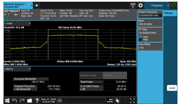
Plot 7-209 26dB BW & 99% OBW Antenna 2a (160MHz BW 802.11be(RU) RU996X2 Index68 - Ch.111)
