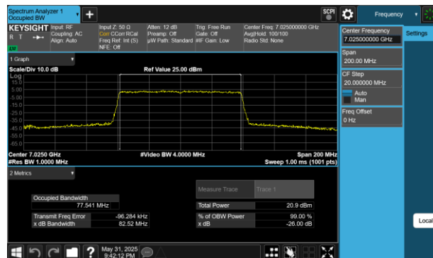
Plot 7-230 26dB BW & 99% OBW Antenna 2a (80MHz BW 802.11be(RU) RU996 Index67 - Ch.215)
