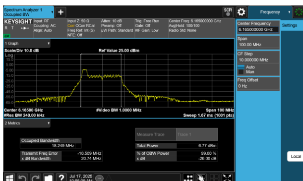
Plot 7-189 26dB BW & 99% OBW Antenna 2a (40MHz BW 802.11be(RU) RU26 Index0 - Ch.43)
