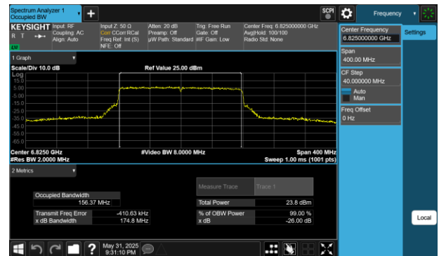
Plot 7-220 26dB BW & 99% OBW Antenna 2a (160MHz BW 802.11be(RU) RU996X2 Index68 - Ch.175)
