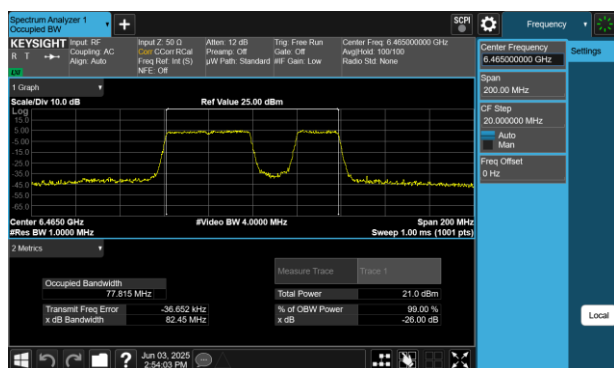
Plot 7-204 26dB BW & 99% OBW Antenna 2a (80MHz BW 802.11be(RU) RU484+242 Index92 - Ch.103)
