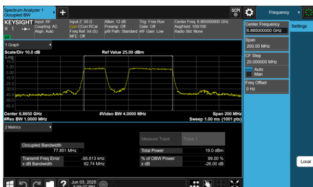
Plot 7-215 26dB BW & 99% OBW Antenna 2a (80MHz BW 802.11be(RU) RU484+242 Index91 - Ch.183)
