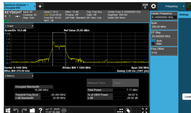
Plot 7-190 26dB BW & 99% OBW Antenna 2a (80MHz BW 802.11be(RU) RU26 Index0 - Ch.39)
