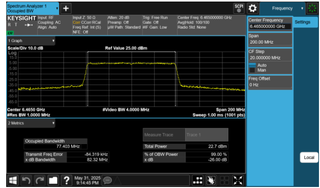
Plot 7-208 26dB BW & 99% OBW Antenna 2a (80MHz BW 802.11be(RU) RU996 Index67 - Ch.103)
