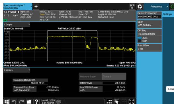
Plot 7-205 26dB BW & 99% OBW Antenna 2a (160MHz BW 802.11be(RU) RU996+484+242 Index98 - Ch.111)
