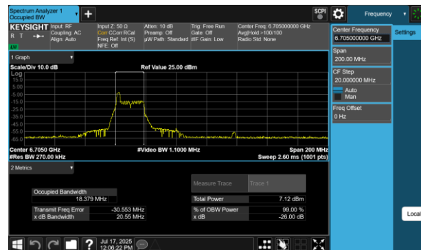
Plot 7-212 26dB BW & 99% OBW Antenna 2a (80MHz BW 802.11be(RU) RU26 Index0 - Ch.151)
