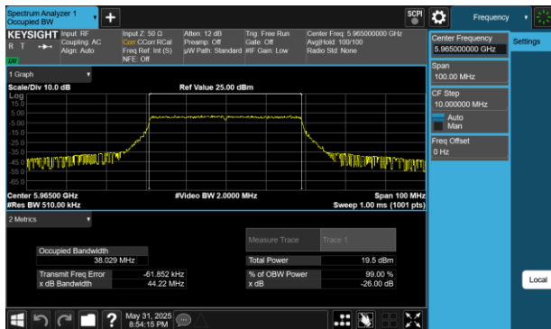
Plot 7-196 26dB BW & 99% OBW Antenna 2a (40MHz BW 802.11be(RU) RU484 Index65 - Ch.3)
