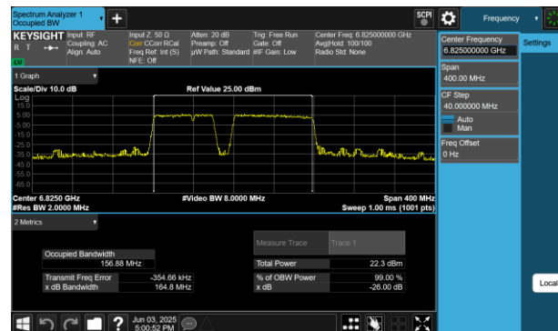
Plot 7-216 26dB BW & 99% OBW Antenna 2a (160MHz BW 802.11be(RU) RU996+484+242 Index99 - Ch.175)
