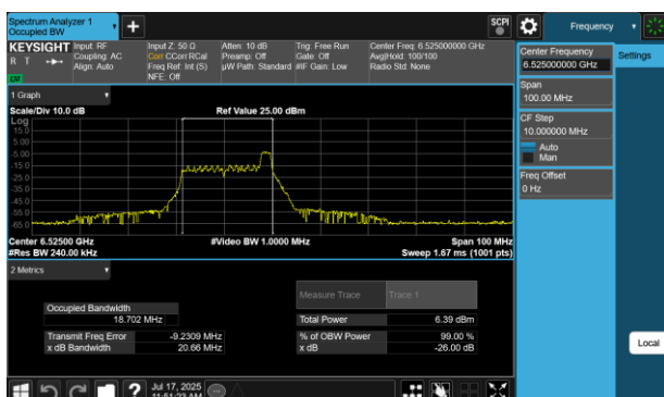
Plot 7-200 26dB BW & 99% OBW Antenna 2a (40MHz BW 802.11be(RU) RU26 Index8 - Ch.115)
