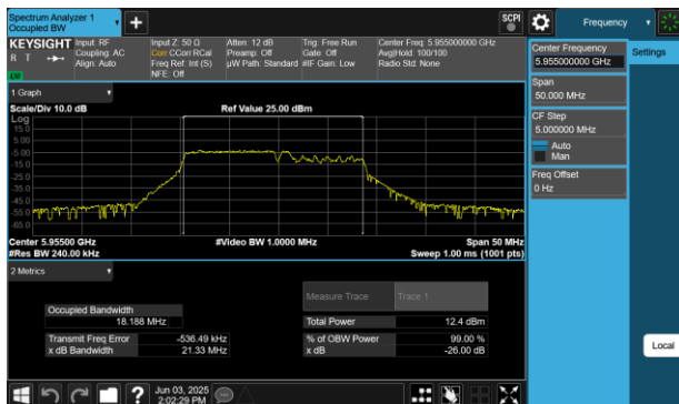
Plot 7-192 26dB BW & 99% OBW Antenna 2a (20MHz BW 802.11be(RU) RU106+26 Index82 - Ch.1)
