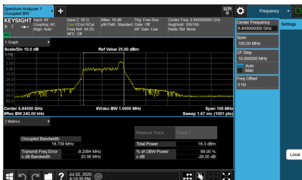
Plot 7-178 26dB BW & 99% OBW Antenna 2a (40MHz BW 802.11be(RU) RU26 Index8 - Ch.179)
