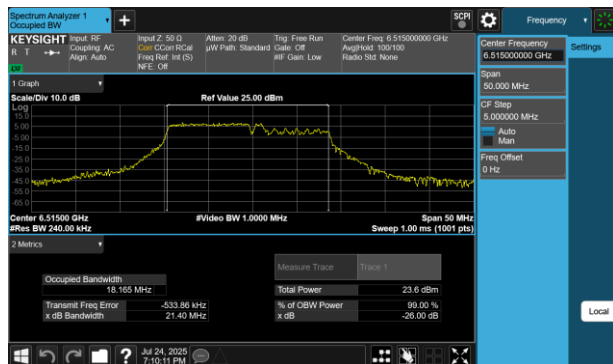
Plot 7-170 26dB BW & 99% OBW Antenna 2a (20MHz BW 802.11be(RU) RU106+26 Index82 - Ch.113)
