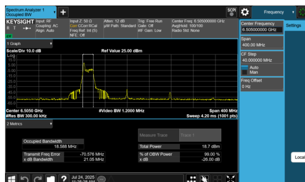
Plot 7-169 26dB BW & 99% OBW Antenna 2a (160MHz BW 802.11be(RU) RU26 Index0 - Ch.111)
