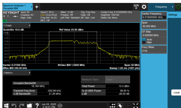
Plot 7-203 26dB BW & 99% OBW Antenna 2a (20MHz BW 802.11be(RU) RU106+26 Index82 - Ch.113)
