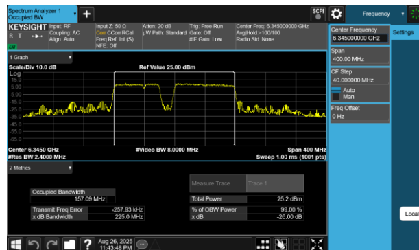
Plot 7-194 26dB BW & 99% OBW Antenna 2a (160MHz BW 802.11be(RU) RU996+484+242 Index99 - Ch.79)
