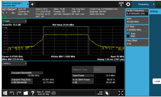
Plot 7-206 26dB BW & 99% OBW Antenna 2a (20MHz BW 802.11be(RU) RU242 Index61 - Ch.105)
