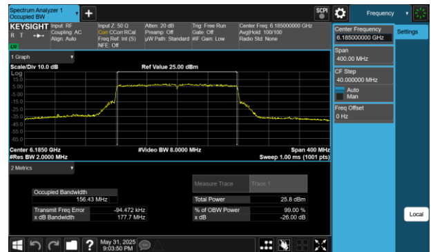
Plot 7-198 26dB BW & 99% OBW Antenna 2a (160MHz BW 802.11be(RU) RU996X2 Index68 - Ch.47)
