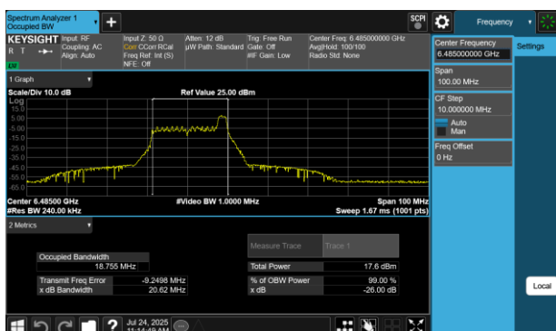
Plot 7-167 26dB BW & 99% OBW Antenna 2a (40MHz BW 802.11be(RU) RU26 Index8 - Ch.107)
