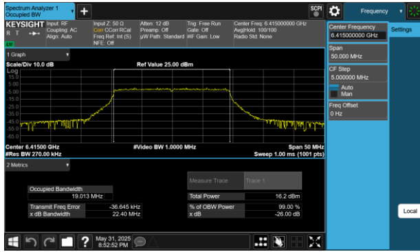
Plot 7-195 26dB BW & 99% OBW Antenna 2a (20MHz BW 802.11be(RU) RU242 Index61 - Ch.93)
