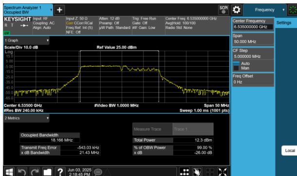
Plot 7-214 26dB BW & 99% OBW Antenna 2a (20MHz BW 802.11be(RU) RU106+26 Index82 - Ch.117)
