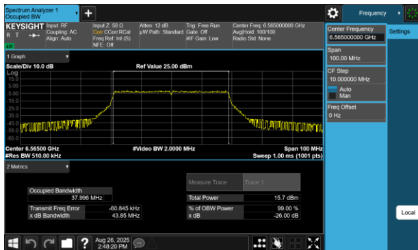
Plot 7-218 26dB BW & 99% OBW Antenna 2a (40MHz BW 802.11be(RU) RU484 Index65 - Ch.123)
