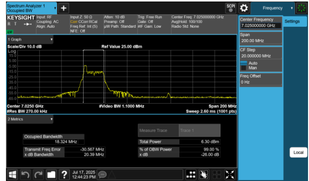
Plot 7-223 26dB BW & 99% OBW Antenna 2a (80MHz BW 802.11be(RU) RU26 Index0 - Ch.215)
