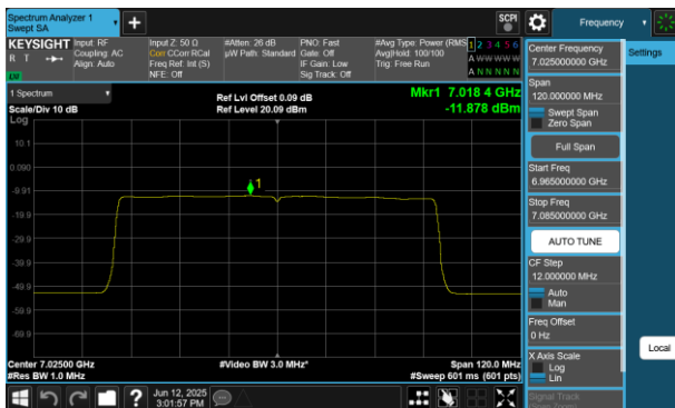
Plot 7-435 PSD SDM Diversity Antenna 4a (80MHz BW 802.11be(RU) RU996 Index67 - Ch.215)
