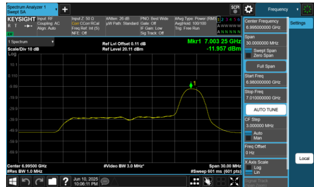
Plot 7-423 PSD SDM Diversity Antenna 2a (20MHz BW 802.11be(RU) RU26 Index8 - Ch.209)
