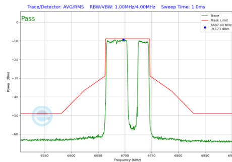
Plot 7-464 In-Band Emission Plot Antenna WF5B (80MHz BW 802.11be(RU) RU484+242 Index92 (UNII Band 7) - Ch.151)
