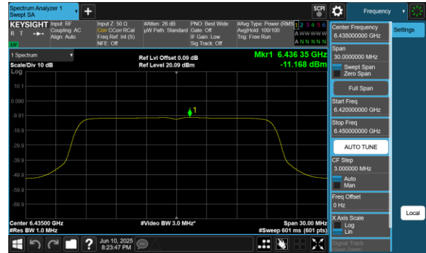
Plot 7-393 PSD SDM Diversity Antenna 2a (20MHz BW 802.11be(RU) RU242 Index61 - Ch.97)
