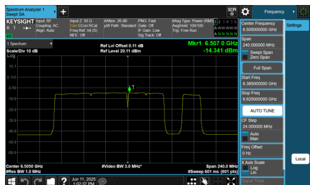
Plot 7-388 PSD SDM Diversity Antenna 2a (160MHz BW 802.11be(RU) RU996+484+242 Index98 - Ch.111)
