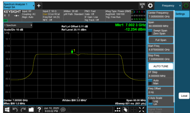
Plot 7-438 PSD SDM Diversity Antenna 2a (40MHz BW 802.11be(RU) RU484 Index65 - Ch.211)
