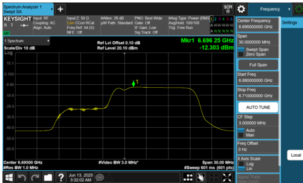
Plot 7-405 PSD SDM Diversity Antenna 4a (20MHz BW 802.11be(RU) RU106+26 Index83 - Ch.149)
