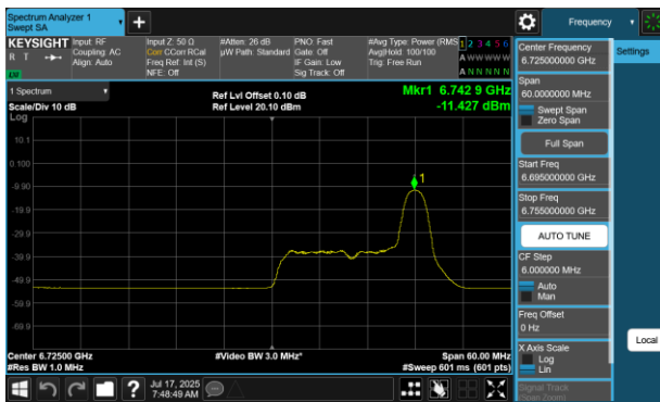
Plot 7-398 PSD SDM Diversity Antenna 4a (40MHz BW 802.11be(RU) RU26 Index17 - Ch.155)
