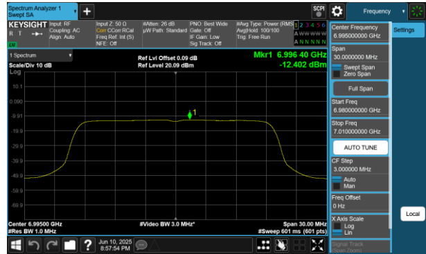
Plot 7-437 PSD SDM Diversity Antenna 2a (20MHz BW 802.11be(RU) RU242 Index61 - Ch.209)
