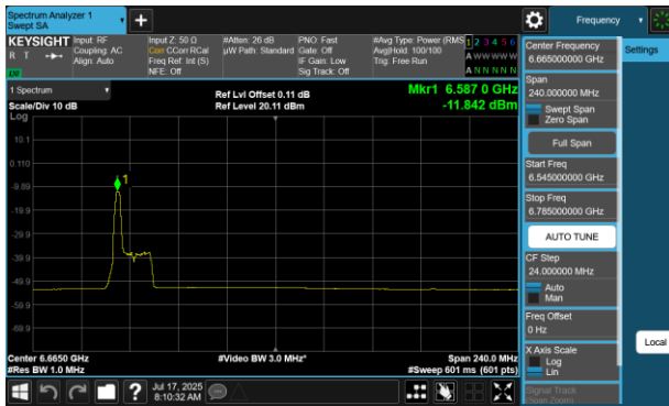
Plot 7-400 PSD SDM Diversity Antenna 4a (160MHz BW 802.11be(RU) RU26 Index0 - Ch.143)
