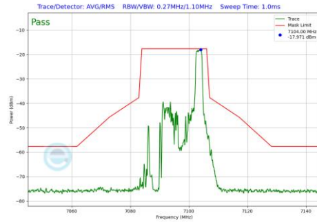
Plot 7-453 In-Band Emission Plot Antenna WF5B (20MHz BW 802.11be(RU) RU26 Index8 (UNII Band 8) - Ch.229)
