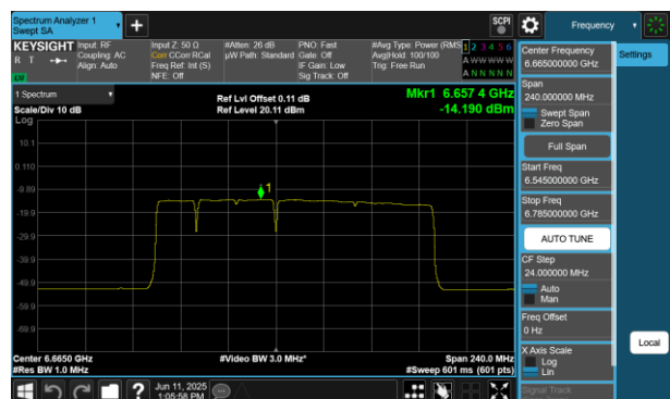
Plot 7-410 PSD SDM Diversity Antenna 2a (160MHz BW 802.11be(RU) RU996+484+242 Index96 - Ch.143)
