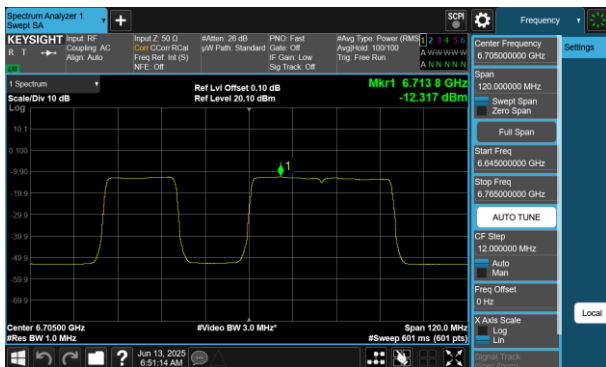
Plot 7-406 PSD SDM Diversity Antenna 4a (80MHz BW 802.11be(RU) RU484+242 Index91 - Ch.151)
