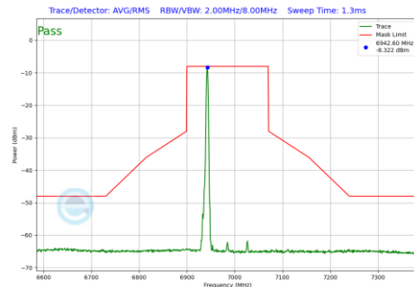
Plot 7-456 In-Band Emission Plot Antenna WF5B (160MHz BW 802.11be(RU) RU26 Index17 (UNII Band 8) - Ch.207)
