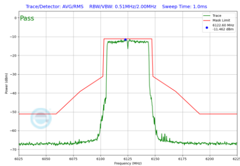
Plot 7-470 In-Band Emission Plot Antenna WF5B (40MHz BW 802.11be(RU) RU484 Index65 (UNII Band 5) - Ch.35)
