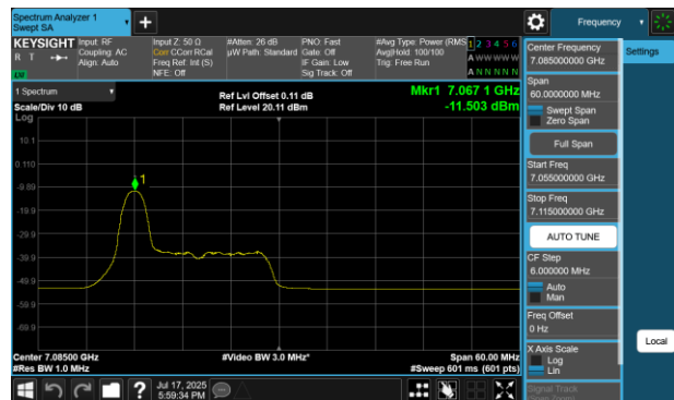
Plot 7-424 PSD SDM Diversity Antenna 2a (40MHz BW 802.11be(RU) RU26 Index0 - Ch.227)
