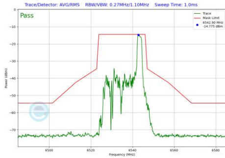
Plot 7-449 In-Band Emission Plot Antenna WF5B (20MHz BW 802.11be(RU) RU26 Index8 (UNII Band 7) - Ch.117)
