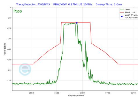
Plot 7-463 In-Band Emission Plot Antenna WF5B (20MHz BW 802.11be(RU) RU106+26 Index82 (UNII Band 7) - Ch.149)
