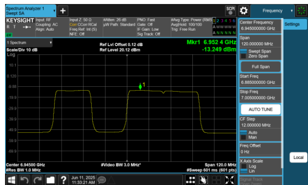
Plot 7-431 PSD SDM Diversity Antenna 2a (80MHz BW 802.11be(RU) RU484+242 Index91 - Ch.199)
