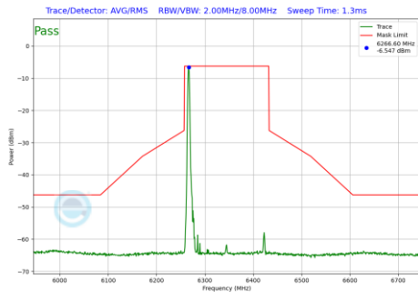
Plot 7-444 In-Band Emission Plot Antenna WF5B (160MHz BW 802.11be(RU) RU26 Index0 (UNII Band 5) - Ch.79)
