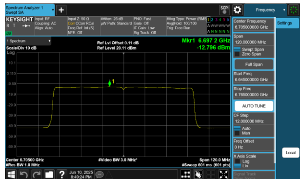
Plot 7-417 PSD SDM Diversity Antenna 2a (80MHz BW 802.11be(RU) RU996 Index67 - Ch.151)
