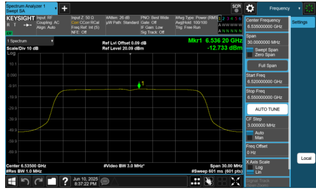
Plot 7-415 PSD SDM Diversity Antenna 2a (20MHz BW 802.11be(RU) RU242 Index61 - Ch.117)
