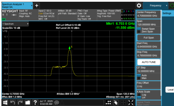
Plot 7-399 PSD SDM Diversity Antenna 4a (80MHz BW 802.11be(RU) RU26 Index17 - Ch.151)
