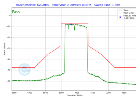
Plot 7-468 In-Band Emission Plot Antenna WF5B (160MHz BW 802.11be(RU) RU996+484+242 Index96 (UNII Band 8) - Ch.207)
