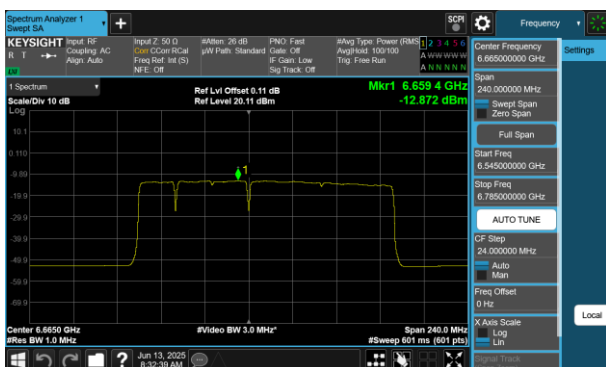
Plot 7-407 PSD SDM Diversity Antenna 4a (160MHz BW 802.11be(RU) RU996+484+242 Index96 - Ch.143)
