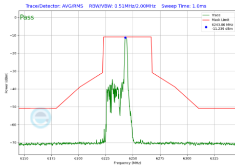
Plot 7-442 In-Band Emission Plot Antenna WF5B (40MHz BW 802.11be(RU) RU26 Index8 (UNII Band 5) - Ch.59)
