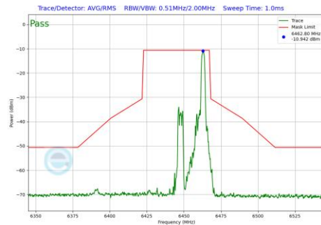
Plot 7-446 In-Band Emission Plot Antenna WF5B (40MHz BW 802.11be(RU) RU26 Index17 (UNII Band 6) - Ch.99)
