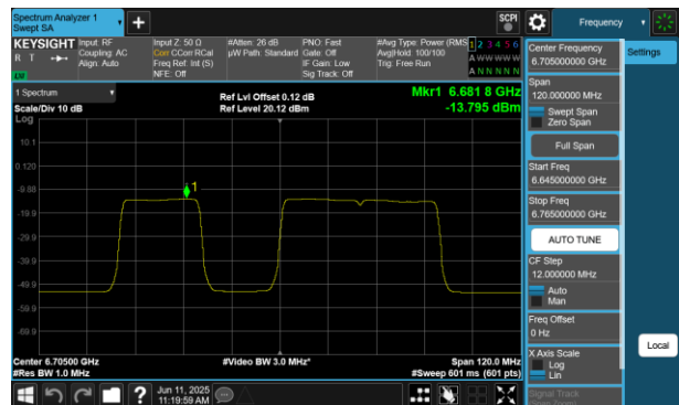
Plot 7-409 PSD SDM Diversity Antenna 2a (80MHz BW 802.11be(RU) RU484+242 Index91 - Ch.151)
