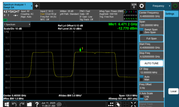
Plot 7-387 PSD SDM Diversity Antenna 2a (80MHz BW 802.11be(RU) RU484+242 Index91 - Ch.103)
