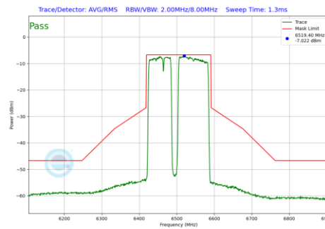
Plot 7-462 In-Band Emission Plot Antenna WF5B (160MHz BW 802.11be(RU) RU996+484+242 Index99 (UNII Band 6) - Ch.111)
