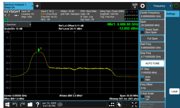
Plot 7-401 PSD SDM Diversity Antenna 2a (20MHz BW 802.11be(RU) RU26 Index0 - Ch.149)
