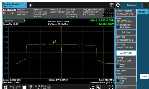
Plot 7-418 PSD SDM Diversity Antenna 2a (160MHz BW 802.11be(RU) RU996X2 Index68 - Ch.175)
