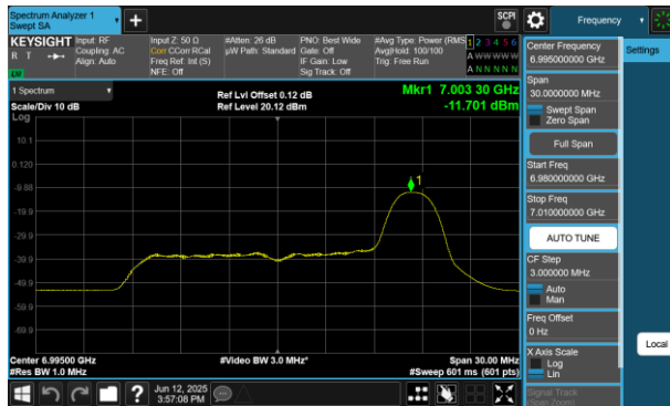
Plot 7-419 PSD SDM Diversity Antenna 4a (20MHz BW 802.11be(RU) RU26 Index8 - Ch.209)
