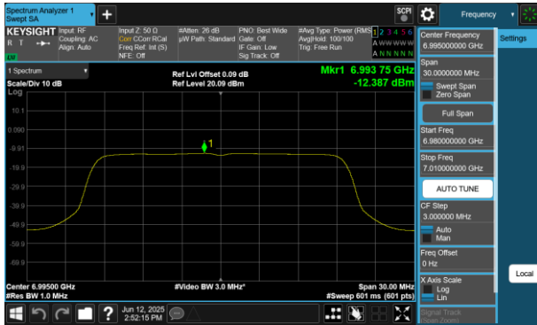
Plot 7-433 PSD SDM Diversity Antenna 4a (20MHz BW 802.11be(RU) RU242 Index61 - Ch.209)
