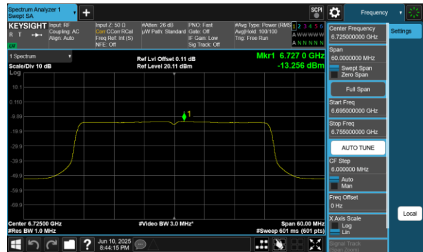
Plot 7-416 PSD SDM Diversity Antenna 2a (40MHz BW 802.11be(RU) RU484 Index65 - Ch.155)
