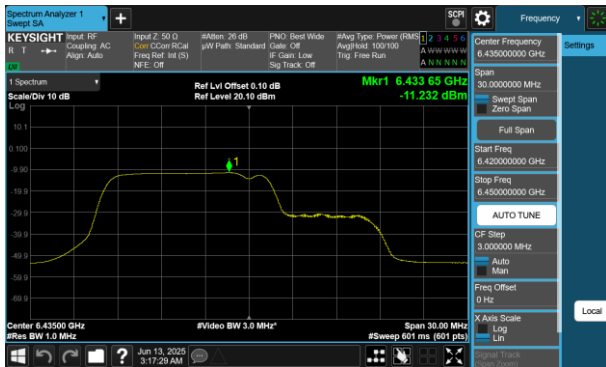
Plot 7-383 PSD SDM Diversity Antenna 4a (20MHz BW 802.11be(RU) RU106+26 Index82 - Ch.97)
