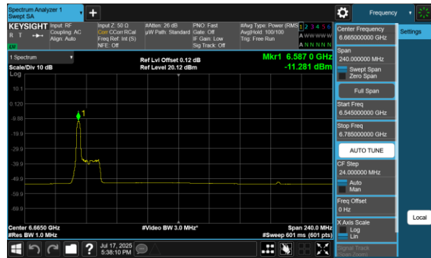
Plot 7-404 PSD SDM Diversity Antenna 2a (160MHz BW 802.11be(RU) RU26 Index0 - Ch.143)
