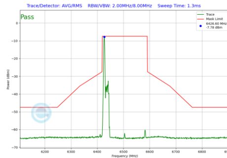
Plot 7-448 In-Band Emission Plot Antenna WF5B (160MHz BW 802.11be(RU) RU26 Index0 (UNII Band 6) - Ch.111)
