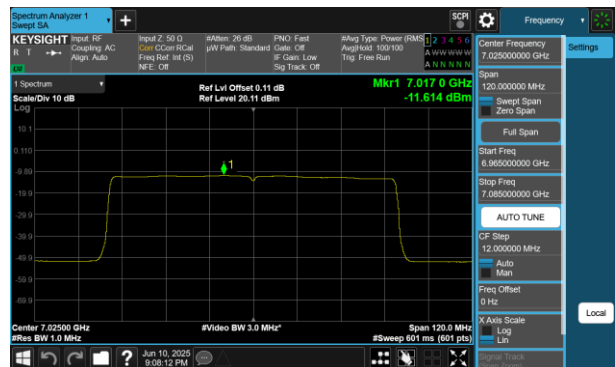
Plot 7-439 PSD SDM Diversity Antenna 2a (80MHz BW 802.11be(RU) RU996 Index67 - Ch.215)
