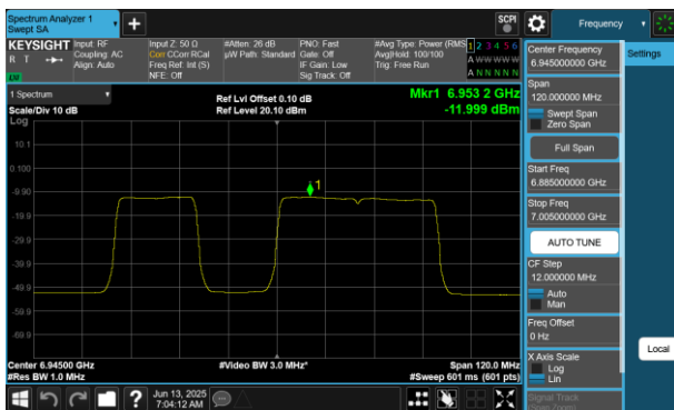
Plot 7-428 PSD SDM Diversity Antenna 4a (80MHz BW 802.11be(RU) RU484+242 Index91 - Ch.199)
