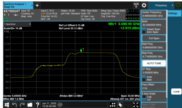
Plot 7-408 PSD SDM Diversity Antenna 2a (20MHz BW 802.11be(RU) RU106+26 Index83 - Ch.149)
