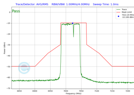
Plot 7-467 In-Band Emission Plot Antenna WF5B (80MHz BW 802.11be(RU) RU484+242 Index93 (UNII Band 8) - Ch.215)
