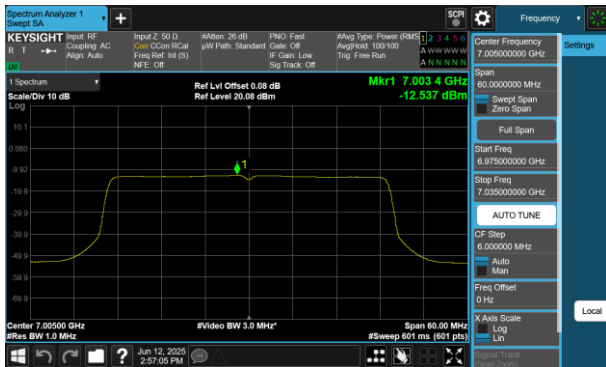
Plot 7-434 PSD SDM Diversity Antenna 4a (40MHz BW 802.11be(RU) RU484 Index65 - Ch.211)
