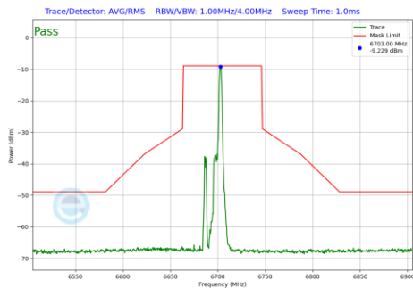
Plot 7-451 In-Band Emission Plot Antenna WF5B (80MHz BW 802.11be(RU) RU26 Index17 (UNII Band 7) - Ch.151)
