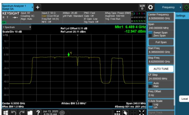
Plot 7-385 PSD SDM Diversity Antenna 4a (160MHz BW 802.11be(RU) RU996+484+242 Index98 - Ch.111)
