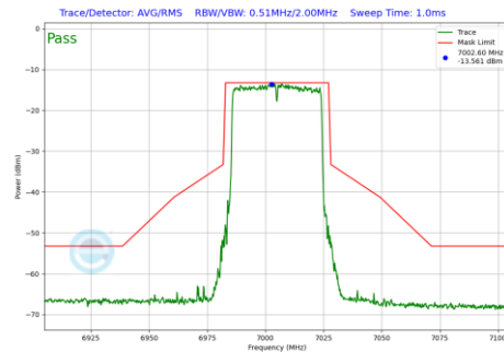
Plot 7-482 In-Band Emission Plot Antenna WF5B (40MHz BW 802.11be(RU) RU484 Index65 (UNII Band 8) - Ch.211)
