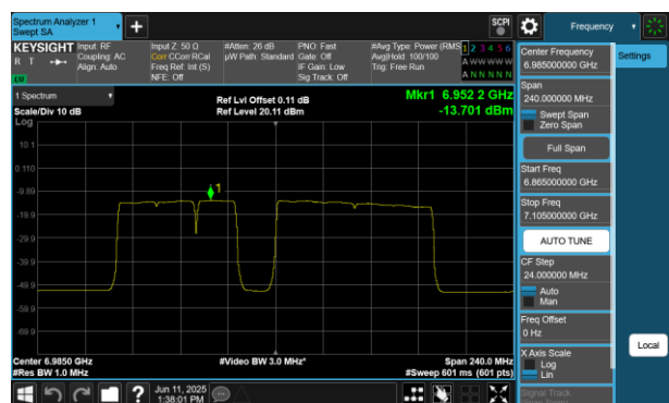
Plot 7-432 PSD SDM Diversity Antenna 2a (160MHz BW 802.11be(RU) RU996+484+242 Index99 - Ch.207)
