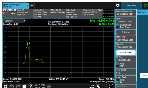
Plot 7-425 PSD SDM Diversity Antenna 2a (80MHz BW 802.11be(RU) RU26 Index0 - Ch.199)
