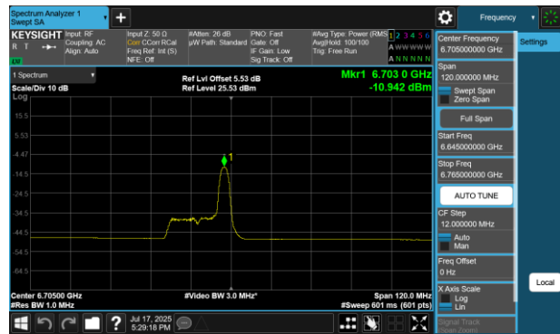
Plot 7-403 PSD SDM Diversity Antenna 2a (80MHz BW 802.11be(RU) RU26 Index17 - Ch.151)
