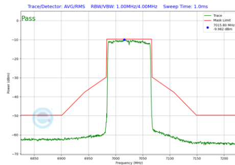
Plot 7-483 In-Band Emission Plot Antenna WF5B (80MHz BW 802.11be(RU) RU996 Index67 (UNII Band 8) - Ch.215)
