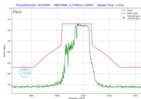
Plot 7-466 In-Band Emission Plot Antenna WF5B (20MHz BW 802.11be(RU) RU106+26 Index83 (UNII Band 8) - Ch.229)
