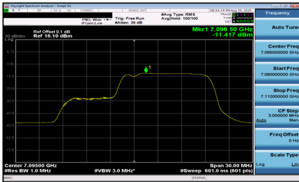
Plot 7-427 PSD SDM Diversity Antenna 4a (20MHz BW 802.11be(RU) RU106+26 Index83 - Ch.229)
