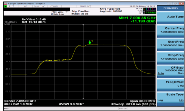
Plot 7-430 PSD SDM Diversity Antenna 2a (20MHz BW 802.11be(RU) RU106+26 Index83 - Ch.229)
