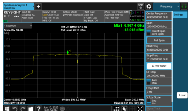
Plot 7-440 PSD SDM Diversity Antenna 2a (160MHz BW 802.11be(RU) RU996X2 Index68 - Ch.207)
