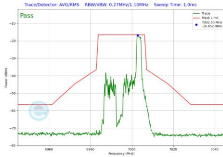
Plot 7-597 In-Band Emission Plot CDD Primary Antenna WF5B (20MHz BW 802.11be(RU) RU26 Index8 (UNII Band 8) - Ch.209)
