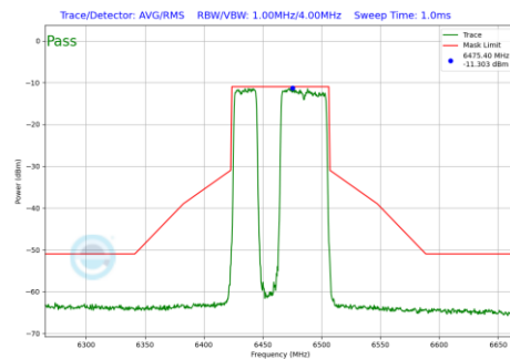
Plot 7-615 In-Band Emission Plot CDD Primary Antenna 4a (80MHz BW 802.11be(RU) RU484+242 Index91 (UNII Band 6) - Ch.103)
