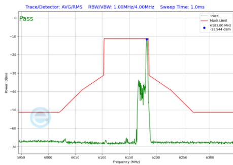
Plot 7-575 In-Band Emission Plot CDD Primary Antenna WF5B (80MHz BW 802.11be(RU) RU26 Index36 (UNII Band 5) - Ch.39)
