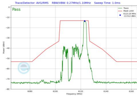
Plot 7-529 In-Band Emission Plot Antenna 2a (20MHz BW 802.11be(RU) RU26 Index8 (UNII Band 5) - Ch.33)
