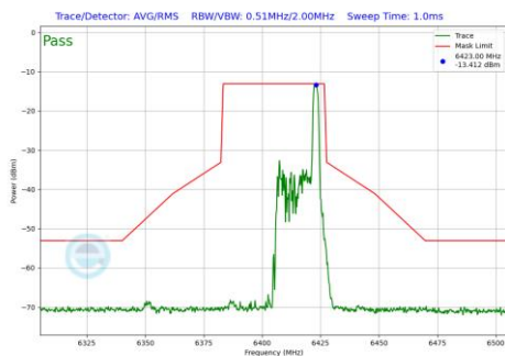
Plot 7-574 In-Band Emission Plot CDD Primary Antenna WF5B (40MHz BW 802.11be(RU) RU26 Index17 (UNII Band 5) - Ch.91)
