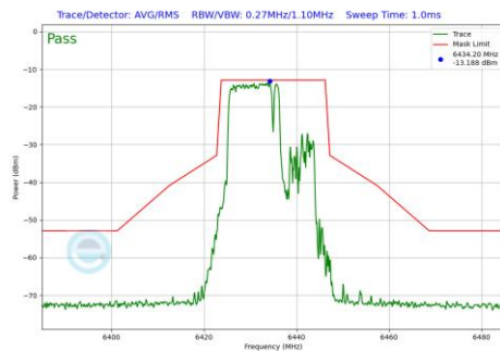
Plot 7-504 In-Band Emission Plot Antenna 4a (20MHz BW 802.11be(RU) RU106+26 Index82 (UNII Band 6) - Ch.97)
