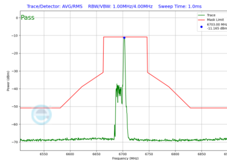
Plot 7-595 In-Band Emission Plot SDM Primary Antenna 4a (80MHz BW 802.11be(RU) RU26 Index17 (UNII Band 7) - Ch.151)
