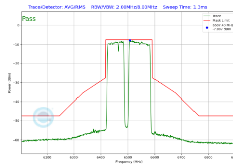
Plot 7-550 In-Band Emission Plot Antenna 2a (160MHz BW 802.11be(RU) RU996+484+242 Index99 (UNII Band 6) - Ch.111)
