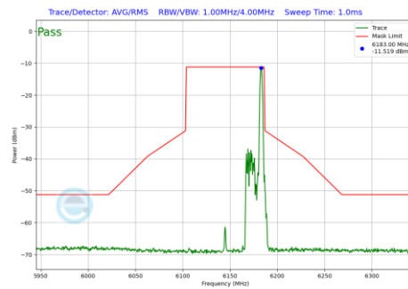
Plot 7-579 In-Band Emission Plot CDD Primary Antenna 4a (80MHz BW 802.11be(RU) RU26 Index36 (UNII Band 5) - Ch.39)
