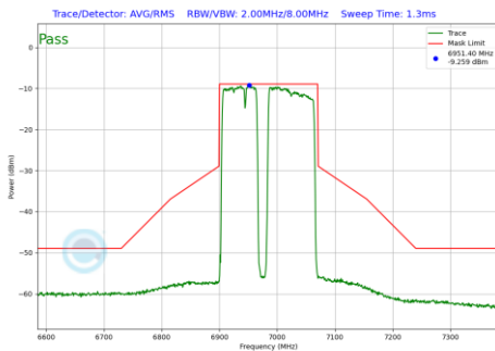
Plot 7-625 In-Band Emission Plot CDD Primary Antenna WF5B (160MHz BW 802.11be(RU) RU996+484+242 Index99 (UNII Band 8) - Ch.207)
