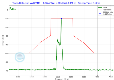
Plot 7-495 In-Band Emission Plot Antenna 4a (80MHz BW 802.11be(RU) RU26 Index17 (UNII Band 7) - Ch.183)
