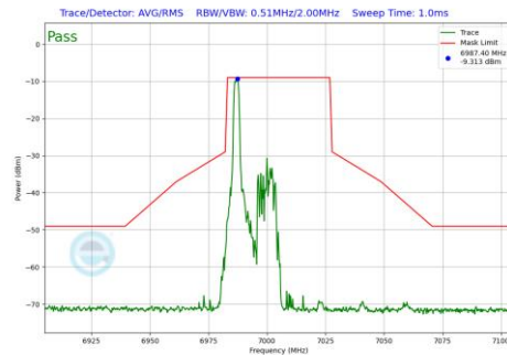
Plot 7-498 In-Band Emission Plot Antenna 4a (40MHz BW 802.11be(RU) RU26 Index0 (UNII Band 8) - Ch.211)
