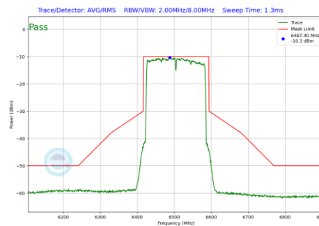
Plot 7-644 In-Band Emission Plot CDD Primary Antenna 4a (160MHz BW 802.11be(RU) RU996X2 Index68 (UNII Band 6) - Ch.111)
