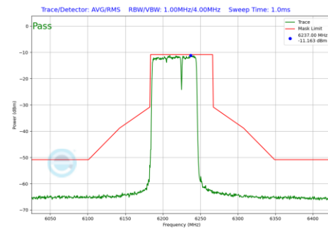
Plot 7-609 In-Band Emission Plot CDD Primary Antenna 4a (80MHz BW 802.11be(RU) RU484+242 Index93 (UNII Band 5) - Ch.55)
