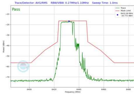
Plot 7-611 In-Band Emission Plot CDD Primary Antenna WF5B (20MHz BW 802.11be(RU) RU106+26 Index82 (UNII Band 6) - Ch.97)
