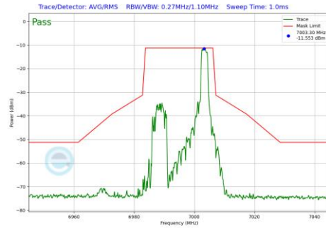
Plot 7-497 In-Band Emission Plot Antenna 4a (20MHz BW 802.11be(RU) RU26 Index8 (UNII Band 8) - Ch.209)
