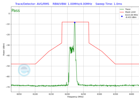
Plot 7-487 In-Band Emission Plot Antenna 4a (80MHz BW 802.11be(RU) RU26 Index17 (UNII Band 5) - Ch.55)
