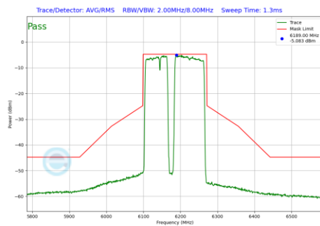
Plot 7-503 In-Band Emission Plot Antenna 4a (160MHz BW 802.11be(RU) RU996+484+242 Index99 (UNII Band 5) - Ch.47)
