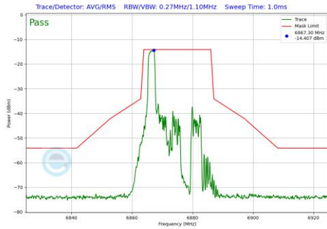
Plot 7-493 In-Band Emission Plot Antenna 4a (20MHz BW 802.11be(RU) RU26 Index0 (UNII Band 7) - Ch.185)
