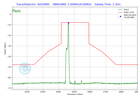
Plot 7-588 In-Band Emission Plot SDM Primary Antenna 4a (160MHz BW 802.11be(RU) RU26 Index17 (UNII Band 6) - Ch.111)
