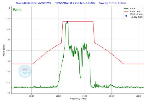
Plot 7-485 In-Band Emission Plot Antenna 4a (20MHz BW 802.11be(RU) RU26 Index0 (UNII Band 5) - Ch.33)
