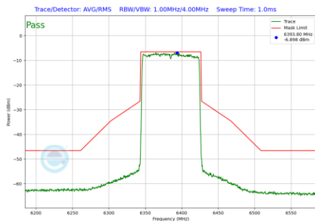
Plot 7-515 In-Band Emission Plot Antenna 4a (80MHz BW 802.11be(RU) RU996 Index67 (UNII Band 5) - Ch.87)
