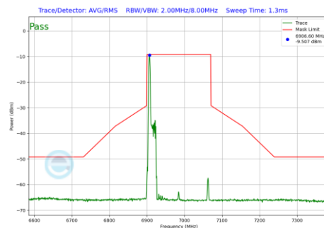
Plot 7-544 In-Band Emission Plot Antenna 2a (160MHz BW 802.11be(RU) RU26 Index0 (UNII Band 8) - Ch.207)
