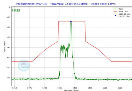
Plot 7-586 In-Band Emission Plot CDD Primary Antenna 4a (40MHz BW 802.11be(RU) RU26 Index8 (UNII Band 6) - Ch.99)
