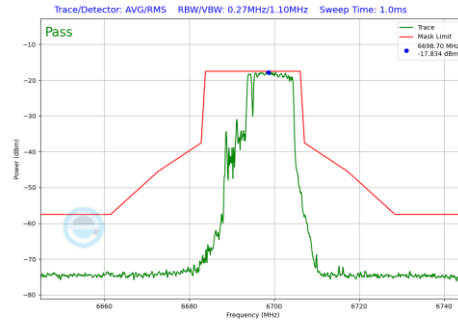
Plot 7-620 In-Band Emission Plot CDD Primary Antenna 4a (20MHz BW 802.11be(RU) RU106+26 Index83 (UNII Band 7) - Ch.149)
