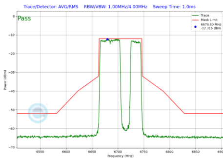
Plot 7-618 In-Band Emission Plot CDD Primary Antenna WF5B (80MHz BW 802.11be(RU) RU484+242 Index92 (UNII Band 7) - Ch.151)
