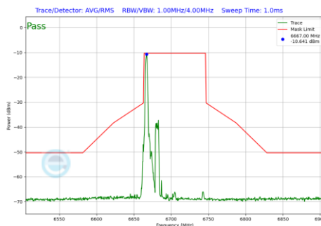
Plot 7-539 In-Band Emission Plot Antenna 2a (80MHz BW 802.11be(RU) RU26 Index0 (UNII Band 7) - Ch.151)
