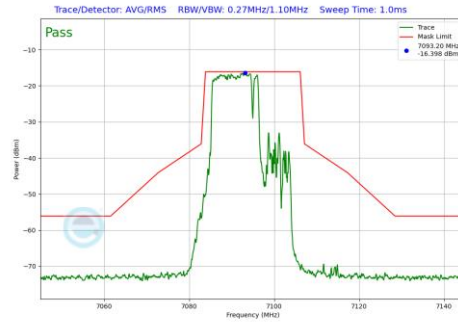
Plot 7-626 In-Band Emission Plot CDD Primary Antenna 4a (20MHz BW 802.11be(RU) RU106+26 Index82 (UNII Band 8) - Ch.229)
