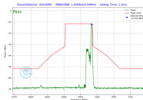
Plot 7-543 In-Band Emission Plot Antenna 2a (80MHz BW 802.11be(RU) RU26 Index36 (UNII Band 8) - Ch.199)
