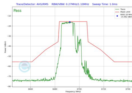
Plot 7-551 In-Band Emission Plot Antenna 2a (20MHz BW 802.11be(RU) RU106+26 Index82 (UNII Band 7) - Ch.149)
