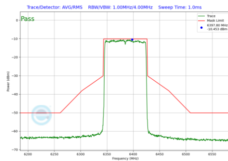
Plot 7-635 In-Band Emission Plot CDD Primary Antenna 4a (80MHz BW 802.11be(RU) RU996 Index67 (UNII Band 5) - Ch.87)
