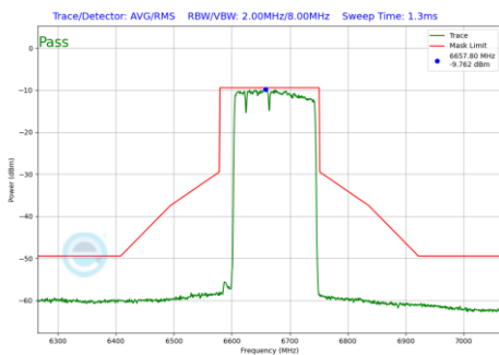
Plot 7-619 In-Band Emission Plot CDD Primary Antenna WF5B (160MHz BW 802.11be(RU) RU996+484+242 Index96 (UNII Band 7) - Ch.143)
