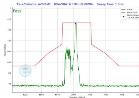
Plot 7-542 In-Band Emission Plot Antenna 2a (40MHz BW 802.11be(RU) RU26 Index8 (UNII Band 8) - Ch.211)
