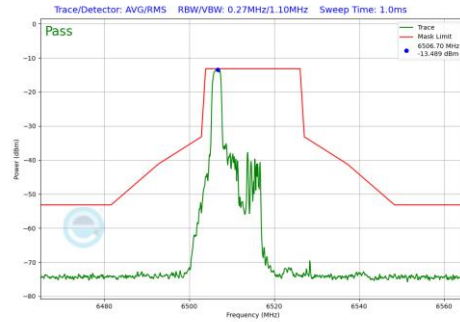
Plot 7-489 In-Band Emission Plot Antenna 4a (20MHz BW 802.11be(RU) RU26 Index0 (UNII Band 6) - Ch.113)
