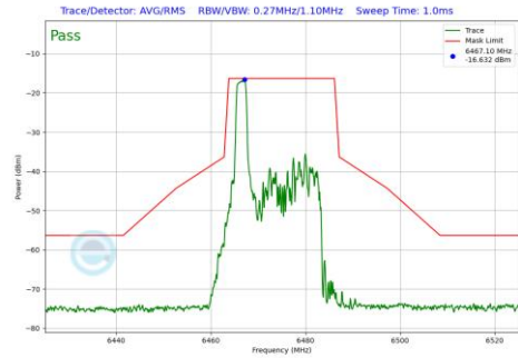
Plot 7-585 In-Band Emission Plot CDD Primary Antenna 4a (20MHz BW 802.11be(RU) RU26 Index0 (UNII Band 6) - Ch.105)
