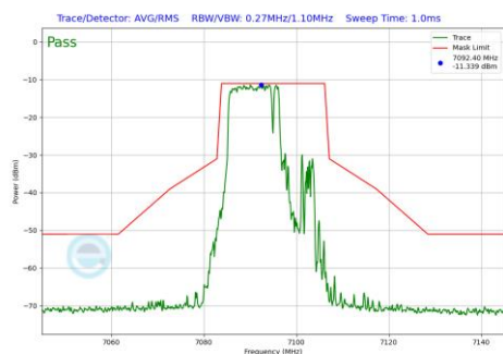
Plot 7-510 In-Band Emission Plot Antenna 4a (20MHz BW 802.11be(RU) RU106+26 Index82 (UNII Band 8) - Ch.229)
