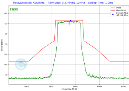
Plot 7-637 In-Band Emission Plot CDD Primary Antenna WF5B (20MHz BW 802.11be(RU) RU242 Index61 (UNII Band 6) - Ch.97)
