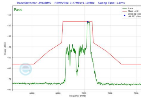
Plot 7-601 In-Band Emission Plot CDD Primary Antenna 4a (20MHz BW 802.11be(RU) RU26 Index8 (UNII Band 8) - Ch.209)
