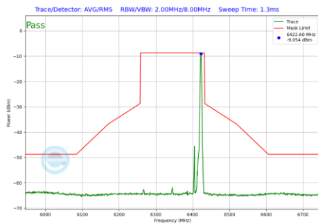
Plot 7-576 In-Band Emission Plot CDD Primary Antenna WF5B (160MHz BW 802.11be(RU) RU26 Index36 (UNII Band 5) - Ch.79)
