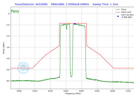
Plot 7-607 In-Band Emission Plot CDD Primary Antenna WF5B (160MHz BW 802.11be(RU) RU996+484+242 Index99 (UNII Band 5) - Ch.79)
