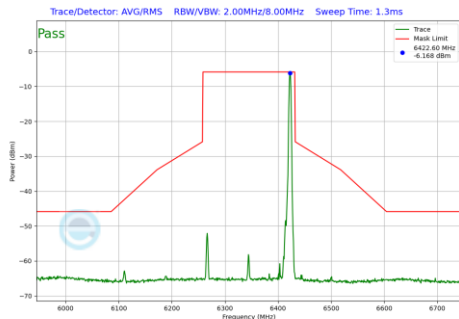
Plot 7-488 In-Band Emission Plot Antenna 4a (160MHz BW 802.11be(RU) RU26 Index36 (UNII Band 5) - Ch.79)
