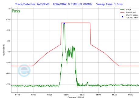
Plot 7-538 In-Band Emission Plot Antenna 2a (40MHz BW 802.11be(RU) RU26 Index0 (UNII Band 7) - Ch.123)
