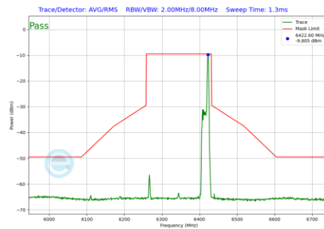
Plot 7-580 In-Band Emission Plot CDD Primary Antenna 4a (160MHz BW 802.11be(RU) RU26 Index36 (UNII Band 5) - Ch.79)
