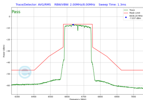
Plot 7-524 In-Band Emission Plot Antenna 4a (160MHz BW 802.11be(RU) RU996X2 Index68 (UNII Band 7) - Ch.143)
