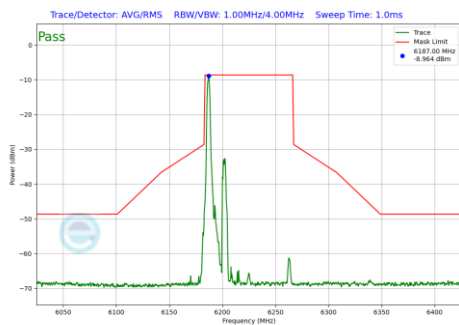
Plot 7-531 In-Band Emission Plot Antenna 2a (80MHz BW 802.11be(RU) RU26 Index0 (UNII Band 5) - Ch.55)
