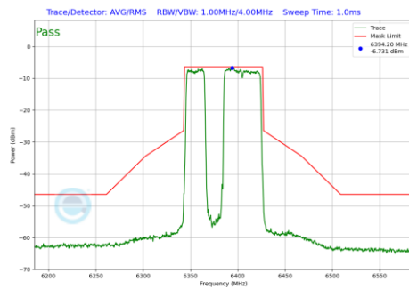
Plot 7-502 In-Band Emission Plot Antenna 4a (80MHz BW 802.11be(RU) RU484+242 Index91 (UNII Band 5) - Ch.87)
