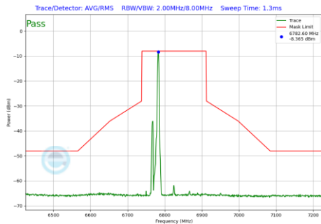
Plot 7-496 In-Band Emission Plot Antenna 4a (160MHz BW 802.11be(RU) RU26 Index17 (UNII Band 7) - Ch.175)
