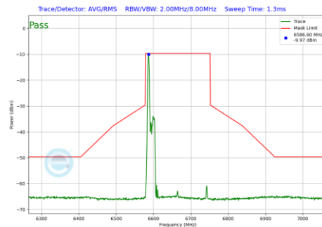
Plot 7-596 In-Band Emission Plot SDM Primary Antenna 4a (160MHz BW 802.11be(RU) RU26 Index0 (UNII Band 7) - Ch.143)
