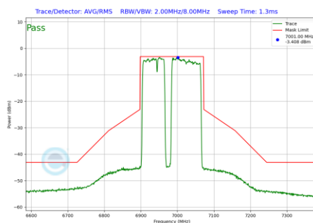
Plot 7-512 In-Band Emission Plot Antenna 4a (160MHz BW 802.11be(RU) RU996+484+242 Index99 (UNII Band 8) - Ch.207)
