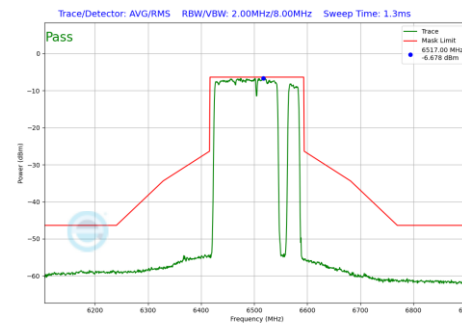
Plot 7-506 In-Band Emission Plot Antenna 4a (160MHz BW 802.11be(RU) RU996+484+242 Index98 (UNII Band 6) - Ch.111)
