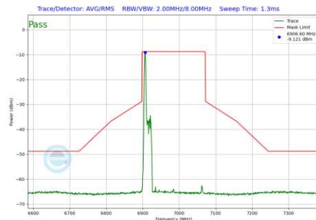
Plot 7-604 In-Band Emission Plot SDM Primary Antenna 4a (160MHz BW 802.11be(RU) RU26 Index0 (UNII Band 8) - Ch.207)
