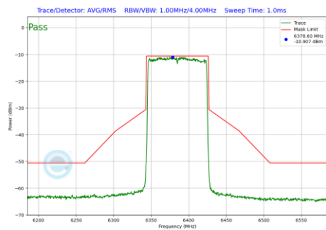
Plot 7-631 In-Band Emission Plot CDD Primary Antenna WF5B (80MHz BW 802.11be(RU) RU996 Index67 (UNII Band 5) - Ch.87)
