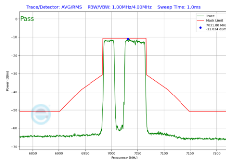
Plot 7-555 In-Band Emission Plot Antenna 2a (80MHz BW 802.11be(RU) RU484+242 Index91 (UNII Band 8) - Ch.215)
