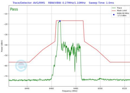
Plot 7-581 In-Band Emission Plot CDD Primary Antenna WF5B (20MHz BW 802.11be(RU) RU26 Index0 (UNII Band 6) - Ch.105)
