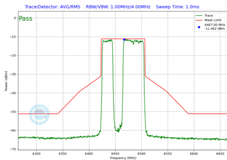
Plot 7-612 In-Band Emission Plot CDD Primary Antenna WF5B (80MHz BW 802.11be(RU) RU484+242 Index91 (UNII Band 6) - Ch.103)
