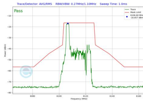
Plot 7-577 In-Band Emission Plot CDD Primary Antenna 4a (20MHz BW 802.11be(RU) RU26 Index0 (UNII Band 5) - Ch.33)
