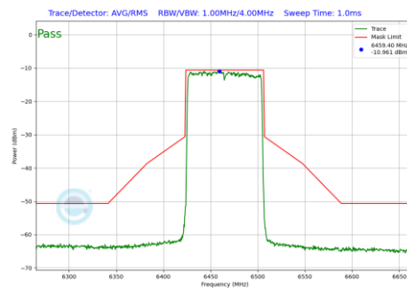
Plot 7-643 In-Band Emission Plot CDD Primary Antenna 4a (80MHz BW 802.11be(RU) RU996 Index67 (UNII Band 6) - Ch.103)
