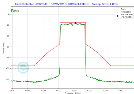
Plot 7-559 In-Band Emission Plot Antenna 2a (80MHz BW 802.11be(RU) RU996 Index67 (UNII Band 5) - Ch.39)
