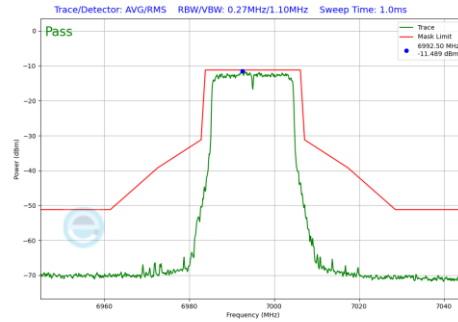
Plot 7-525 In-Band Emission Plot Antenna 4a (20MHz BW 802.11be(RU) RU242 Index61 (UNII Band 8) - Ch.209)
