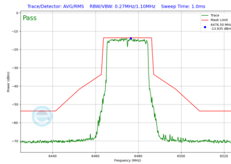
Plot 7-561 In-Band Emission Plot Antenna 2a (20MHz BW 802.11be(RU) RU242 Index61 (UNII Band 6) - Ch.105)
