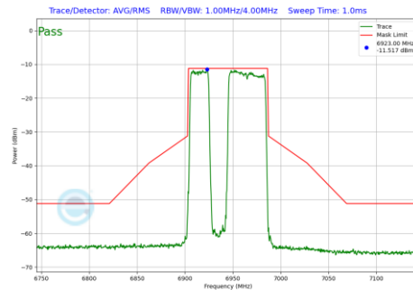
Plot 7-627 In-Band Emission Plot CDD Primary Antenna 4a (80MHz BW 802.11be(RU) RU484+242 Index91 (UNII Band 8) - Ch.199)
