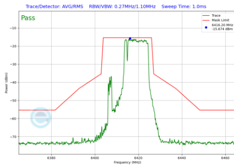
Plot 7-605 In-Band Emission Plot CDD Primary Antenna WF5B (20MHz BW 802.11be(RU) RU106+26 Index83 (UNII Band 5) - Ch.93)
