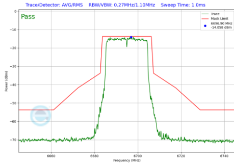
Plot 7-565 In-Band Emission Plot Antenna 2a (20MHz BW 802.11be(RU) RU242 Index61 (UNII Band 7) - Ch.149)
