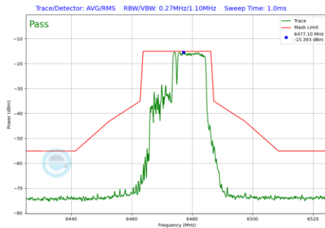
Plot 7-548 In-Band Emission Plot Antenna 2a (20MHz BW 802.11be(RU) RU106+26 Index83 (UNII Band 6) - Ch.105)
