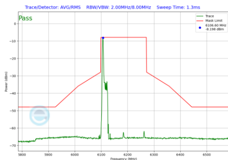
Plot 7-532 In-Band Emission Plot Antenna 2a (160MHz BW 802.11be(RU) RU26 Index0 (UNII Band 5) - Ch.47)
