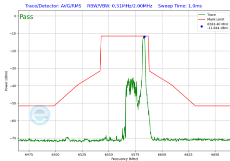
Plot 7-494 In-Band Emission Plot Antenna 4a (40MHz BW 802.11be(RU) RU26 Index17 (UNII Band 7) - Ch.123)
