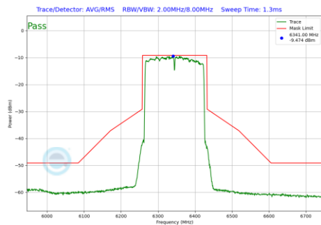
Plot 7-632 In-Band Emission Plot CDD Primary Antenna WF5B (160MHz BW 802.11be(RU) RU996X2 Index68 (UNII Band 5) - Ch.79)
