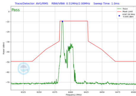
Plot 7-486 In-Band Emission Plot Antenna 4a (40MHz BW 802.11be(RU) RU26 Index0 (UNII Band 5) - Ch.91)
