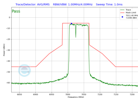
Plot 7-511 In-Band Emission Plot Antenna 4a (80MHz BW 802.11be(RU) RU484+242 Index90 (UNII Band 8) - Ch.215)
