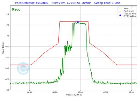
Plot 7-617 In-Band Emission Plot CDD Primary Antenna WF5B (20MHz BW 802.11be(RU) RU106+26 Index83 (UNII Band 7) - Ch.149)
