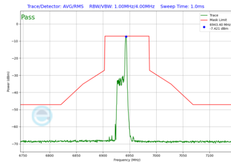
Plot 7-499 In-Band Emission Plot Antenna 4a (80MHz BW 802.11be(RU) RU26 Index17 (UNII Band 8) - Ch.199)
