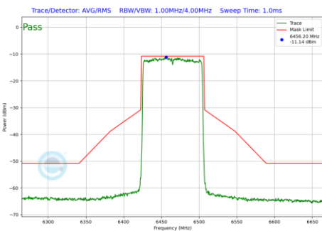
Plot 7-639 In-Band Emission Plot CDD Primary Antenna WF5B (80MHz BW 802.11be(RU) RU996 Index67 (UNII Band 6) - Ch.103)
