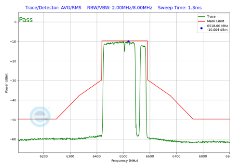
Plot 7-613 In-Band Emission Plot CDD Primary Antenna WF5B (160MHz BW 802.11be(RU) RU996+484+242 Index98 (UNII Band 6) - Ch.111)
