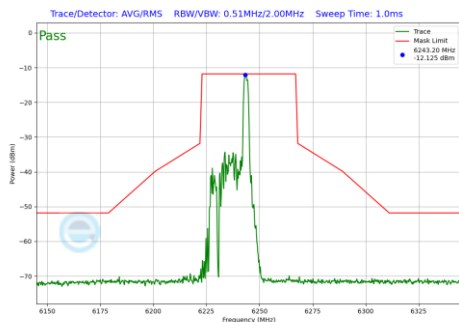
Plot 7-530 In-Band Emission Plot Antenna 2a (40MHz BW 802.11be(RU) RU26 Index8 (UNII Band 5) - Ch.59)
