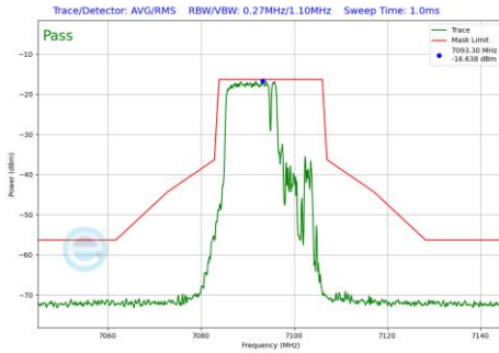
Plot 7-623 In-Band Emission Plot CDD Primary Antenna WF5B (20MHz BW 802.11be(RU) RU106+26 Index82 (UNII Band 8) - Ch.229)
