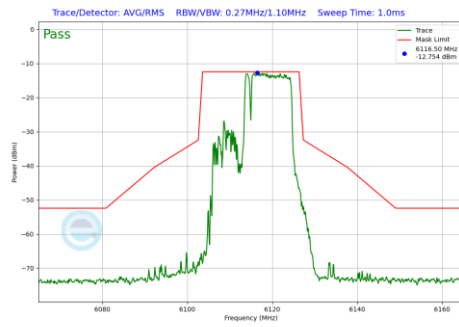
Plot 7-501 In-Band Emission Plot Antenna 4a (20MHz BW 802.11be(RU) RU106+26 Index83 (UNII Band 5) - Ch.33)
