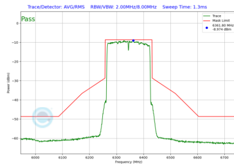
Plot 7-636 In-Band Emission Plot CDD Primary Antenna 4a (160MHz BW 802.11be(RU) RU996X2 Index68 (UNII Band 5) - Ch.79)
