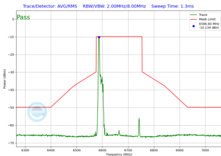
Plot 7-592 In-Band Emission Plot SDM Primary Antenna WF5B (160MHz BW 802.11be(RU) RU26 Index0 (UNII Band 7) - Ch.143)
