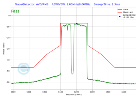
Plot 7-547 In-Band Emission Plot Antenna 2a (160MHz BW 802.11be(RU) RU996+484+242 Index99 (UNII Band 5) - Ch.47)
