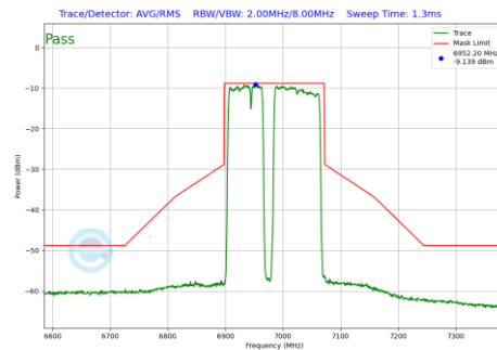
Plot 7-628 In-Band Emission Plot CDD Primary Antenna 4a (160MHz BW 802.11be(RU) RU996+484+242 Index99 (UNII Band 8) - Ch.207)
