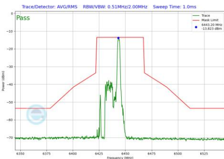
Plot 7-582 In-Band Emission Plot CDD Primary Antenna WF5B (40MHz BW 802.11be(RU) RU26 Index8 (UNII Band 6) - Ch.99)
