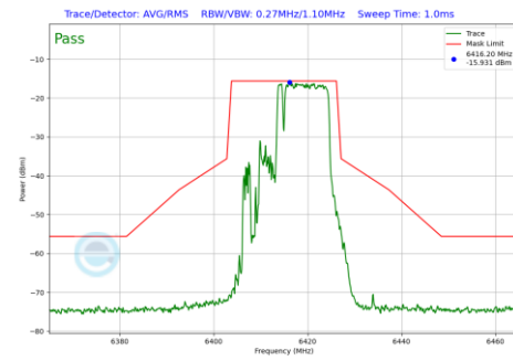
Plot 7-608 In-Band Emission Plot CDD Primary Antenna 4a (20MHz BW 802.11be(RU) RU106+26 Index83 (UNII Band 5) - Ch.93)
