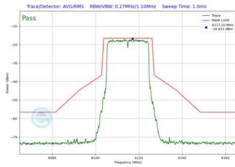
Plot 7-629 In-Band Emission Plot CDD Primary Antenna WF5B (20MHz BW 802.11be(RU) RU242 Index61 (UNII Band 5) - Ch.33)
