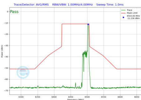
Plot 7-583 In-Band Emission Plot CDD Primary Antenna WF5B (80MHz BW 802.11be(RU) RU26 Index36 (UNII Band 6) - Ch.103)
