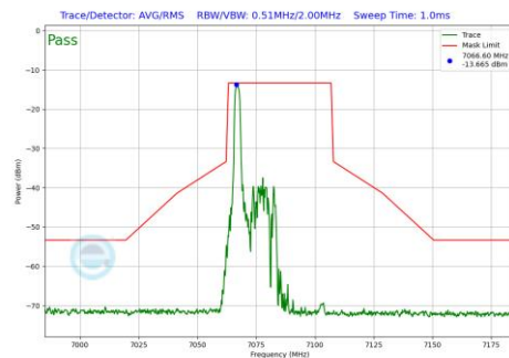
Plot 7-602 In-Band Emission Plot SDM Primary Antenna 4a (40MHz BW 802.11be(RU) RU26 Index0 (UNII Band 8) - Ch.227)
