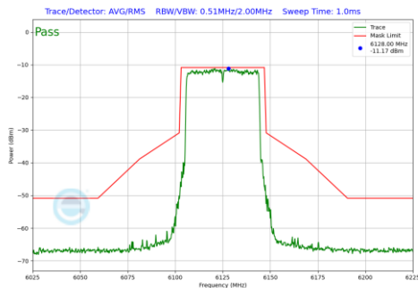
Plot 7-558 In-Band Emission Plot Antenna 2a (40MHz BW 802.11be(RU) RU484 Index65 (UNII Band 5) - Ch.35)
