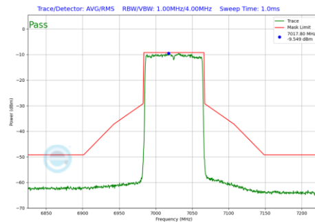
Plot 7-571 In-Band Emission Plot Antenna 2a (80MHz BW 802.11be(RU) RU996 Index67 (UNII Band 8) - Ch.215)
