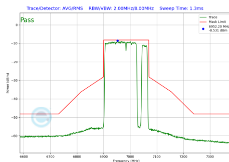
Plot 7-556 In-Band Emission Plot Antenna 2a (160MHz BW 802.11be(RU) RU996+484+242 Index98 (UNII Band 8) - Ch.207)
