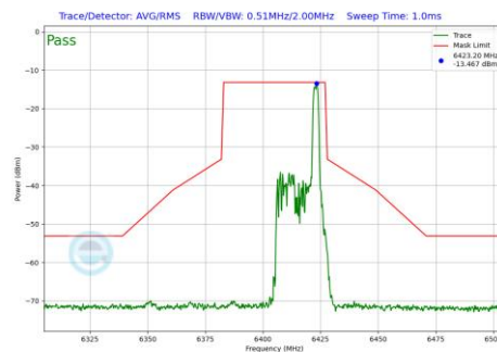
Plot 7-578 In-Band Emission Plot CDD Primary Antenna 4a (40MHz BW 802.11be(RU) RU26 Index17 (UNII Band 5) - Ch.91)
