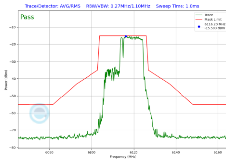
Plot 7-545 In-Band Emission Plot Antenna 2a (20MHz BW 802.11be(RU) RU106+26 Index83 (UNII Band 5) - Ch.33)
