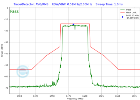
Plot 7-638 In-Band Emission Plot CDD Primary Antenna WF5B (40MHz BW 802.11be(RU) RU484 Index65 (UNII Band 6) - Ch.107)
