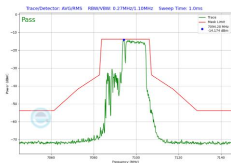
Plot 7-554 In-Band Emission Plot Antenna 2a (20MHz BW 802.11be(RU) RU106+26 Index83 (UNII Band 8) - Ch.229)
