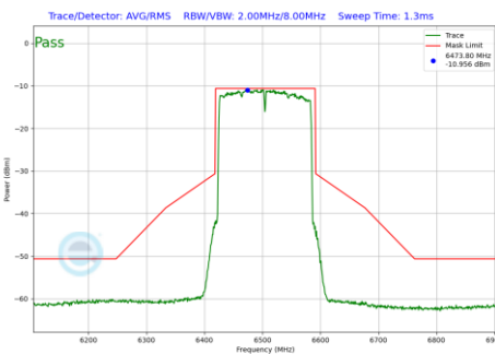
Plot 7-640 In-Band Emission Plot CDD Primary Antenna WF5B (160MHz BW 802.11be(RU) RU996X2 Index68 (UNII Band 6) - Ch.111)
