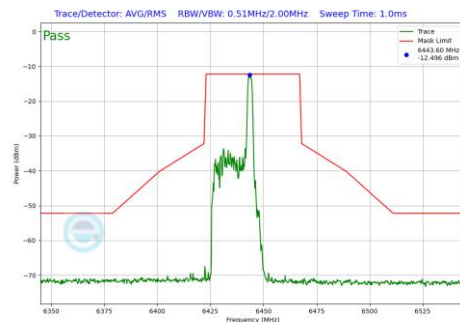
Plot 7-534 In-Band Emission Plot Antenna 2a (40MHz BW 802.11be(RU) RU26 Index8 (UNII Band 6) - Ch.99)
