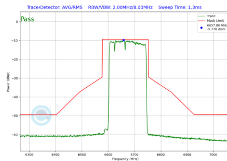
Plot 7-622 In-Band Emission Plot CDD Primary Antenna 4a (160MHz BW 802.11be(RU) RU996+484+242 Index96 (UNII Band 7) - Ch.143)
