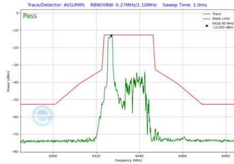
Plot 7-533 In-Band Emission Plot Antenna 2a (20MHz BW 802.11be(RU) RU26 Index0 (UNII Band 6) - Ch.97)
