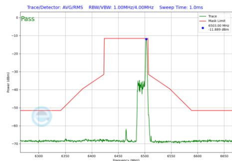
Plot 7-587 In-Band Emission Plot CDD Primary Antenna 4a (80MHz BW 802.11be(RU) RU26 Index36 (UNII Band 6) - Ch.103)
