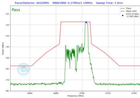
Plot 7-589 In-Band Emission Plot CDD Primary Antenna WF5B (20MHz BW 802.11be(RU) RU26 Index8 (UNII Band 7) - Ch.149)
