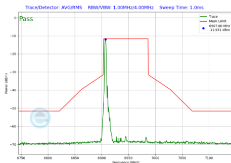
Plot 7-599 In-Band Emission Plot SDM Primary Antenna WF5B (80MHz BW 802.11be(RU) RU26 Index0 (UNII Band 8) - Ch.199)
