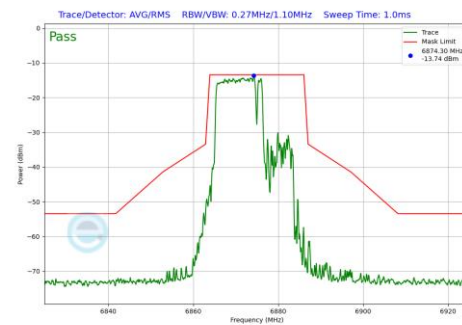
Plot 7-507 In-Band Emission Plot Antenna 4a (20MHz BW 802.11be(RU) RU106+26 Index82 (UNII Band 7) - Ch.185)
