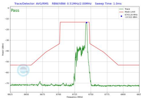
Plot 7-590 In-Band Emission Plot SDM Primary Antenna WF5B (40MHz BW 802.11be(RU) RU26 Index17 (UNII Band 7) - Ch.155)
