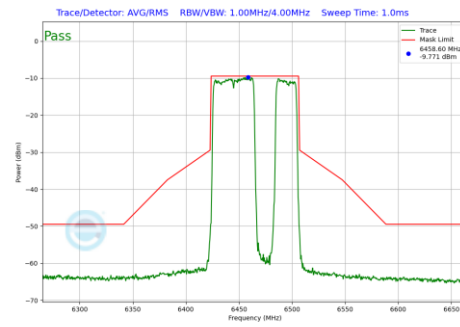
Plot 7-549 In-Band Emission Plot Antenna 2a (80MHz BW 802.11be(RU) RU484+242 Index92 (UNII Band 6) - Ch.103)
