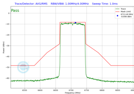
Plot 7-567 In-Band Emission Plot Antenna 2a (80MHz BW 802.11be(RU) RU996 Index67 (UNII Band 7) - Ch.151)
