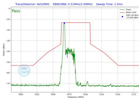
Plot 7-598 In-Band Emission Plot SDM Primary Antenna WF5B (40MHz BW 802.11be(RU) RU26 Index0 (UNII Band 8) - Ch.227)
