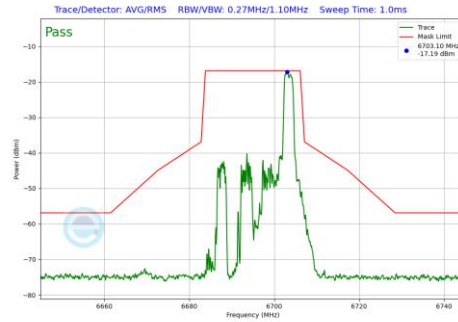
Plot 7-593 In-Band Emission Plot CDD Primary Antenna 4a (20MHz BW 802.11be(RU) RU26 Index8 (UNII Band 7) - Ch.149)
