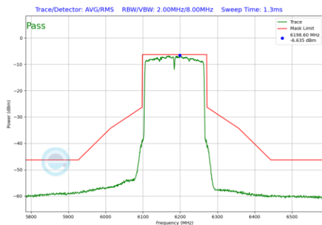
Plot 7-560 In-Band Emission Plot Antenna 2a (160MHz BW 802.11be(RU) RU996X2 Index68 (UNII Band 5) - Ch.47)
