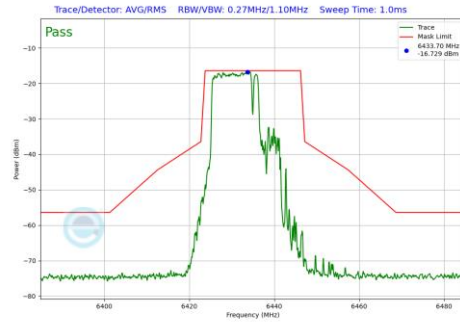
Plot 7-614 In-Band Emission Plot CDD Primary Antenna 4a (20MHz BW 802.11be(RU) RU106+26 Index82 (UNII Band 6) - Ch.97)
