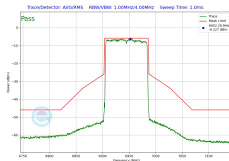
Plot 7-527 In-Band Emission Plot Antenna 4a (80MHz BW 802.11be(RU) RU996 Index67 (UNII Band 8) - Ch.199)
