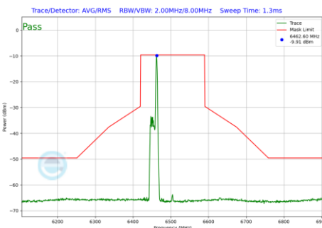
Plot 7-584 In-Band Emission Plot SDM Primary Antenna WF5B (160MHz BW 802.11be(RU) RU26 Index17 (UNII Band 6) - Ch.111)
