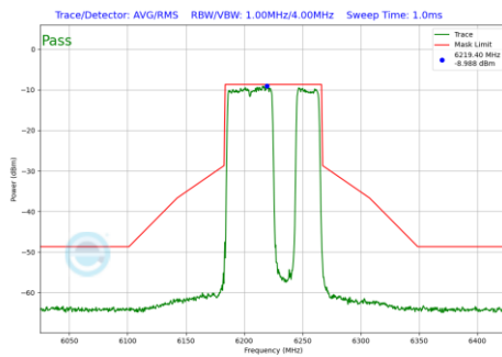
Plot 7-546 In-Band Emission Plot Antenna 2a (80MHz BW 802.11be(RU) RU484+242 Index92 (UNII Band 5) - Ch.55)
