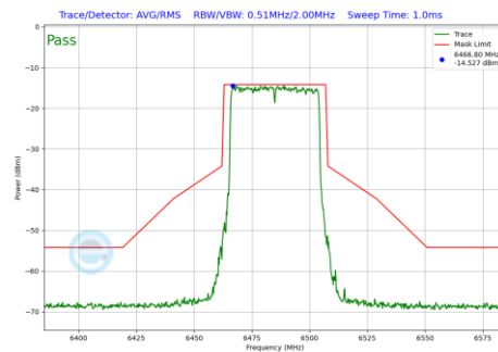
Plot 7-642 In-Band Emission Plot CDD Primary Antenna 4a (40MHz BW 802.11be(RU) RU484 Index65 (UNII Band 6) - Ch.107)
