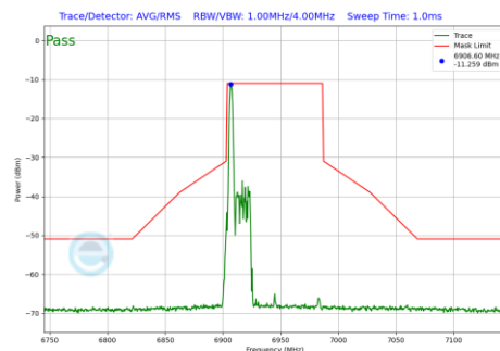
Plot 7-603 In-Band Emission Plot SDM Primary Antenna 4a (80MHz BW 802.11be(RU) RU26 Index0 (UNII Band 8) - Ch.199)
