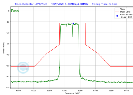
Plot 7-606 In-Band Emission Plot CDD Primary Antenna WF5B (80MHz BW 802.11be(RU) RU484+242 Index93 (UNII Band 5) - Ch.55)
