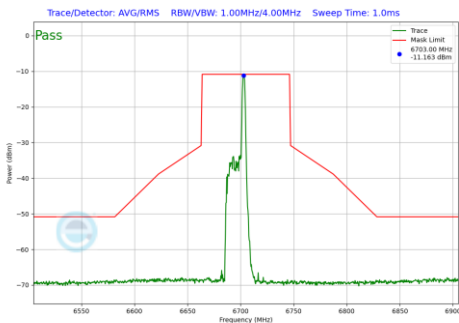
Plot 7-591 In-Band Emission Plot SDM Primary Antenna WF5B (80MHz BW 802.11be(RU) RU26 Index17 (UNII Band 7) - Ch.151)
