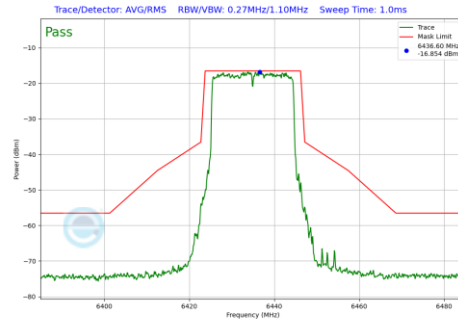
Plot 7-641 In-Band Emission Plot CDD Primary Antenna 4a (20MHz BW 802.11be(RU) RU242 Index61 (UNII Band 6) - Ch.97)
