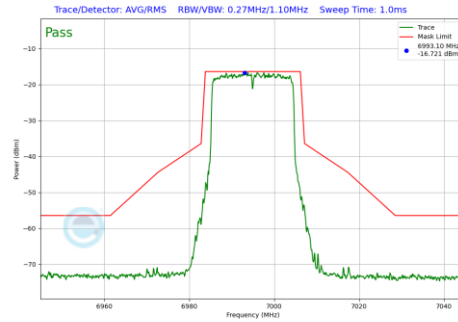
Plot 7-569 In-Band Emission Plot Antenna 2a (20MHz BW 802.11be(RU) RU242 Index61 (UNII Band 8) - Ch.209)
