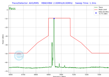
Plot 7-600 In-Band Emission Plot SDM Primary Antenna WF5B (160MHz BW 802.11be(RU) RU26 Index17 (UNII Band 8) - Ch.207)
