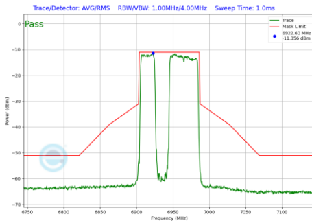
Plot 7-624 In-Band Emission Plot CDD Primary Antenna WF5B (80MHz BW 802.11be(RU) RU484+242 Index91 (UNII Band 8) - Ch.199)
