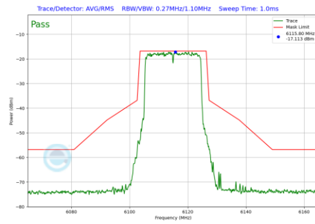
Plot 7-633 In-Band Emission Plot CDD Primary Antenna 4a (20MHz BW 802.11be(RU) RU242 Index61 (UNII Band 5) - Ch.33)
