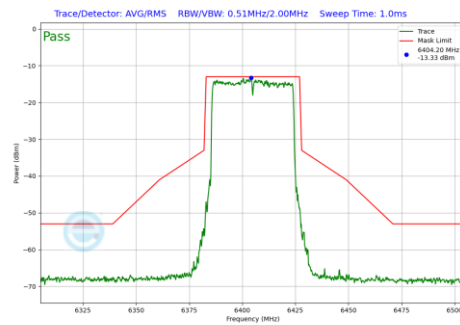
Plot 7-634 In-Band Emission Plot CDD Primary Antenna 4a (40MHz BW 802.11be(RU) RU484 Index65 (UNII Band 5) - Ch.91)
