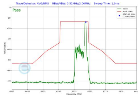
Plot 7-594 In-Band Emission Plot SDM Primary Antenna 4a (40MHz BW 802.11be(RU) RU26 Index17 (UNII Band 7) - Ch.155)
