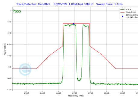
Plot 7-621 In-Band Emission Plot CDD Primary Antenna 4a (80MHz BW 802.11be(RU) RU484+242 Index92 (UNII Band 7) - Ch.151)
