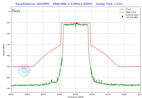
Plot 7-514 In-Band Emission Plot Antenna 4a (40MHz BW 802.11be(RU) RU484 Index65 (UNII Band 5) - Ch.35)
