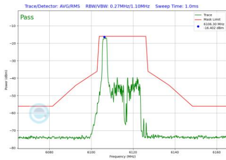
Plot 7-573 In-Band Emission Plot CDD Primary Antenna WF5B (20MHz BW 802.11be(RU) RU26 Index0 (UNII Band 5) - Ch.33)
