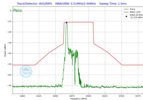
Plot 7-490 In-Band Emission Plot Antenna 4a (40MHz BW 802.11be(RU) RU26 Index0 (UNII Band 6) - Ch.107)
