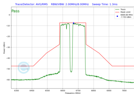
Plot 7-553 In-Band Emission Plot Antenna 2a (160MHz BW 802.11be(RU) RU996+484+242 Index99 (UNII Band 7) - Ch.143)
