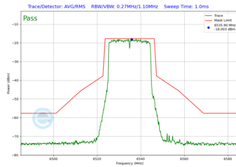
Plot 7-737 In-Band Emission Plot CDD Diversity Antenna 4a (20MHz BW 802.11be(RU) RU242 Index61 (UNII Band 7) - Ch.117)
