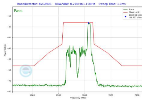
Plot 7-689 In-Band Emission Plot CDD Diversity Antenna 4a (20MHz BW 802.11be(RU) RU26 Index8 (UNII Band 8) - Ch.209)
