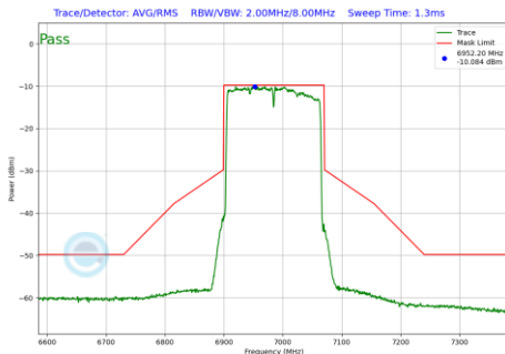
Plot 7-656 In-Band Emission Plot CDD Primary Antenna WF5B (160MHz BW 802.11be(RU) RU996X2 Index68 (UNII Band 8) - Ch.207)
