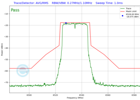
Plot 7-645 In-Band Emission Plot CDD Primary Antenna WF5B (20MHz BW 802.11be(RU) RU242 Index61 (UNII Band 7) - Ch.117)
