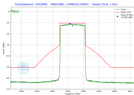
Plot 7-727 In-Band Emission Plot CDD Diversity Antenna 2a (80MHz BW 802.11be(RU) RU996 Index67 (UNII Band 6) - Ch.103)
