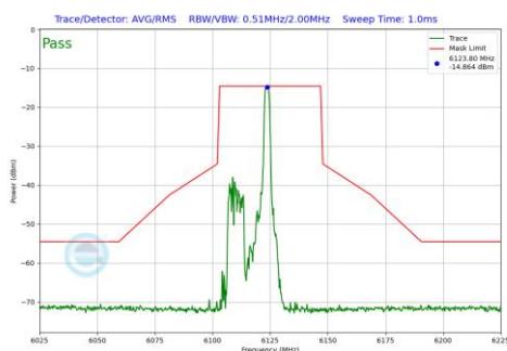
Plot 7-662 In-Band Emission Plot CDD Diversity Antenna 2a (40MHz BW 802.11be(RU) RU26 Index8 (UNII Band 5) - Ch.35)
