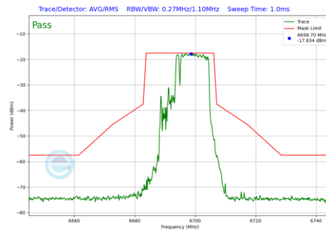
Plot 7-708 In-Band Emission Plot CDD Diversity Antenna 4a (20MHz BW 802.11be(RU) RU106+26 Index83 (UNII Band 7) - Ch.149)
