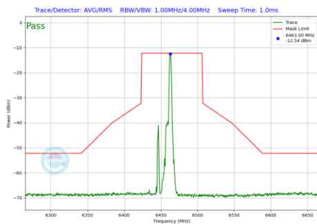
Plot 7-671 In-Band Emission Plot CDD Diversity Antenna 2a (80MHz BW 802.11be(RU) RU26 Index17 (UNII Band 6) - Ch.103)
