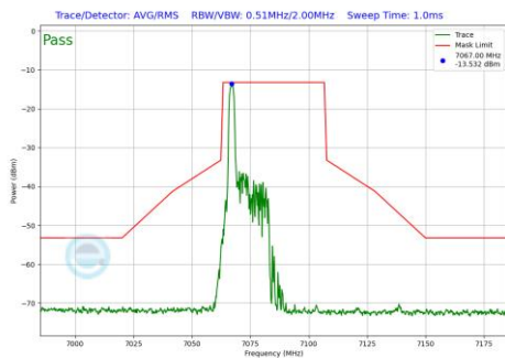
Plot 7-686 In-Band Emission Plot SDM Diversity Antenna 2a (40MHz BW 802.11be(RU) RU26 Index0 (UNII Band 8) - Ch.227)
