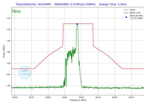
Plot 7-670 In-Band Emission Plot CDD Diversity Antenna 2a (40MHz BW 802.11be(RU) RU26 Index8 (UNII Band 6) - Ch.99)
