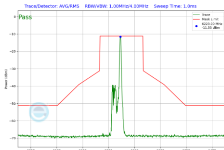
Plot 7-663 In-Band Emission Plot CDD Diversity Antenna 2a (80MHz BW 802.11be(RU) RU26 Index17 (UNII Band 5) - Ch.55)
