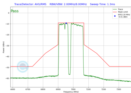
Plot 7-713 In-Band Emission Plot CDD Diversity Antenna 2a (160MHz BW 802.11be(RU) RU996+484+242 Index99 (UNII Band 8) - Ch.207)
