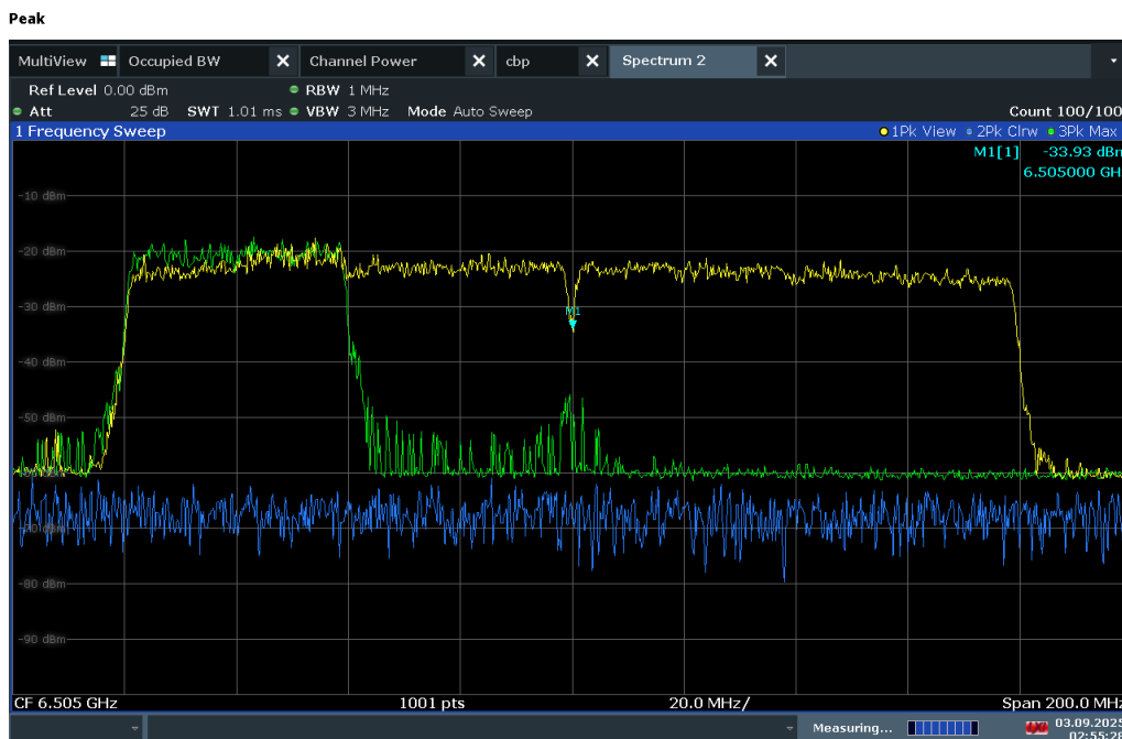
Plot 7-782. 160MHz Bandwidth, AWGN Signal Injected – 6505MHz
