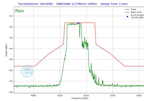
Plot 7-696 In-Band Emission Plot CDD Diversity Antenna 4a (20MHz BW 802.11be(RU) RU106+26 Index82 (UNII Band 5) - Ch.33)
