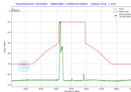
Plot 7-676 In-Band Emission Plot SDM Diversity Antenna 4a (160MHz BW 802.11be(RU) RU26 Index0 (UNII Band 6) - Ch.111)
