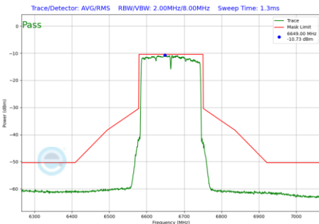
Plot 7-648 In-Band Emission Plot CDD Primary Antenna WF5B (160MHz BW 802.11be(RU) RU996X2 Index68 (UNII Band 7) - Ch.143)
