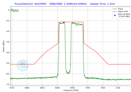
Plot 7-712 In-Band Emission Plot CDD Diversity Antenna 2a (80MHz BW 802.11be(RU) RU484+242 Index91 (UNII Band 8) - Ch.199)
