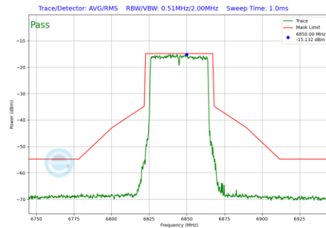
Plot 7-650 In-Band Emission Plot CDD Primary Antenna 4a (40MHz BW 802.11be(RU) RU484 Index65 (UNII Band 7) - Ch.179)
