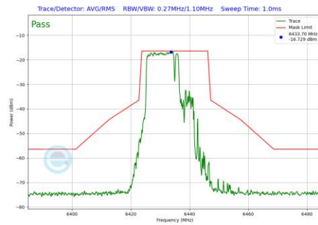
Plot 7-702 In-Band Emission Plot CDD Diversity Antenna 4a (20MHz BW 802.11be(RU) RU106+26 Index82 (UNII Band 6) - Ch.97)
