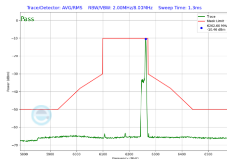
Plot 7-668 In-Band Emission Plot CDD Diversity Antenna 4a (160MHz BW 802.11be(RU) RU26 Index36 (UNII Band 5) - Ch.47)
