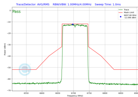
Plot 7-739 In-Band Emission Plot CDD Diversity Antenna 4a (80MHz BW 802.11be(RU) RU996 Index67 (UNII Band 7) - Ch.151)
