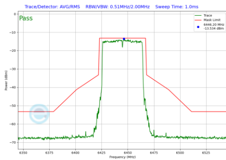
Plot 7-726 In-Band Emission Plot CDD Diversity Antenna 2a (40MHz BW 802.11be(RU) RU484 Index65 (UNII Band 6) - Ch.99)
