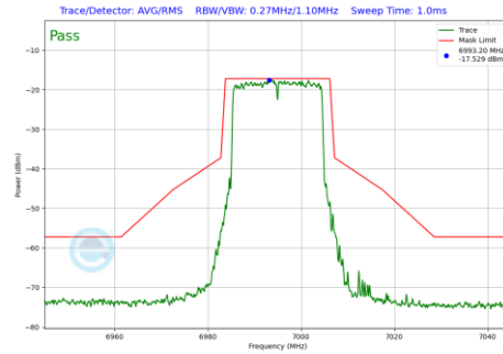
Plot 7-657 In-Band Emission Plot CDD Primary Antenna 4a (20MHz BW 802.11be(RU) RU242 Index61 (UNII Band 8) - Ch.209)
