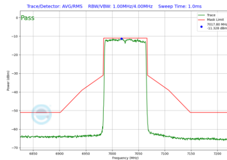
Plot 7-659 In-Band Emission Plot CDD Primary Antenna 4a (80MHz BW 802.11be(RU) RU996 Index67 (UNII Band 8) - Ch.215)
