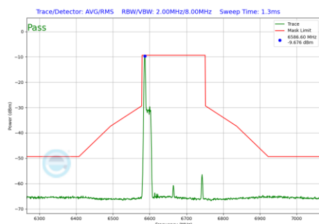
Plot 7-680 In-Band Emission Plot SDM Diversity Antenna 2a (160MHz BW 802.11be(RU) RU26 Index0 (UNII Band 7) - Ch.143)
