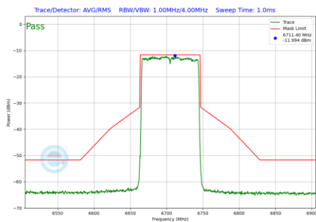
Plot 7-735 In-Band Emission Plot CDD Diversity Antenna 2a (80MHz BW 802.11be(RU) RU996 Index67 (UNII Band 7) - Ch.151)
