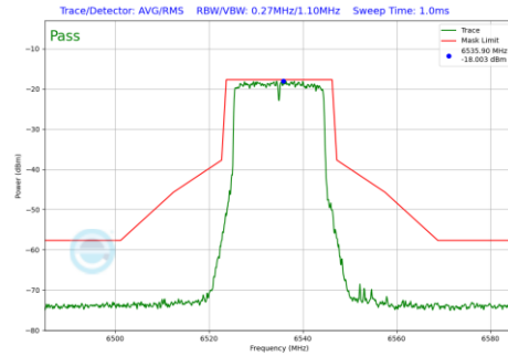
Plot 7-649 In-Band Emission Plot CDD Primary Antenna 4a (20MHz BW 802.11be(RU) RU242 Index61 (UNII Band 7) - Ch.117)
