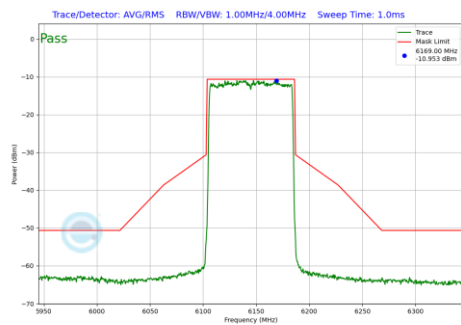
Plot 7-719 In-Band Emission Plot CDD Diversity Antenna 2a (80MHz BW 802.11be(RU) RU996 Index67 (UNII Band 5) - Ch.39)
