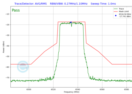
Plot 7-733 In-Band Emission Plot CDD Diversity Antenna 2a (20MHz BW 802.11be(RU) RU242 Index61 (UNII Band 7) - Ch.117)
