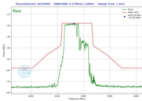
Plot 7-699 In-Band Emission Plot CDD Diversity Antenna 2a (20MHz BW 802.11be(RU) RU106+26 Index82 (UNII Band 6) - Ch.97)
