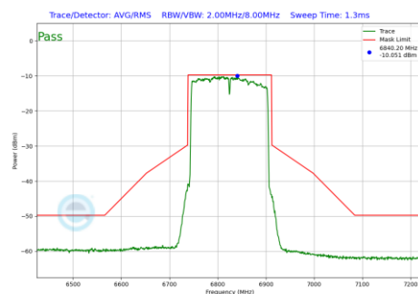
Plot 7-740 In-Band Emission Plot CDD Diversity Antenna 4a (160MHz BW 802.11be(RU) RU996X2 Index68 (UNII Band 7) - Ch.175)
