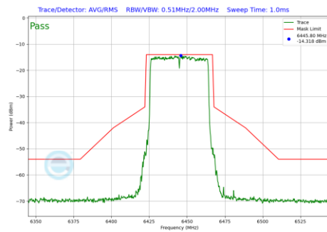
Plot 7-730 In-Band Emission Plot CDD Diversity Antenna 4a (40MHz BW 802.11be(RU) RU484 Index65 (UNII Band 6) - Ch.99)
