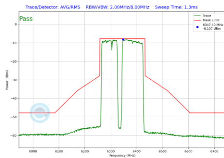
Plot 7-695 In-Band Emission Plot CDD Diversity Antenna 2a (160MHz BW 802.11be(RU) RU996+484+242 Index99 (UNII Band 5) - Ch.79)
