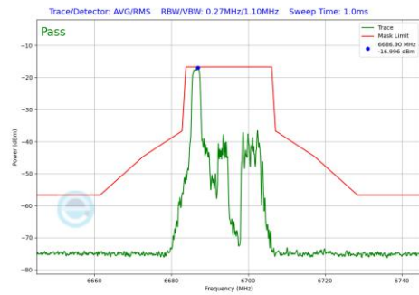
Plot 7-681 In-Band Emission Plot CDD Diversity Antenna 4a (20MHz BW 802.11be(RU) RU26 Index0 (UNII Band 7) - Ch.149)
