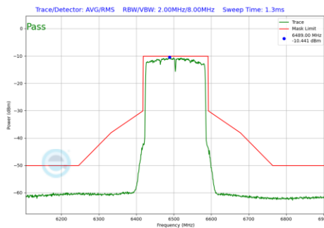
Plot 7-728 In-Band Emission Plot CDD Diversity Antenna 2a (160MHz BW 802.11be(RU) RU996X2 Index68 (UNII Band 6) - Ch.111)
