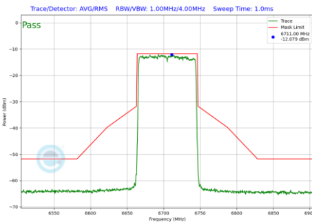
Plot 7-647 In-Band Emission Plot CDD Primary Antenna WF5B (80MHz BW 802.11be(RU) RU996 Index67 (UNII Band 7) - Ch.151)
