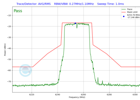
Plot 7-721 In-Band Emission Plot CDD Diversity Antenna 4a (20MHz BW 802.11be(RU) RU242 Index61 (UNII Band 5) - Ch.61)
