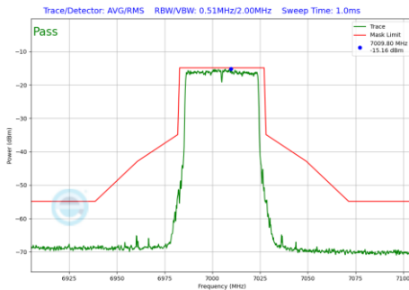
Plot 7-654 In-Band Emission Plot CDD Primary Antenna WF5B (40MHz BW 802.11be(RU) RU484 Index65 (UNII Band 8) - Ch.211)
