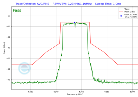
Plot 7-717 In-Band Emission Plot CDD Diversity Antenna 2a (20MHz BW 802.11be(RU) RU242 Index61 (UNII Band 5) - Ch.61)
