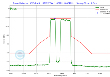
Plot 7-715 In-Band Emission Plot CDD Diversity Antenna 4a (80MHz BW 802.11be(RU) RU484+242 Index91 (UNII Band 8) - Ch.199)
