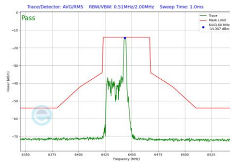
Plot 7-674 In-Band Emission Plot CDD Diversity Antenna 4a (40MHz BW 802.11be(RU) RU26 Index8 (UNII Band 6) - Ch.99)
