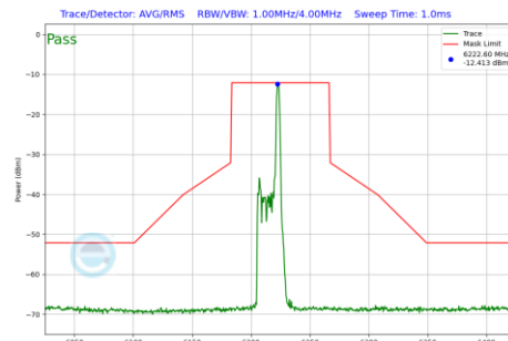
Plot 7-667 In-Band Emission Plot CDD Diversity Antenna 4a (80MHz BW 802.11be(RU) RU26 Index17 (UNII Band 5) - Ch.55)
