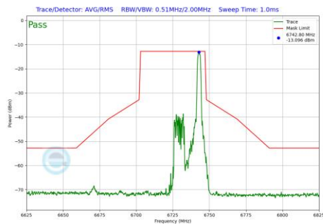
Plot 7-678 In-Band Emission Plot SDM Diversity Antenna 2a (40MHz BW 802.11be(RU) RU26 Index17 (UNII Band 7) - Ch.155)
