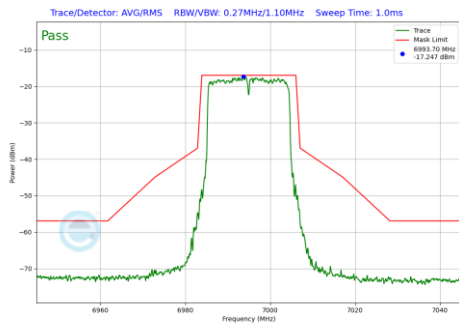
Plot 7-741 In-Band Emission Plot CDD Diversity Antenna 2a (20MHz BW 802.11be(RU) RU242 Index61 (UNII Band 8) - Ch.209)
