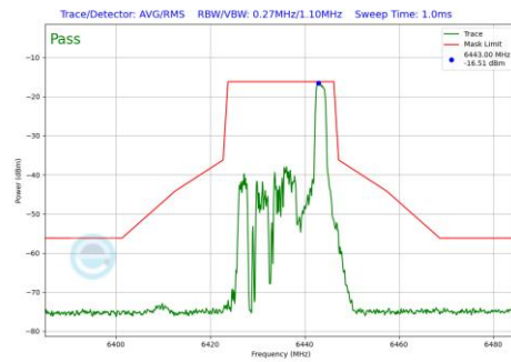
Plot 7-673 In-Band Emission Plot CDD Diversity Antenna 4a (20MHz BW 802.11be(RU) RU26 Index8 (UNII Band 6) - Ch.97)
