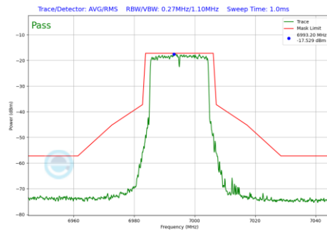
Plot 7-745 In-Band Emission Plot CDD Diversity Antenna 4a (20MHz BW 802.11be(RU) RU242 Index61 (UNII Band 8) - Ch.209)
