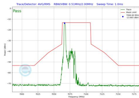
Plot 7-690 In-Band Emission Plot SDM Diversity Antenna 4a (40MHz BW 802.11be(RU) RU26 Index0 (UNII Band 8) - Ch.227)
