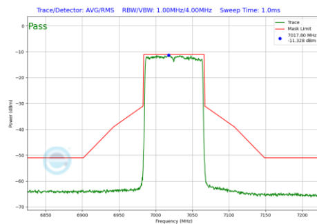
Plot 7-747 In-Band Emission Plot CDD Diversity Antenna 4a (80MHz BW 802.11be(RU) RU996 Index67 (UNII Band 8) - Ch.215)
