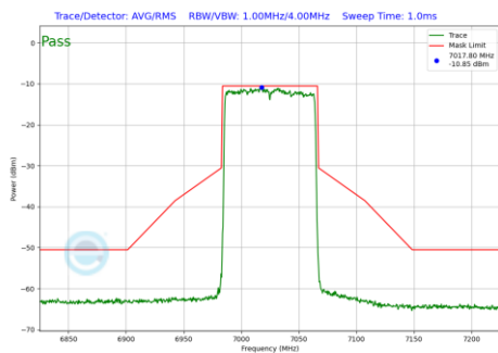
Plot 7-743 In-Band Emission Plot CDD Diversity Antenna 2a (80MHz BW 802.11be(RU) RU996 Index67 (UNII Band 8) - Ch.215)
