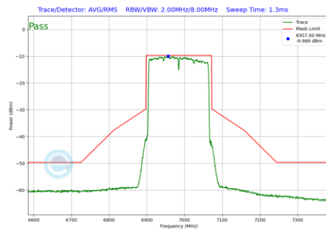
Plot 7-748 In-Band Emission Plot CDD Diversity Antenna 4a (160MHz BW 802.11be(RU) RU996X2 Index68 (UNII Band 8) - Ch.207)
