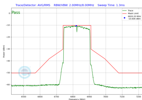
Plot 7-736 In-Band Emission Plot CDD Diversity Antenna 2a (160MHz BW 802.11be(RU) RU996X2 Index68 (UNII Band 7) - Ch.175)
