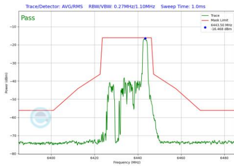
Plot 7-669 In-Band Emission Plot CDD Diversity Antenna 2a (20MHz BW 802.11be(RU) RU26 Index8 (UNII Band 6) - Ch.97)
