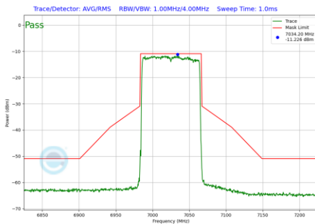
Plot 7-655 In-Band Emission Plot CDD Primary Antenna WF5B (80MHz BW 802.11be(RU) RU996 Index67 (UNII Band 8) - Ch.215)
