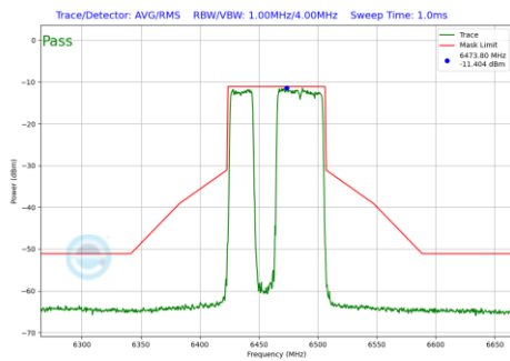
Plot 7-700 In-Band Emission Plot CDD Diversity Antenna 2a (80MHz BW 802.11be(RU) RU484+242 Index91 (UNII Band 6) - Ch.103)
