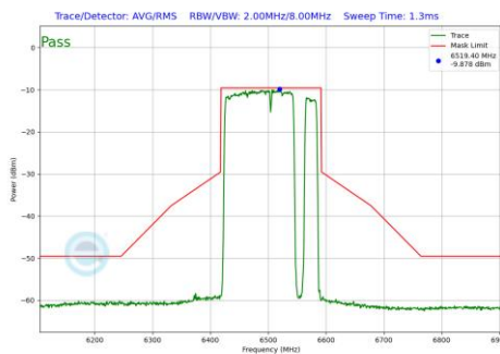
Plot 7-701 In-Band Emission Plot CDD Diversity Antenna 2a (160MHz BW 802.11be(RU) RU996+484+242 Index98 (UNII Band 6) - Ch.111)
