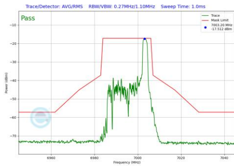
Plot 7-685 In-Band Emission Plot CDD Diversity Antenna 2a (20MHz BW 802.11be(RU) RU26 Index8 (UNII Band 8) - Ch.209)
