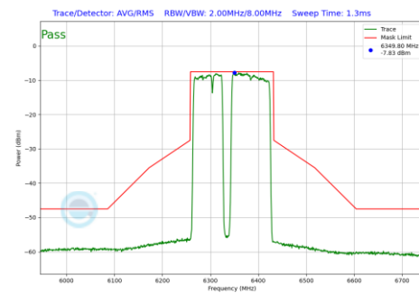
Plot 7-698 In-Band Emission Plot CDD Diversity Antenna 4a (160MHz BW 802.11be(RU) RU996+484+242 Index99 (UNII Band 5) - Ch.79)
