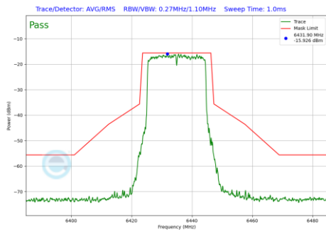
Plot 7-725 In-Band Emission Plot CDD Diversity Antenna 2a (20MHz BW 802.11be(RU) RU242 Index61 (UNII Band 6) - Ch.97)
