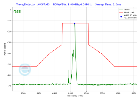
Plot 7-675 In-Band Emission Plot CDD Diversity Antenna 4a (80MHz BW 802.11be(RU) RU26 Index17 (UNII Band 6) - Ch.103)
