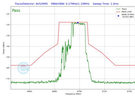
Plot 7-705 In-Band Emission Plot CDD Diversity Antenna 2a (20MHz BW 802.11be(RU) RU106+26 Index83 (UNII Band 7) - Ch.149)
