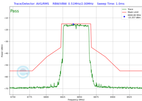
Plot 7-646 In-Band Emission Plot CDD Primary Antenna WF5B (40MHz BW 802.11be(RU) RU484 Index65 (UNII Band 7) - Ch.179)
