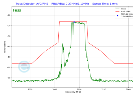
Plot 7-714 In-Band Emission Plot CDD Diversity Antenna 4a (20MHz BW 802.11be(RU) RU106+26 Index83 (UNII Band 8) - Ch.229)
