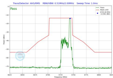
Plot 7-682 In-Band Emission Plot SDM Diversity Antenna 4a (40MHz BW 802.11be(RU) RU26 Index17 (UNII Band 7) - Ch.155)
