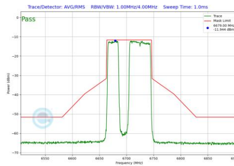
Plot 7-709 In-Band Emission Plot CDD Diversity Antenna 4a (80MHz BW 802.11be(RU) RU484+242 Index91 (UNII Band 7) - Ch.151)
