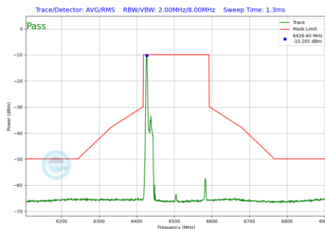
Plot 7-672 In-Band Emission Plot SDM Diversity Antenna 2a (160MHz BW 802.11be(RU) RU26 Index0 (UNII Band 6) - Ch.111)
