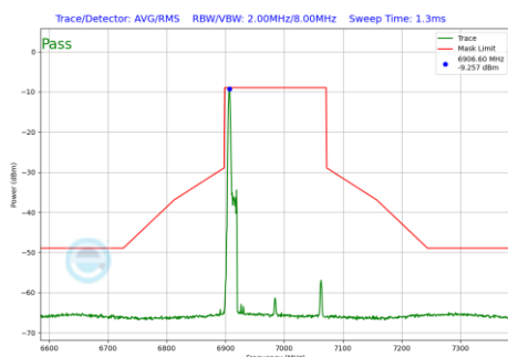
Plot 7-688 In-Band Emission Plot SDM Diversity Antenna 2a (160MHz BW 802.11be(RU) RU26 Index0 (UNII Band 8) - Ch.207)
