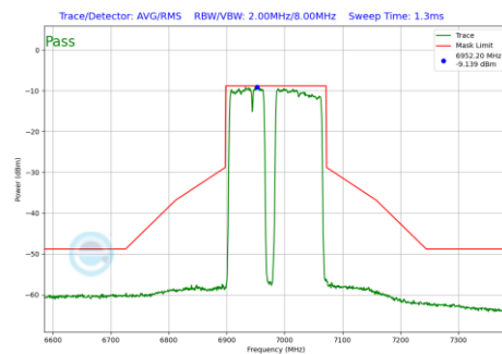
Plot 7-716 In-Band Emission Plot CDD Diversity Antenna 4a (160MHz BW 802.11be(RU) RU996+484+242 Index99 (UNII Band 8) - Ch.207)
