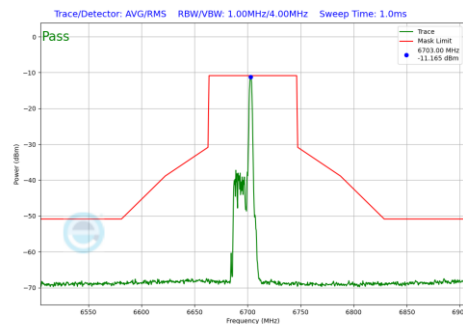
Plot 7-683 In-Band Emission Plot SDM Diversity Antenna 4a (80MHz BW 802.11be(RU) RU26 Index17 (UNII Band 7) - Ch.151)
