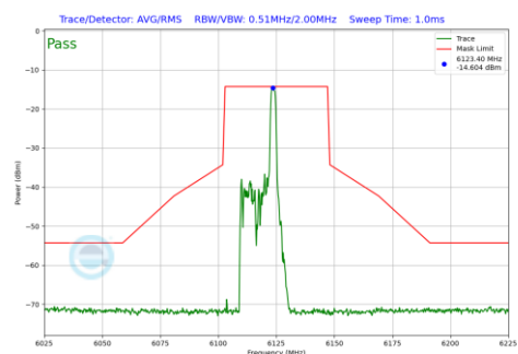
Plot 7-666 In-Band Emission Plot CDD Diversity Antenna 4a (40MHz BW 802.11be(RU) RU26 Index8 (UNII Band 5) - Ch.35)
