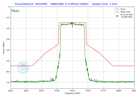
Plot 7-734 In-Band Emission Plot CDD Diversity Antenna 2a (40MHz BW 802.11be(RU) RU484 Index65 (UNII Band 7) - Ch.155)
