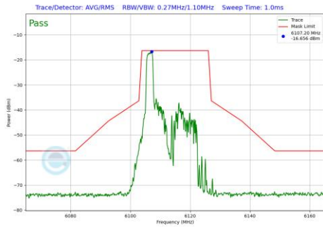
Plot 7-661 In-Band Emission Plot CDD Diversity Antenna 2a (20MHz BW 802.11be(RU) RU26 Index0 (UNII Band 5) - Ch.33)
