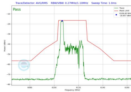
Plot 7-665 In-Band Emission Plot CDD Diversity Antenna 4a (20MHz BW 802.11be(RU) RU26 Index0 (UNII Band 5) - Ch.33)
