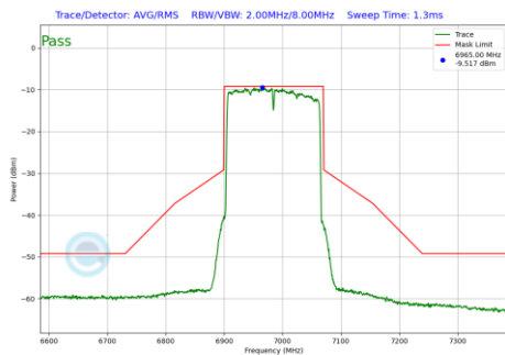
Plot 7-744 In-Band Emission Plot CDD Diversity Antenna 2a (160MHz BW 802.11be(RU) RU996X2 Index68 (UNII Band 8) - Ch.207)
