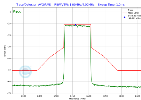
Plot 7-731 In-Band Emission Plot CDD Diversity Antenna 4a (80MHz BW 802.11be(RU) RU996 Index67 (UNII Band 6) - Ch.103)
