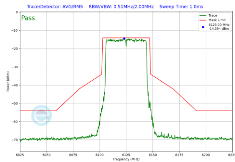
Plot 7-722 In-Band Emission Plot CDD Diversity Antenna 4a (40MHz BW 802.11be(RU) RU484 Index65 (UNII Band 5) - Ch.35)
