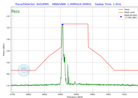
Plot 7-687 In-Band Emission Plot SDM Diversity Antenna 2a (80MHz BW 802.11be(RU) RU26 Index0 (UNII Band 8) - Ch.199)
