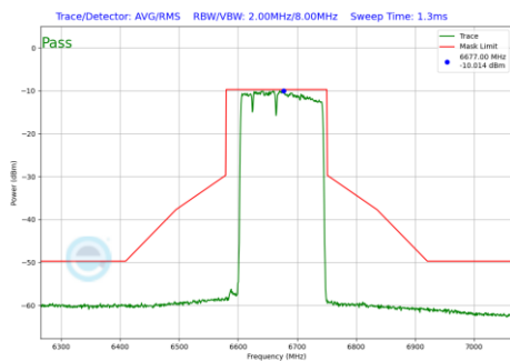
Plot 7-707 In-Band Emission Plot CDD Diversity Antenna 2a (160MHz BW 802.11be(RU) RU996+484+242 Index96 (UNII Band 7) - Ch.143)
