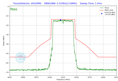
Plot 7-718 In-Band Emission Plot CDD Diversity Antenna 2a (40MHz BW 802.11be(RU) RU484 Index65 (UNII Band 5) - Ch.35)
