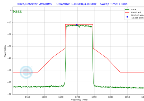
Plot 7-651 In-Band Emission Plot CDD Primary Antenna 4a (80MHz BW 802.11be(RU) RU996 Index67 (UNII Band 7) - Ch.151)
