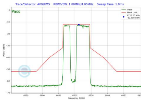
Plot 7-706 In-Band Emission Plot CDD Diversity Antenna 2a (80MHz BW 802.11be(RU) RU484+242 Index91 (UNII Band 7) - Ch.151)
