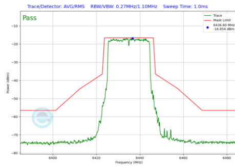
Plot 7-729 In-Band Emission Plot CDD Diversity Antenna 4a (20MHz BW 802.11be(RU) RU242 Index61 (UNII Band 6) - Ch.97)
