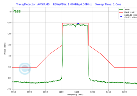
Plot 7-723 In-Band Emission Plot CDD Diversity Antenna 4a (80MHz BW 802.11be(RU) RU996 Index67 (UNII Band 5) - Ch.39)
