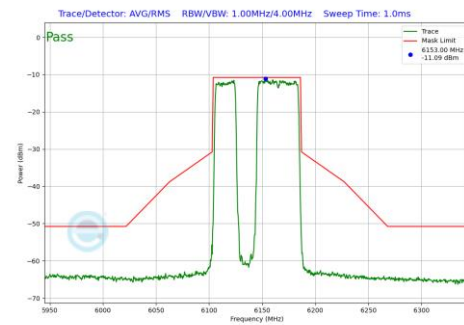
Plot 7-697 In-Band Emission Plot CDD Diversity Antenna 4a (80MHz BW 802.11be(RU) RU484+242 Index91 (UNII Band 5) - Ch.39)
