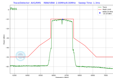
Plot 7-652 In-Band Emission Plot CDD Primary Antenna 4a (160MHz BW 802.11be(RU) RU996X2 Index68 (UNII Band 7) - Ch.143)
