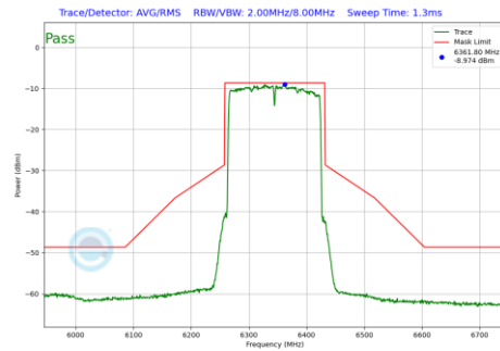
Plot 7-724 In-Band Emission Plot CDD Diversity Antenna 4a (160MHz BW 802.11be(RU) RU996X2 Index68 (UNII Band 5) - Ch.79)
