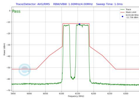
Plot 7-694 In-Band Emission Plot CDD Diversity Antenna 2a (80MHz BW 802.11be(RU) RU484+242 Index91 (UNII Band 5) - Ch.39)
