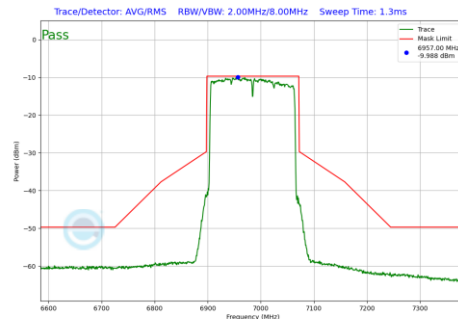
Plot 7-660 In-Band Emission Plot CDD Primary Antenna 4a (160MHz BW 802.11be(RU) RU996X2 Index68 (UNII Band 8) - Ch.207)
