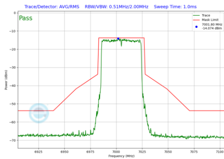
Plot 7-742 In-Band Emission Plot CDD Diversity Antenna 2a (40MHz BW 802.11be(RU) RU484 Index65 (UNII Band 8) - Ch.211)
