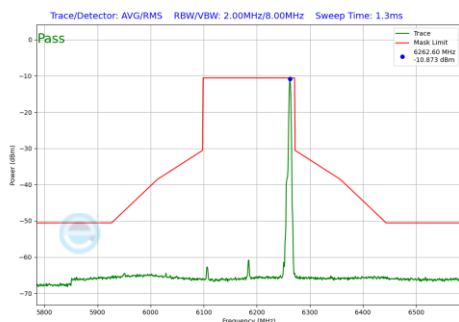
Plot 7-664 In-Band Emission Plot CDD Diversity Antenna 2a (160MHz BW 802.11be(RU) RU26 Index36 (UNII Band 5) - Ch.47)
