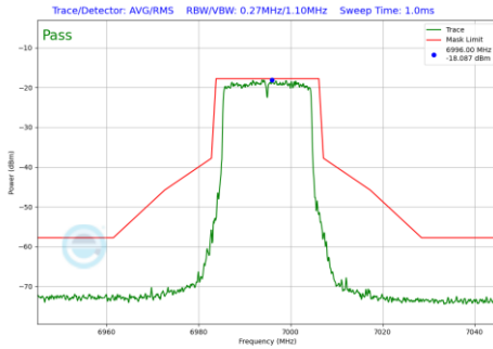
Plot 7-653 In-Band Emission Plot CDD Primary Antenna WF5B (20MHz BW 802.11be(RU) RU242 Index61 (UNII Band 8) - Ch.209)
