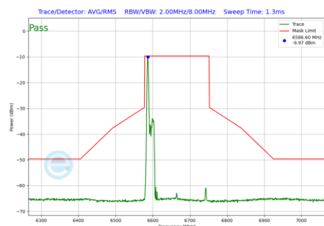
Plot 7-684 In-Band Emission Plot SDM Diversity Antenna 4a (160MHz BW 802.11be(RU) RU26 Index0 (UNII Band 7) - Ch.143)
