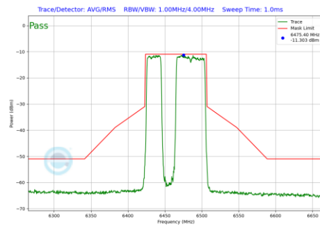
Plot 7-703 In-Band Emission Plot CDD Diversity Antenna 4a (80MHz BW 802.11be(RU) RU484+242 Index91 (UNII Band 6) - Ch.103)
