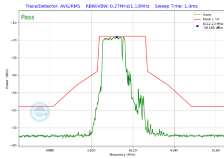
Plot 7-693 In-Band Emission Plot CDD Diversity Antenna 2a (20MHz BW 802.11be(RU) RU106+26 Index82 (UNII Band 5) - Ch.33)
