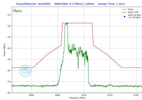
Plot 7-677 In-Band Emission Plot CDD Diversity Antenna 2a (20MHz BW 802.11be(RU) RU26 Index0 (UNII Band 7) - Ch.149)
