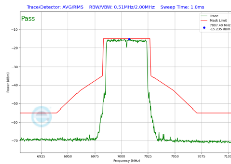
Plot 7-746 In-Band Emission Plot CDD Diversity Antenna 4a (40MHz BW 802.11be(RU) RU484 Index65 (UNII Band 8) - Ch.211)
