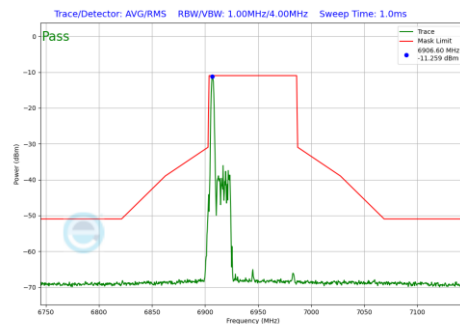
Plot 7-691 In-Band Emission Plot SDM Diversity Antenna 4a (80MHz BW 802.11be(RU) RU26 Index0 (UNII Band 8) - Ch.199)
