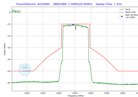
Plot 7-732 In-Band Emission Plot CDD Diversity Antenna 4a (160MHz BW 802.11be(RU) RU996X2 Index68 (UNII Band 6) - Ch.111)
