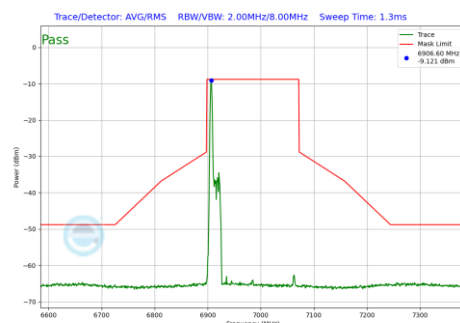
Plot 7-692 In-Band Emission Plot SDM Diversity Antenna 4a (160MHz BW 802.11be(RU) RU26 Index0 (UNII Band 8) - Ch.207)
