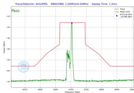
Plot 7-679 In-Band Emission Plot SDM Diversity Antenna 2a (80MHz BW 802.11be(RU) RU26 Index17 (UNII Band 7) - Ch.151)
