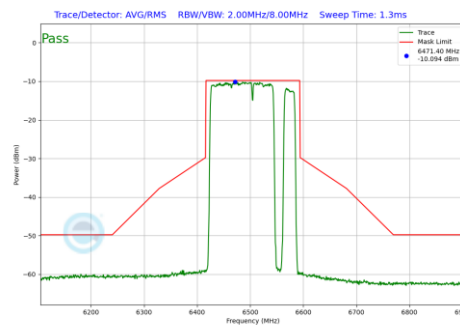
Plot 7-704 In-Band Emission Plot CDD Diversity Antenna 4a (160MHz BW 802.11be(RU) RU996+484+242 Index98 (UNII Band 6) - Ch.111)
