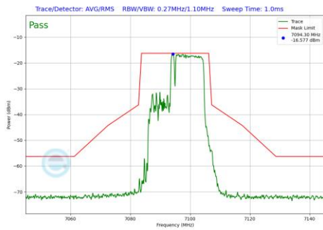
Plot 7-711 In-Band Emission Plot CDD Diversity Antenna 2a (20MHz BW 802.11be(RU) RU106+26 Index83 (UNII Band 8) - Ch.229)
