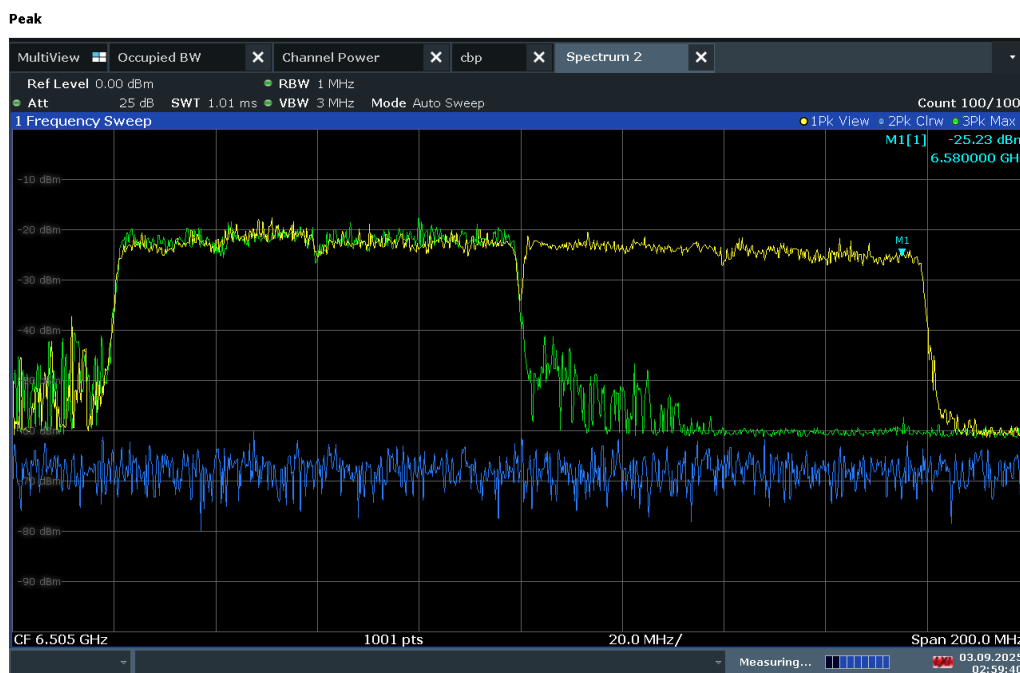
Plot 7-783. 160MHz Bandwidth, AWGN Signal Injected – 6580MHz
