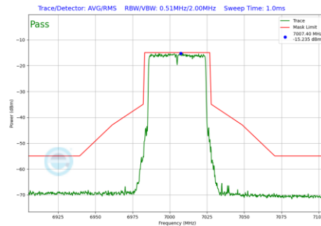
Plot 7-658 In-Band Emission Plot CDD Primary Antenna 4a (40MHz BW 802.11be(RU) RU484 Index65 (UNII Band 8) - Ch.211)
