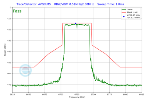
Plot 7-738 In-Band Emission Plot CDD Diversity Antenna 4a (40MHz BW 802.11be(RU) RU484 Index65 (UNII Band 7) - Ch.155)
