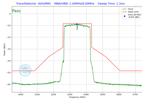
Plot 7-720 In-Band Emission Plot CDD Diversity Antenna 2a (160MHz BW 802.11be(RU) RU996X2 Index68 (UNII Band 5) - Ch.79)
