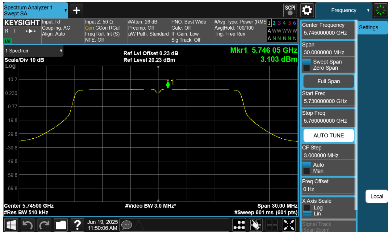
Plot 7-26 PSD Antenna WF5B (20MHz BW 802.11n - Ch.149)
