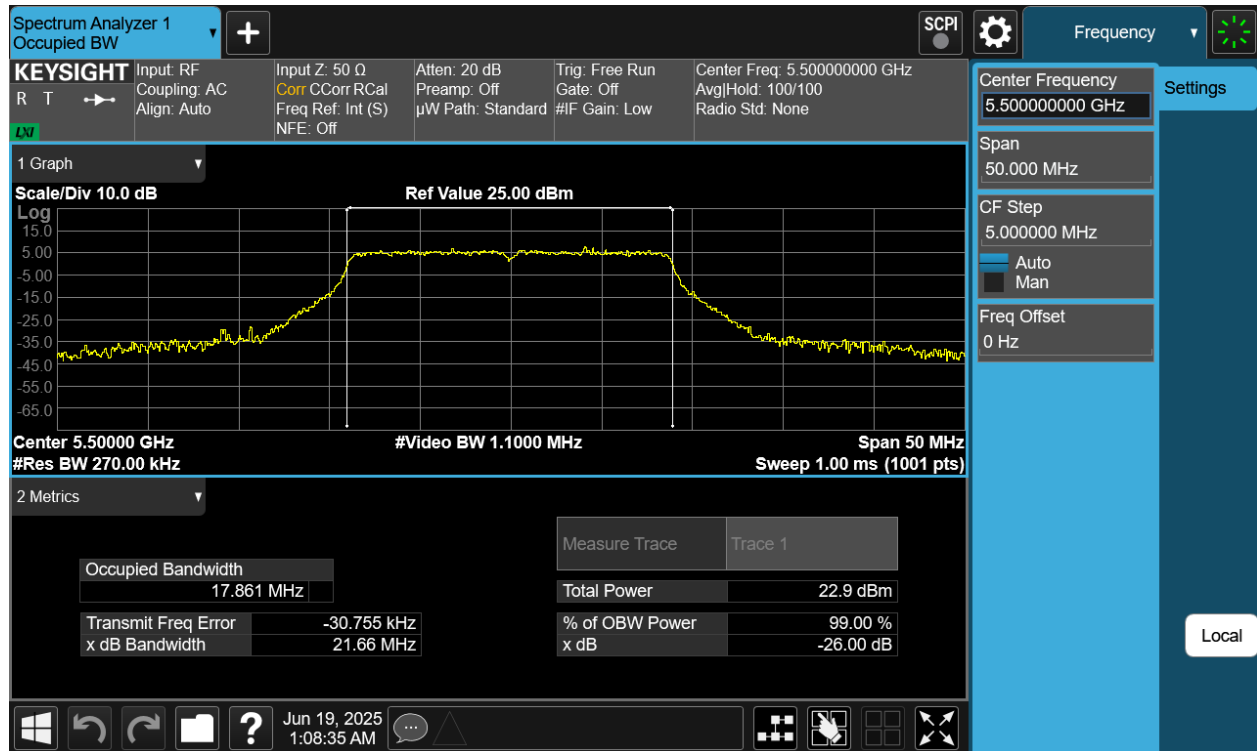
Plot 7-1 26dB BW & 99% OBW Antenna WF5B (20MHz BW 802.11n - Ch.100)
