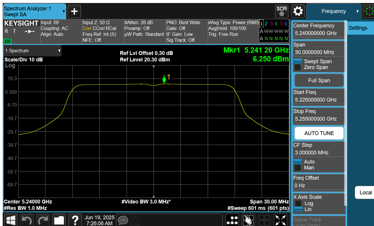
Plot 7-22 PSD Antenna WF5B (20MHz BW 802.11a - Ch.48)
