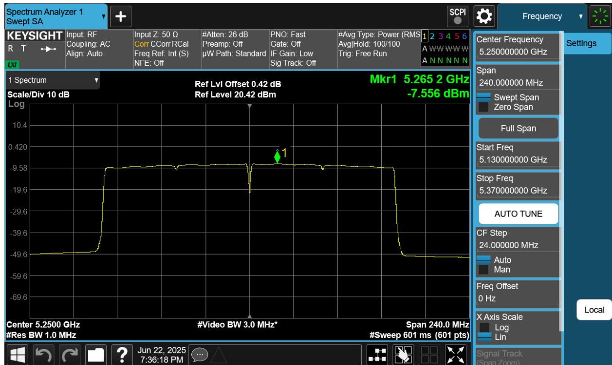
Plot 7-43 PSD Antenna 4a (160MHz BW 802.11be(SU) - Ch.50)
