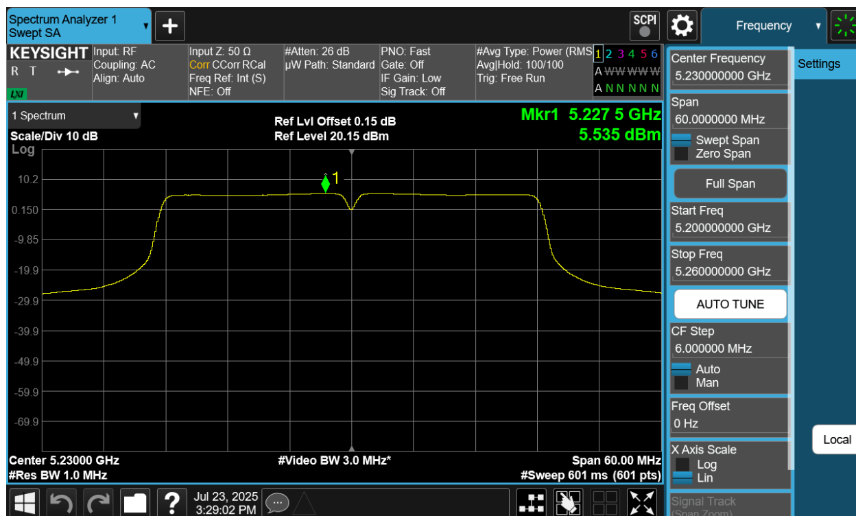
Plot 7-41 PSD Antenna 4a (40MHz BW 802.11n - Ch.46)
