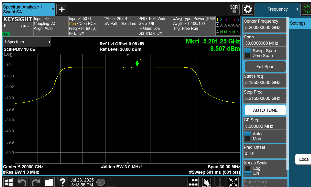
Plot 7-40 PSD Antenna 4a (20MHz BW 802.11n - Ch.40)
