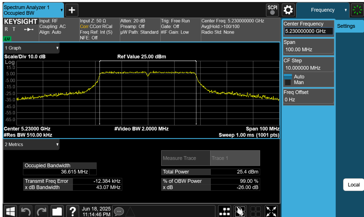
Plot 7-2 26dB BW & 99% OBW Antenna WF5B (40MHz BW 802.11n - Ch.46)
