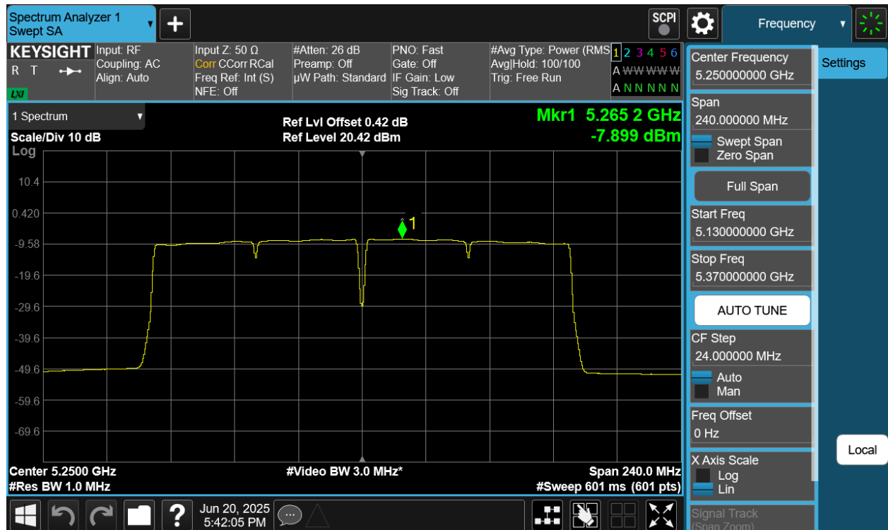
Plot 7-36 PSD Antenna 4a (160MHz BW 802.11ac - Ch.50)
