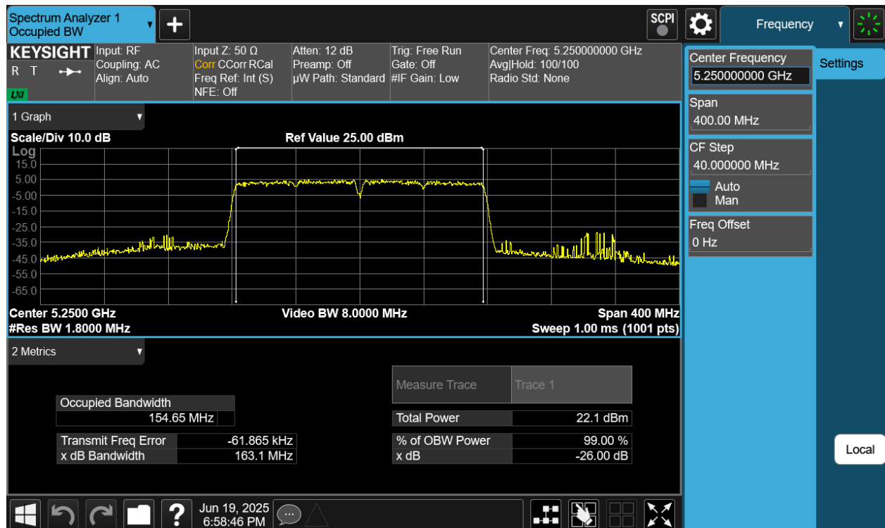
Plot 7-12 26dB BW & 99% OBW Antenna 2a (160MHz BW 802.11ac - Ch.50)
