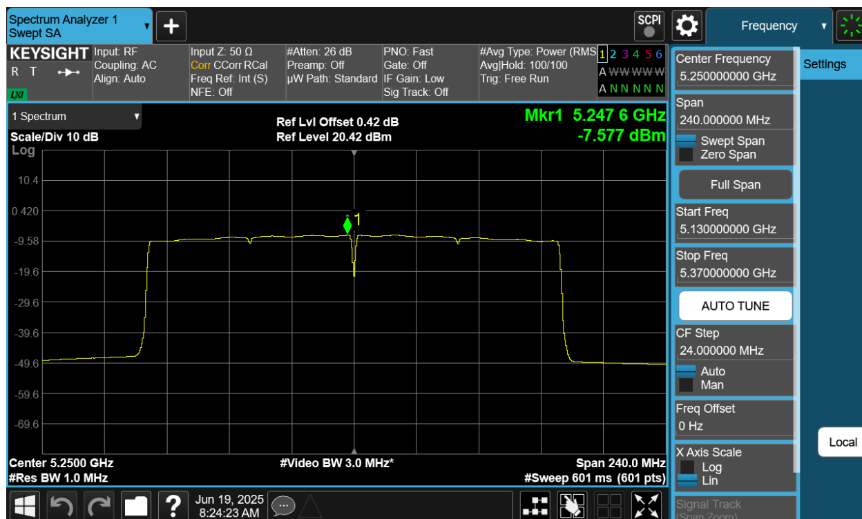
Plot 7-25 PSD Antenna WF5B (160MHz BW 802.11be(SU) - Ch.50)
