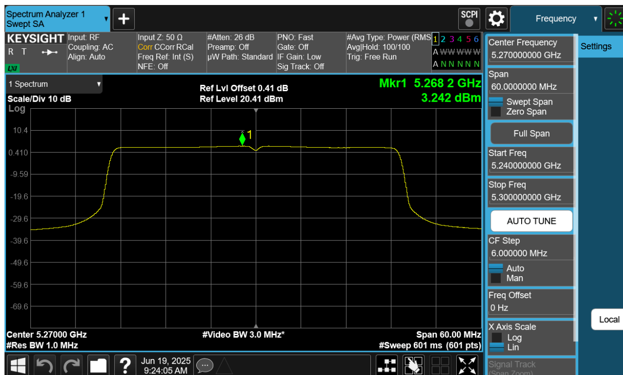
Plot 7-23 PSD Antenna WF5B (40MHz BW 802.11be(SU) - Ch.54)
