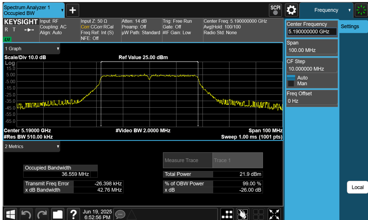
Plot 7-10 26dB BW & 99% OBW Antenna 2a (40MHz BW 802.11n - Ch.38)
