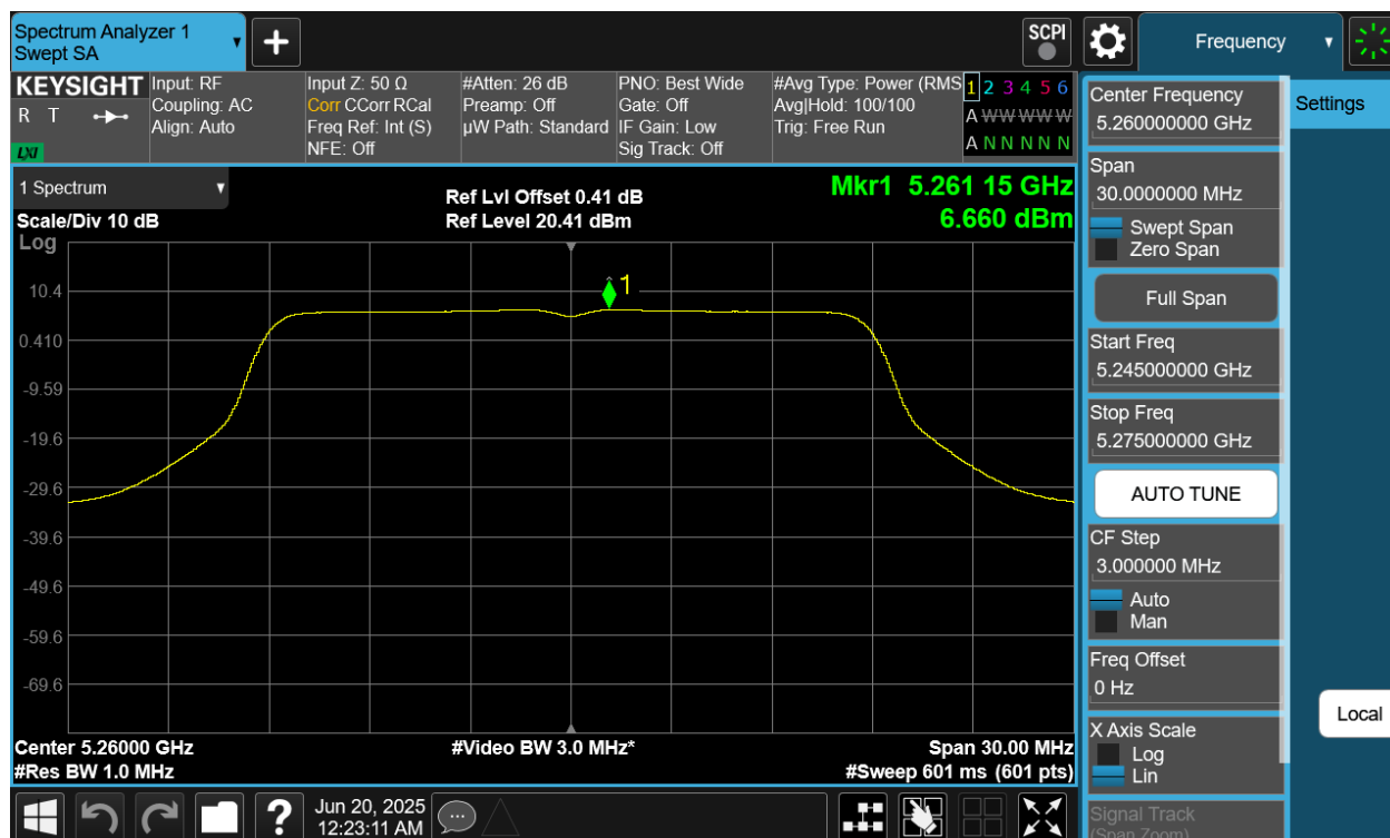
Plot 7-44 PSD Antenna 2a (20MHz BW 802.11n - Ch.52)
