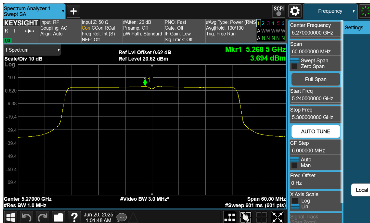
Plot 7-45 PSD Antenna 2a (40MHz BW 802.11be(SU) - Ch.54)
