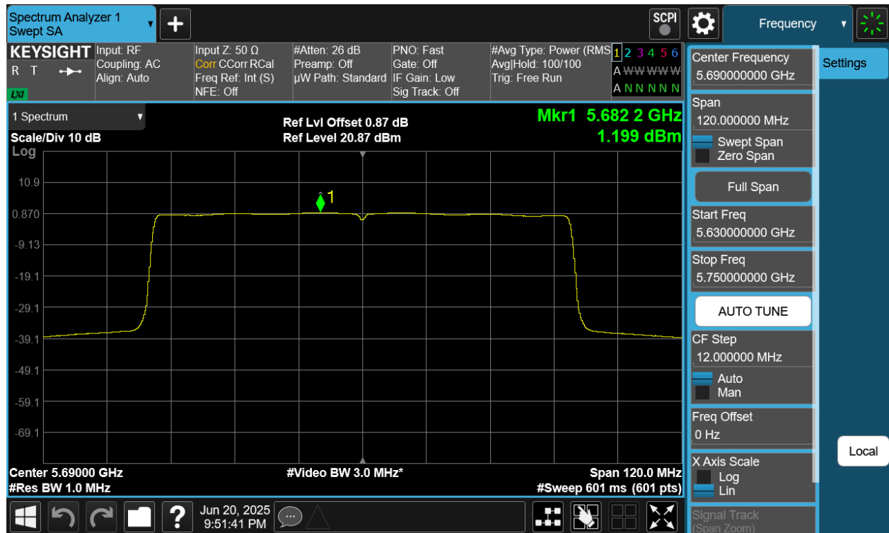
Plot 7-35 PSD Antenna 4a (80MHz BW 802.11be(SU) - Ch.138)
