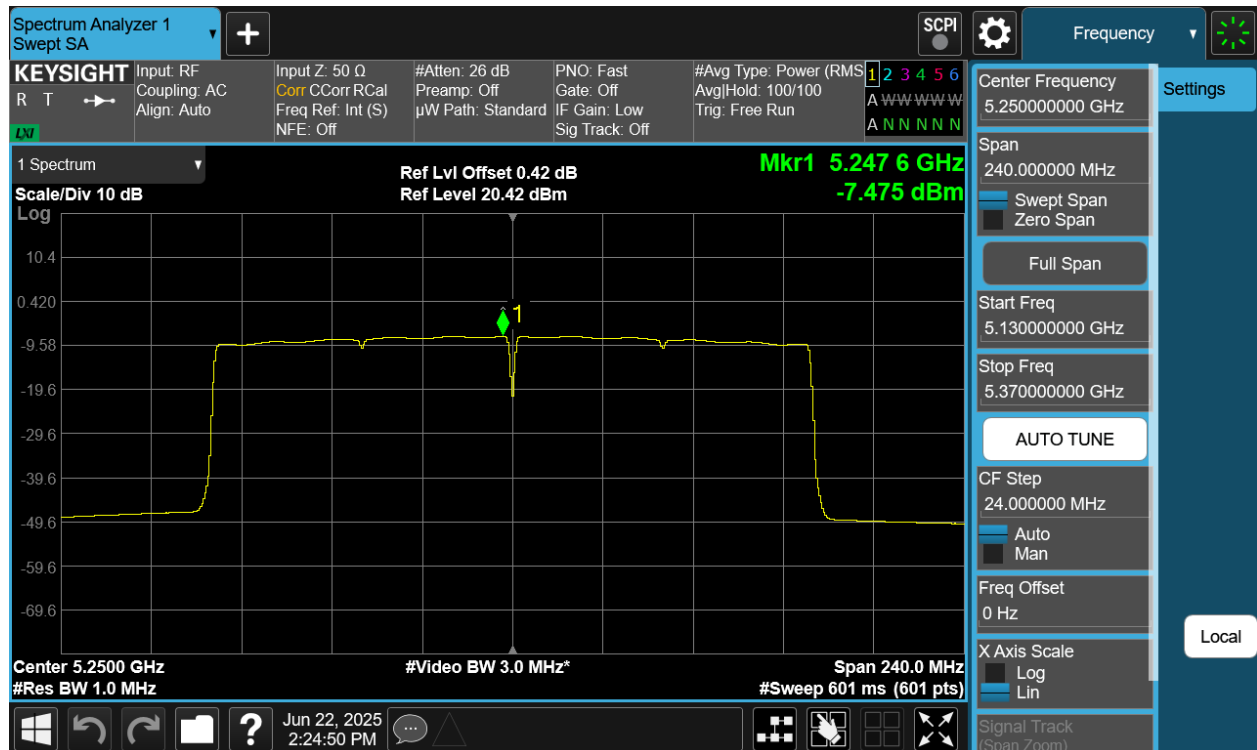
Plot 7-32 PSD Antenna WF5B (160MHz BW 802.11be(SU) - Ch.50)
