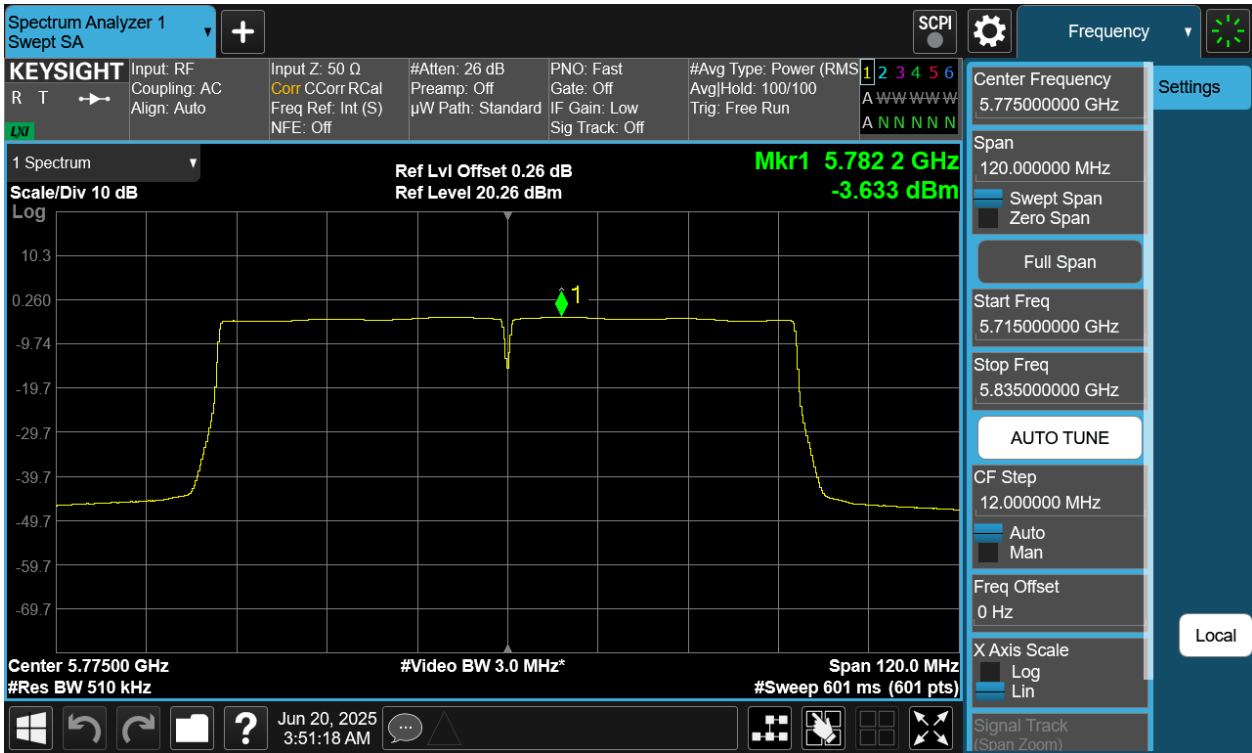
Plot 7-50 PSD Antenna 2a (80MHz BW 802.11ac - Ch.155)
