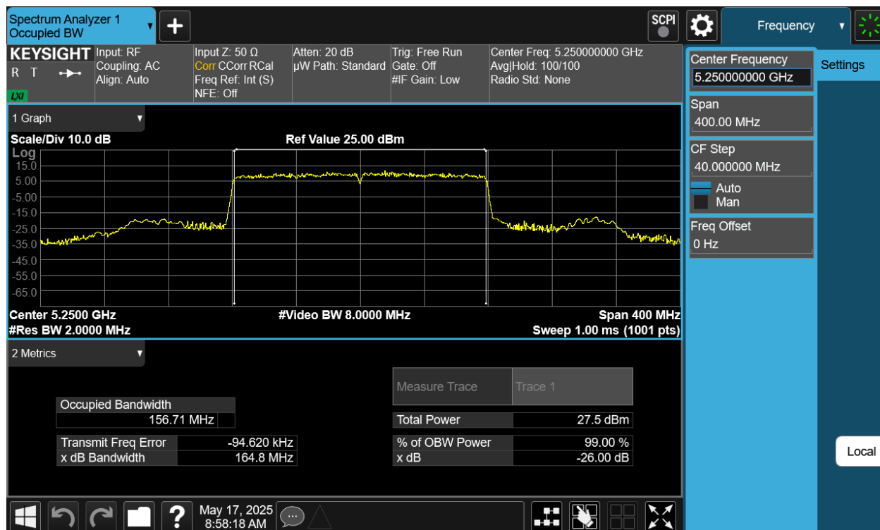
Plot 7-8 26dB BW & 99% OBW Antenna 4a (160MHz BW 802.11be(SU) - Ch.50)
