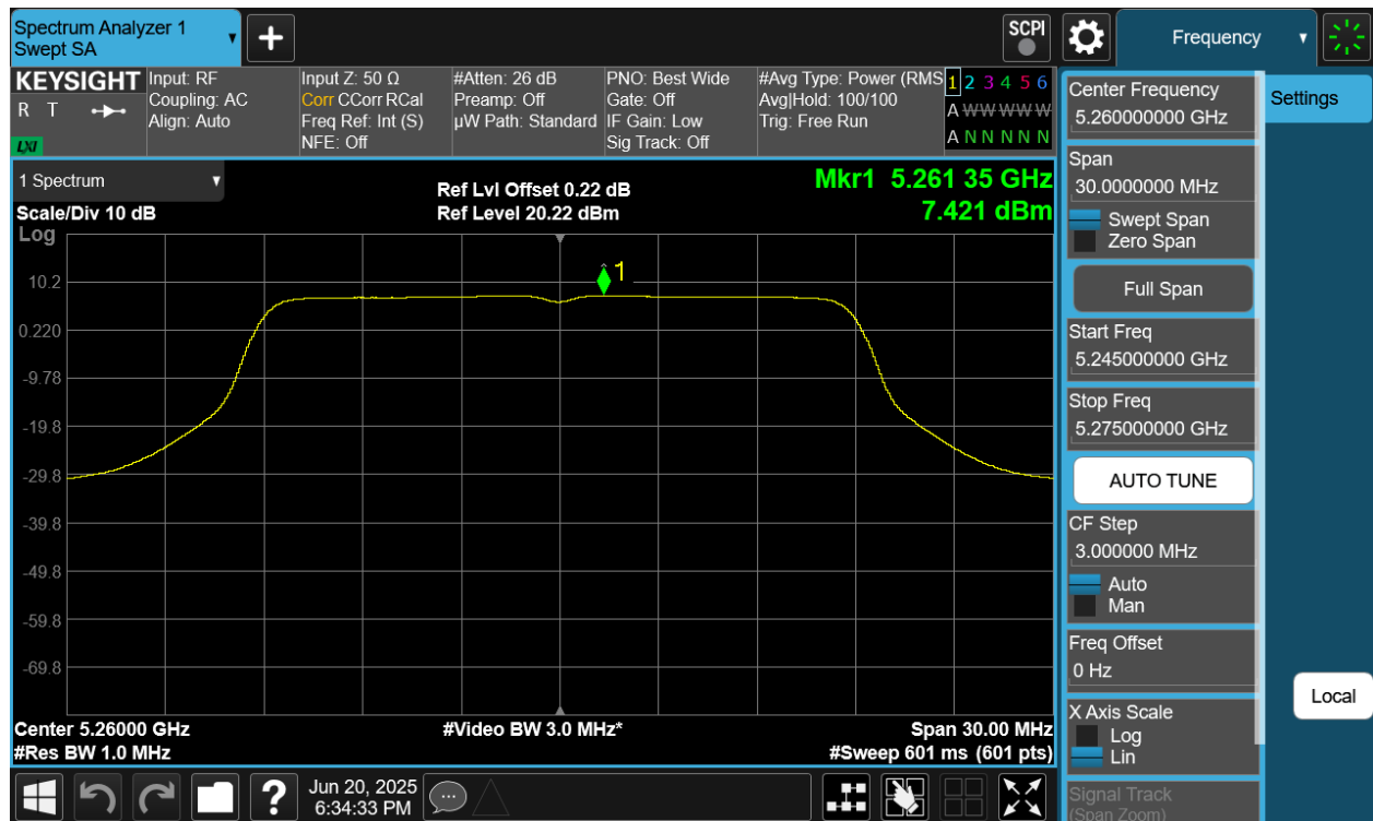
Plot 7-33 PSD Antenna 4a (20MHz BW 802.11n - Ch.52)
