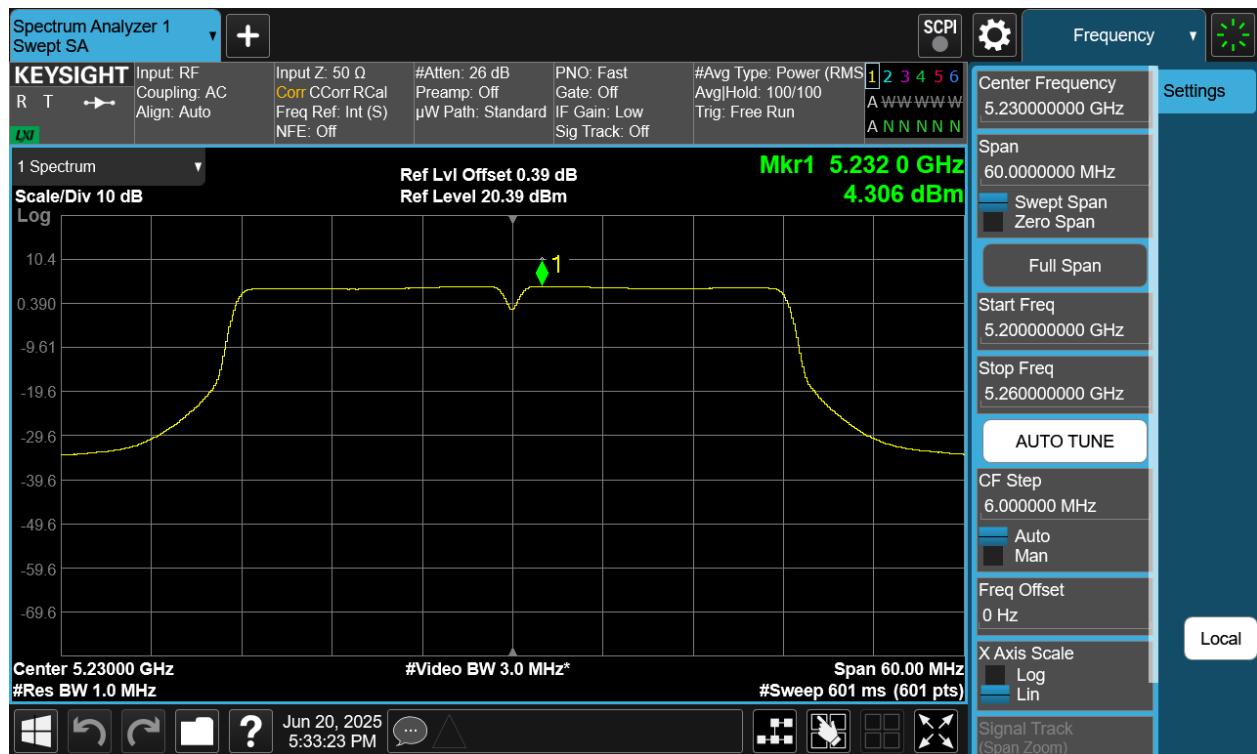
Plot 7-34 PSD Antenna 4a (40MHz BW 802.11n - Ch.46)
