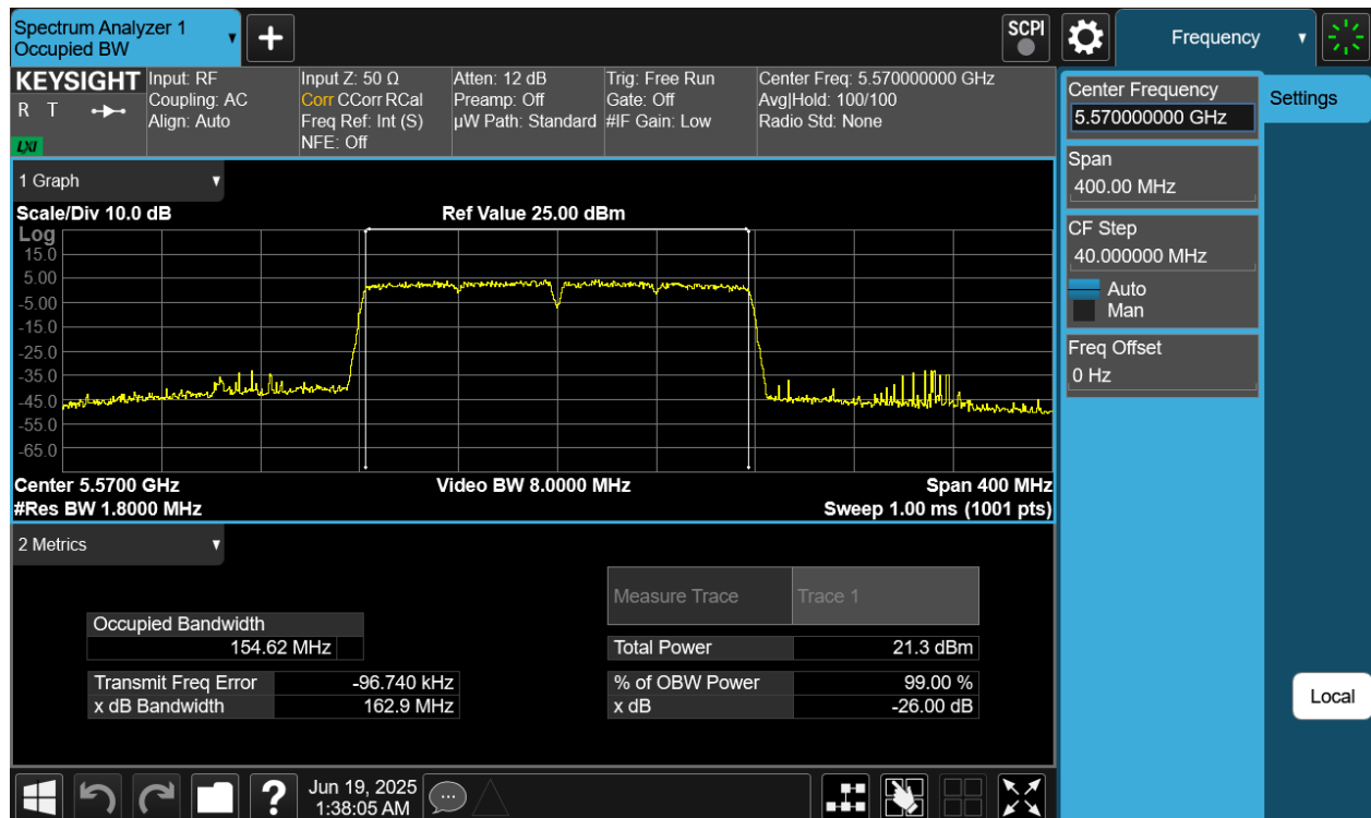
Plot 7-4 26dB BW & 99% OBW Antenna WF5B (160MHz BW 802.11ac - Ch.114 FCC ONLY)
