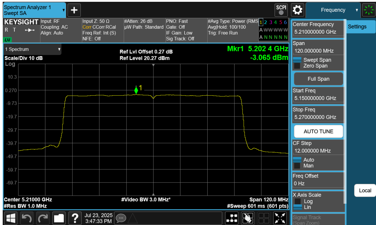
Plot 7-42 PSD Antenna 4a (80MHz BW 802.11be(SU) - Ch.42)
