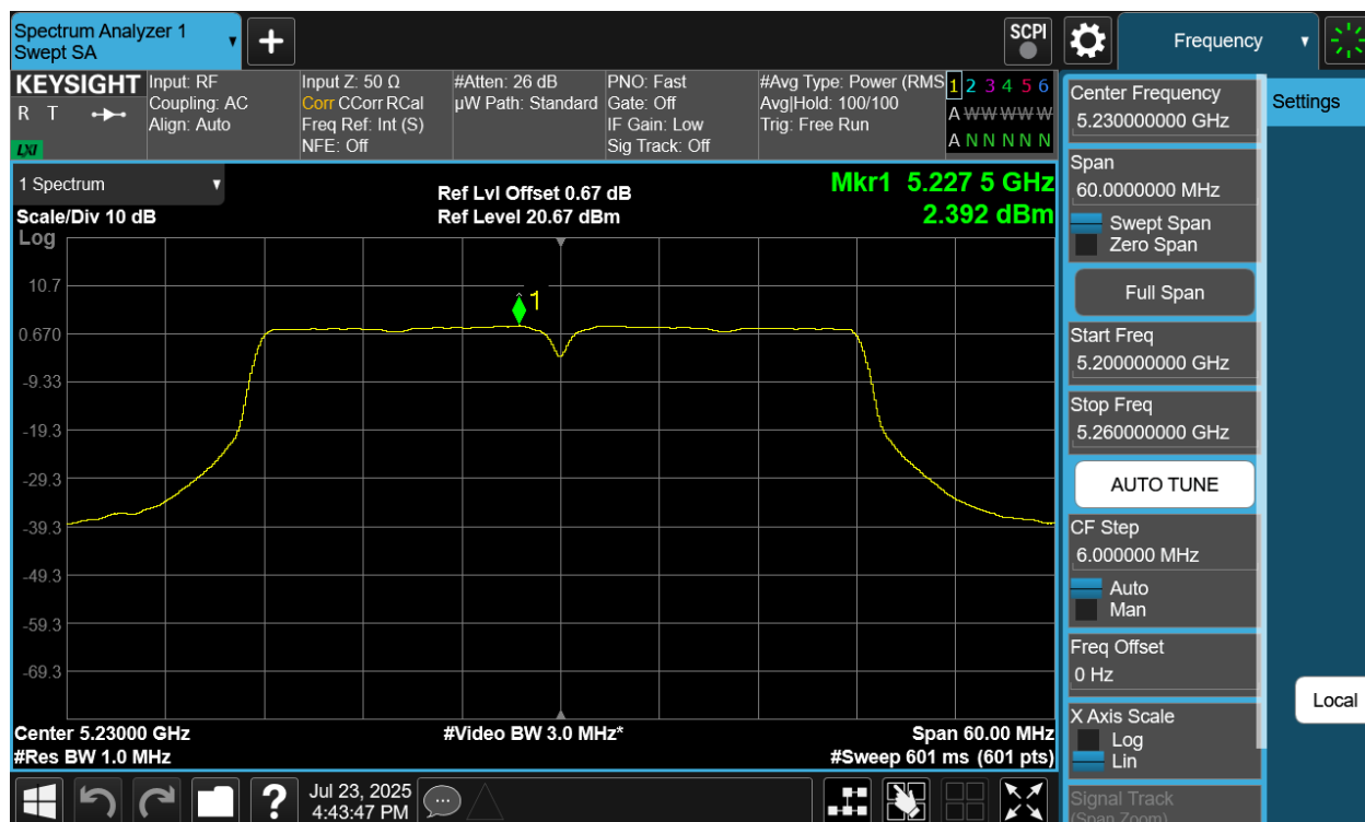
Plot 7-70 PSD SDM Primary Antenna WF5B (40MHz BW 802.11n - Ch.46)
