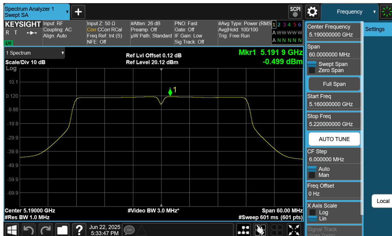
Plot 7-96 PSD CDD Diversity Antenna 2a (40MHz BW 802.11n - Ch.38)
