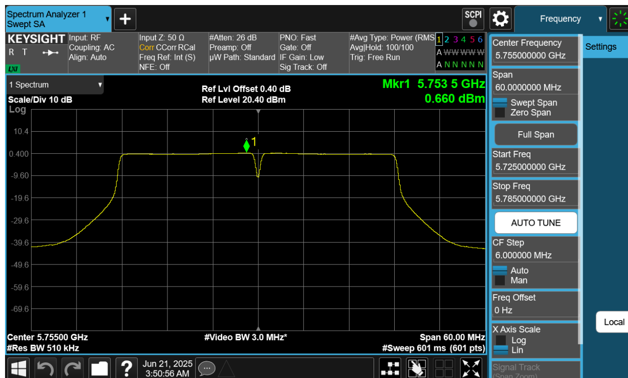
Plot 7-86 PSD CDD Diversity Antenna 4a (40MHz BW 802.11n - Ch.151)
