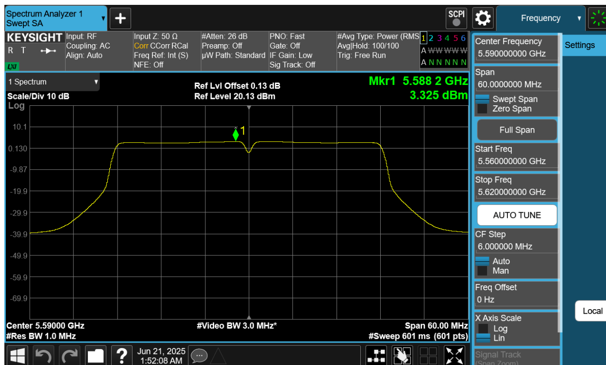
Plot 7-60 PSD CDD Primary Antenna 4a (40MHz BW 802.11n - Ch.118)
