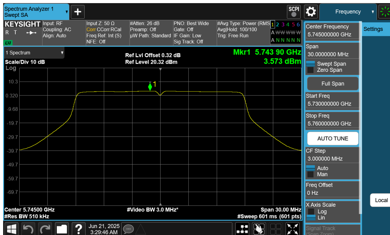
Plot 7-85 PSD CDD Diversity Antenna 4a (20MHz BW 802.11a - Ch.149)
