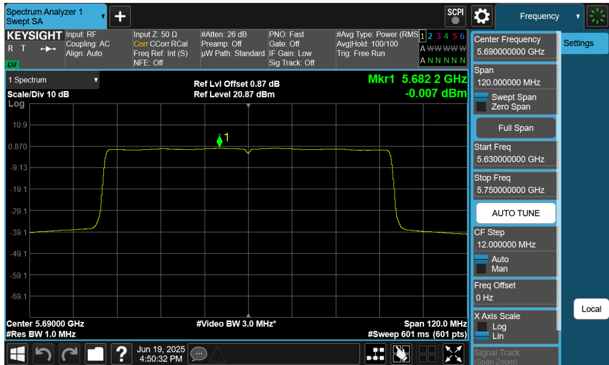
Plot 7-57 PSD CDD Primary Antenna WF5B (80MHz BW 802.11be(SU) - Ch.138)
