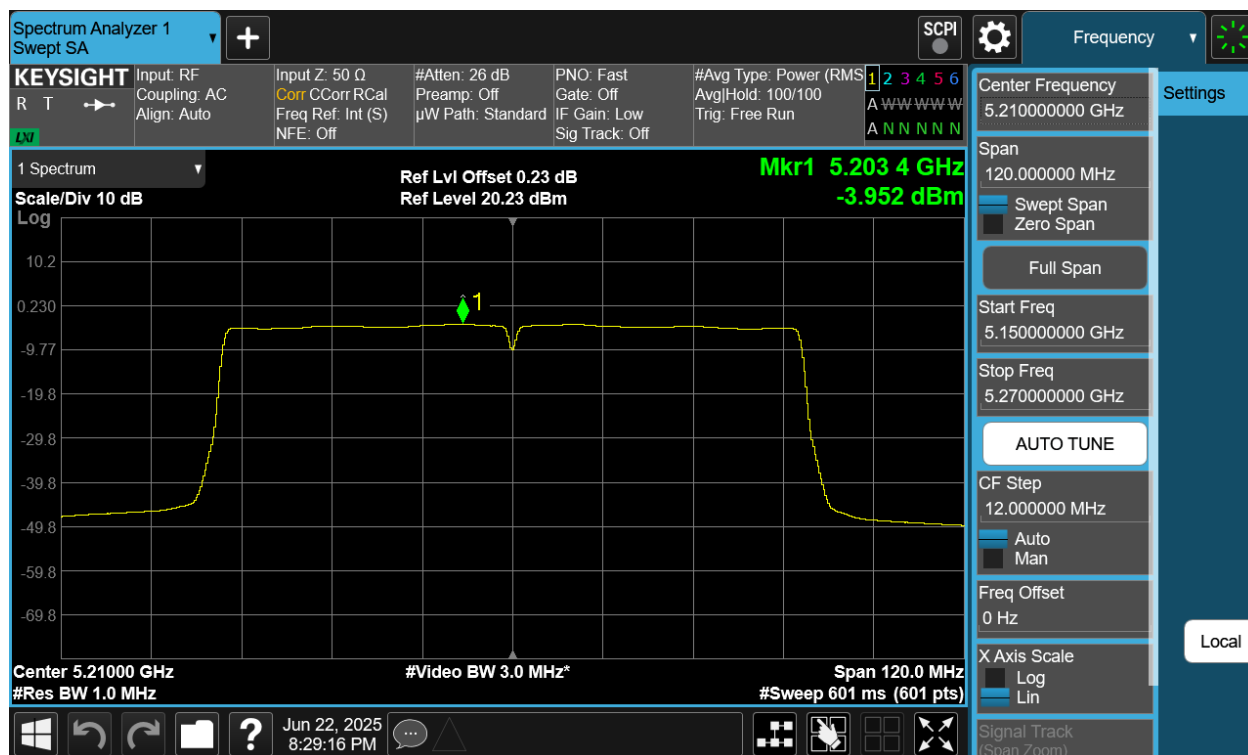
Plot 7-75 PSD CDD Primary Antenna 4a (80MHz BW 802.11ac - Ch.42)
