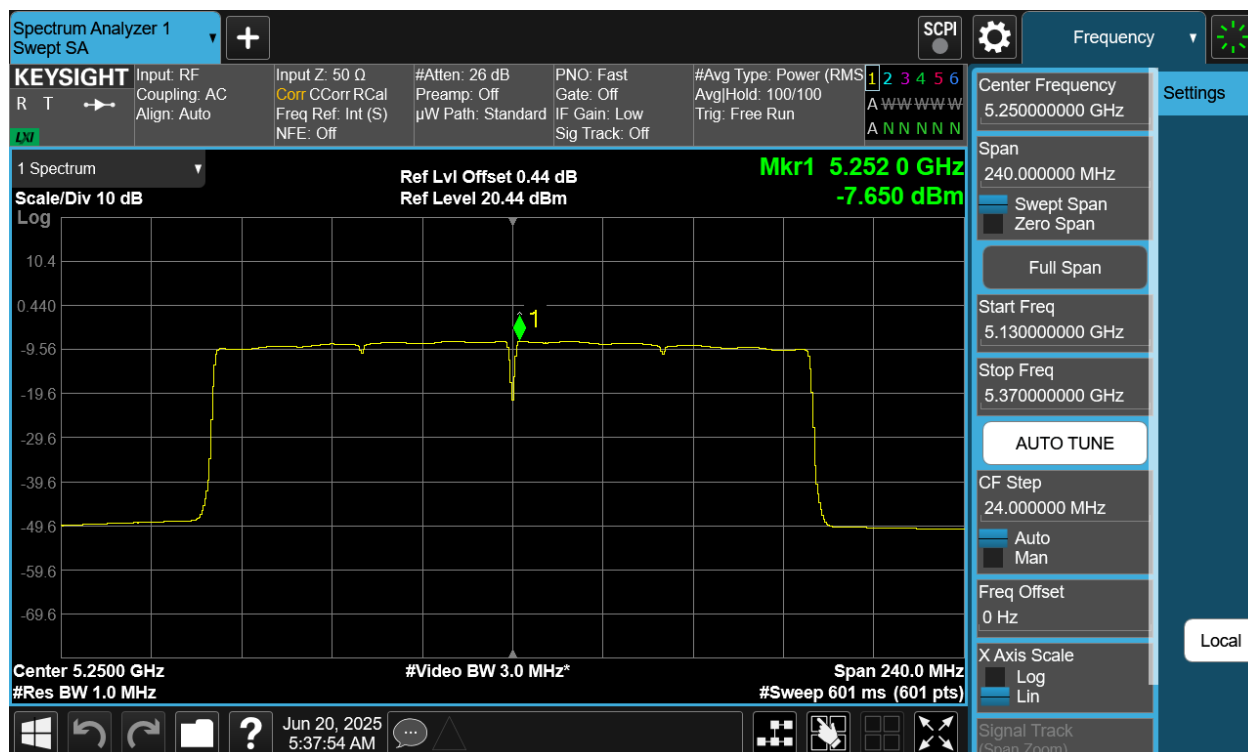
Plot 7-84 PSD CDD Diversity Antenna 2a (160MHz BW 802.11be(SU) - Ch.50)
