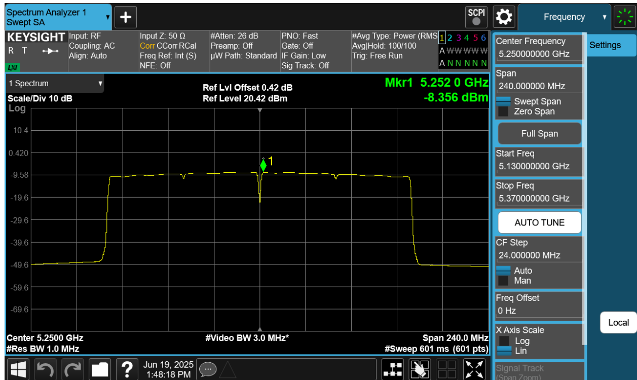
Plot 7-58 PSD CDD Primary Antenna WF5B (160MHz BW 802.11be(SU) - Ch.50)
