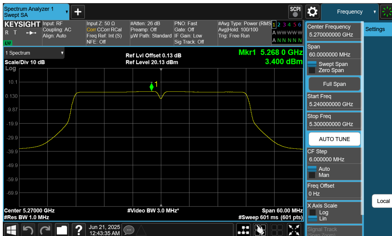
Plot 7-78 PSD CDD Diversity Antenna 4a (40MHz BW 802.11n - Ch.54)
