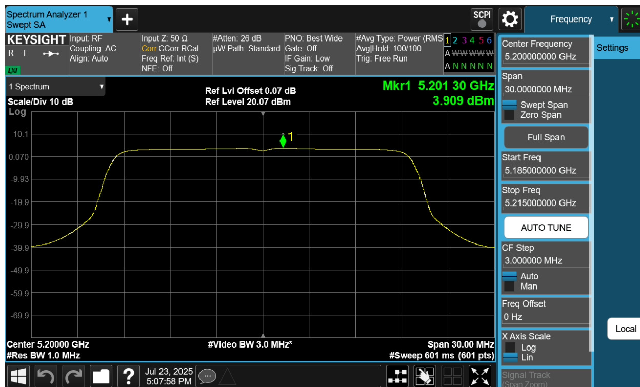
Plot 7-95 PSD SDM Diversity Antenna 2a (20MHz BW 802.11be(SU) - Ch.40)
