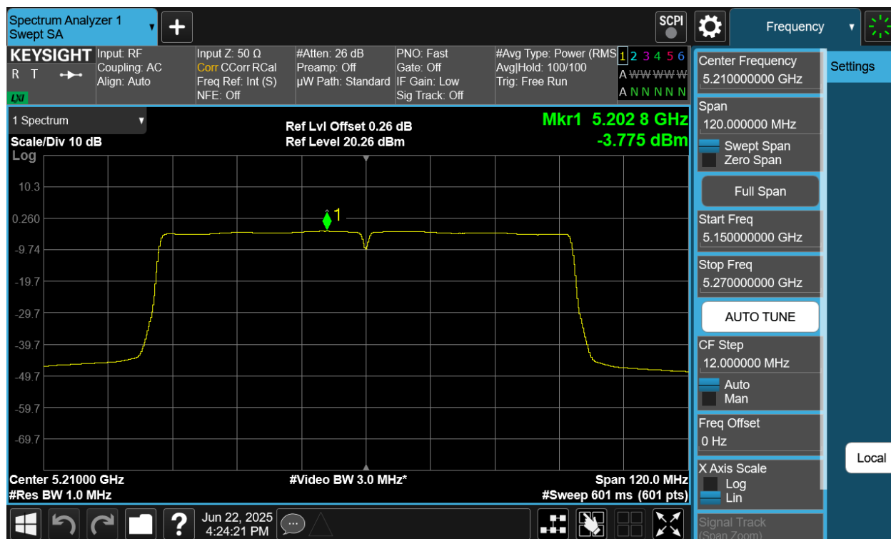
Plot 7-53 PSD Antenna 2a (80MHz BW 802.11ac - Ch.42)
