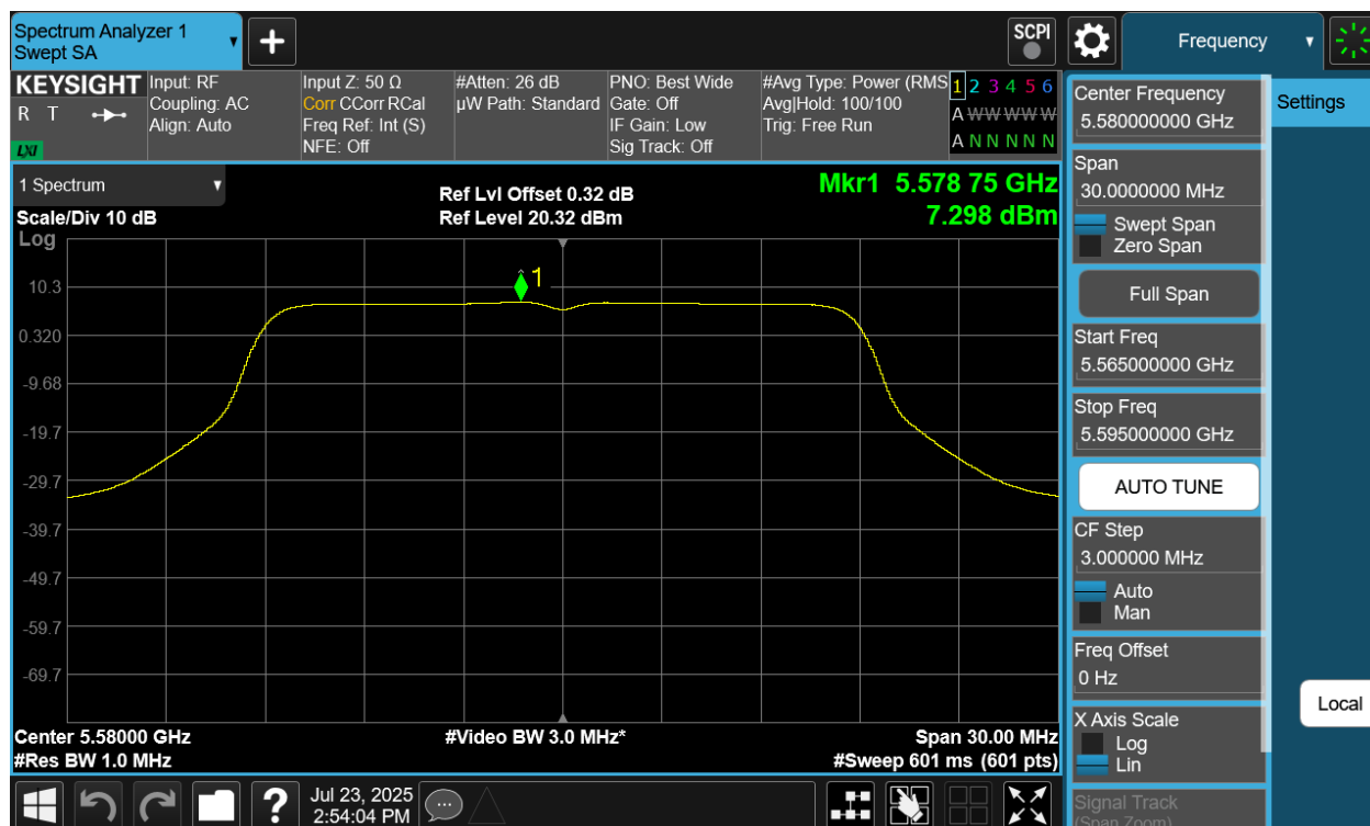
Plot 7-59 PSD CDD Primary Antenna 4a (20MHz BW 802.11a - Ch.116)
