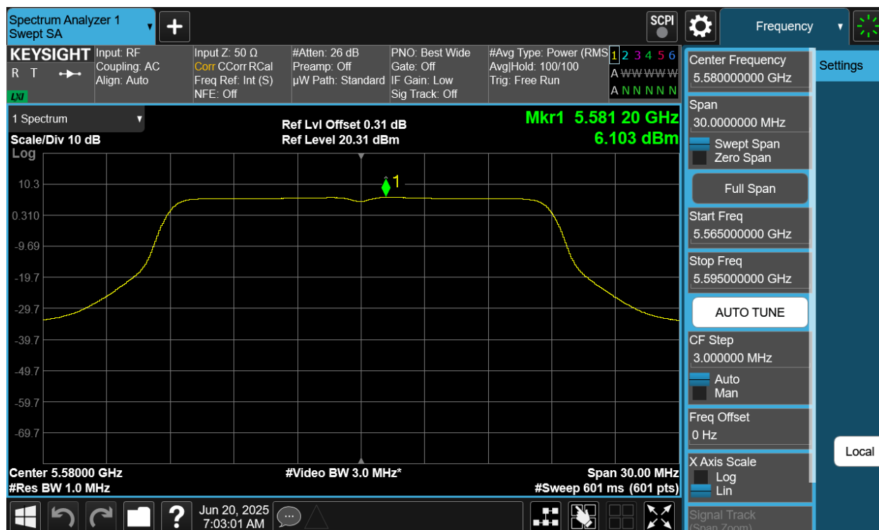
Plot 7-81 PSD CDD Diversity Antenna 2a (20MHz BW 802.11a - Ch.116)
