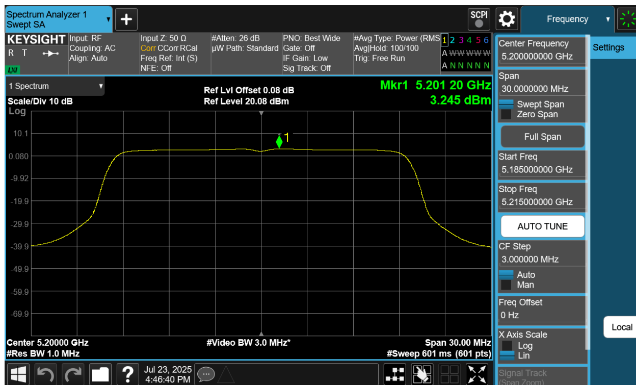
Plot 7-69 PSD SDM Primary Antenna WF5B (20MHz BW 802.11be(SU) - Ch.40)
