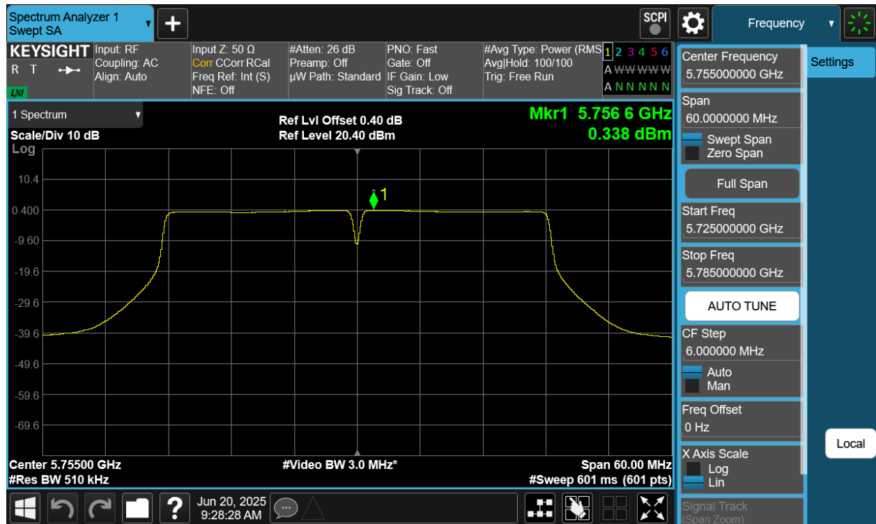
Plot 7-89 PSD CDD Diversity Antenna 2a (40MHz BW 802.11n - Ch.151)
