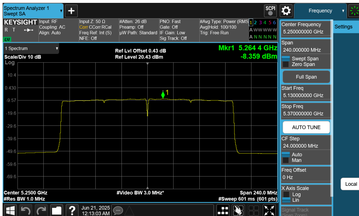
Plot 7-62 PSD CDD Primary Antenna 4a (160MHz BW 802.11be(SU) - Ch.50)
