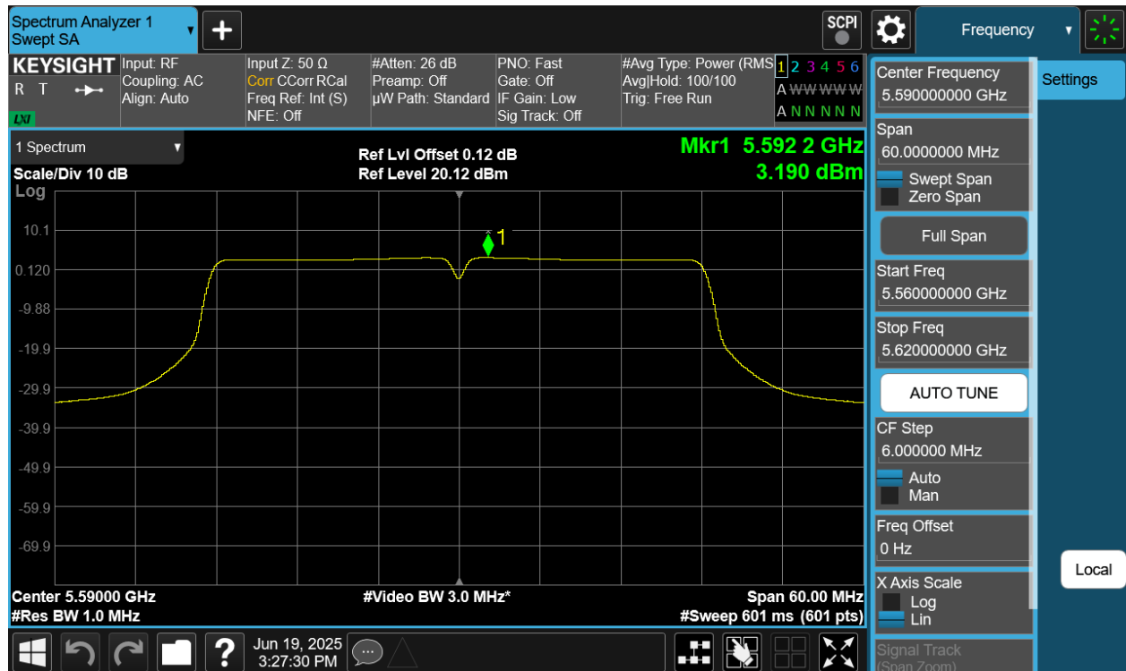
Plot 7-56 PSD CDD Primary Antenna WF5B (40MHz BW 802.11n - Ch.118)
