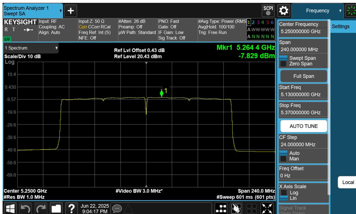
Plot 7-76 PSD CDD Primary Antenna 4a (160MHz BW 802.11be(SU) - Ch.50)
