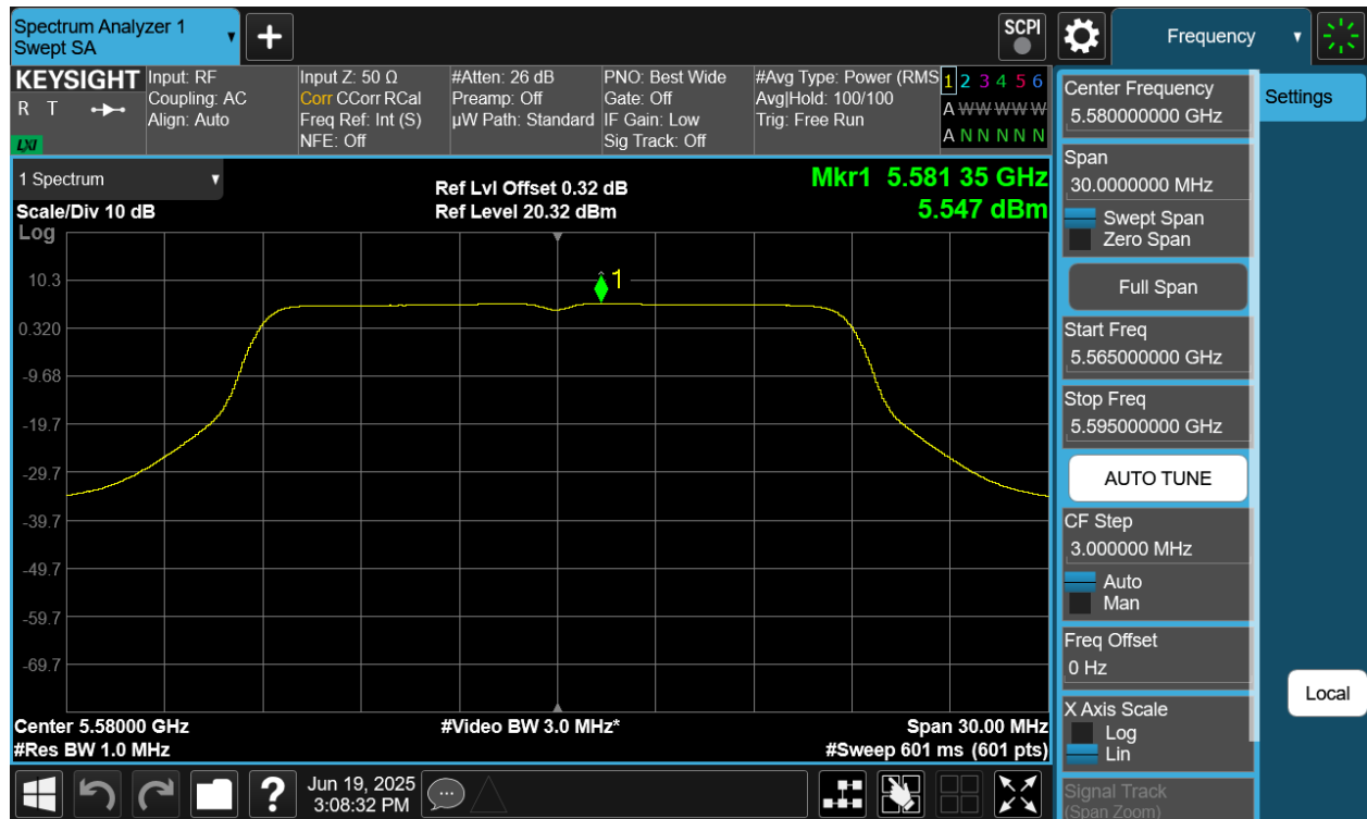
Plot 7-55 PSD CDD Primary Antenna WF5B (20MHz BW 802.11a - Ch.116)
