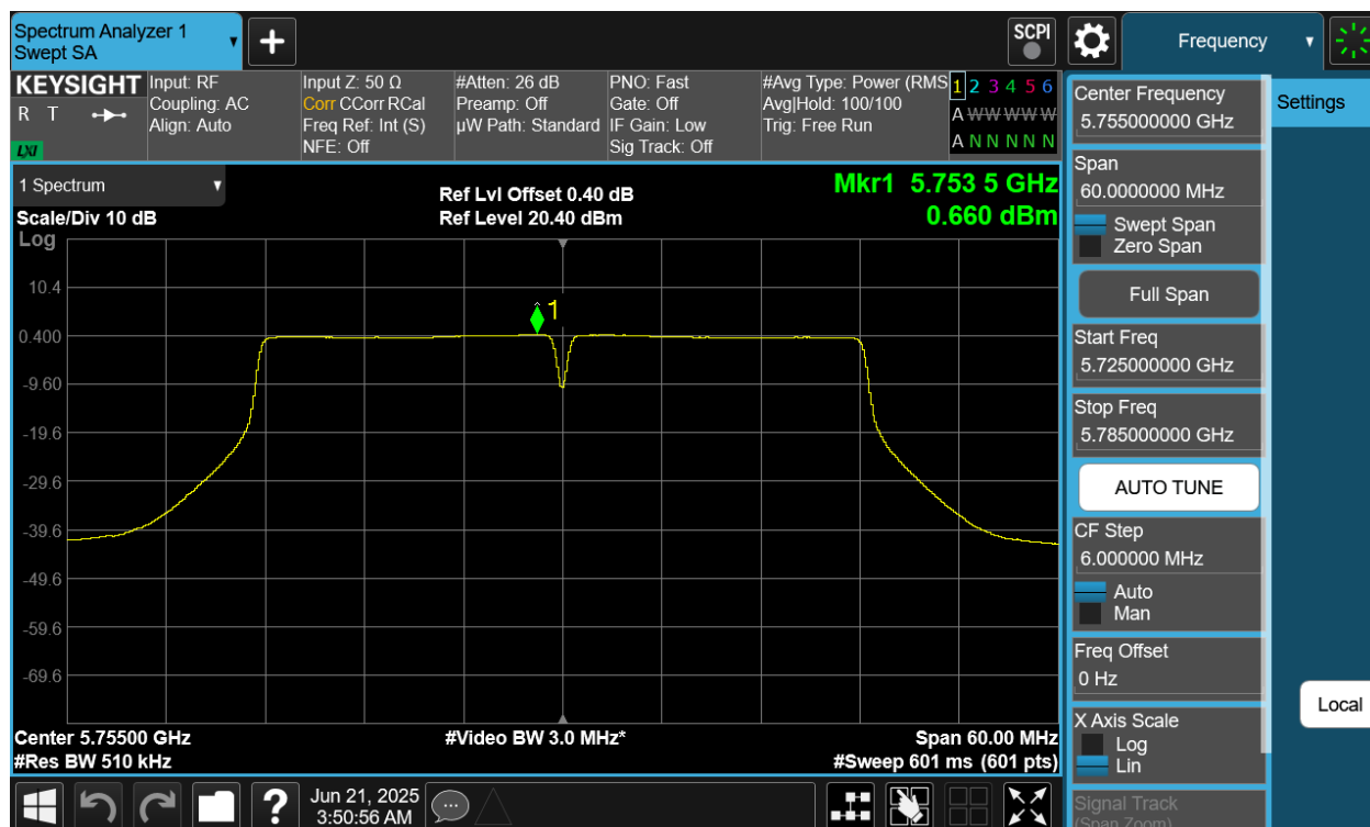
Plot 7-67 PSD CDD Primary Antenna 4a (40MHz BW 802.11n - Ch.151)
