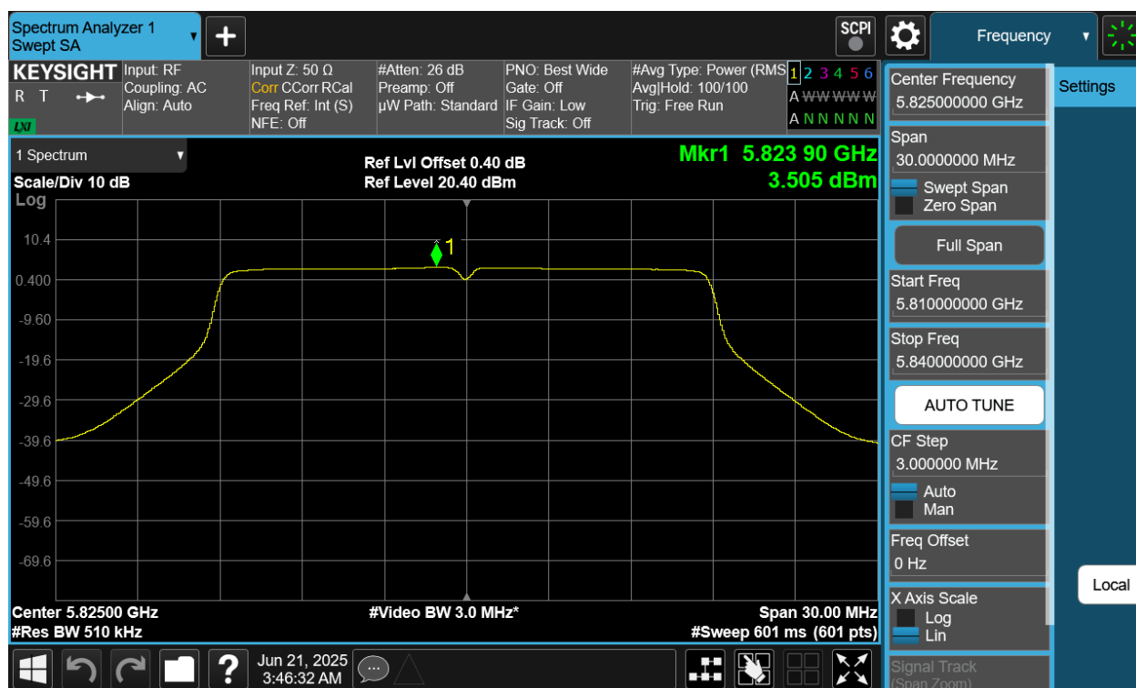
Plot 7-66 PSD CDD Primary Antenna 4a (20MHz BW 802.11n - Ch.165)
