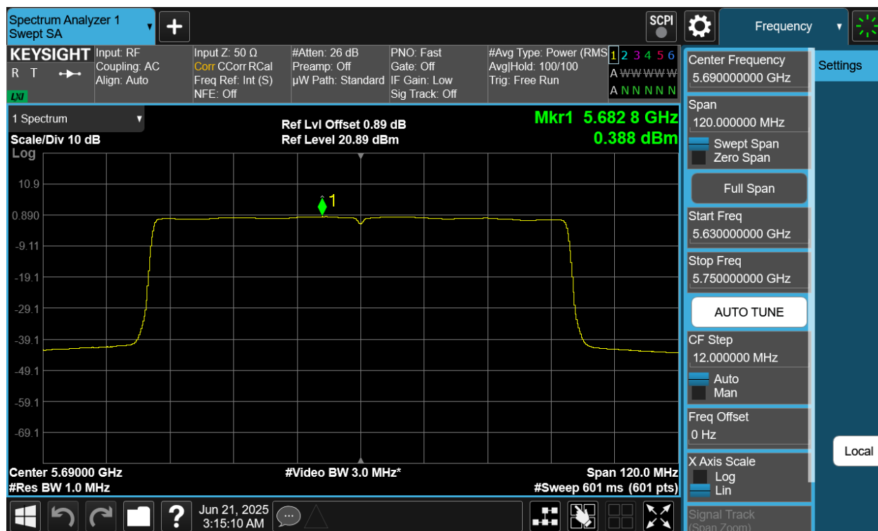
Plot 7-61 PSD CDD Primary Antenna 4a (80MHz BW 802.11be(SU) - Ch.138)
