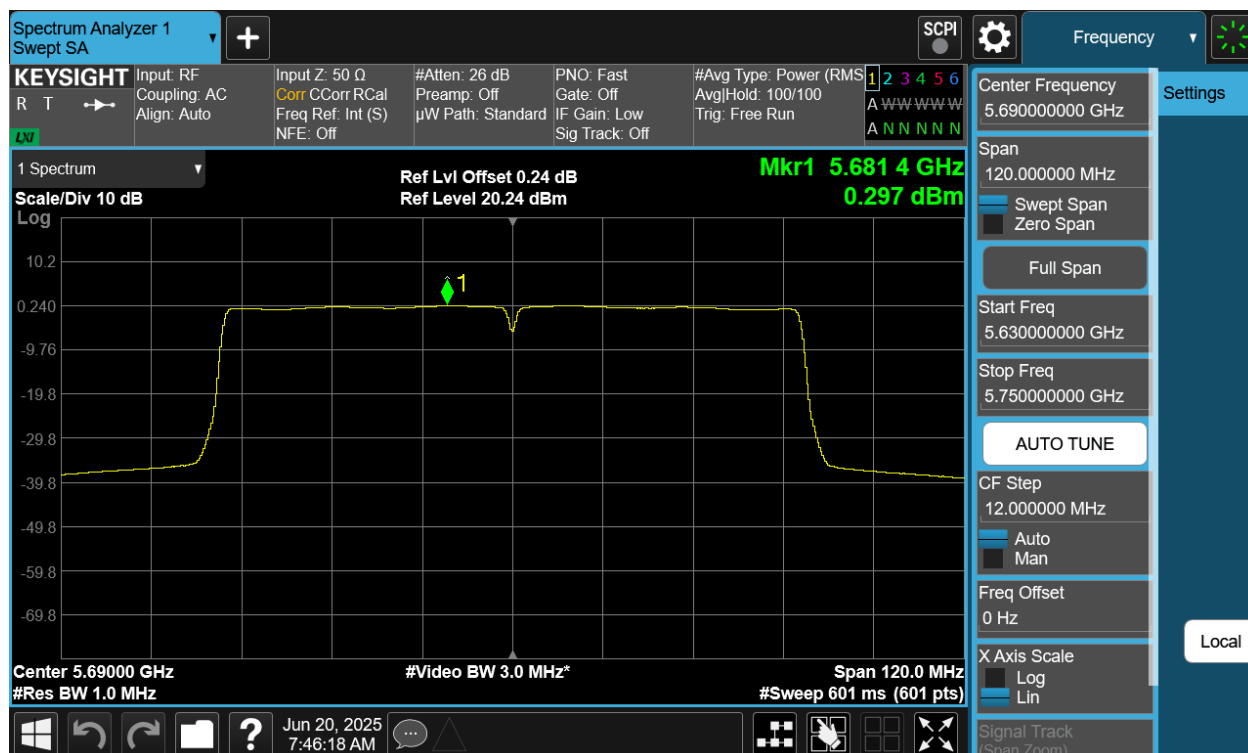
Plot 7-83 PSD CDD Diversity Antenna 2a (80MHz BW 802.11ac - Ch.138)
