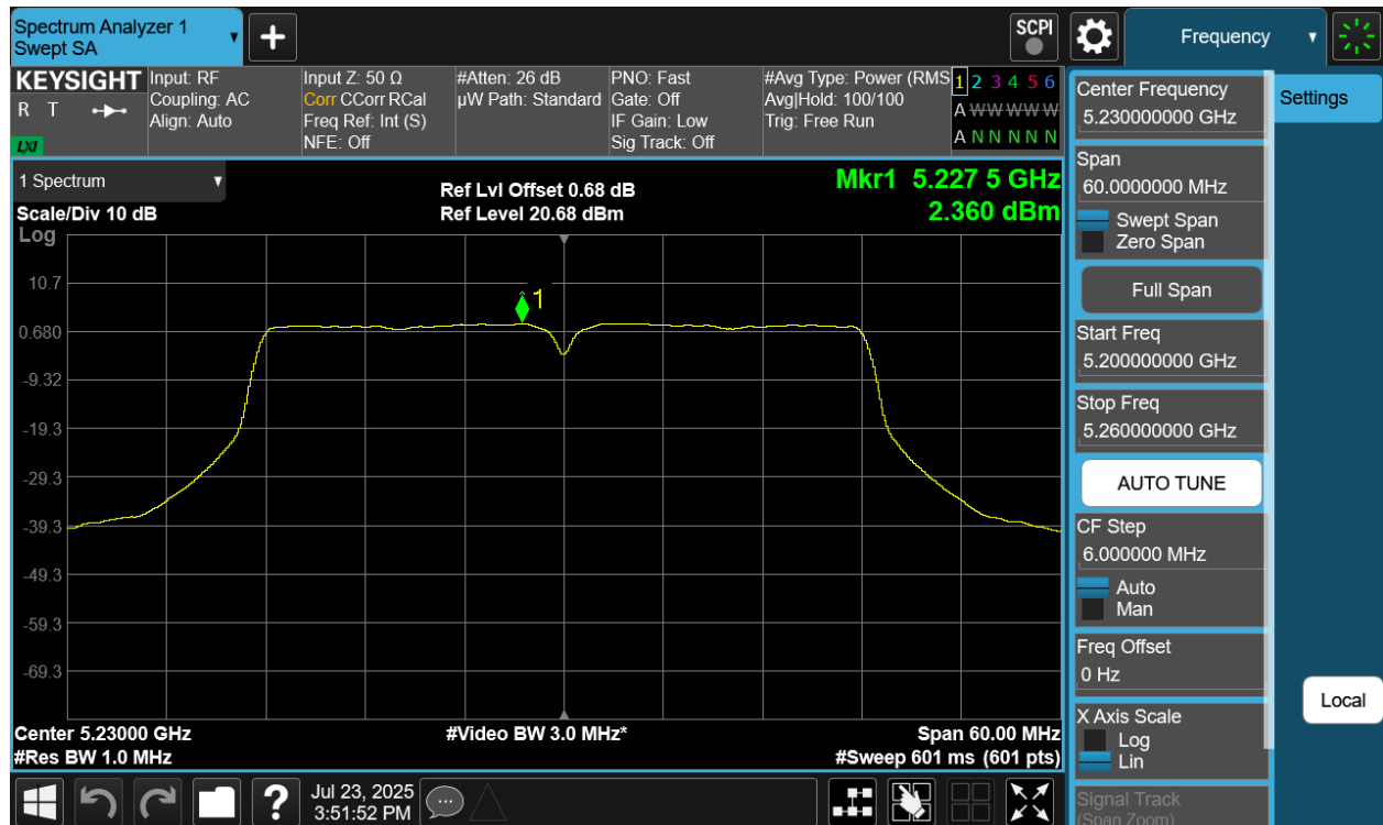
Plot 7-74 PSD SDM Primary Antenna 4a (40MHz BW 802.11n - Ch.46)
