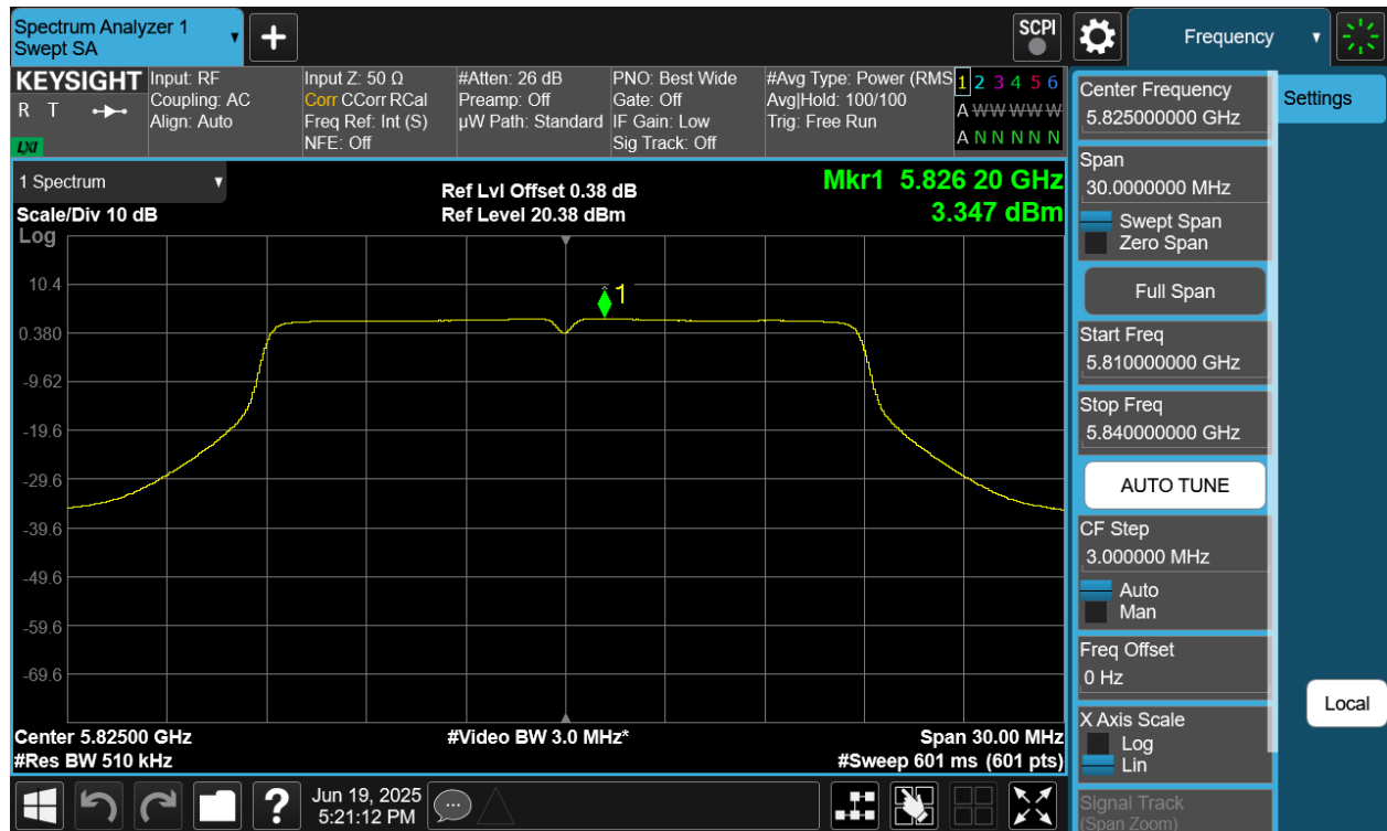
Plot 7-63 PSD CDD Primary Antenna WF5B (20MHz BW 802.11n - Ch.165)
