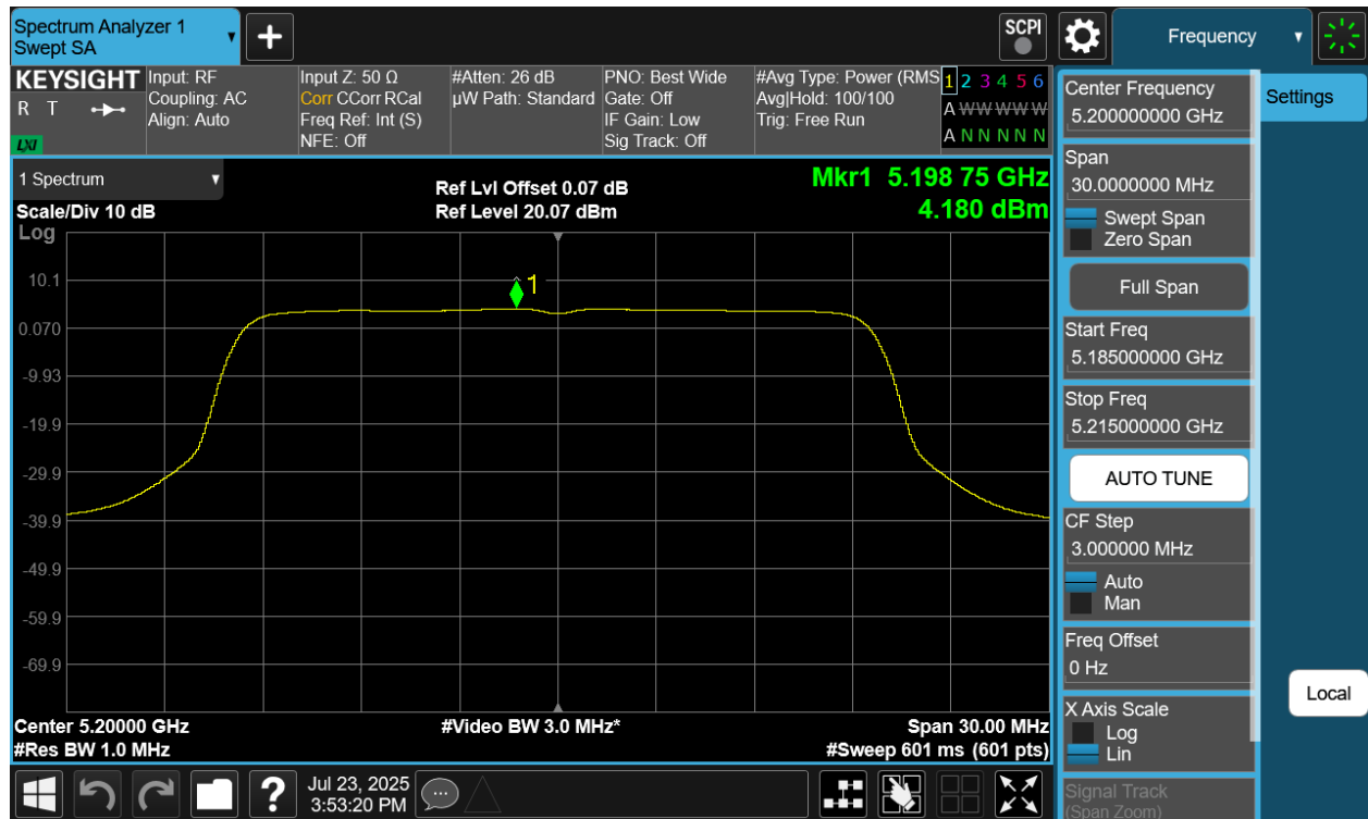
Plot 7-73 PSD SDM Primary Antenna 4a (20MHz BW 802.11be(SU) - Ch.40)
