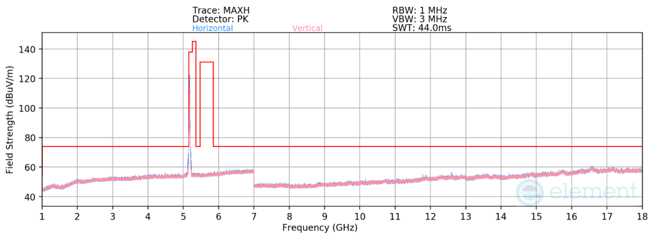
Plot 7-268. RSE above 1GHz CDD Primary (11be – Ch.36 – RU26)
