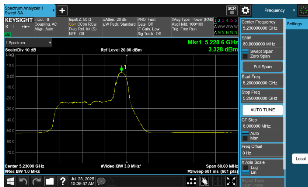
Plot 7-247 PSD SDM Diversity Antenna 2a (40MHz BW 802.11be(RU) RU26 Index8 - Ch.46)
