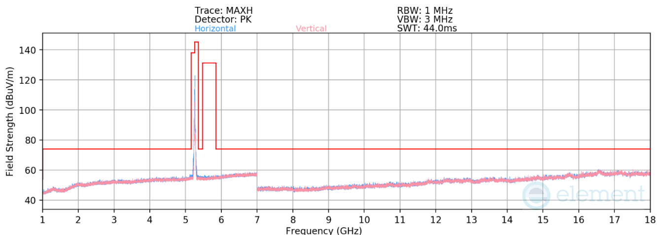
Plot 7-272. RSE above 1GHz CDD Primary (11be – Ch.52 – RU26)
