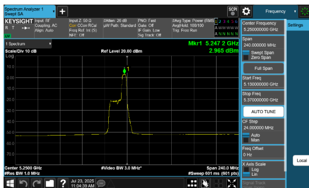
Plot 7-249 PSD SDM Diversity Antenna 2a (160MHz BW 802.11be(RU) RU52 Index52 - Ch.50)
