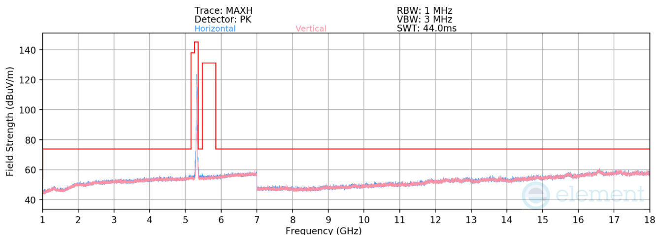
Plot 7-275. RSE above 1GHz CDD Primary (11be – Ch.64 – RU26)
