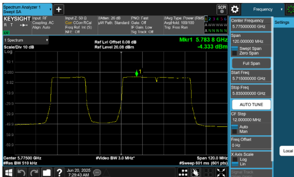
Plot 7-239 PSD CDD Diversity Antenna 4a (80MHz BW 802.11be(RU) RU484+242 Index91 - Ch.155)
