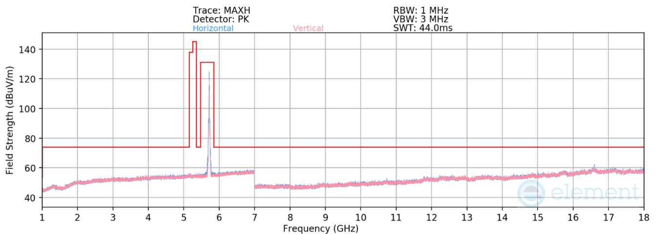
Plot 7-279. RSE above 1GHz CDD Primary (11be – Ch.144 – RU26)
