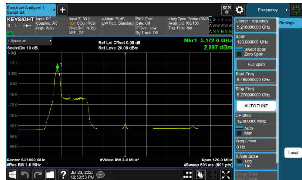
Plot 7-252 PSD SDM Diversity Antenna 4a (80MHz BW 802.11be(RU) RU26 Index0 - Ch.42)
