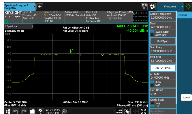
Plot 7-267 PSD CDD Diversity Antenna 4a (160MHz BW 802.11be(RU) RU996X2 Index68 - Ch.50)
