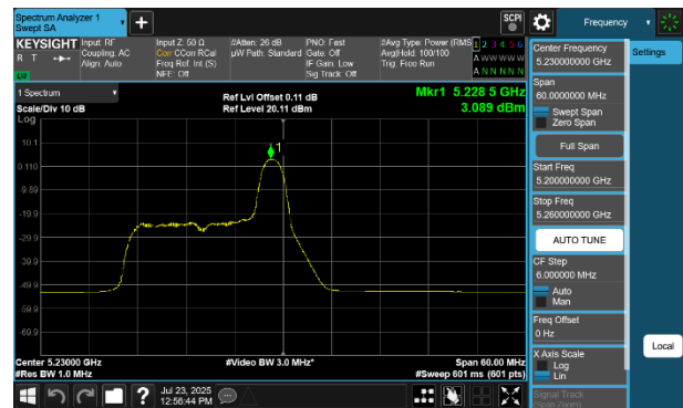
Plot 7-251 PSD SDM Diversity Antenna 4a (40MHz BW 802.11be(RU) RU26 Index8 - Ch.46)
