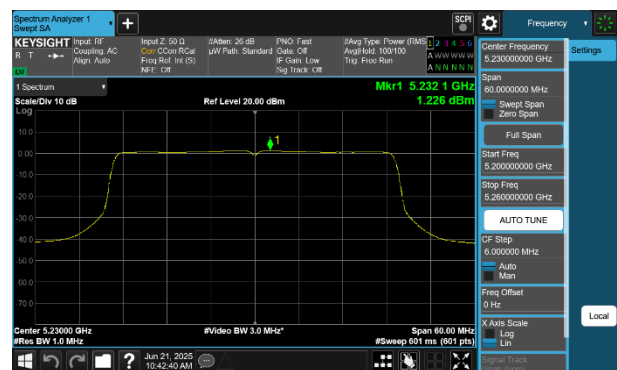
Plot 7-261 PSD SDM Diversity Antenna 2a (40MHz BW 802.11be(RU) RU484 Index65 - Ch.46)
