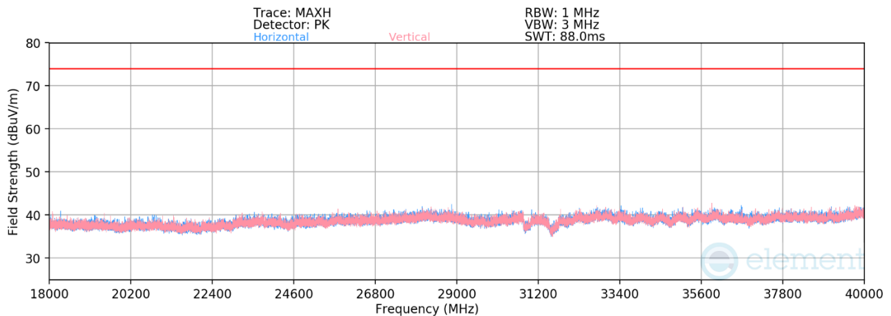
Plot 7-290. RSE 18GHz – 40 GHz CDD Primary (11be Ch.56 — RU242)
