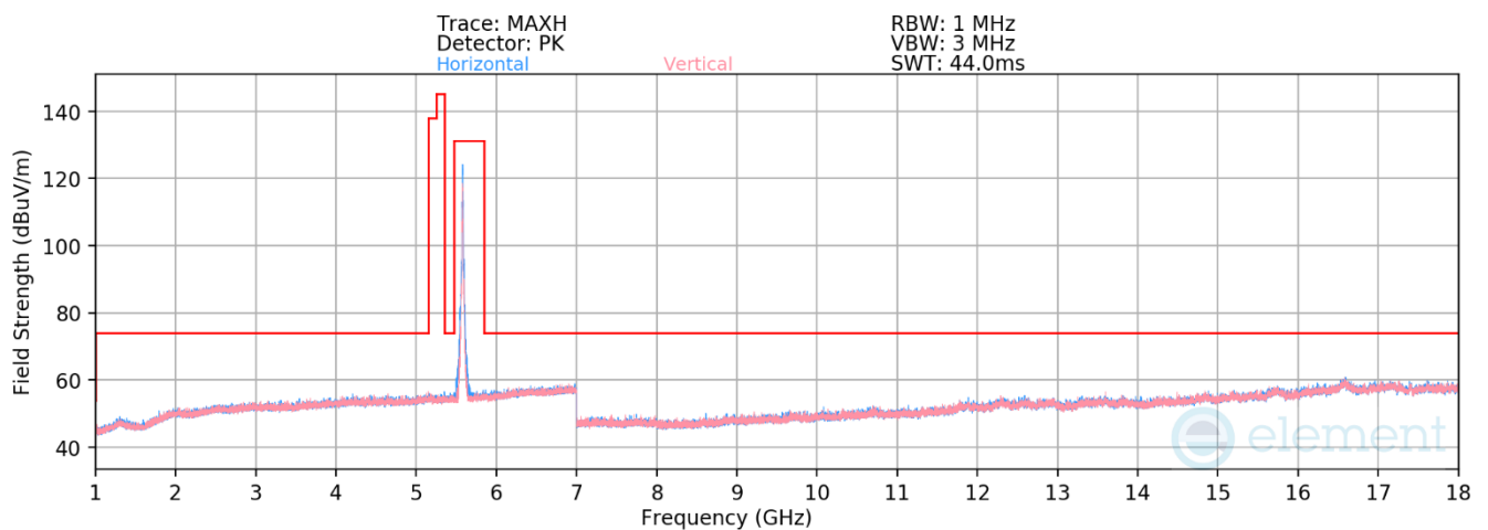
Plot 7-277. RSE above 1GHz CDD Primary (11be – Ch.116 – RU26)
