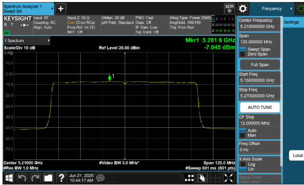
Plot 7-262 PSD CDD Diversity Antenna 2a (80MHz BW 802.11be(RU) RU996 Index67 - Ch.42)
