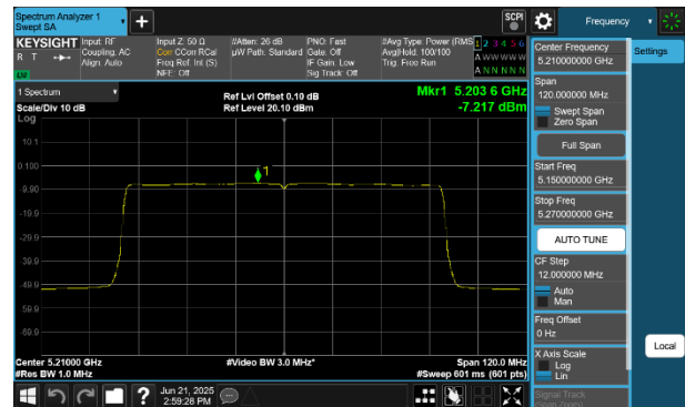
Plot 7-266 PSD CDD Diversity Antenna 4a (80MHz BW 802.11be(RU) RU996 Index67 - Ch.42)
