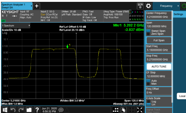
Plot 7-255 PSD CDD Diversity Antenna 2a (80MHz BW 802.11be(RU) RU484+242 Index92 - Ch.42)
