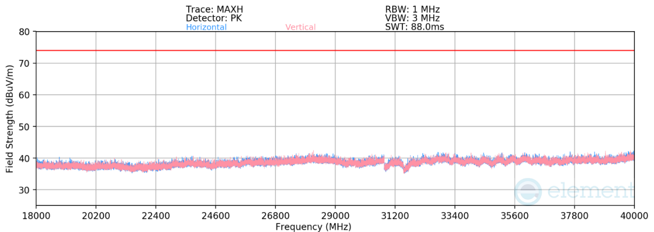
Plot 7-286. RSE 18GHz – 40 GHz CDD Primary (11be Ch.40 — RU242)
