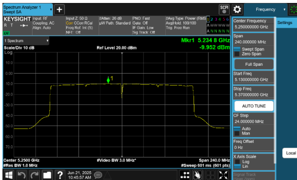
Plot 7-263 PSD CDD Diversity Antenna 2a (160MHz BW 802.11be(RU) RU996X2 Index68 - Ch.50)
