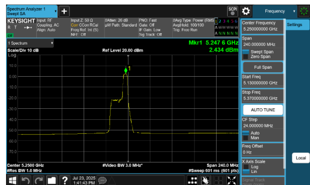
Plot 7-253 PSD SDM Diversity Antenna 4a (160MHz BW 802.11be(RU) RU52 Index52 - Ch.50)
