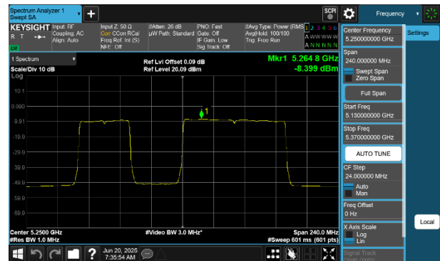
Plot 7-259 PSD CDD Diversity Antenna 4a (160MHz BW 802.11be(RU) RU996+484 Index95 - Ch.50)
