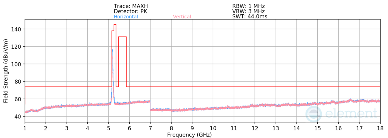
Plot 7-285. RSE above 1GHz CDD Primary (11be – Ch.40 – RU242)
