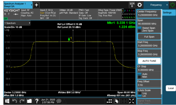
Plot 7-265 PSD SDM Diversity Antenna 4a (40MHz BW 802.11be(RU) RU484 Index65 - Ch.46)
