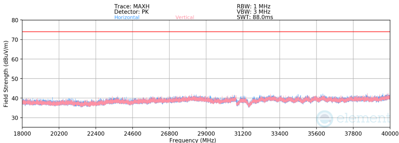
Plot 7-274. RSE 18GHz – 40 GHz CDD Primary (11be Ch.56 — RU26)
