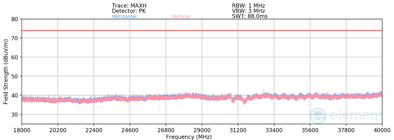
Plot 7-278. RSE 18GHz – 40 GHz CDD Primary (11be Ch.116 — RU26)
