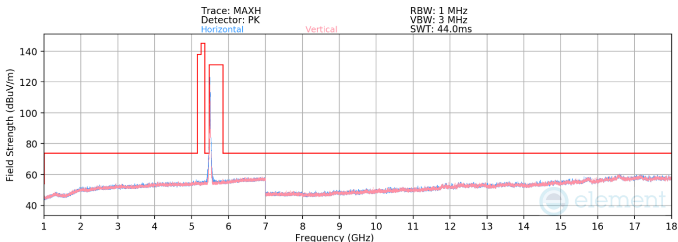
Plot 7-276. RSE above 1GHz CDD Primary (11be – Ch.100 – RU26)
