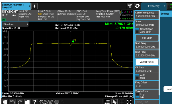
Plot 7-241 PSD CDD Diversity Antenna 2a (40MHz BW 802.11be(RU) RU484 Index65 - Ch.159)
