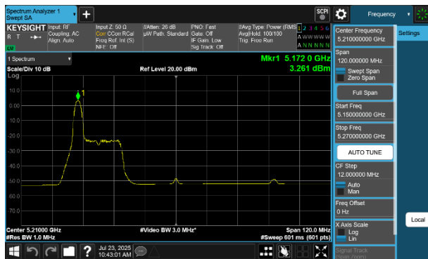
Plot 7-248 PSD SDM Diversity Antenna 2a (80MHz BW 802.11be(RU) RU26 Index0 - Ch.42)
