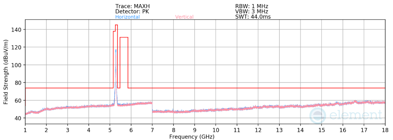
Plot 7-289. RSE above 1GHz CDD Primary (11be – Ch.56 – RU242)
