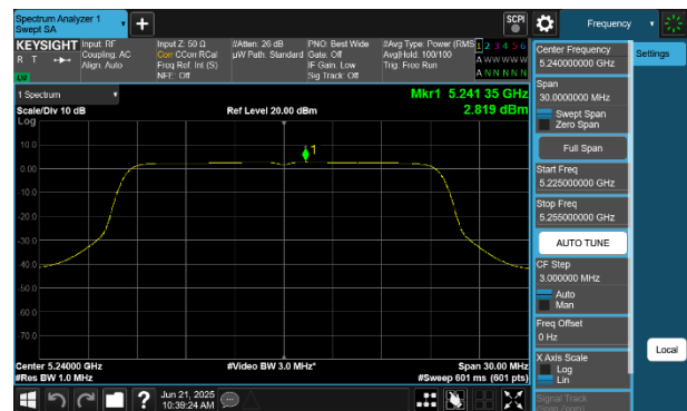
Plot 7-260 PSD SDM Diversity Antenna 2a (20MHz BW 802.11be(RU) RU242 Index61 - Ch.48)
