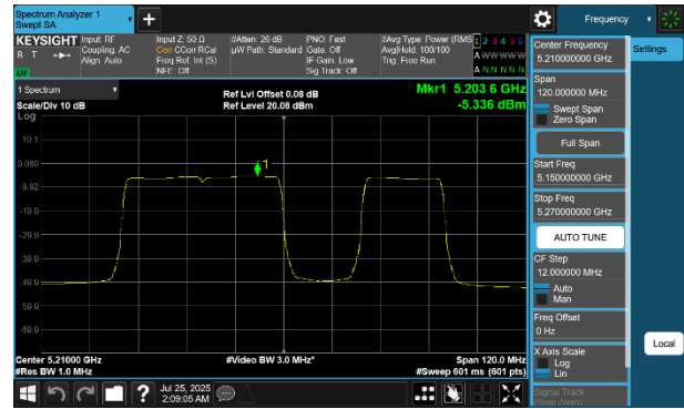
Plot 7-258 PSD CDD Diversity Antenna 4a (80MHz BW 802.11be(RU) RU484+242 Index92 - Ch.42)
