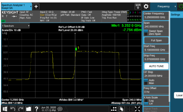
Plot 7-256 PSD CDD Diversity Antenna 2a (160MHz BW 802.11be(RU) RU996+484 Index95 - Ch.50)
