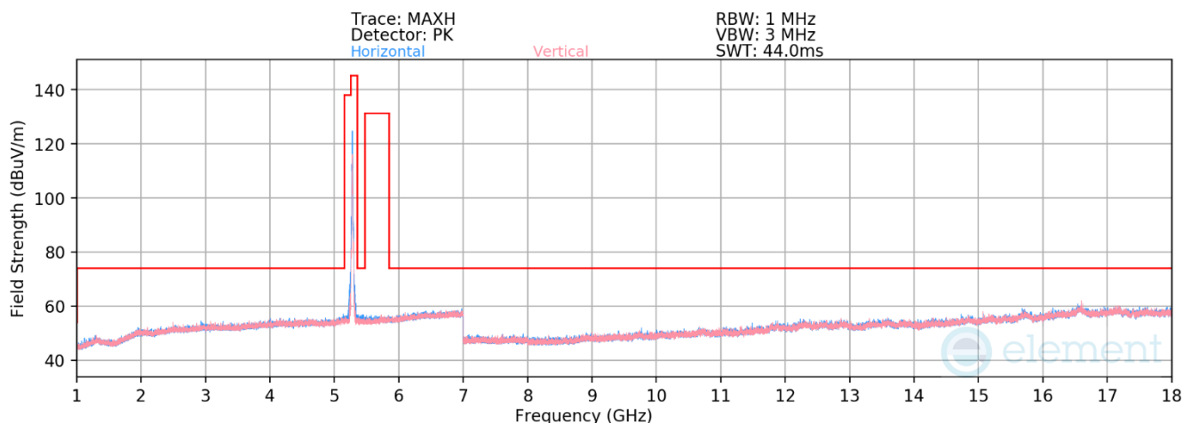
Plot 7-273. RSE above 1GHz CDD Primary (11be – Ch.56 – RU26)
