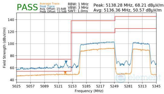
Plot 7-779. Antenna 2a (Peak & Average, RU996+484, Index 94 (H), Ch.50, MCS11)
