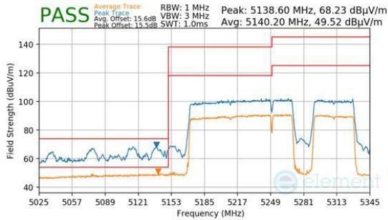
Plot 7-797. Antenna 2a (Peak & Average, RU996+484+242, Index 97 (H), Ch.50, MCS11)
