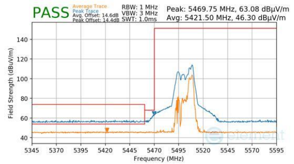
Plot 7-840. CDD Primary (Peak & Average, RU52, Index 40, Ch.100, MCS11)
