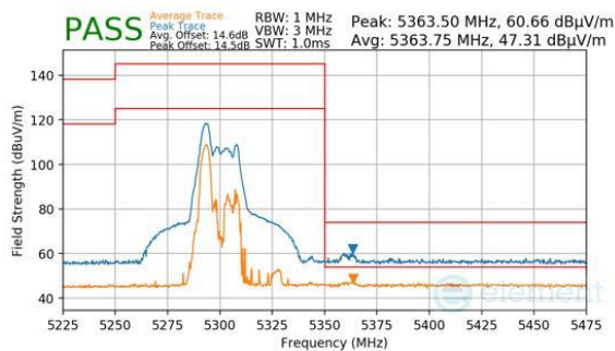
Plot 7-876. CDD Primary (Peak & Average, RU52, Index 37, Ch.62, MCS11)
