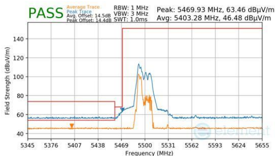
Plot 7-903. CDD Primary (Peak & Average, RU52, Index 37, Ch.106, MCS11)
