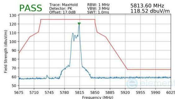
Plot 7-875. CDD Primary (Peak, RU26, Index 17, Ch.159, MCS11)
