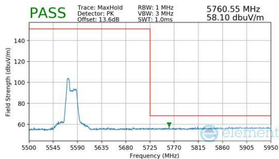
Plot 7-777. Antenna 2a (Peak, RU52, Index 37, Ch.114 (FCC ONLY), MCS11)
