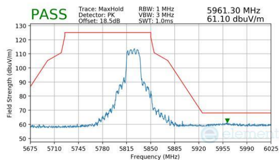
Plot 7-869. CDD Primary (Peak, RU242, Index 61, Ch.165, MCS11)
