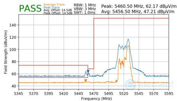
Plot 7-879. CDD Primary (Peak & Average, RU52, Index 44, Ch.102, MCS11)
