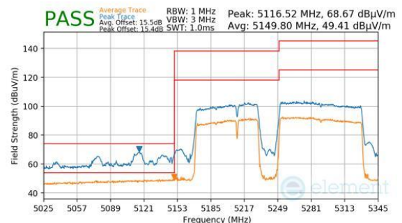
Plot 7-802. Antenna 2a (Peak & Average, RU996+484+242, Index 99 (L), Ch.50, MCS11)
