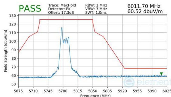
Plot 7-874. CDD Primary (Peak, RU26, Index 0, Ch.159, MCS11)
