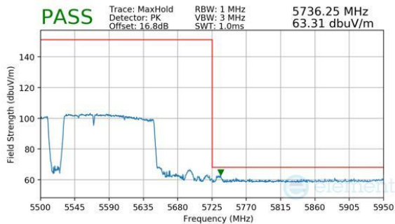
Plot 7-822. Antenna 2a (Peak, RU996+484+242, Index 97 (L), Ch.114 (FCC ONLY), MCS11)
