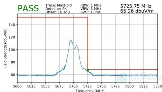
Plot 7-853. CDD Primary (Peak, RU52+26, Index 70, Ch.140, MCS11)
