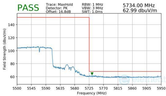
Plot 7-793. Antenna 2a (Peak, RU996+484, Index 95 (H), Ch.114 (FCC ONLY), MCS11)
