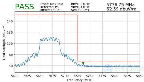
Plot 7-892. CDD Primary (Peak, RU484, Index 65, Ch.134, MCS11)
