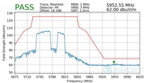
Plot 7-762. Antenna 2a (Peak, RU484+242, Index 92, Ch.155, MCS11)
