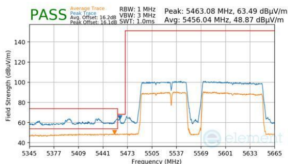
Plot 7-817. Antenna 2a (Peak & Average, RU996+484+242, Index 99 (L), Ch.114 (FCC ONLY), MCS11)
