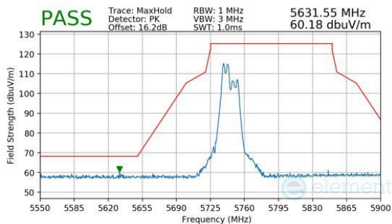
Plot 7-855. CDD Primary (Peak, RU52+26, Index 70, Ch.149, MCS11)
