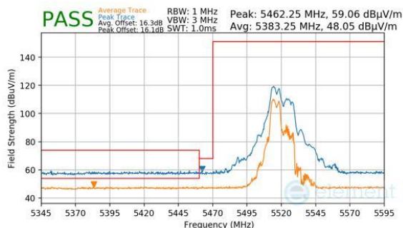
Plot 7-849. CDD Primary (Peak & Average, RU52+26, Index 70, Ch.104, MCS11)
