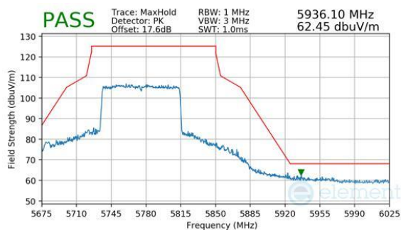
Plot 7-770. Antenna 2a (Peak, RU996, Index 67, Ch.155, MCS11)
