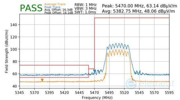
Plot 7-888. CDD Primary (Peak & Average, RU484, Index 65, Ch.102, MCS11)
