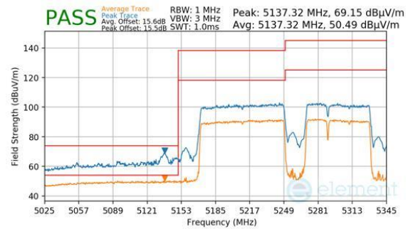
Plot 7-795. Antenna 2a (Peak & Average, RU996+484+242, Index 96 (H), Ch.50, MCS11)
