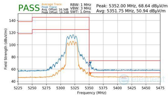
Plot 7-862. CDD Primary (Peak & Average, RU242, Index 61, Ch.64, MCS11)
