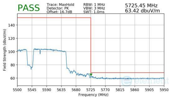
Plot 7-823. Antenna 2a (Peak, RU996+484+242, Index 98 (L), Ch.114 (FCC ONLY), MCS11)
