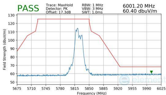
Plot 7-857. CDD Primary (Peak, RU52+26, Index 70, Ch.165, MCS11)
