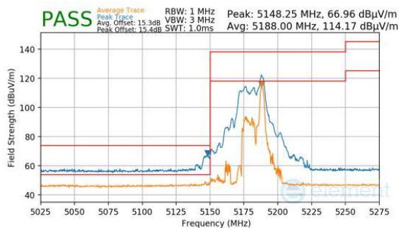
Plot 7-832. CDD Primary (Peak & Average, RU26, Index 8, Ch.36, MCS11)
