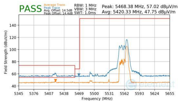
Plot 7-904. CDD Primary (Peak & Average, RU52, Index 52, Ch.106, MCS11)
