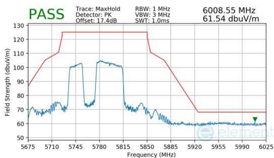
Plot 7-761. Antenna 2a (Peak, RU484+242, Index 91, Ch.155, MCS11)
