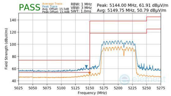
Plot 7-910. CDD Primary (Peak & Average, RU484+242, Index 93, Ch.42, MCS11)
