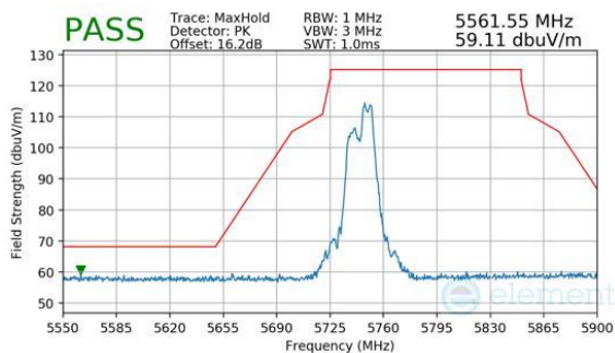
Plot 7-856. CDD Primary (Peak, RU52+26, Index 72, Ch.149, MCS11)
