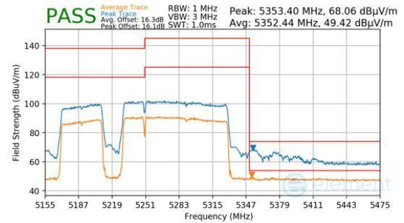
Plot 7-807. Antenna 2a (Peak & Average, RU996+484+242, Index 98 (L), Ch.50, MCS11)
