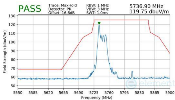
Plot 7-897. CDD Primary (Peak, RU26, Index 0, Ch.155, MCS11)
