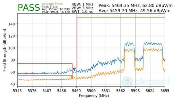
Plot 7-920. CDD Primary (Peak & Average, RU484+242, Index 91, Ch.122 (FCC ONLY), MCS11)
