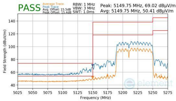
Plot 7-907. CDD Primary (Peak & Average, RU484+242, Index 90, Ch.42, MCS11)
