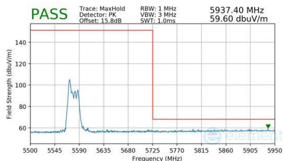
Plot 7-905. CDD Primary (Peak, RU52, Index 37, Ch.122 (FCC ONLY), MCS11)
