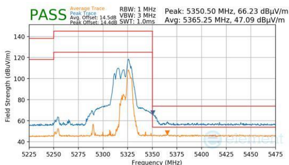
Plot 7-902. CDD Primary (Peak & Average, RU52, Index 52, Ch.58, MCS11)
