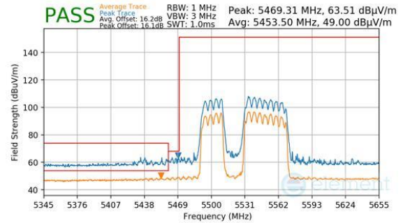
Plot 7-916. CDD Primary (Peak & Average, RU484+242, Index 91, Ch.106, MCS11)
