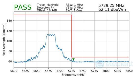
Plot 7-866. CDD Primary (Peak, RU242, Index 61, Ch.136, MCS11)
