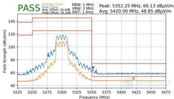
Plot 7-861. CDD Primary (Peak & Average, RU242, Index 61, Ch.60, MCS11)
