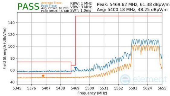
Plot 7-919. CDD Primary (Peak & Average, RU484+242, Index 90, Ch.122 (FCC ONLY), MCS11)
