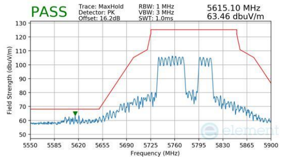
Plot 7-929. CDD Primary (Peak, RU484+242, Index 92, Ch.155, MCS11)
