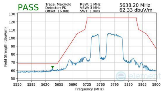
Plot 7-757. Antenna 2a (Peak, RU484+242, Index 91, Ch.155, MCS11)
