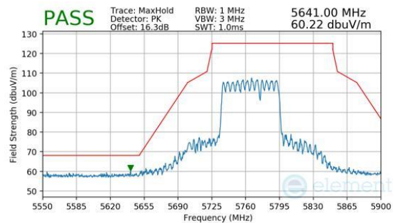
Plot 7-930. CDD Primary (Peak, RU484+242, Index 93, Ch.155, MCS11)
