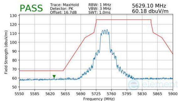
Plot 7-868. CDD Primary (Peak, RU242, Index 61, Ch.149, MCS11)
