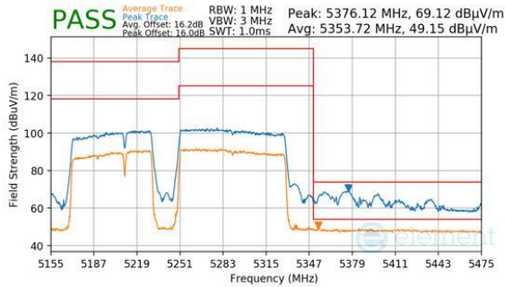
Plot 7-809. Antenna 2a (Peak & Average, RU996+484+242, Index 99 (L), Ch.50, MCS11)
