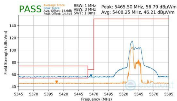
Plot 7-880. CDD Primary (Peak & Average, RU52, Index 37, Ch.110, MCS11)
