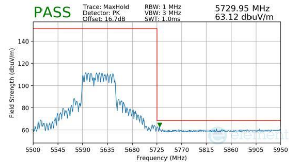
Plot 7-923. CDD Primary (Peak, RU484+242, Index 90, Ch.122 (FCC ONLY), MCS11)
