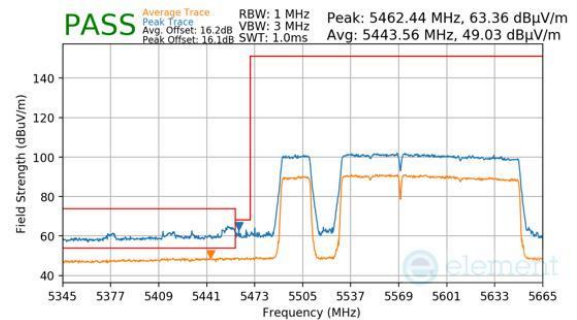
Plot 7-813. Antenna 2a (Peak & Average, RU996+484+242, Index 97 (L), Ch.114 (FCC ONLY), MCS11)
