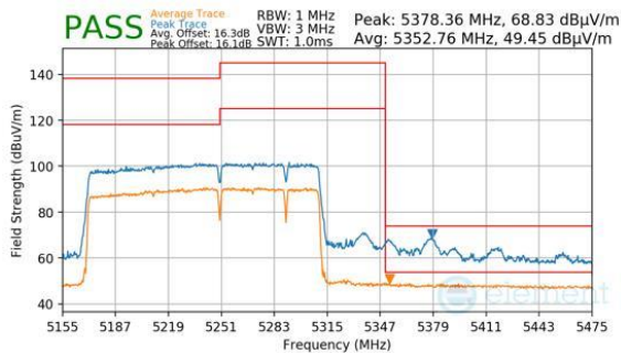
Plot 7-810. Antenna 2a (Peak & Average, RU996+484+242, Index 99 (H), Ch.50, MCS11)
