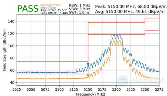
Plot 7-860. CDD Primary (Peak & Average, RU242, Index 61, Ch.40, MCS11)
