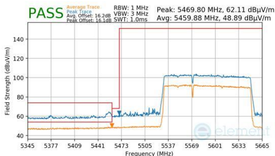
Plot 7-787. Antenna 2a (Peak & Average, RU996+484, Index 94 (L), Ch.114 (FCC ONLY), MCS11)
