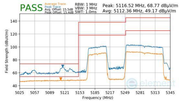
Plot 7-782. Antenna 2a (Peak & Average, RU996+484, Index 95 (L), Ch.50, MCS11)
