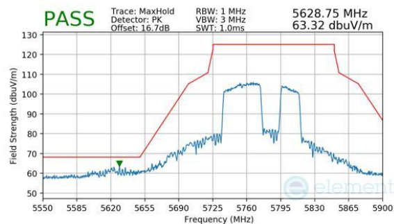
Plot 7-758. Antenna 2a (Peak, RU484+242, Index 92, Ch.155, MCS11)
