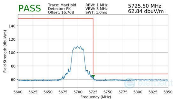
Plot 7-867. CDD Primary (Peak, RU242, Index 61, Ch.140, MCS11)
