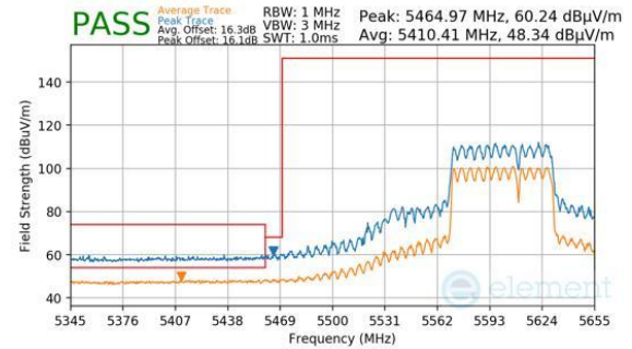
Plot 7-922. CDD Primary (Peak & Average, RU484+242, Index 93, Ch.122 (FCC ONLY), MCS11)
