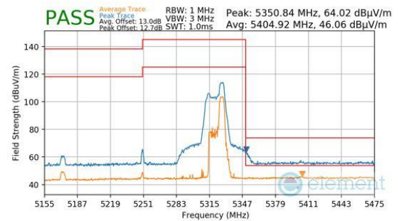
Plot 7-774. Antenna 2a (Peak & Average, RU52, Index 52 (H), Ch.50, MCS11)
