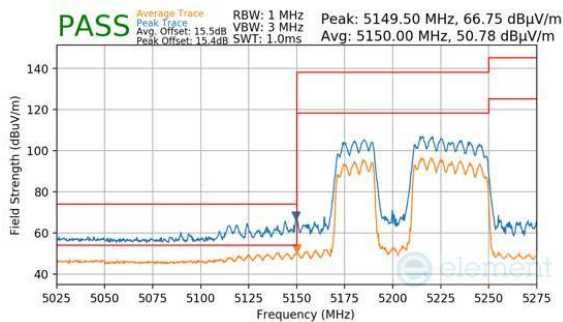
Plot 7-908. CDD Primary (Peak & Average, RU484+242, Index 91, Ch.42, MCS11)
