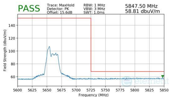
Plot 7-882. CDD Primary (Peak, RU52, Index 37, Ch.134, MCS11)
