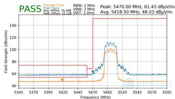
Plot 7-863. CDD Primary (Peak & Average, RU242, Index 61, Ch.100, MCS11)
