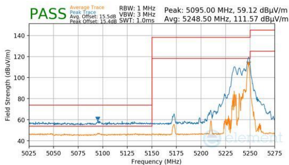
Plot 7-896. CDD Primary (Peak & Average, RU26, Index 36, Ch.42, MCS11)
