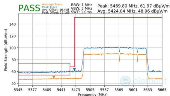
Plot 7-818. Antenna 2a (Peak & Average, RU996+484+242, Index 99 (H), Ch.114 (FCC ONLY), MCS11)
