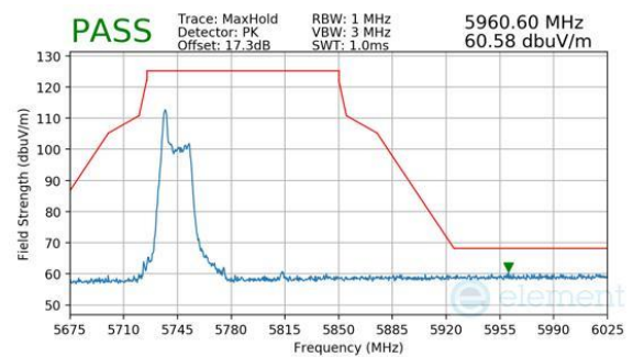
Plot 7-899. CDD Primary (Peak, RU26, Index 0, Ch.155, MCS11)
