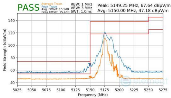
Plot 7-843. CDD Primary (Peak & Average, RU52+26, Index 70, Ch.36, MCS11)
