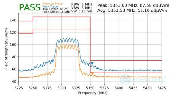
Plot 7-887. CDD Primary (Peak & Average, RU484, Index 65, Ch.62, MCS11)
