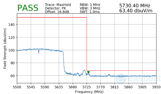
Plot 7-830. Antenna 2a (Peak, RU996X2, Index 68, Ch.114 FCC ONLY, MCS11)
