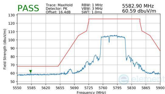
Plot 7-756. Antenna 2a (Peak, RU484+242, Index 90, Ch.155, MCS11)
