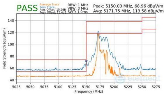
Plot 7-895. CDD Primary (Peak & Average, RU26, Index 0, Ch.42, MCS11)
