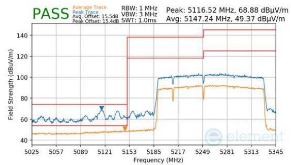
Plot 7-796. Antenna 2a (Peak & Average, RU996+484+242, Index 96 (L), Ch.50, MCS11)
