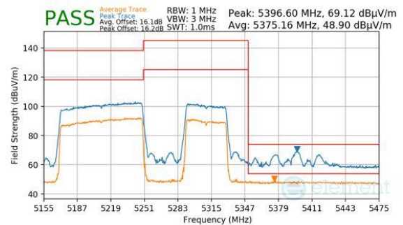
Plot 7-783. Antenna 2a (Peak & Average, RU996+484, Index 94 (H), Ch.50, MCS11)
