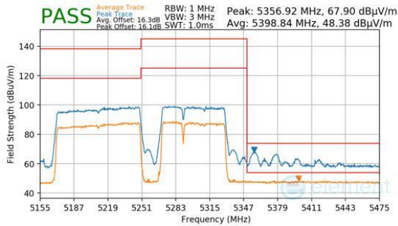
Plot 7-804. Antenna 2a (Peak & Average, RU996+484+242, Index 96 (H), Ch.50, MCS11)
