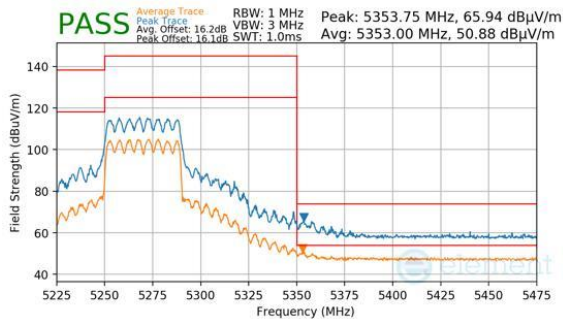
Plot 7-886. CDD Primary (Peak & Average, RU484, Index 65, Ch.54, MCS11)
