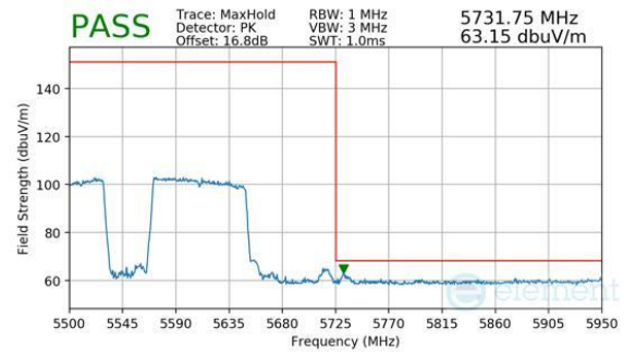
Plot 7-794. Antenna 2a (Peak, RU996+484, Index 95 (L), Ch.114 (FCC ONLY), MCS11)
