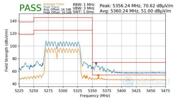
Plot 7-911. CDD Primary (Peak & Average, RU484+242, Index 90, Ch.58, MCS11)
