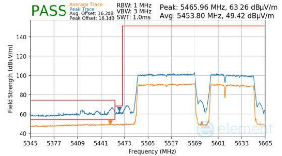
Plot 7-812. Antenna 2a (Peak & Average, RU996+484+242, Index 96 (H), Ch.114 (FCC ONLY), MCS11)
