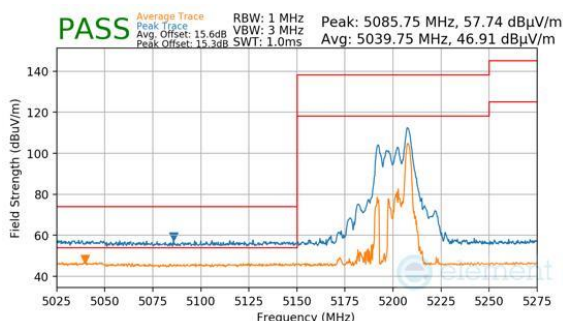
Plot 7-871. CDD Primary (Peak & Average, RU26, Index 17, Ch.38, MCS11)
