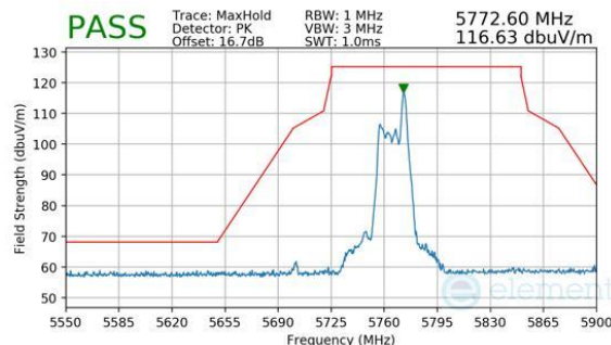
Plot 7-873. CDD Primary (Peak, RU26, Index 17, Ch.151, MCS11)
