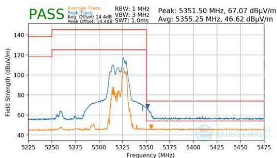
Plot 7-877. CDD Primary (Peak & Average, RU52, Index 44, Ch.62, MCS11)
