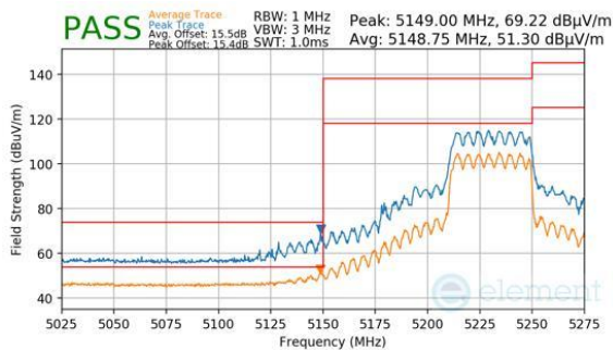
Plot 7-885. CDD Primary (Peak & Average, RU484, Index 65, Ch.46, MCS11)
