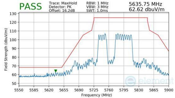
Plot 7-928. CDD Primary (Peak, RU484+242, Index 91, Ch.155, MCS11)
