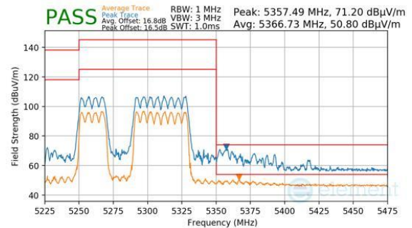
Plot 7-912. CDD Primary (Peak & Average, RU484+242, Index 91, Ch.58, MCS11)
