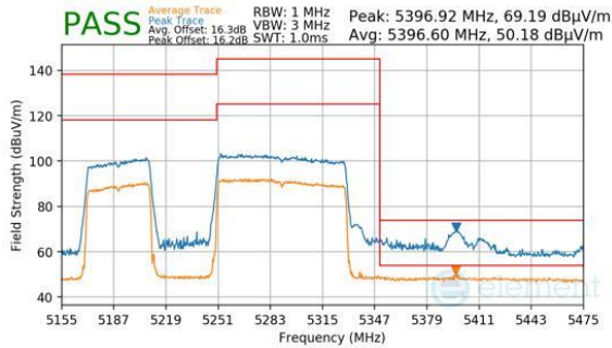
Plot 7-785. Antenna 2a (Peak & Average, RU996+484, Index 95 (L), Ch.50, MCS11)
