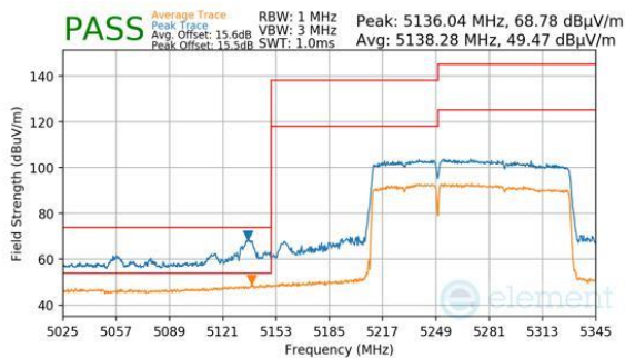
Plot 7-780. Antenna 2a (Peak & Average, RU996+484, Index 94 (L), Ch.50, MCS11)
