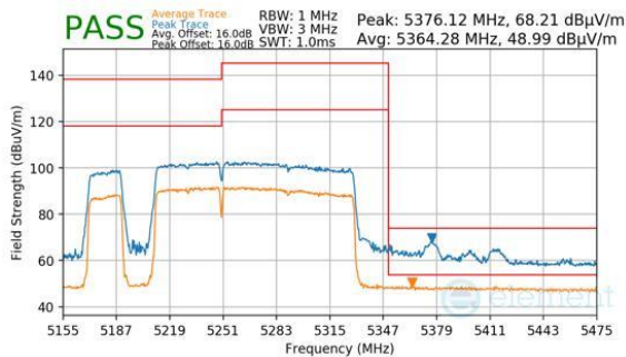
Plot 7-805. Antenna 2a (Peak & Average, RU996+484+242, Index 97 (L), Ch.50, MCS11)
