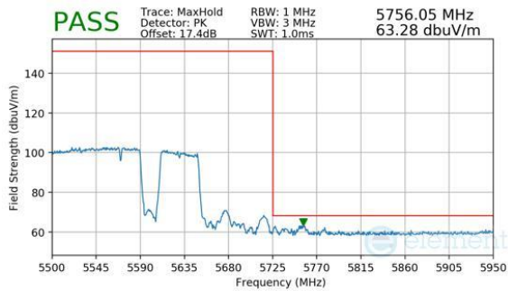
Plot 7-821. Antenna 2a (Peak, RU996+484+242, Index 97 (H), Ch.114 (FCC ONLY), MCS11)
