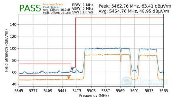
Plot 7-814. Antenna 2a (Peak & Average, RU996+484+242, Index 97 (H), Ch.114 (FCC ONLY), MCS11)
