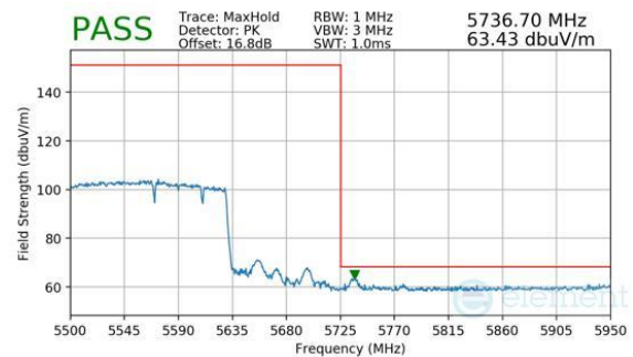
Plot 7-826. Antenna 2a (Peak, RU996+484+242, Index 99 (H), Ch.114 (FCC ONLY), MCS11)
