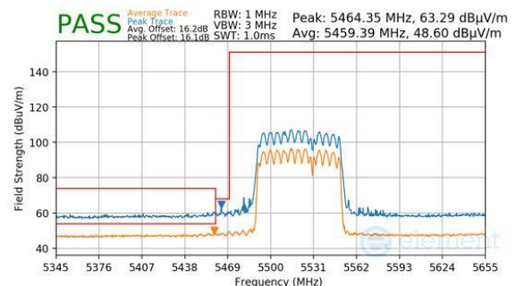
Plot 7-918. CDD Primary (Peak & Average, RU484+242, Index 93, Ch.106, MCS11)
