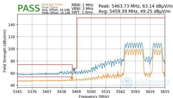
Plot 7-921. CDD Primary (Peak & Average, RU484+242, Index 92, Ch.122 (FCC ONLY), MCS11)
