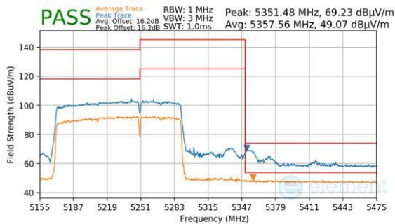
Plot 7-786. Antenna 2a (Peak & Average, RU996+484, Index 95 (H), Ch.50, MCS11)
