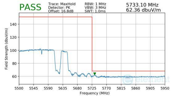
Plot 7-824. Antenna 2a (Peak, RU996+484+242, Index 98 (H), Ch.114 (FCC ONLY), MCS11)
