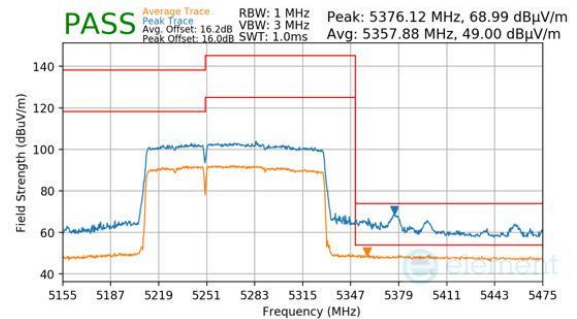
Plot 7-784. Antenna 2a (Peak & Average, RU996+484, Index 94 (L), Ch.50, MCS11)
