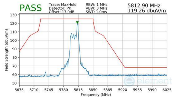
Plot 7-900. CDD Primary (Peak, RU26, Index 36, Ch.155, MCS11)
