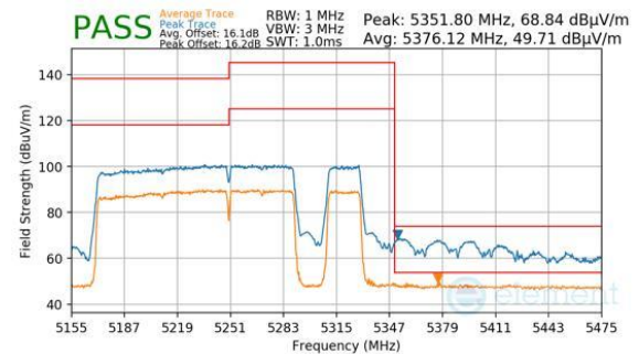
Plot 7-808. Antenna 2a (Peak & Average, RU996+484+242, Index 98 (H), Ch.50, MCS11)
