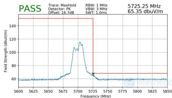
Plot 7-854. CDD Primary (Peak, RU52+26, Index 72, Ch.140, MCS11)
