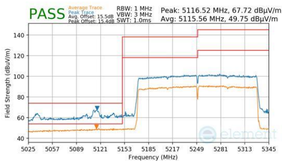
Plot 7-827. Antenna 2a (Peak & Average, RU996X2, Index 68, Ch.50, MCS11)
