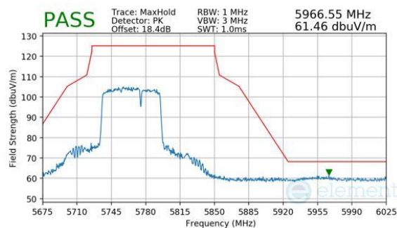
Plot 7-763. Antenna 2a (Peak, RU484+242, Index 93, Ch.155, MCS11)
