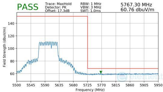
Plot 7-926. CDD Primary (Peak, RU484+242, Index 93, Ch.122 (FCC ONLY), MCS11)
