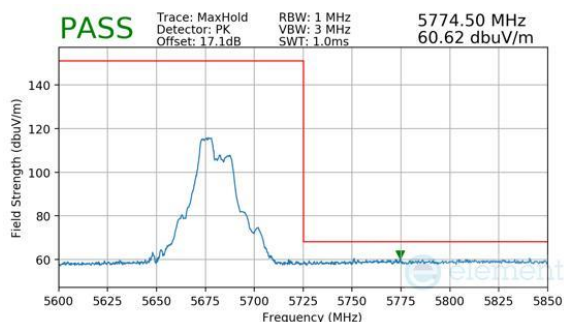
Plot 7-851. CDD Primary (Peak, RU52+26, Index 70, Ch.136, MCS11)
