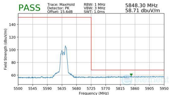
Plot 7-906. CDD Primary (Peak, RU52, Index 52, Ch.122 (FCC ONLY), MCS11)
