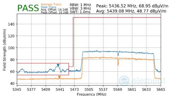
Plot 7-829. Antenna 2a (Peak & Average, RU996X2, Index 68, Ch.114 FCC ONLY, MCS11)
