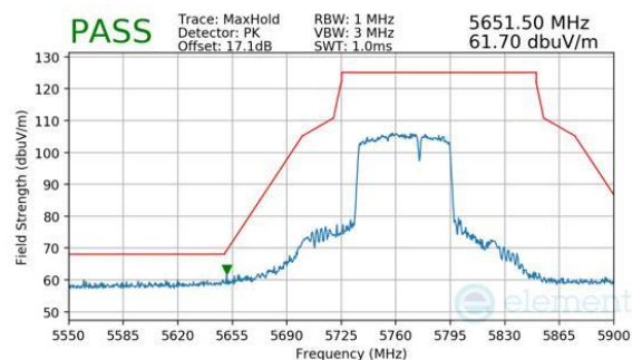
Plot 7-759. Antenna 2a (Peak, RU484+242, Index 93, Ch.155, MCS11)
