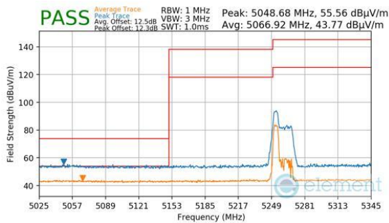
Plot 7-771. Antenna 2a (Peak & Average, RU52, Index 37, Ch.50, MCS11)
