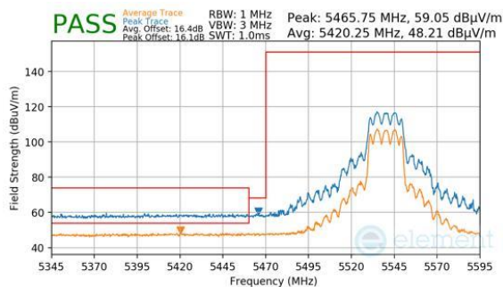
Plot 7-865. CDD Primary (Peak & Average, RU242, Index 61, Ch.108, MCS11)
