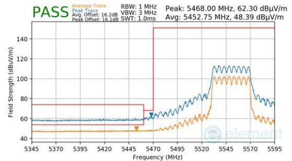
Plot 7-889. CDD Primary (Peak & Average, RU484, Index 65, Ch.110, MCS11)
