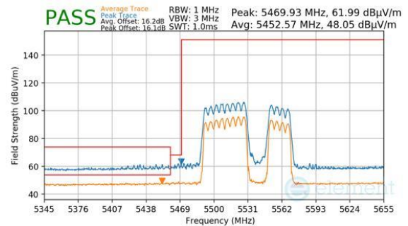
Plot 7-917. CDD Primary (Peak & Average, RU484+242, Index 92, Ch.106, MCS11)
