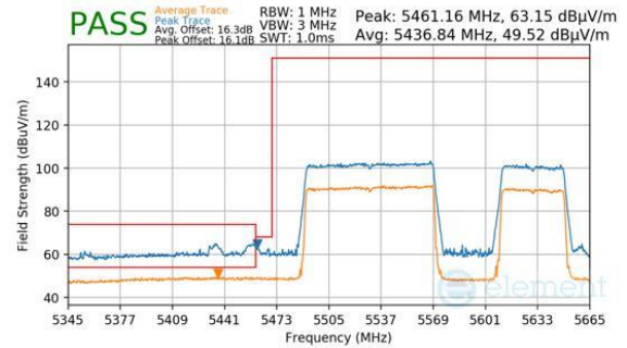
Plot 7-788. Antenna 2a (Peak & Average, RU996+484, Index 94 (H), Ch.114 (FCC ONLY), MCS11)
