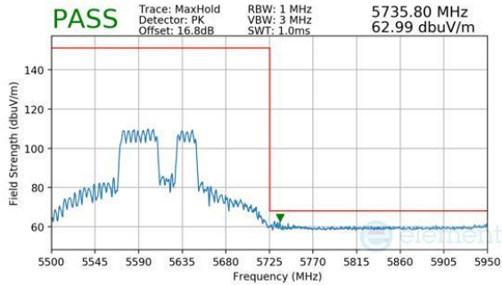
Plot 7-925. CDD Primary (Peak, RU484+242, Index 92, Ch.122 (FCC ONLY), MCS11)
