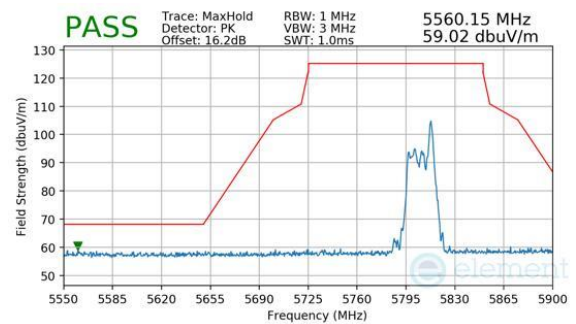
Plot 7-898. CDD Primary (Peak, RU26, Index 36, Ch.155, MCS11)
