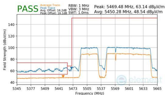
Plot 7-816. Antenna 2a (Peak & Average, RU996+484+242, Index 98 (L), Ch.114 (FCC ONLY), MCS11)
