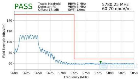
Plot 7-891. CDD Primary (Peak, RU484, Index 65, Ch.126 (FCC ONLY), MCS11)
