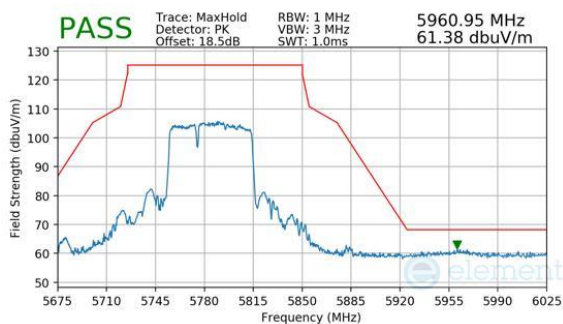
Plot 7-760. Antenna 2a (Peak, RU484+242, Index 90, Ch.155, MCS11)
