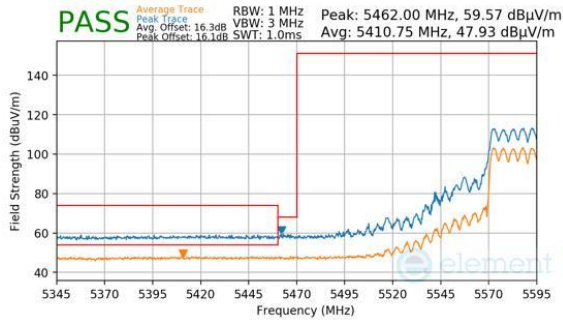
Plot 7-890. CDD Primary (Peak & Average, RU484, Index 65, Ch.118 (FCC ONLY), MCS11)
