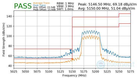
Plot 7-884. CDD Primary (Peak & Average, RU484, Index 65, Ch.38, MCS11)
