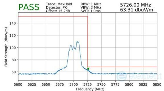
Plot 7-842. CDD Primary (Peak, RU52, Index 40, Ch.140, MCS11)
