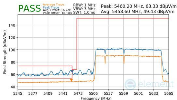
Plot 7-811. Antenna 2a (Peak & Average, RU996+484+242, Index 96 (L), Ch.114 (FCC ONLY), MCS11)
