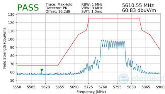
Plot 7-927. CDD Primary (Peak, RU484+242, Index 90, Ch.155, MCS11)
