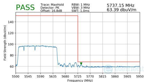
Plot 7-819. Antenna 2a (Peak, RU996+484+242, Index 96 (L), Ch.114 (FCC ONLY), MCS11)
