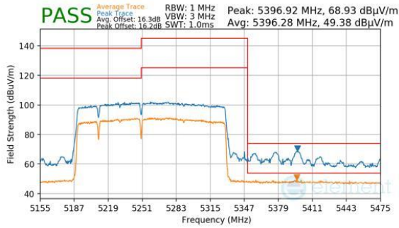
Plot 7-803. Antenna 2a (Peak & Average, RU996+484+242, Index 96 (L), Ch.50, MCS11)
