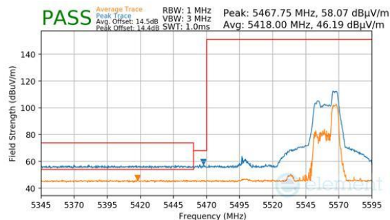
Plot 7-881. CDD Primary (Peak & Average, RU52, Index 44, Ch.110, MCS11)
