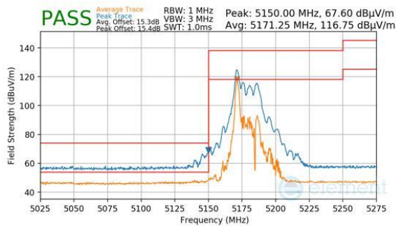
Plot 7-831. CDD Primary (Peak & Average, RU26, Index 0, Ch.36, MCS11)
