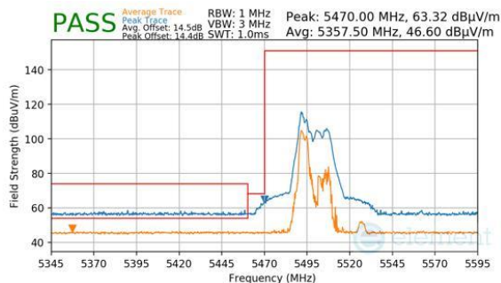
Plot 7-878. CDD Primary (Peak & Average, RU52, Index 37, Ch.102, MCS11)
