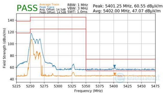
Plot 7-901. CDD Primary (Peak & Average, RU52, Index 37, Ch.58, MCS11)
