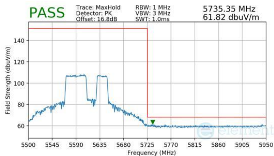
Plot 7-754. Antenna 2a (Peak, RU484+242, Index 92, Ch.122 (FCC ONLY), MCS11)
