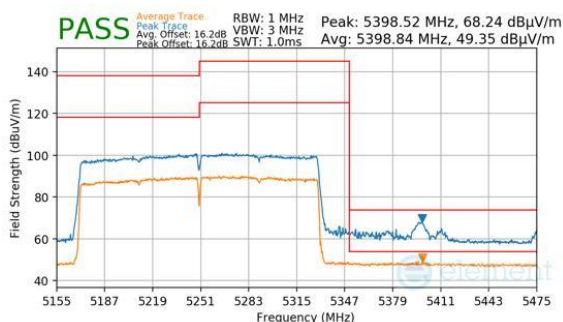
Plot 7-828. Antenna 2a (Peak & Average, RU996X2, Index 68, Ch.50, MCS11)
