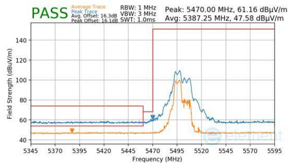
Plot 7-847. CDD Primary (Peak & Average, RU52+26, Index 70, Ch.100, MCS11)
