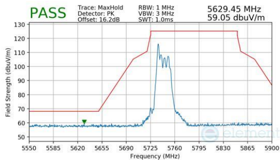
Plot 7-833. CDD Primary (Peak, RU26, Index 0, Ch.149, MCS11)
