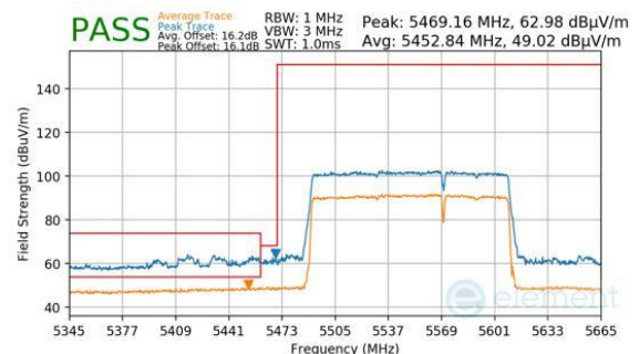
Plot 7-790. Antenna 2a (Peak & Average, RU996+484, Index 95 (H), Ch.114 (FCC ONLY), MCS11)
