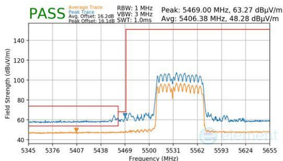
Plot 7-915. CDD Primary (Peak & Average, RU484+242, Index 90, Ch.106, MCS11)
