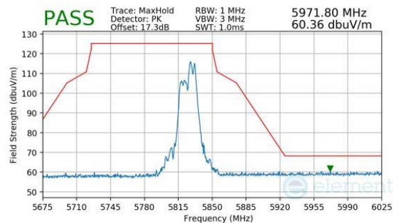
Plot 7-858. CDD Primary (Peak, RU52+26, Index 72, Ch.165, MCS11)
