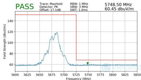
Plot 7-852. CDD Primary (Peak, RU52+26, Index 72, Ch.136, MCS11)
