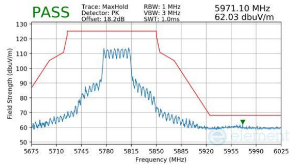
Plot 7-894. CDD Primary (Peak, RU484, Index 65, Ch.159, MCS11)
