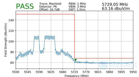
Plot 7-924. CDD Primary (Peak, RU484+242, Index 91, Ch.122 (FCC ONLY), MCS11)
