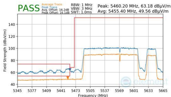
Plot 7-815. Antenna 2a (Peak & Average, RU996+484+242, Index 98 (H), Ch.114 (FCC ONLY), MCS11)
