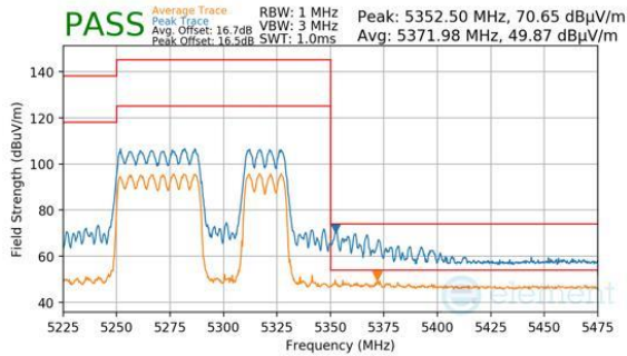
Plot 7-913. CDD Primary (Peak & Average, RU484+242, Index 92, Ch.58, MCS11)
