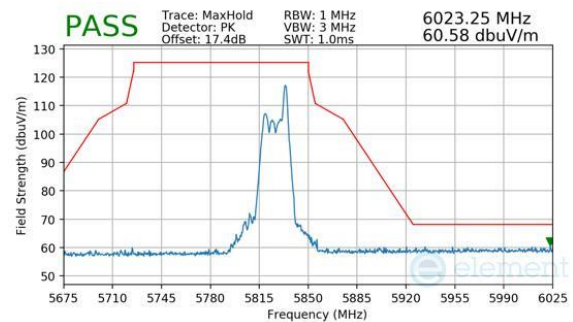
Plot 7-836. CDD Primary (Peak, RU26, Index 8, Ch.165, MCS11)
