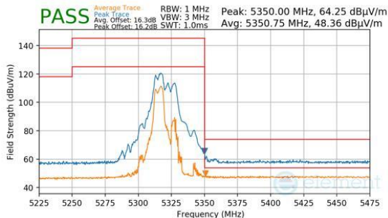
Plot 7-845. CDD Primary (Peak & Average, RU52+26, Index 70, Ch.64, MCS11)
