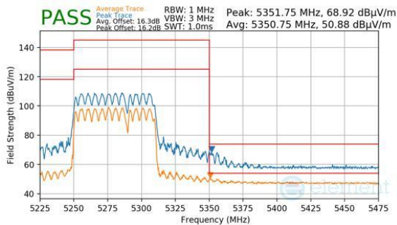
Plot 7-914. CDD Primary (Peak & Average, RU484+242, Index 93, Ch.58, MCS11)
