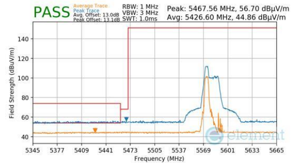
Plot 7-775. Antenna 2a (Peak & Average, RU52, Index 37, Ch.114 (FCC ONLY), MCS11)
