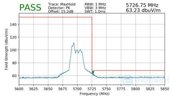
Plot 7-841. CDD Primary (Peak, RU52, Index 37, Ch.140, MCS11)
