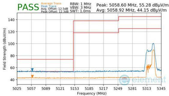
Plot 7-772. Antenna 2a (Peak & Average, RU52, Index 52 (H), Ch.50, MCS11)
