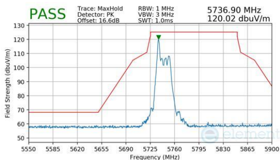
Plot 7-872. CDD Primary (Peak, RU26, Index 0, Ch.151, MCS11)
