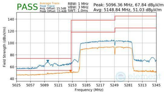
Plot 7-781. Antenna 2a (Peak & Average, RU996+484, Index 95 (H), Ch.50, MCS11)
