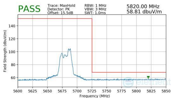
Plot 7-883. CDD Primary (Peak, RU52, Index 44, Ch.134, MCS11)
