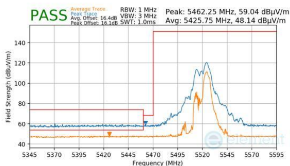
Plot 7-850. CDD Primary (Peak & Average, RU52+26, Index 72, Ch.104, MCS11)
