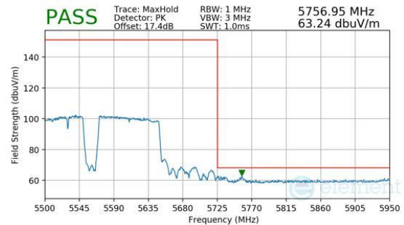
Plot 7-825. Antenna 2a (Peak, RU996+484+242, Index 99 (L), Ch.114 (FCC ONLY), MCS11)
