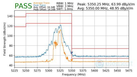
Plot 7-846. CDD Primary (Peak & Average, RU52+26, Index 72, Ch.64, MCS11)
