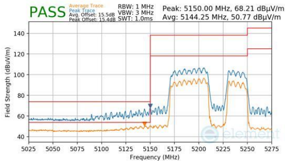
Plot 7-909. CDD Primary (Peak & Average, RU484+242, Index 92, Ch.42, MCS11)
