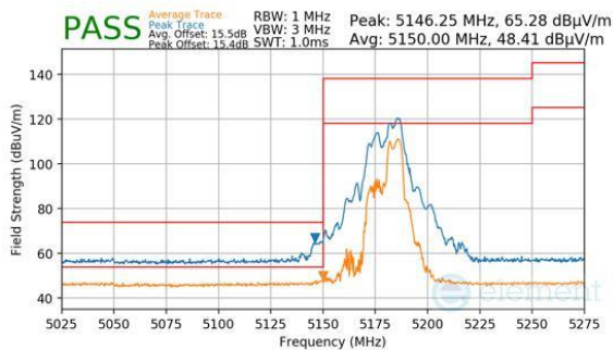
Plot 7-844. CDD Primary (Peak & Average, RU52+26, Index 72, Ch.36, MCS11)
