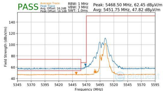
Plot 7-848. CDD Primary (Peak & Average, RU52+26, Index 72, Ch.100, MCS11)
