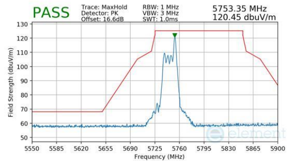
Plot 7-834. CDD Primary (Peak, RU26, Index 8, Ch.149, MCS11)
