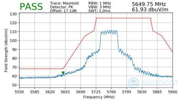
Plot 7-893. CDD Primary (Peak, RU484, Index 65, Ch.151, MCS11)
