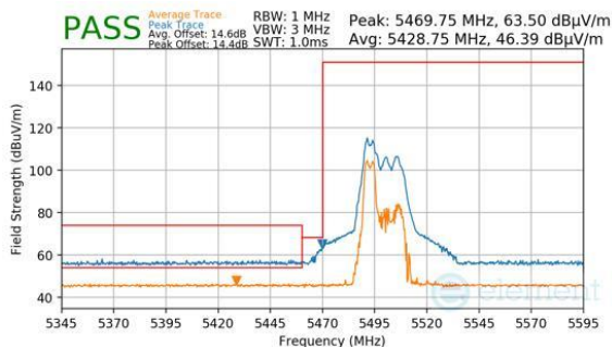
Plot 7-839. CDD Primary (Peak & Average, RU52, Index 37, Ch.100, MCS11)
