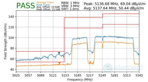
Plot 7-800. Antenna 2a (Peak & Average, RU996+484+242, Index 98 (L), Ch.50, MCS11)
