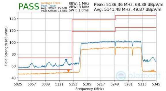
Plot 7-801. Antenna 2a (Peak & Average, RU996+484+242, Index 99 (H), Ch.50, MCS11)
