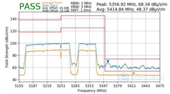
Plot 7-806. Antenna 2a (Peak & Average, RU996+484+242, Index 97 (H), Ch.50, MCS11)
