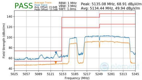
Plot 7-798. Antenna 2a (Peak & Average, RU996+484+242, Index 97 (L), Ch.50, MCS11)
