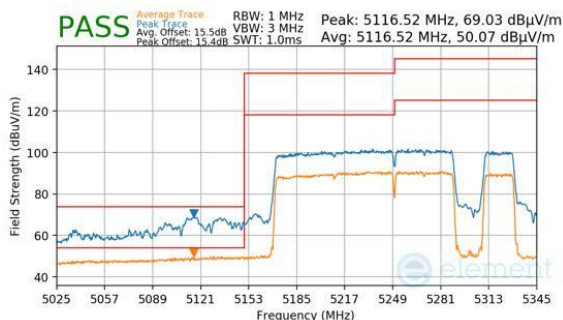
Plot 7-799. Antenna 2a (Peak & Average, RU996+484+242, Index 98 (H), Ch.50, MCS11)
