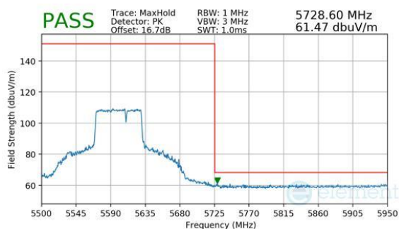
Plot 7-755. Antenna 2a (Peak, RU484+242, Index 93, Ch.122 (FCC ONLY), MCS11)
