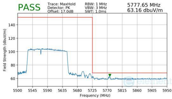
Plot 7-791. Antenna 2a (Peak, RU996+484, Index 94 (L), Ch.114 (FCC ONLY), MCS11)
