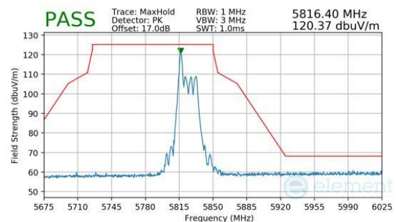
Plot 7-835. CDD Primary (Peak, RU26, Index 0, Ch.165, MCS11)
