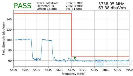
Plot 7-792. Antenna 2a (Peak, RU996+484, Index 94 (H), Ch.114 (FCC ONLY), MCS11)
