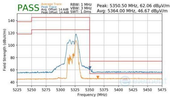
Plot 7-838. CDD Primary (Peak & Average, RU52, Index 40, Ch.64, MCS11)
