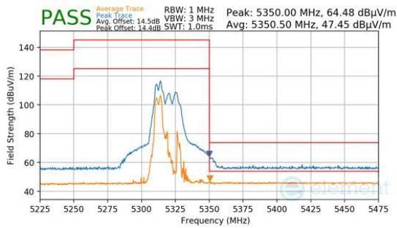
Plot 7-837. CDD Primary (Peak & Average, RU52, Index 37, Ch.64, MCS11)
