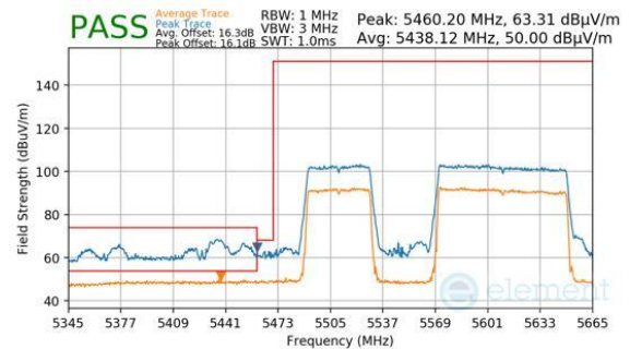
Plot 7-789. Antenna 2a (Peak & Average, RU996+484, Index 95 (L), Ch.114 (FCC ONLY), MCS11)
