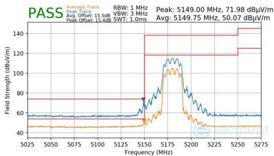
Plot 7-859. CDD Primary (Peak & Average, RU242, Index 61, Ch.36, MCS11)
