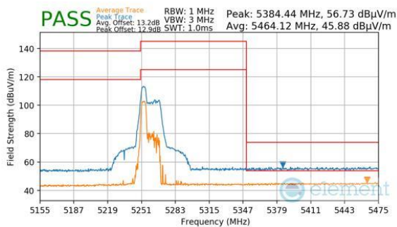
Plot 7-773. Antenna 2a (Peak & Average, RU52, Index 37, Ch.50, MCS11)
