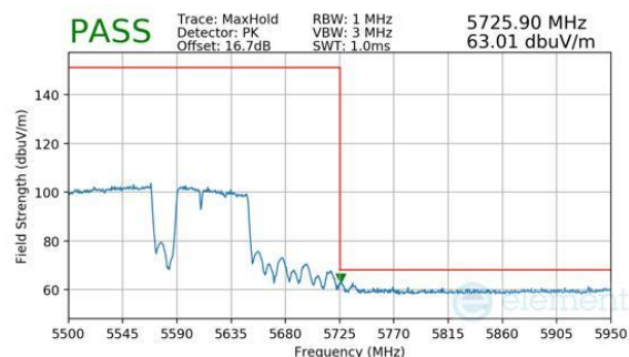
Plot 7-820. Antenna 2a (Peak, RU996+484+242, Index 96 (H), Ch.114 (FCC ONLY), MCS11)
