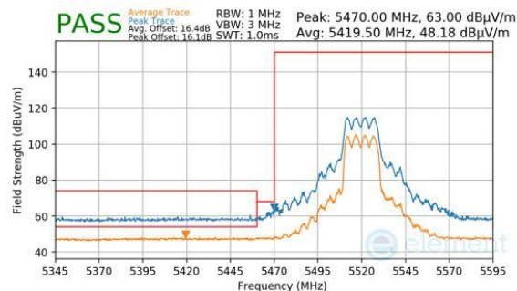
Plot 7-864. CDD Primary (Peak & Average, RU242, Index 61, Ch.104, MCS11)
